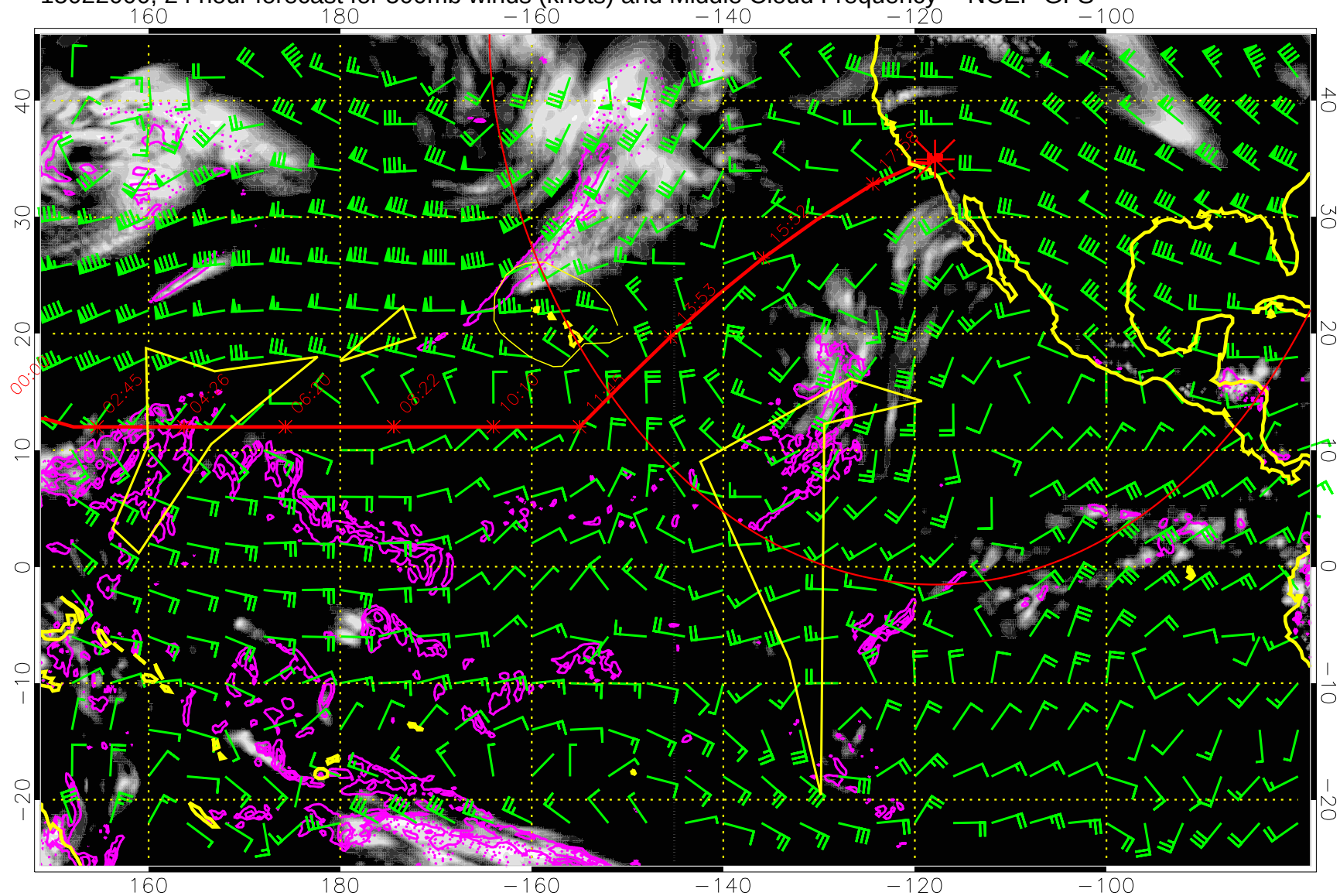
15022000, 24 hour forecast for 500mb winds (knots) and Middle Cloud Frequency -- NCEP GFS
