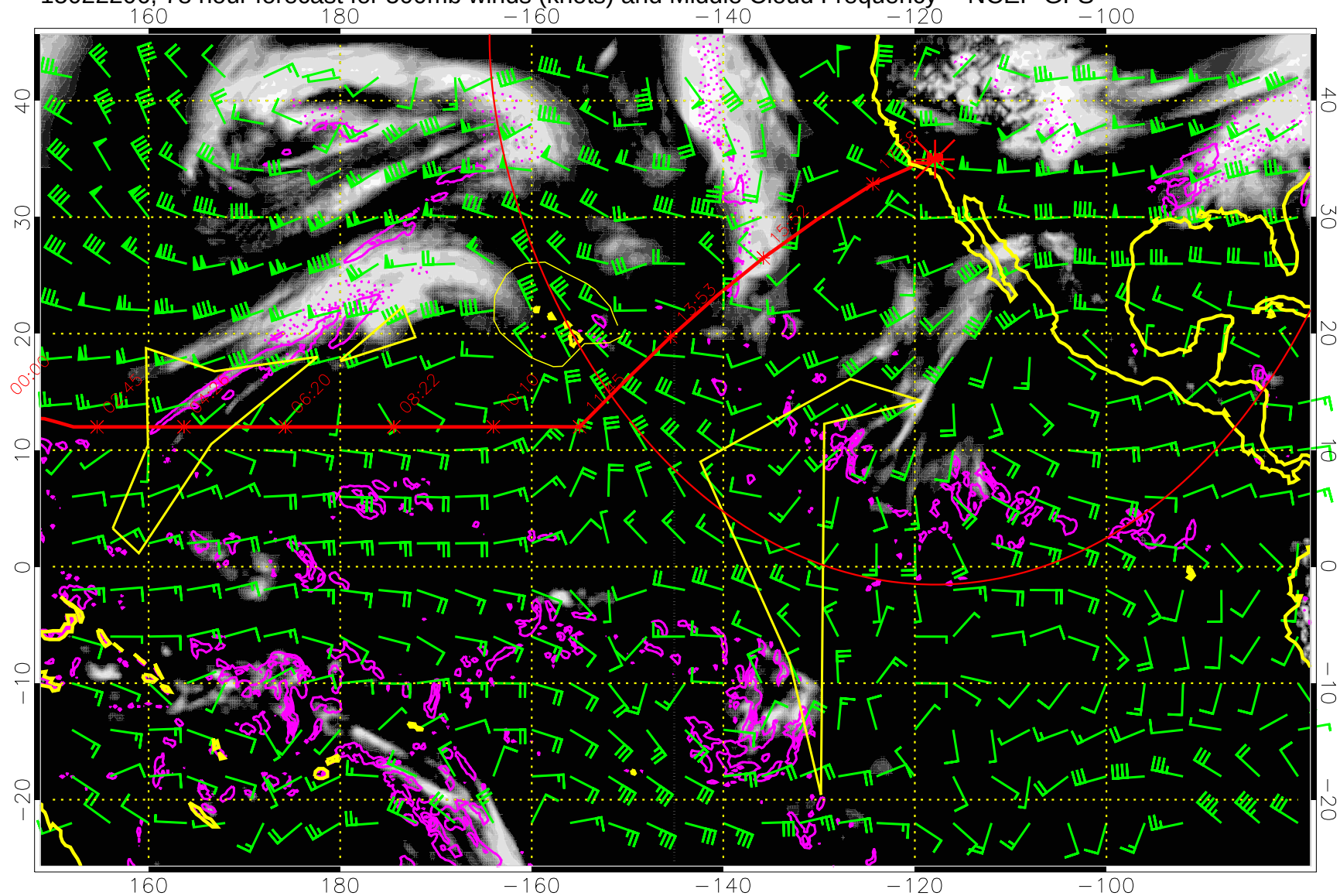
15022206, 78 hour forecast for 500mb winds (knots) and Middle Cloud Frequency -- NCEP GFS
