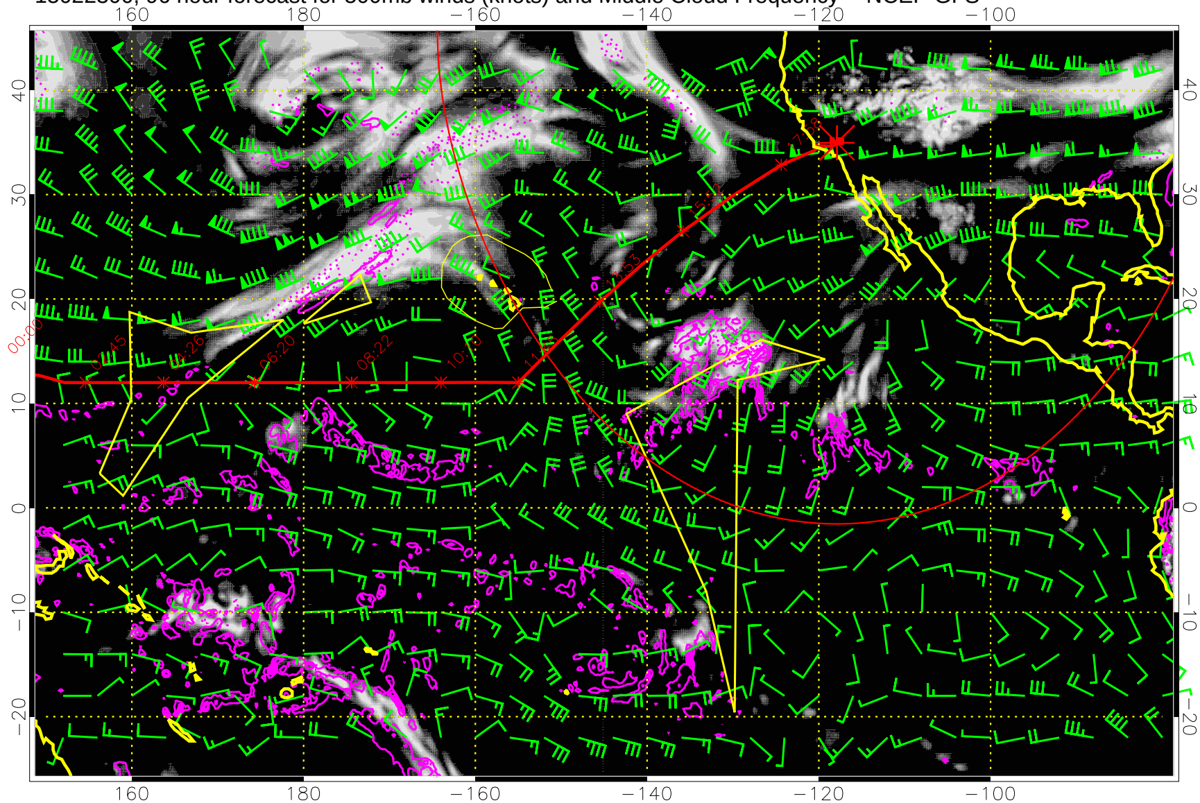
15022300, 96 hour forecast for 500mb winds (knots) and Middle Cloud Frequency -- NCEP GFS
