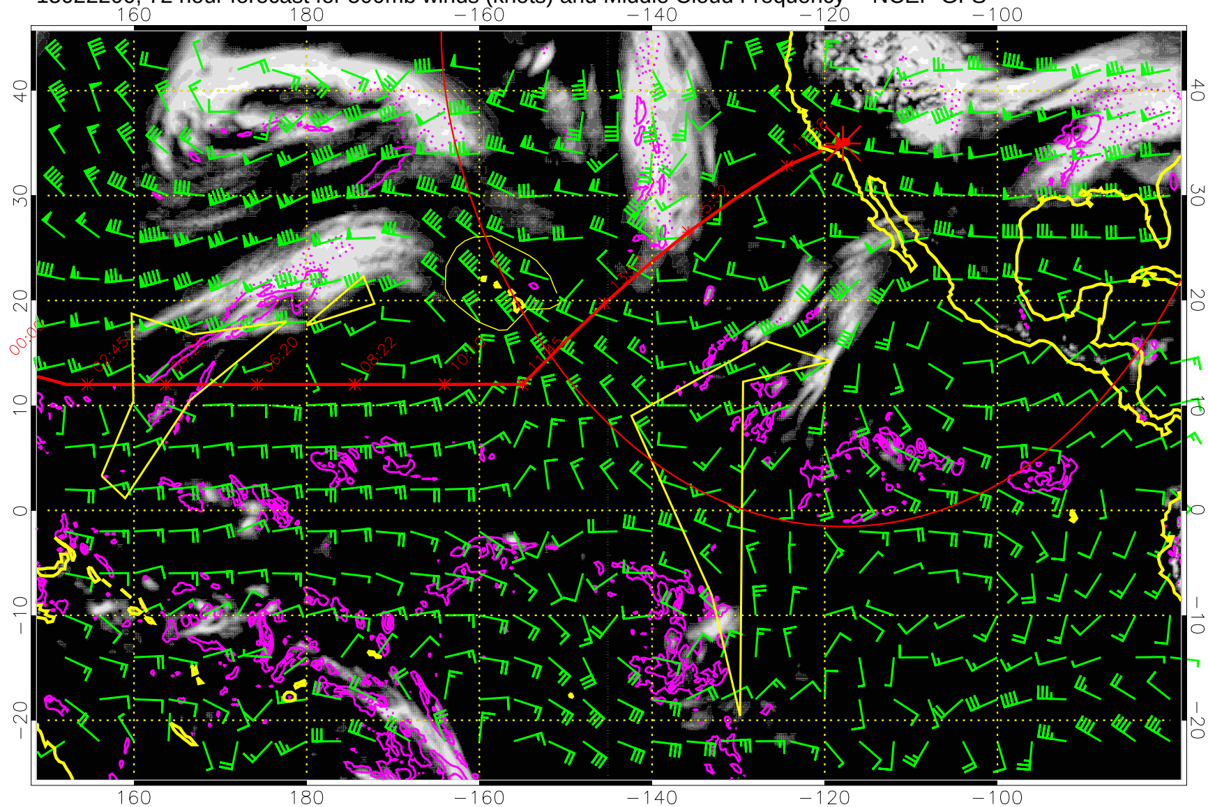
15022200, 72 hour forecast for 500mb winds (knots) and Middle Cloud Frequency -- NCEP GFS
