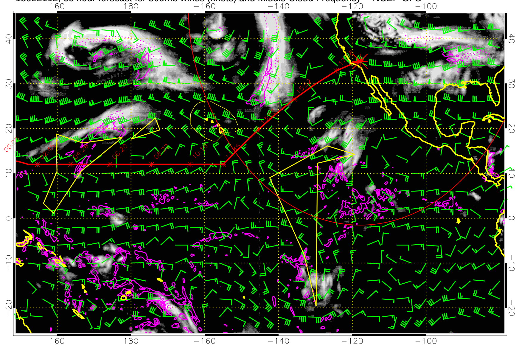
15022112, 60 hour forecast for 500mb winds (knots) and Middle Cloud Frequency -- NCEP GFS
