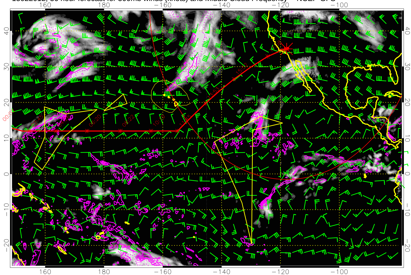
15022012, 36 hour forecast for 500mb winds (knots) and Middle Cloud Frequency -- NCEP GFS
