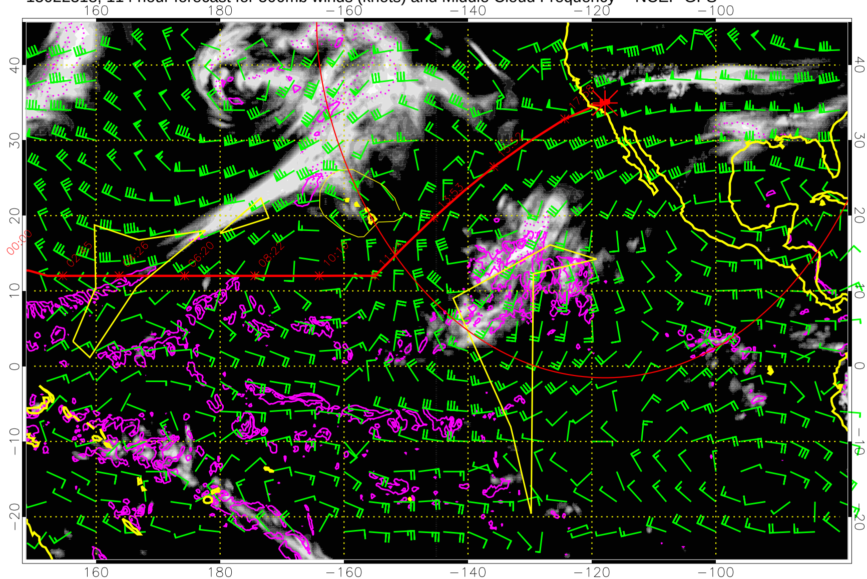
15022318, 114 hour forecast for 500mb winds (knots) and Middle Cloud Frequency -- NCEP GFS
