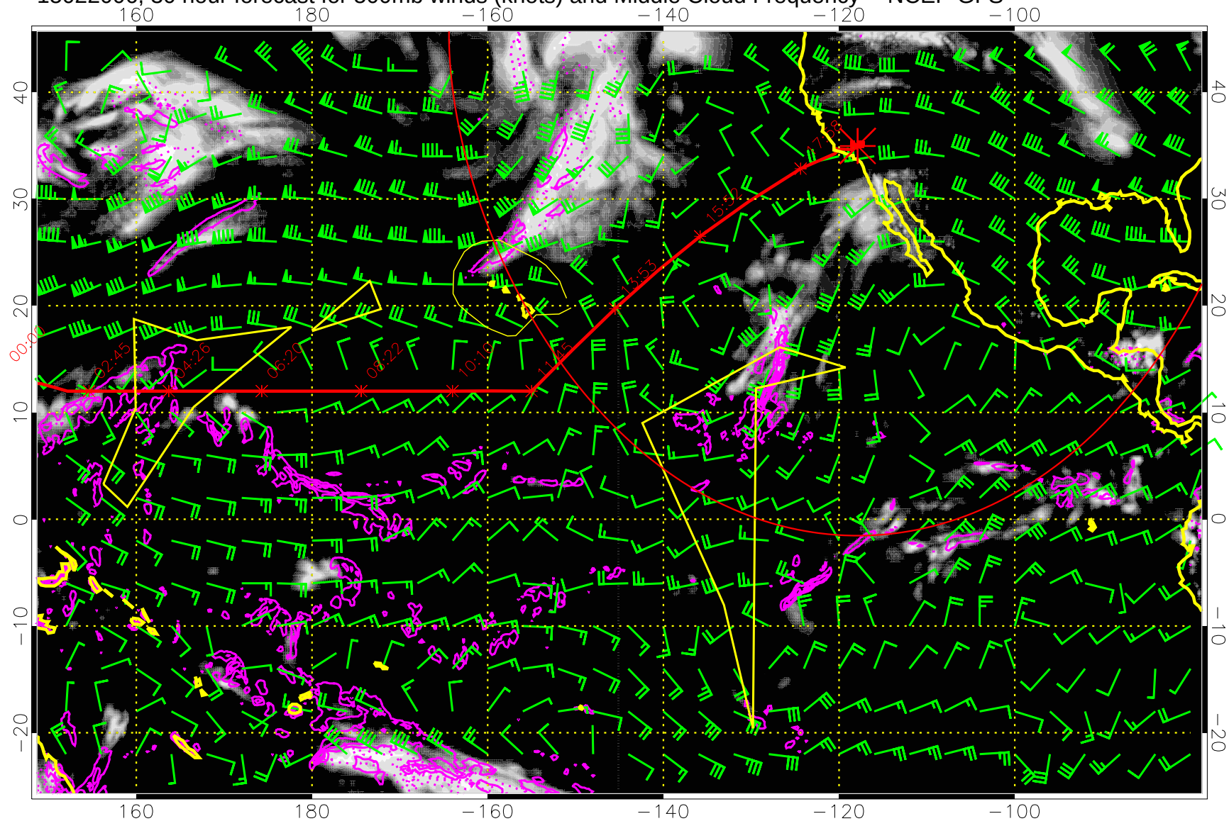
15022006, 30 hour forecast for 500mb winds (knots) and Middle Cloud Frequency -- NCEP GFS
