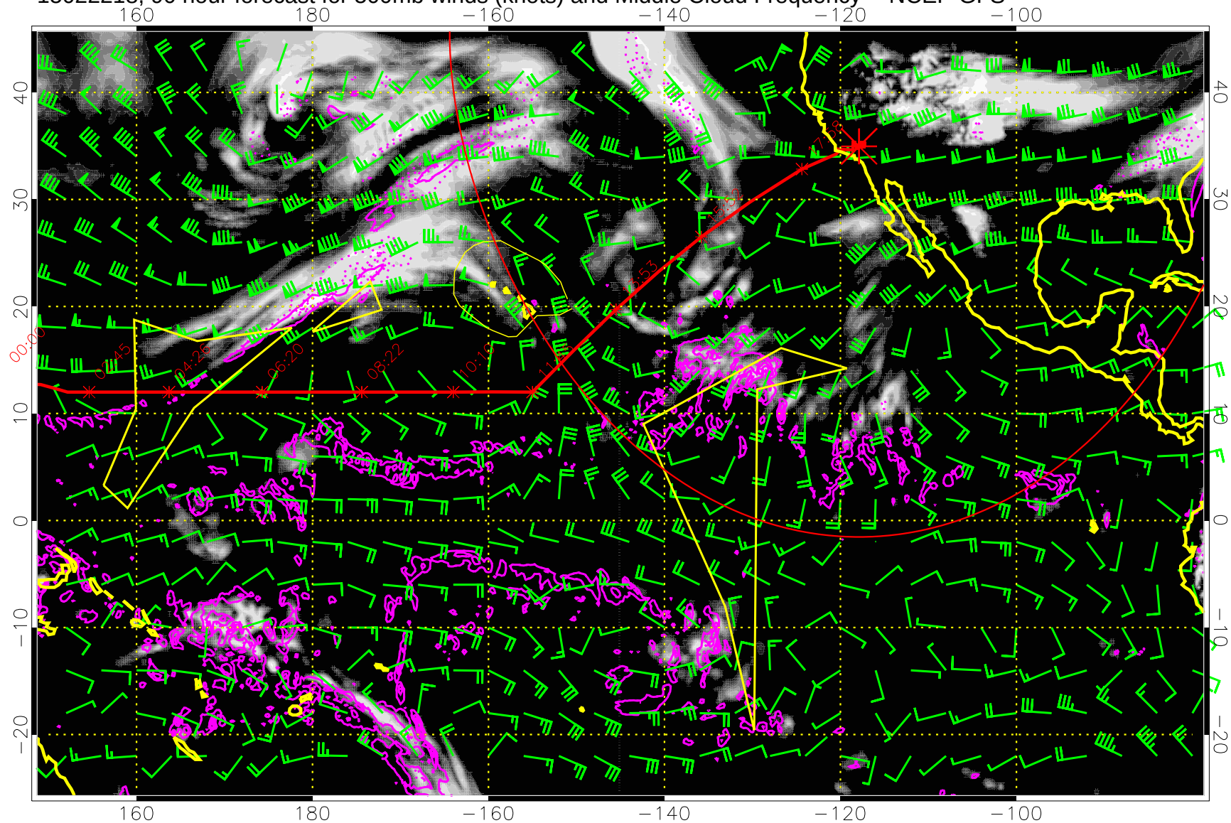
15022218, 90 hour forecast for 500mb winds (knots) and Middle Cloud Frequency -- NCEP GFS
