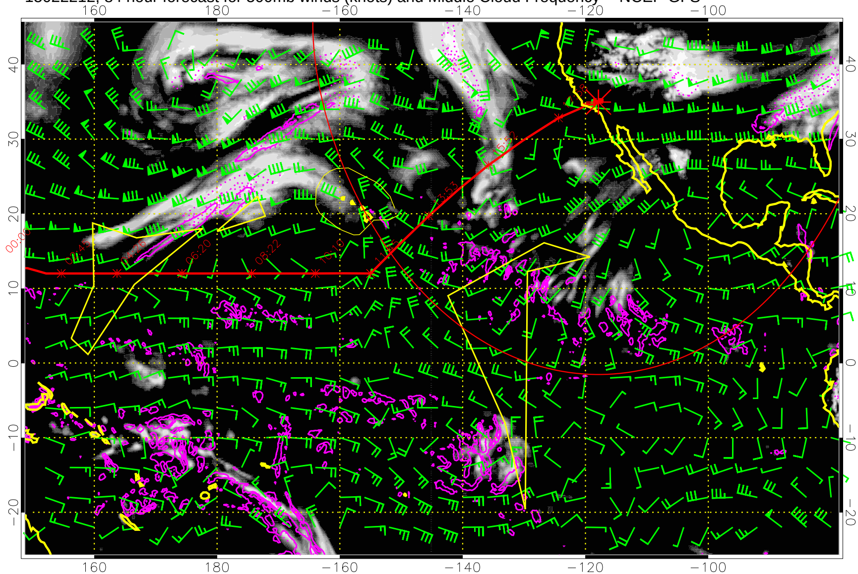
15022212, 84 hour forecast for 500mb winds (knots) and Middle Cloud Frequency -- NCEP GFS
