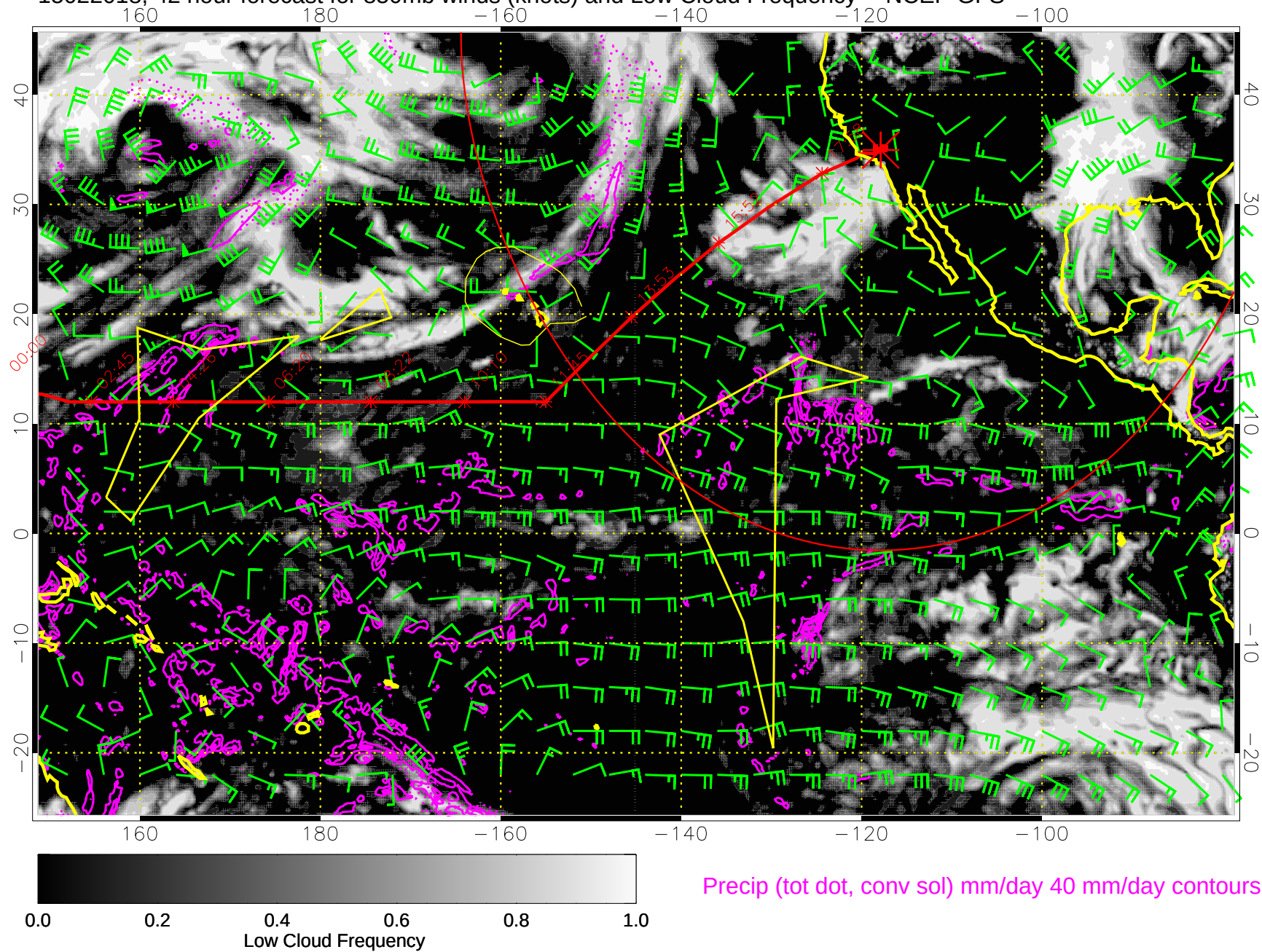
15022018, 42 hour forecast for 850mb winds (knots) and Low Cloud Frequency -- NCEP GFS
