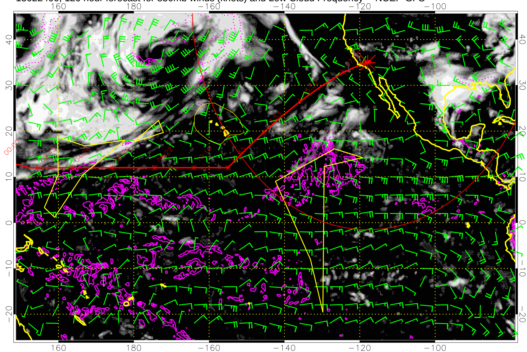
15022400, 120 hour forecast for 850mb winds (knots) and Low Cloud Frequency -- NCEP GFS
