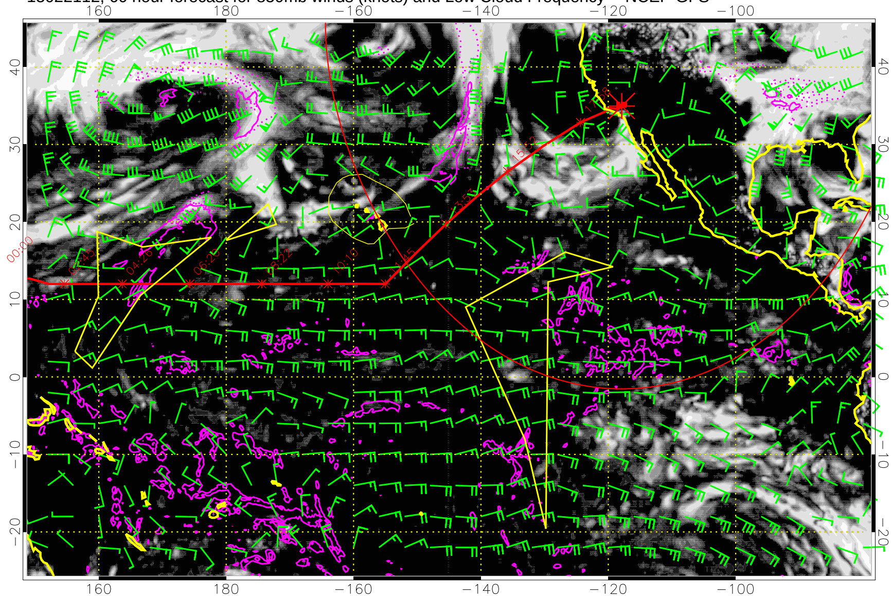
15022112, 60 hour forecast for 850mb winds (knots) and Low Cloud Frequency -- NCEP GFS
