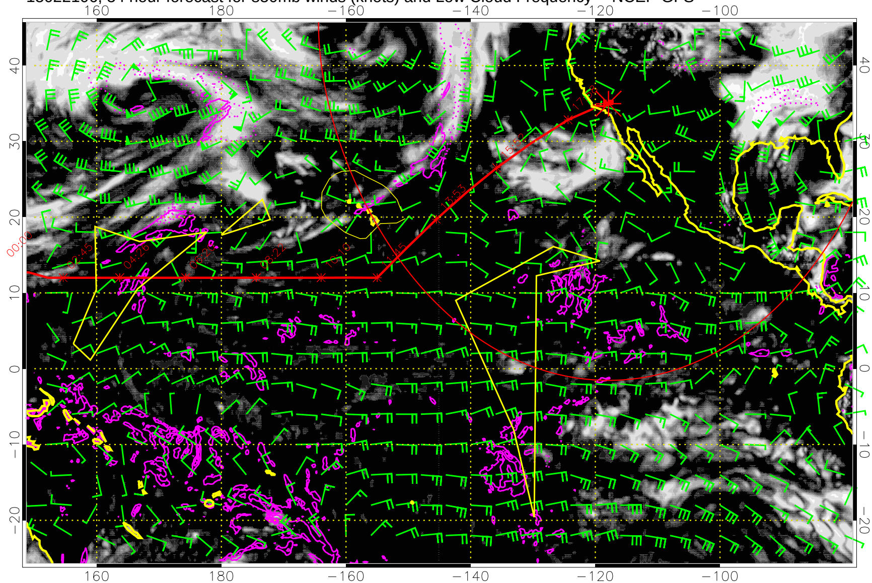
15022106, 54 hour forecast for 850mb winds (knots) and Low Cloud Frequency -- NCEP GFS
