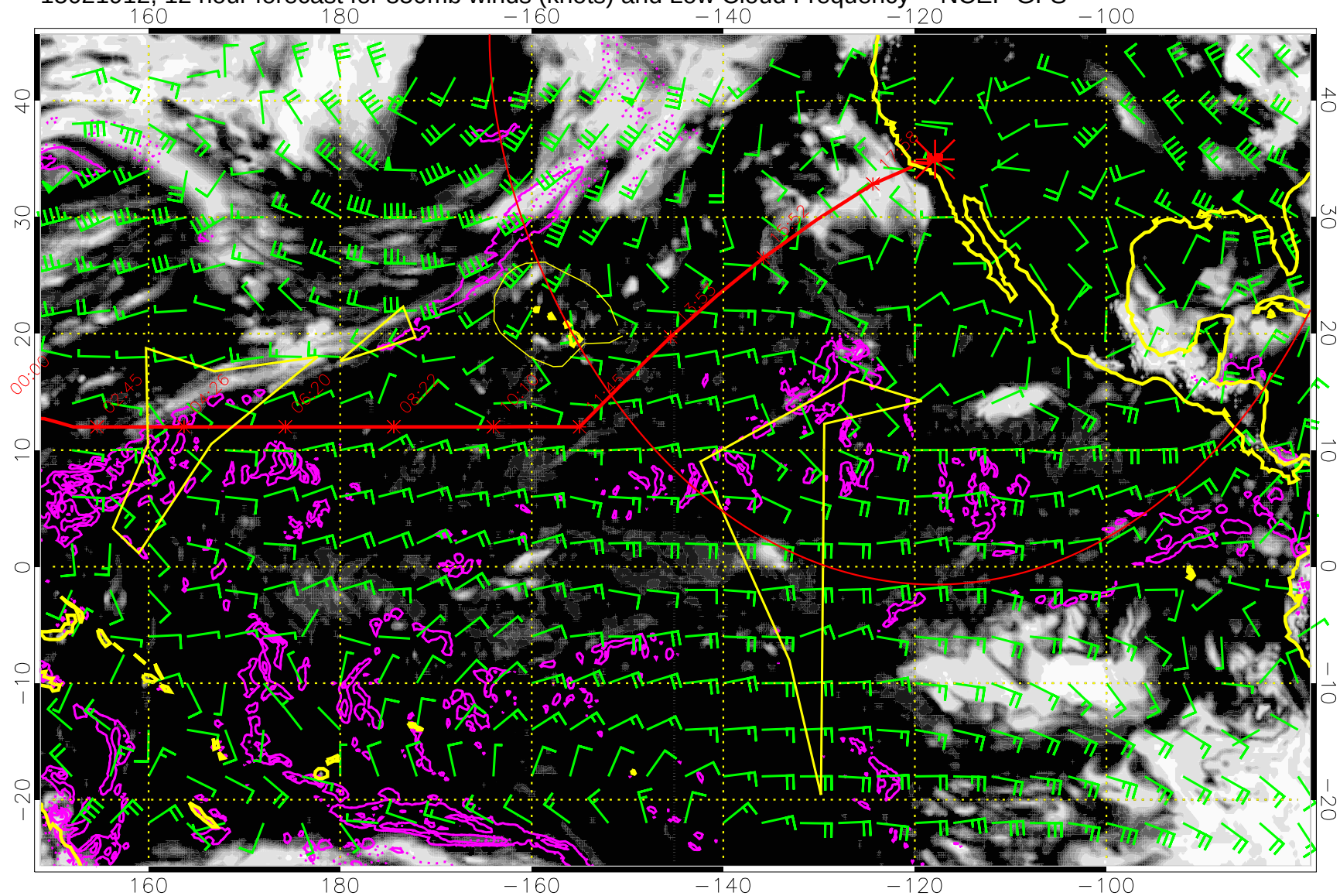
15021912, 12 hour forecast for 850mb winds (knots) and Low Cloud Frequency -- NCEP GFS
