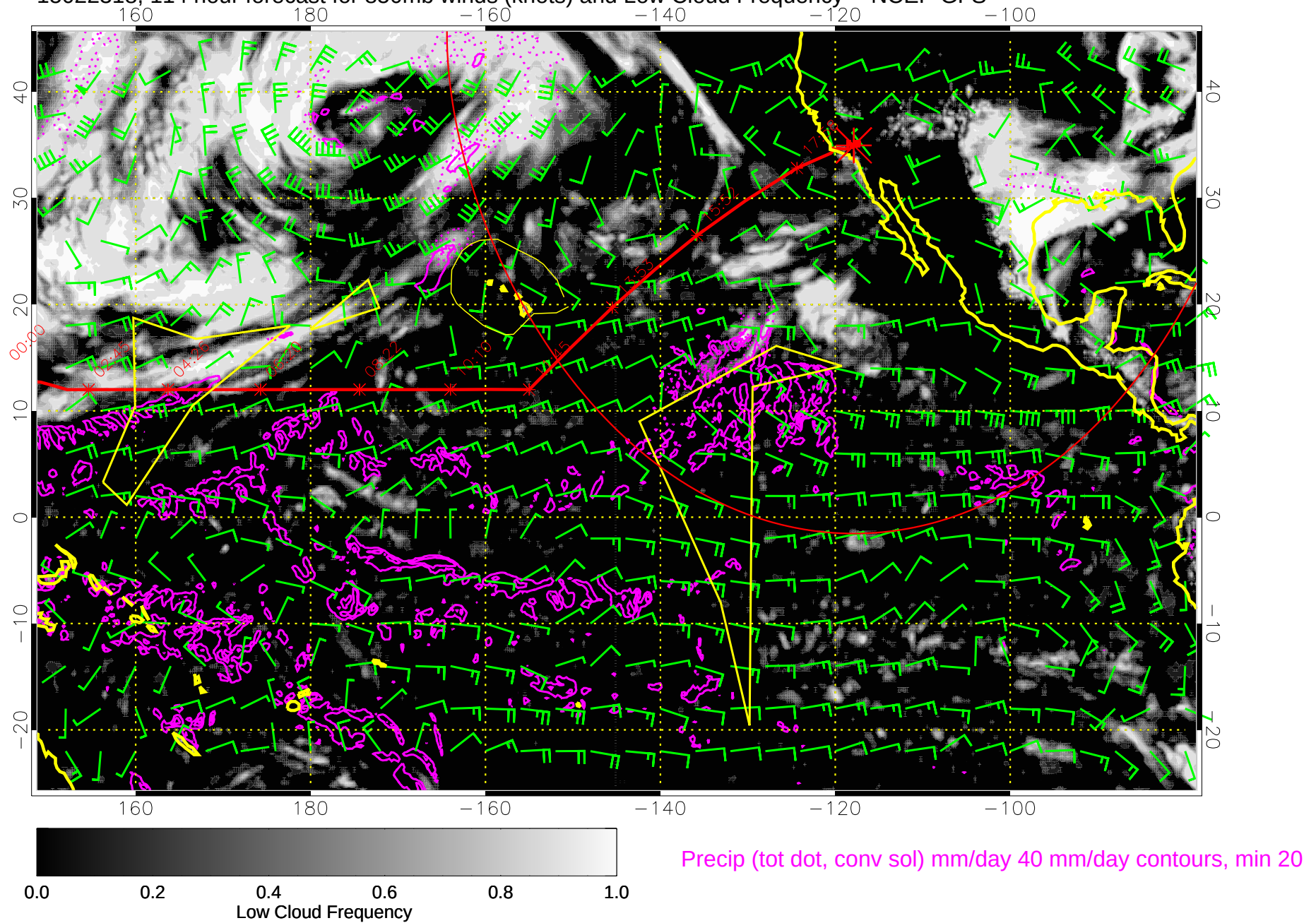
15022318, 114 hour forecast for 850mb winds (knots) and Low Cloud Frequency -- NCEP GFS
