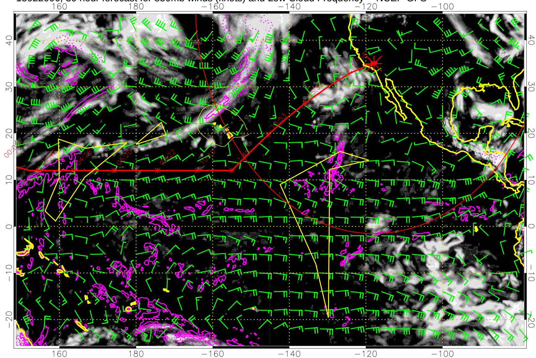
15022006, 30 hour forecast for 850mb winds (knots) and Low Cloud Frequency -- NCEP GFS
