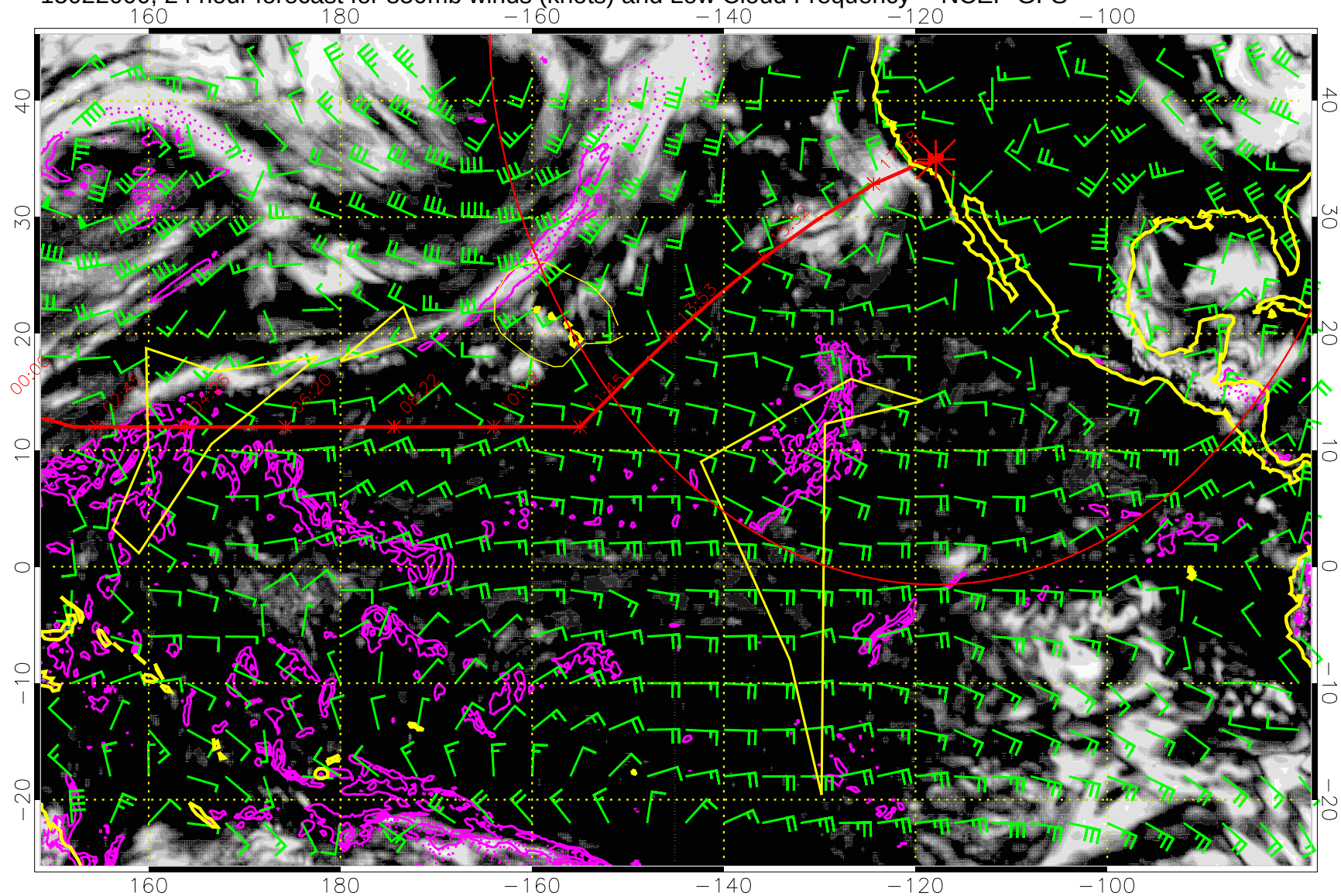
15022000, 24 hour forecast for 850mb winds (knots) and Low Cloud Frequency -- NCEP GFS
