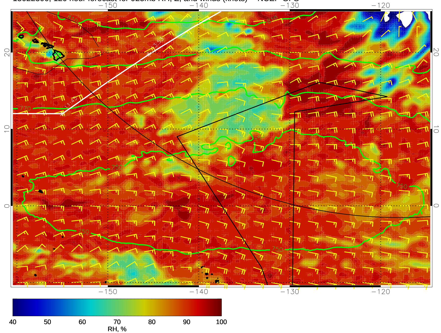
15022300, 120 hour forecast for 925mb RH, Z, and winds (knots) -- NCEP GFS
