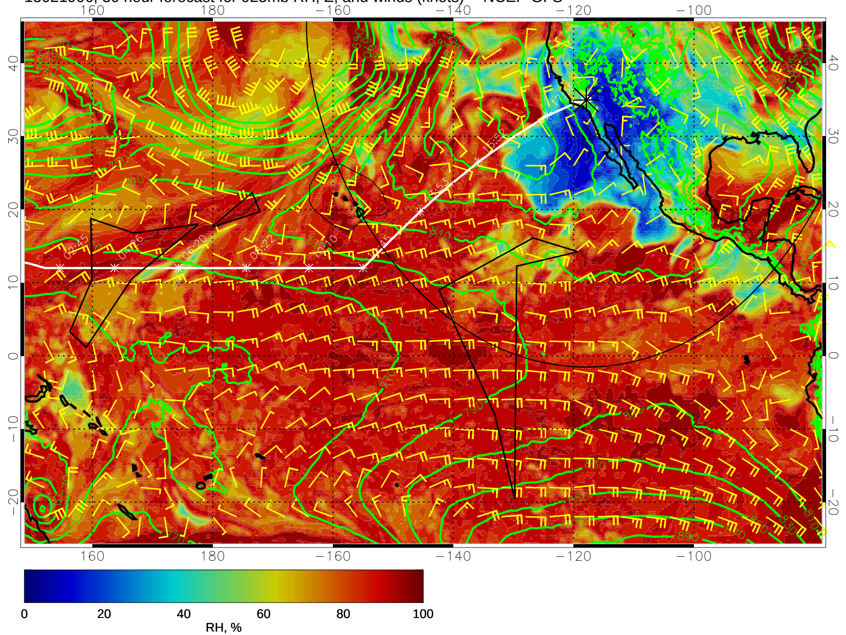
15021906, 30 hour forecast for 925mb RH, Z, and winds (knots) -- NCEP GFS
