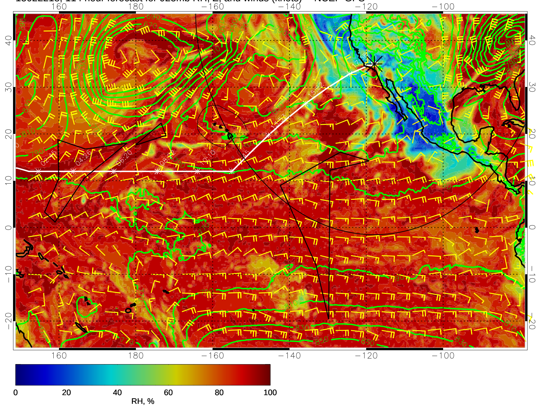
15022218, 114 hour forecast for 925mb RH, Z, and winds (knots) -- NCEP GFS
