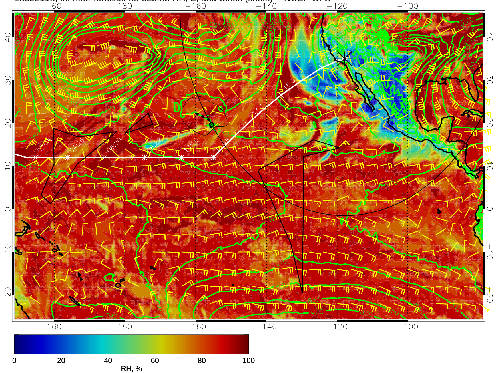
15022118, 90 hour forecast for 925mb RH, Z, and winds (knots) -- NCEP GFS
