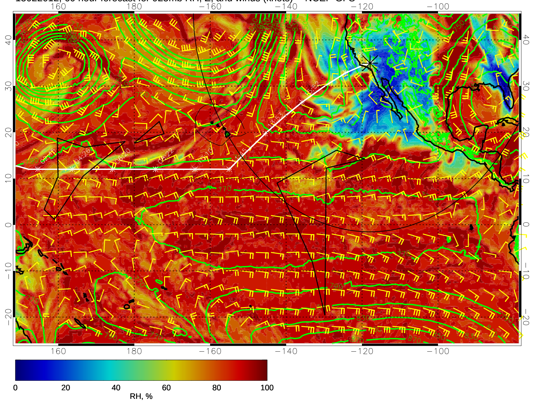
15022012, 60 hour forecast for 925mb RH, Z, and winds (knots) -- NCEP GFS
