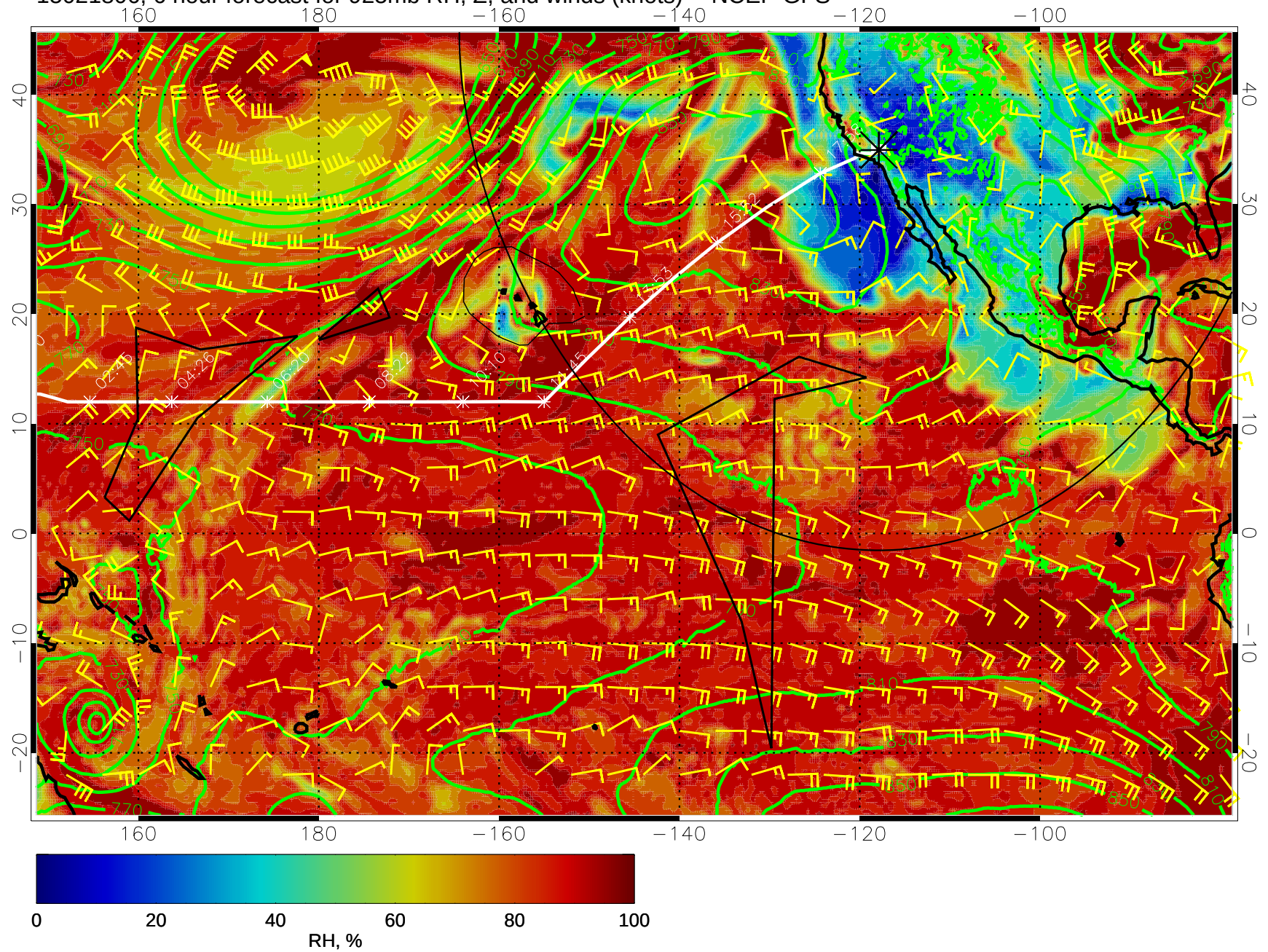
15021806, 6 hour forecast for 925mb RH, Z, and winds (knots) -- NCEP GFS
