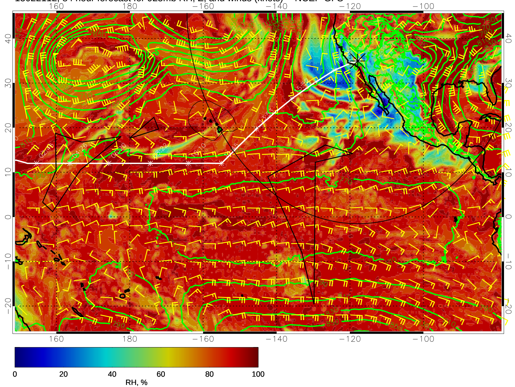
15022112, 84 hour forecast for 925mb RH, Z, and winds (knots) -- NCEP GFS
