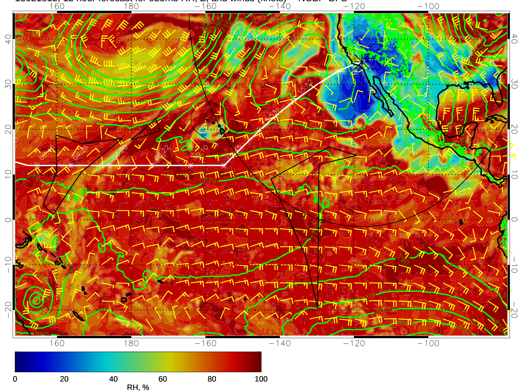
15021812, 12 hour forecast for 925mb RH, Z, and winds (knots) -- NCEP GFS
