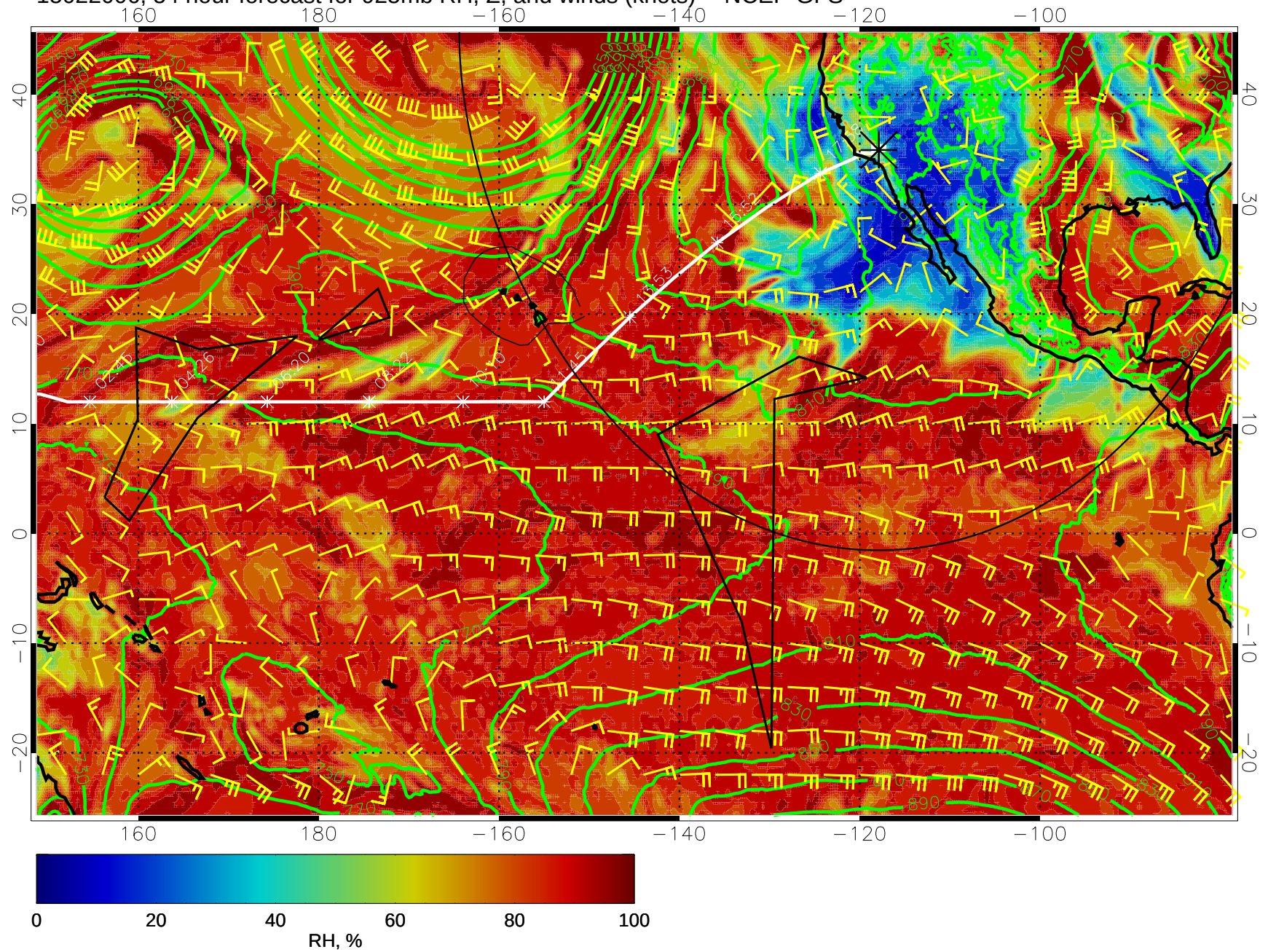
15022006, 54 hour forecast for 925mb RH, Z, and winds (knots) -- NCEP GFS
