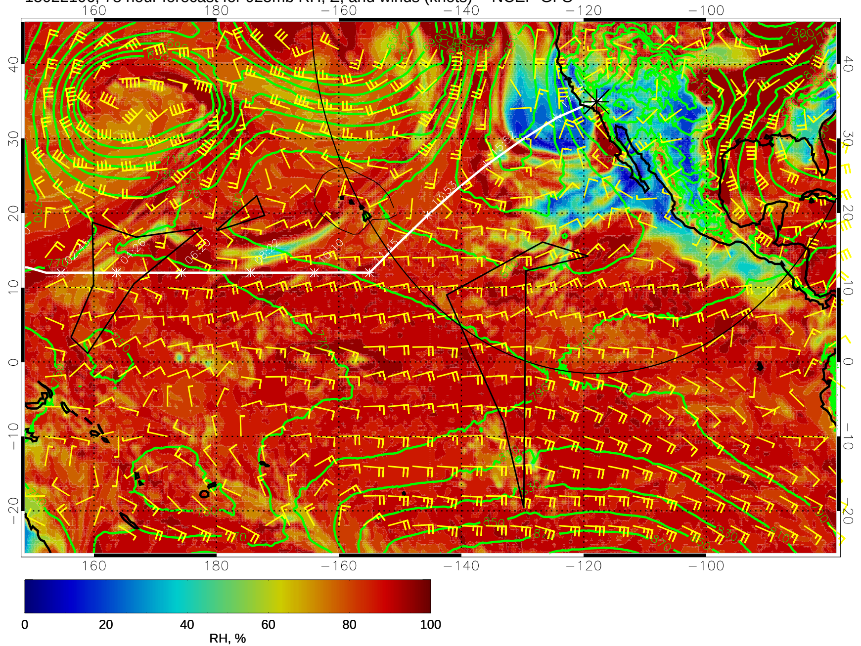
15022106, 78 hour forecast for 925mb RH, Z, and winds (knots) -- NCEP GFS
