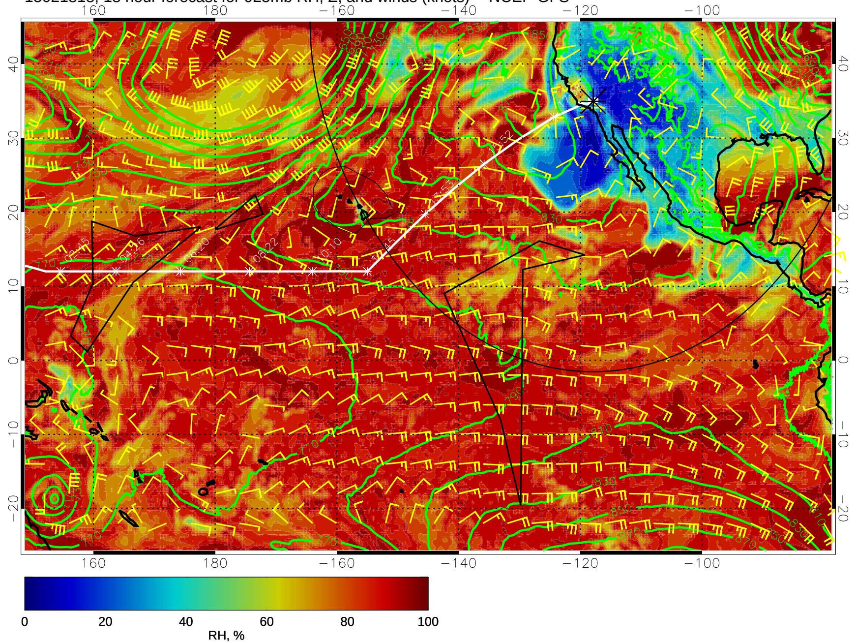
15021818, 18 hour forecast for 925mb RH, Z, and winds (knots) -- NCEP GFS
