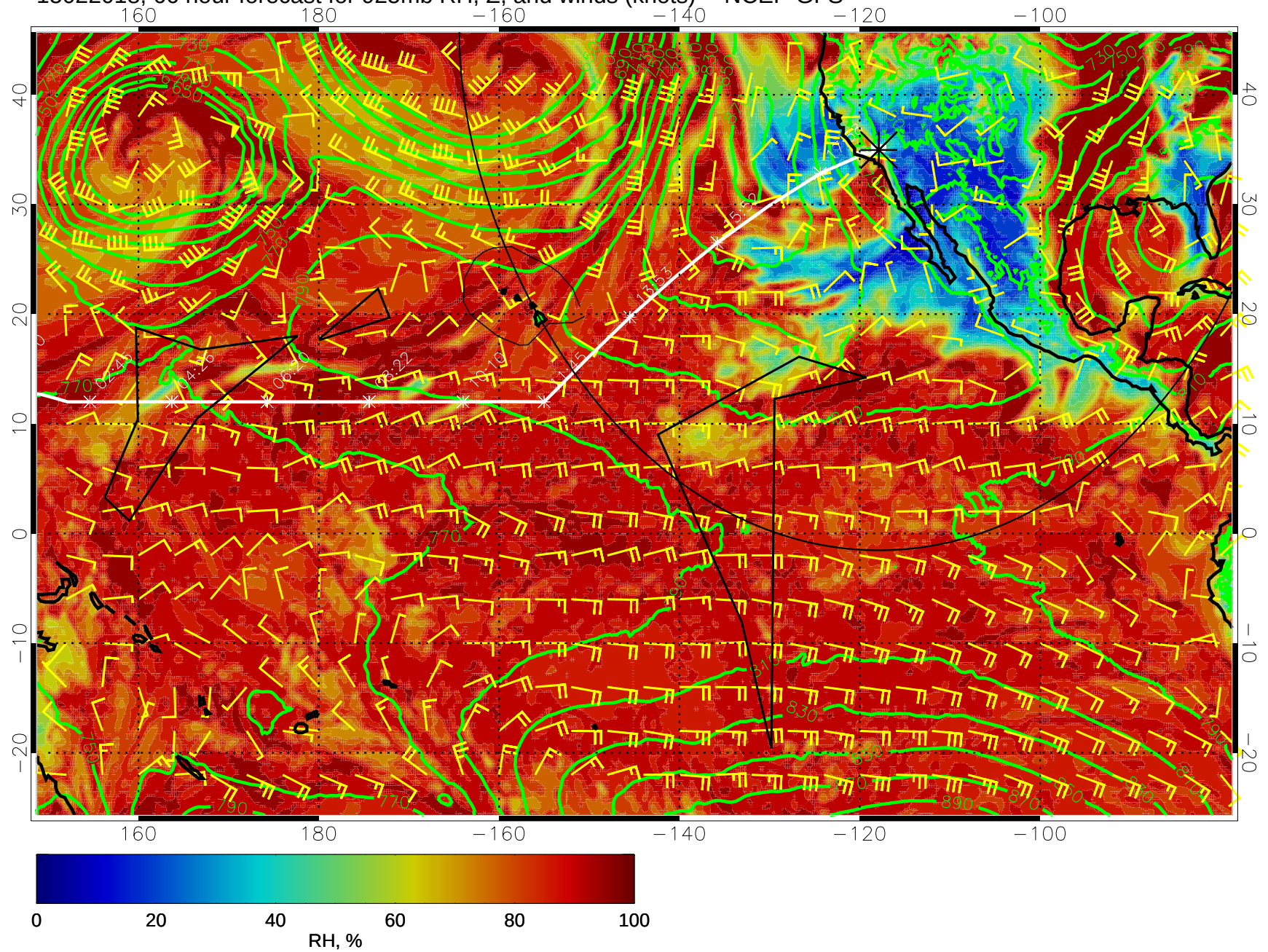
15022018, 66 hour forecast for 925mb RH, Z, and winds (knots) -- NCEP GFS
