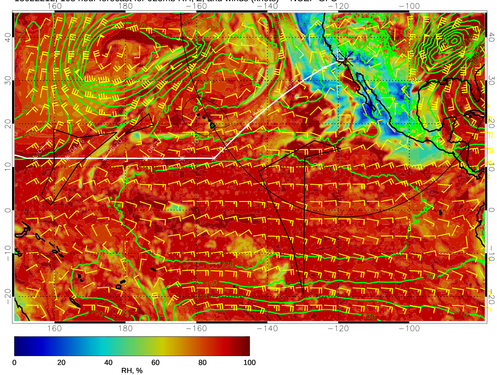
15022212, 108 hour forecast for 925mb RH, Z, and winds (knots) -- NCEP GFS
