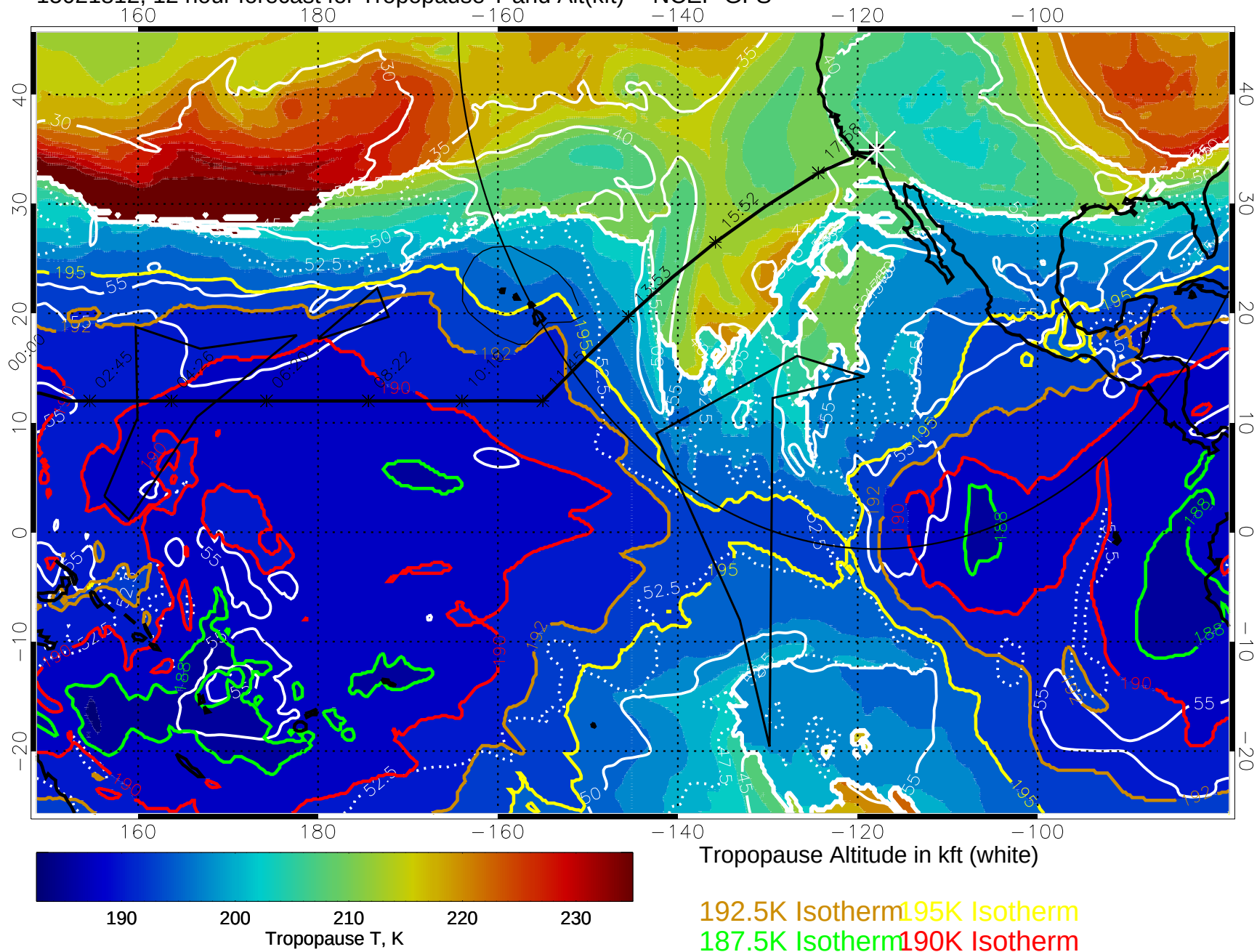
15021812, 12 hour forecast for Tropopause T and Alt(kft) -- NCEP GFS
