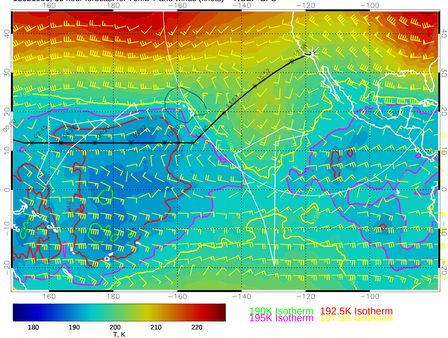
15021906, 30 hour forecast for 70mb T and winds (knots) -- NCEP GFS
