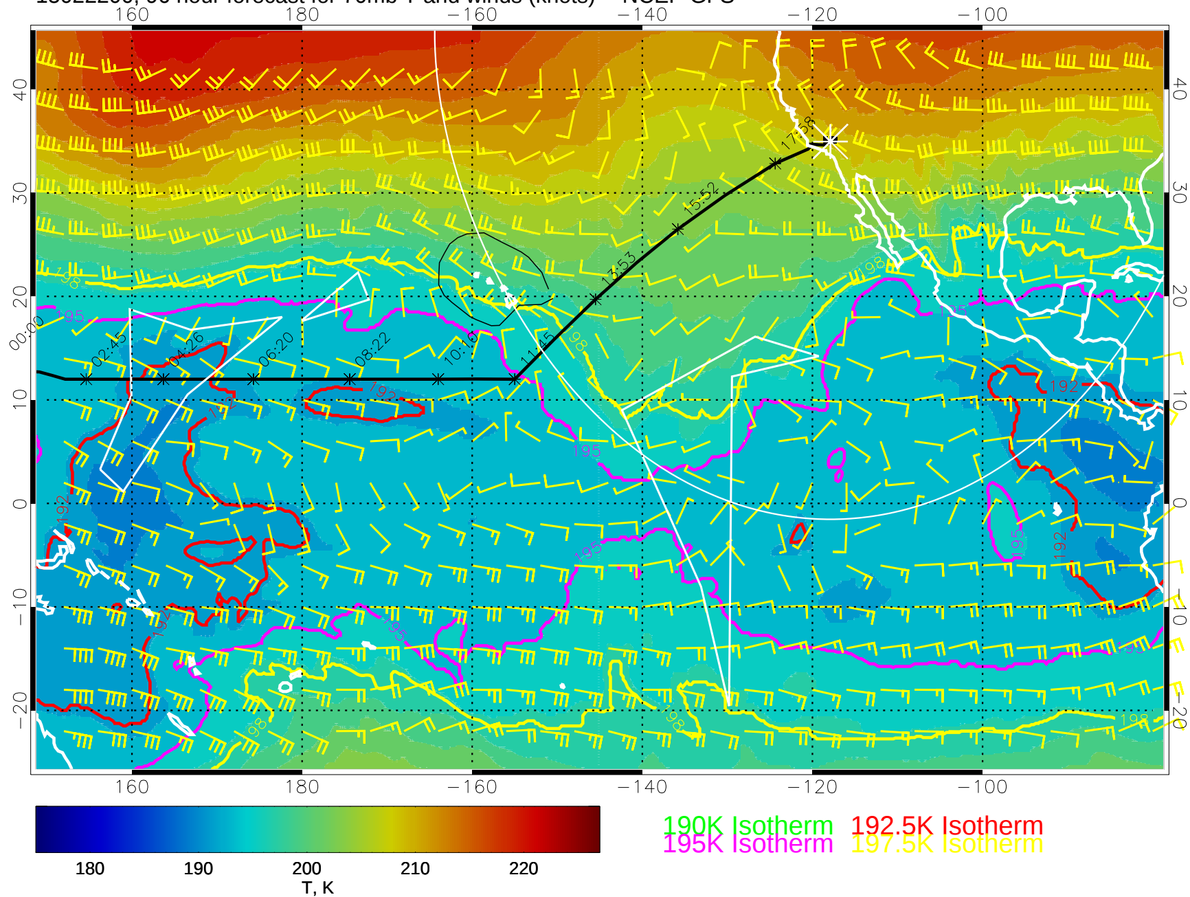
15022200, 96 hour forecast for 70mb T and winds (knots) -- NCEP GFS
