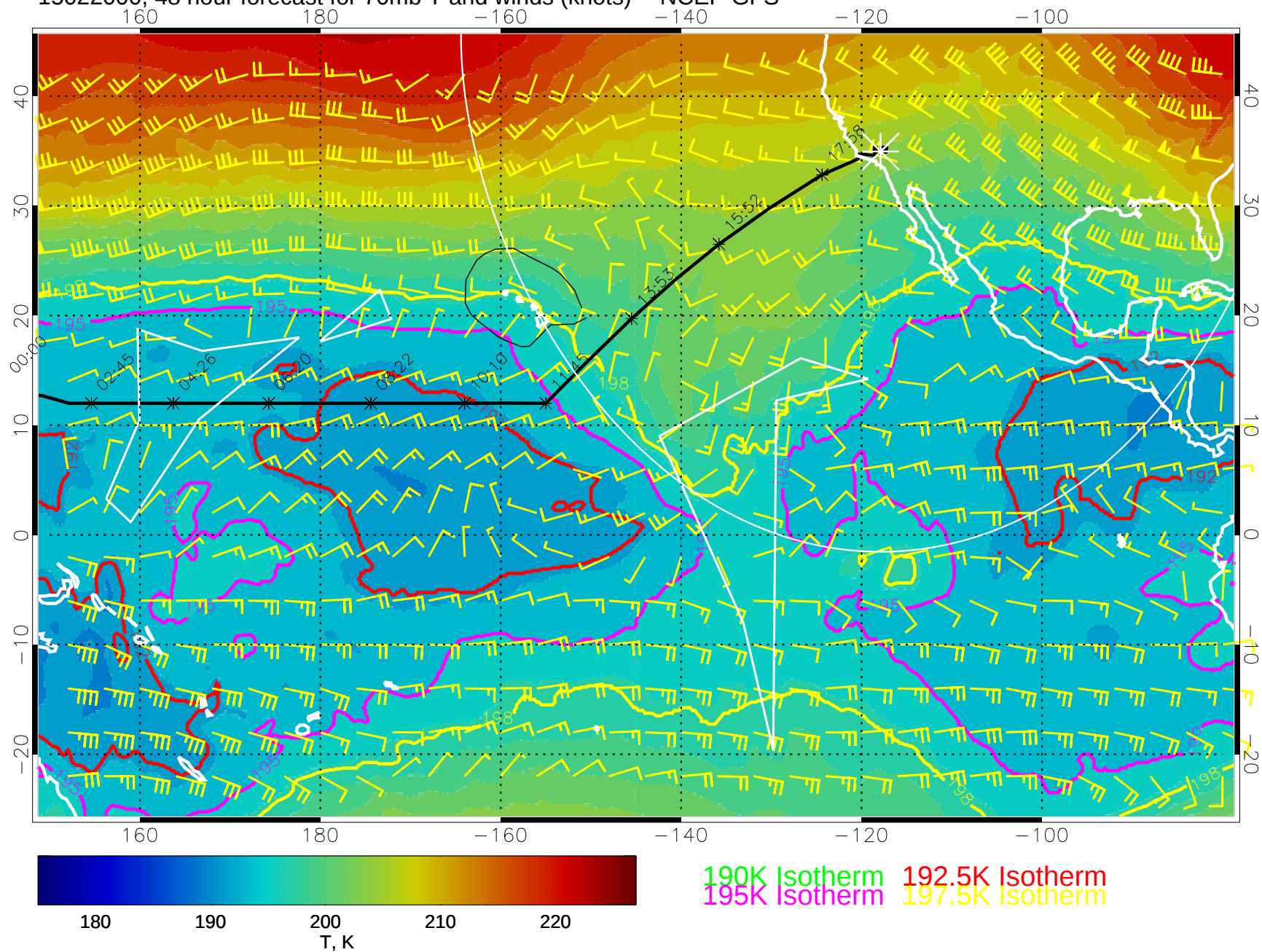
15022000, 48 hour forecast for 70mb T and winds (knots) -- NCEP GFS
