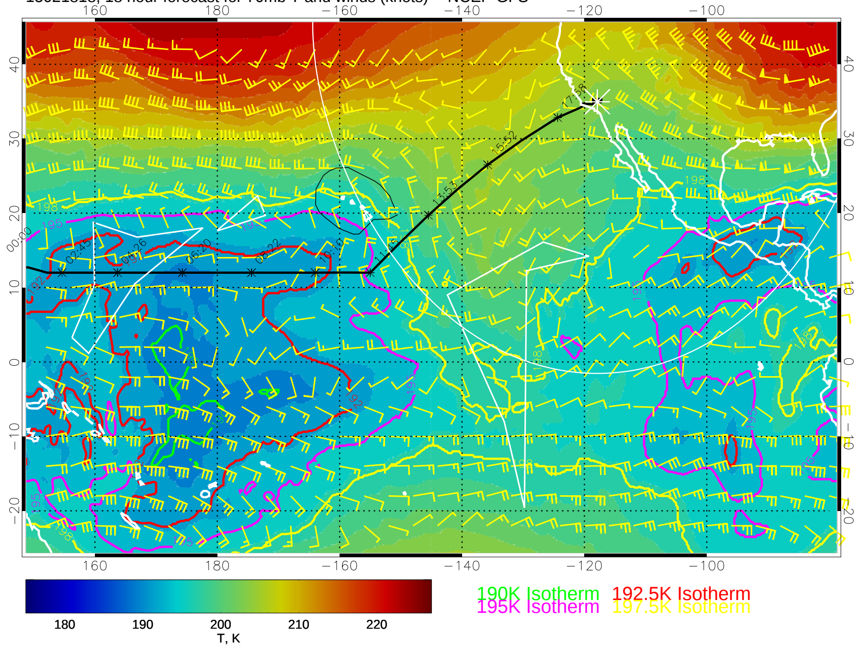
15021818, 18 hour forecast for 70mb T and winds (knots) -- NCEP GFS
