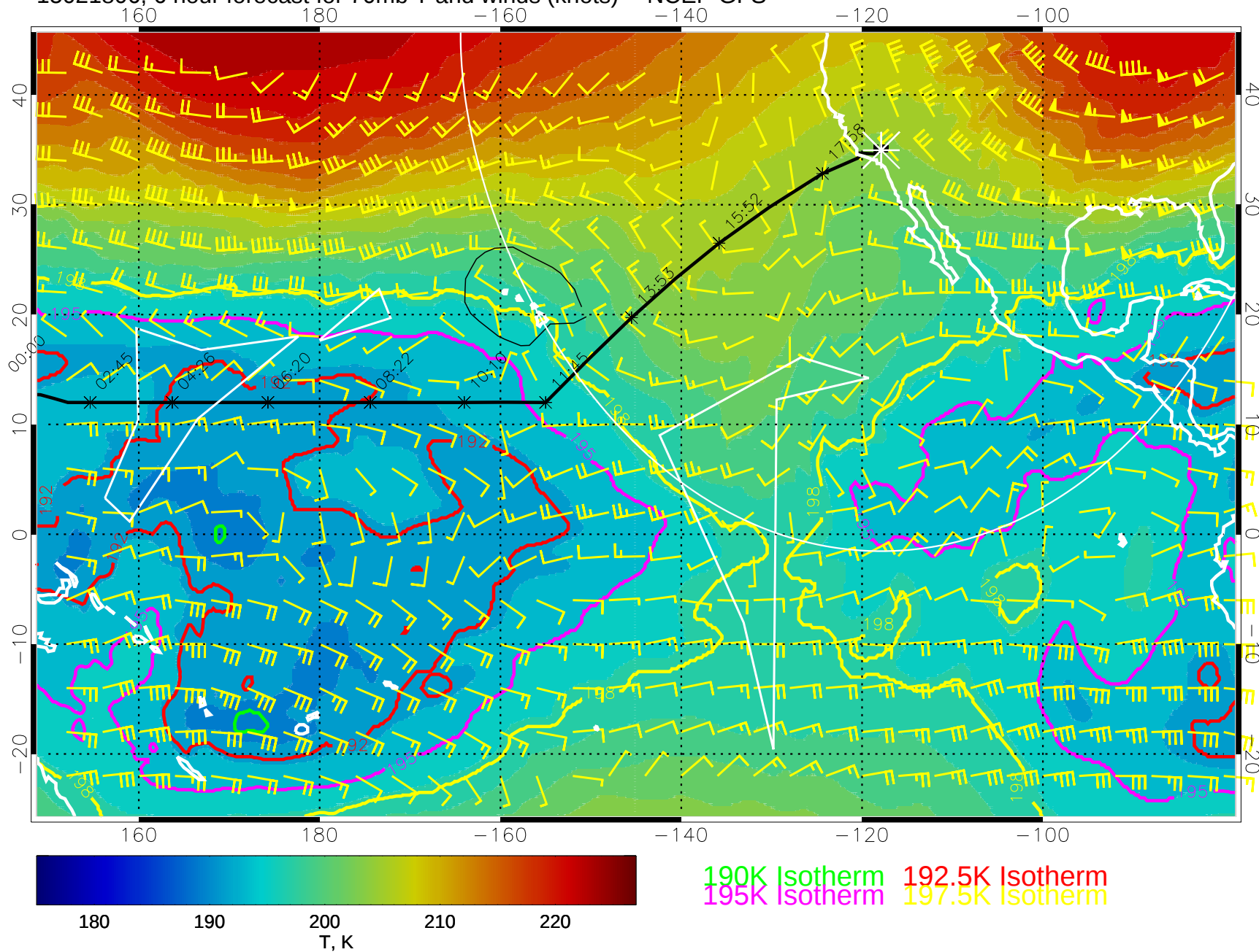
15021806, 6 hour forecast for 70mb T and winds (knots) -- NCEP GFS
