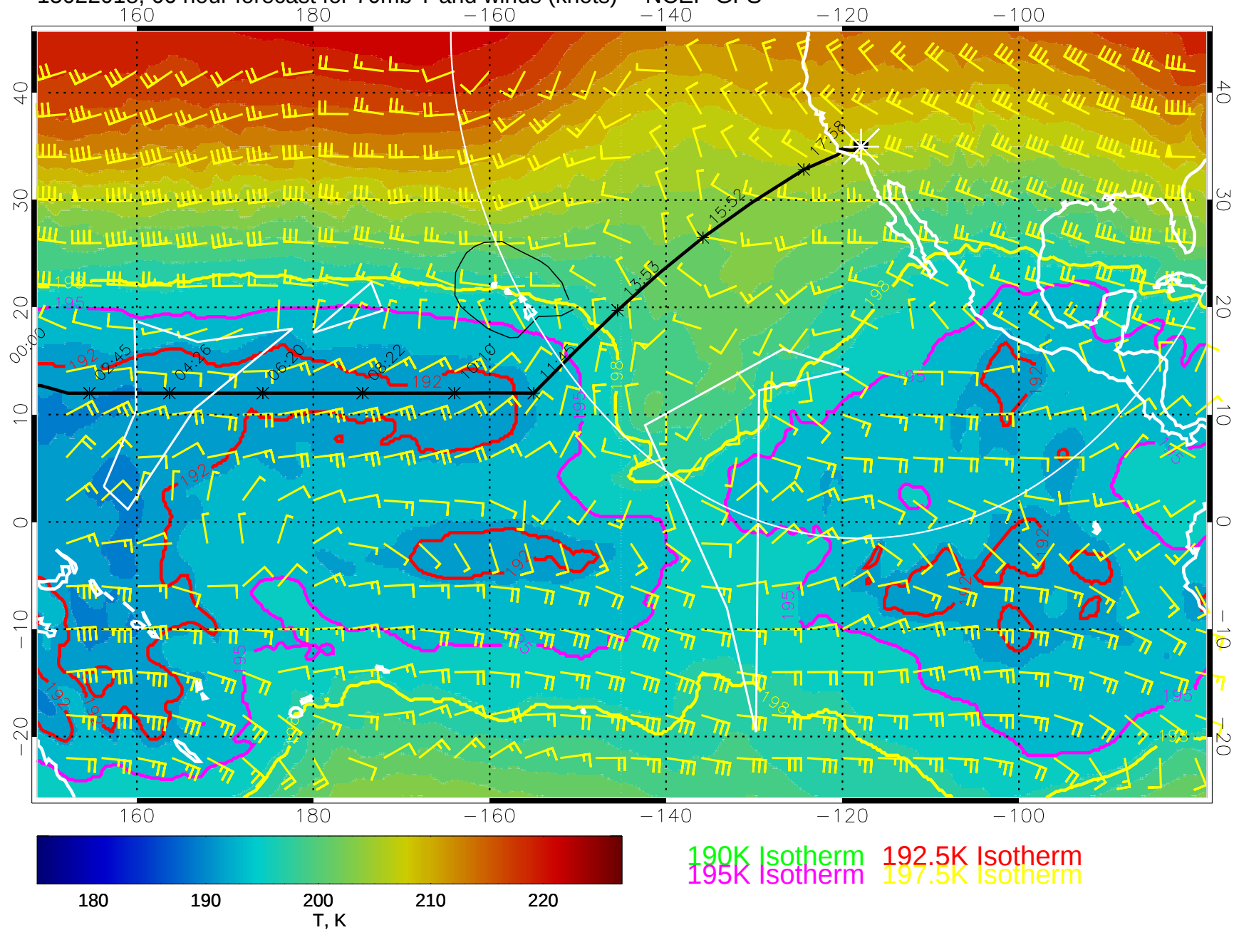
15022018, 66 hour forecast for 70mb T and winds (knots) -- NCEP GFS
