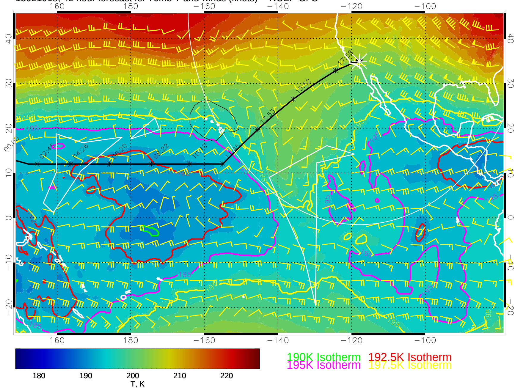
15021918, 42 hour forecast for 70mb T and winds (knots) -- NCEP GFS
