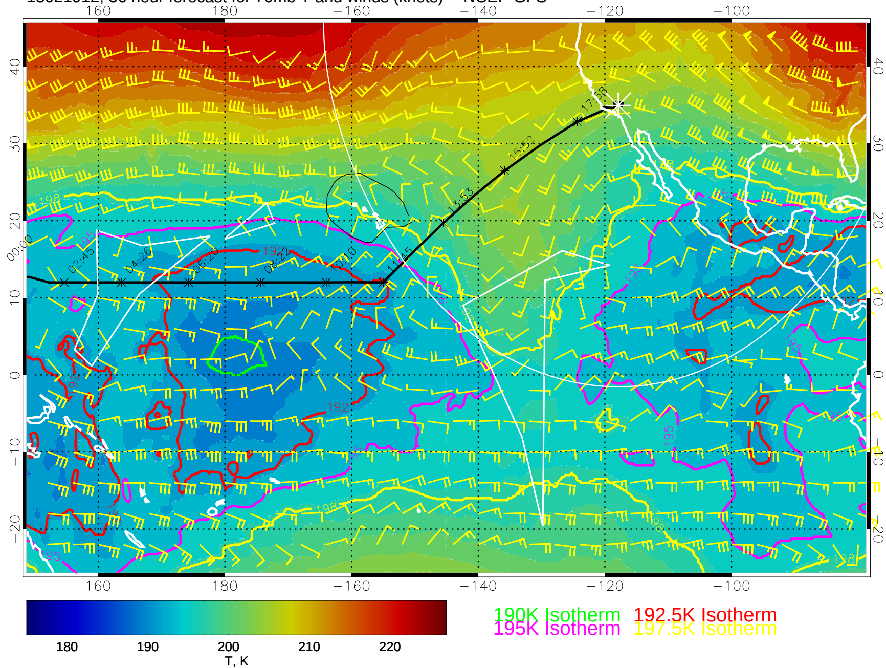
15021912, 36 hour forecast for 70mb T and winds (knots) -- NCEP GFS
