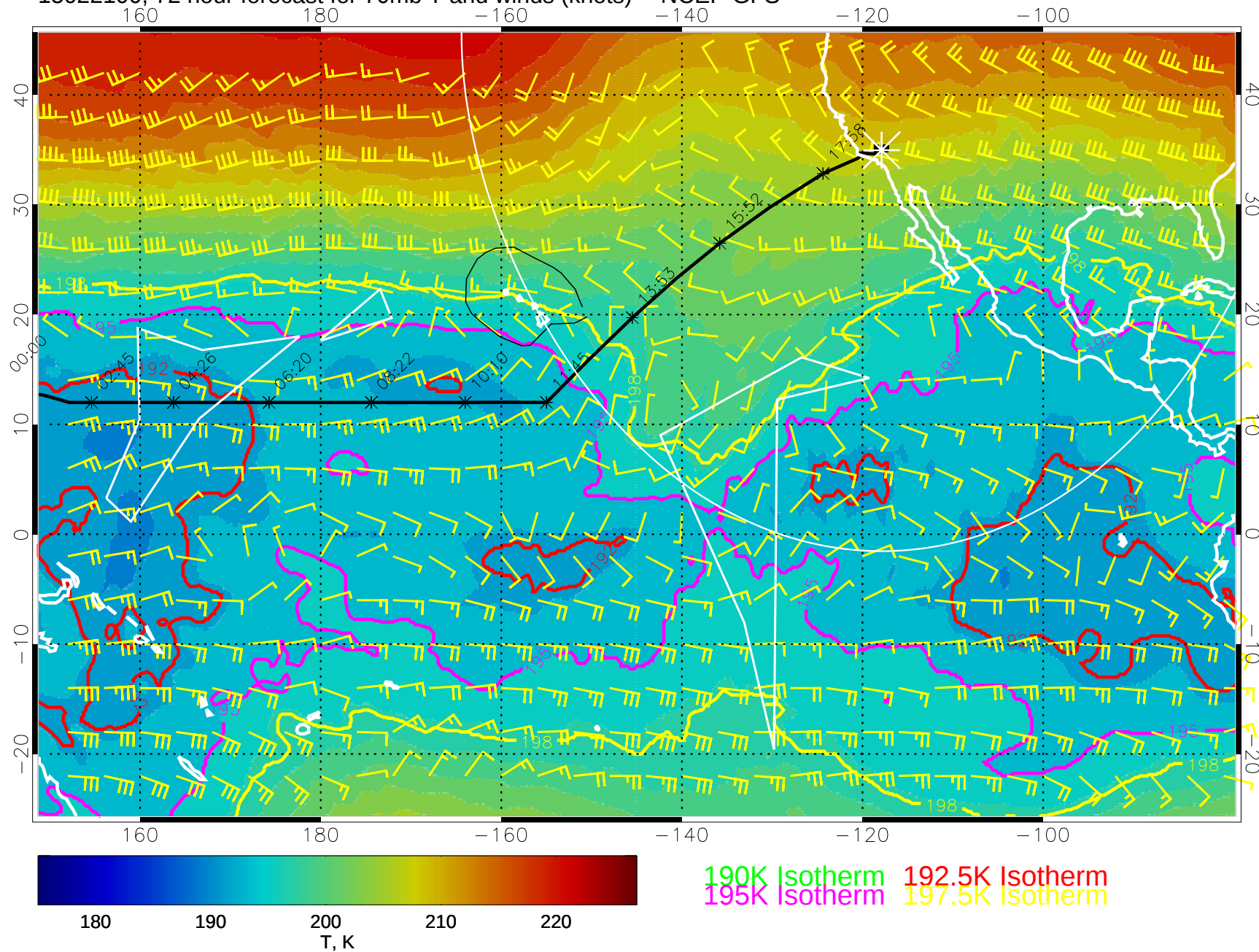
15022100, 72 hour forecast for 70mb T and winds (knots) -- NCEP GFS
