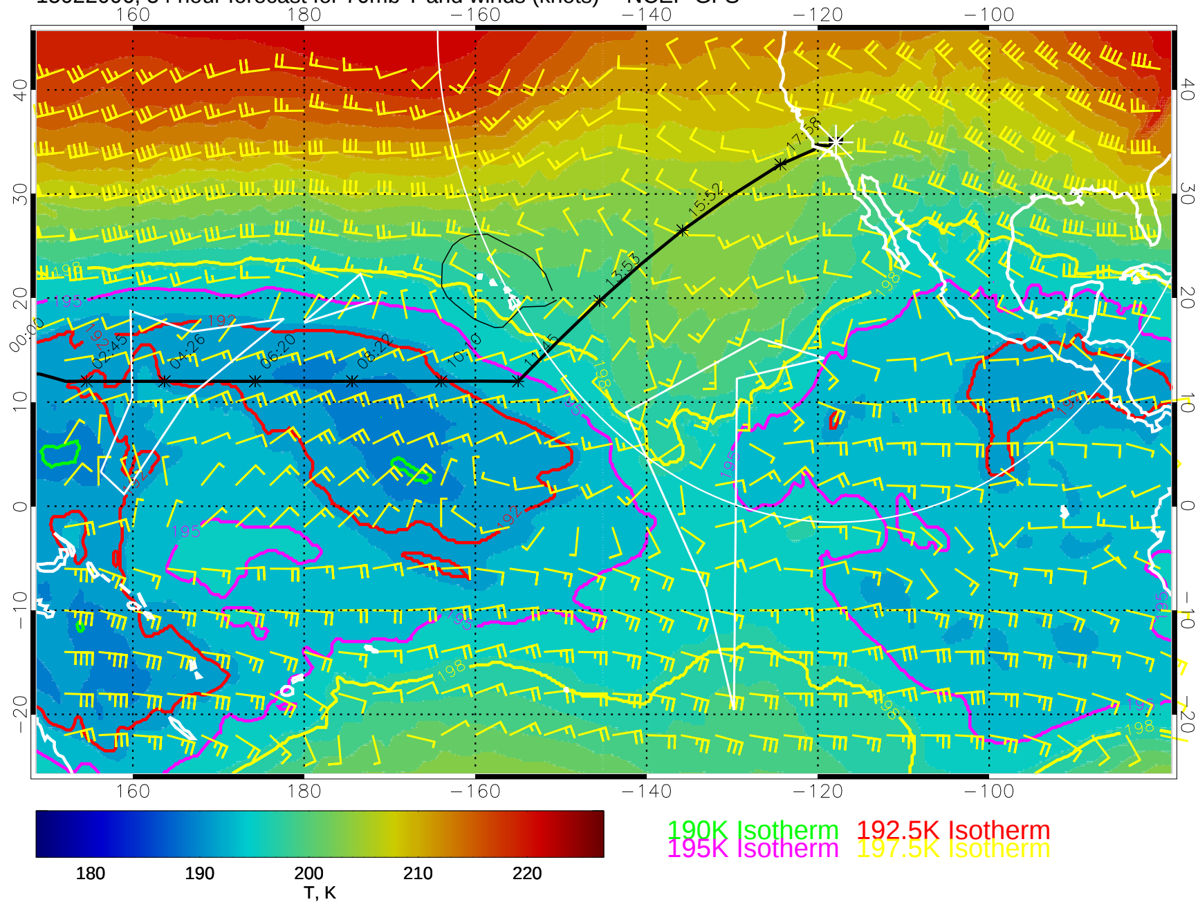
15022006, 54 hour forecast for 70mb T and winds (knots) -- NCEP GFS
