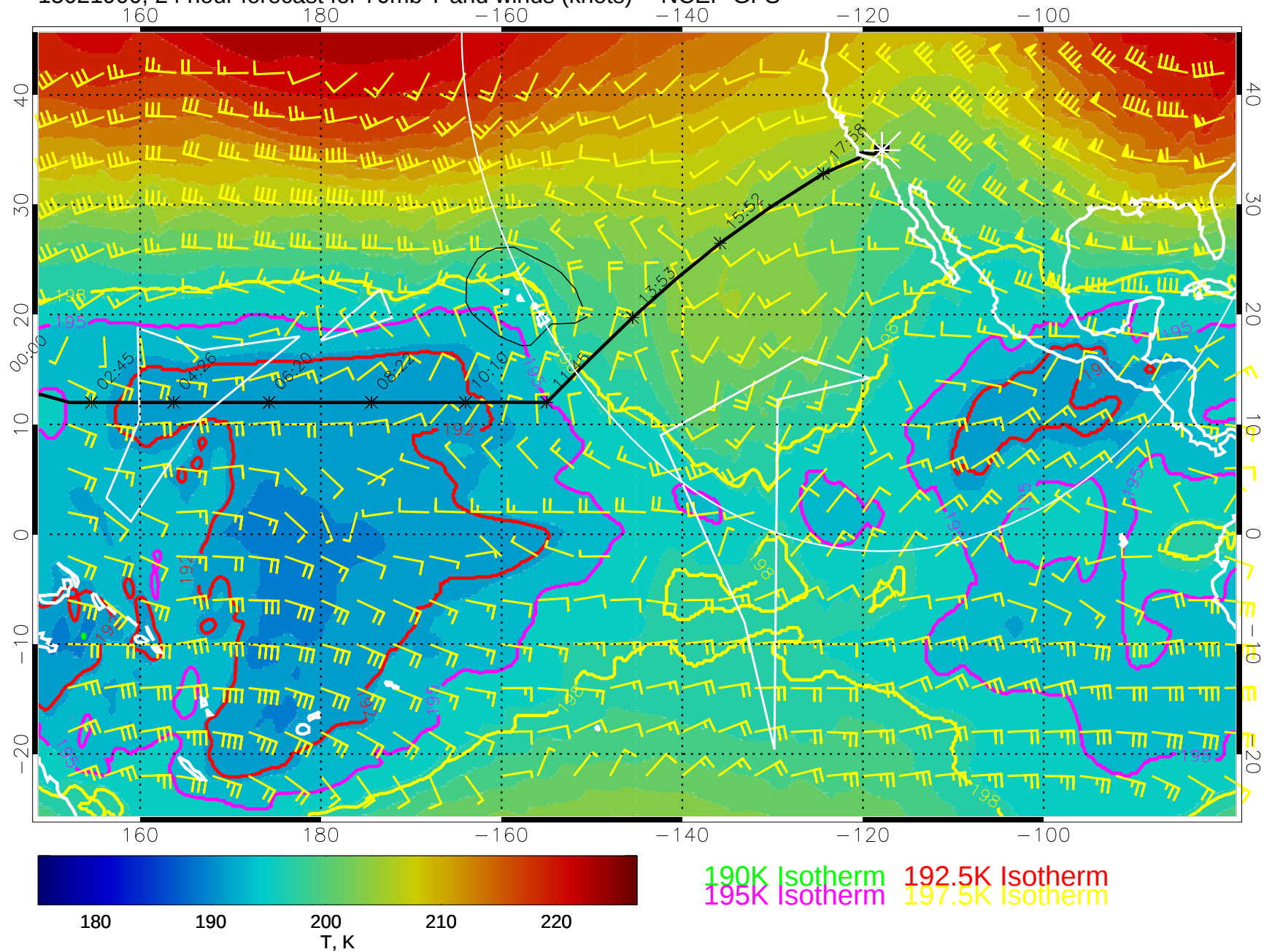
15021900, 24 hour forecast for 70mb T and winds (knots) -- NCEP GFS
