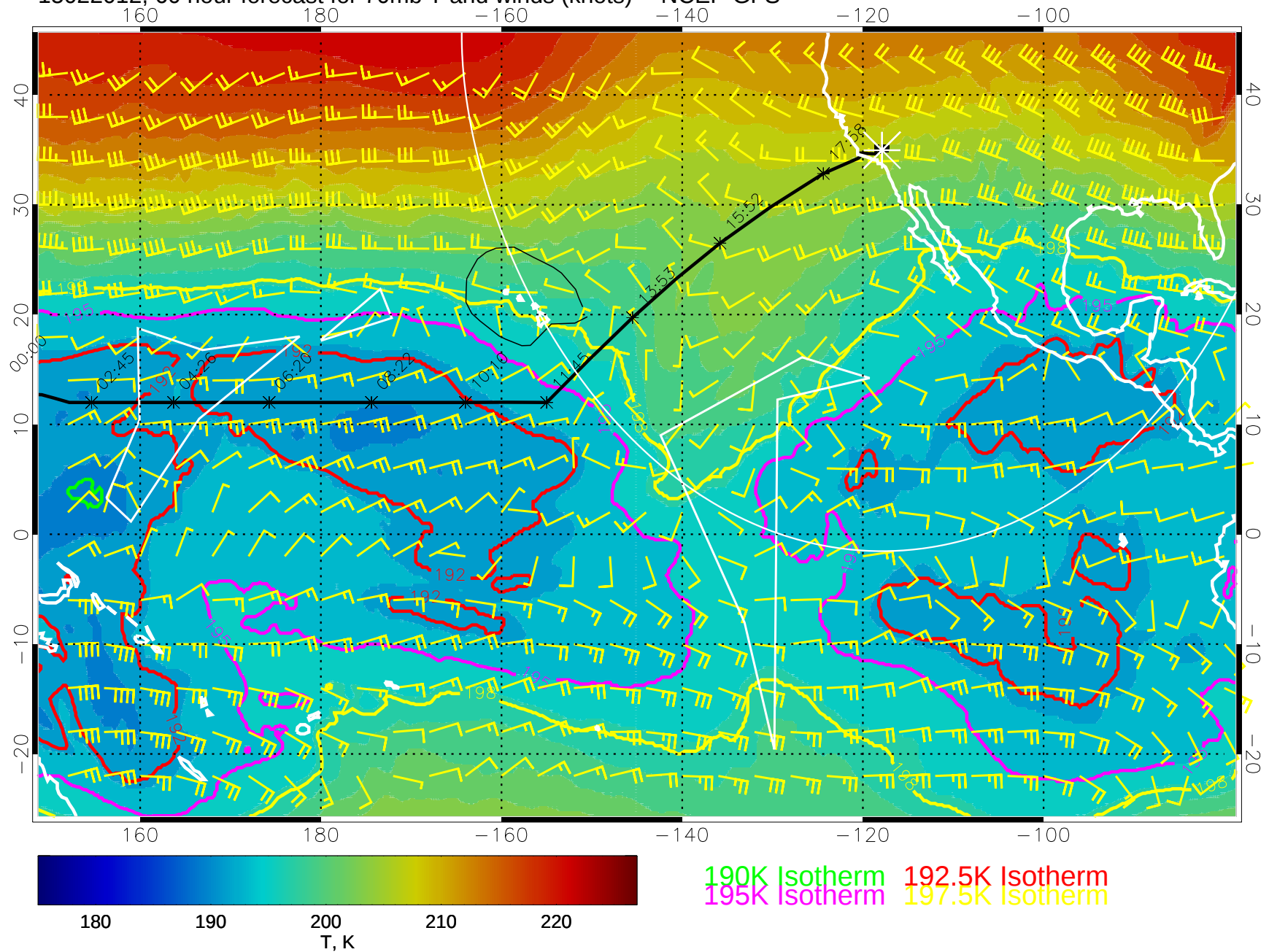
15022012, 60 hour forecast for 70mb T and winds (knots) -- NCEP GFS
