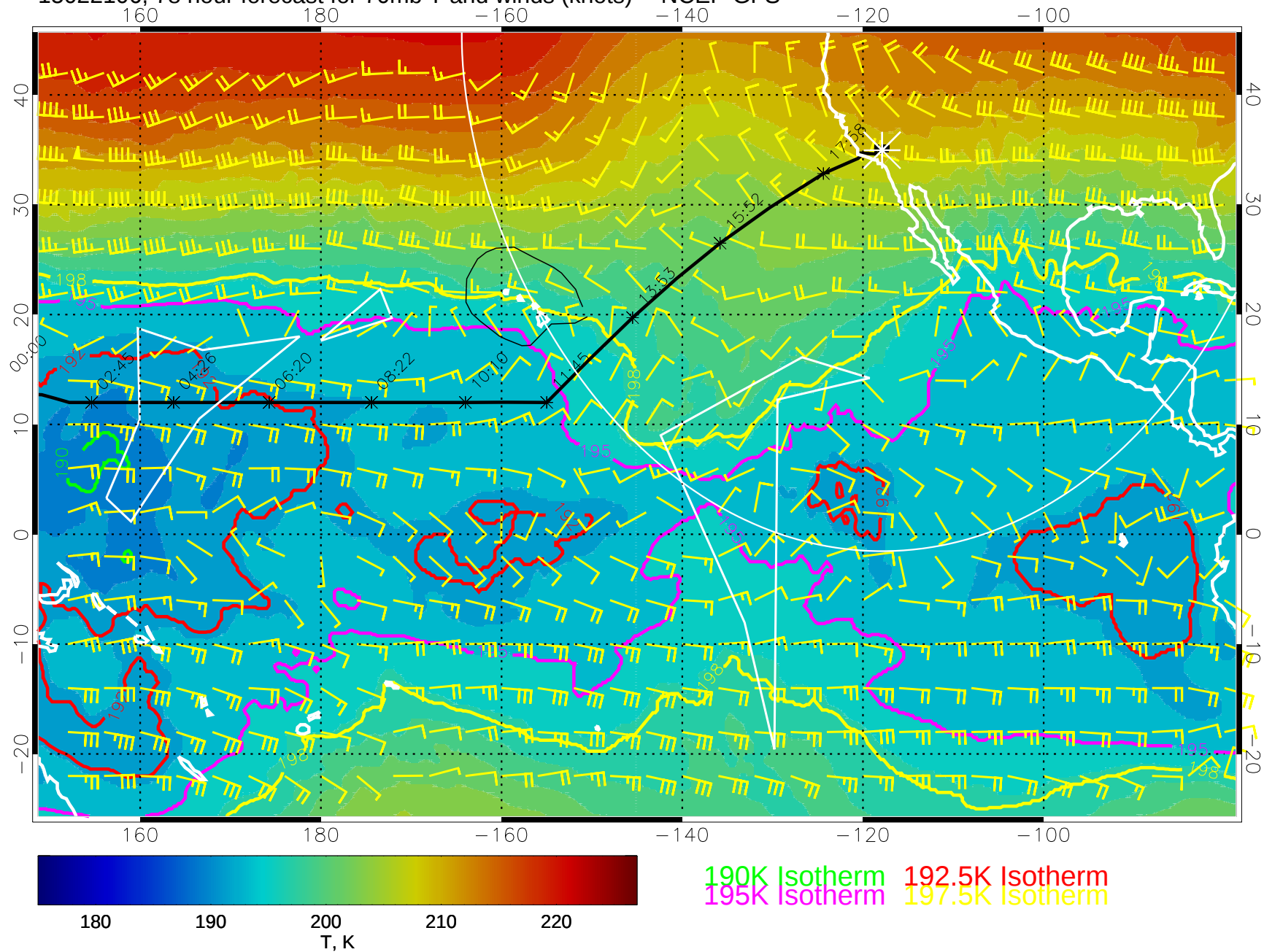
15022106, 78 hour forecast for 70mb T and winds (knots) -- NCEP GFS
