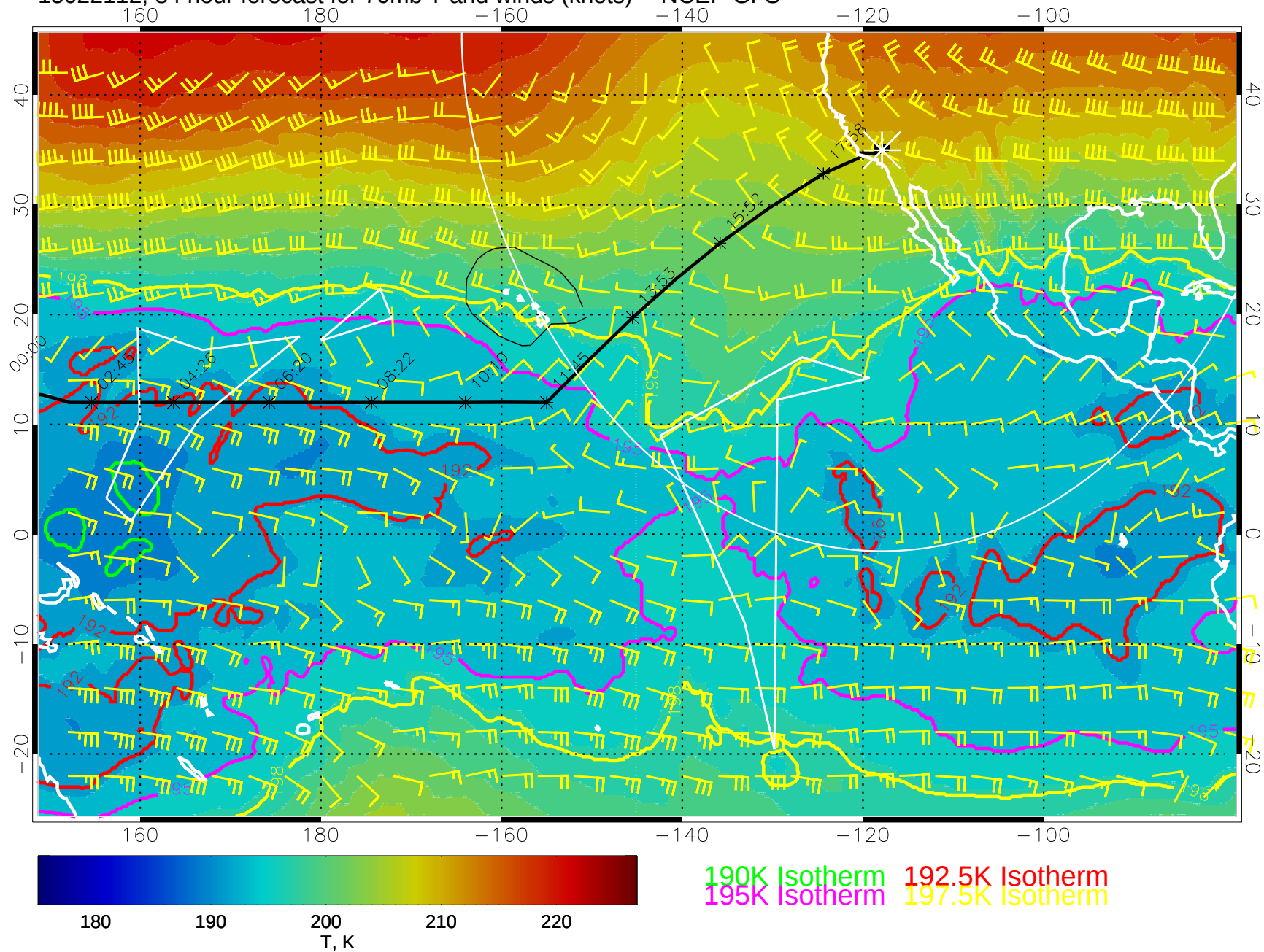
15022112, 84 hour forecast for 70mb T and winds (knots) -- NCEP GFS
