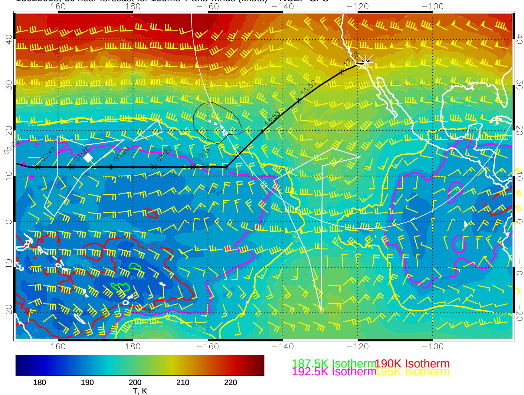
15022018, 66 hour forecast for 100mb T and winds (knots) -- NCEP GFS
