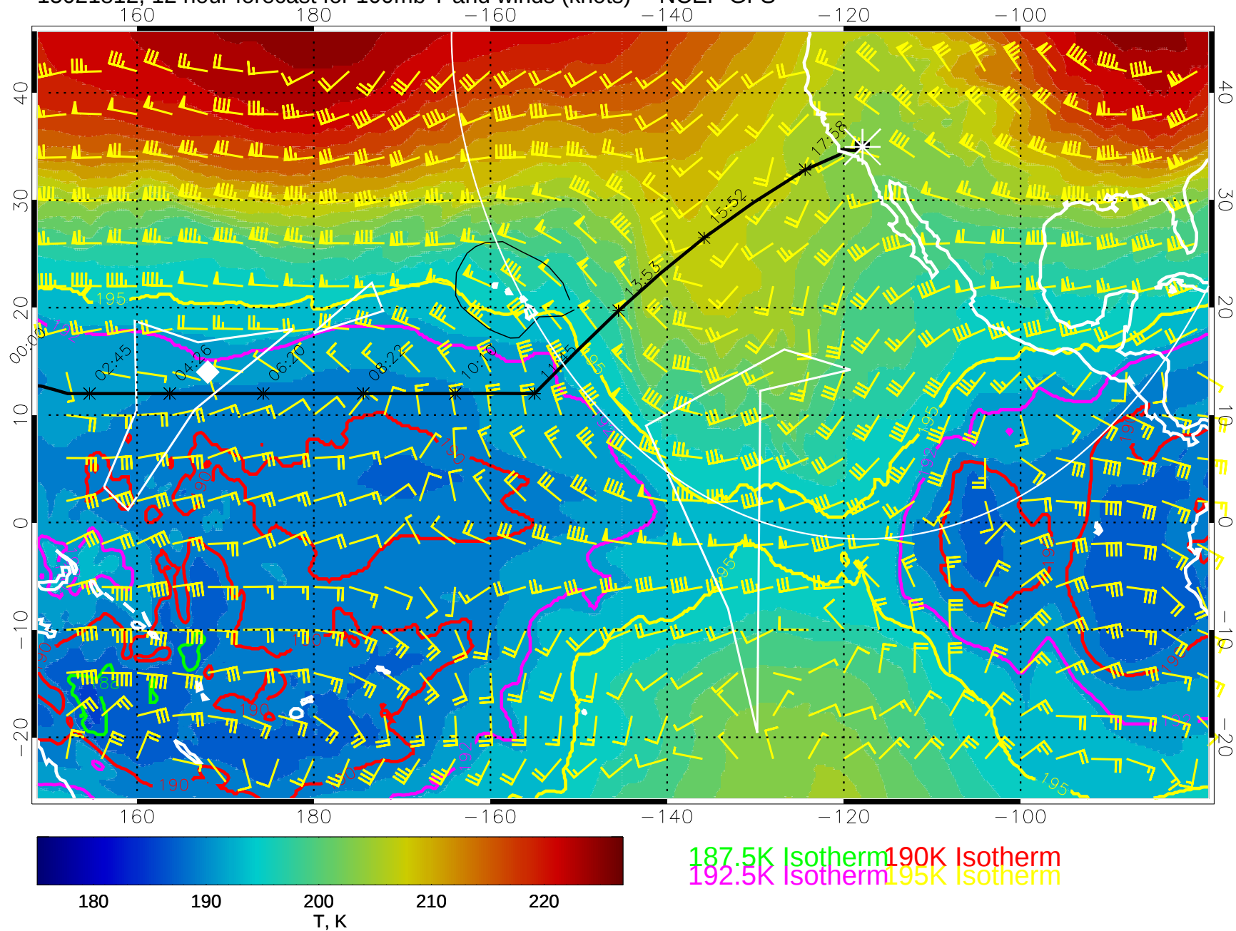
15021812, 12 hour forecast for 100mb T and winds (knots) -- NCEP GFS
