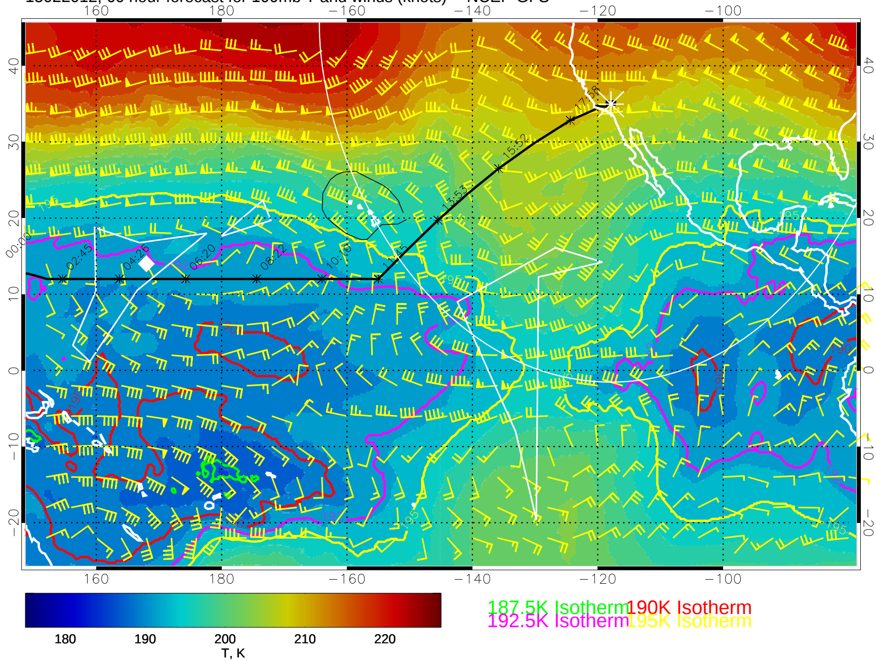
15022012, 60 hour forecast for 100mb T and winds (knots) -- NCEP GFS
