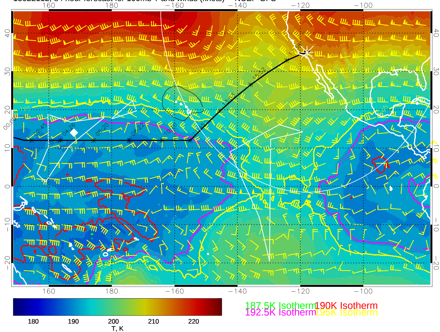
15022112, 84 hour forecast for 100mb T and winds (knots) -- NCEP GFS
