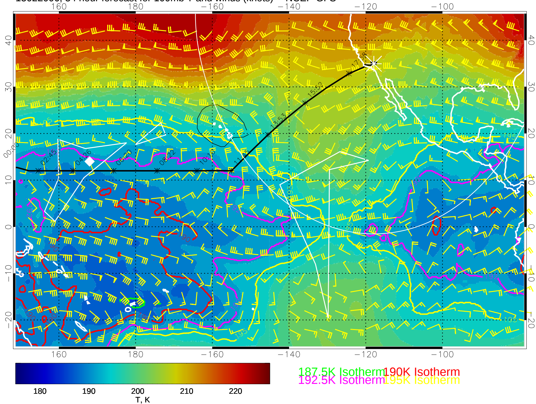
15022006, 54 hour forecast for 100mb T and winds (knots) -- NCEP GFS
