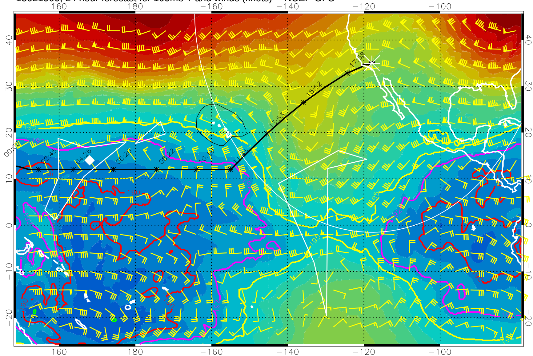
15021900, 24 hour forecast for 100mb T and winds (knots) -- NCEP GFS
