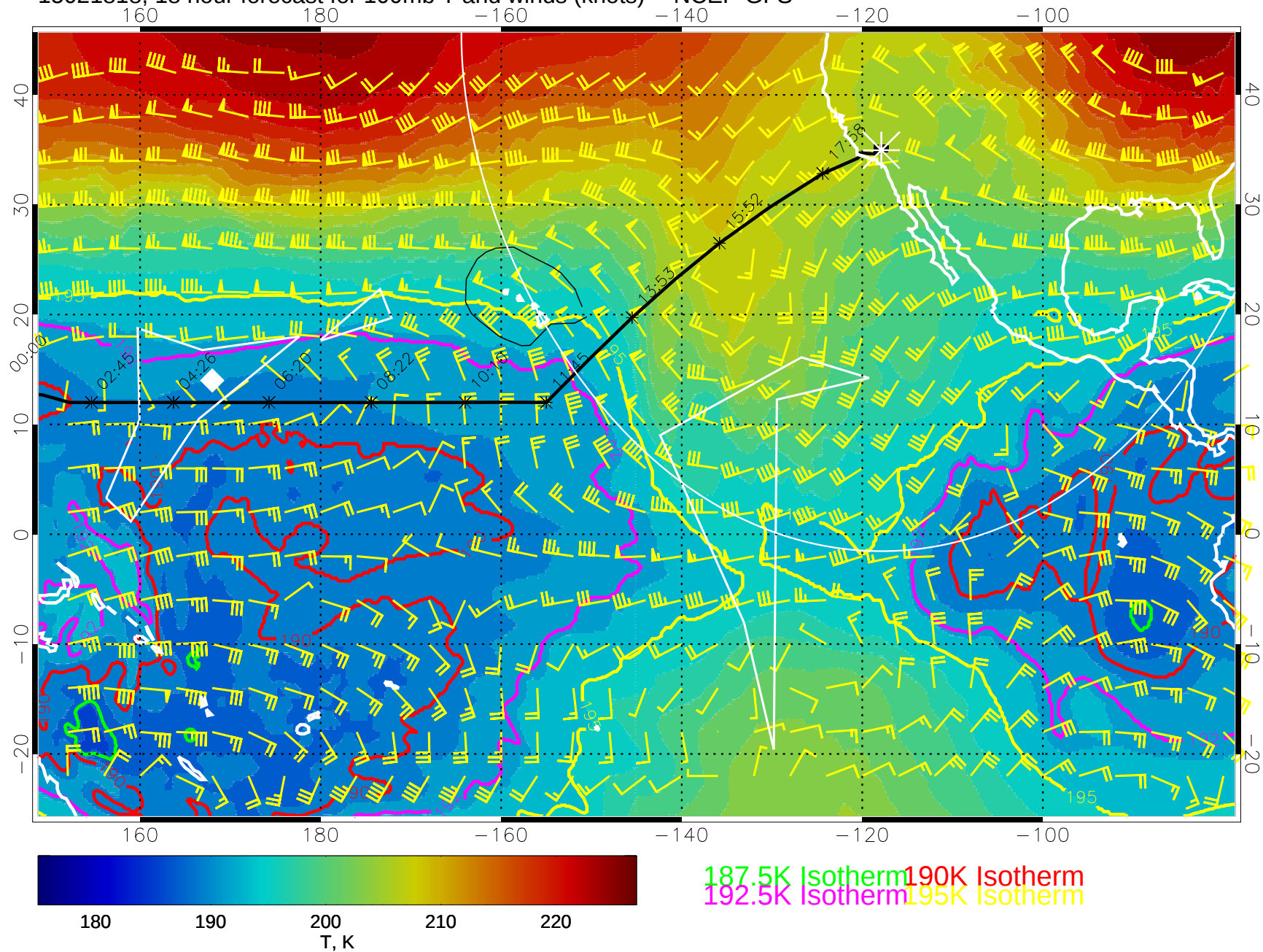
15021818, 18 hour forecast for 100mb T and winds (knots) -- NCEP GFS
