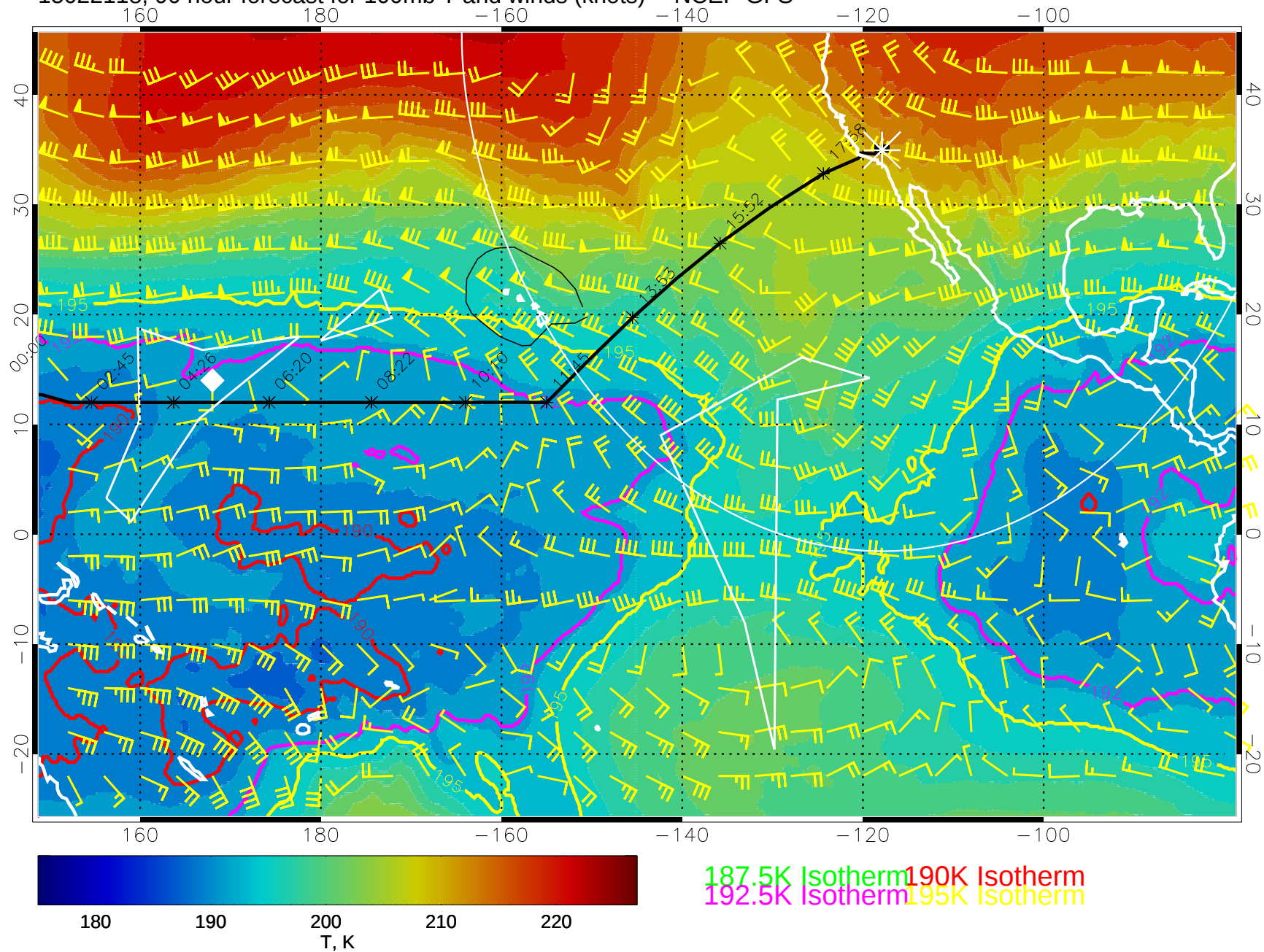
15022118, 90 hour forecast for 100mb T and winds (knots) -- NCEP GFS
