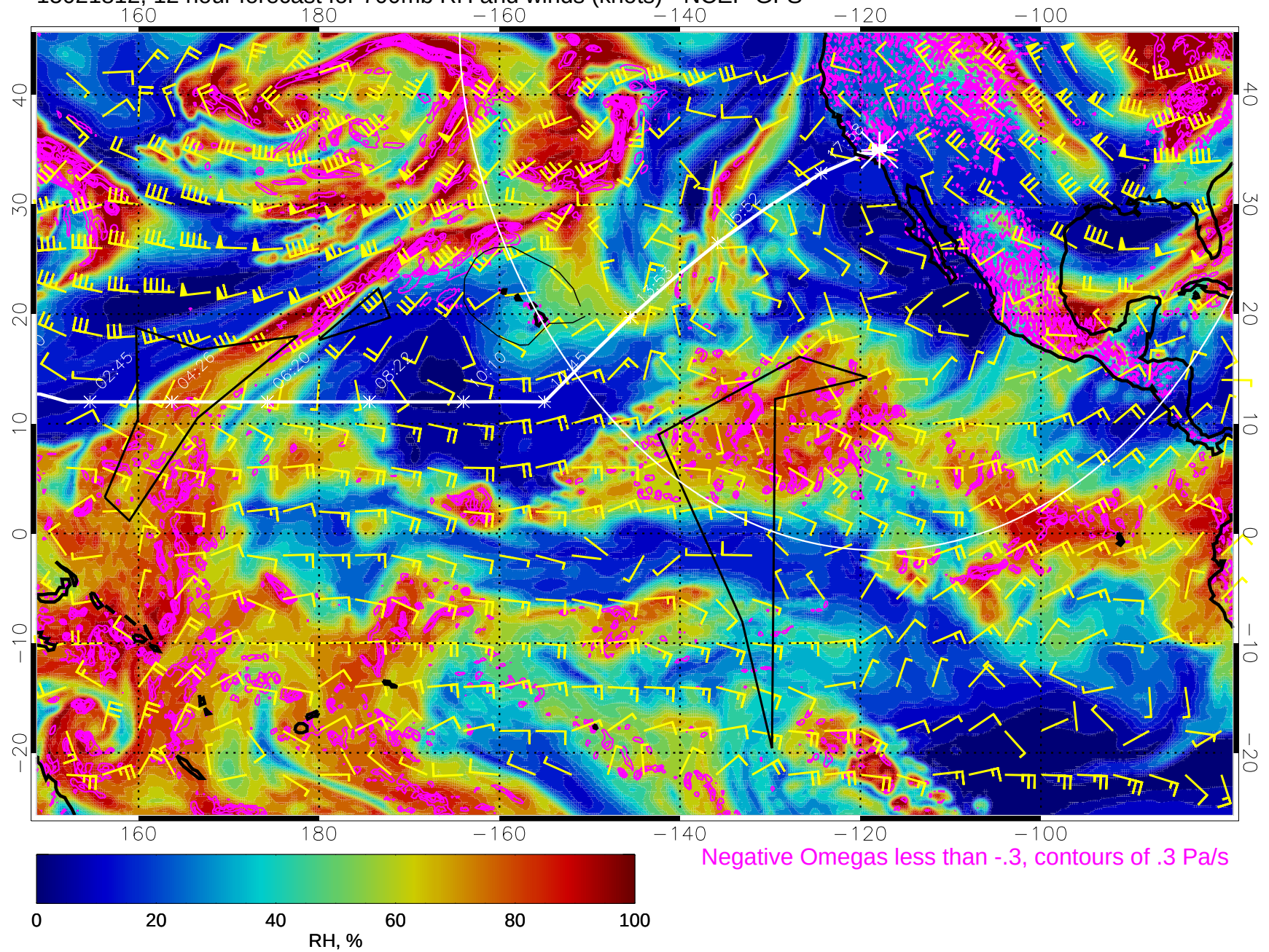
15021812, 12 hour forecast for 700mb RH and winds (knots) - NCEP GFS
