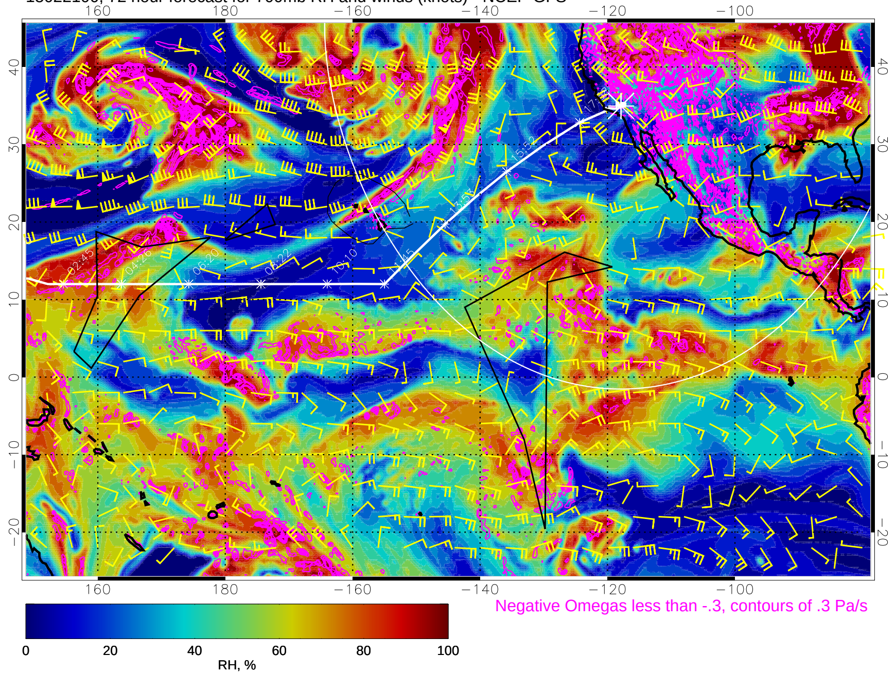
15022100, 72 hour forecast for 700mb RH and winds (knots) - NCEP GFS
