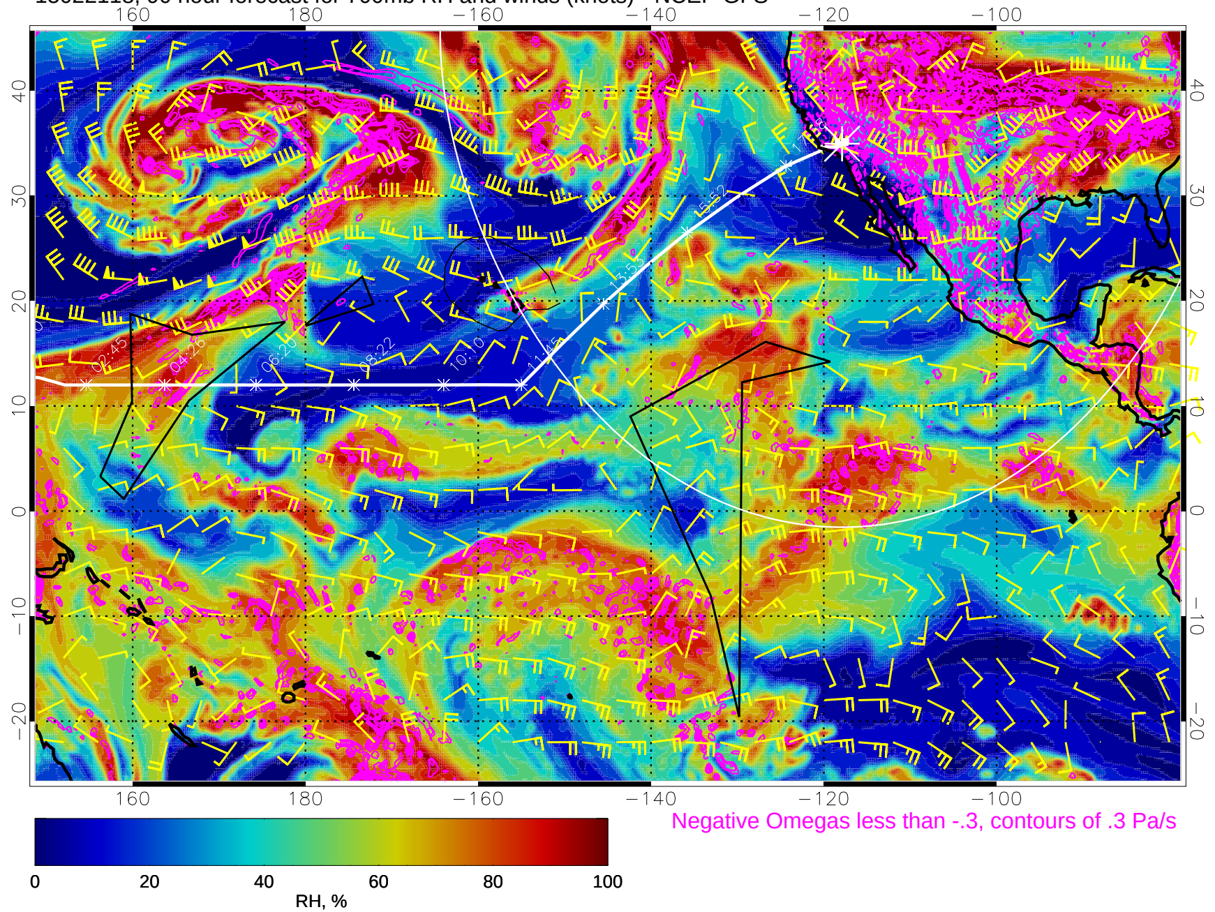
15022118, 90 hour forecast for 700mb RH and winds (knots) - NCEP GFS
