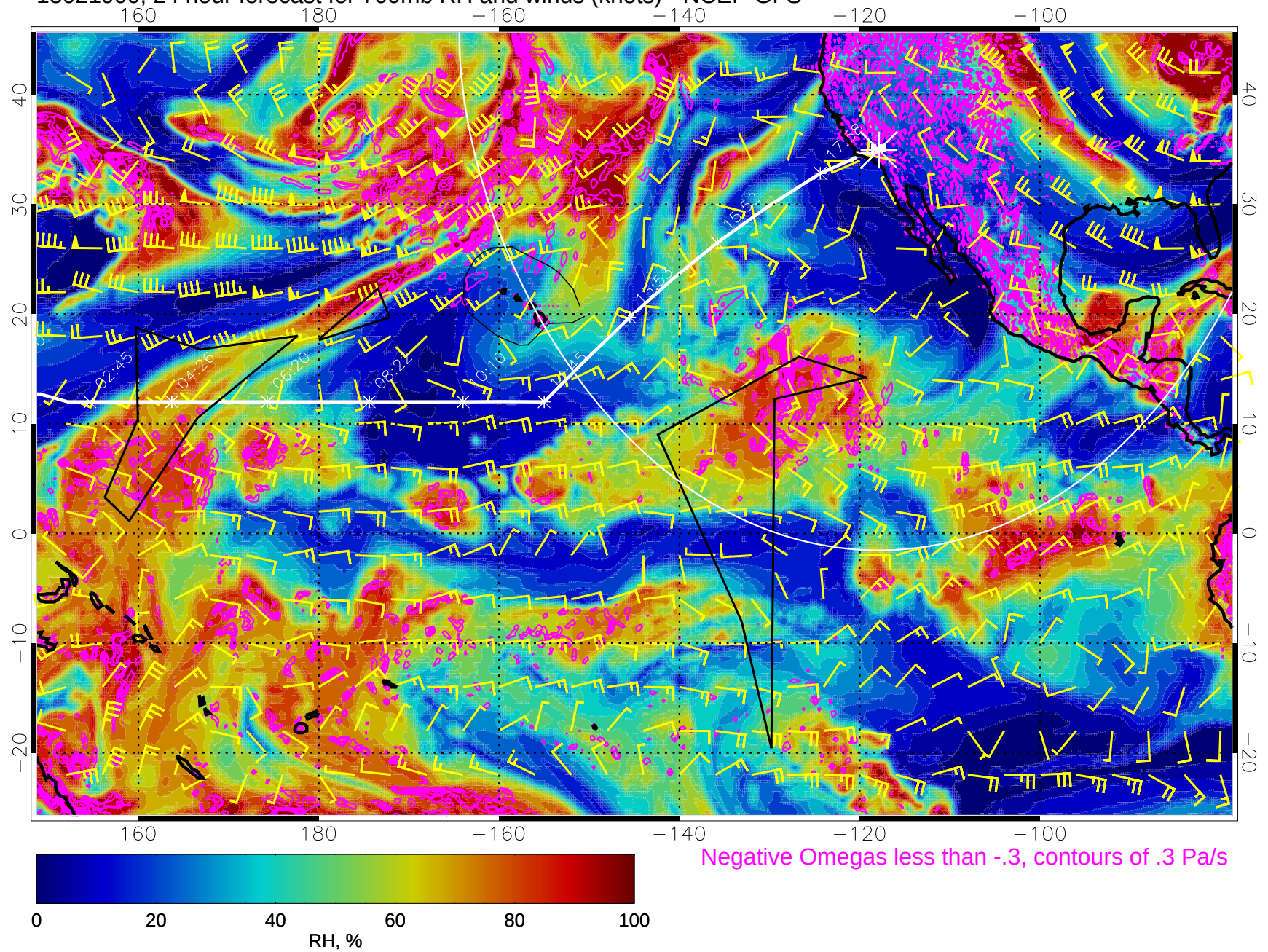
15021900, 24 hour forecast for 700mb RH and winds (knots) - NCEP GFS
