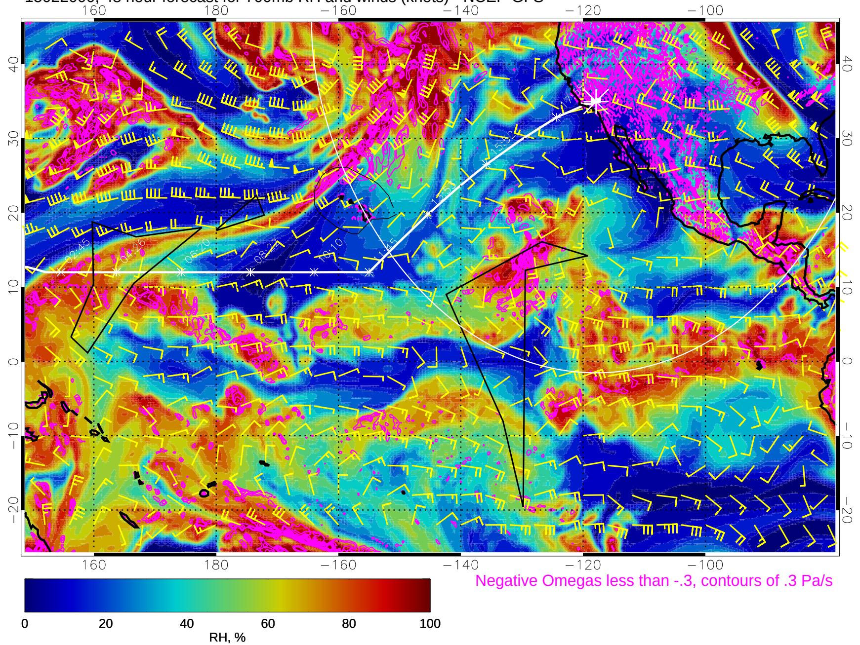
15022000, 48 hour forecast for 700mb RH and winds (knots) - NCEP GFS
