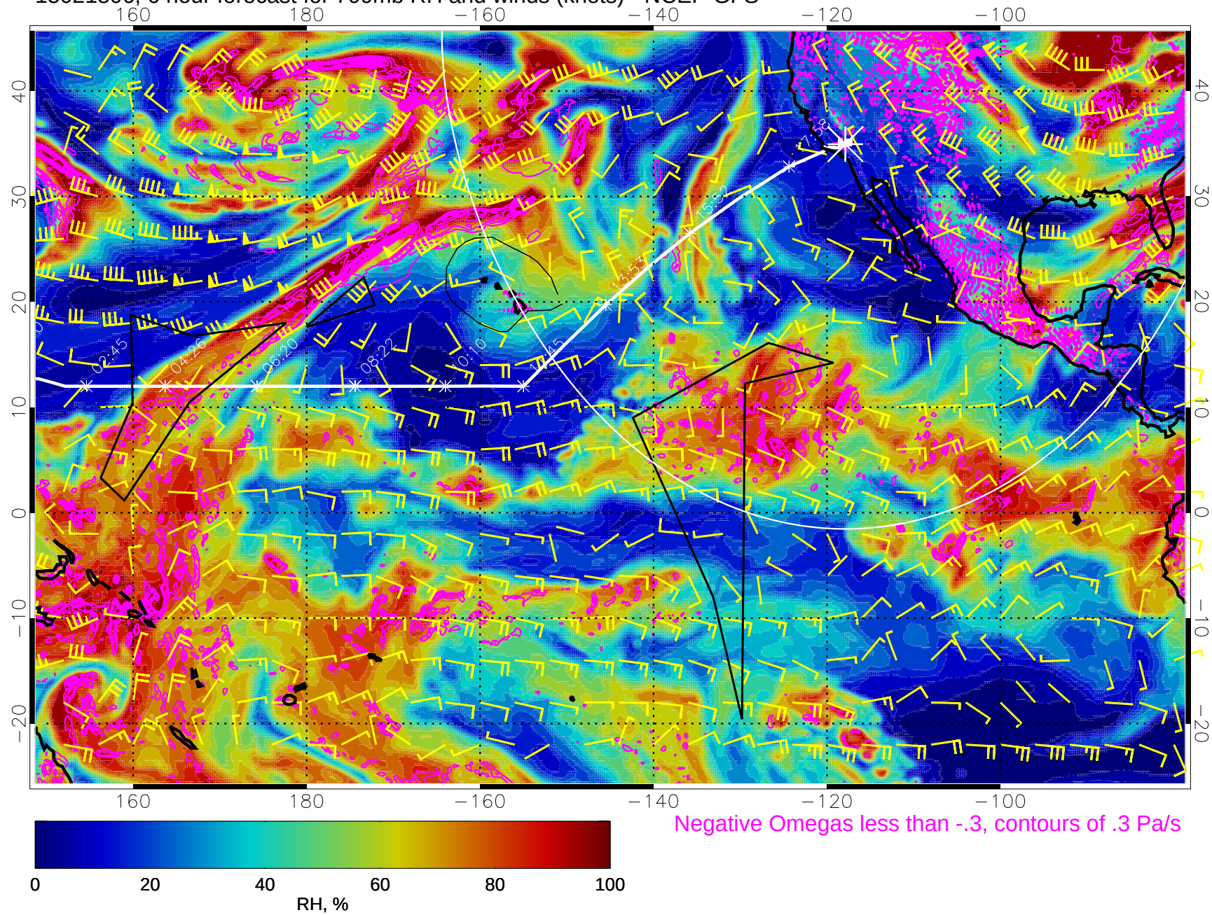
15021806, 6 hour forecast for 700mb RH and winds (knots) - NCEP GFS
