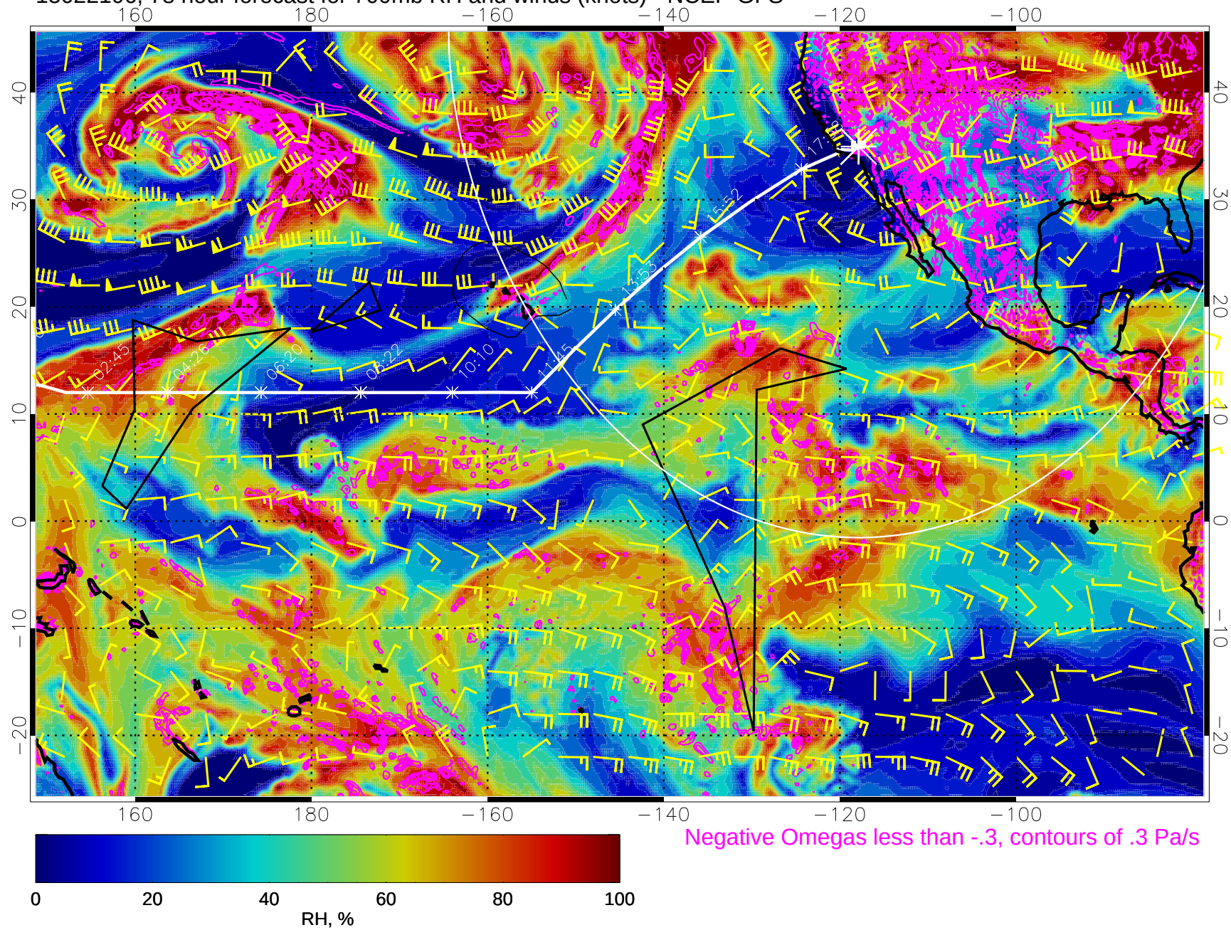
15022106, 78 hour forecast for 700mb RH and winds (knots) - NCEP GFS
