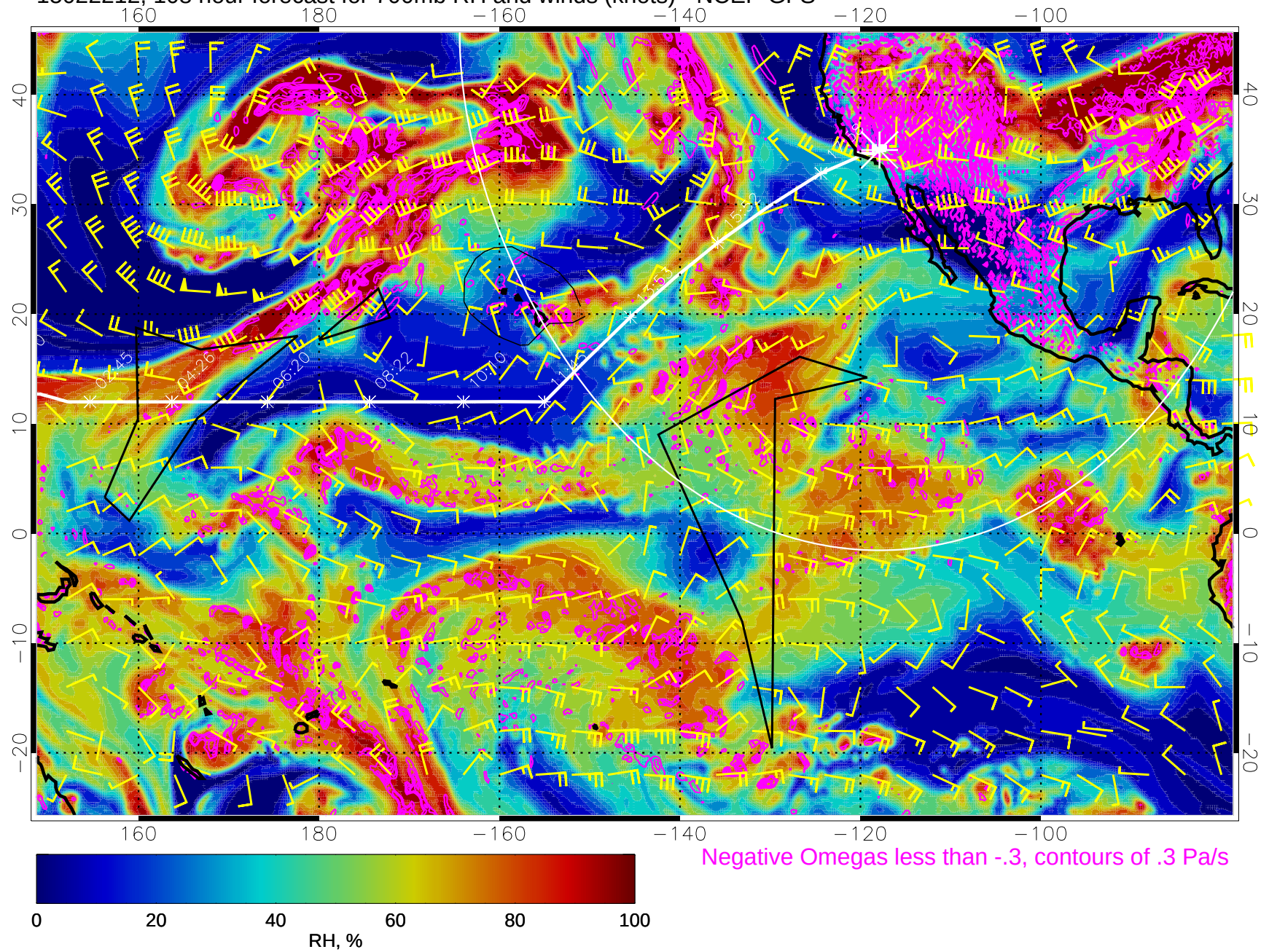
15022212, 108 hour forecast for 700mb RH and winds (knots) - NCEP GFS
