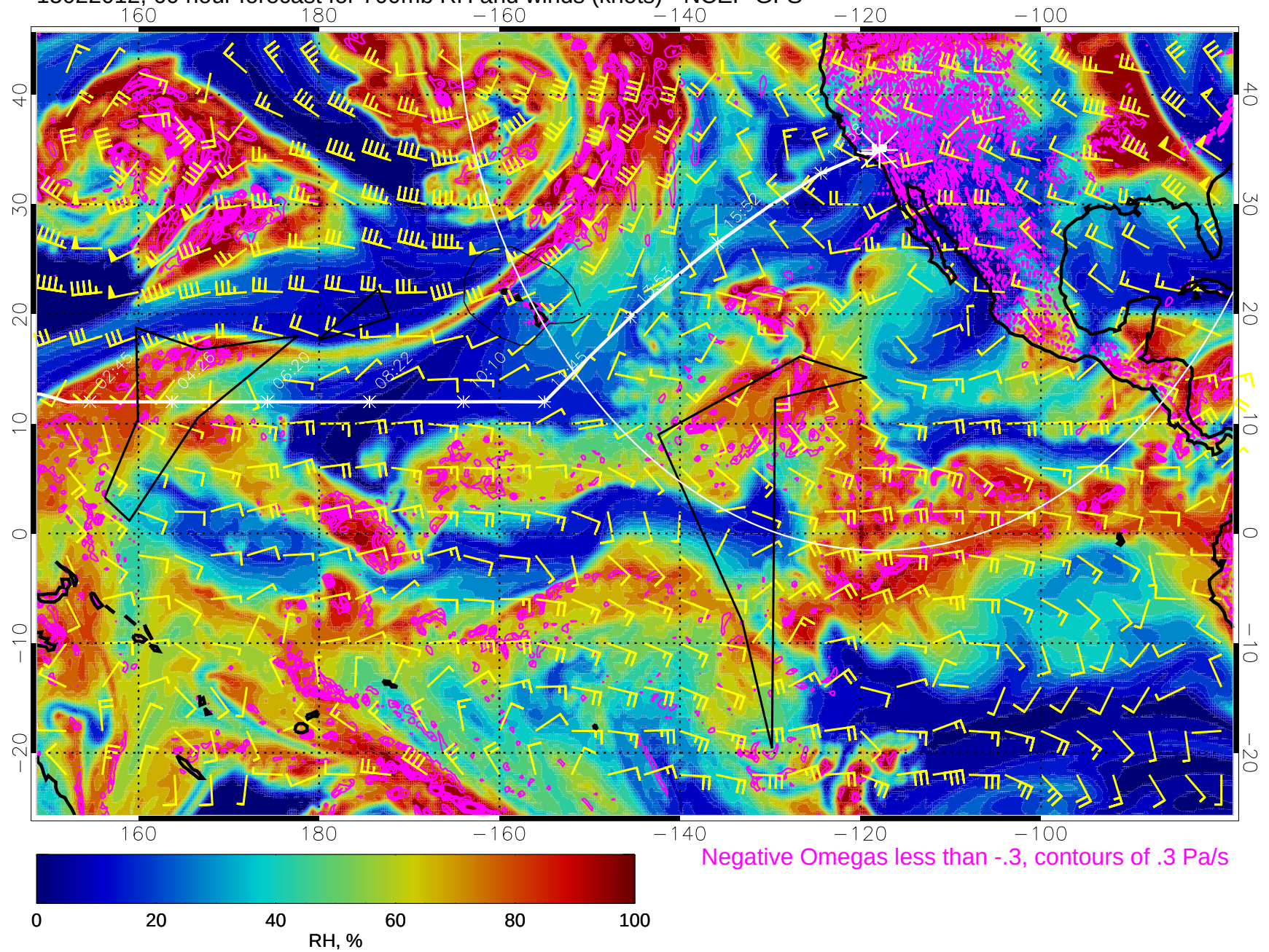
15022012, 60 hour forecast for 700mb RH and winds (knots) - NCEP GFS
