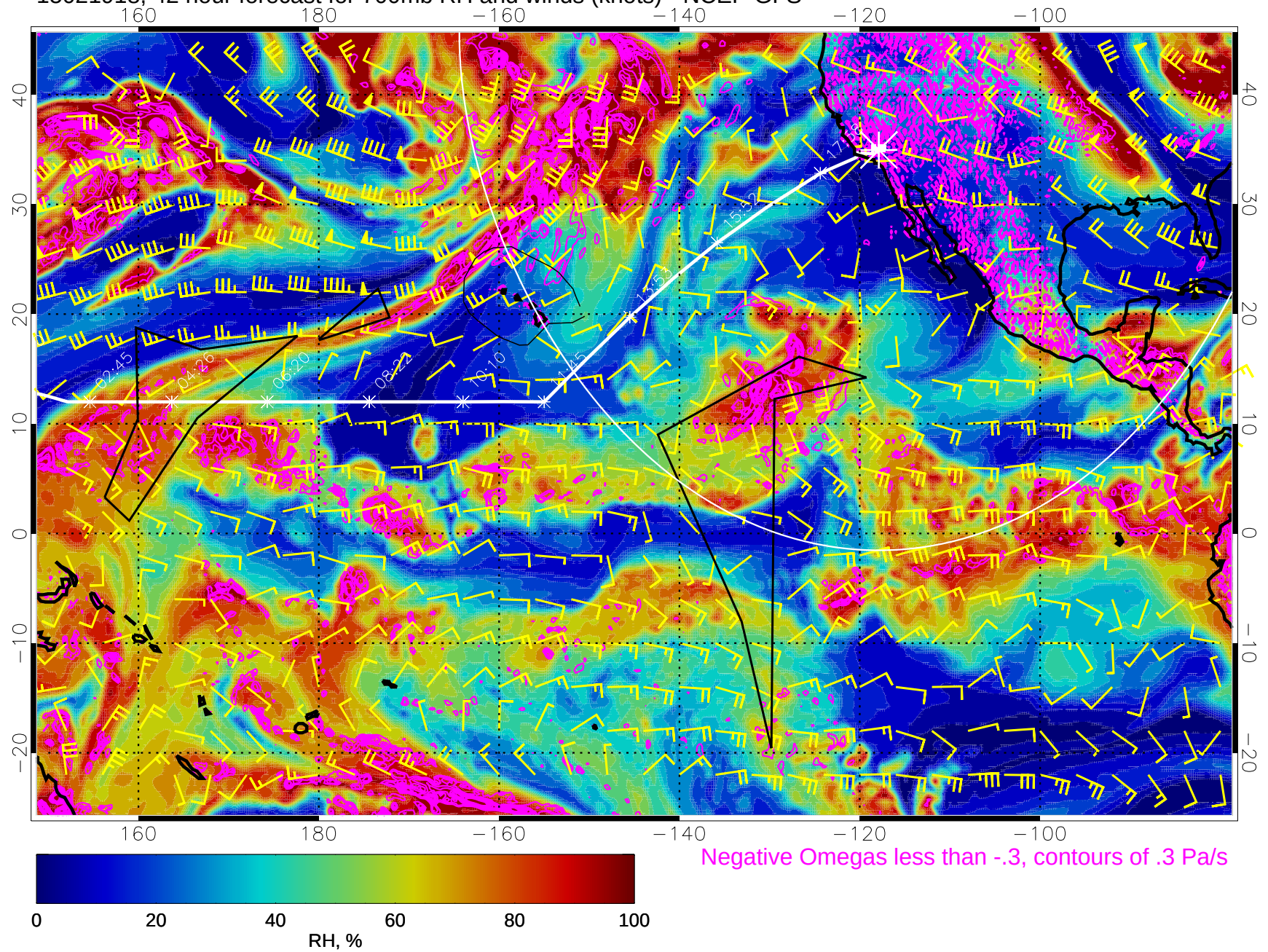
15021918, 42 hour forecast for 700mb RH and winds (knots) - NCEP GFS
