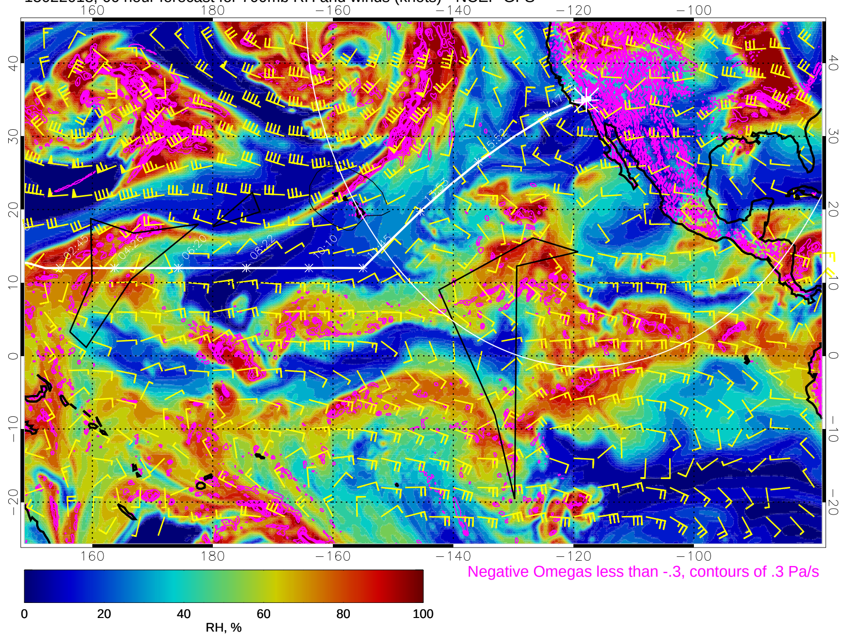
15022018, 66 hour forecast for 700mb RH and winds (knots) - NCEP GFS
