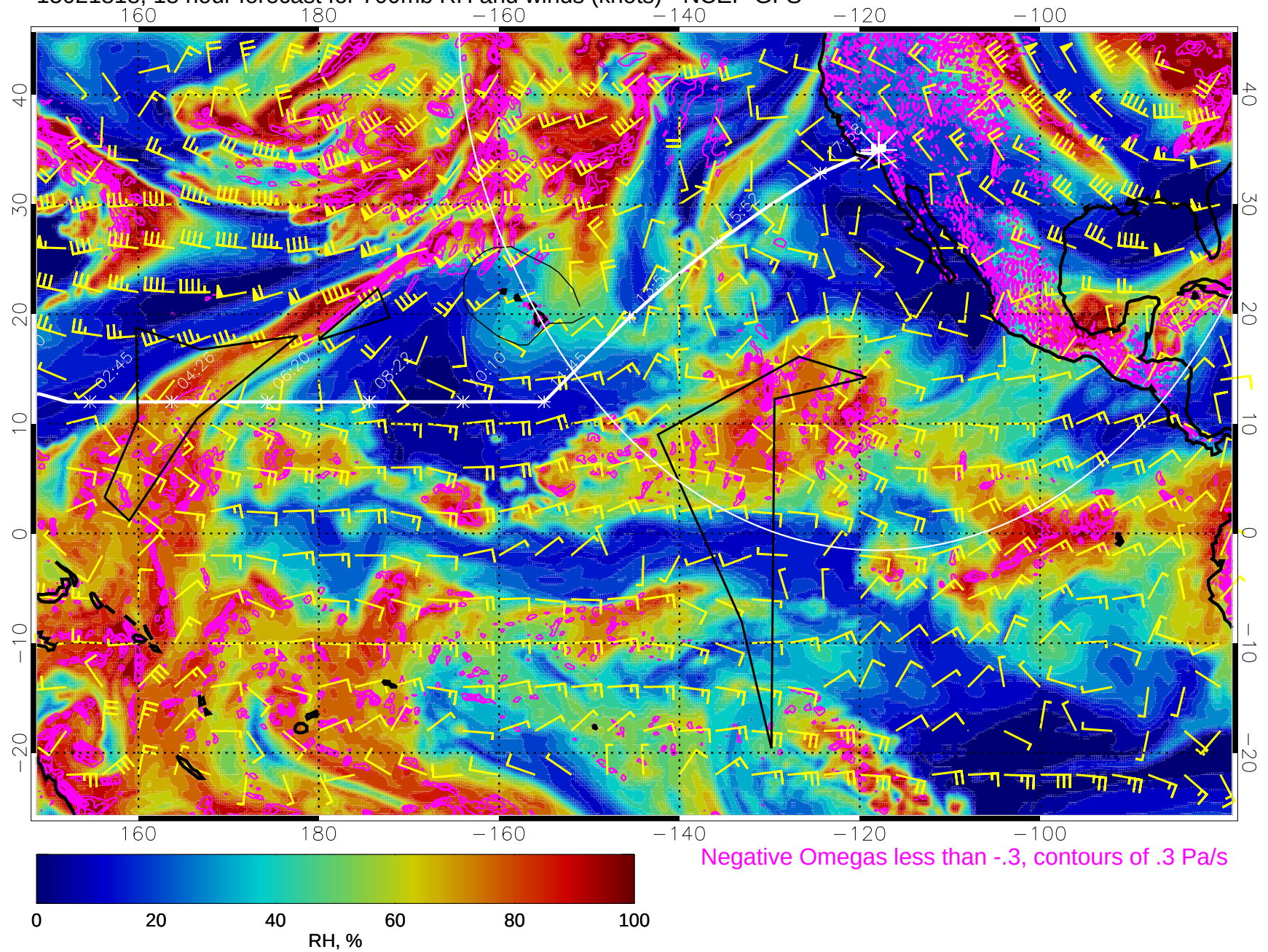
15021818, 18 hour forecast for 700mb RH and winds (knots) - NCEP GFS
