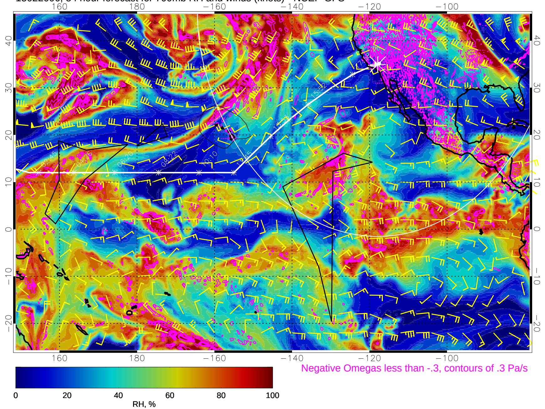
15022006, 54 hour forecast for 700mb RH and winds (knots) - NCEP GFS
