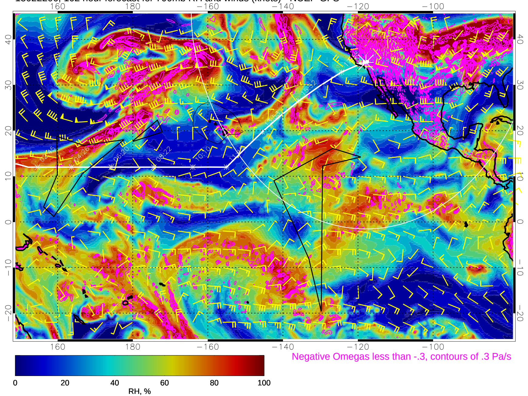
15022206, 102 hour forecast for 700mb RH and winds (knots) - NCEP GFS
