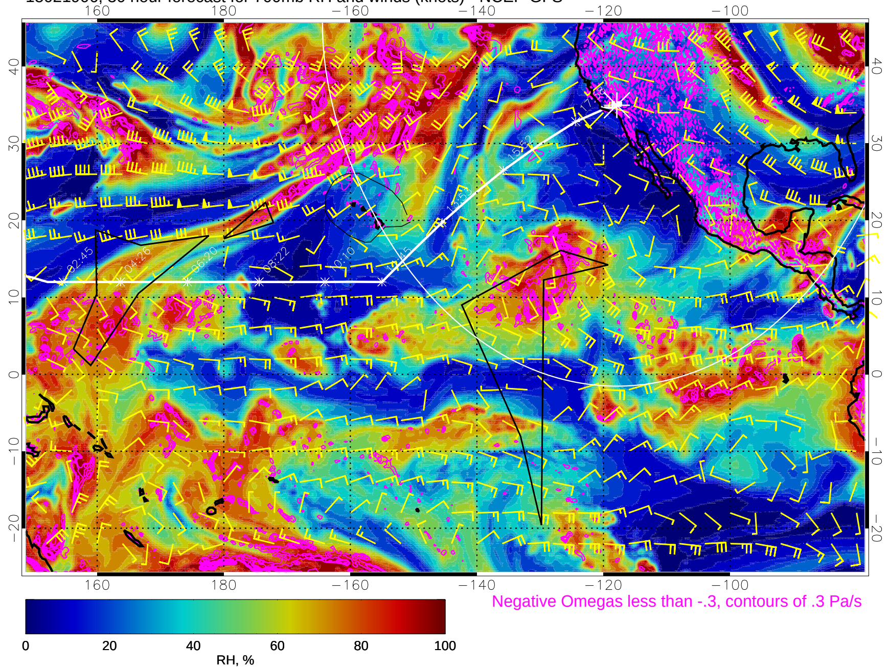
15021906, 30 hour forecast for 700mb RH and winds (knots) - NCEP GFS
