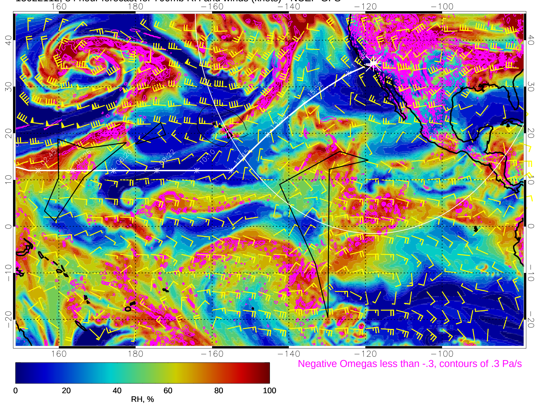
15022112, 84 hour forecast for 700mb RH and winds (knots) - NCEP GFS
