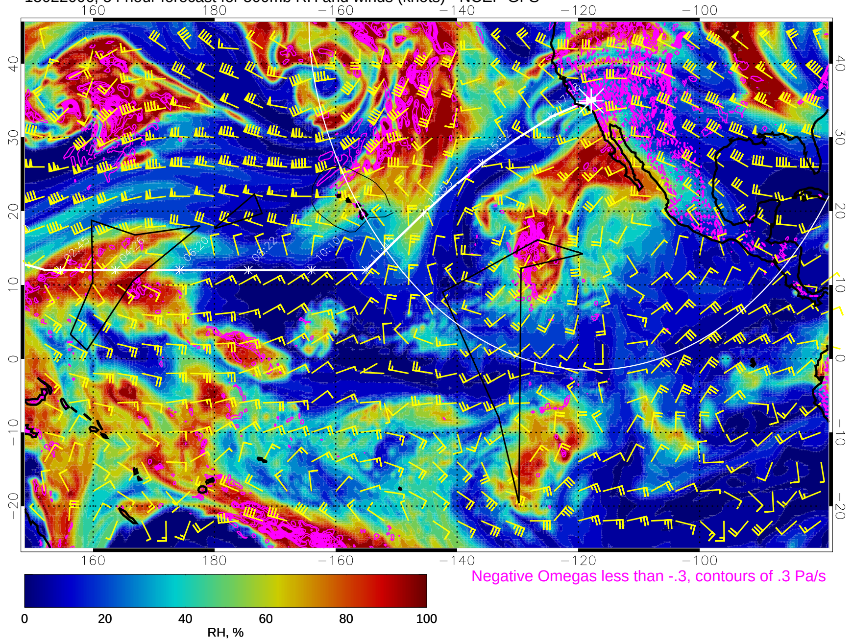
15022006, 54 hour forecast for 500mb RH and winds (knots) - NCEP GFS
