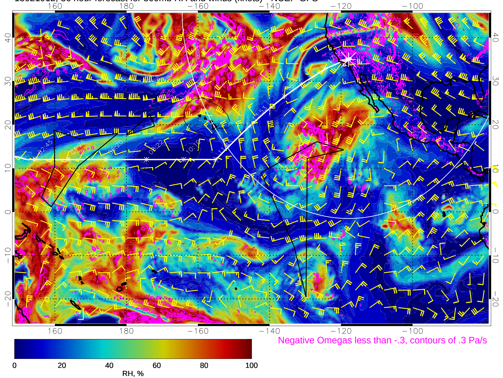
15021912, 36 hour forecast for 500mb RH and winds (knots) - NCEP GFS
