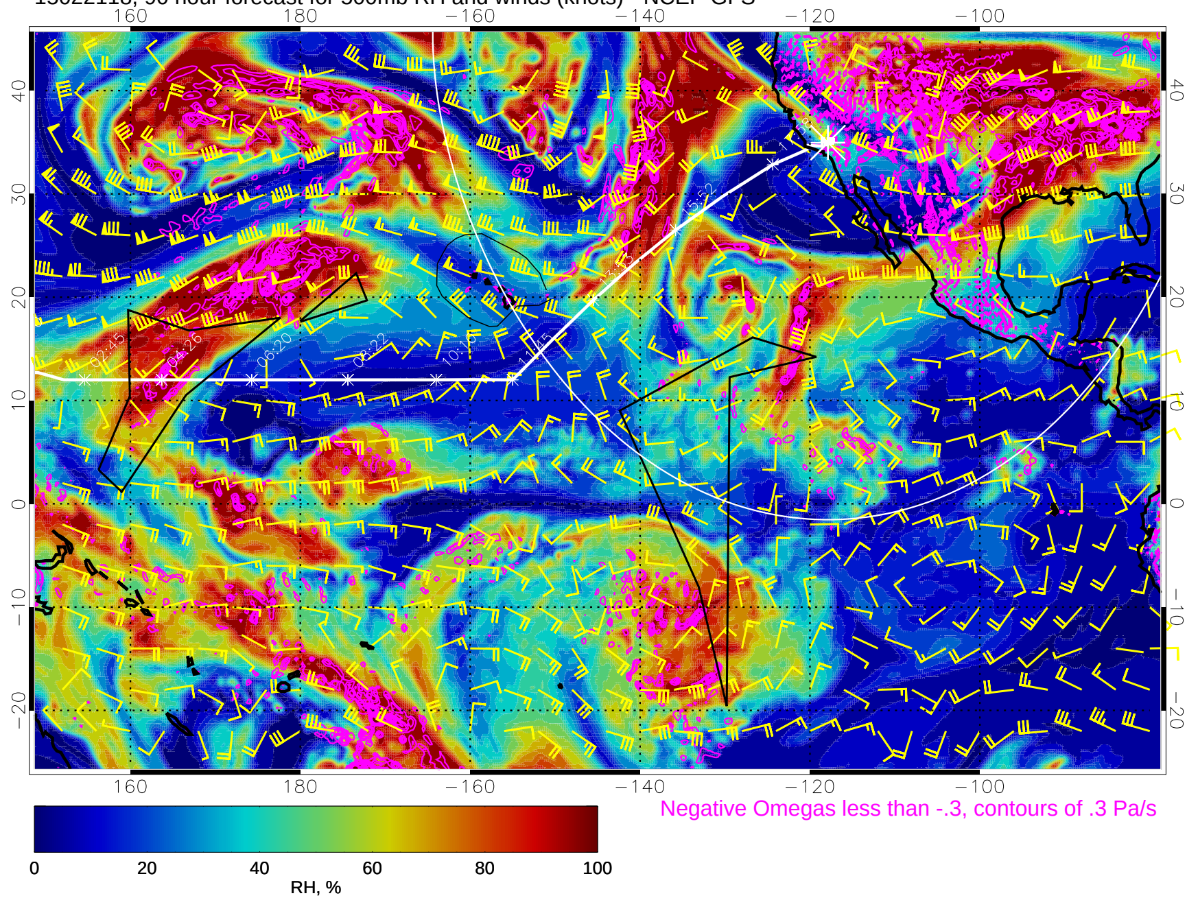
15022118, 90 hour forecast for 500mb RH and winds (knots) - NCEP GFS
