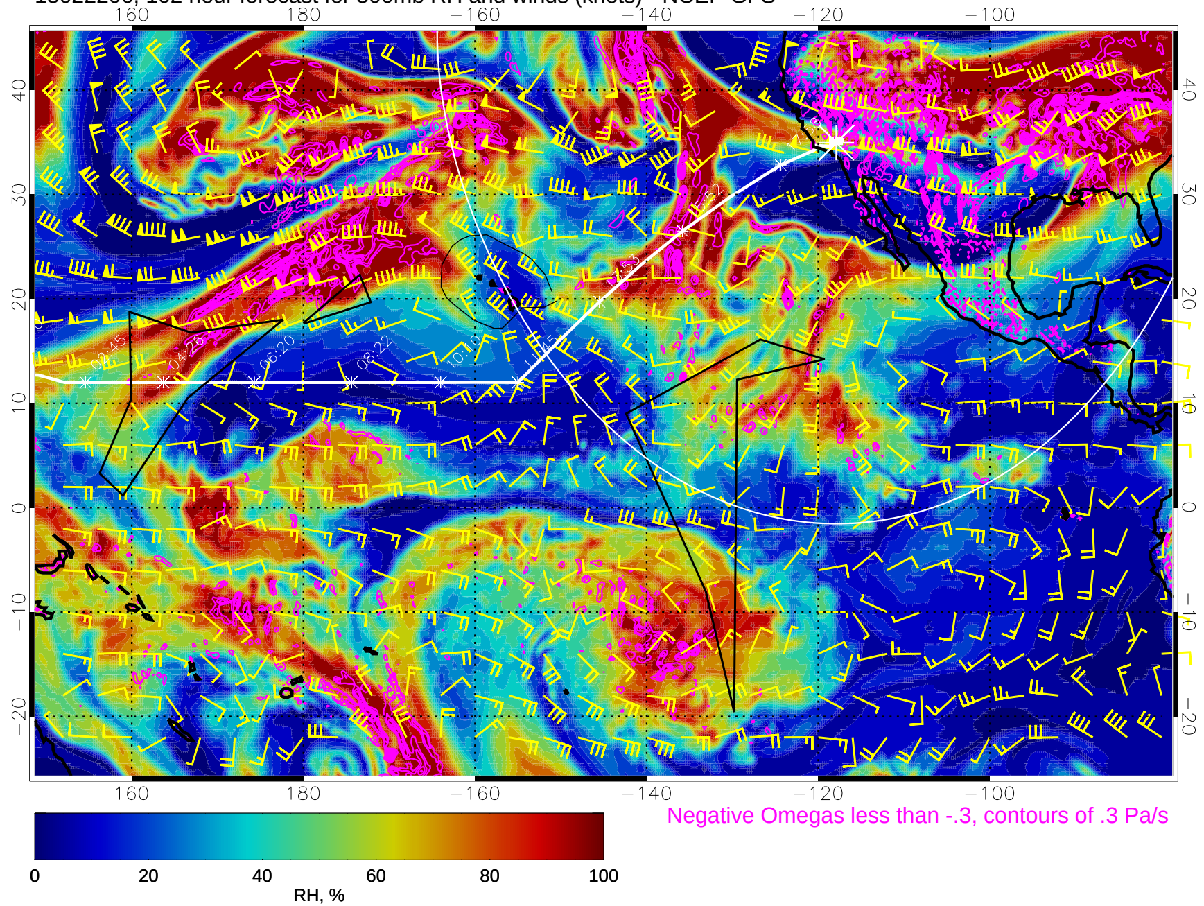
15022206, 102 hour forecast for 500mb RH and winds (knots) - NCEP GFS
