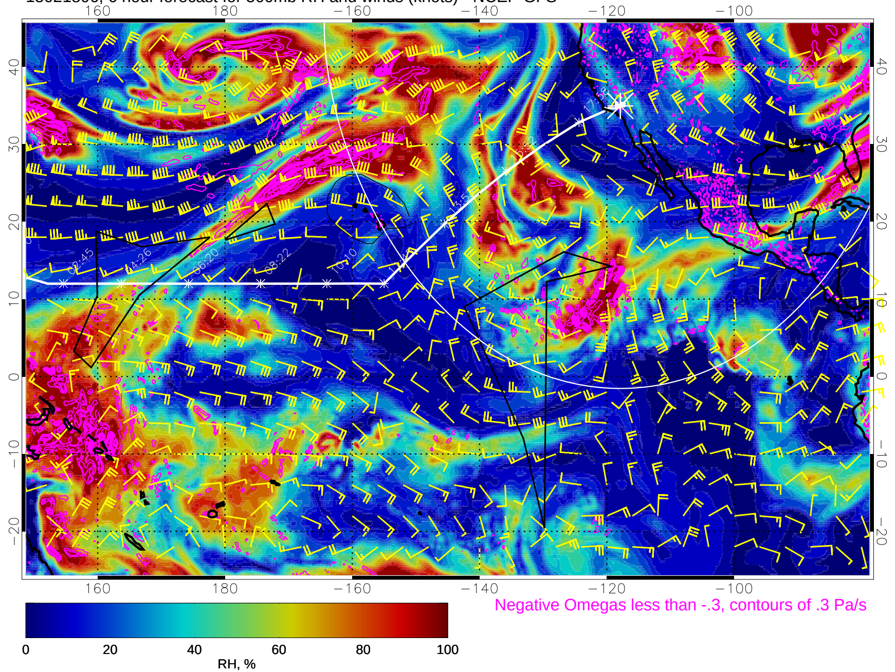
15021806, 6 hour forecast for 500mb RH and winds (knots) - NCEP GFS
