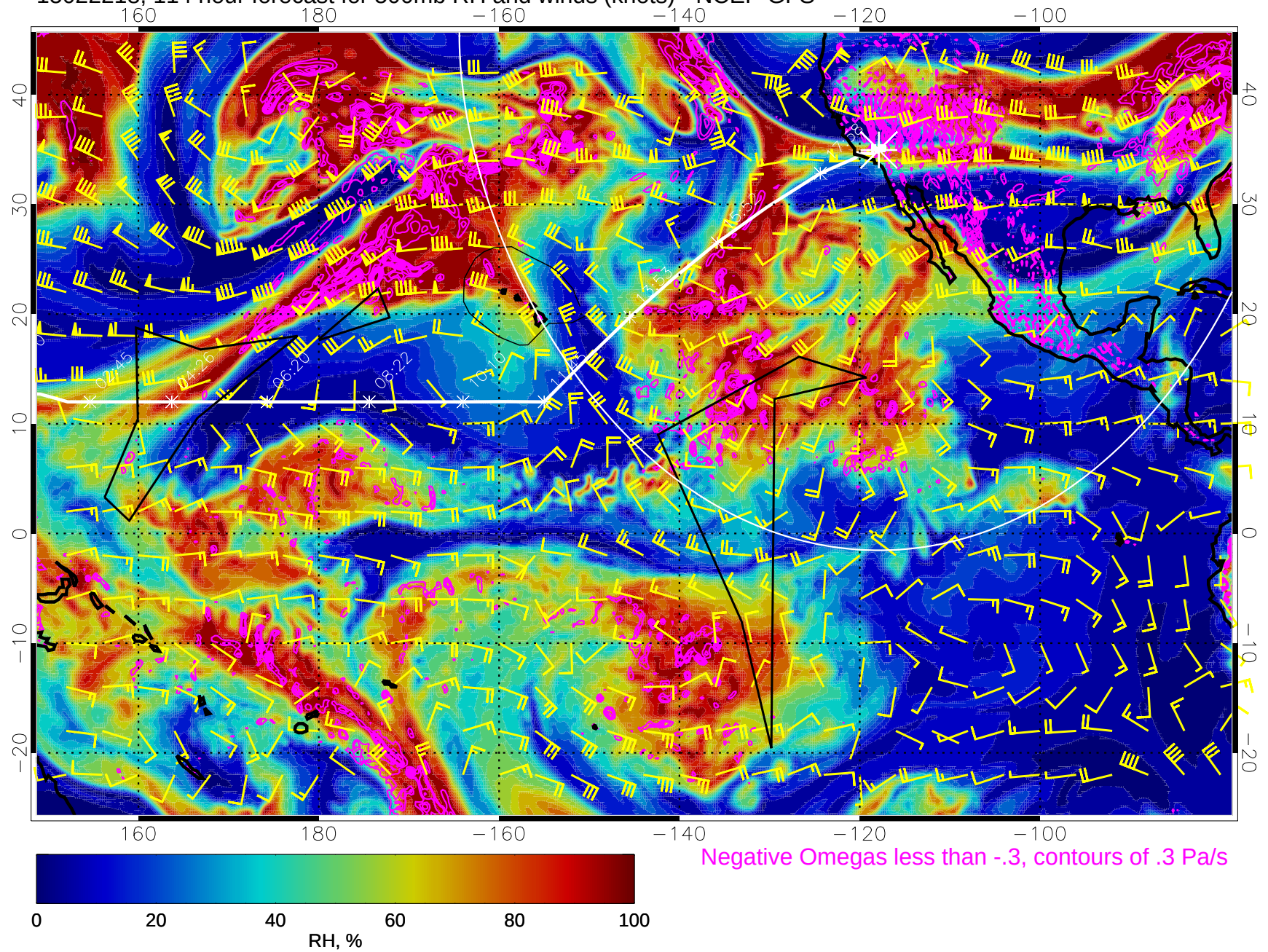
15022218, 114 hour forecast for 500mb RH and winds (knots) - NCEP GFS
