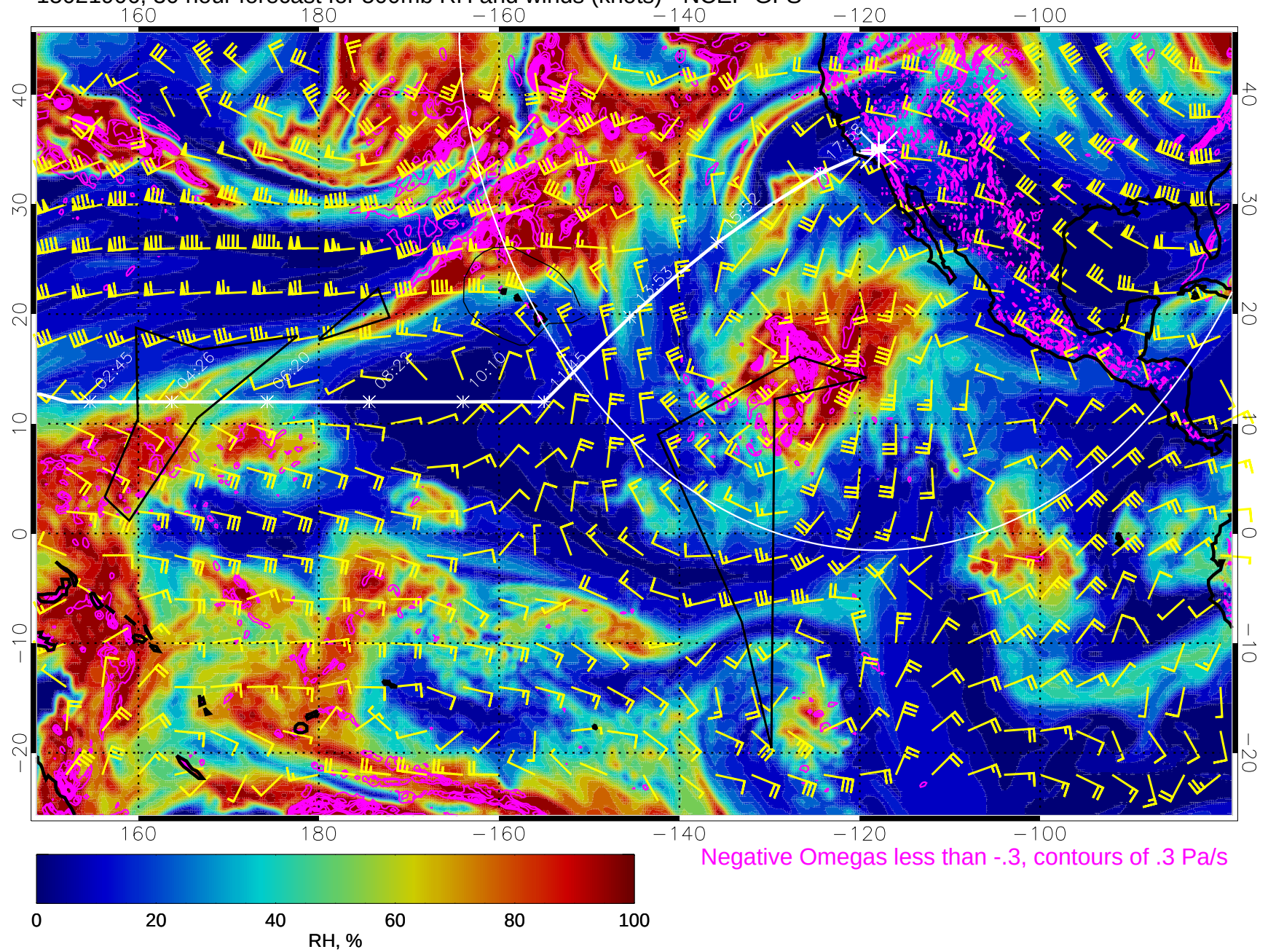
15021906, 30 hour forecast for 500mb RH and winds (knots) - NCEP GFS
