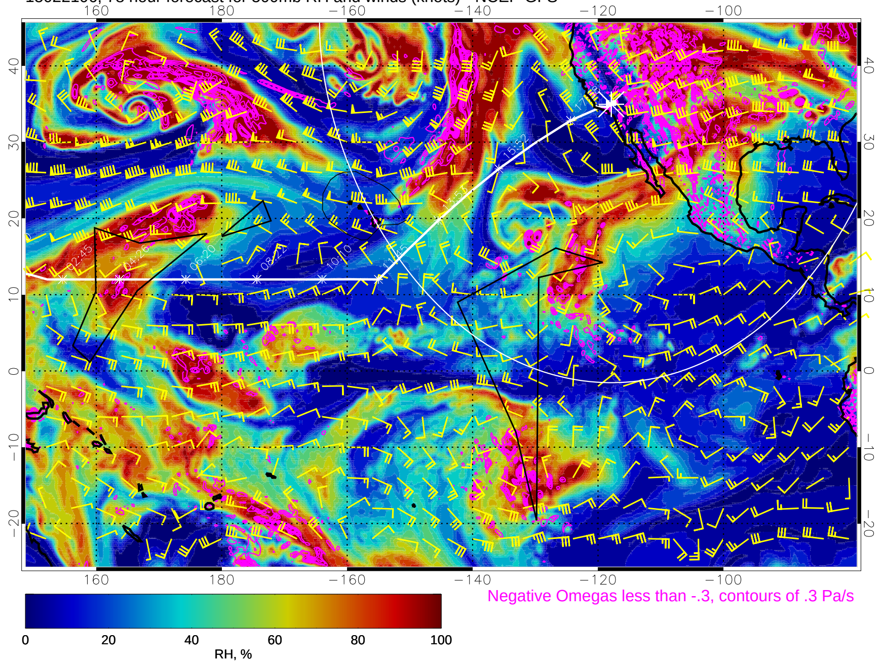
15022106, 78 hour forecast for 500mb RH and winds (knots) - NCEP GFS
