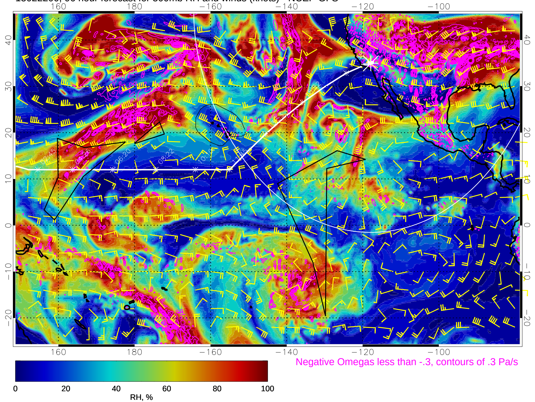
15022200, 96 hour forecast for 500mb RH and winds (knots) - NCEP GFS
