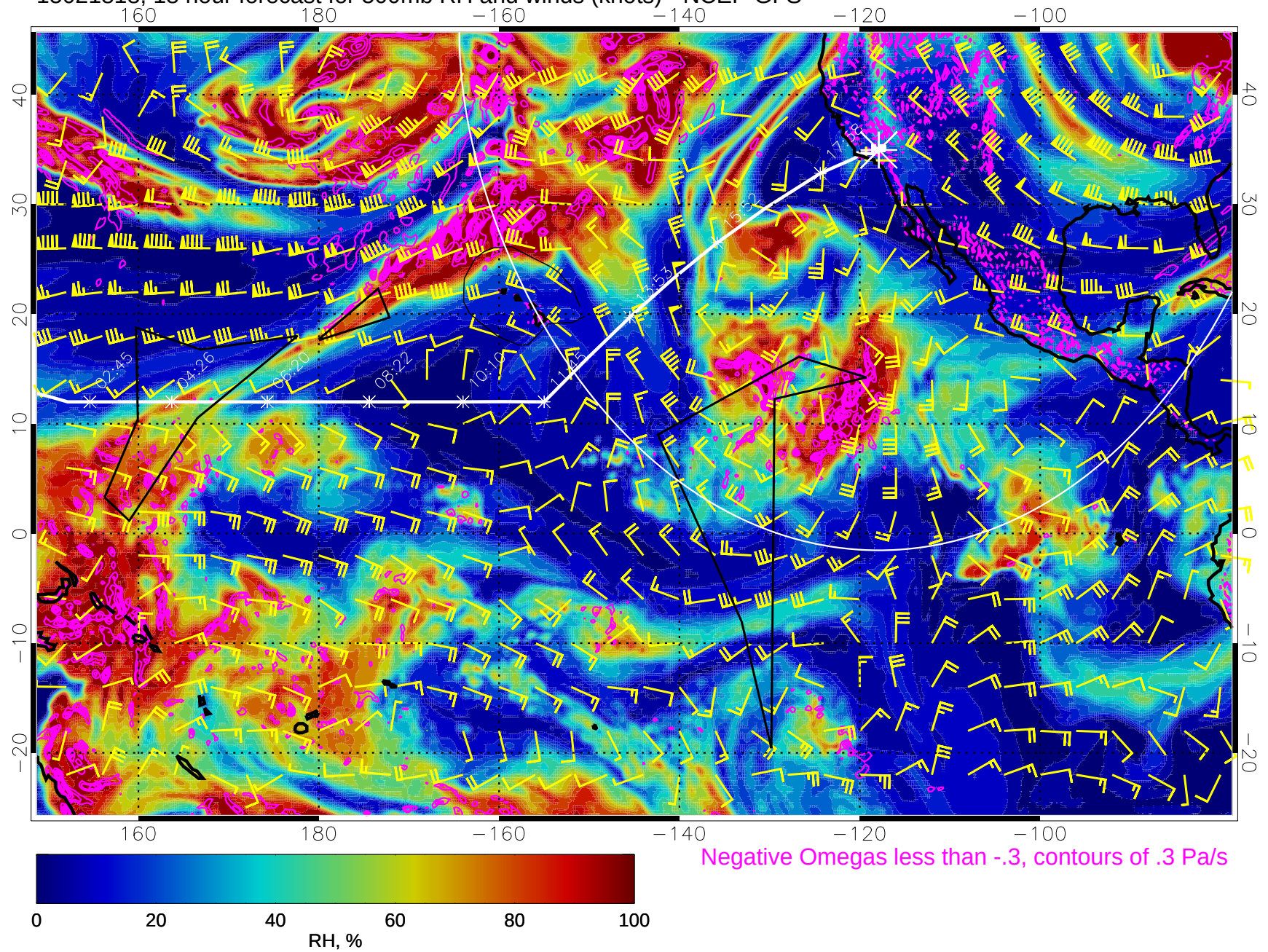
15021818, 18 hour forecast for 500mb RH and winds (knots) - NCEP GFS
