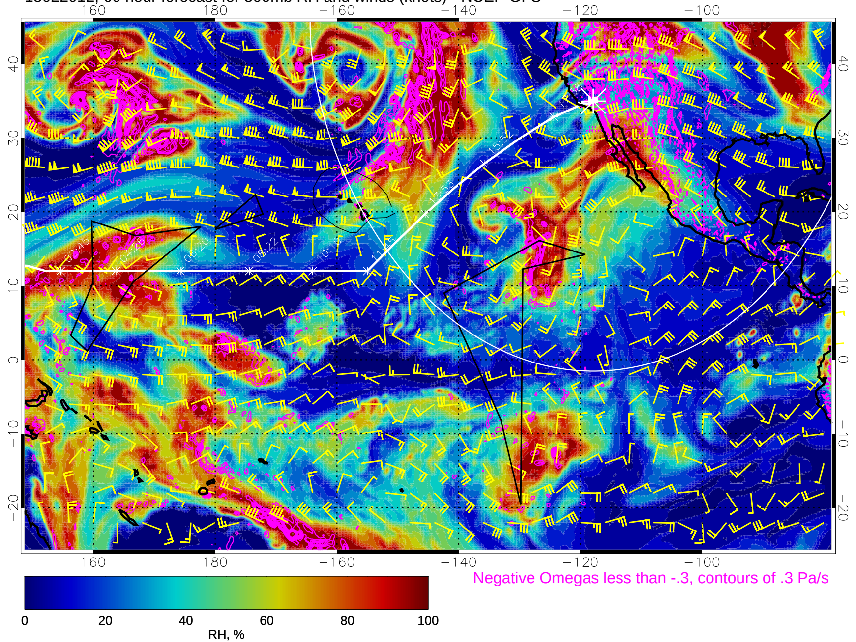
15022012, 60 hour forecast for 500mb RH and winds (knots) - NCEP GFS
