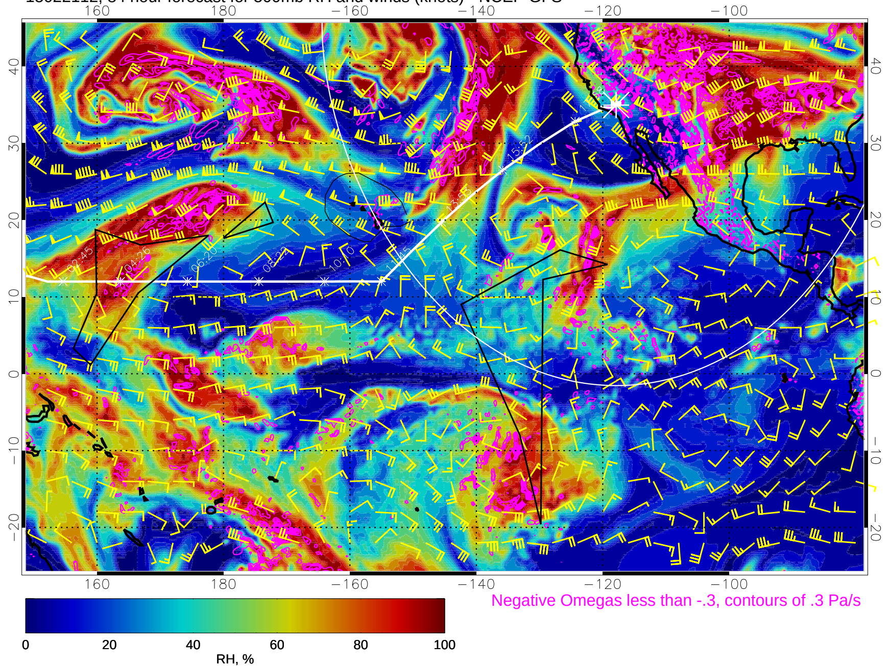
15022112, 84 hour forecast for 500mb RH and winds (knots) - NCEP GFS
