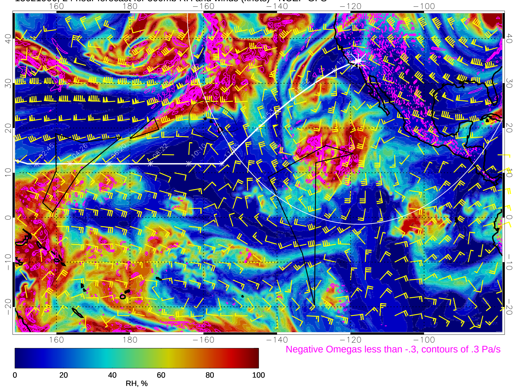
15021900, 24 hour forecast for 500mb RH and winds (knots) - NCEP GFS
