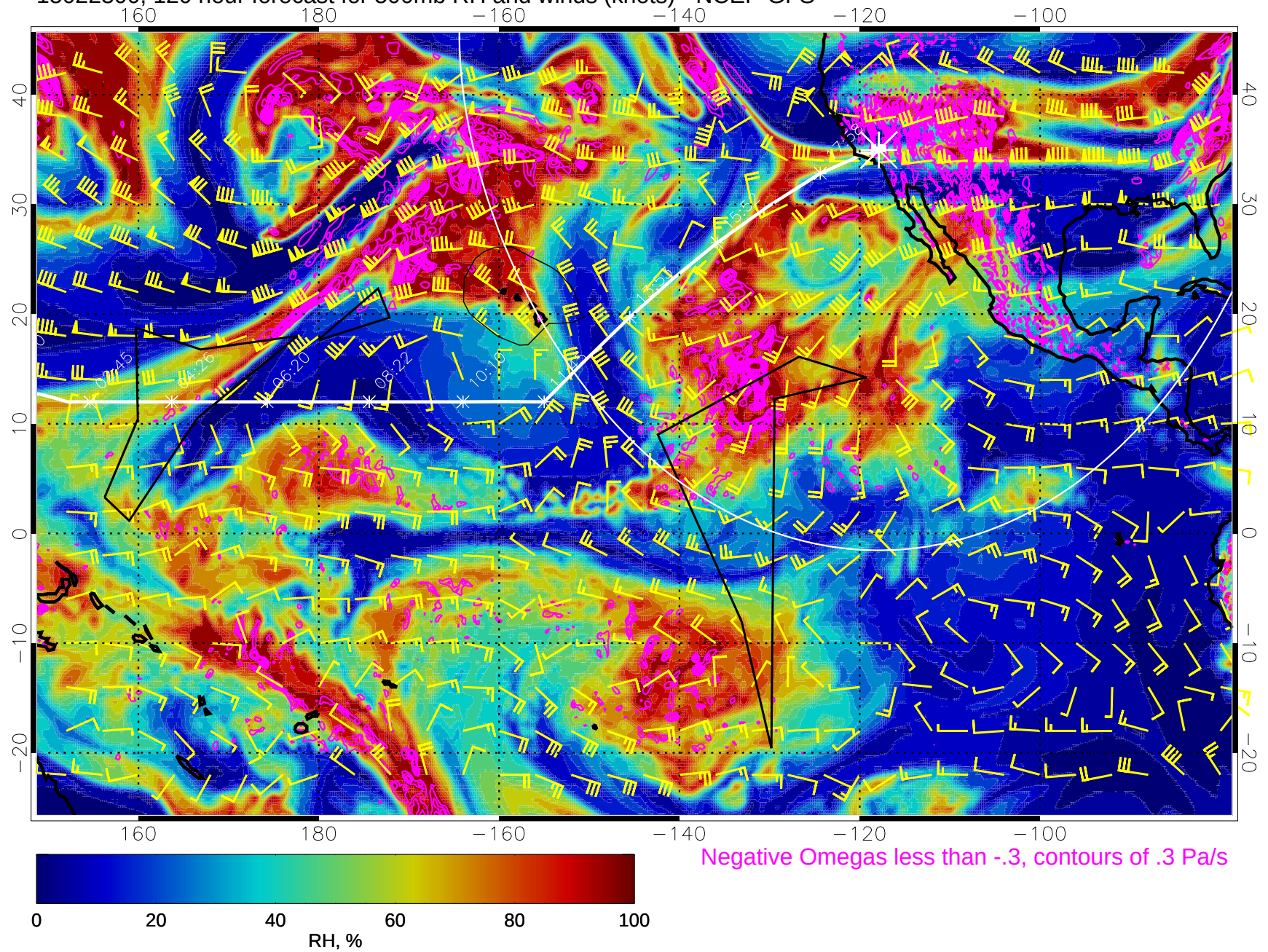
15022300, 120 hour forecast for 500mb RH and winds (knots) - NCEP GFS
