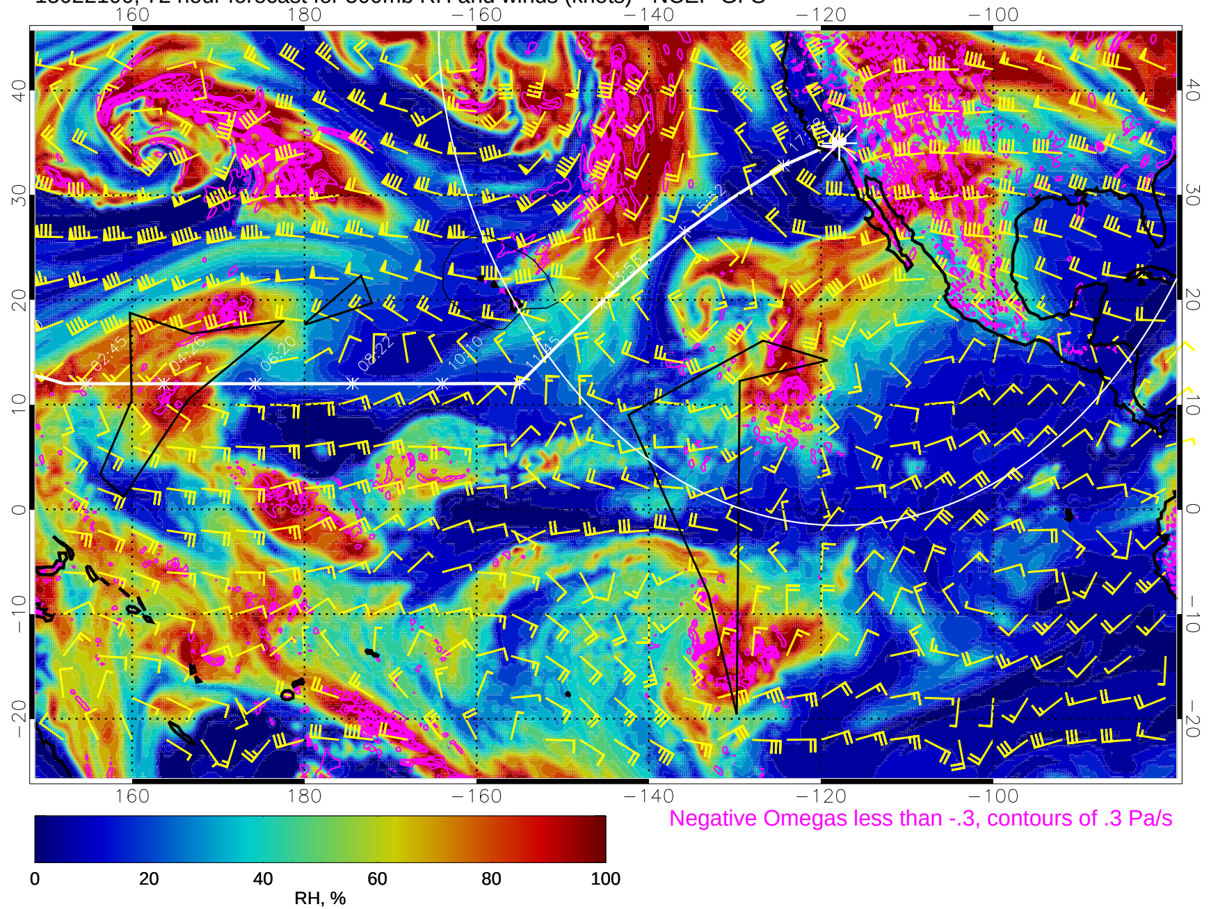
15022100, 72 hour forecast for 500mb RH and winds (knots) - NCEP GFS
