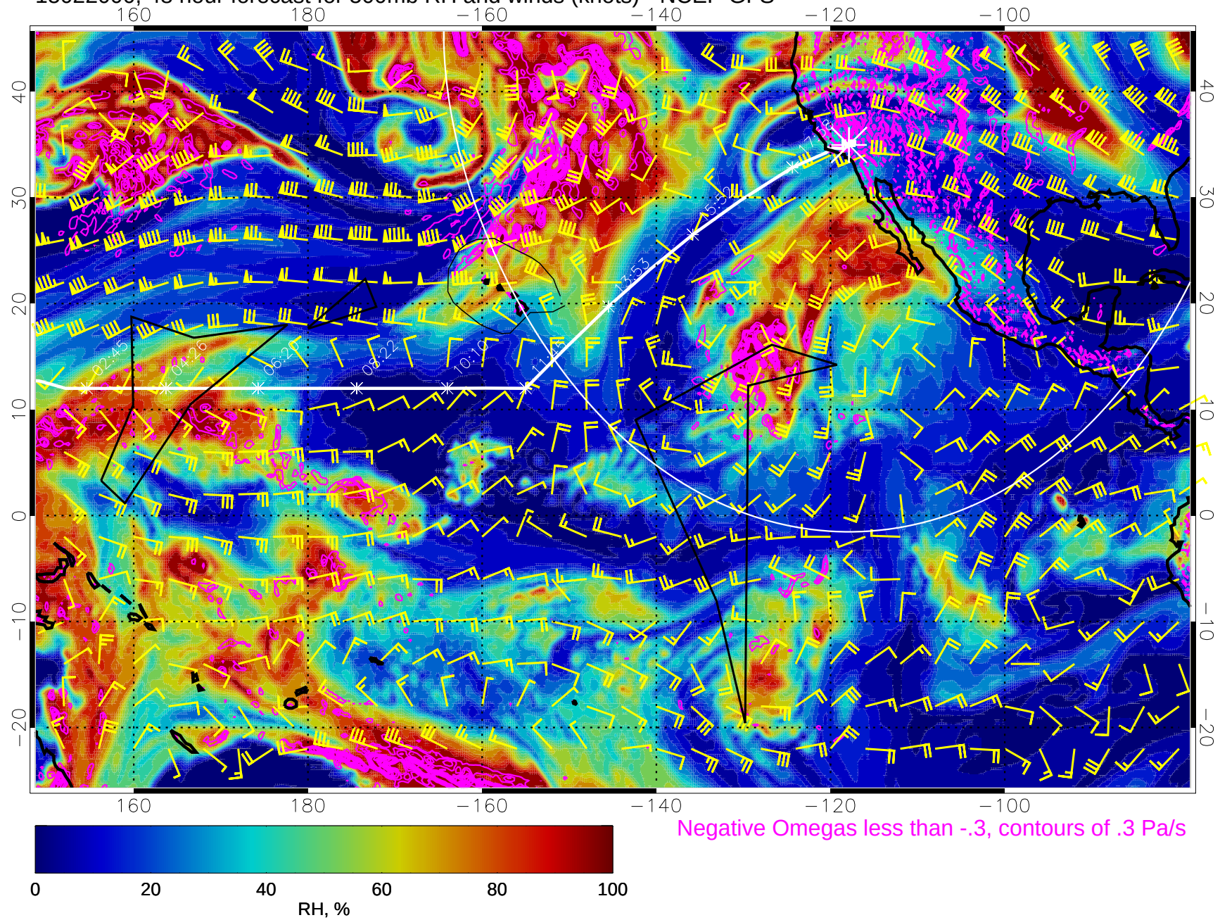
15022000, 48 hour forecast for 500mb RH and winds (knots) - NCEP GFS
