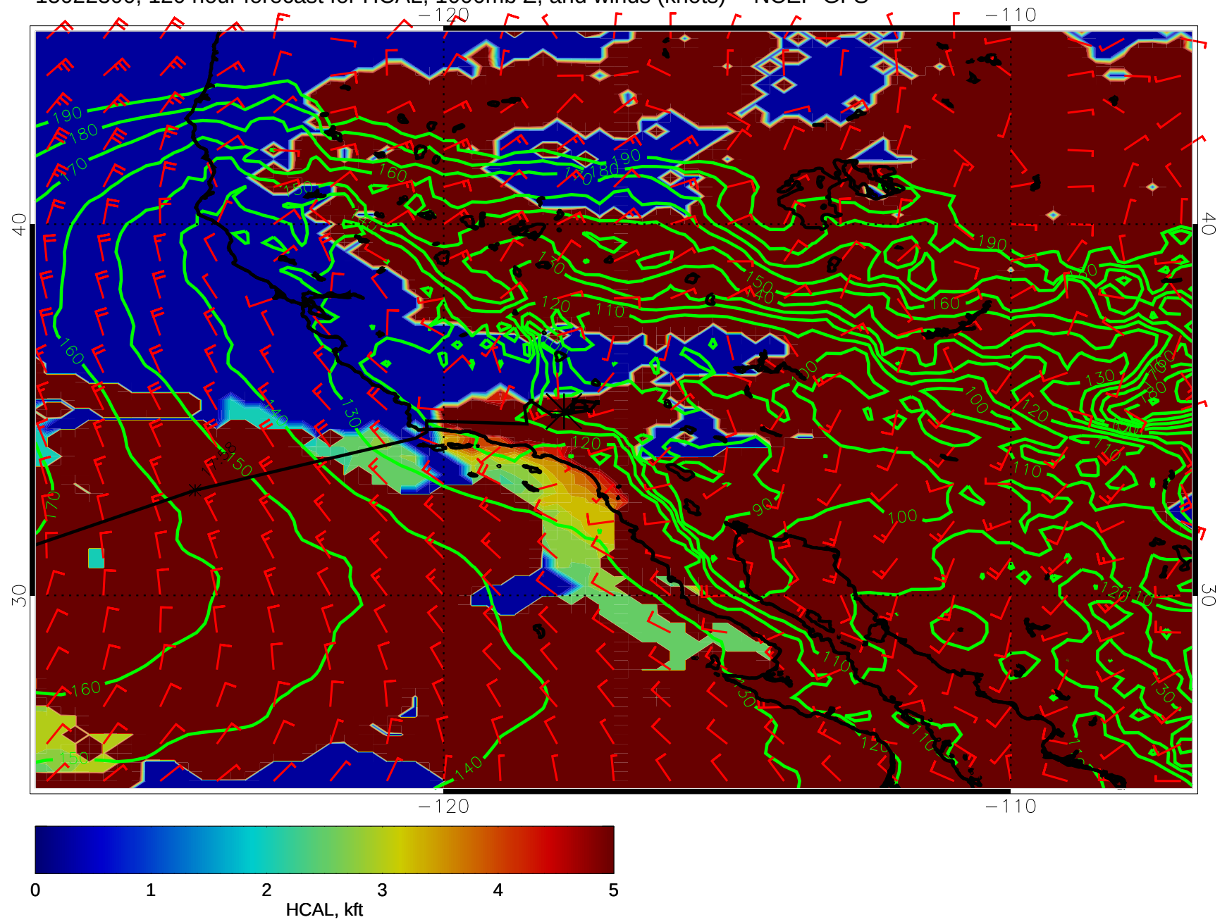
15022300, 120 hour forecast for HCAL, 1000mb Z, and winds (knots) -- NCEP GFS
