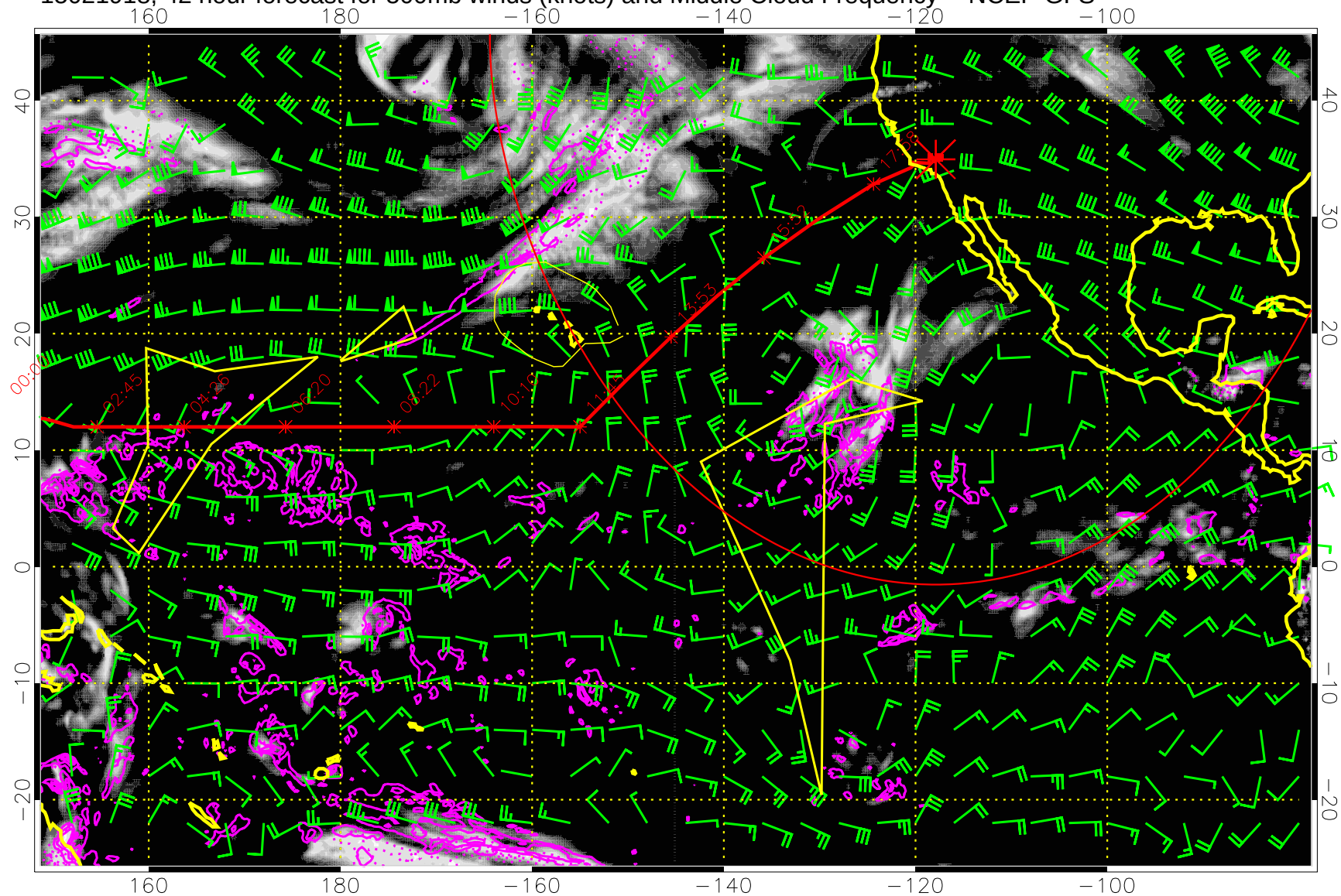
15021918, 42 hour forecast for 500mb winds (knots) and Middle Cloud Frequency -- NCEP GFS
