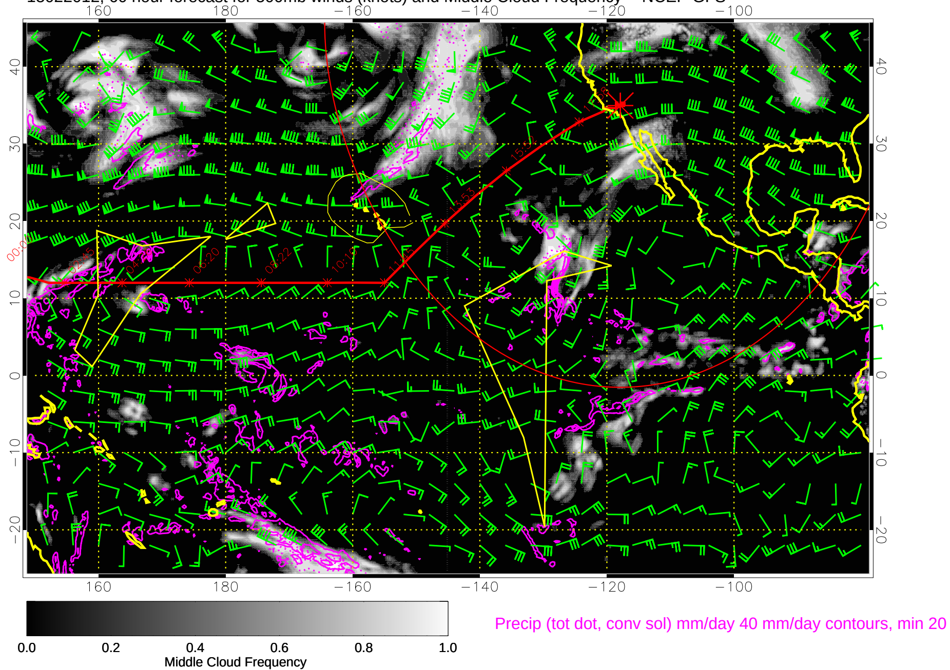
15022012, 60 hour forecast for 500mb winds (knots) and Middle Cloud Frequency -- NCEP GFS
