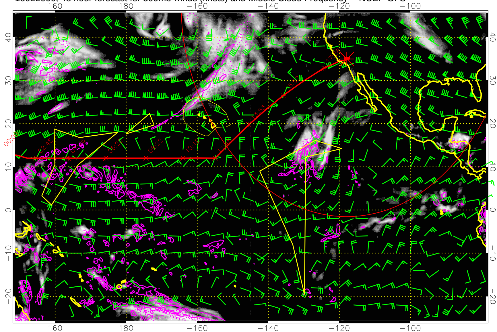
15022000, 48 hour forecast for 500mb winds (knots) and Middle Cloud Frequency -- NCEP GFS
