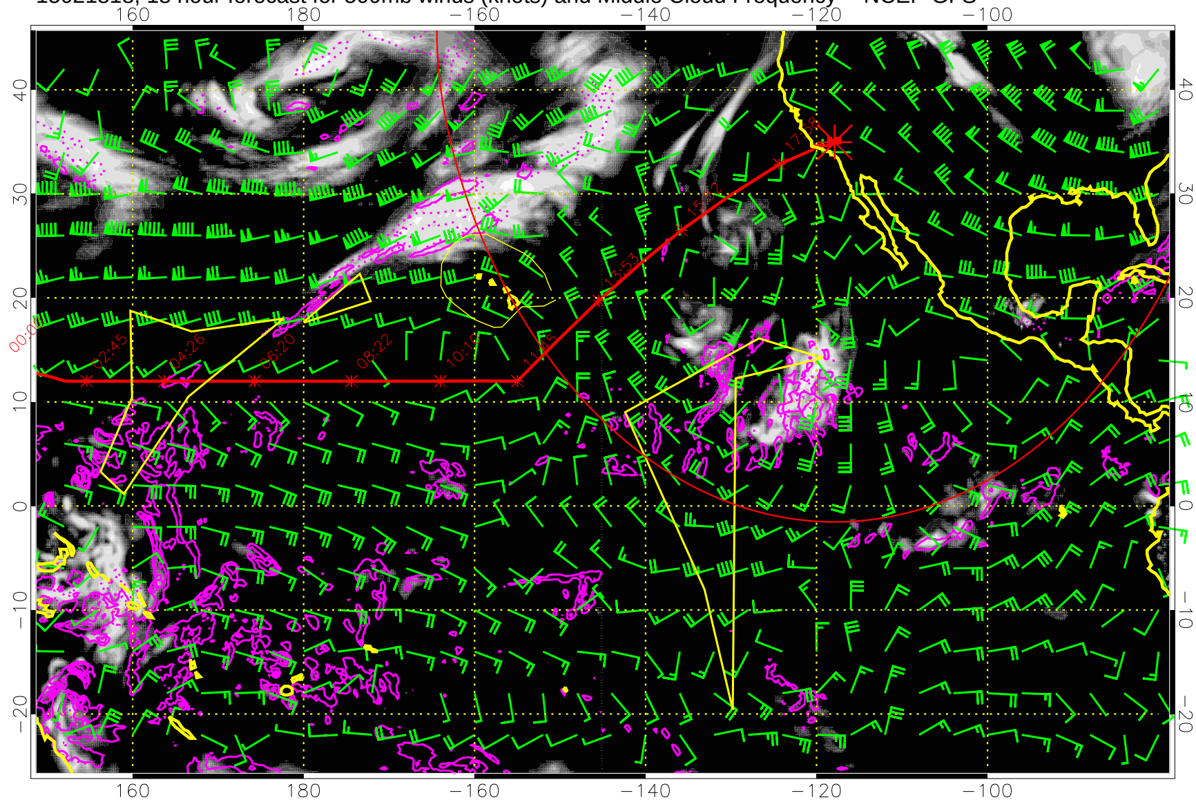
15021818, 18 hour forecast for 500mb winds (knots) and Middle Cloud Frequency -- NCEP GFS
