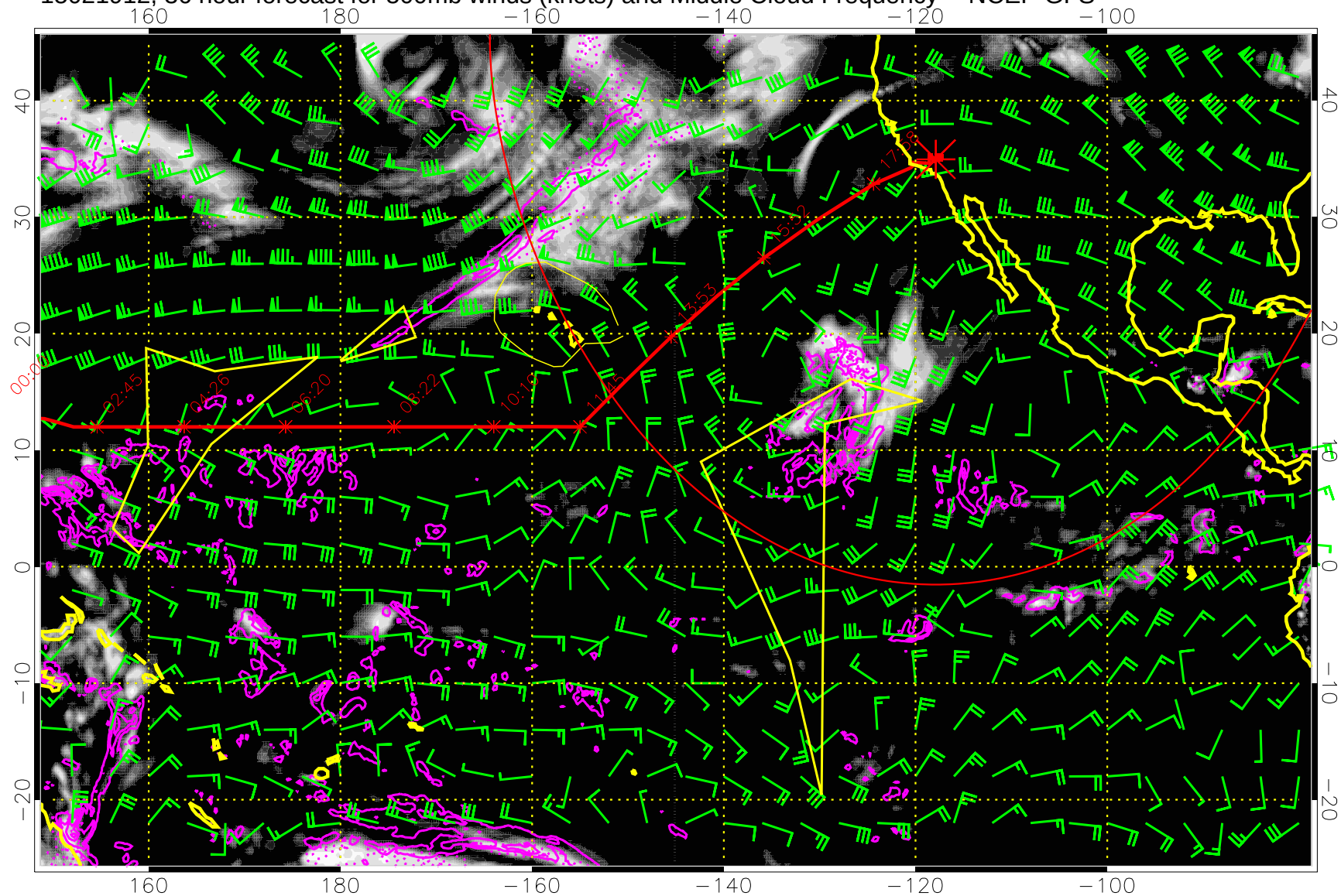
15021912, 36 hour forecast for 500mb winds (knots) and Middle Cloud Frequency -- NCEP GFS
