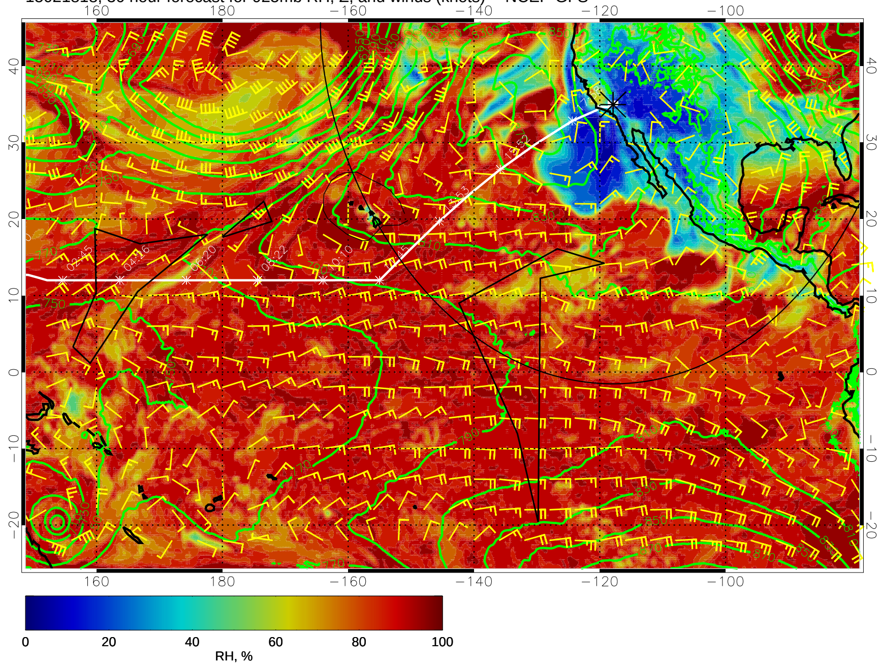
15021818, 30 hour forecast for 925mb RH, Z, and winds (knots) -- NCEP GFS
