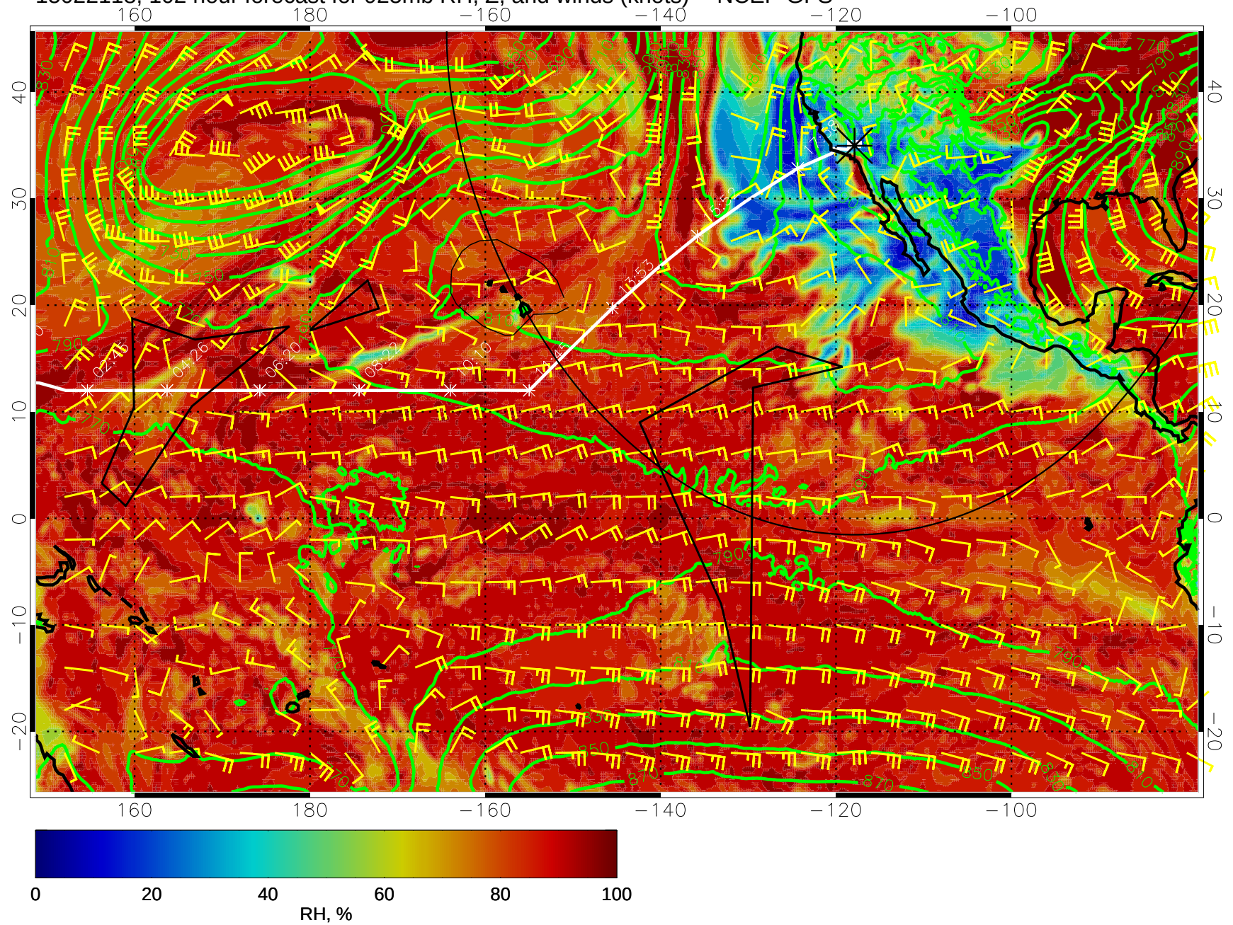
15022118, 102 hour forecast for 925mb RH, Z, and winds (knots) -- NCEP GFS
