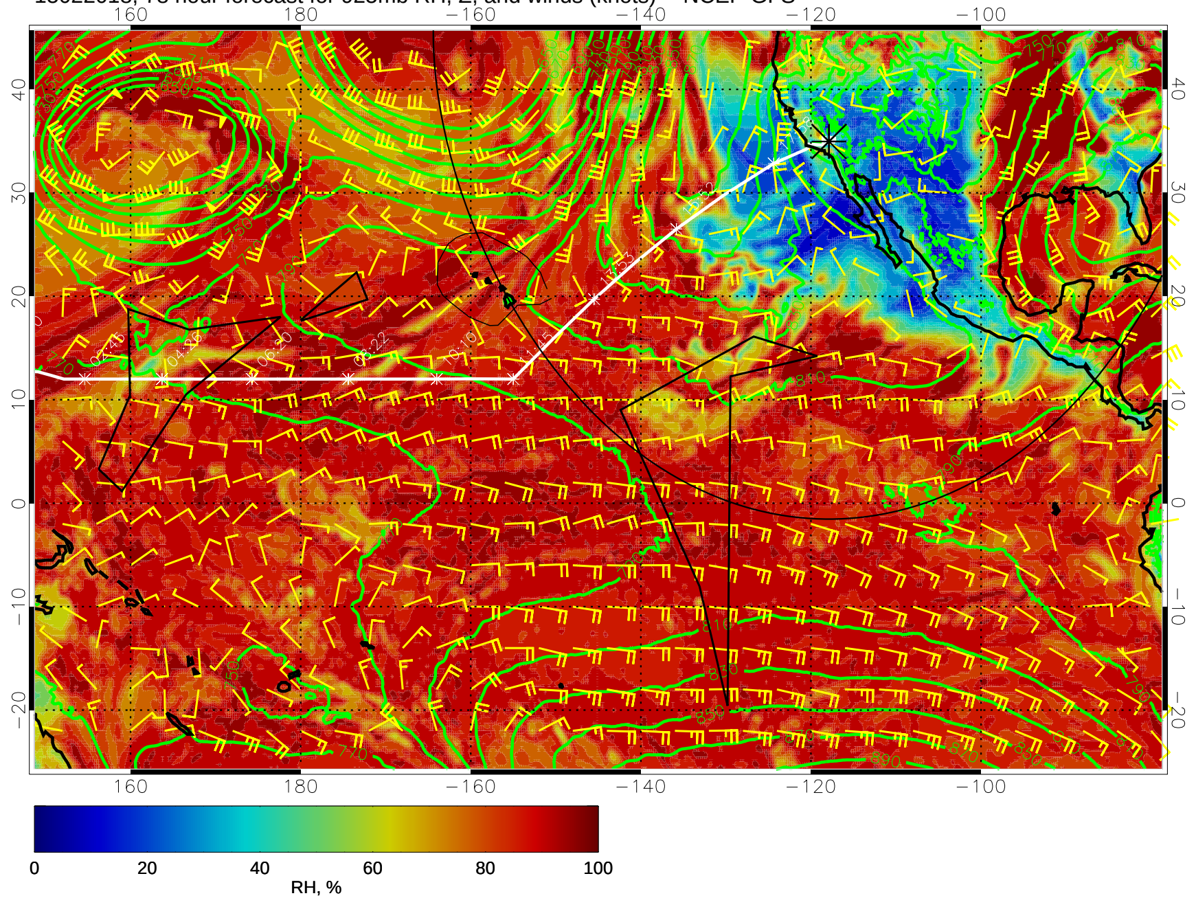
15022018, 78 hour forecast for 925mb RH, Z, and winds (knots) -- NCEP GFS
