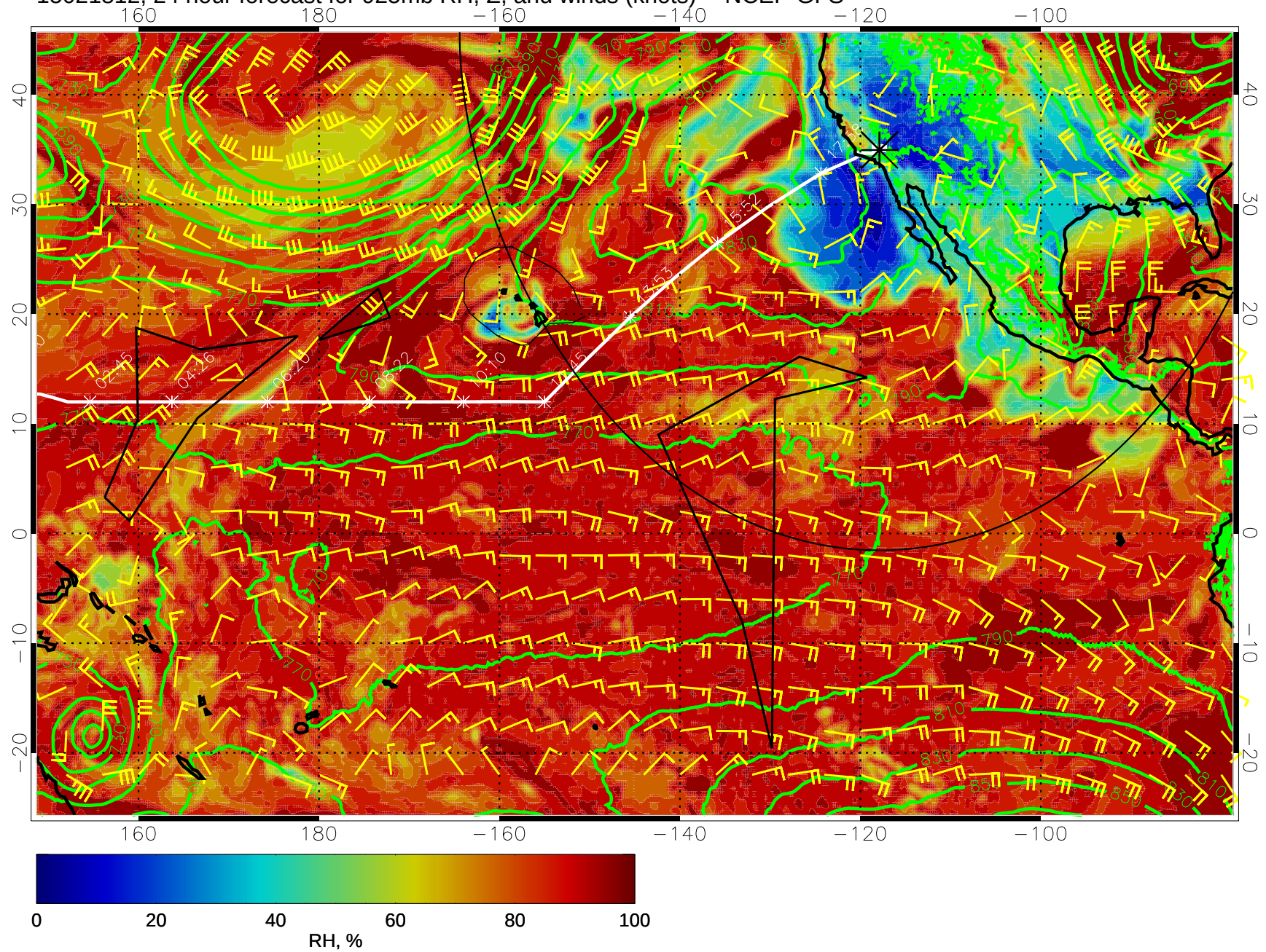
15021812, 24 hour forecast for 925mb RH, Z, and winds (knots) -- NCEP GFS
