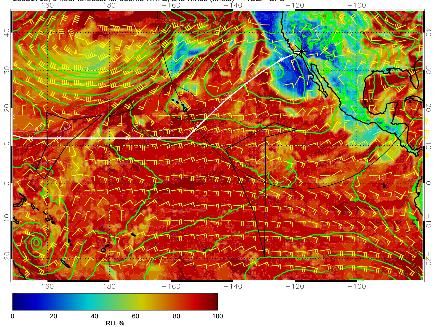
15021718, 6 hour forecast for 925mb RH, Z, and winds (knots) -- NCEP GFS
