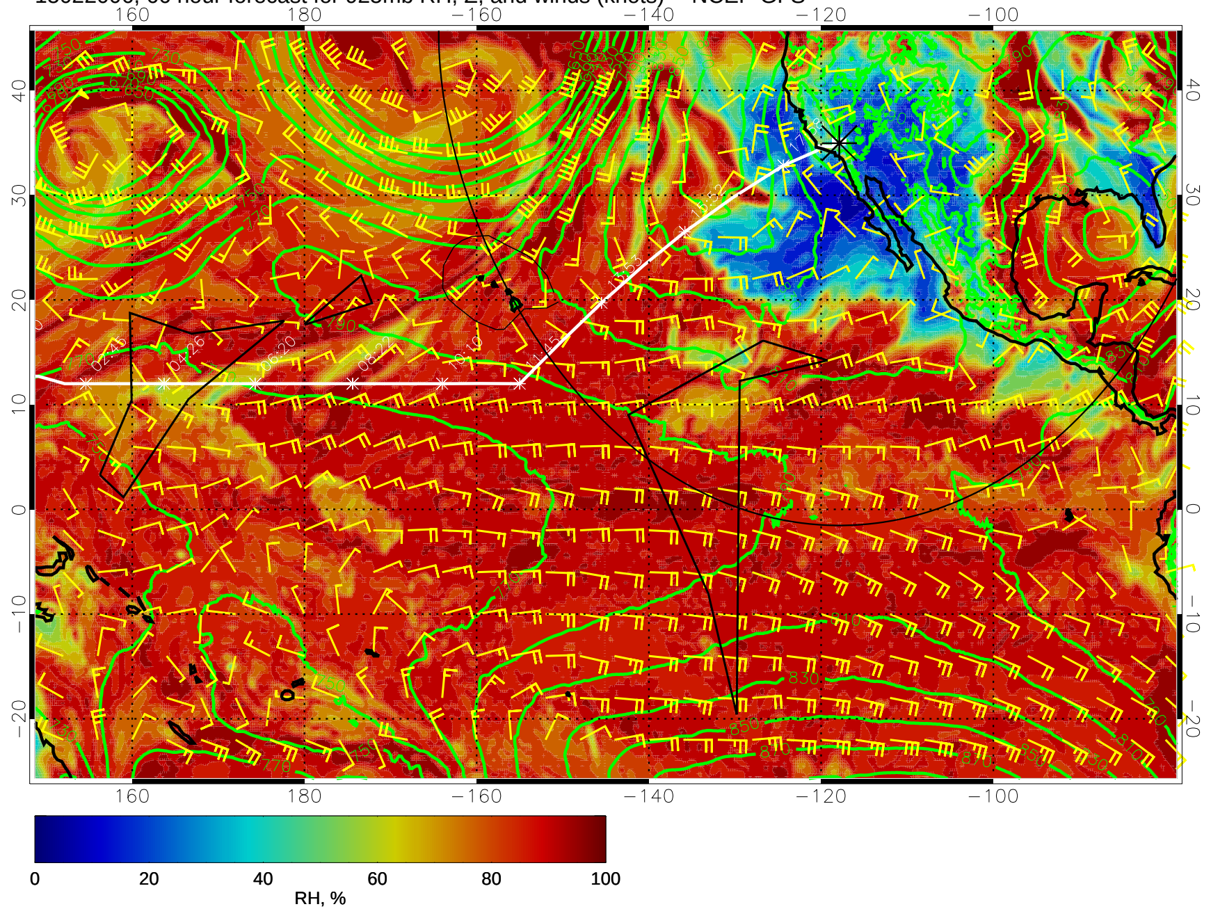
15022006, 66 hour forecast for 925mb RH, Z, and winds (knots) -- NCEP GFS
