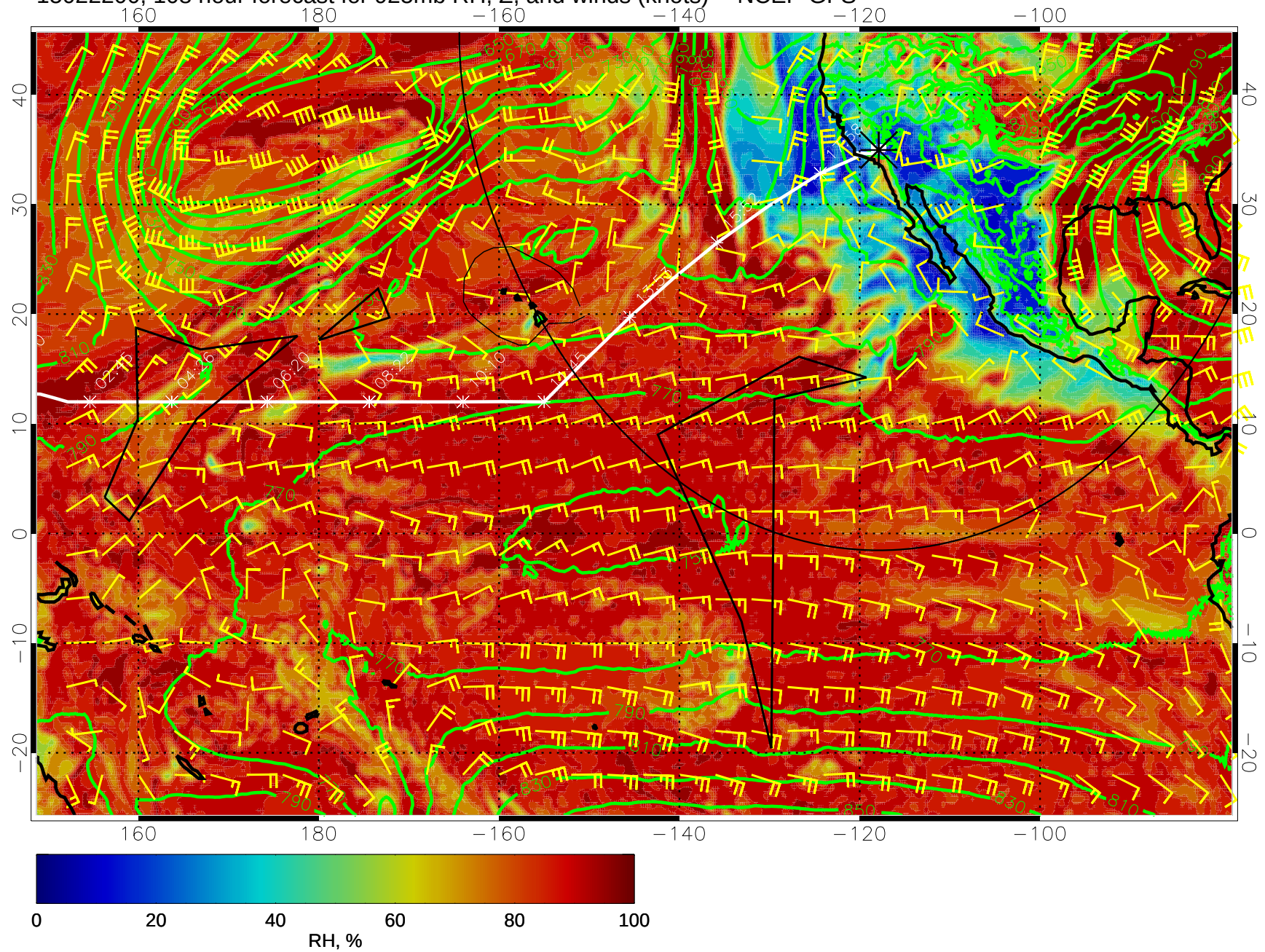
15022200, 108 hour forecast for 925mb RH, Z, and winds (knots) -- NCEP GFS
