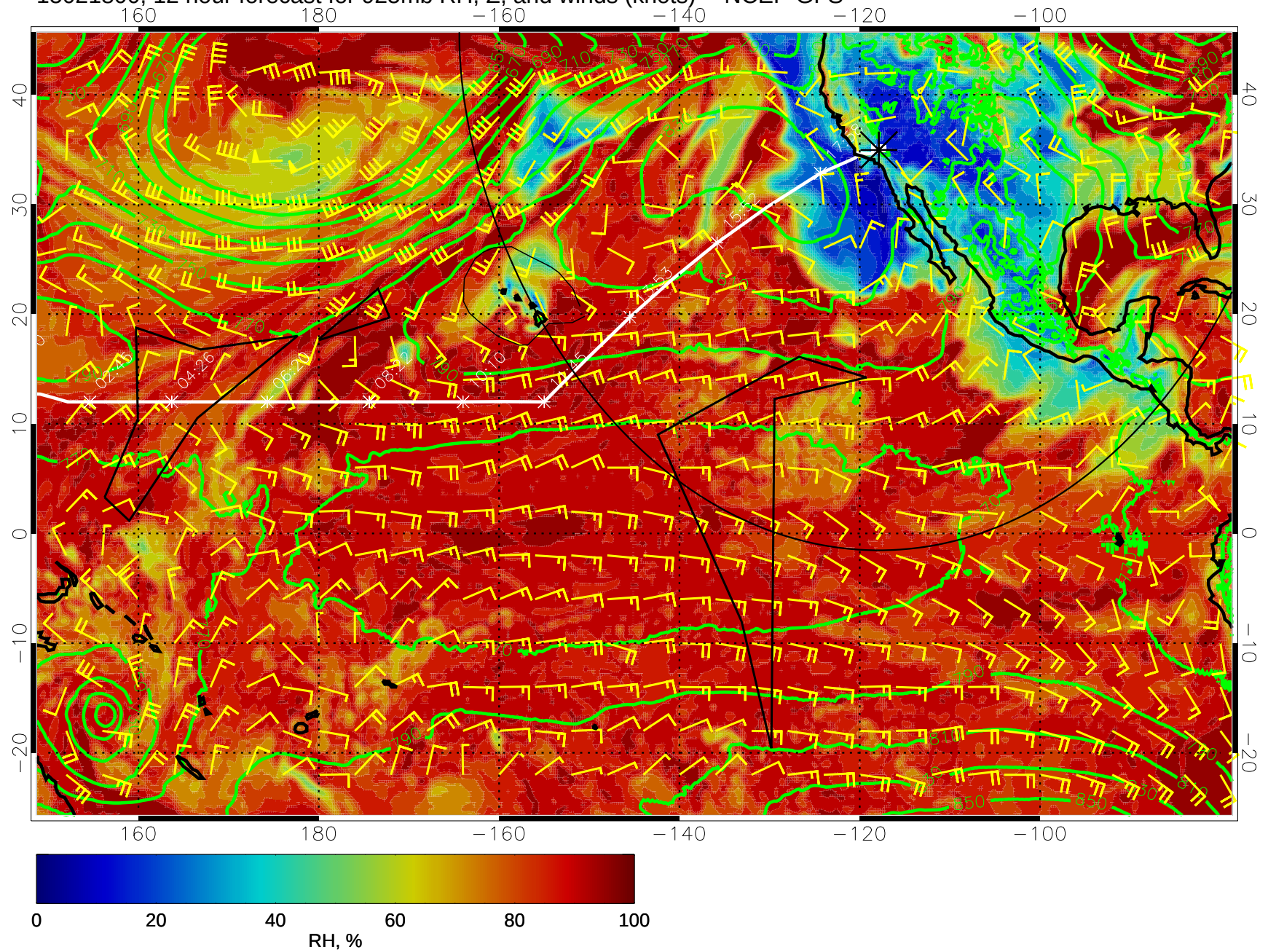
15021800, 12 hour forecast for 925mb RH, Z, and winds (knots) -- NCEP GFS
