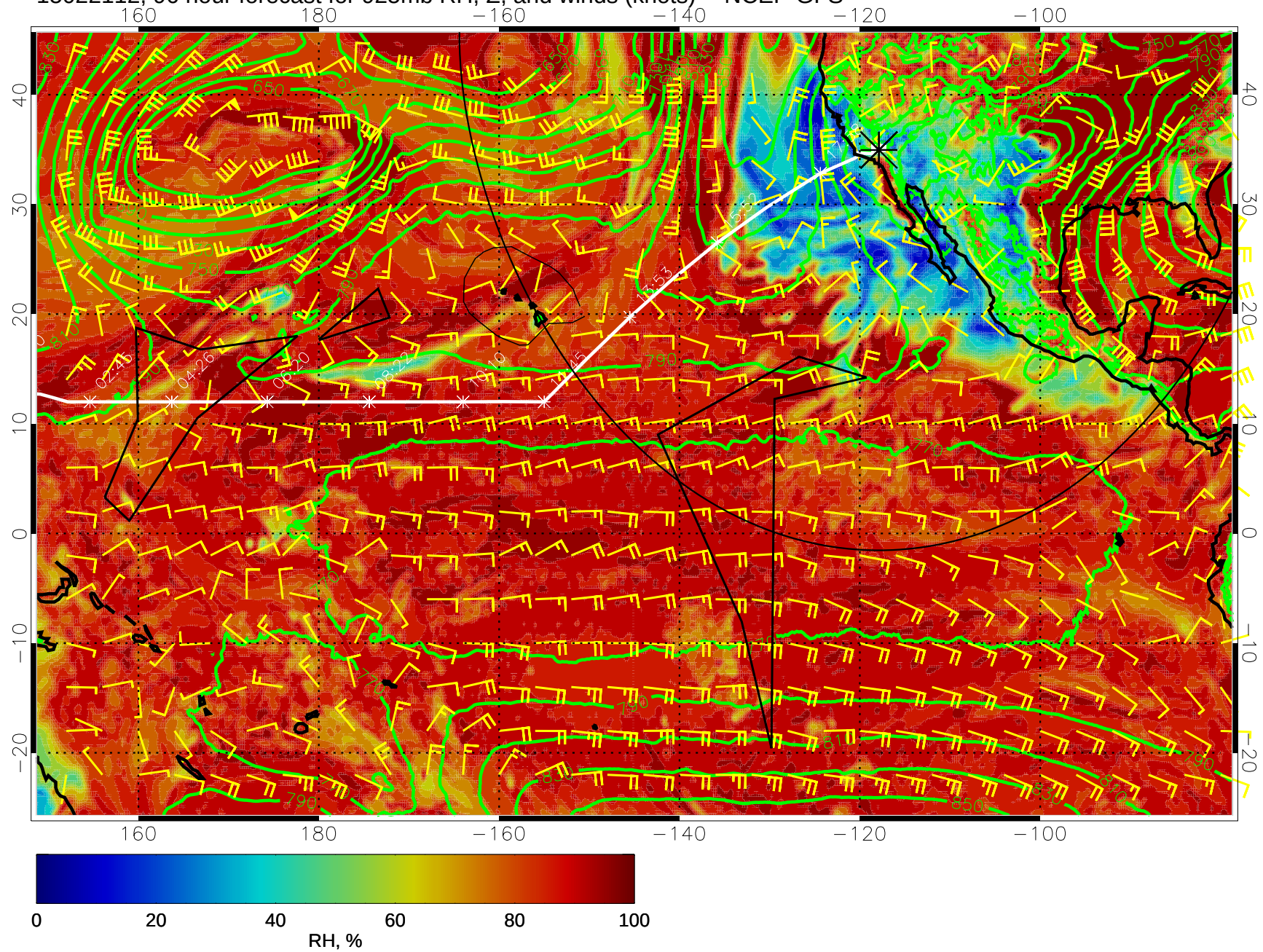
15022112, 96 hour forecast for 925mb RH, Z, and winds (knots) -- NCEP GFS
