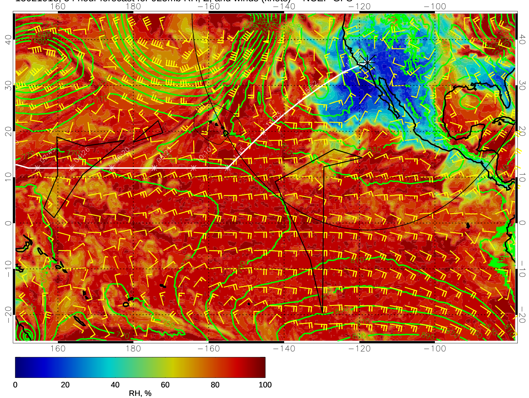
15021918, 54 hour forecast for 925mb RH, Z, and winds (knots) -- NCEP GFS
