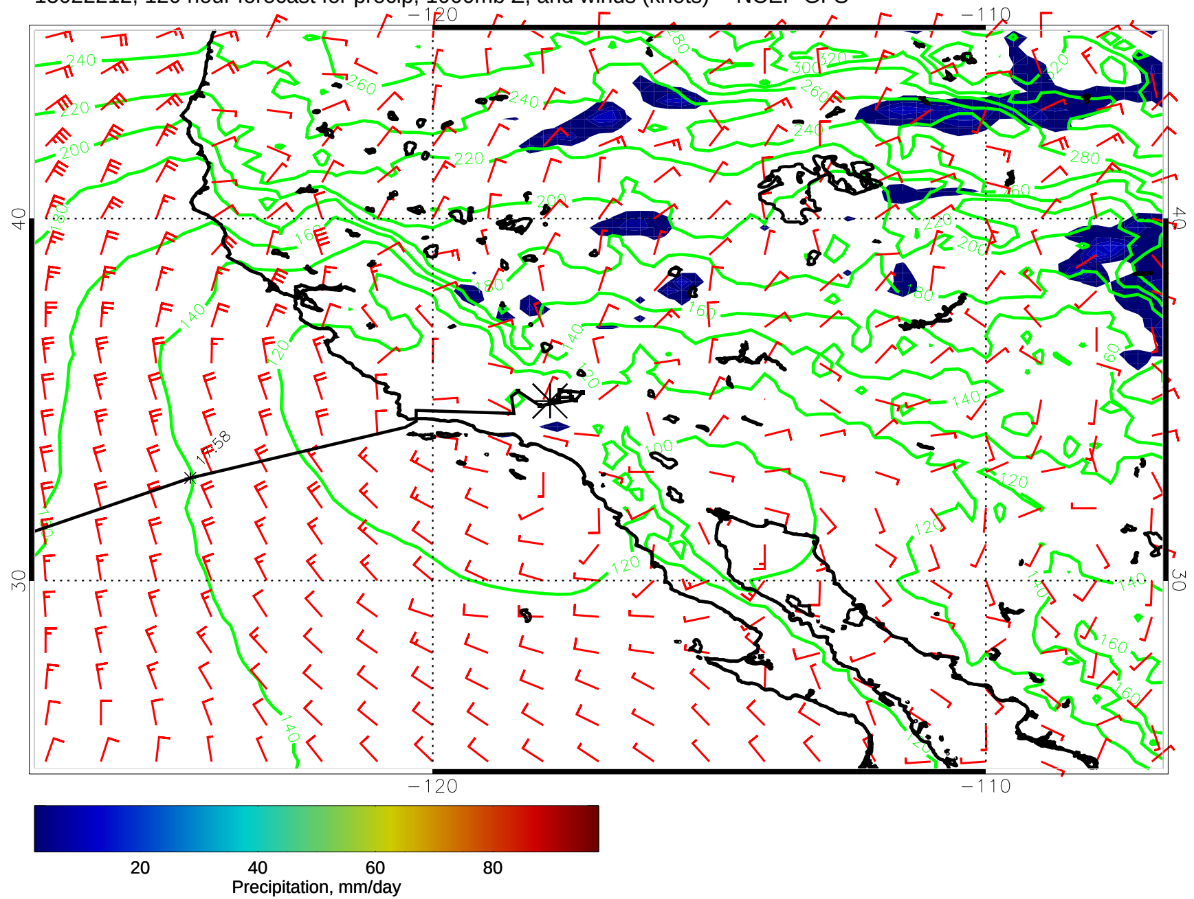
15022212, 120 hour forecast for precip, 1000mb Z, and winds (knots) -- NCEP GFS
