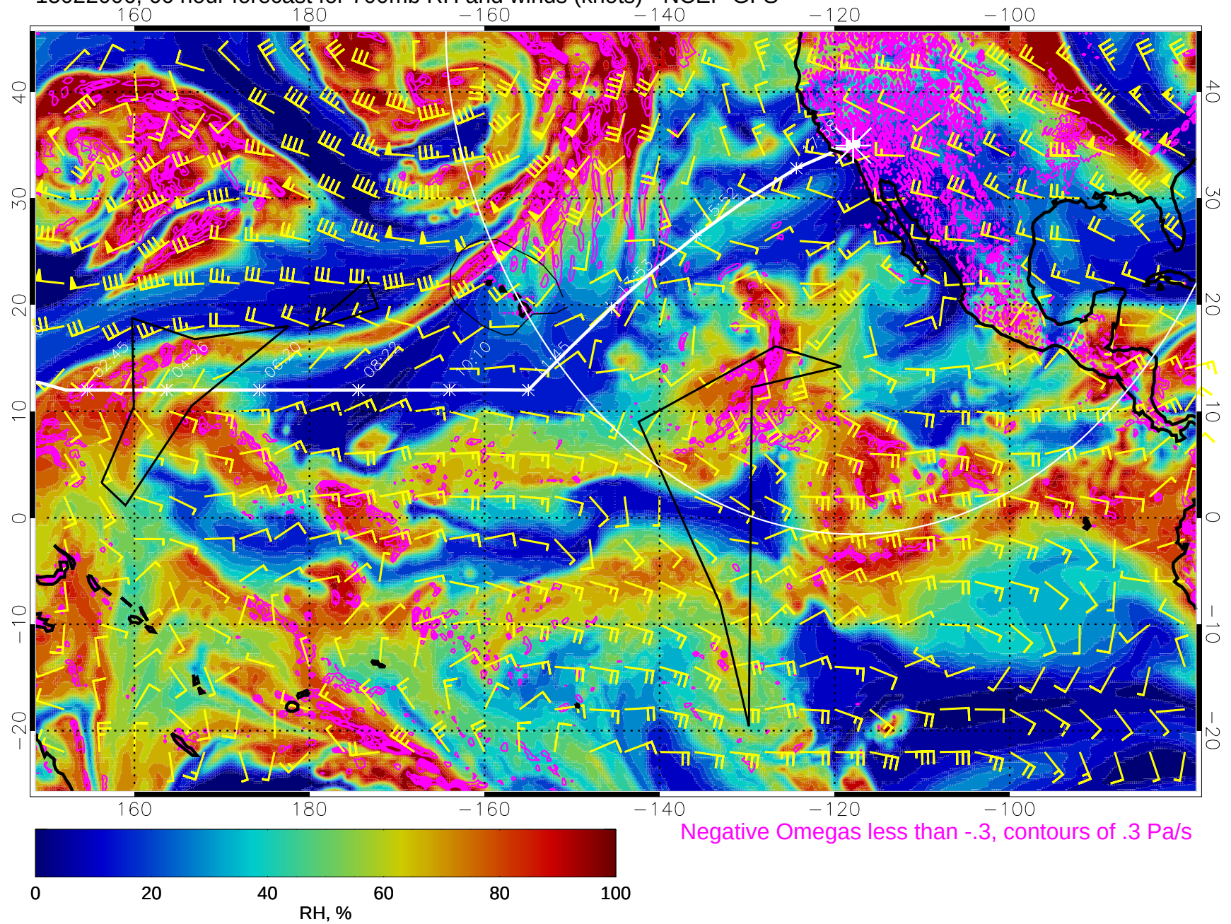
15022006, 66 hour forecast for 700mb RH and winds (knots) - NCEP GFS
