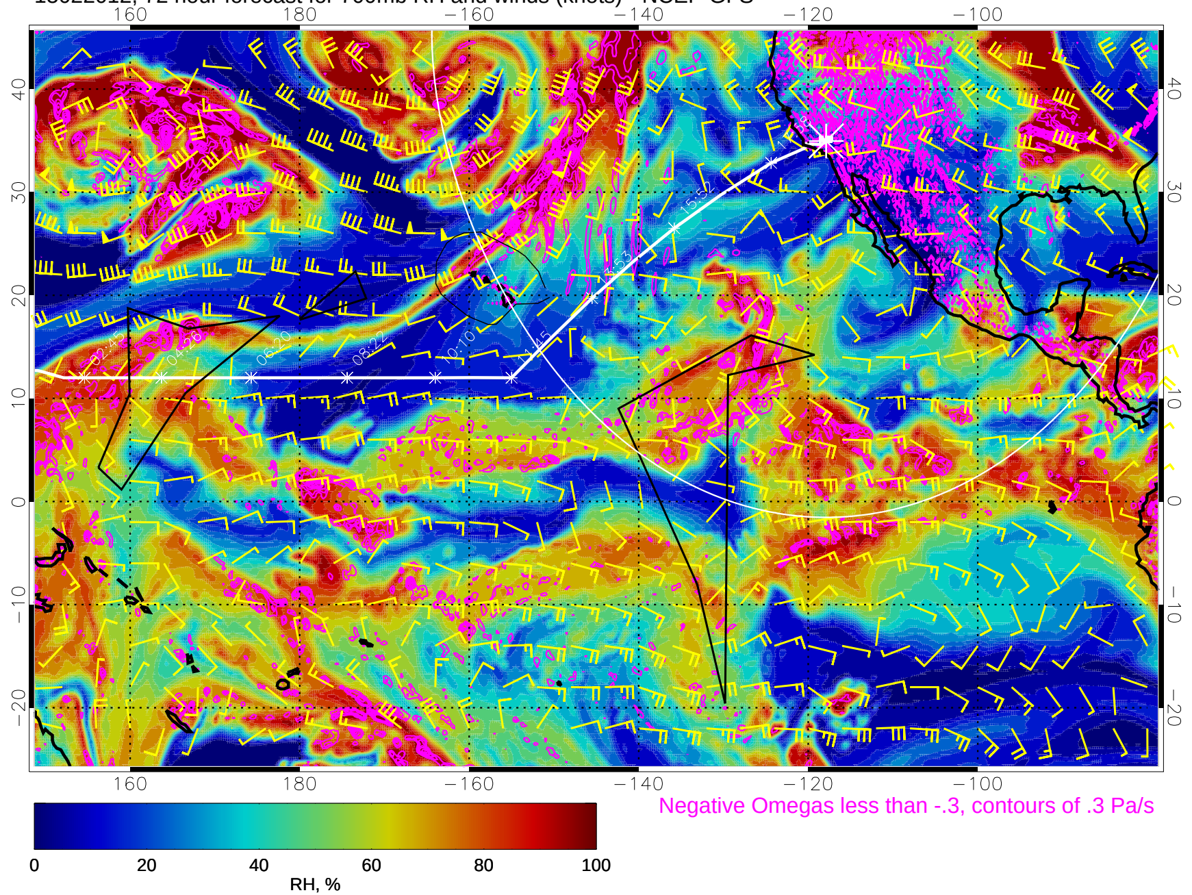
15022012, 72 hour forecast for 700mb RH and winds (knots) - NCEP GFS
