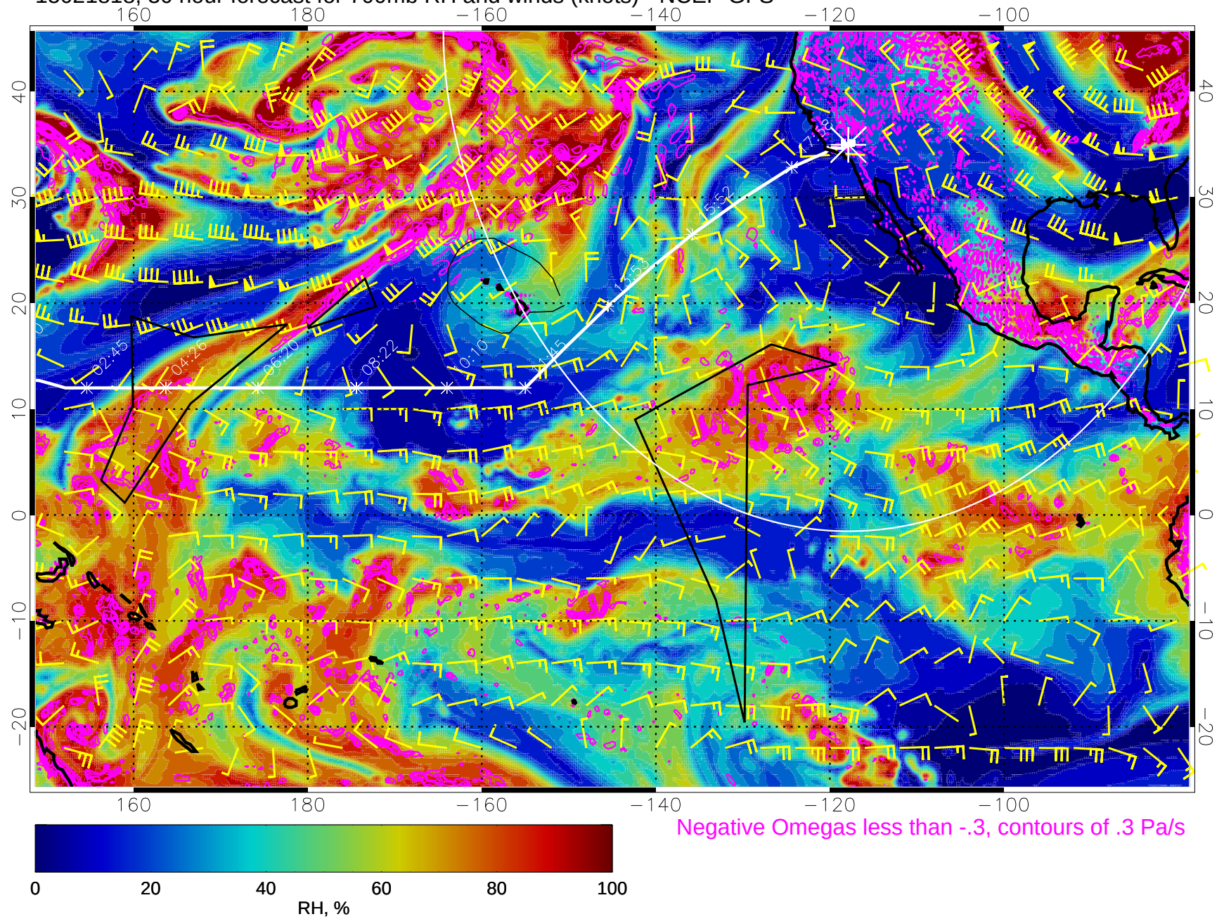
15021818, 30 hour forecast for 700mb RH and winds (knots) - NCEP GFS
