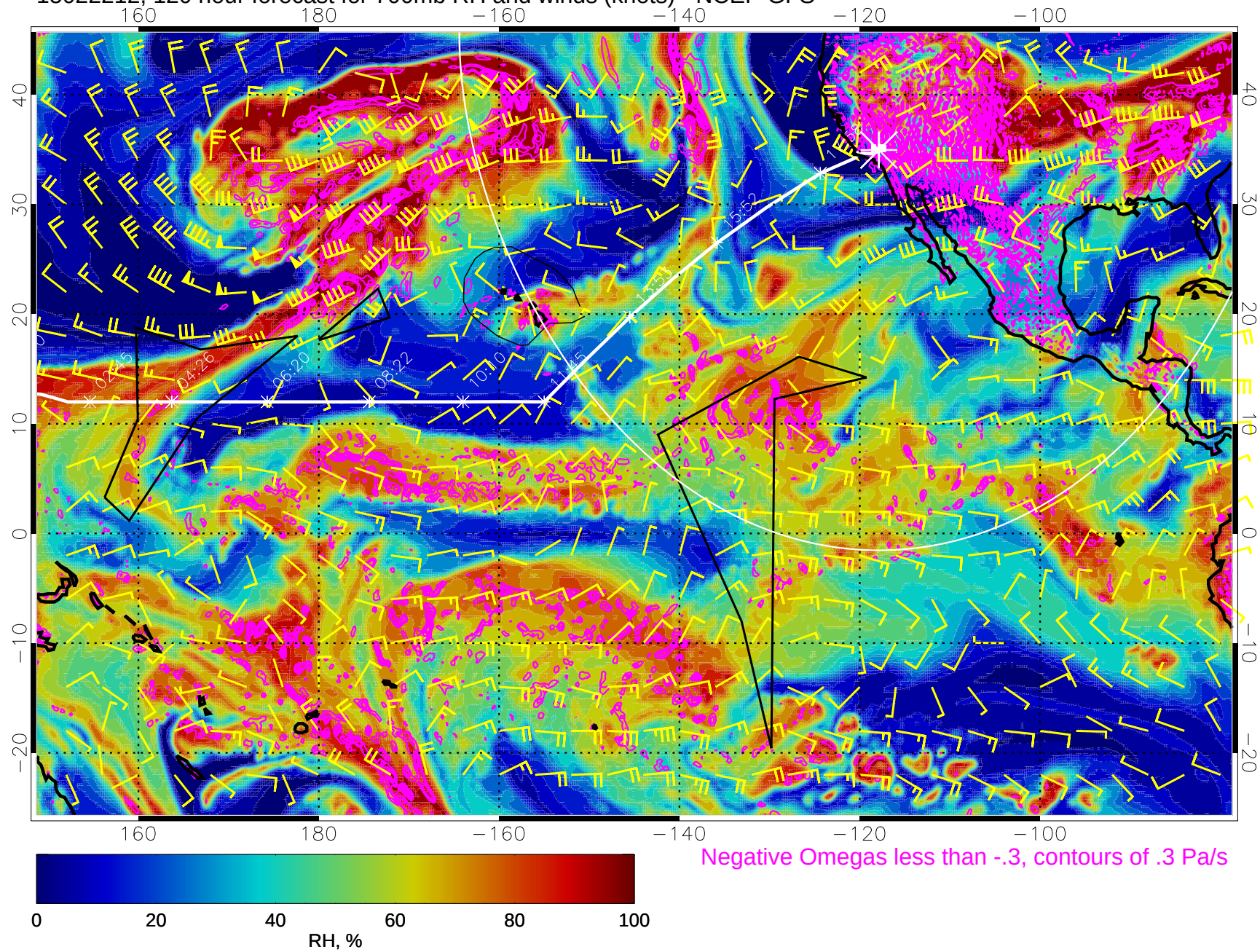
15022212, 120 hour forecast for 700mb RH and winds (knots) - NCEP GFS
