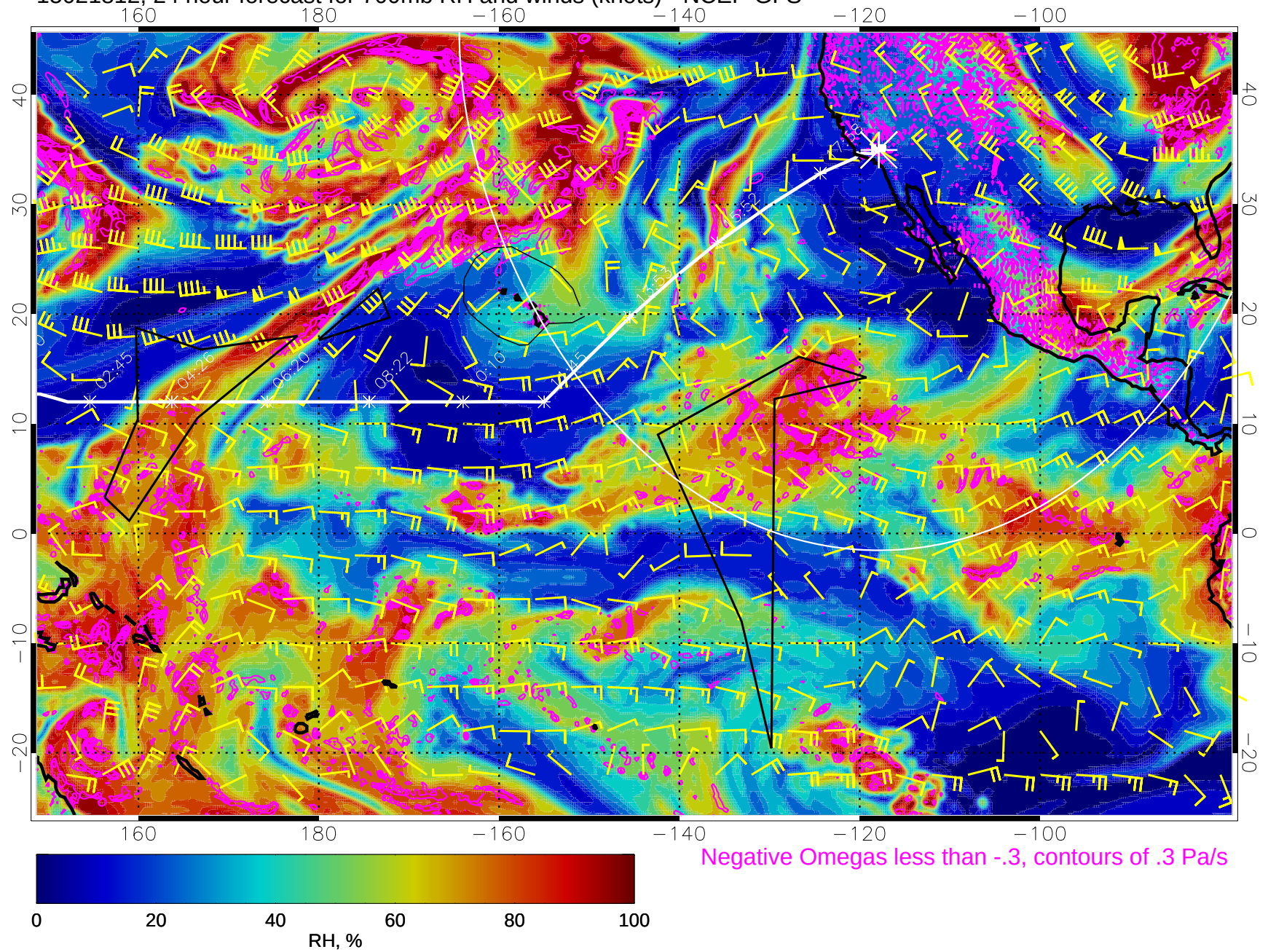
15021812, 24 hour forecast for 700mb RH and winds (knots) - NCEP GFS
