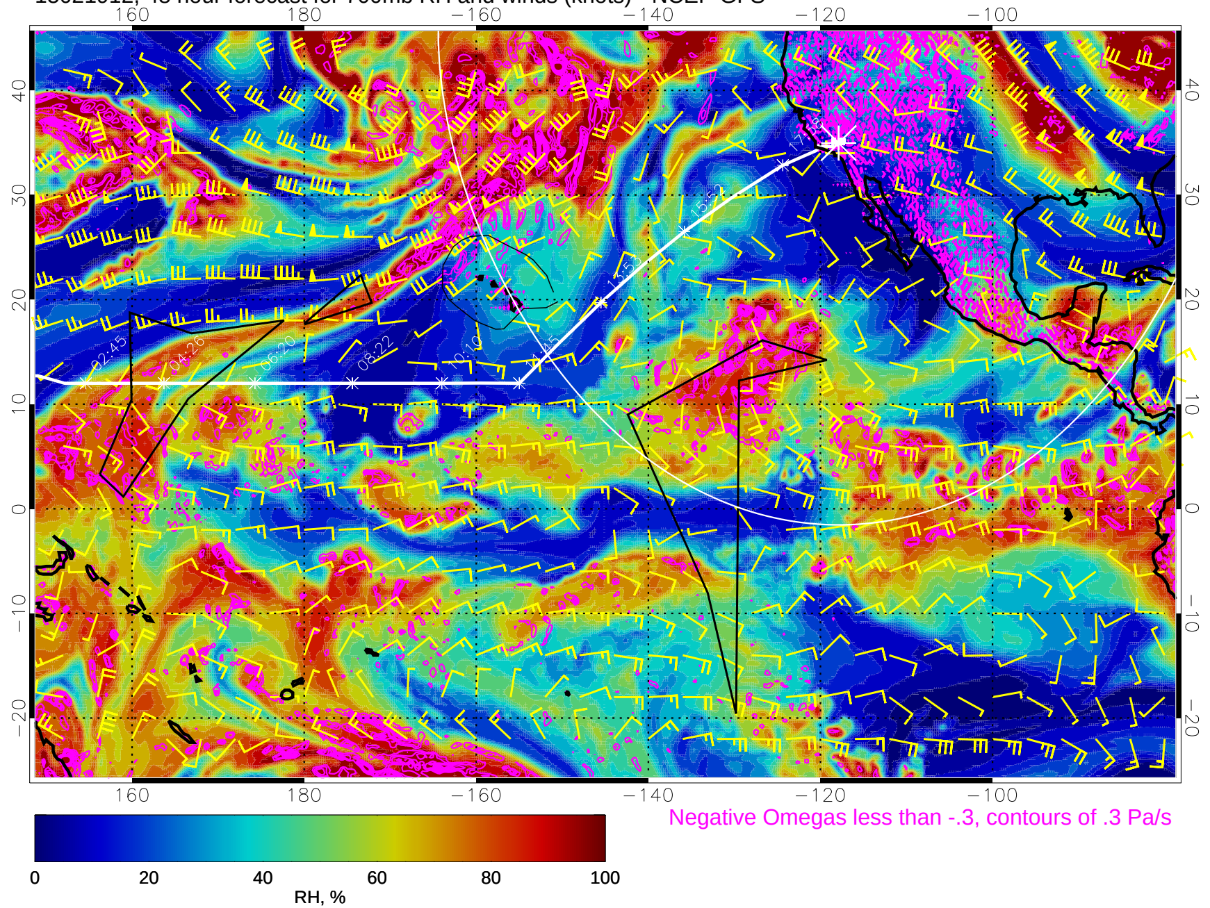
15021912, 48 hour forecast for 700mb RH and winds (knots) - NCEP GFS
