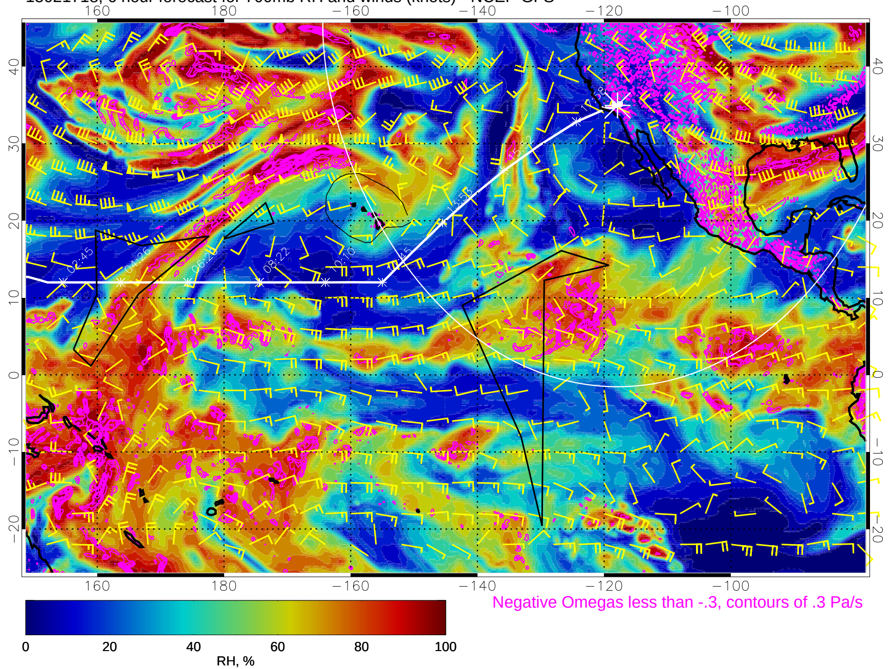
15021718, 6 hour forecast for 700mb RH and winds (knots) - NCEP GFS
