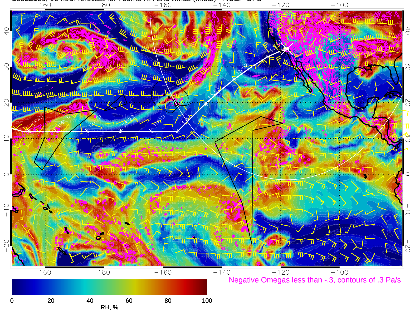
15022106, 90 hour forecast for 700mb RH and winds (knots) - NCEP GFS
