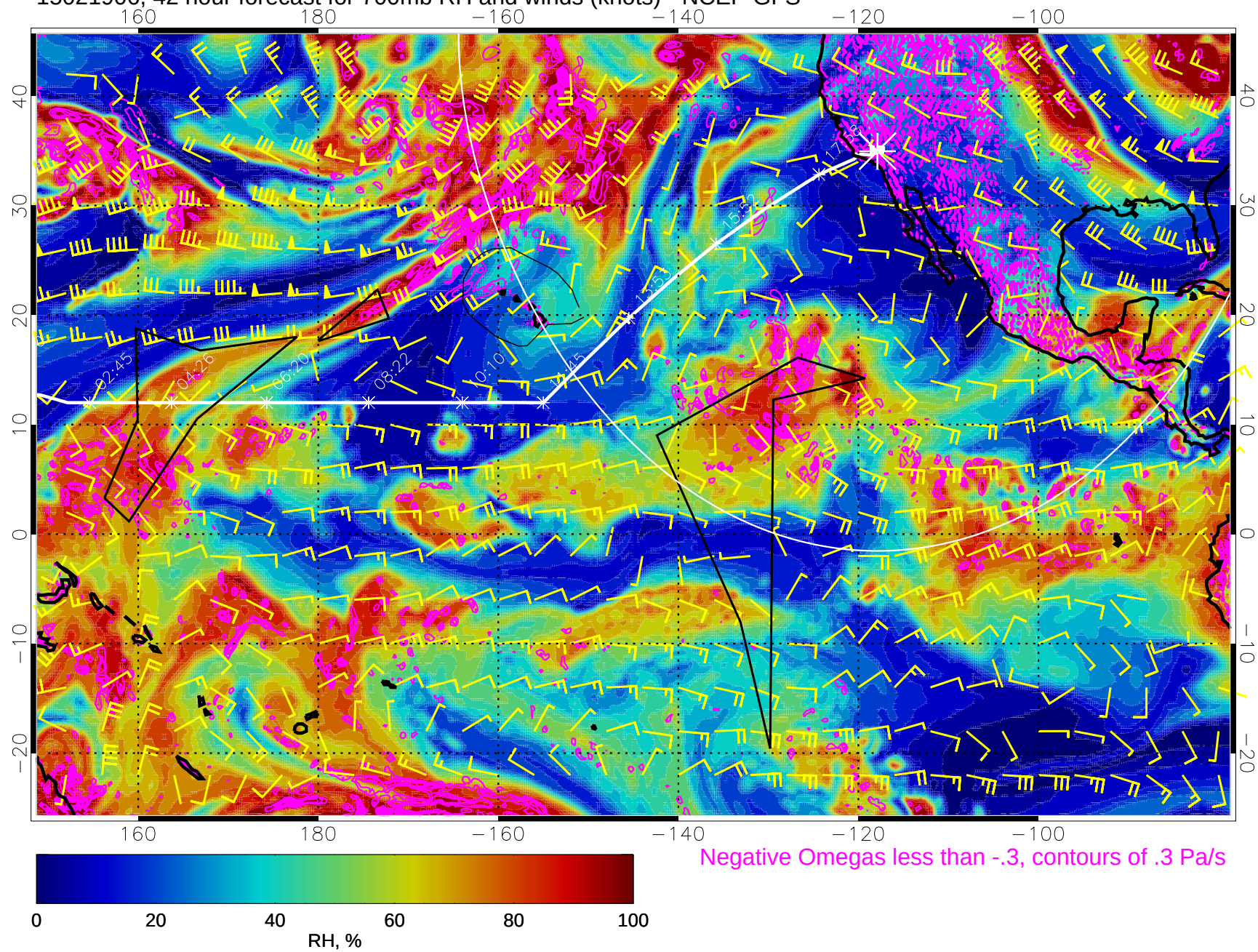
15021906, 42 hour forecast for 700mb RH and winds (knots) - NCEP GFS
