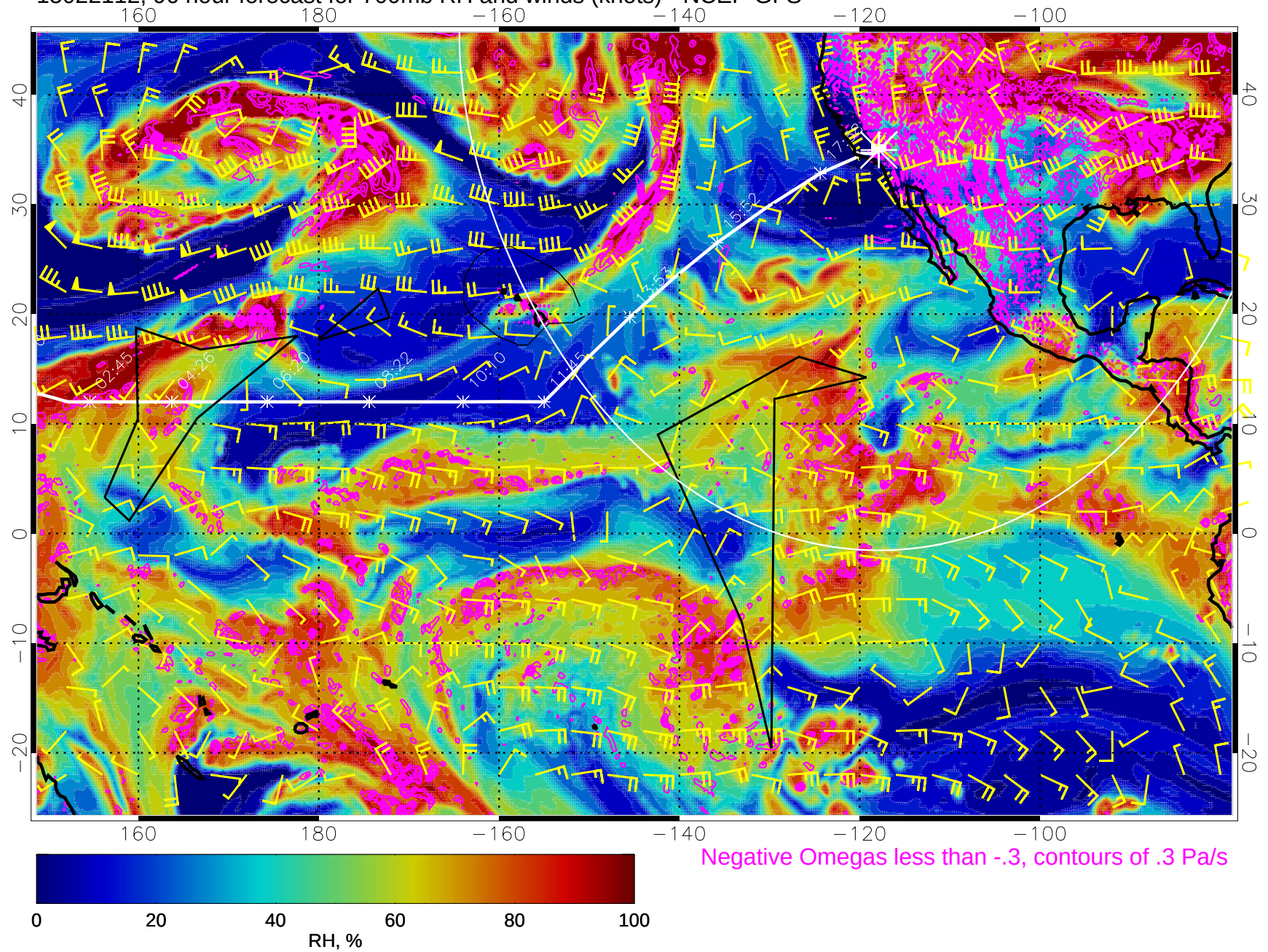
15022112, 96 hour forecast for 700mb RH and winds (knots) - NCEP GFS
