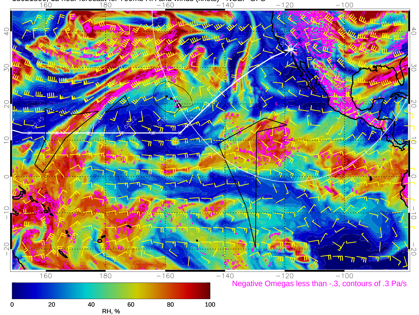
15021800, 12 hour forecast for 700mb RH and winds (knots) - NCEP GFS
