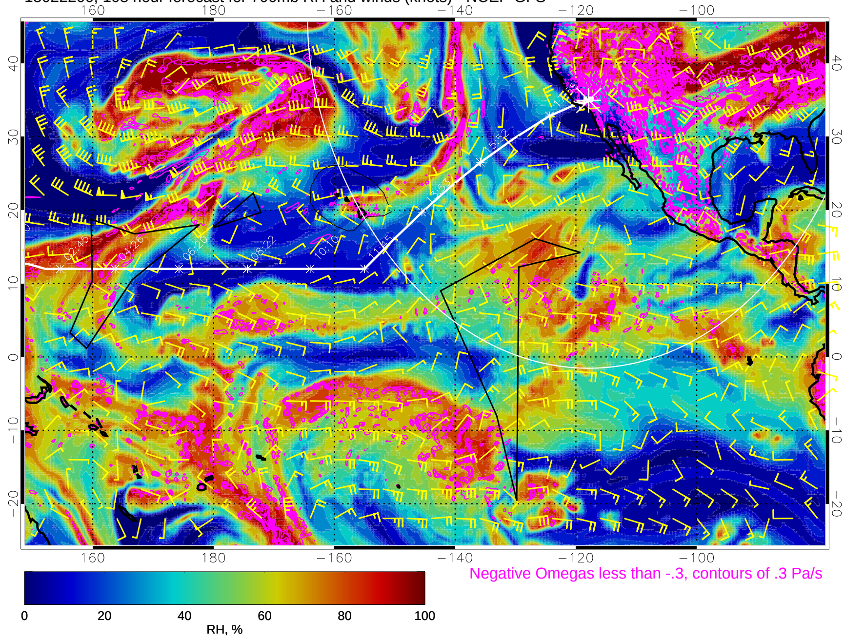
15022200, 108 hour forecast for 700mb RH and winds (knots) - NCEP GFS
