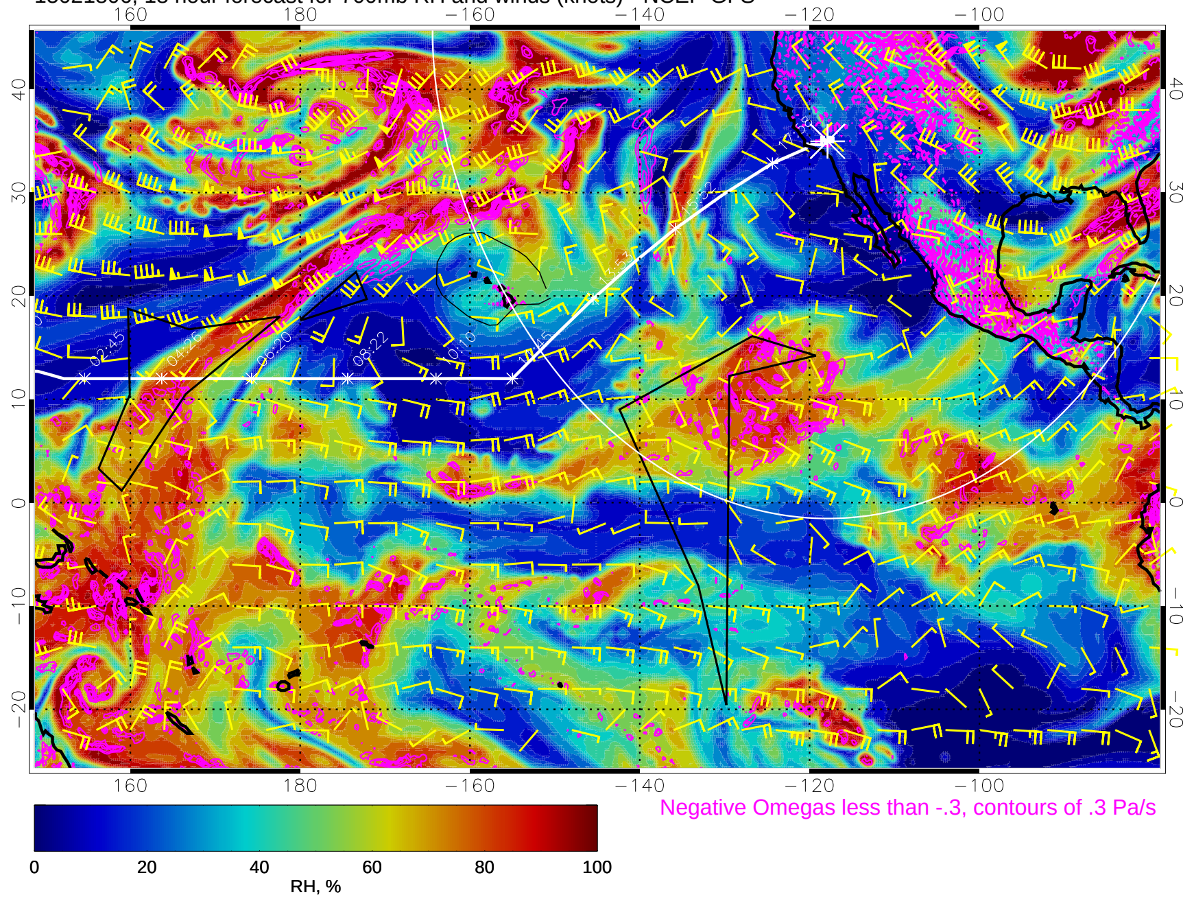
15021806, 18 hour forecast for 700mb RH and winds (knots) - NCEP GFS
