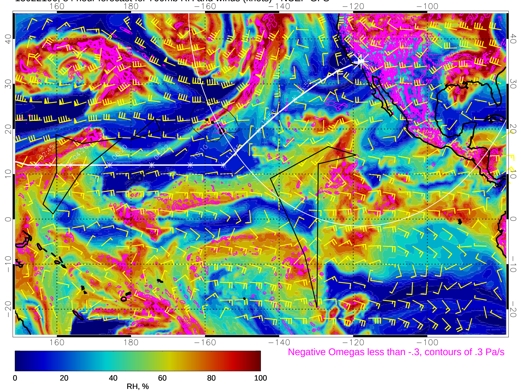
15022100, 84 hour forecast for 700mb RH and winds (knots) - NCEP GFS
