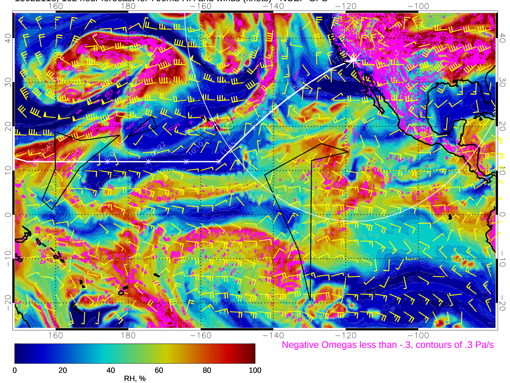
15022118, 102 hour forecast for 700mb RH and winds (knots) - NCEP GFS
