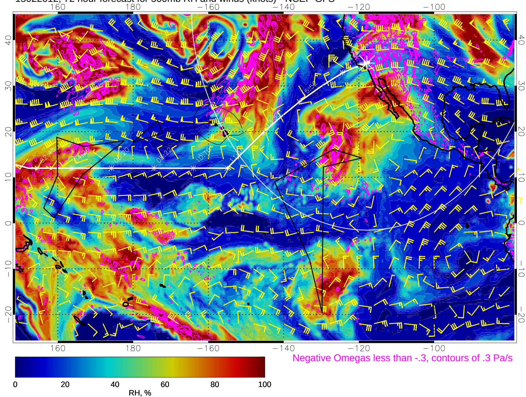
15022012, 72 hour forecast for 500mb RH and winds (knots) - NCEP GFS
