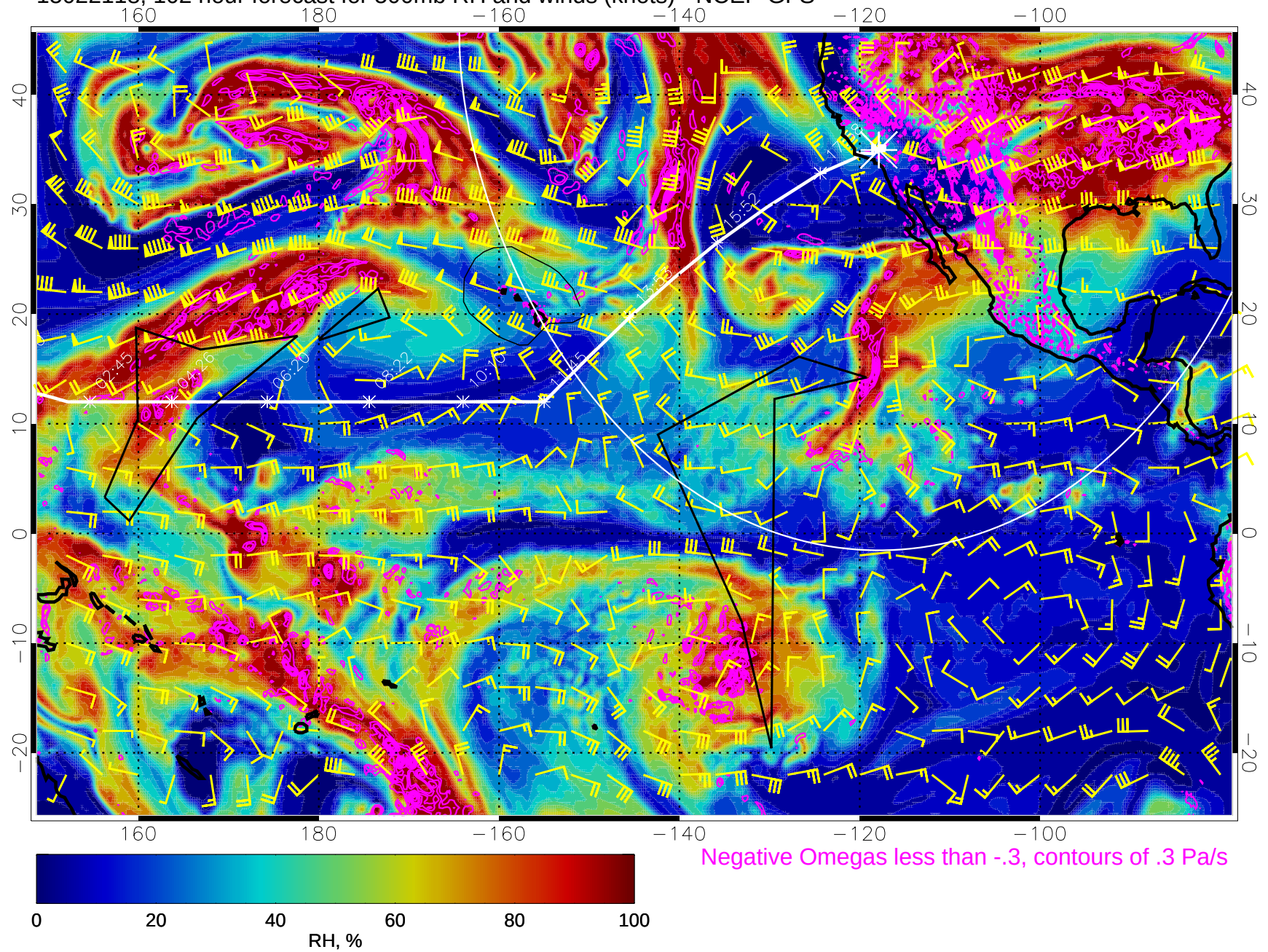
15022118, 102 hour forecast for 500mb RH and winds (knots) - NCEP GFS
