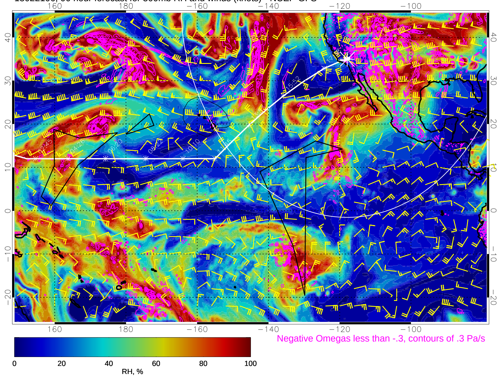
15022106, 90 hour forecast for 500mb RH and winds (knots) - NCEP GFS
