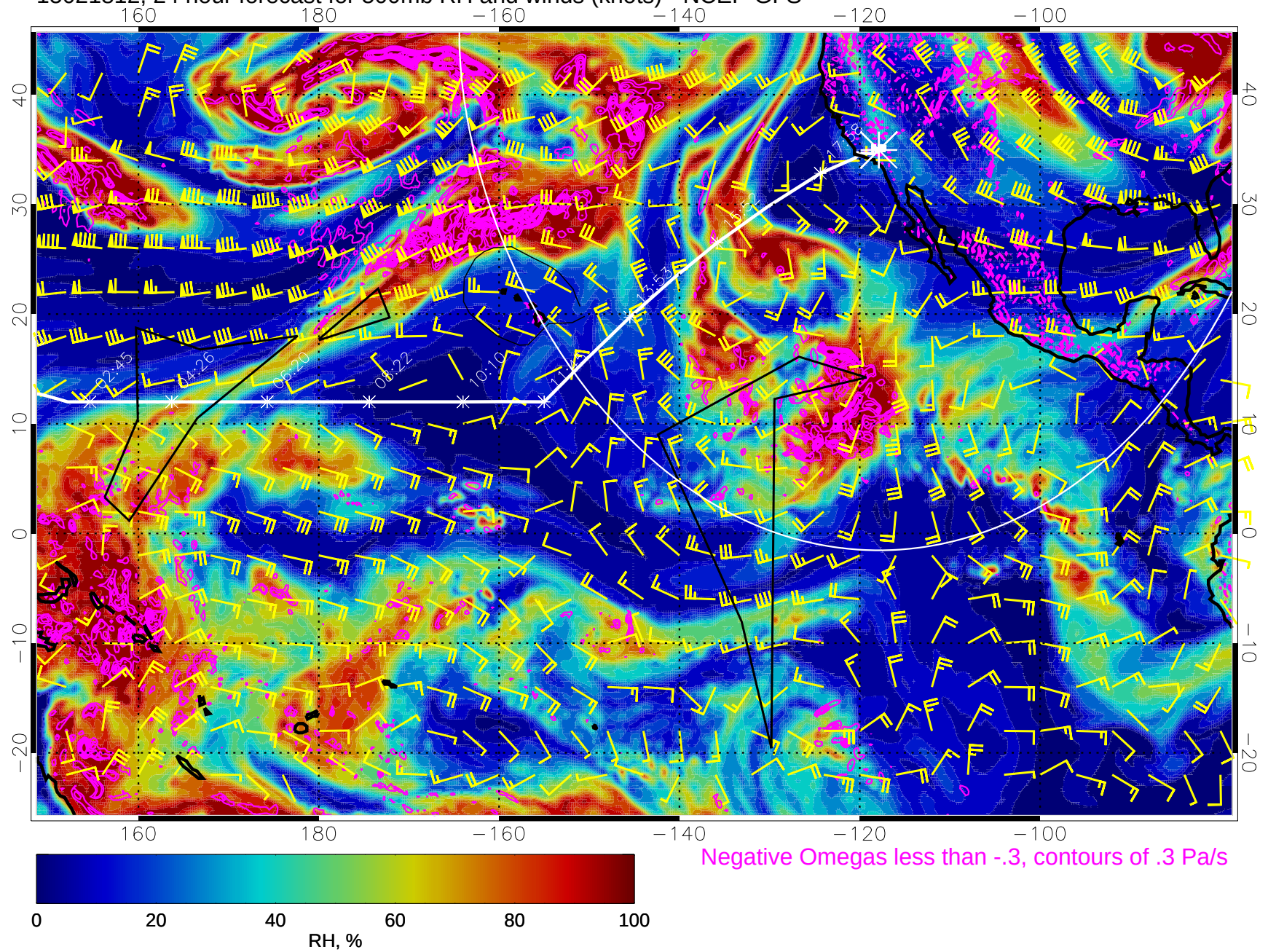
15021812, 24 hour forecast for 500mb RH and winds (knots) - NCEP GFS
