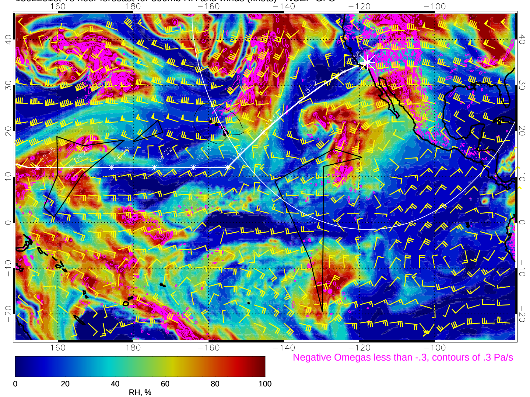
15022018, 78 hour forecast for 500mb RH and winds (knots) - NCEP GFS
