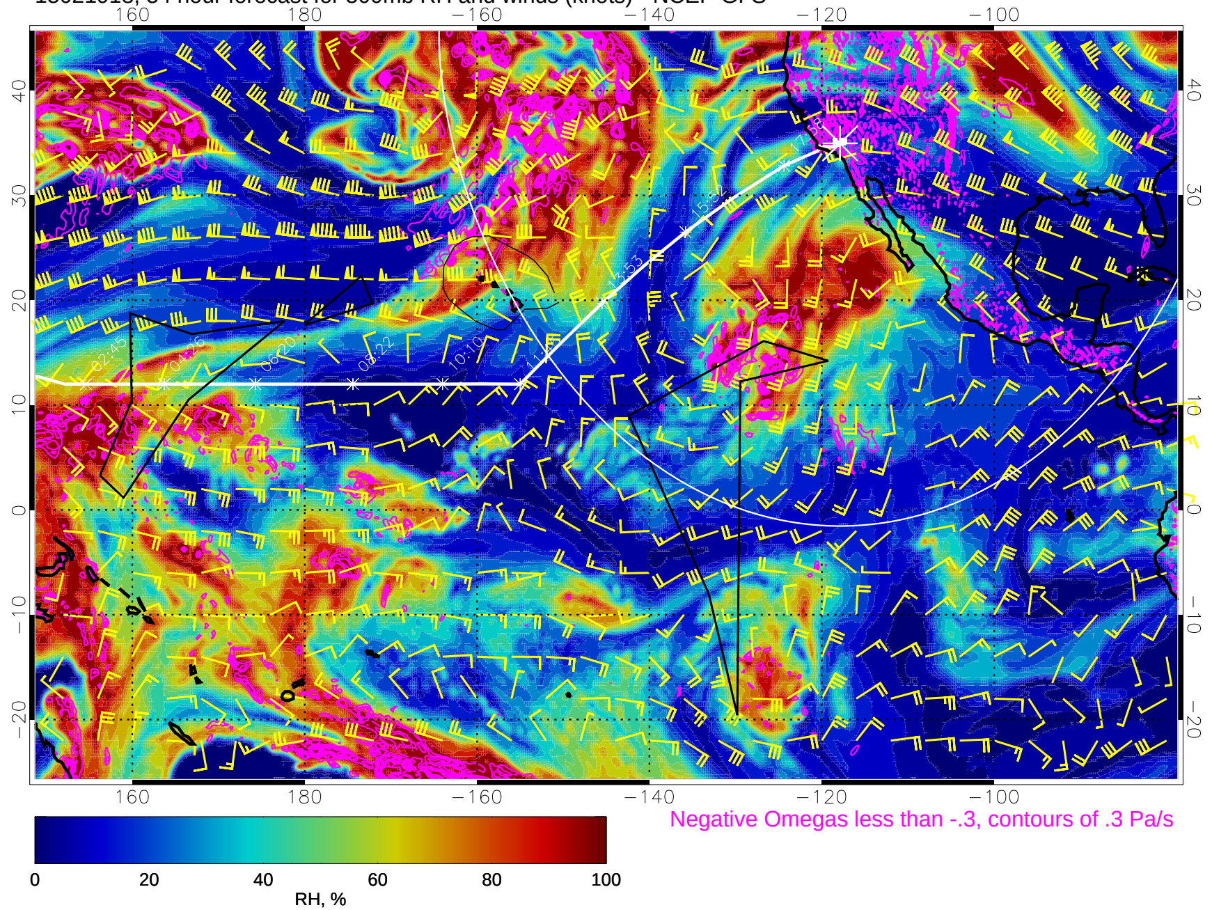
15021918, 54 hour forecast for 500mb RH and winds (knots) - NCEP GFS
