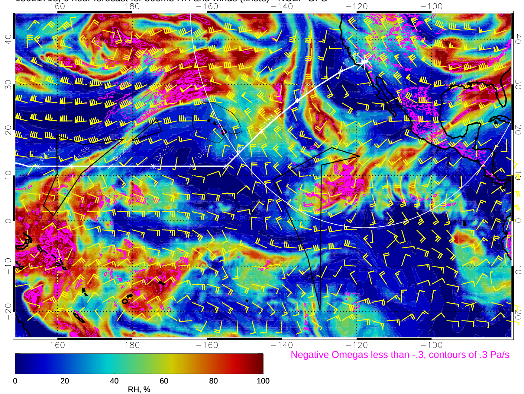
15021718, 6 hour forecast for 500mb RH and winds (knots) - NCEP GFS
