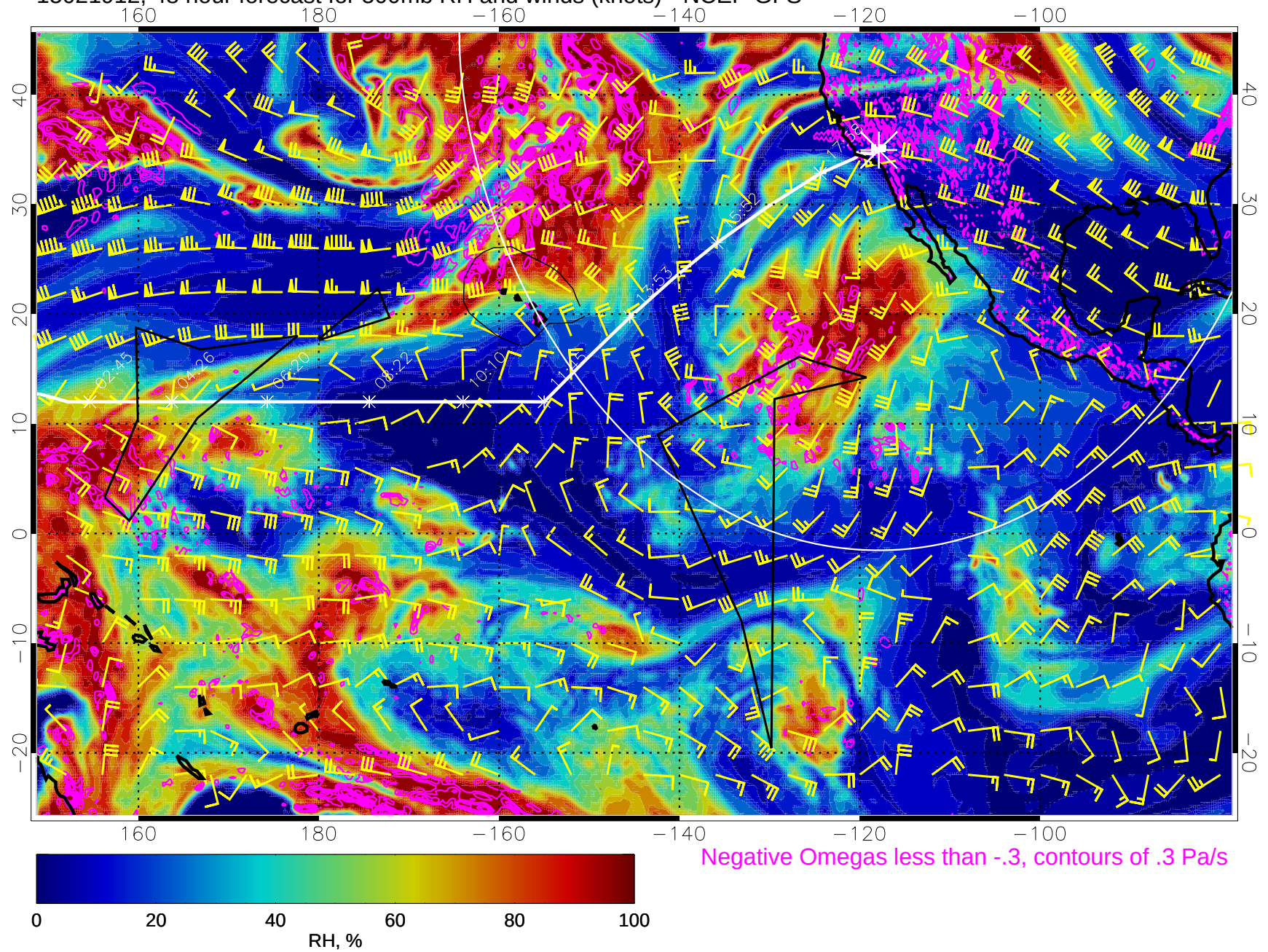
15021912, 48 hour forecast for 500mb RH and winds (knots) - NCEP GFS
