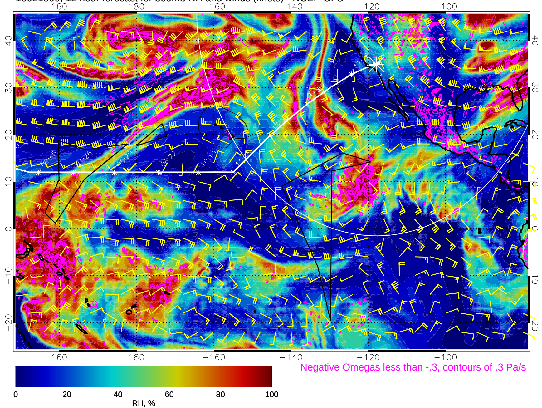
15021800, 12 hour forecast for 500mb RH and winds (knots) - NCEP GFS
