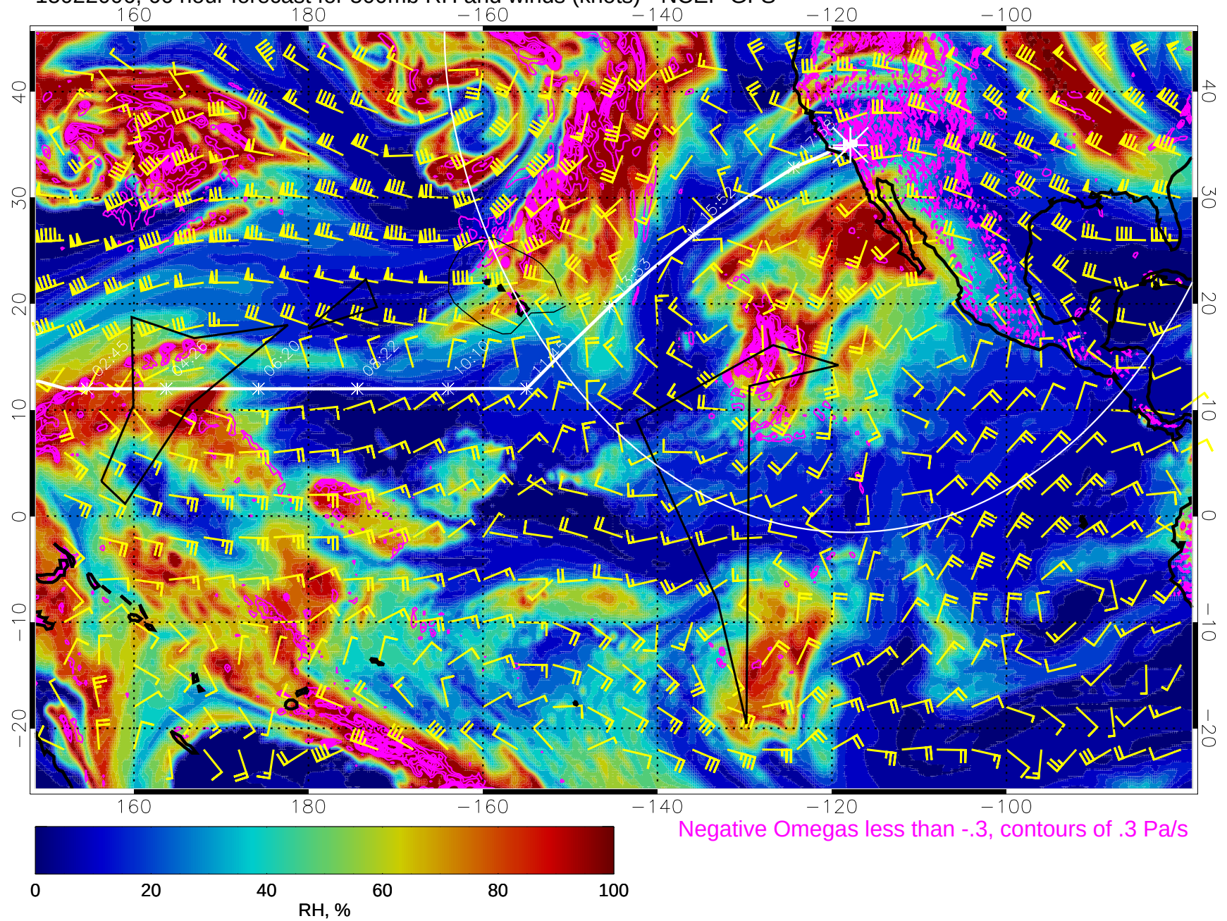
15022006, 66 hour forecast for 500mb RH and winds (knots) - NCEP GFS
