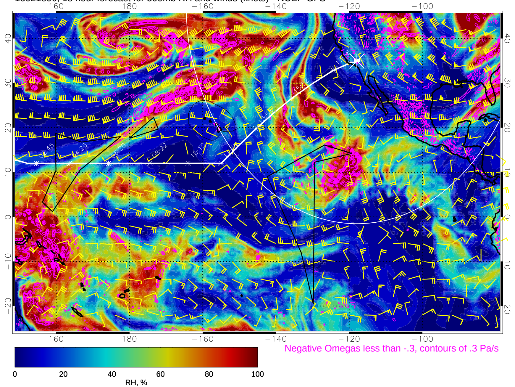
15021806, 18 hour forecast for 500mb RH and winds (knots) - NCEP GFS
