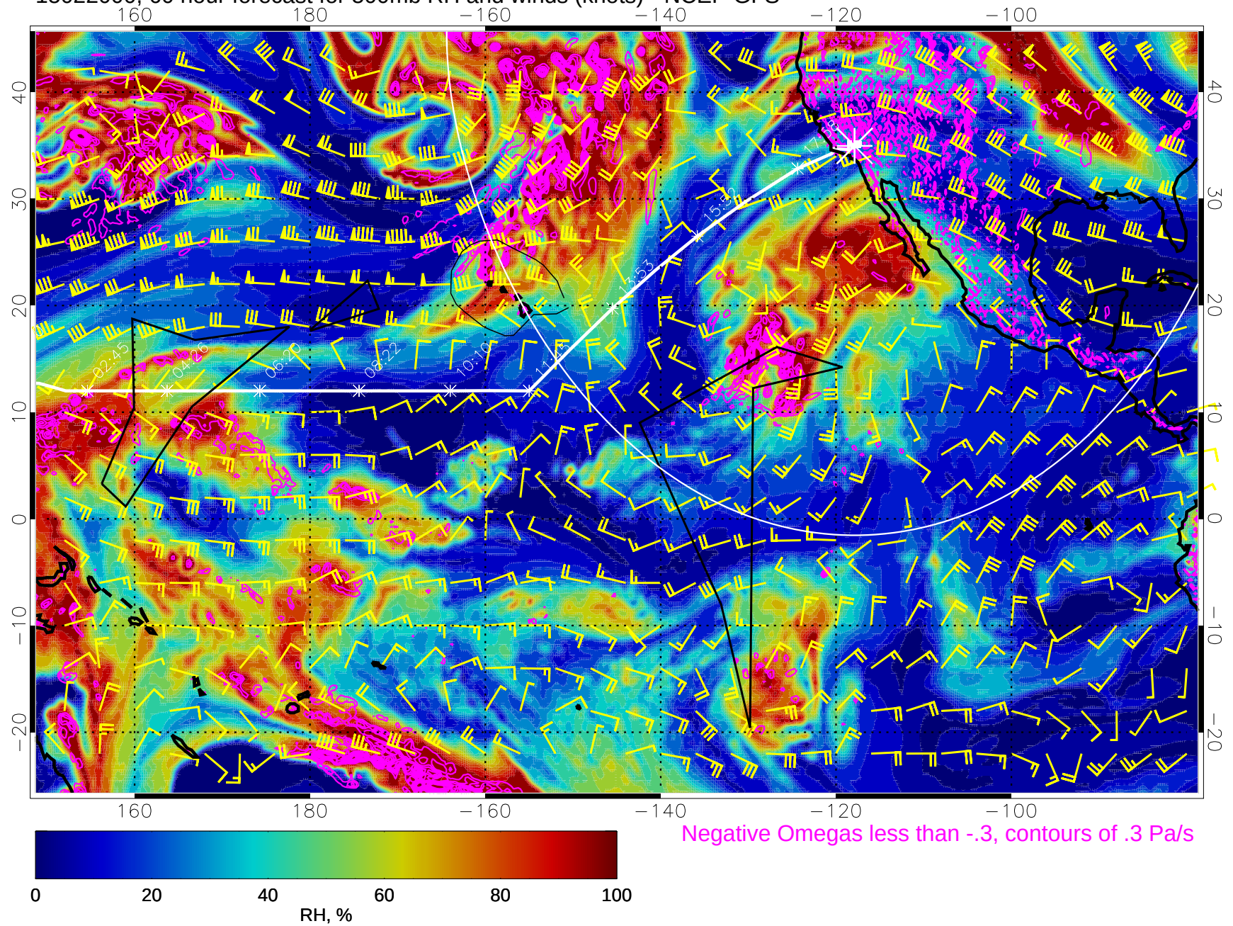
15022000, 60 hour forecast for 500mb RH and winds (knots) - NCEP GFS
