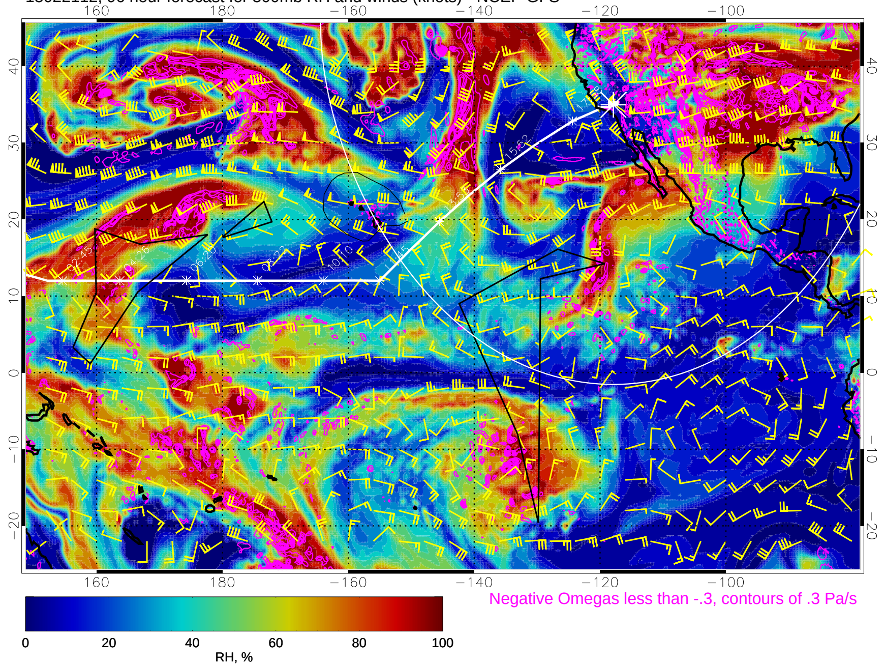
15022112, 96 hour forecast for 500mb RH and winds (knots) - NCEP GFS
