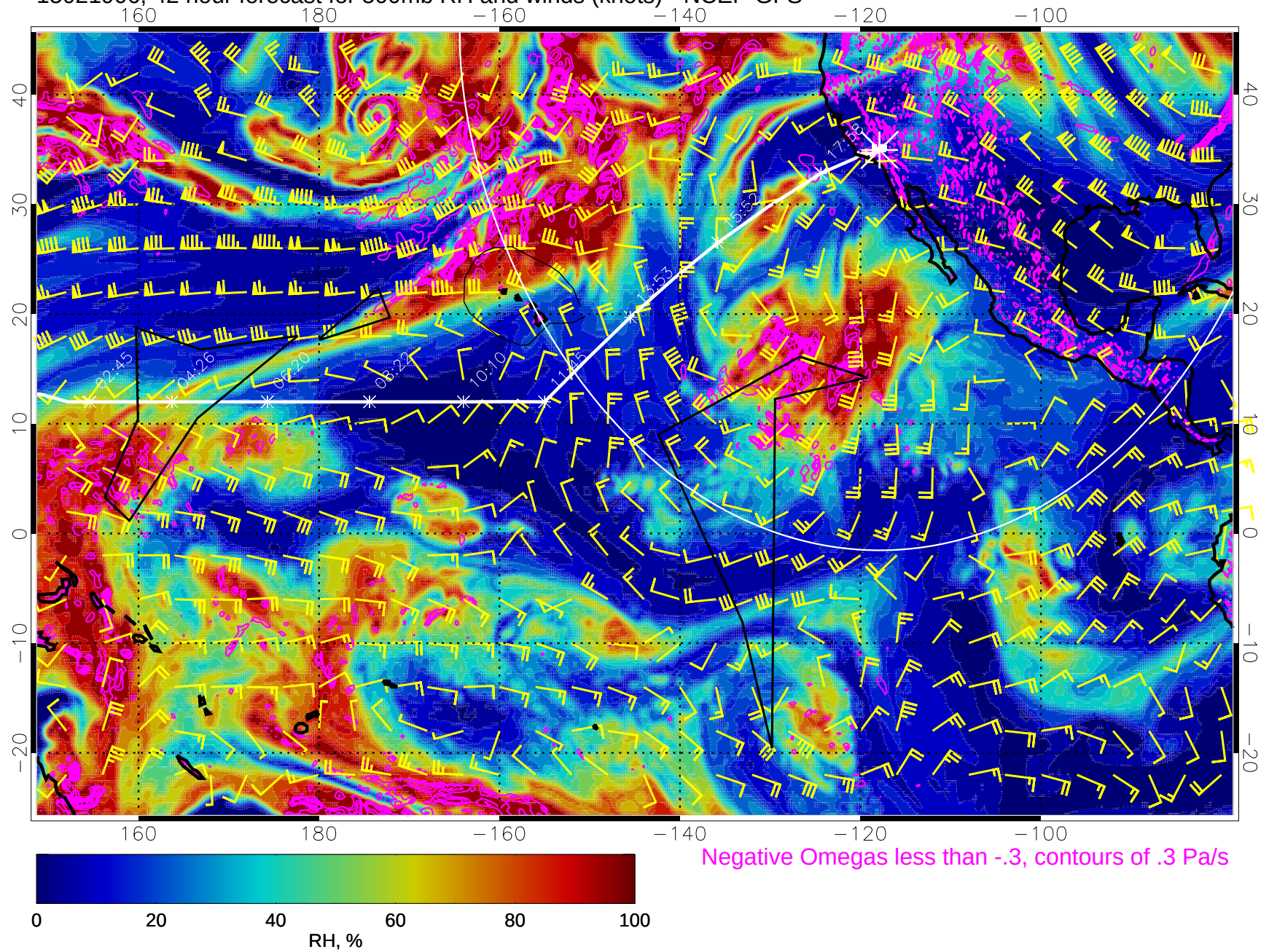
15021906, 42 hour forecast for 500mb RH and winds (knots) - NCEP GFS
