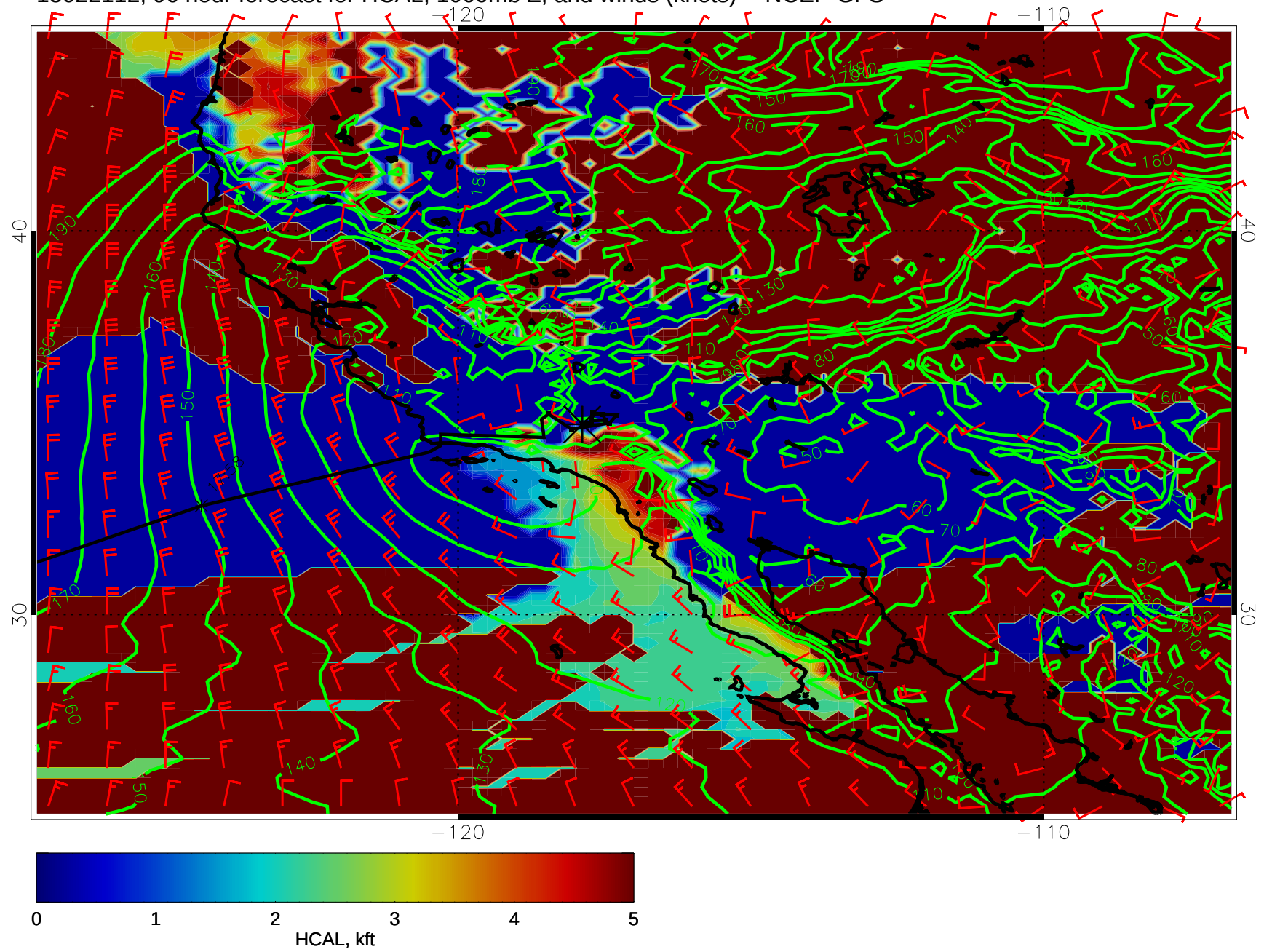
15022112, 96 hour forecast for HCAL, 1000mb Z, and winds (knots) -- NCEP GFS
