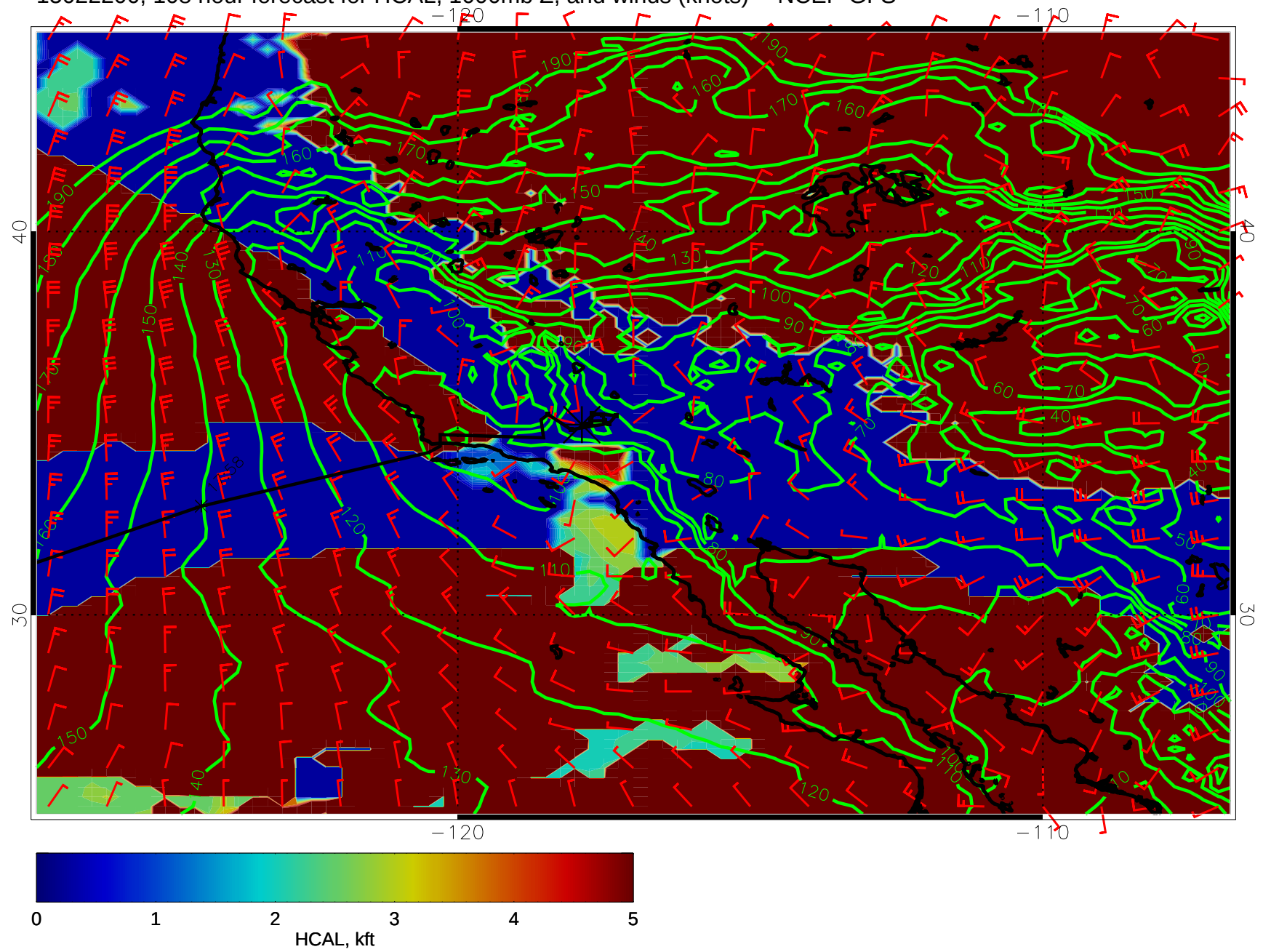
15022200, 108 hour forecast for HCAL, 1000mb Z, and winds (knots) -- NCEP GFS
