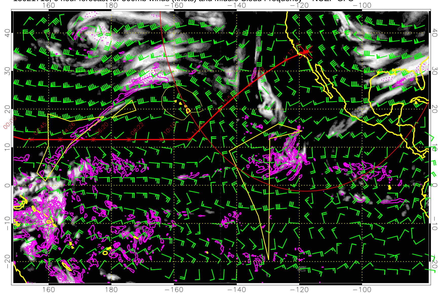
15021718, 6 hour forecast for 500mb winds (knots) and Middle Cloud Frequency -- NCEP GFS
