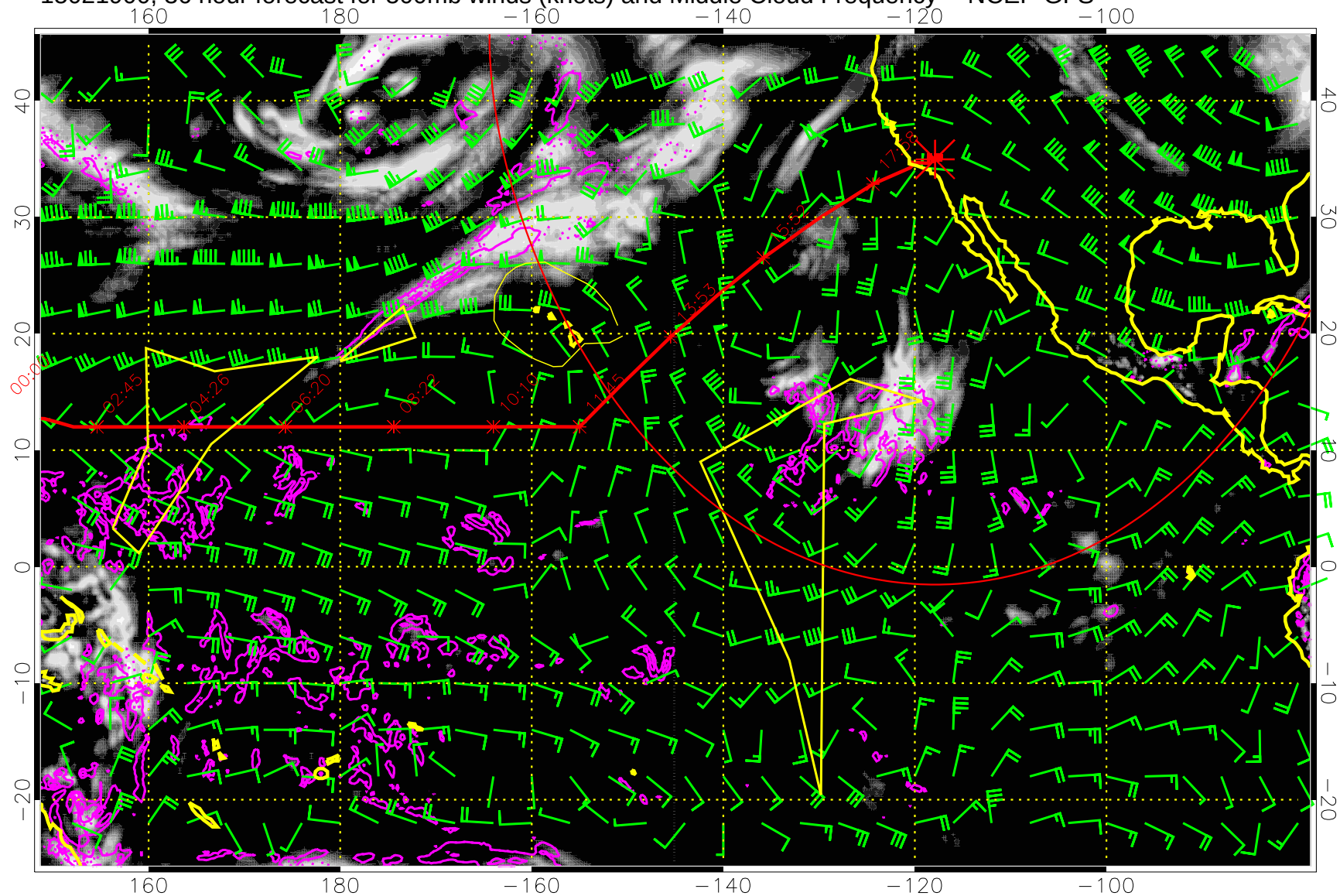
15021900, 36 hour forecast for 500mb winds (knots) and Middle Cloud Frequency -- NCEP GFS
