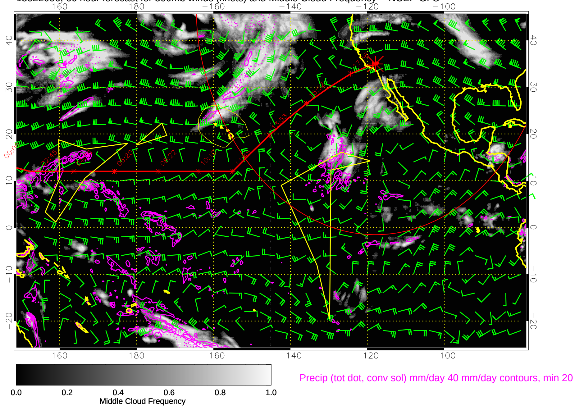
15022006, 66 hour forecast for 500mb winds (knots) and Middle Cloud Frequency -- NCEP GFS
