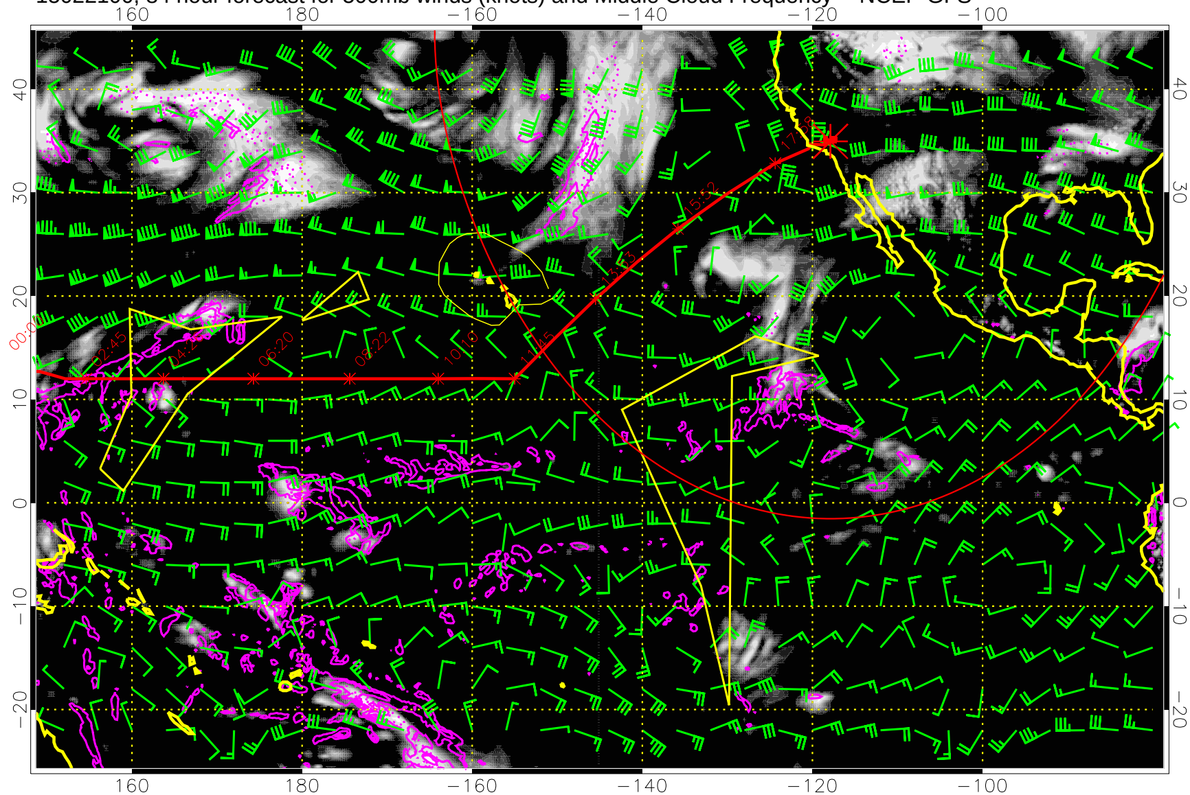
15022100, 84 hour forecast for 500mb winds (knots) and Middle Cloud Frequency -- NCEP GFS
