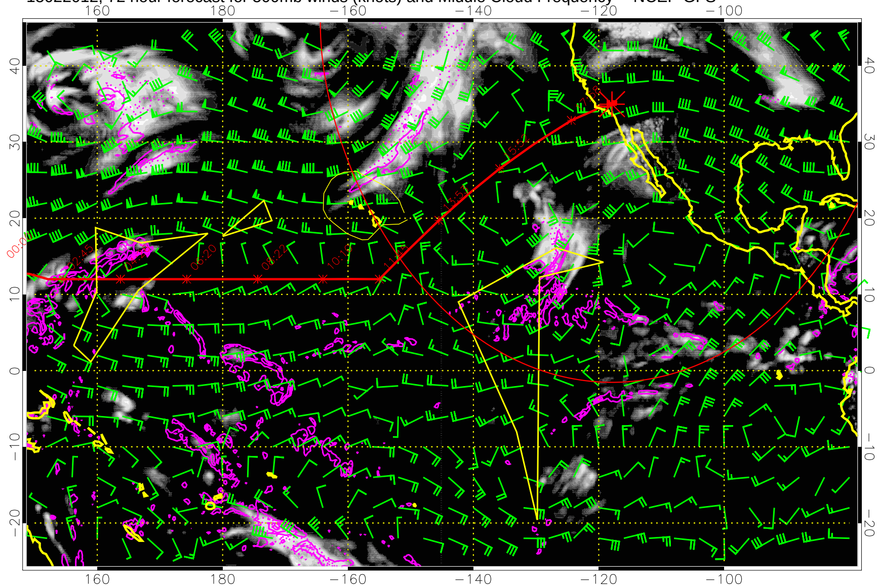
15022012, 72 hour forecast for 500mb winds (knots) and Middle Cloud Frequency -- NCEP GFS
