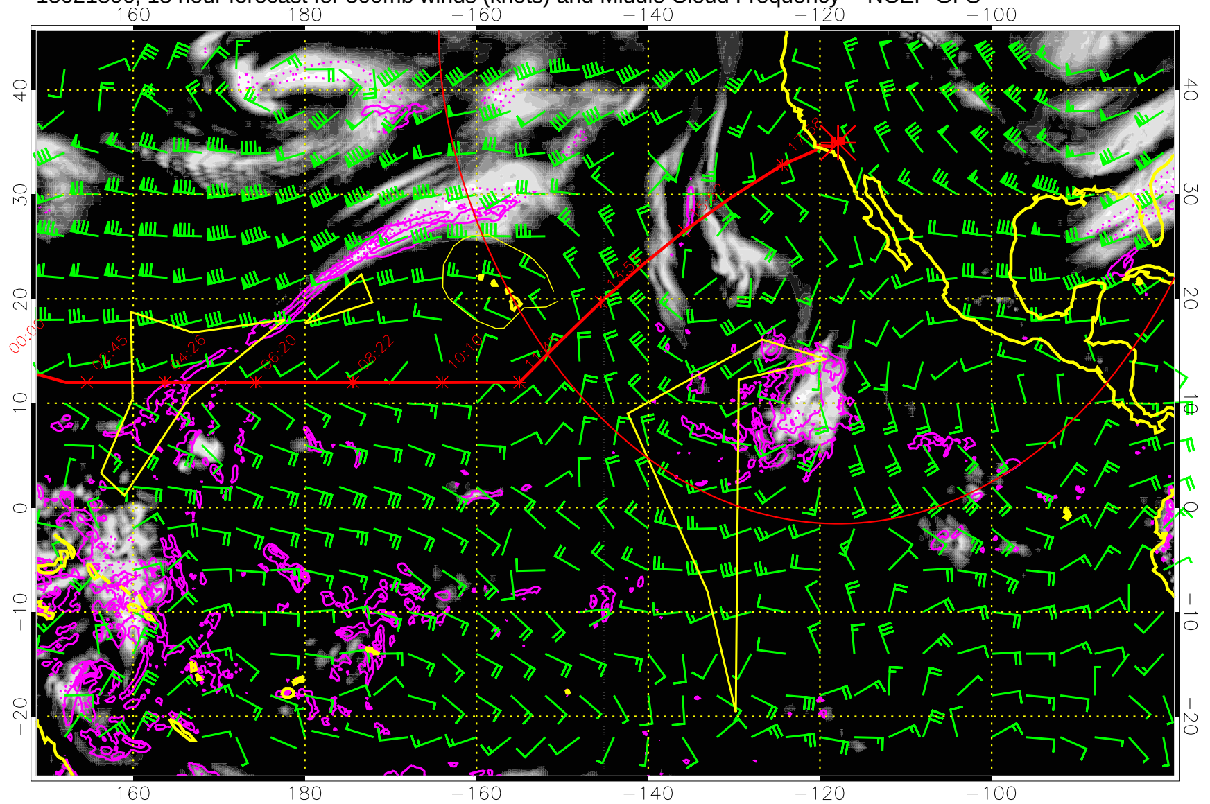
15021806, 18 hour forecast for 500mb winds (knots) and Middle Cloud Frequency -- NCEP GFS
