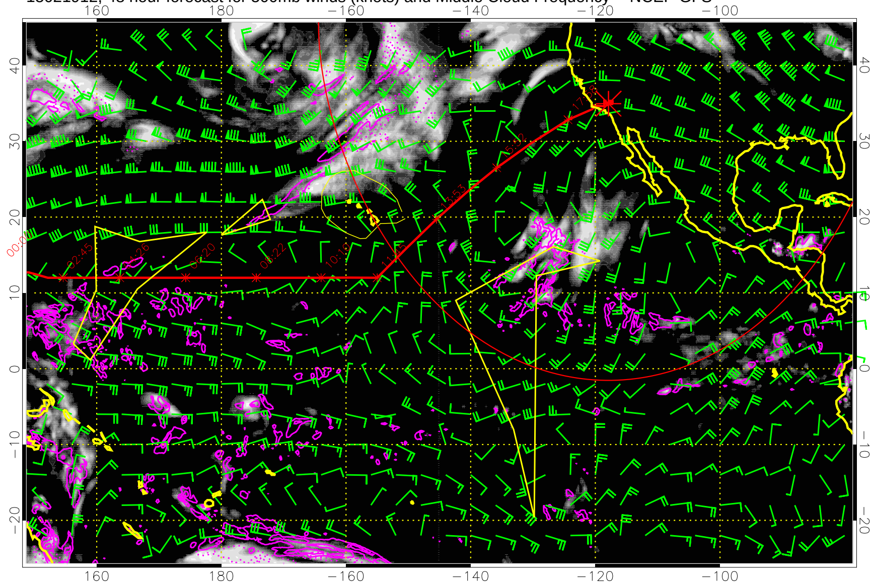
15021912, 48 hour forecast for 500mb winds (knots) and Middle Cloud Frequency -- NCEP GFS
