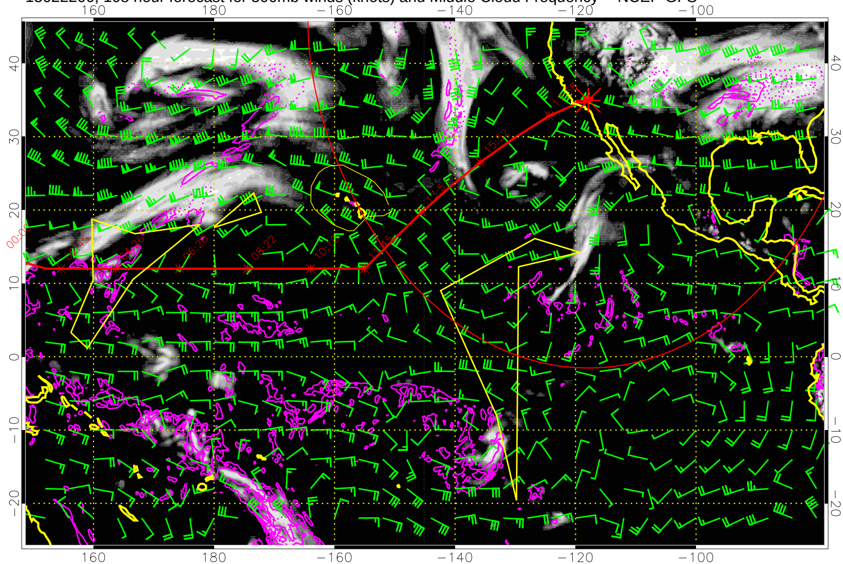
15022200, 108 hour forecast for 500mb winds (knots) and Middle Cloud Frequency -- NCEP GFS
