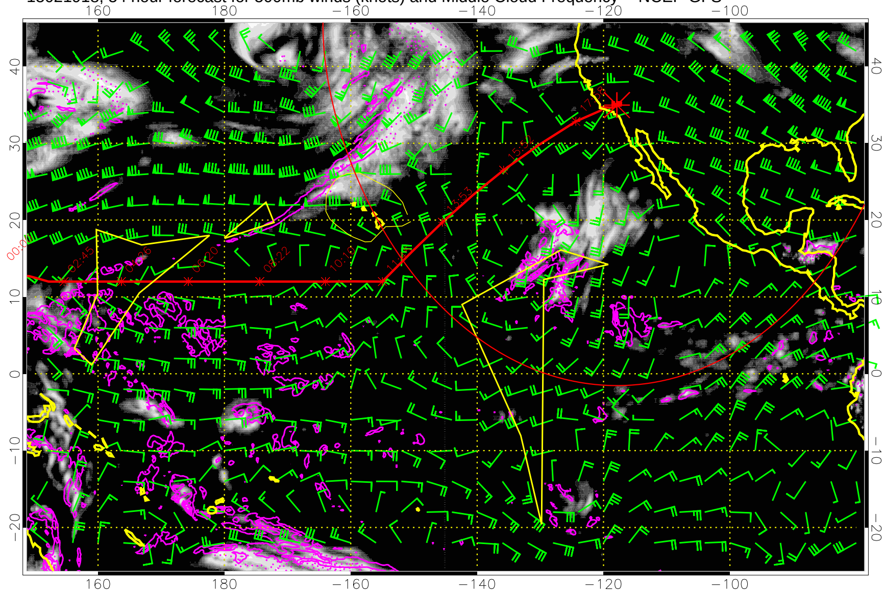
15021918, 54 hour forecast for 500mb winds (knots) and Middle Cloud Frequency -- NCEP GFS
