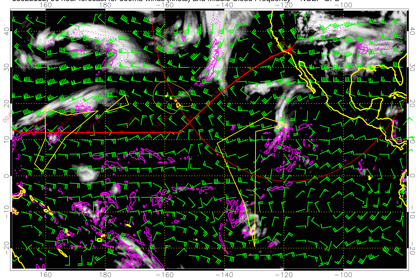
15022112, 96 hour forecast for 500mb winds (knots) and Middle Cloud Frequency -- NCEP GFS
