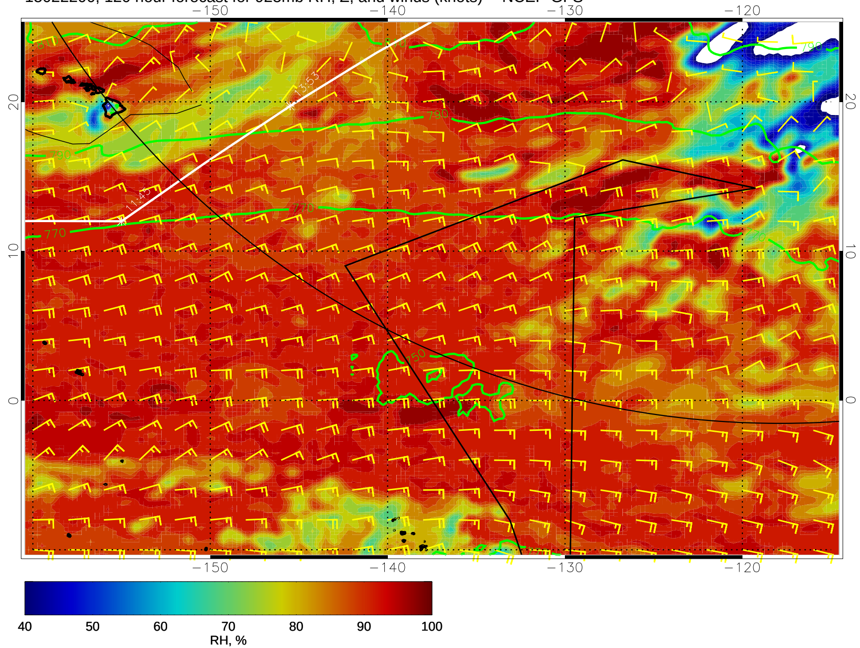
15022200, 120 hour forecast for 925mb RH, Z, and winds (knots) -- NCEP GFS
