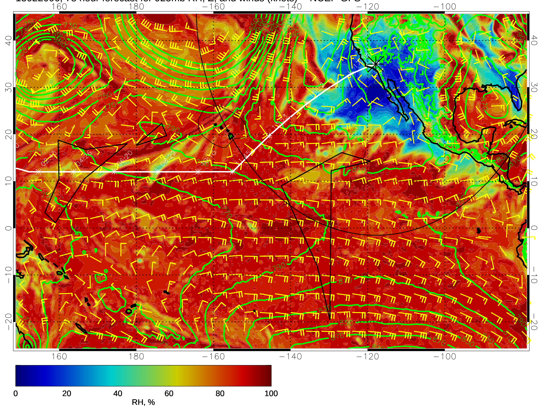
15022006, 78 hour forecast for 925mb RH, Z, and winds (knots) -- NCEP GFS
