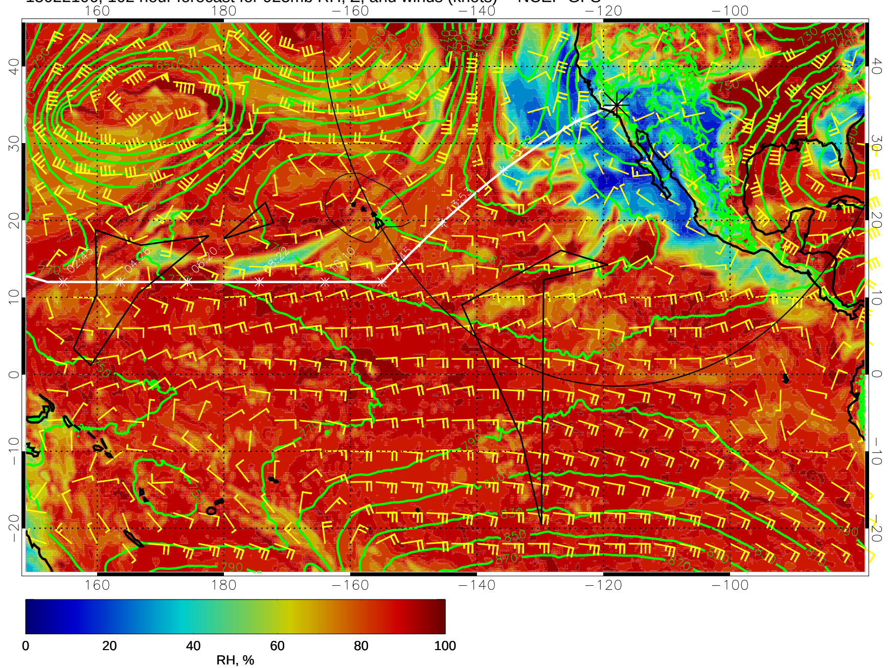
15022106, 102 hour forecast for 925mb RH, Z, and winds (knots) -- NCEP GFS
