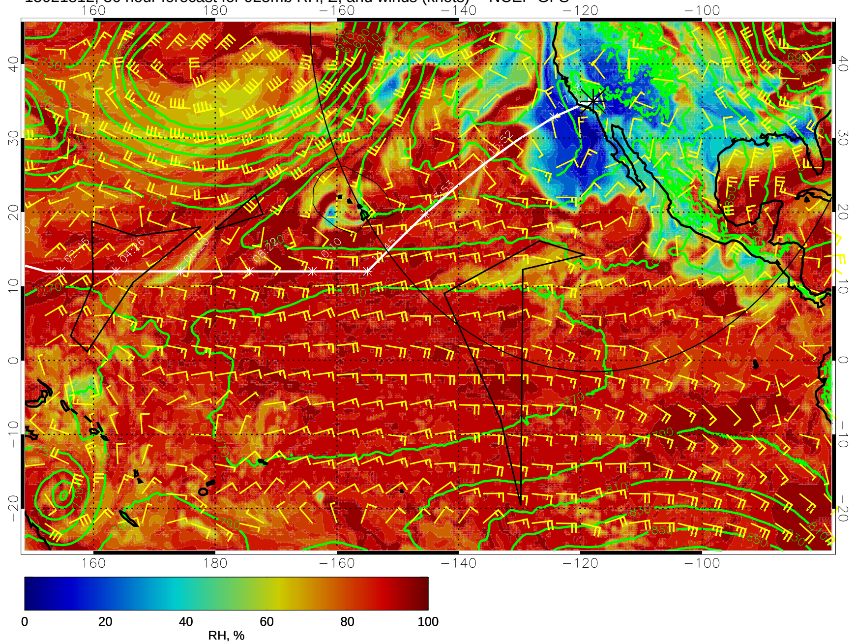
15021812, 36 hour forecast for 925mb RH, Z, and winds (knots) -- NCEP GFS
