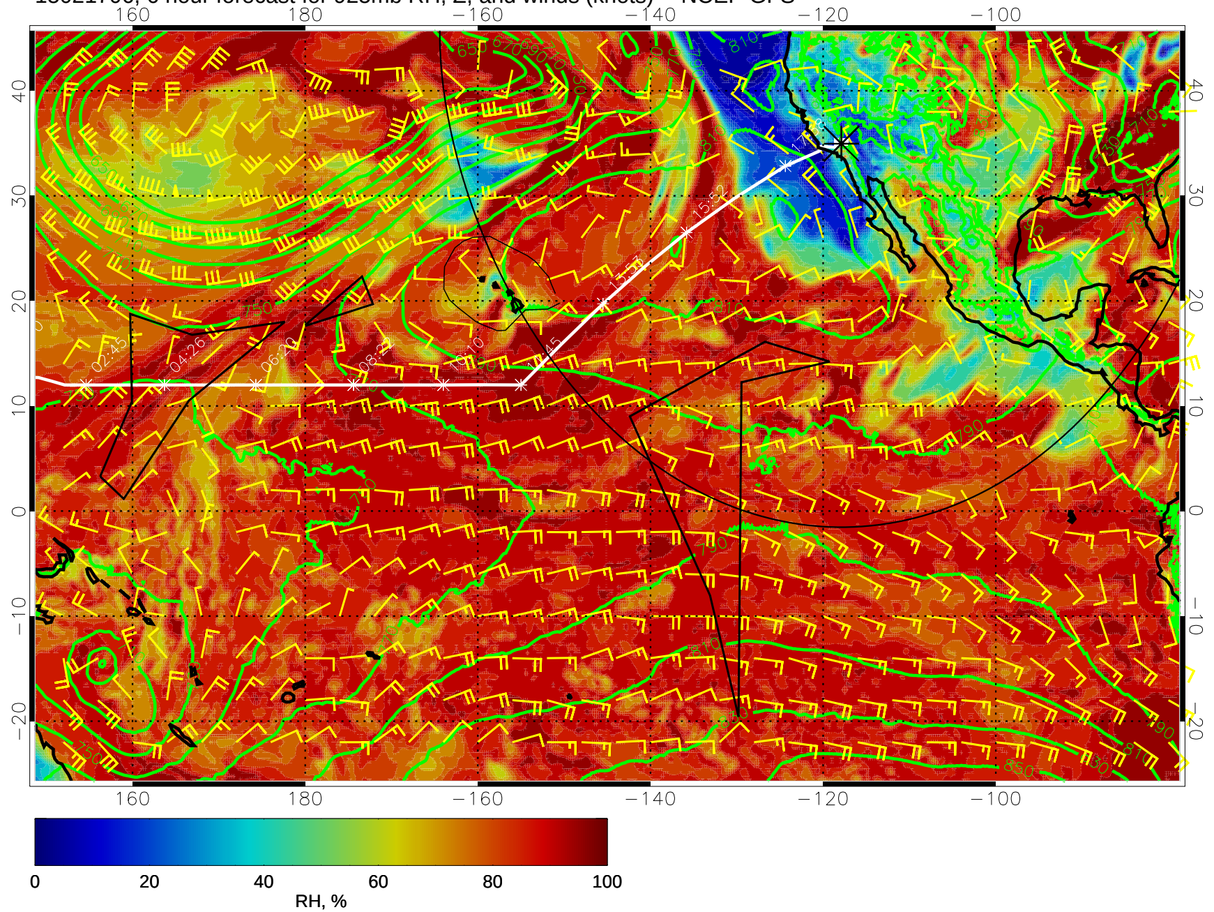
15021706, 6 hour forecast for 925mb RH, Z, and winds (knots) -- NCEP GFS
