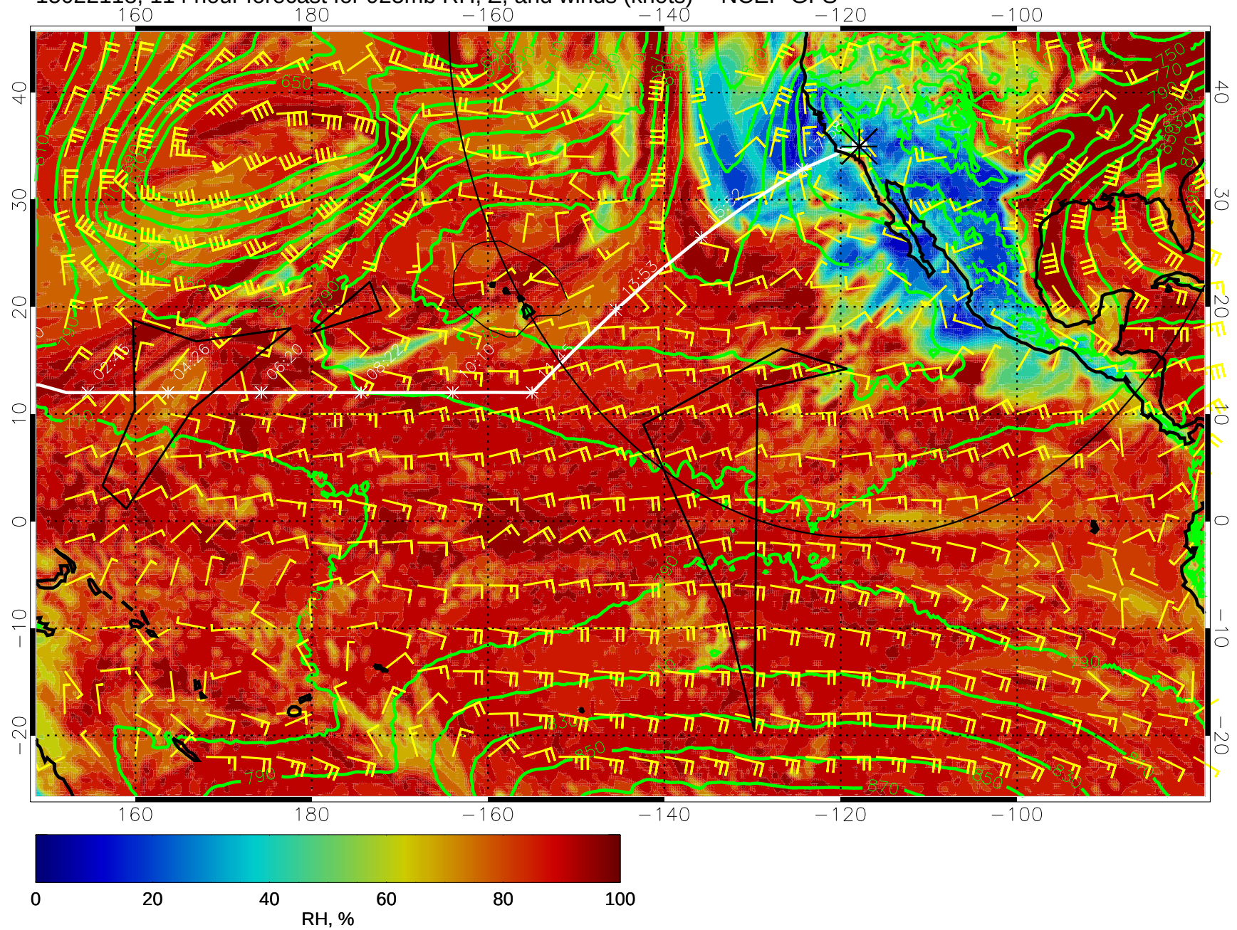
15022118, 114 hour forecast for 925mb RH, Z, and winds (knots) -- NCEP GFS
