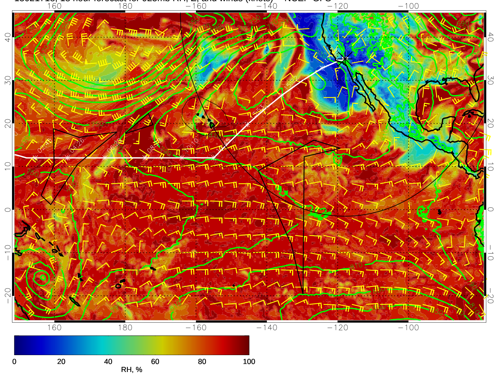
15021718, 18 hour forecast for 925mb RH, Z, and winds (knots) -- NCEP GFS
