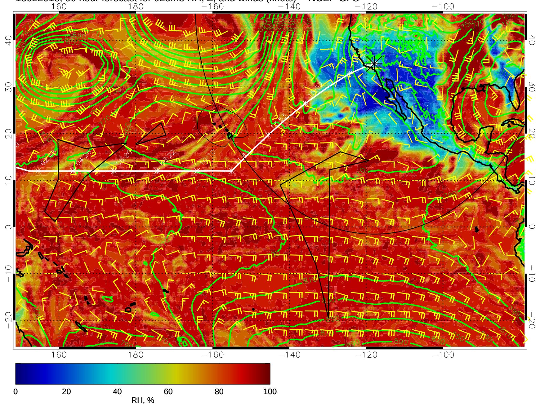
15022018, 90 hour forecast for 925mb RH, Z, and winds (knots) -- NCEP GFS
