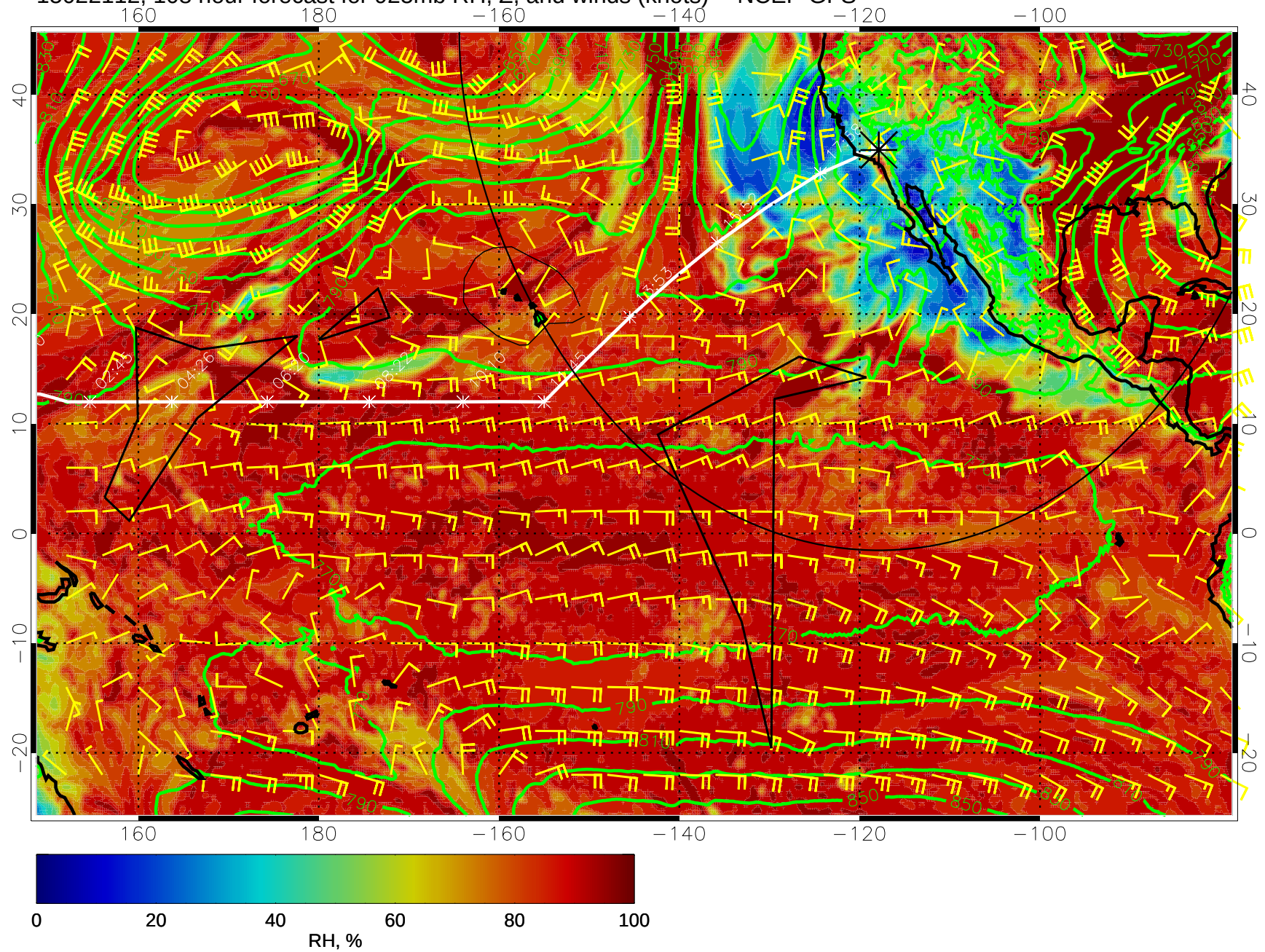
15022112, 108 hour forecast for 925mb RH, Z, and winds (knots) -- NCEP GFS
