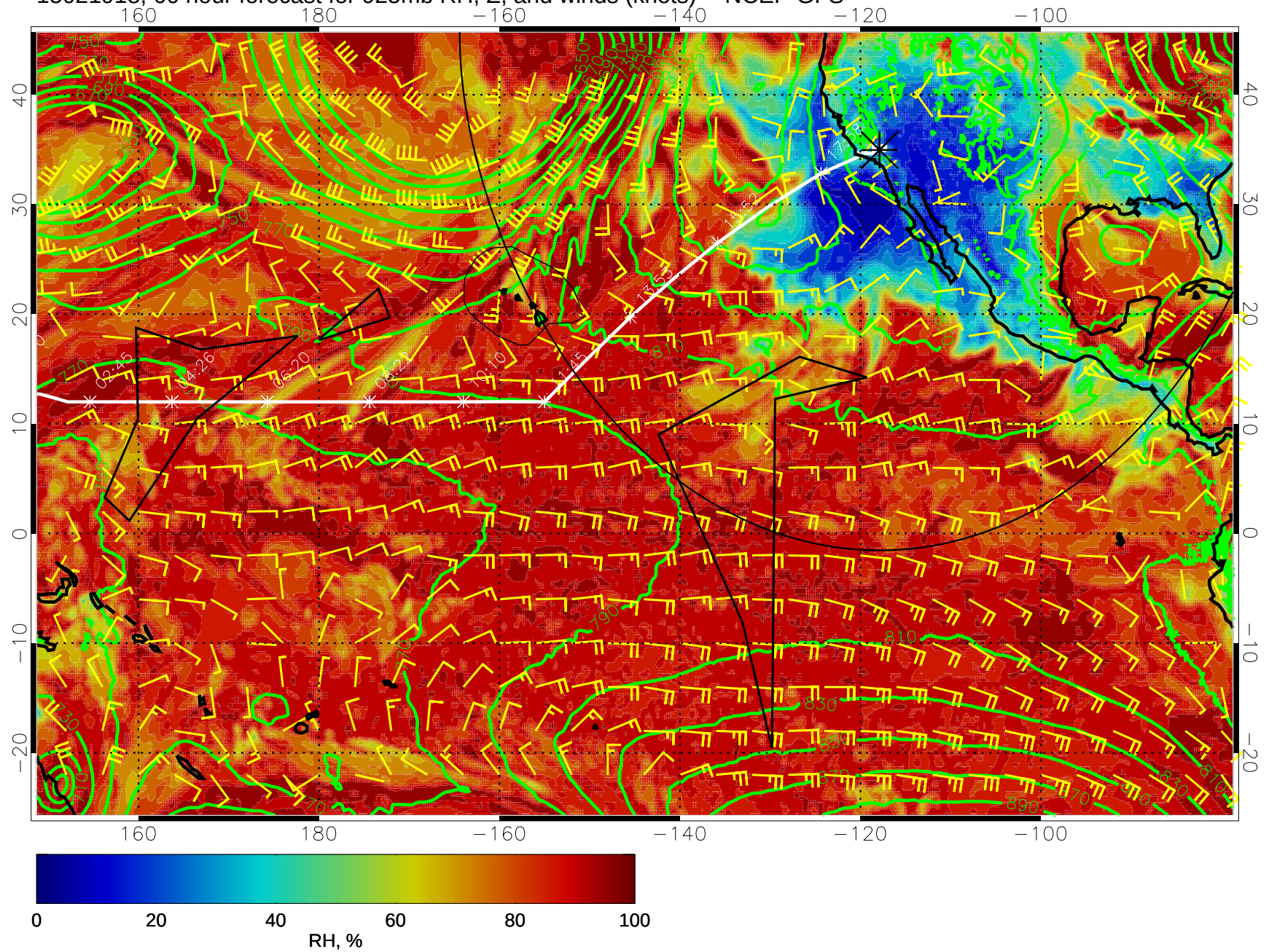
15021918, 66 hour forecast for 925mb RH, Z, and winds (knots) -- NCEP GFS
