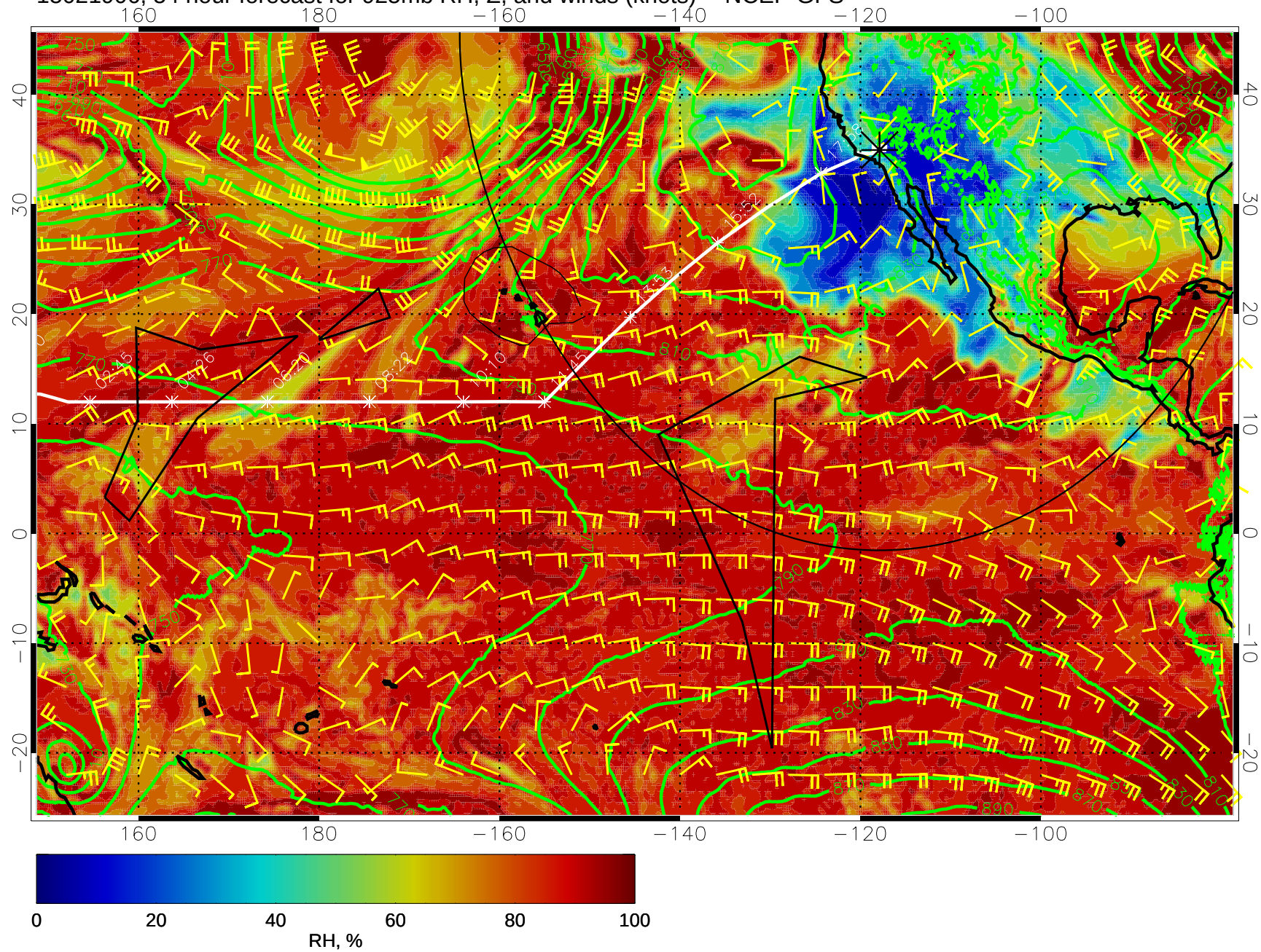
15021906, 54 hour forecast for 925mb RH, Z, and winds (knots) -- NCEP GFS
