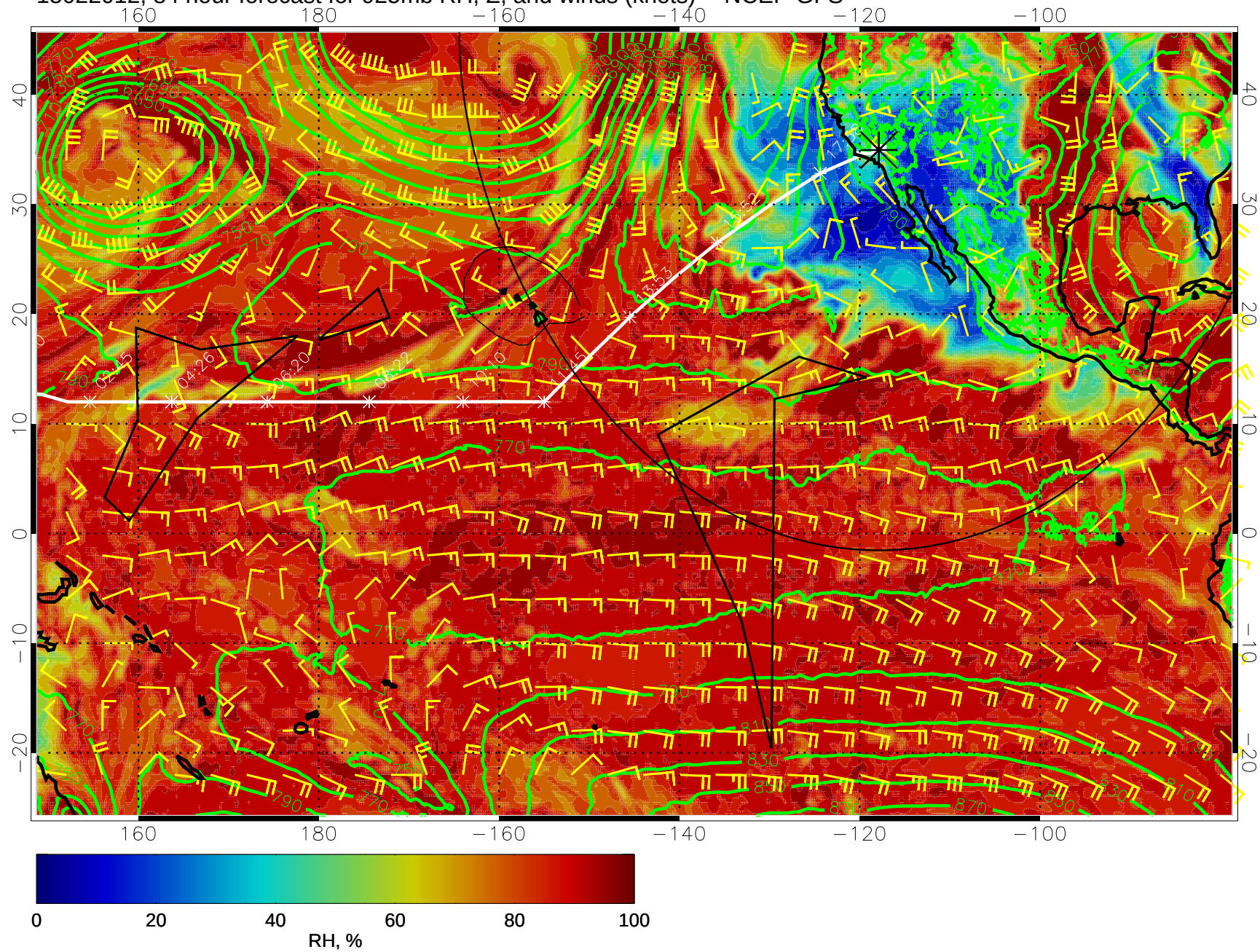
15022012, 84 hour forecast for 925mb RH, Z, and winds (knots) -- NCEP GFS
