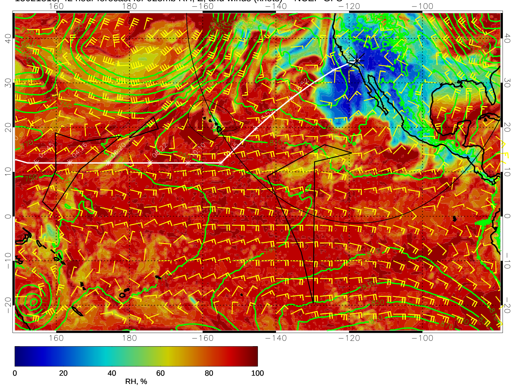
15021818, 42 hour forecast for 925mb RH, Z, and winds (knots) -- NCEP GFS
