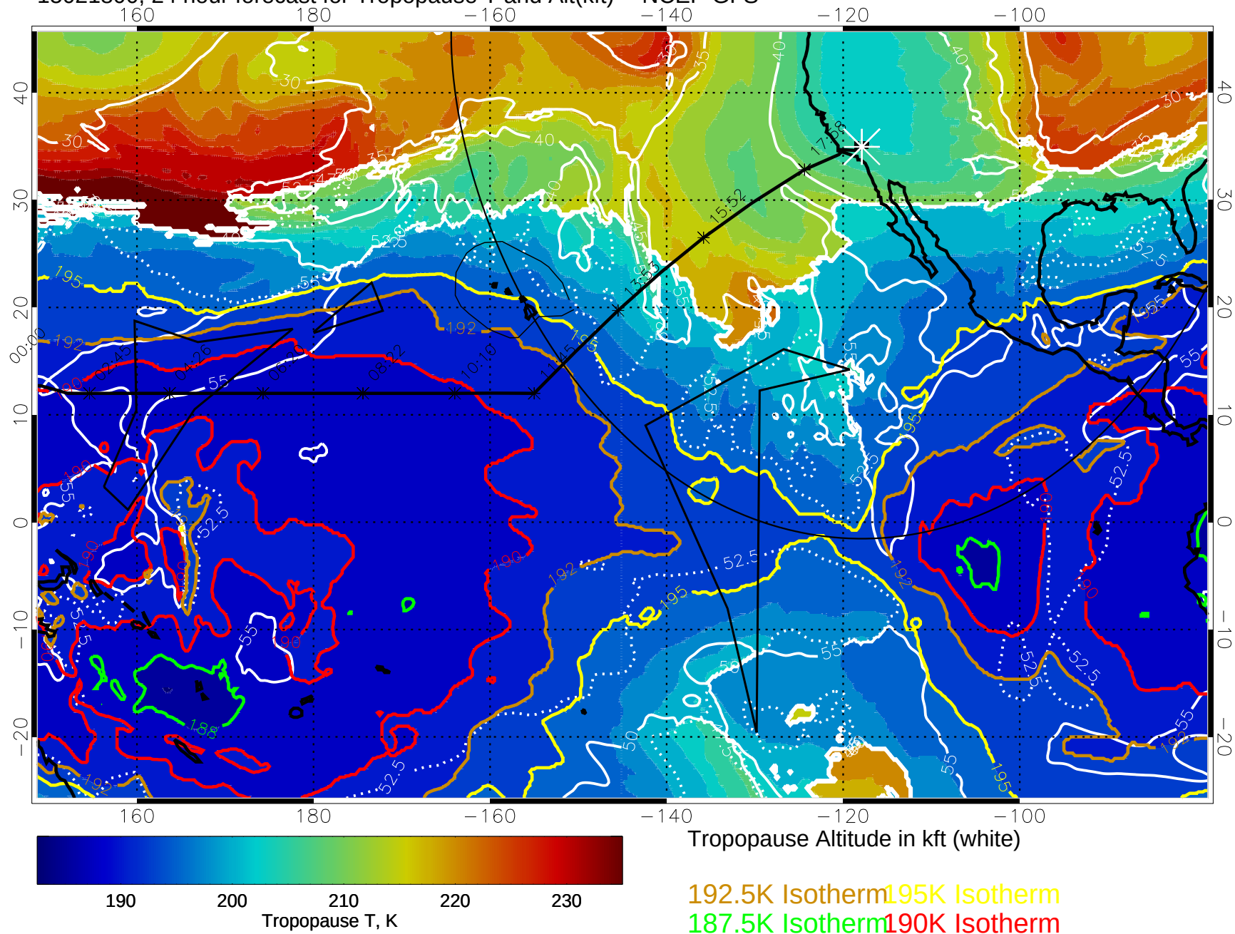
15021800, 24 hour forecast for Tropopause T and Alt(kft) -- NCEP GFS
