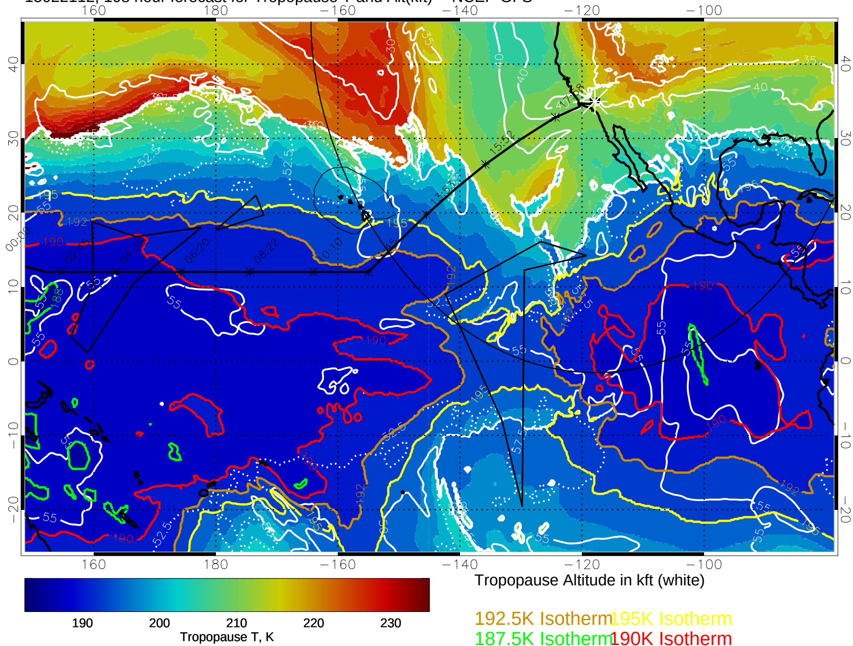
15022112, 108 hour forecast for Tropopause T and Alt(kft) -- NCEP GFS
