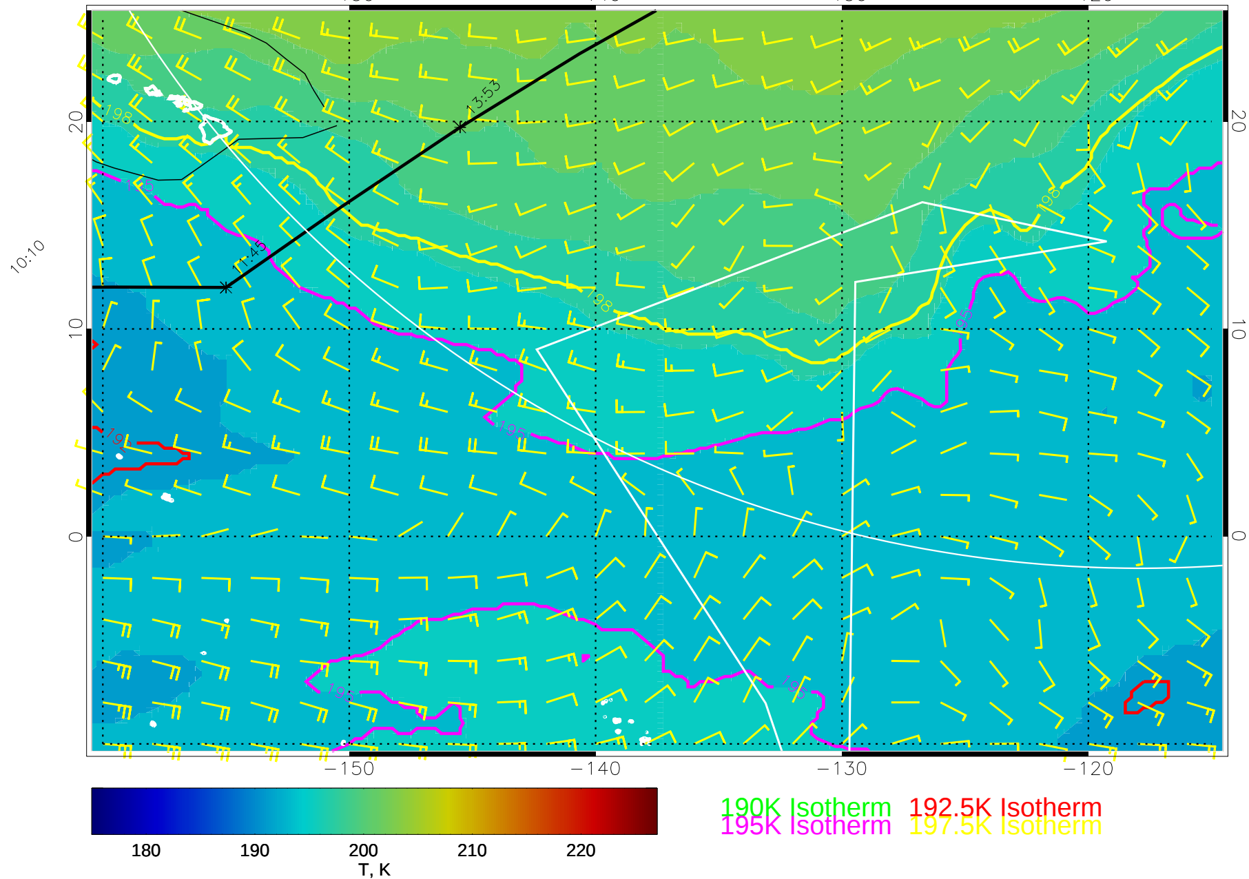
15022200, 120 hour forecast for 70mb T and winds (knots) -- NCEP GFS
