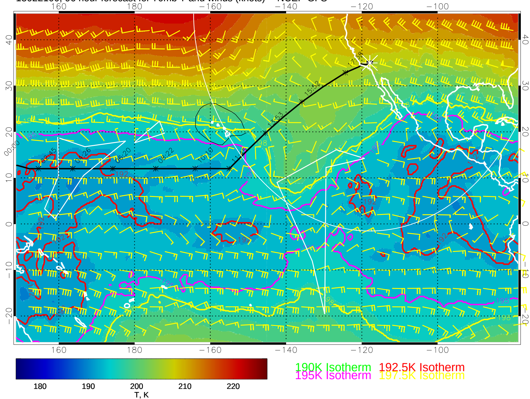
15022100, 96 hour forecast for 70mb T and winds (knots) -- NCEP GFS
