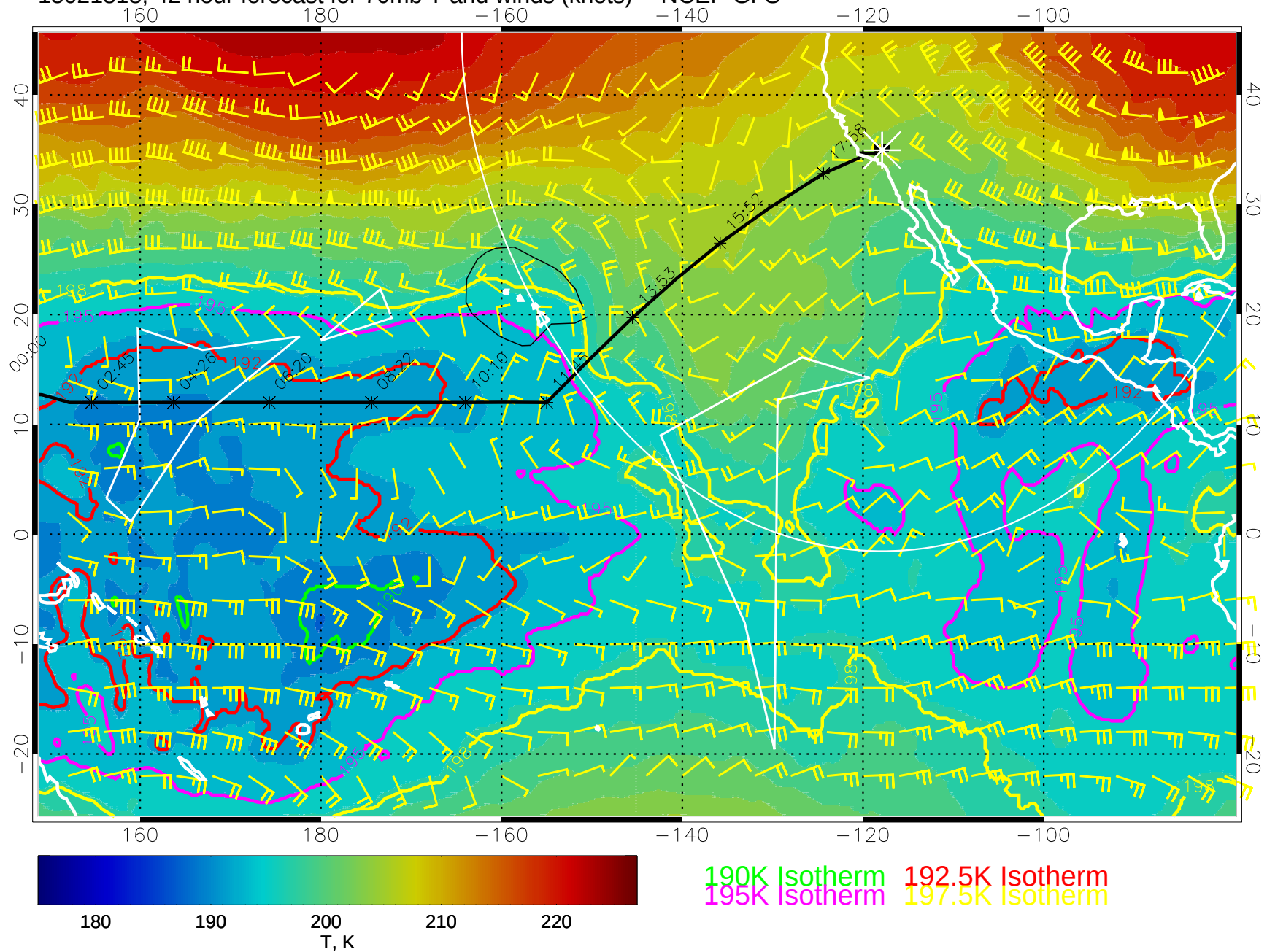
15021818, 42 hour forecast for 70mb T and winds (knots) -- NCEP GFS
