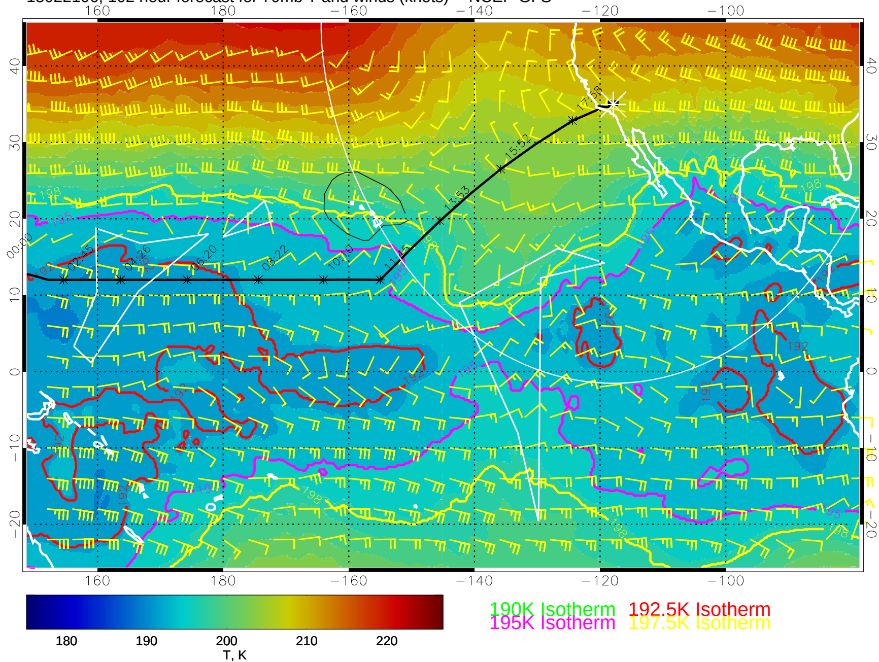
15022106, 102 hour forecast for 70mb T and winds (knots) -- NCEP GFS
