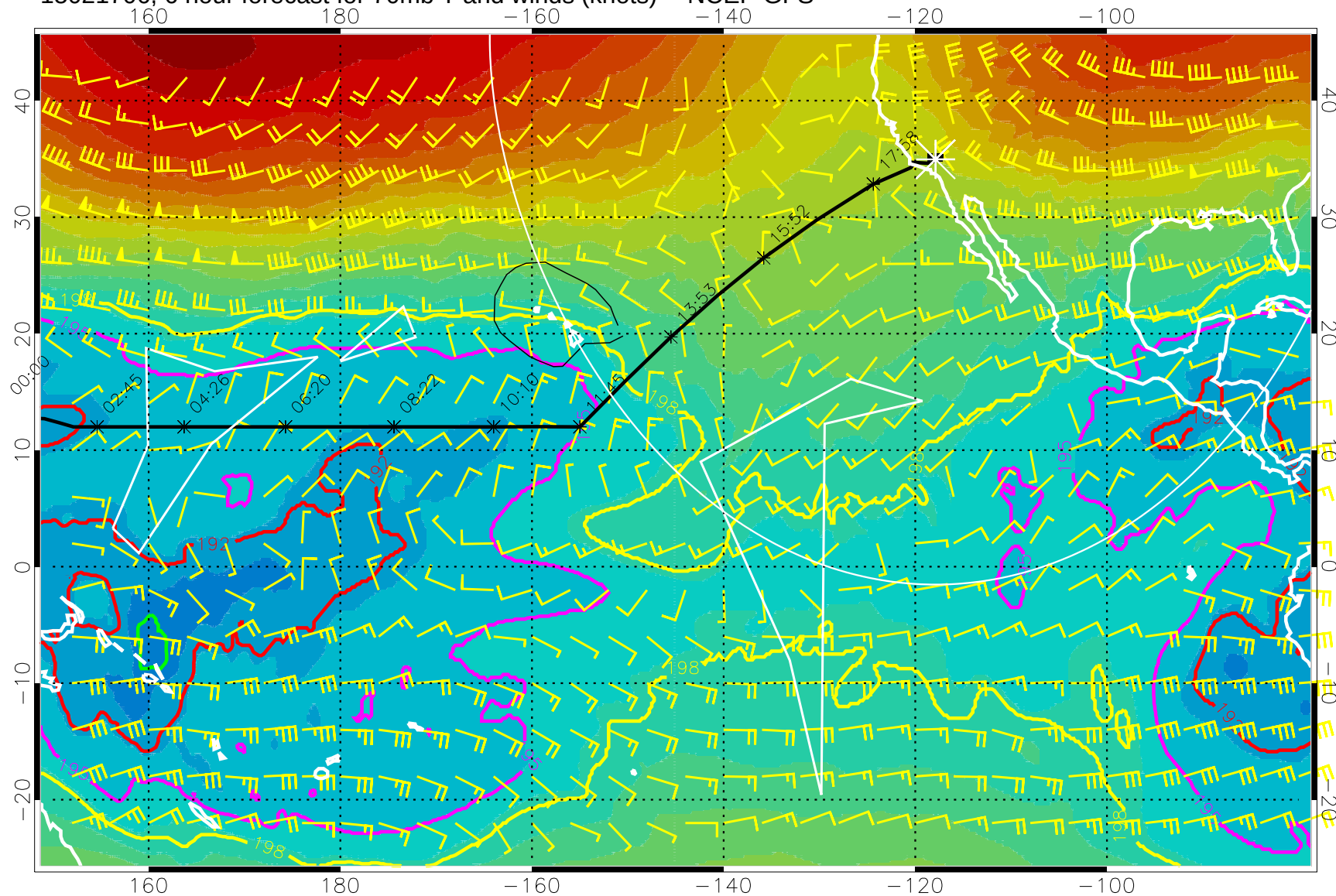
15021706, 6 hour forecast for 70mb T and winds (knots) -- NCEP GFS
