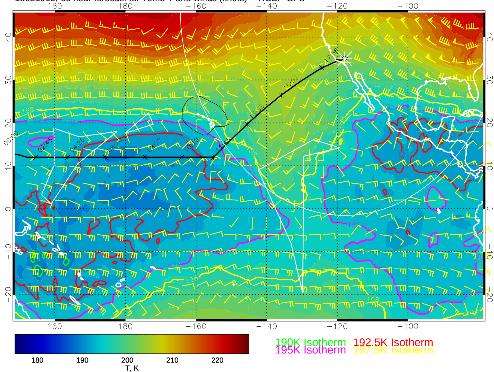
15021912, 60 hour forecast for 70mb T and winds (knots) -- NCEP GFS
