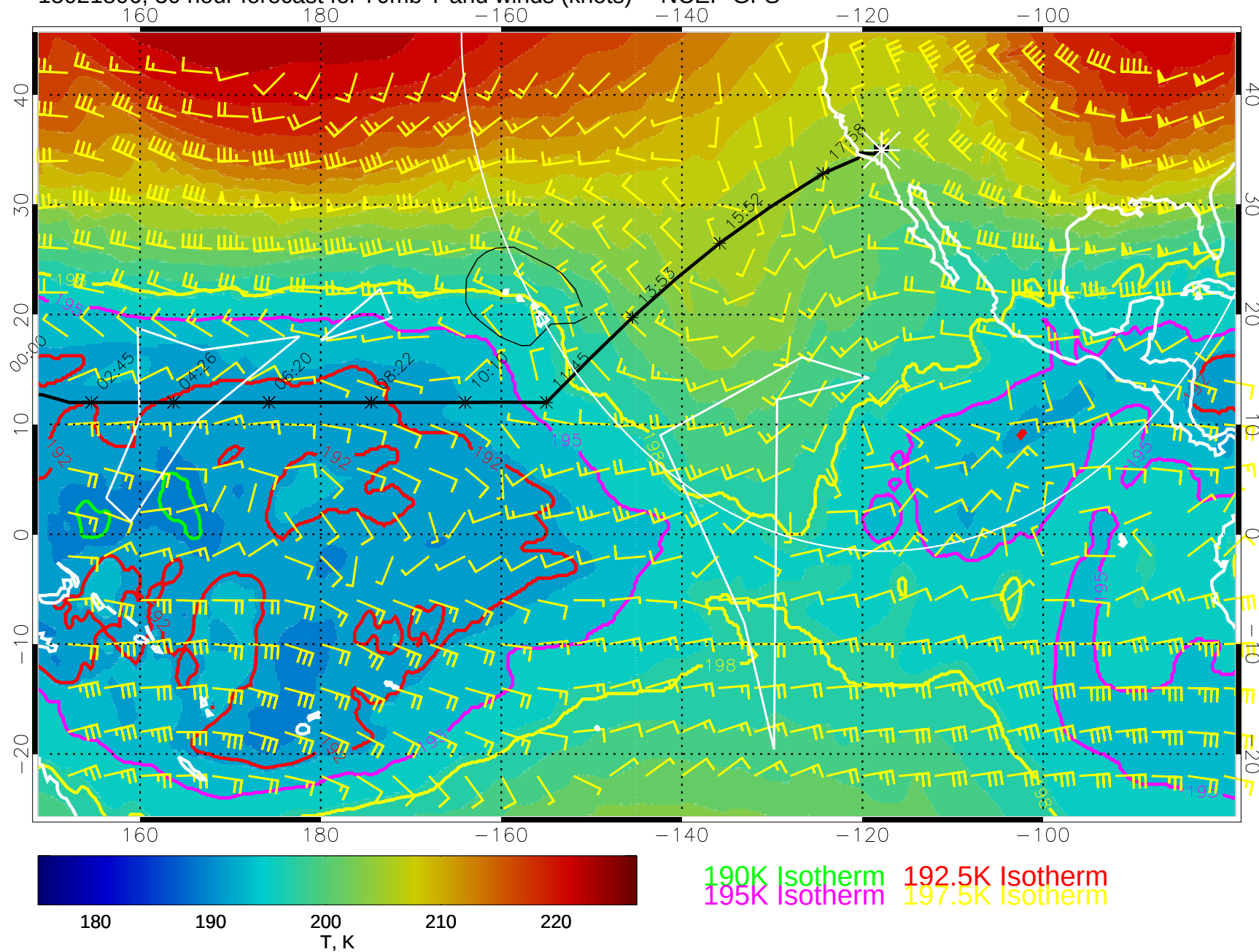
15021806, 30 hour forecast for 70mb T and winds (knots) -- NCEP GFS
