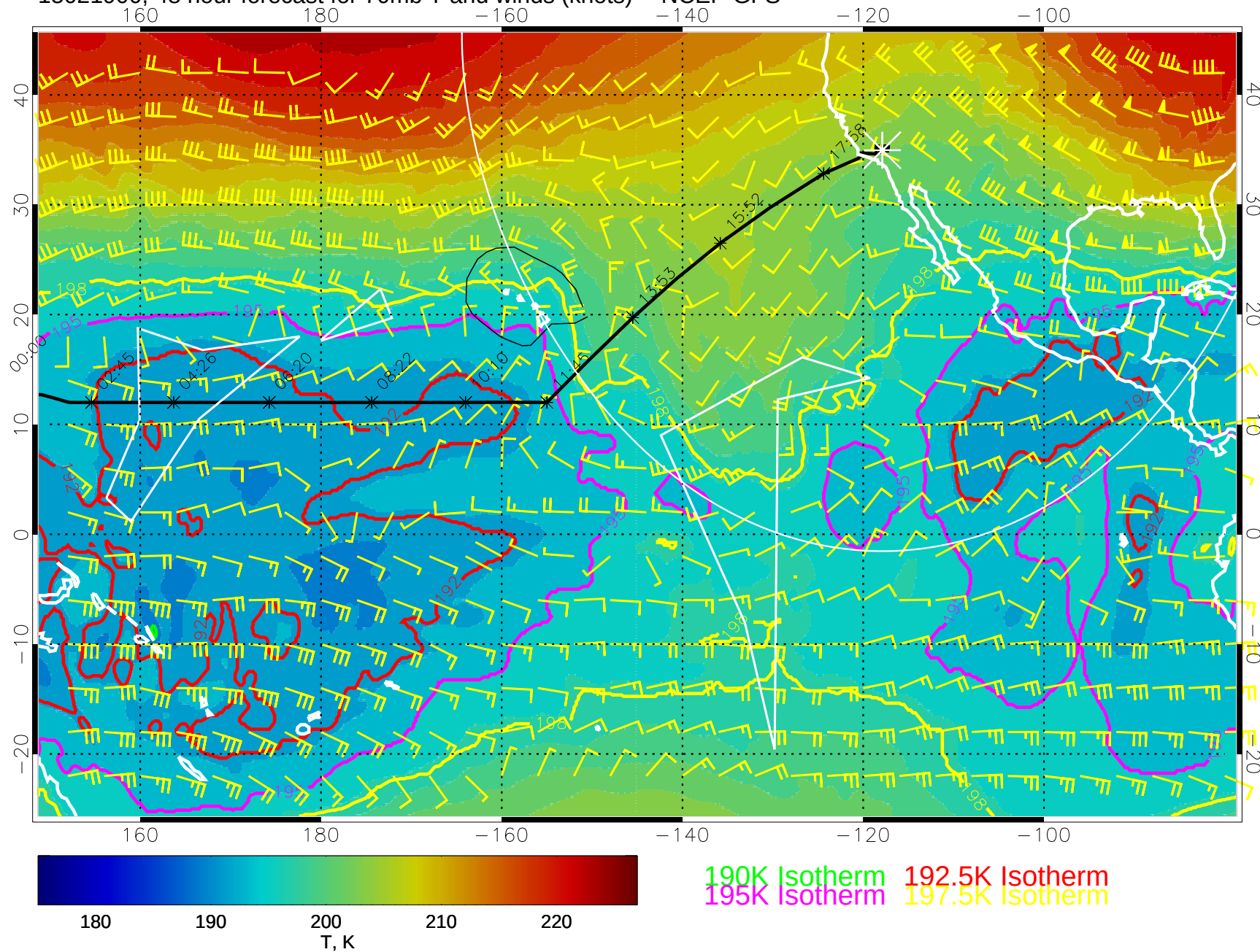
15021900, 48 hour forecast for 70mb T and winds (knots) -- NCEP GFS
