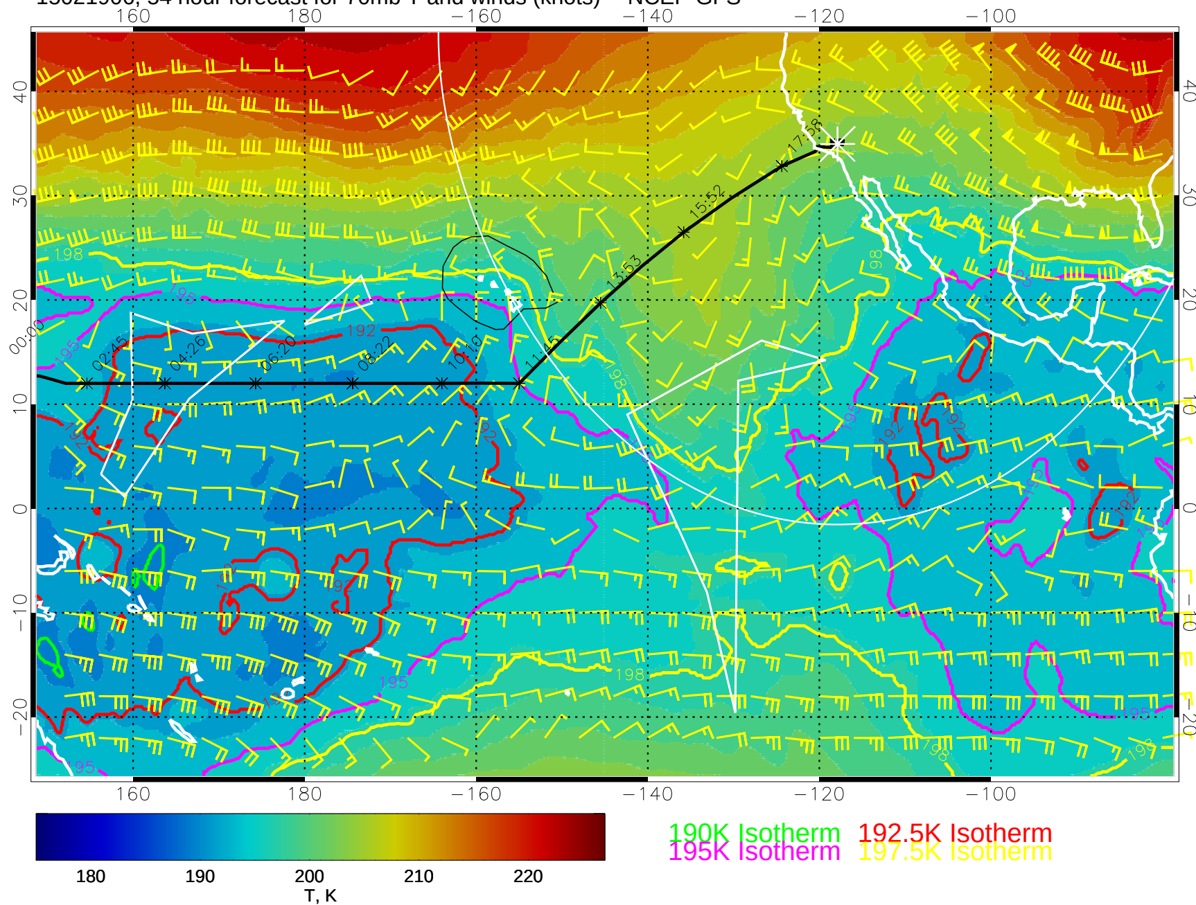
15021906, 54 hour forecast for 70mb T and winds (knots) -- NCEP GFS
