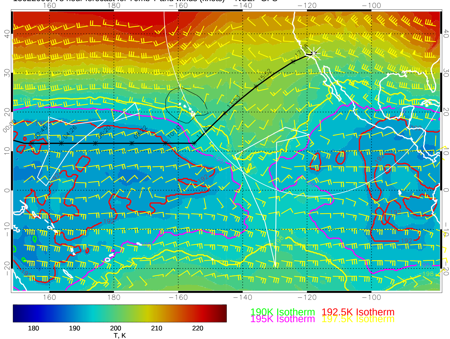
15022006, 78 hour forecast for 70mb T and winds (knots) -- NCEP GFS
