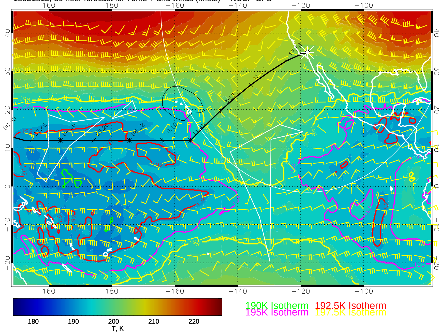
15021812, 36 hour forecast for 70mb T and winds (knots) -- NCEP GFS
