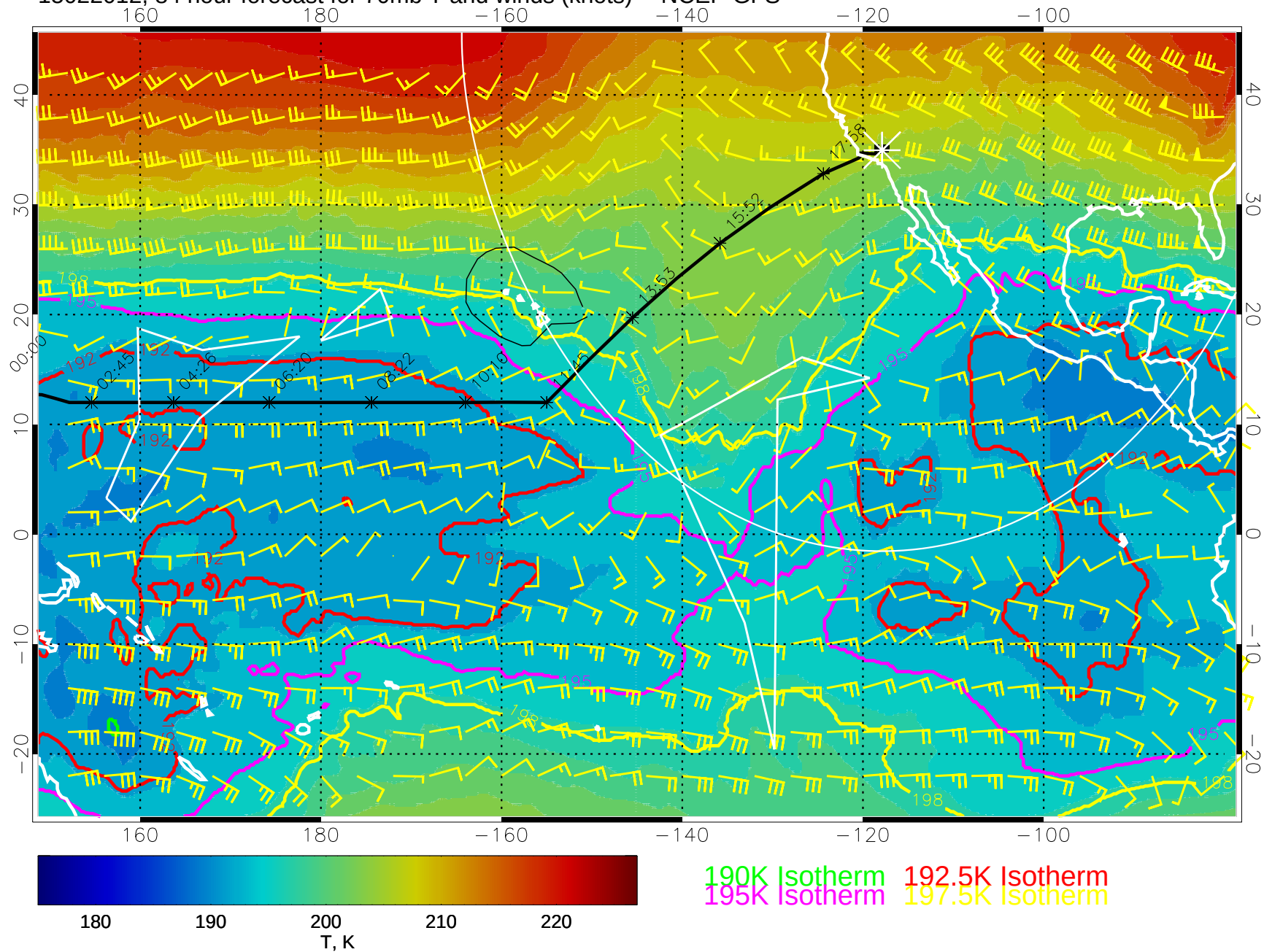
15022012, 84 hour forecast for 70mb T and winds (knots) -- NCEP GFS
