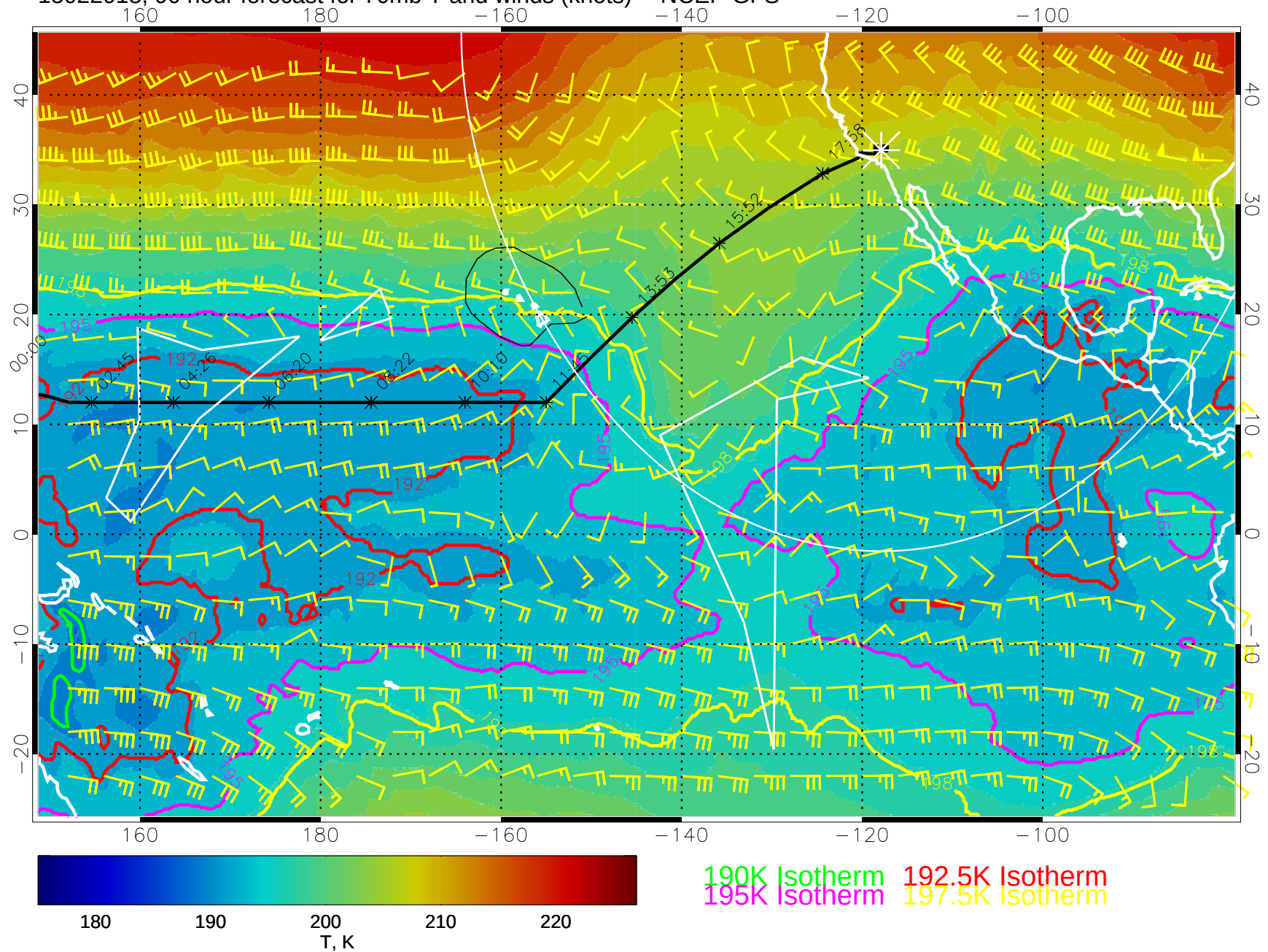
15022018, 90 hour forecast for 70mb T and winds (knots) -- NCEP GFS
