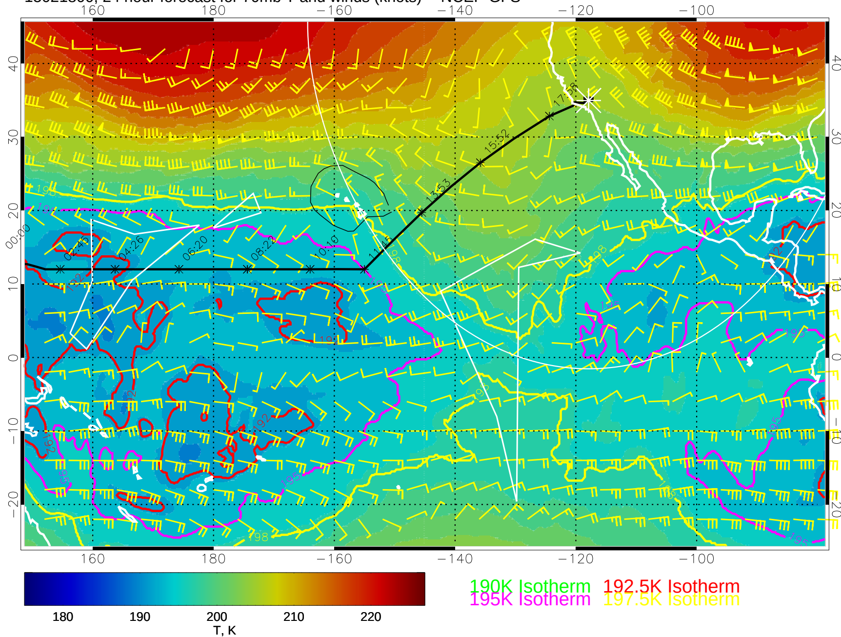
15021800, 24 hour forecast for 70mb T and winds (knots) -- NCEP GFS
