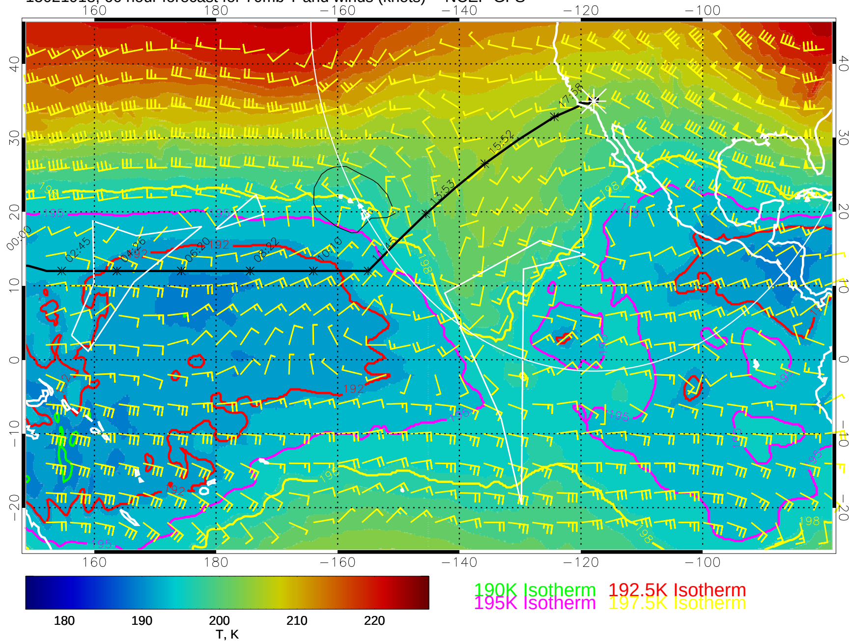
15021918, 66 hour forecast for 70mb T and winds (knots) -- NCEP GFS
