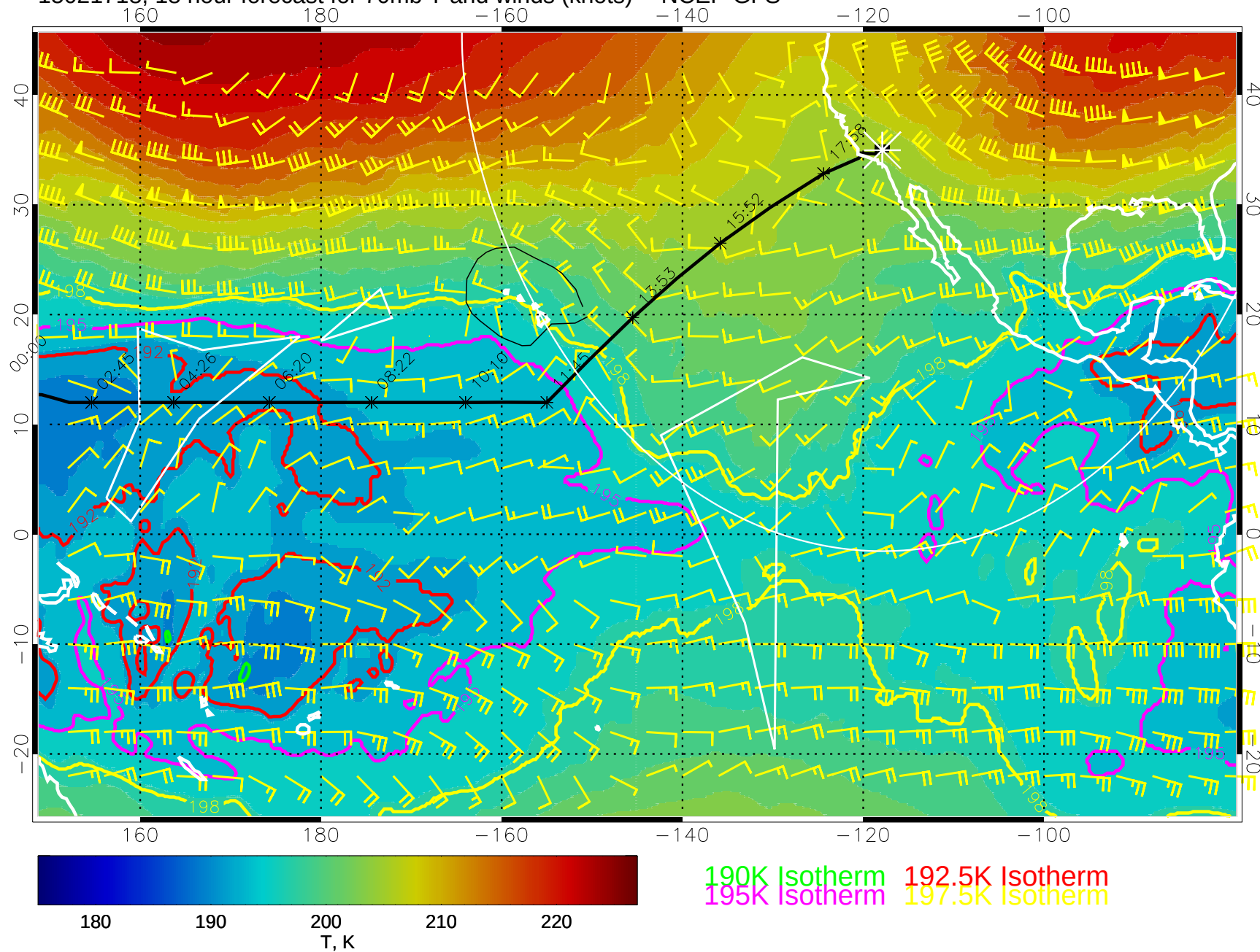
15021718, 18 hour forecast for 70mb T and winds (knots) -- NCEP GFS
