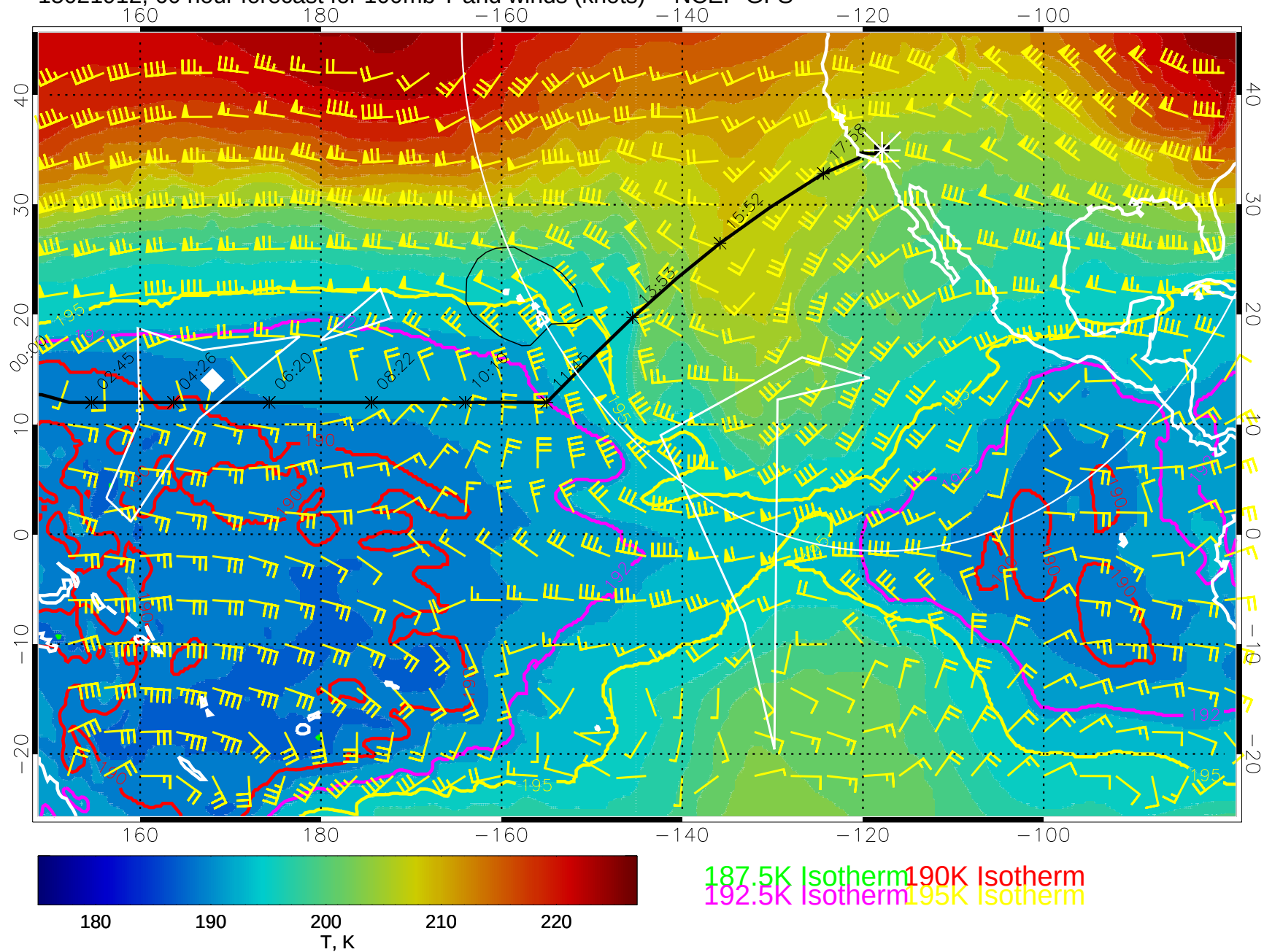
15021912, 60 hour forecast for 100mb T and winds (knots) -- NCEP GFS
