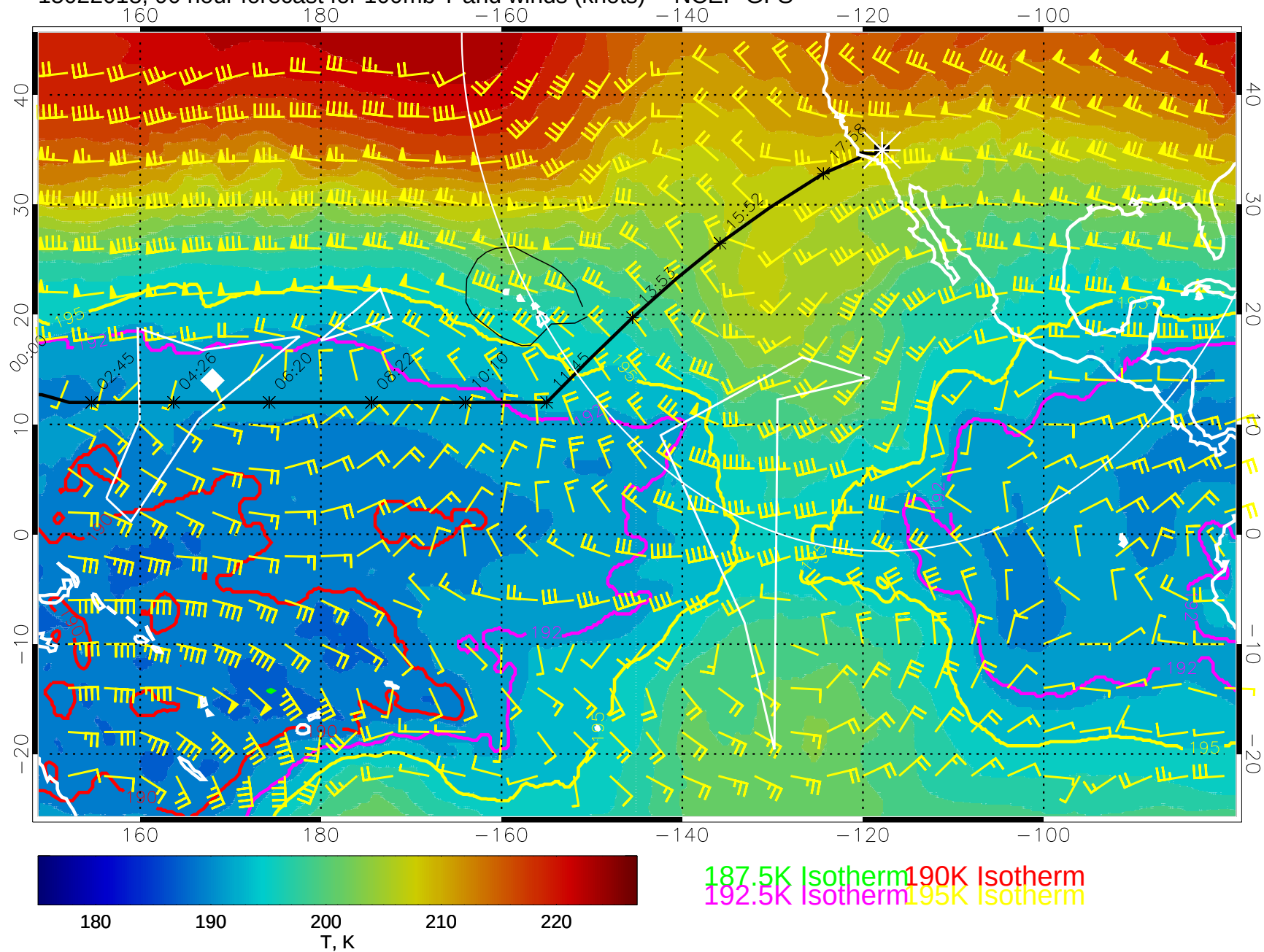
15022018, 90 hour forecast for 100mb T and winds (knots) -- NCEP GFS
