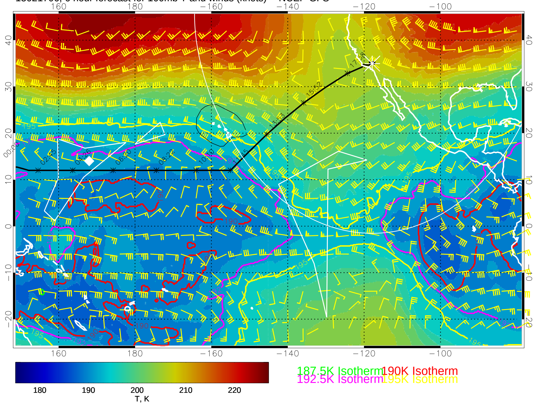
15021706, 6 hour forecast for 100mb T and winds (knots) -- NCEP GFS
