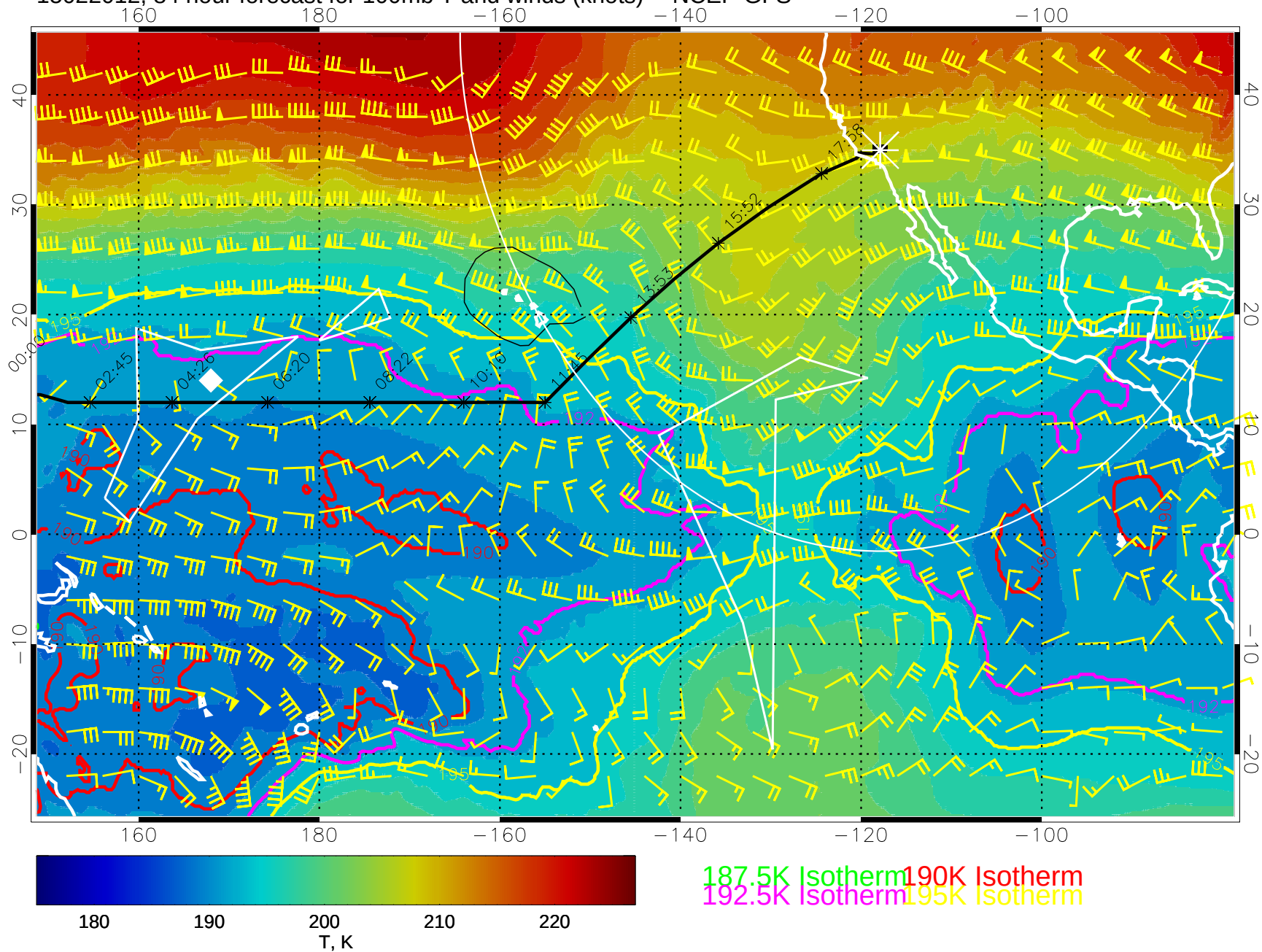
15022012, 84 hour forecast for 100mb T and winds (knots) -- NCEP GFS
