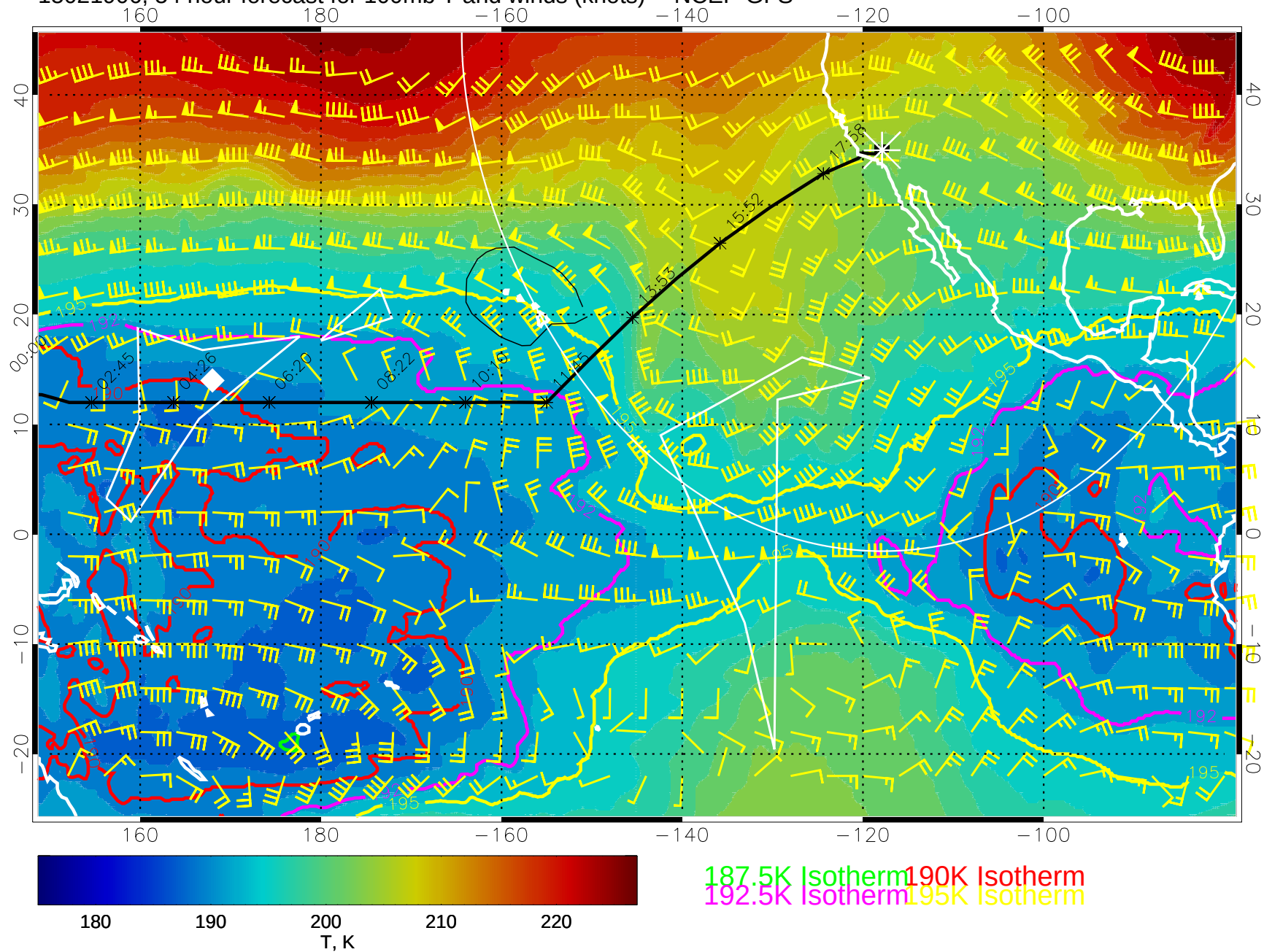
15021906, 54 hour forecast for 100mb T and winds (knots) -- NCEP GFS
