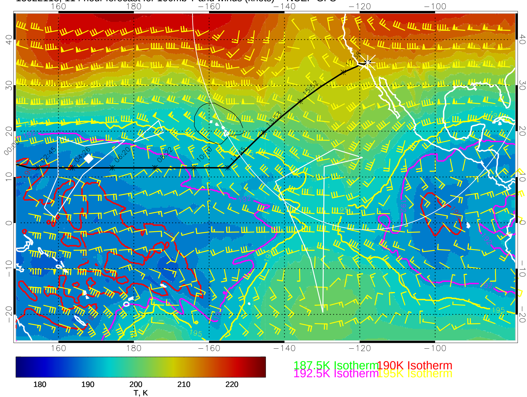
15022118, 114 hour forecast for 100mb T and winds (knots) -- NCEP GFS
