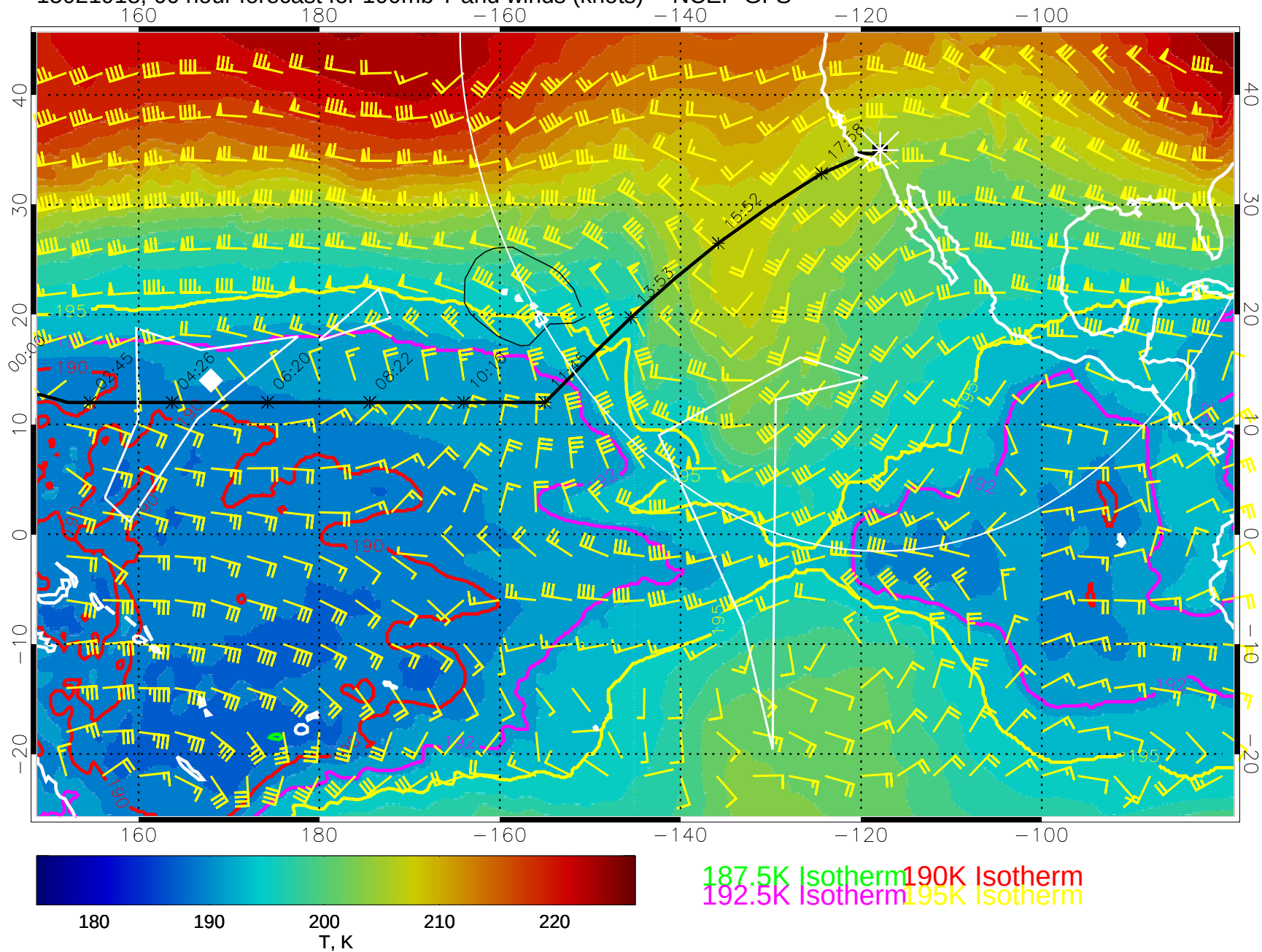
15021918, 66 hour forecast for 100mb T and winds (knots) -- NCEP GFS
