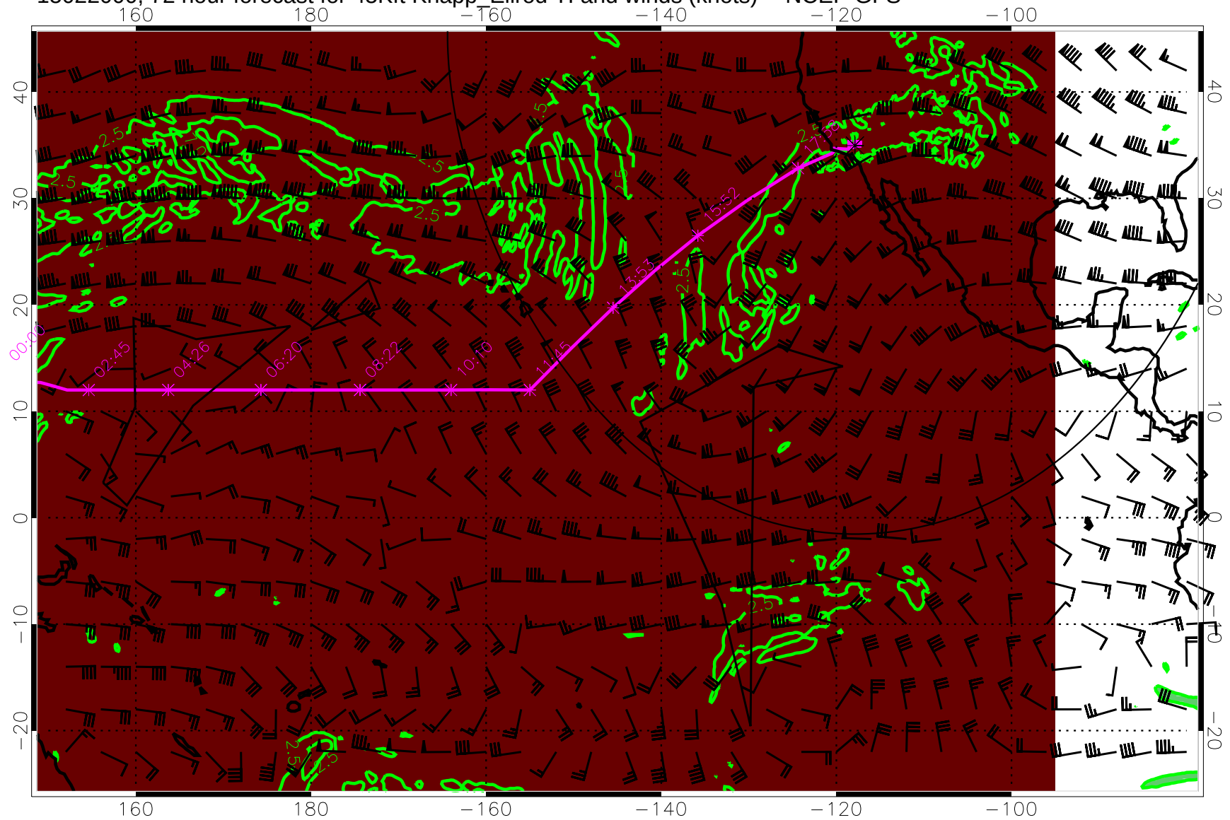
15022000, 72 hour forecast for 45Kft Knapp_Ellrod TI and winds (knots) -- NCEP GFS
