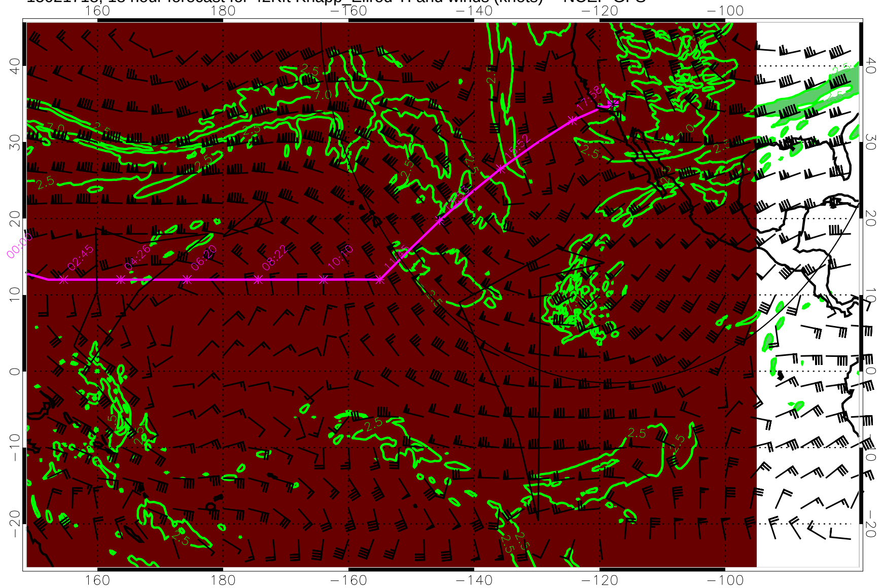
15021718, 18 hour forecast for 42Kft Knapp_Ellrod TI and winds (knots) -- NCEP GFS
