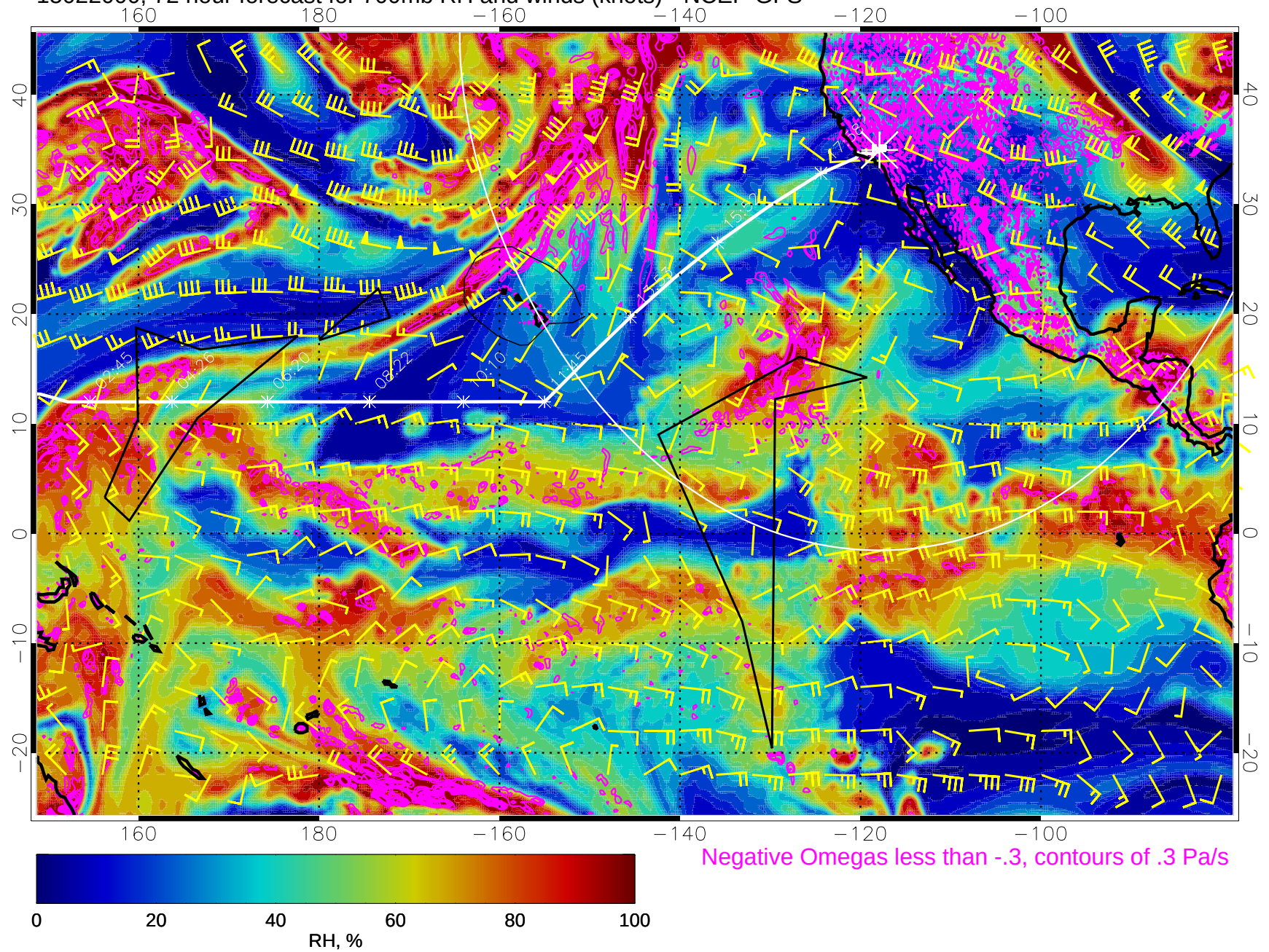
15022000, 72 hour forecast for 700mb RH and winds (knots) - NCEP GFS
