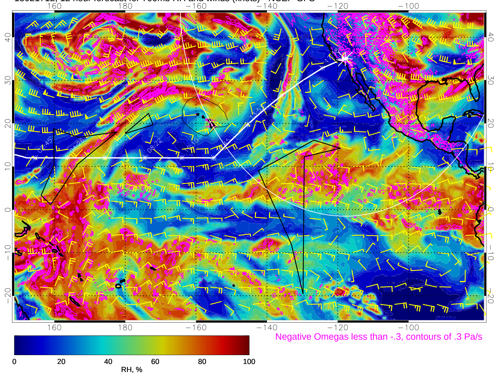
15021712, 12 hour forecast for 700mb RH and winds (knots) - NCEP GFS
