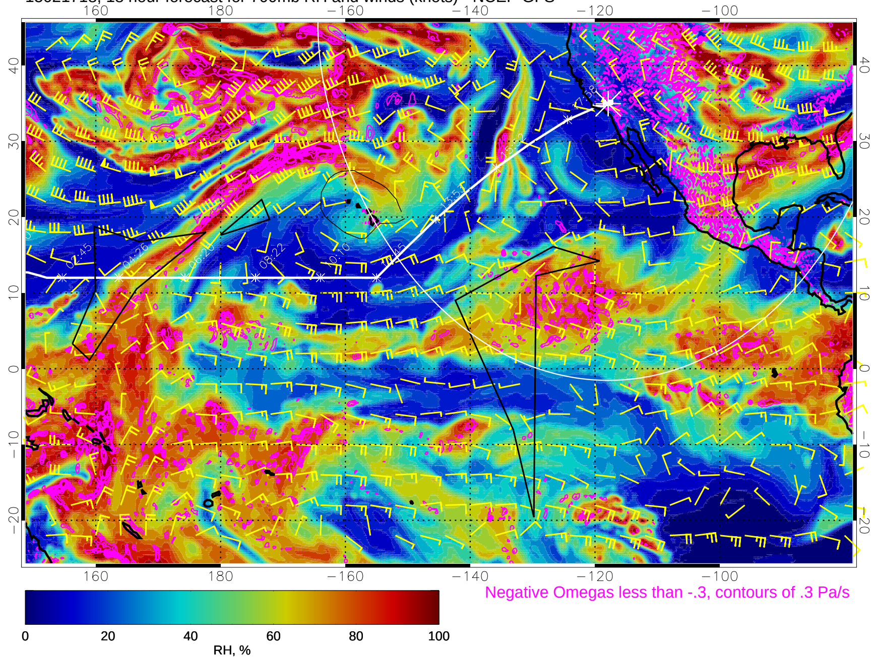
15021718, 18 hour forecast for 700mb RH and winds (knots) - NCEP GFS
