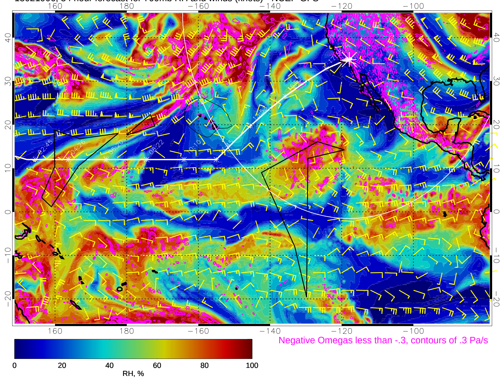
15021906, 54 hour forecast for 700mb RH and winds (knots) - NCEP GFS
