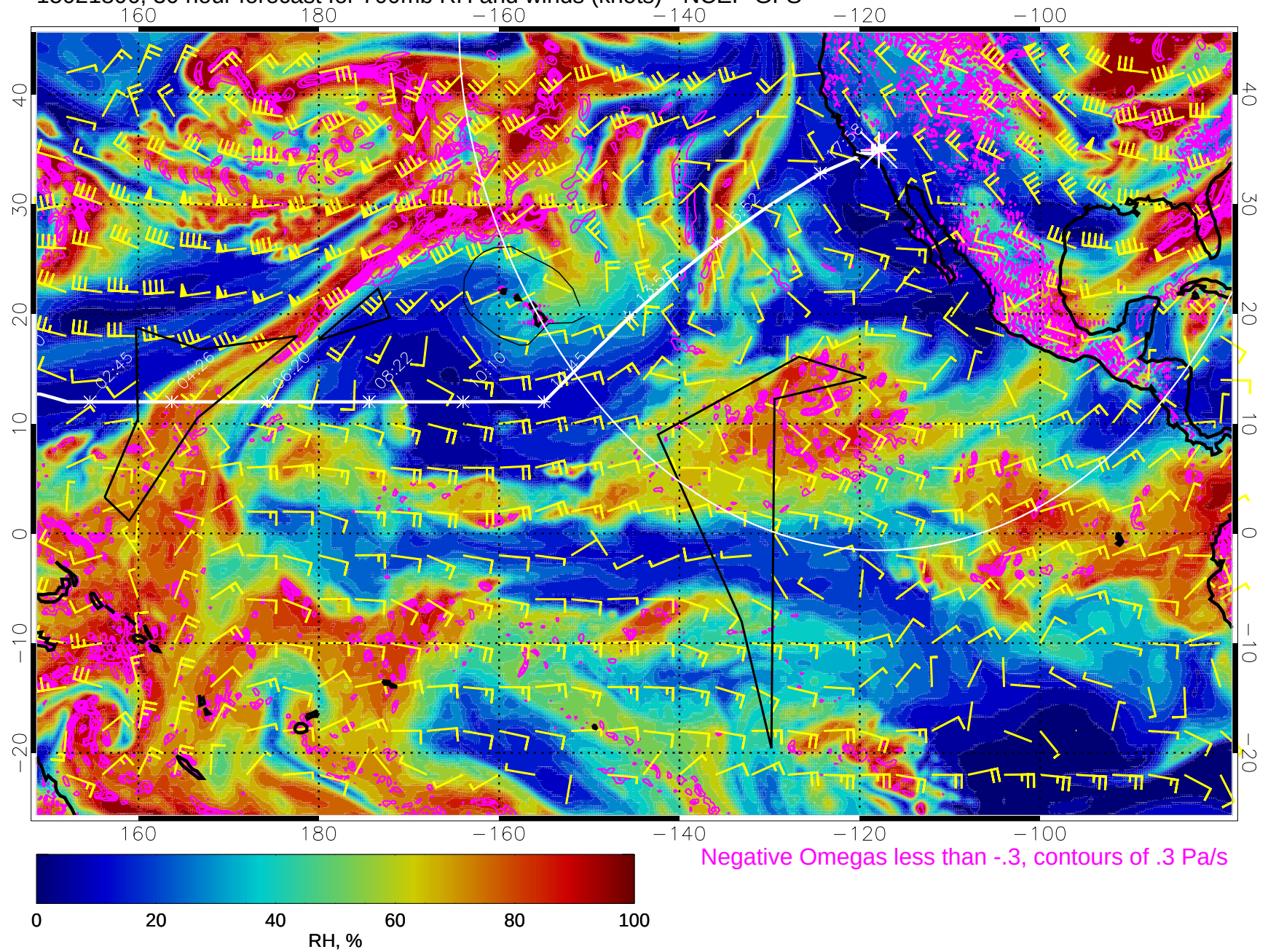
15021806, 30 hour forecast for 700mb RH and winds (knots) - NCEP GFS
