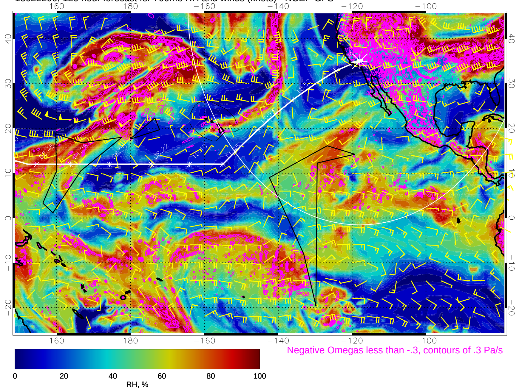
15022200, 120 hour forecast for 700mb RH and winds (knots) - NCEP GFS
