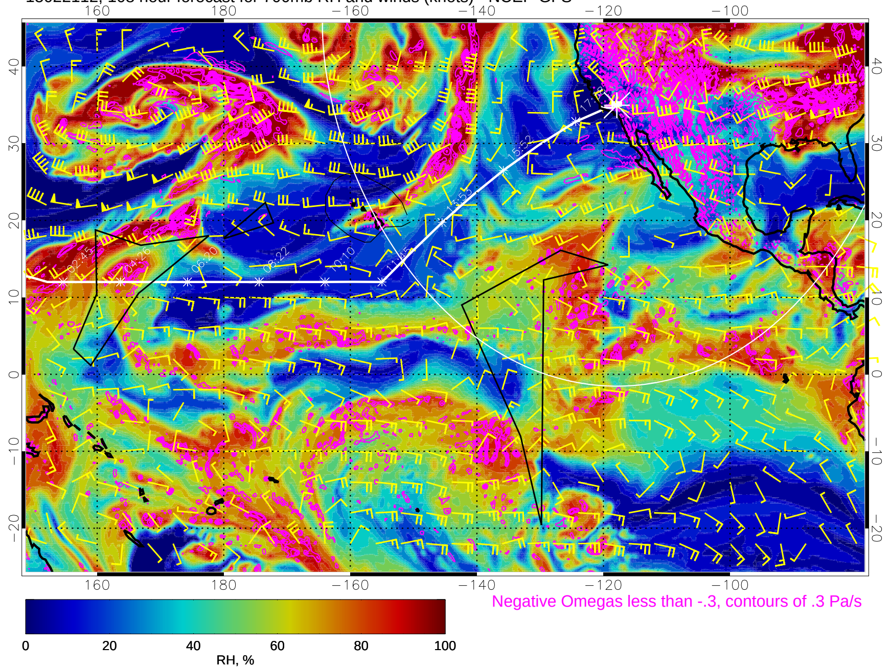
15022112, 108 hour forecast for 700mb RH and winds (knots) - NCEP GFS
