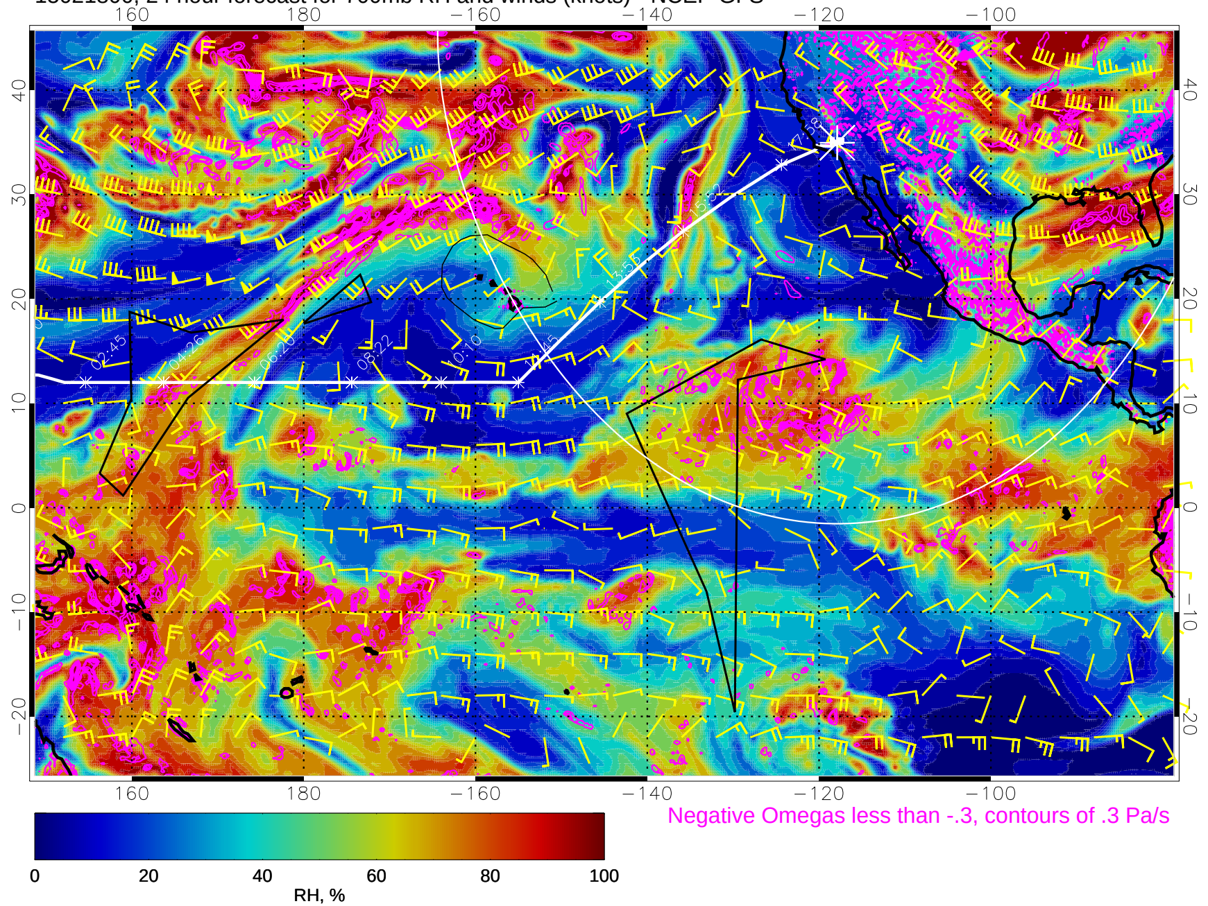
15021800, 24 hour forecast for 700mb RH and winds (knots) - NCEP GFS
