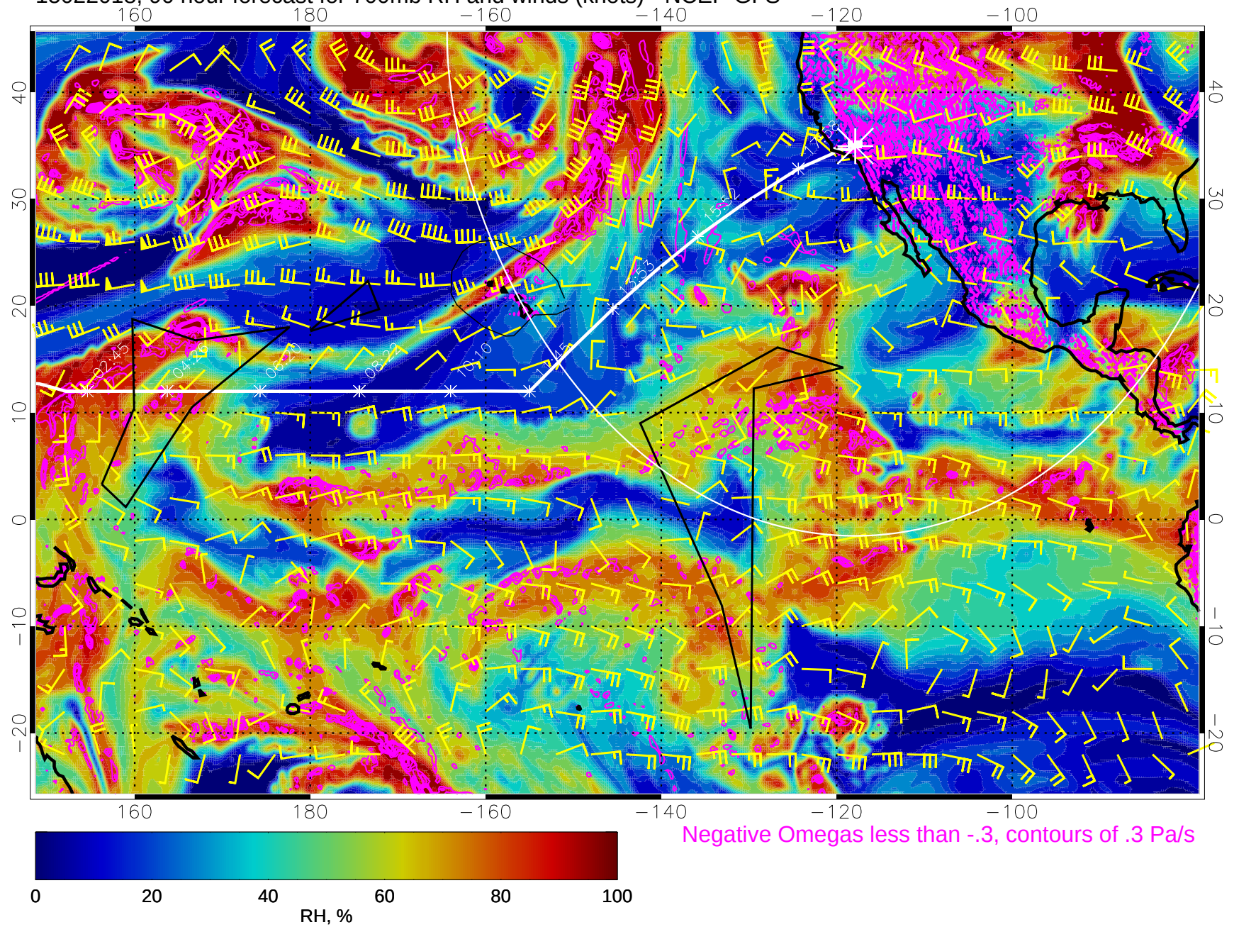
15022018, 90 hour forecast for 700mb RH and winds (knots) - NCEP GFS
