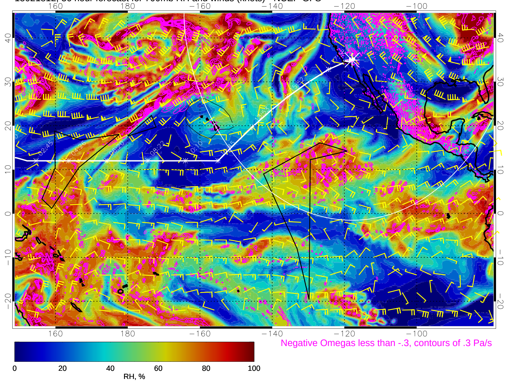
15021812, 36 hour forecast for 700mb RH and winds (knots) - NCEP GFS
