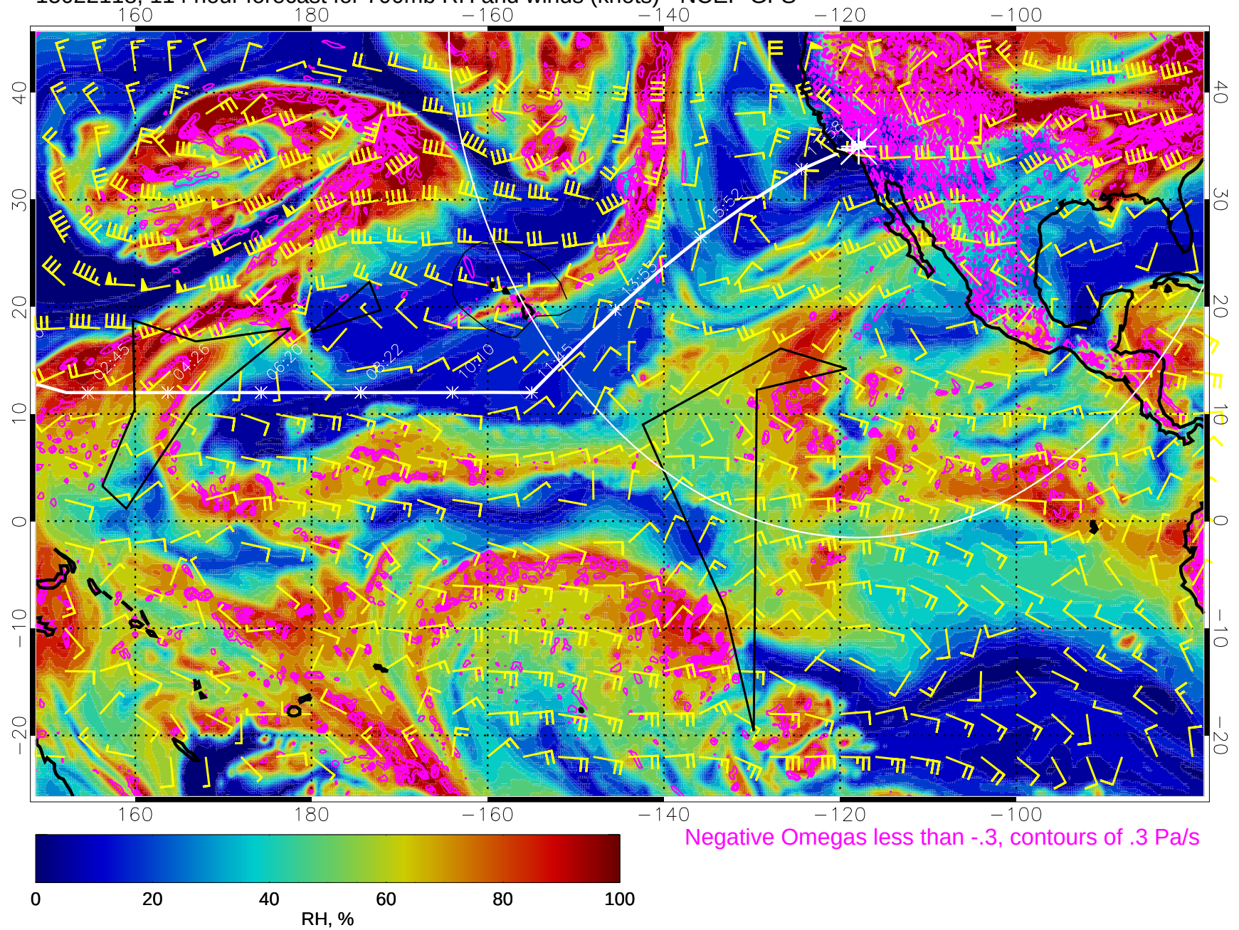
15022118, 114 hour forecast for 700mb RH and winds (knots) - NCEP GFS
