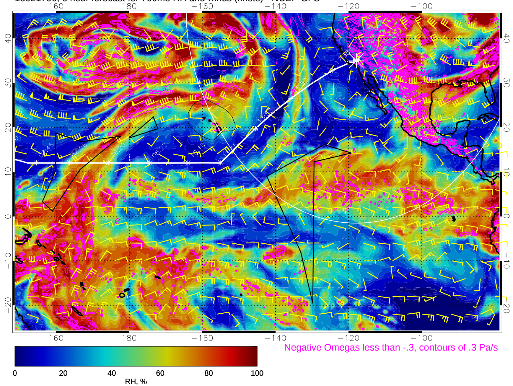
15021706, 6 hour forecast for 700mb RH and winds (knots) - NCEP GFS
