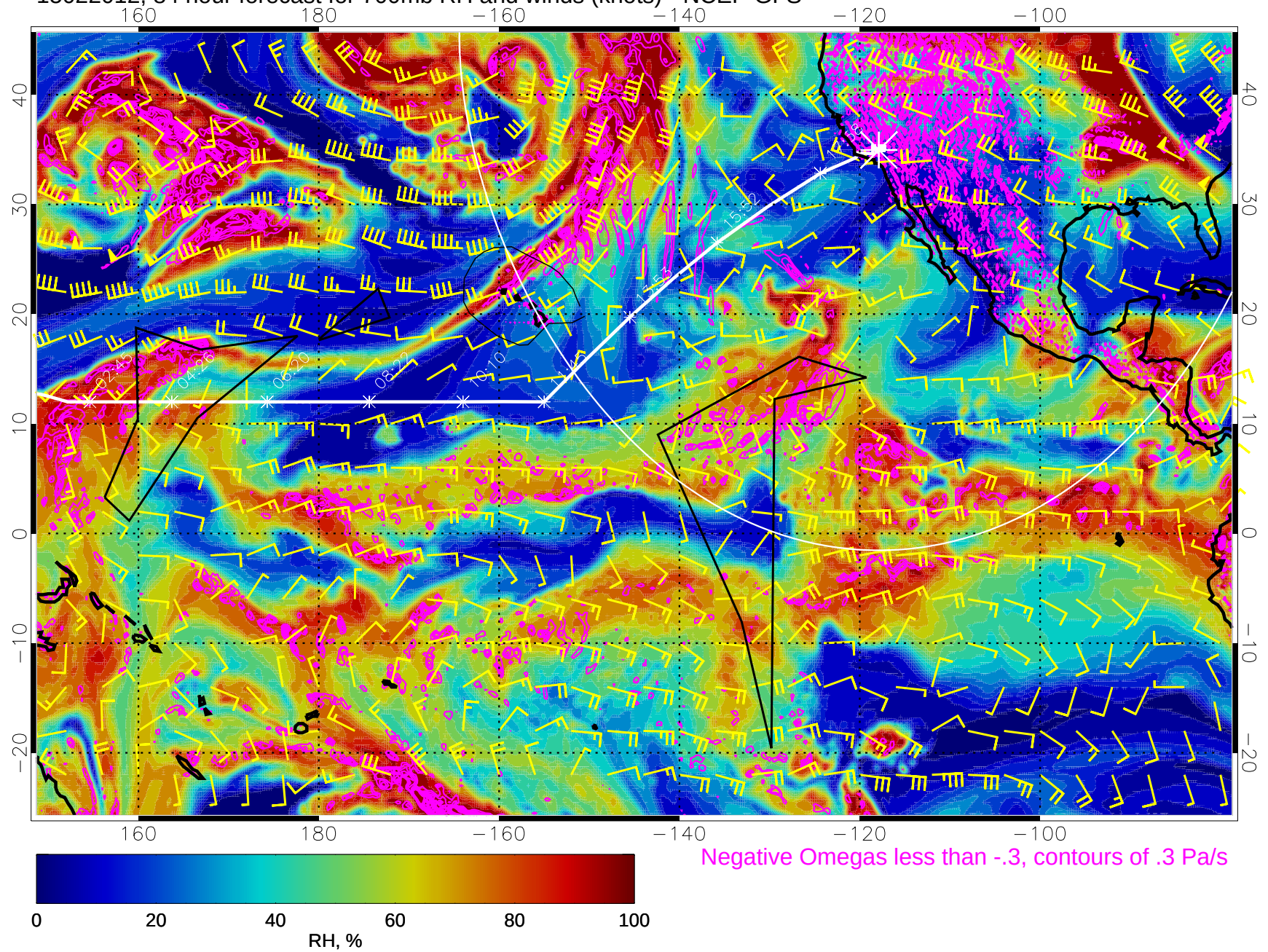
15022012, 84 hour forecast for 700mb RH and winds (knots) - NCEP GFS
