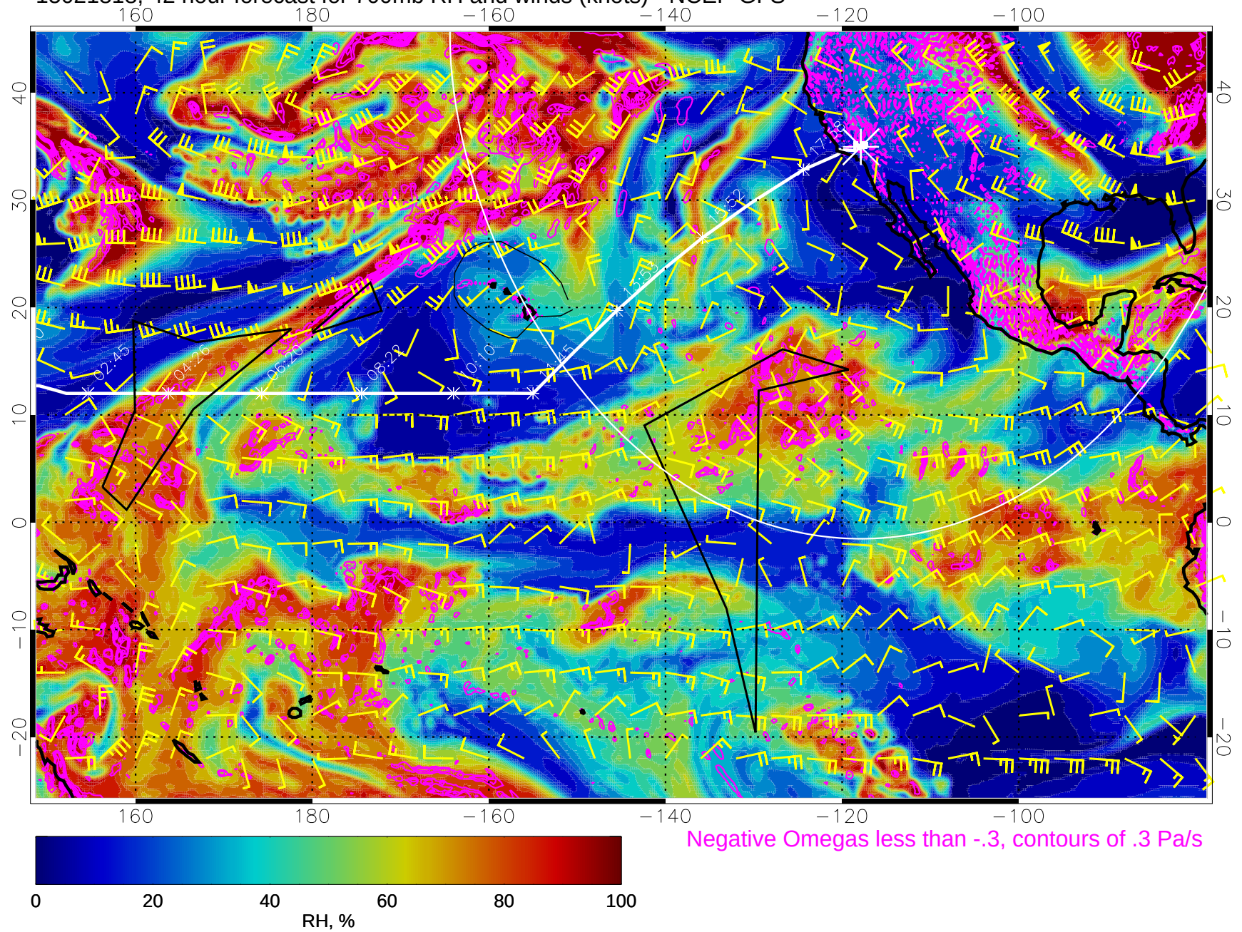
15021818, 42 hour forecast for 700mb RH and winds (knots) - NCEP GFS
