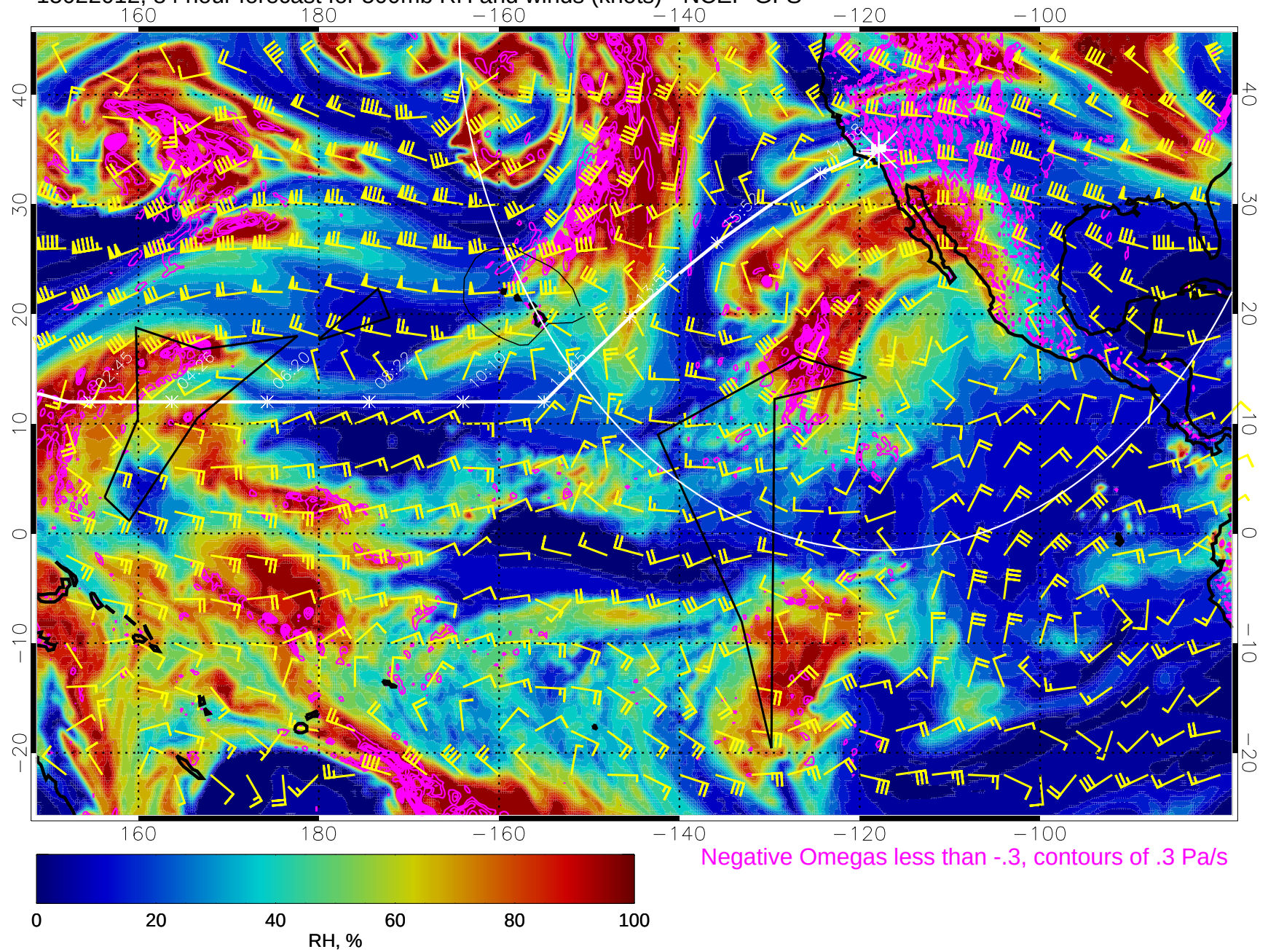
15022012, 84 hour forecast for 500mb RH and winds (knots) - NCEP GFS
