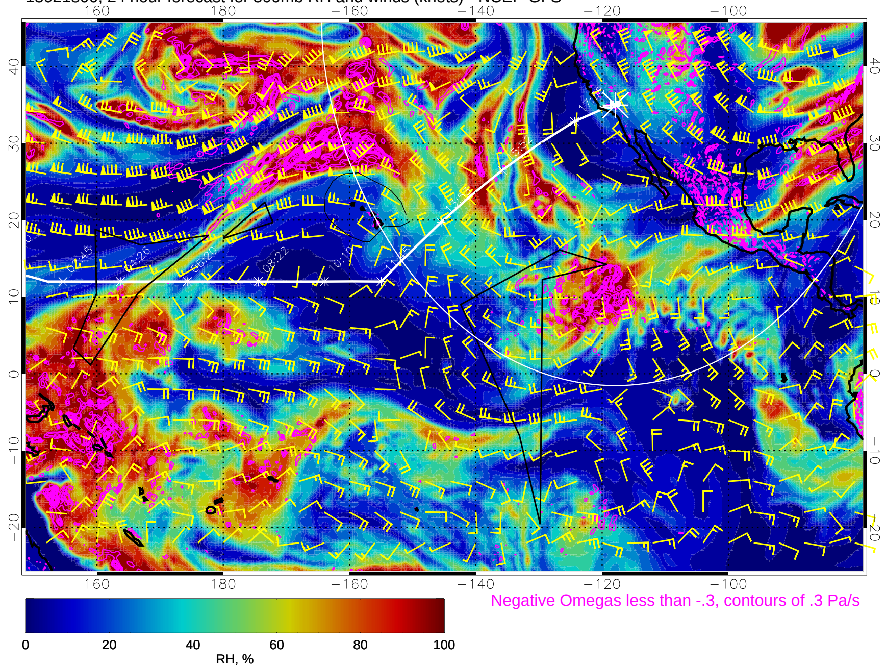
15021800, 24 hour forecast for 500mb RH and winds (knots) - NCEP GFS
