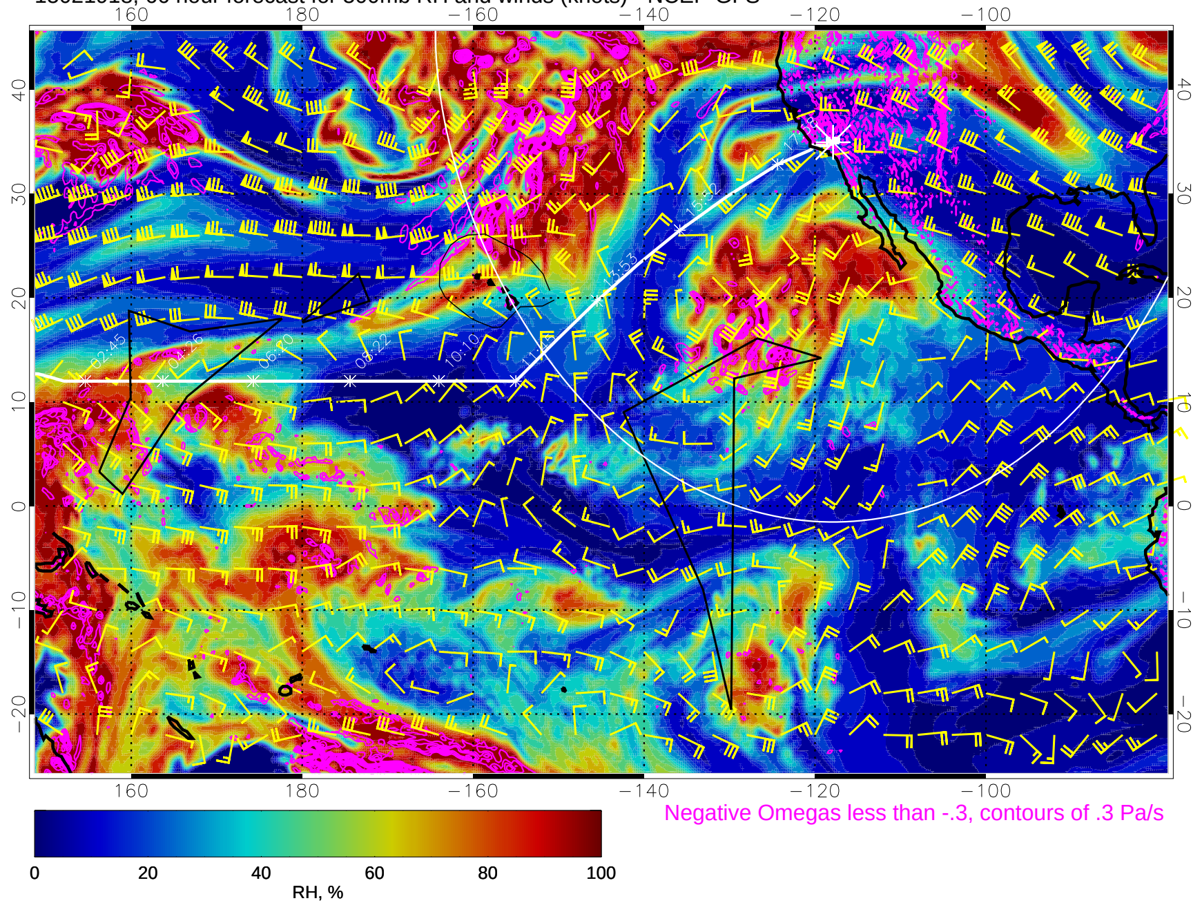
15021918, 66 hour forecast for 500mb RH and winds (knots) - NCEP GFS
