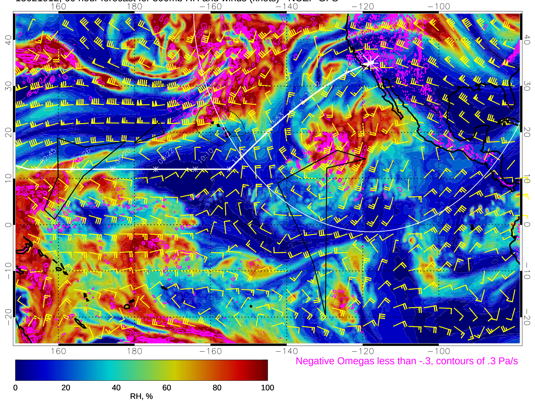
15021912, 60 hour forecast for 500mb RH and winds (knots) - NCEP GFS
