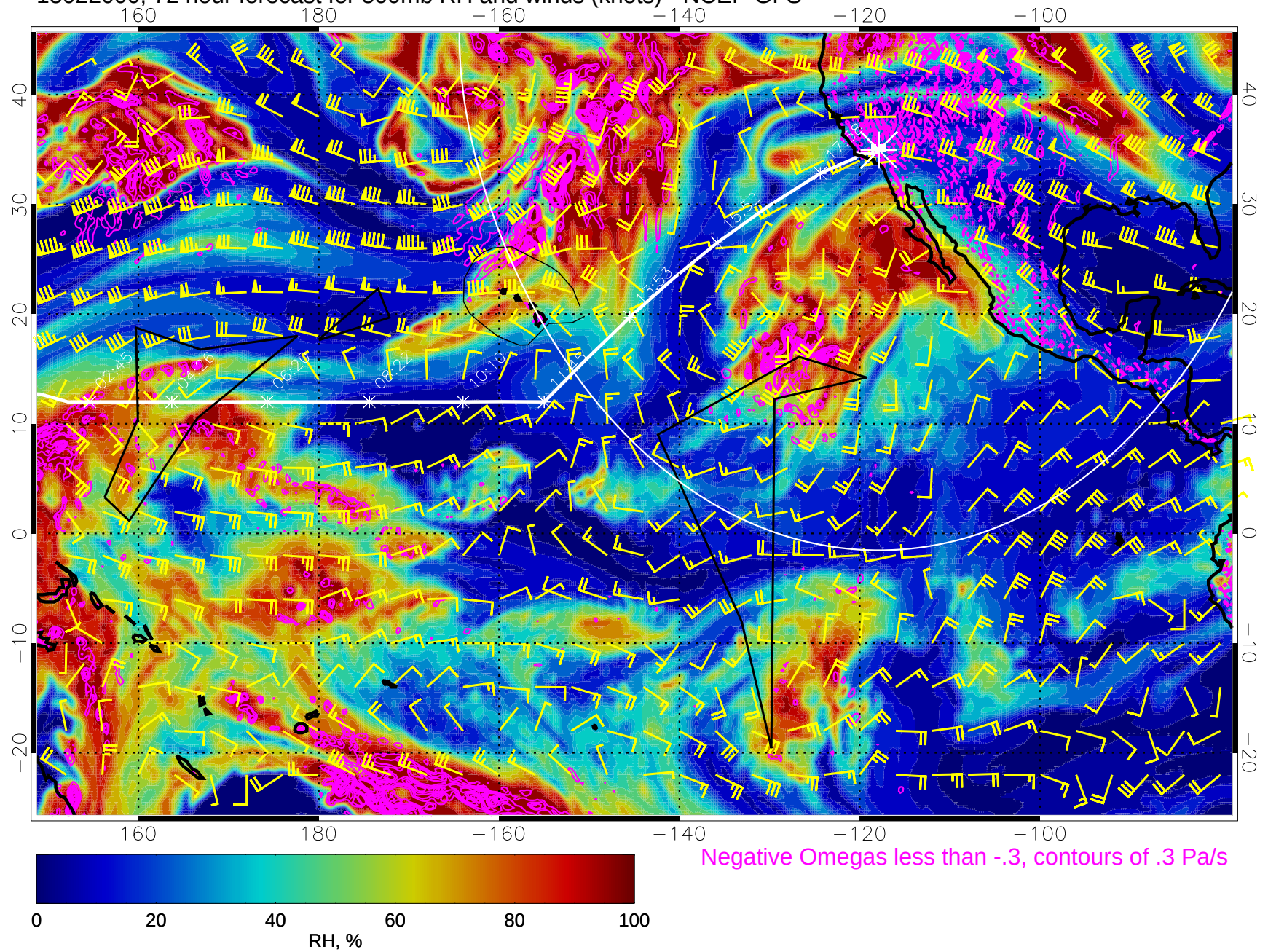
15022000, 72 hour forecast for 500mb RH and winds (knots) - NCEP GFS
