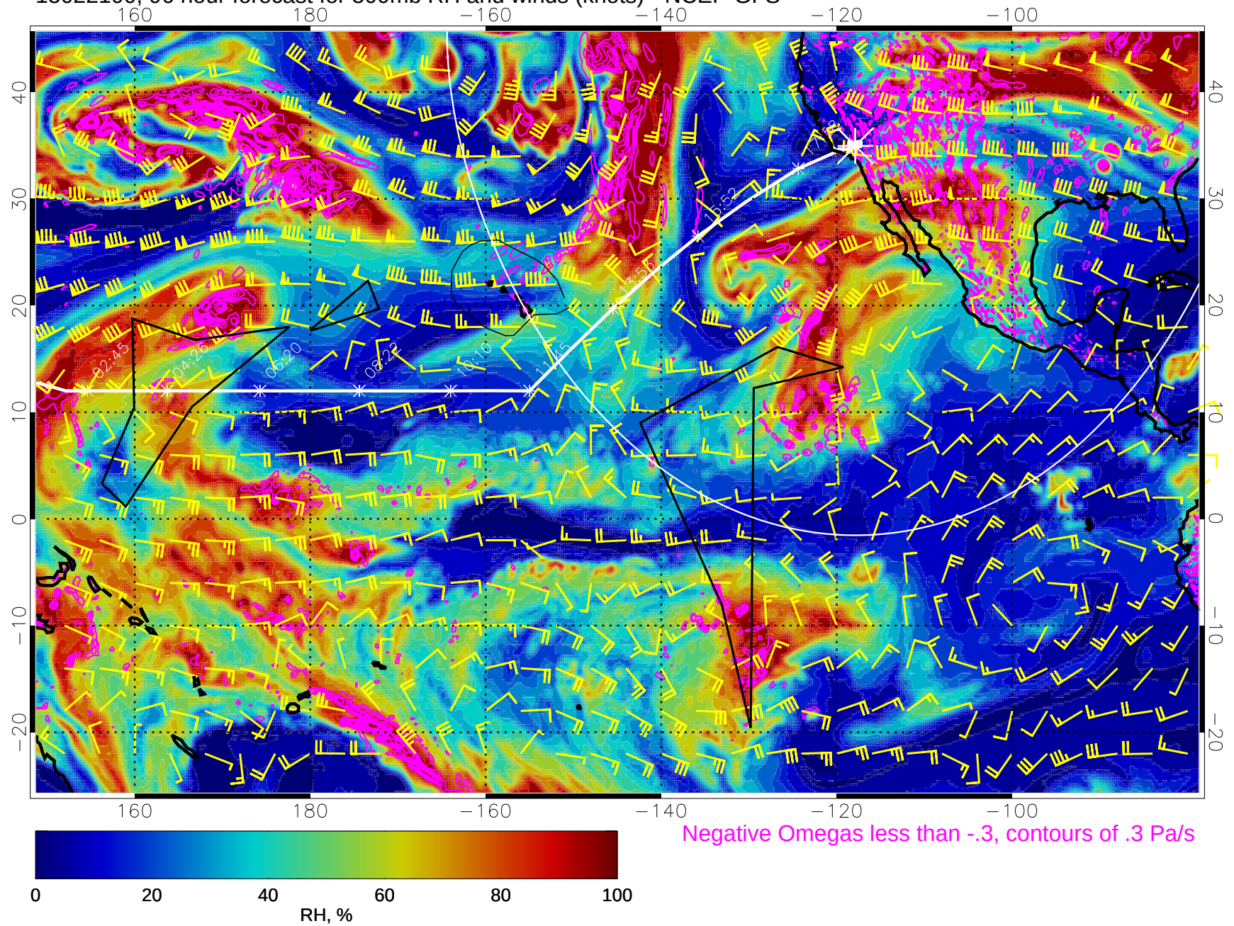
15022100, 96 hour forecast for 500mb RH and winds (knots) - NCEP GFS
