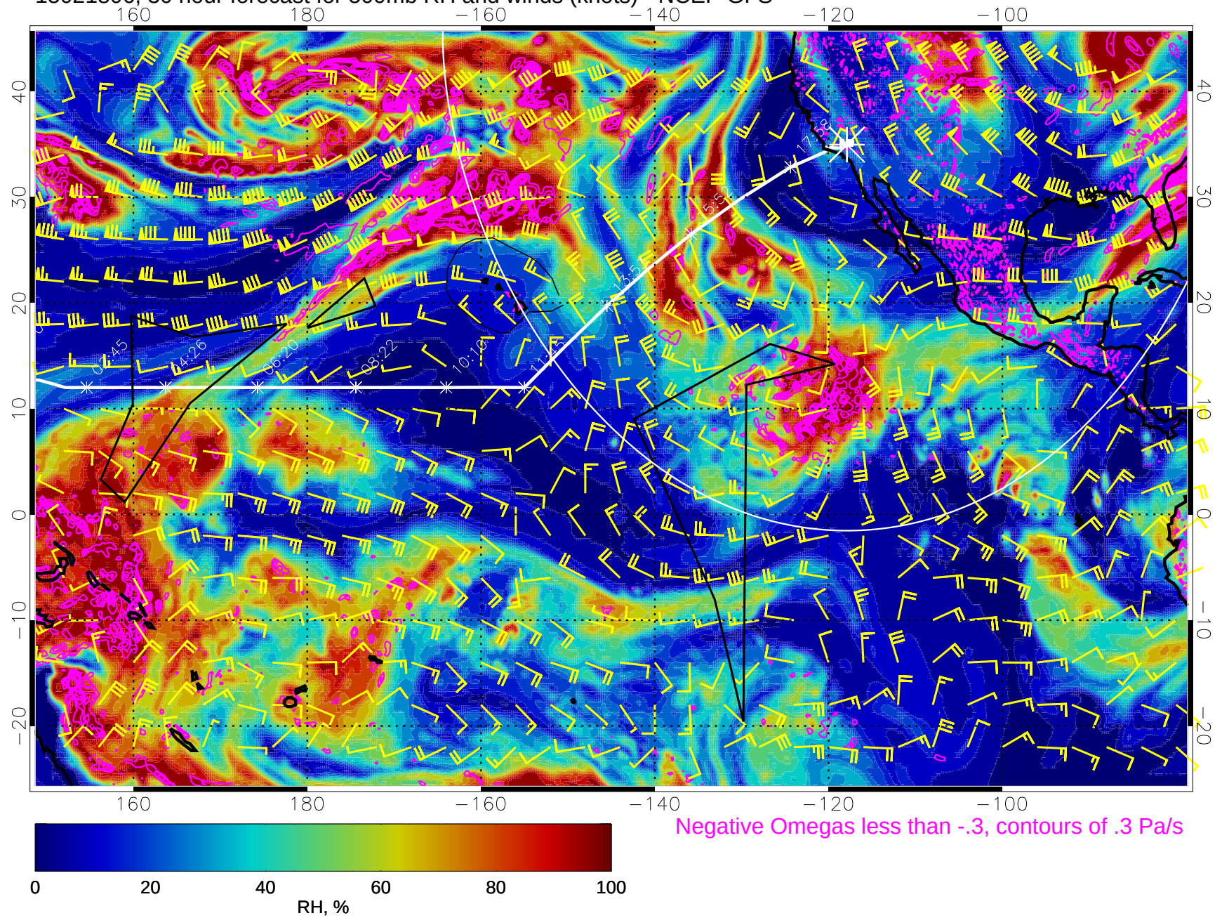
15021806, 30 hour forecast for 500mb RH and winds (knots) - NCEP GFS
