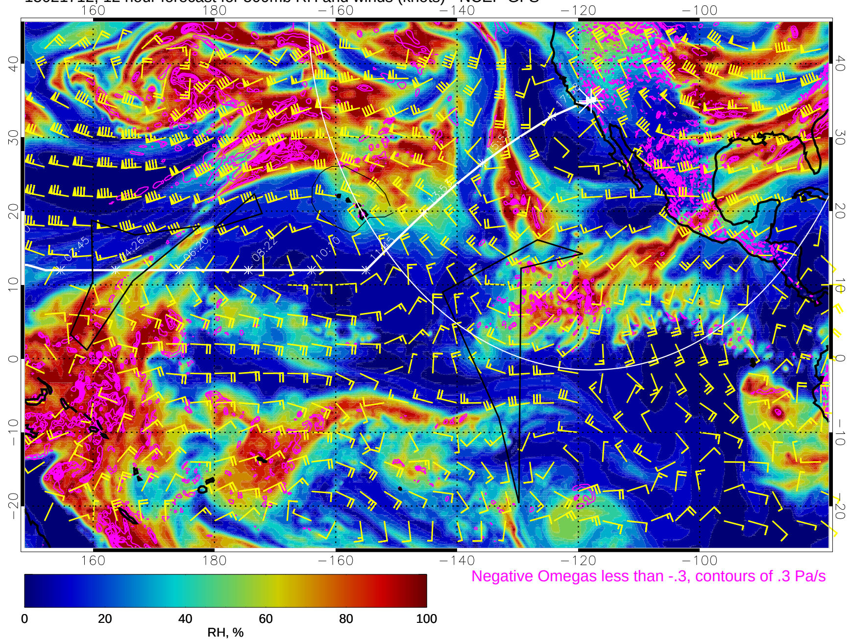
15021712, 12 hour forecast for 500mb RH and winds (knots) - NCEP GFS
