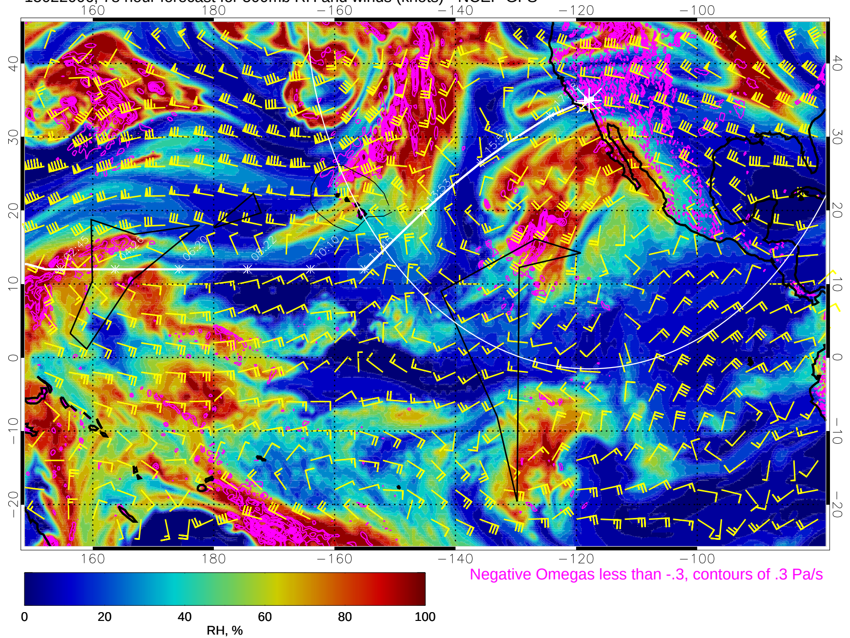
15022006, 78 hour forecast for 500mb RH and winds (knots) - NCEP GFS
