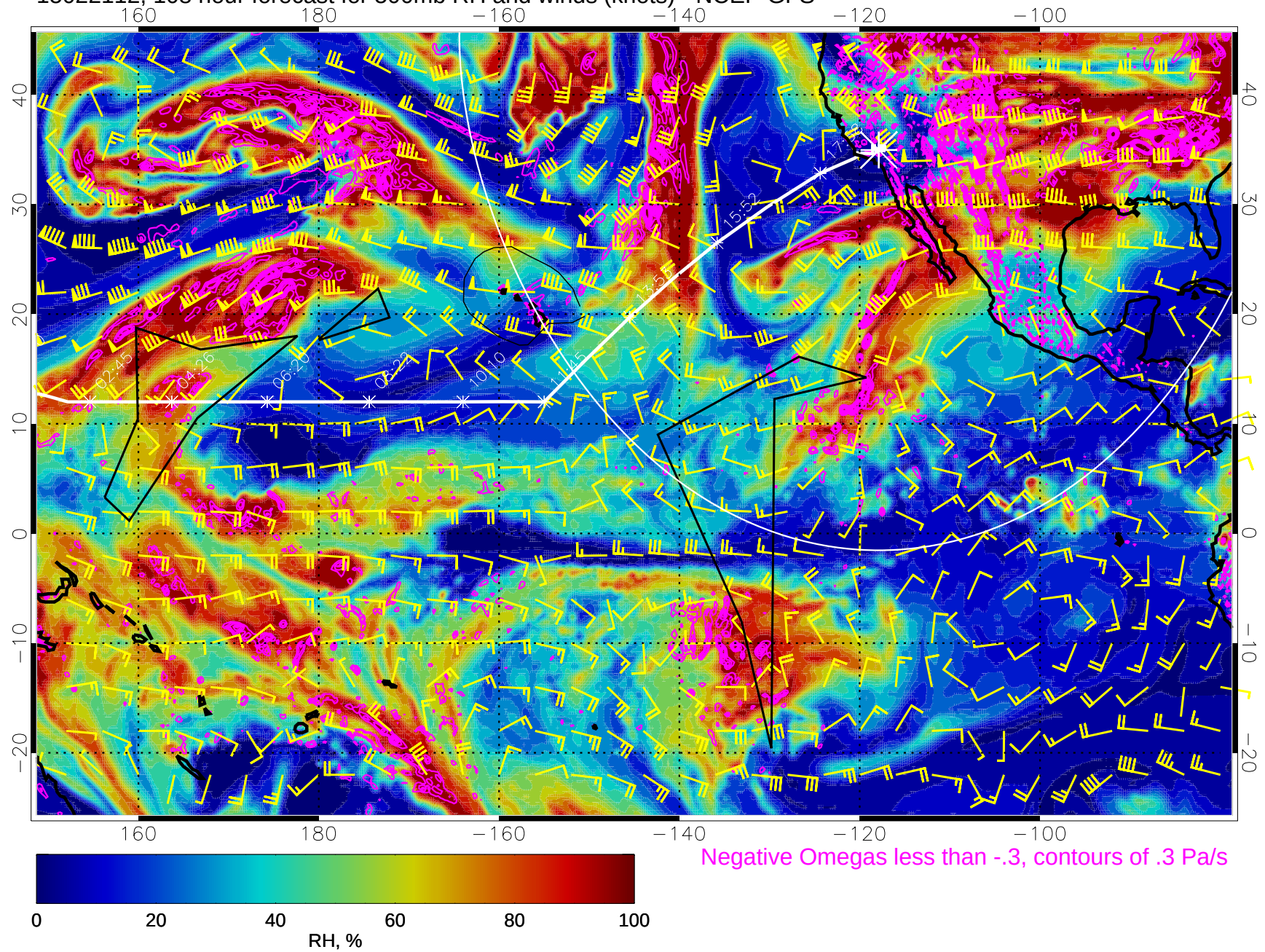
15022112, 108 hour forecast for 500mb RH and winds (knots) - NCEP GFS
