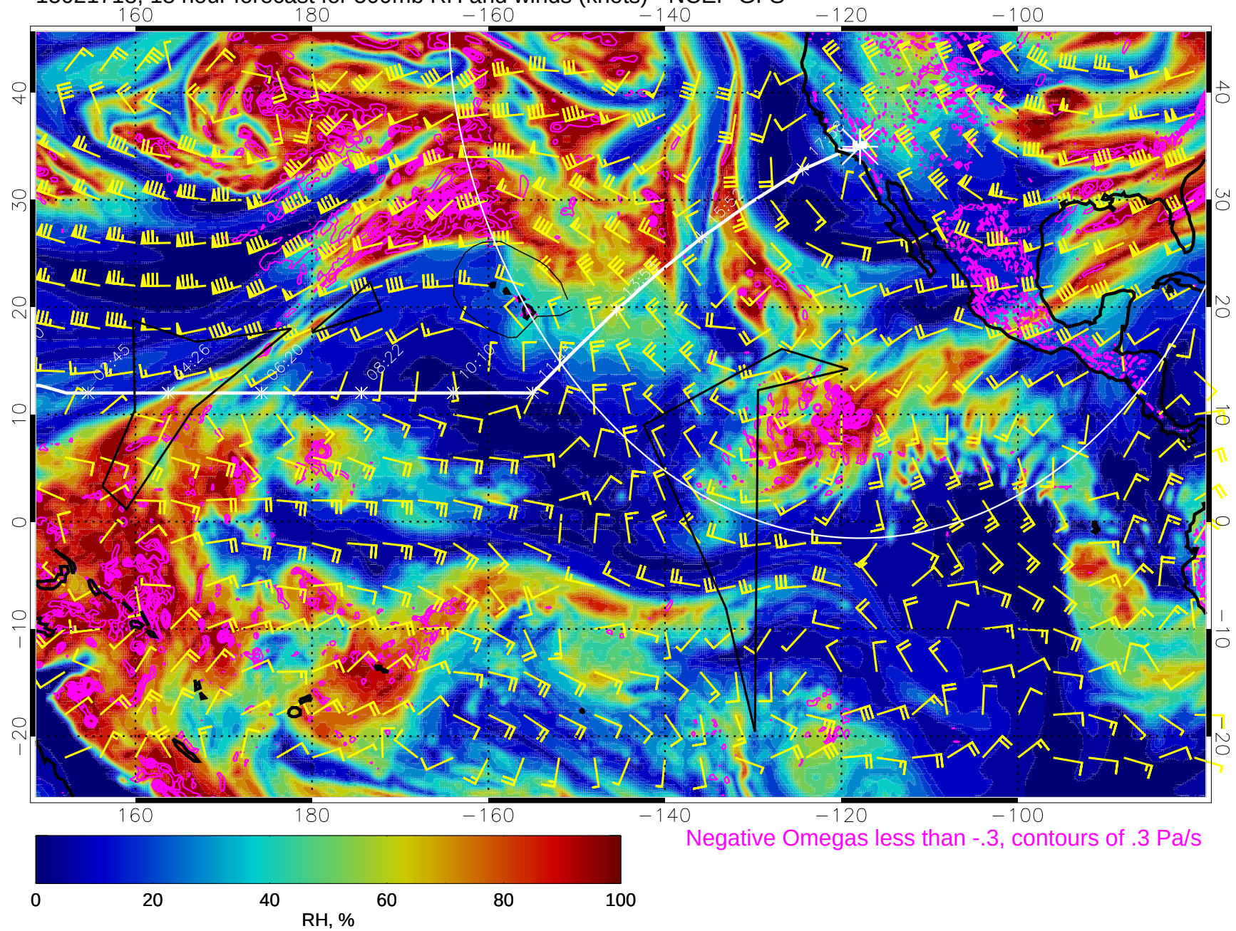
15021718, 18 hour forecast for 500mb RH and winds (knots) - NCEP GFS
