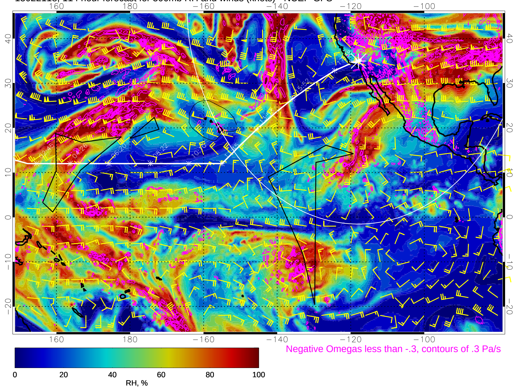
15022118, 114 hour forecast for 500mb RH and winds (knots) - NCEP GFS
