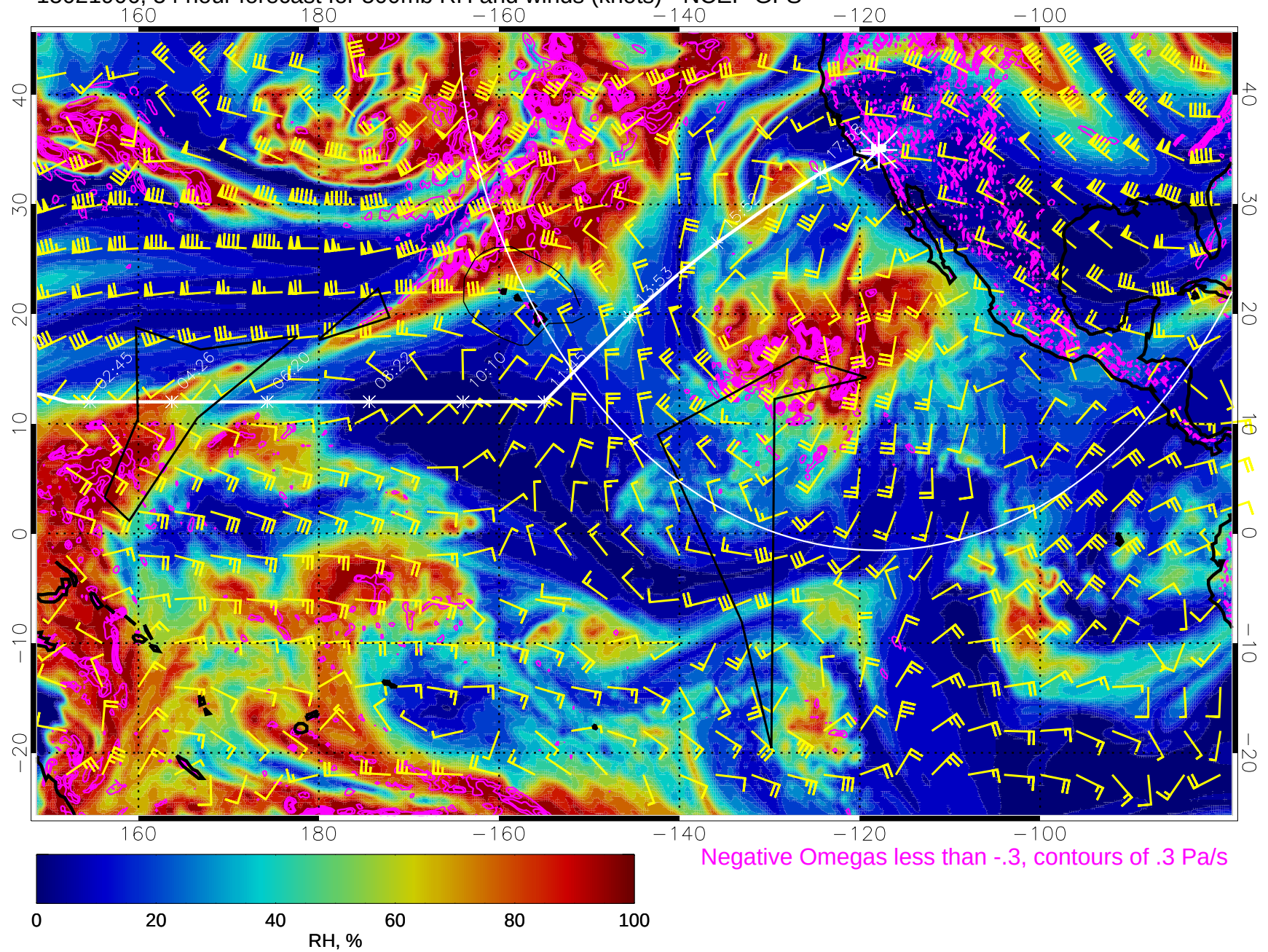
15021906, 54 hour forecast for 500mb RH and winds (knots) - NCEP GFS
