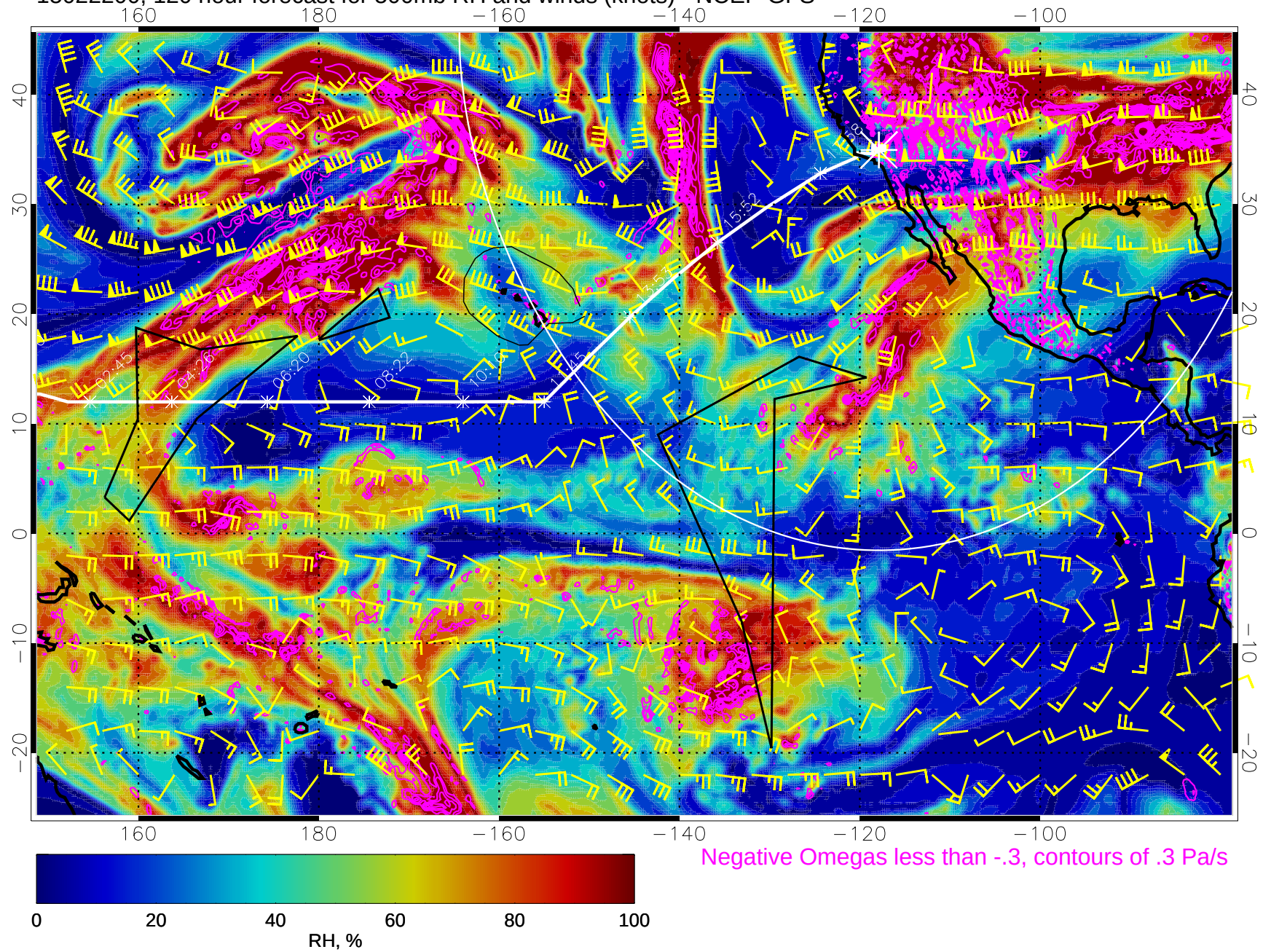
15022200, 120 hour forecast for 500mb RH and winds (knots) - NCEP GFS
