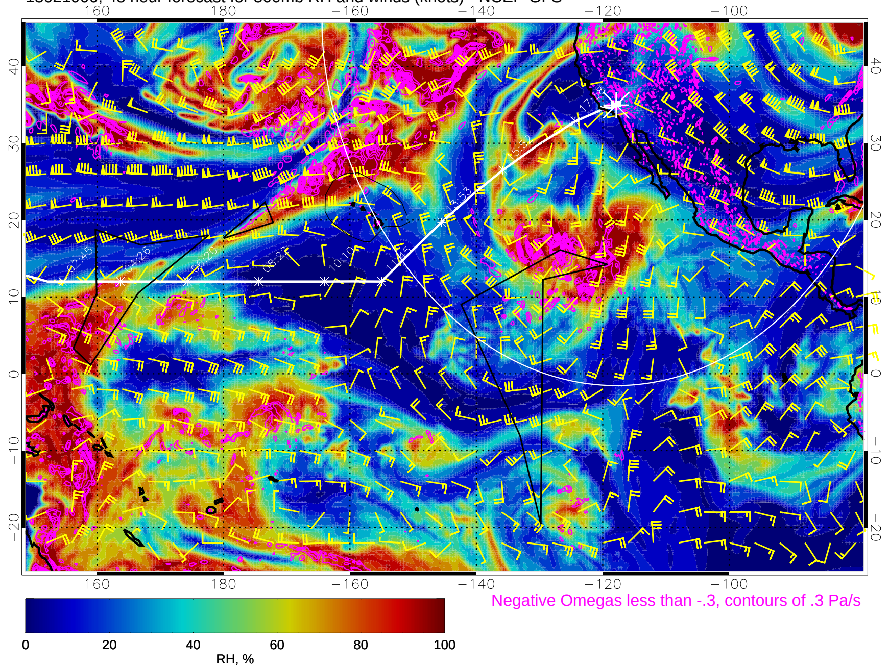
15021900, 48 hour forecast for 500mb RH and winds (knots) - NCEP GFS
