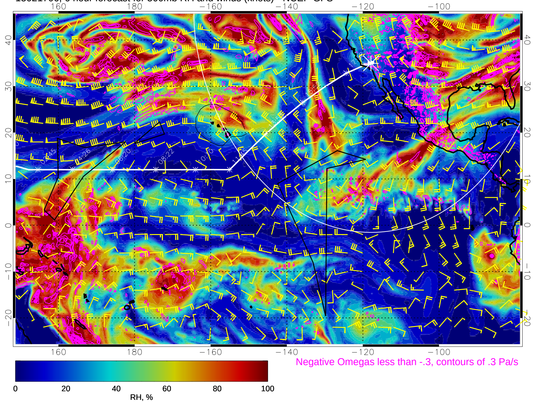
15021706, 6 hour forecast for 500mb RH and winds (knots) - NCEP GFS
