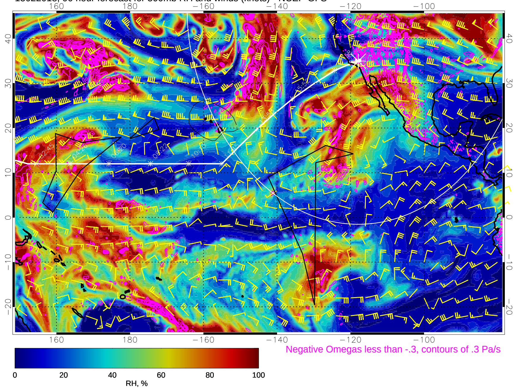
15022018, 90 hour forecast for 500mb RH and winds (knots) - NCEP GFS
