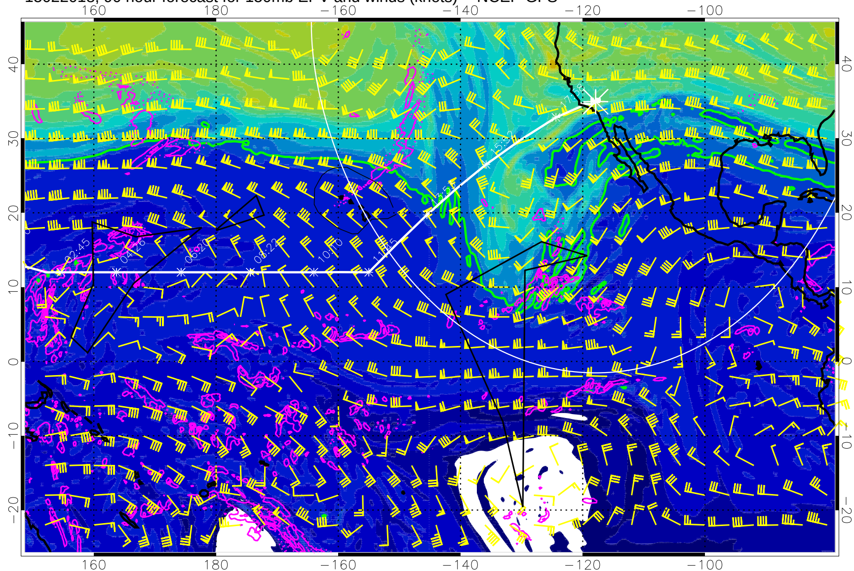
15022018, 90 hour forecast for 150mb EPV and winds (knots) -- NCEP GFS
