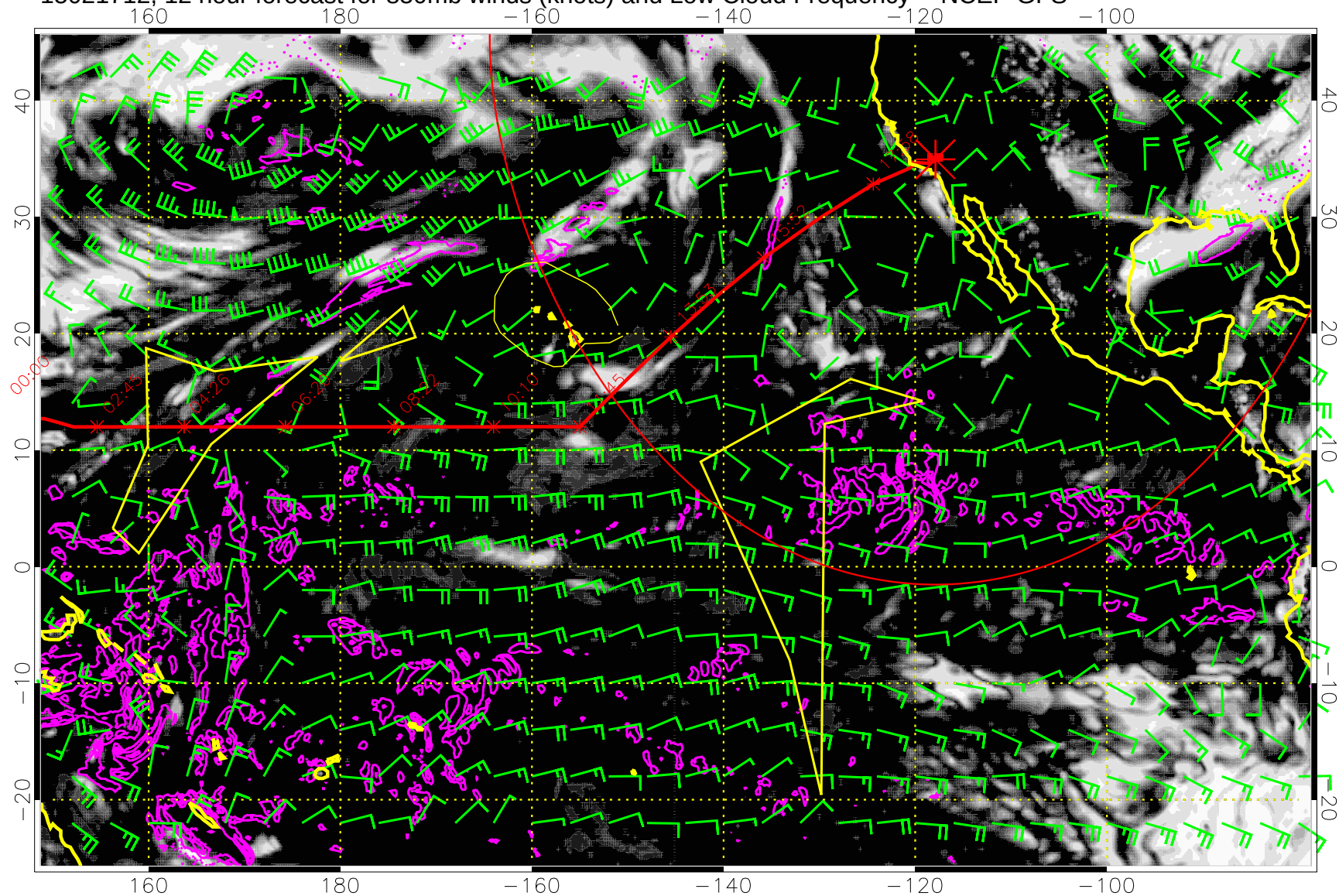
15021712, 12 hour forecast for 850mb winds (knots) and Low Cloud Frequency -- NCEP GFS
