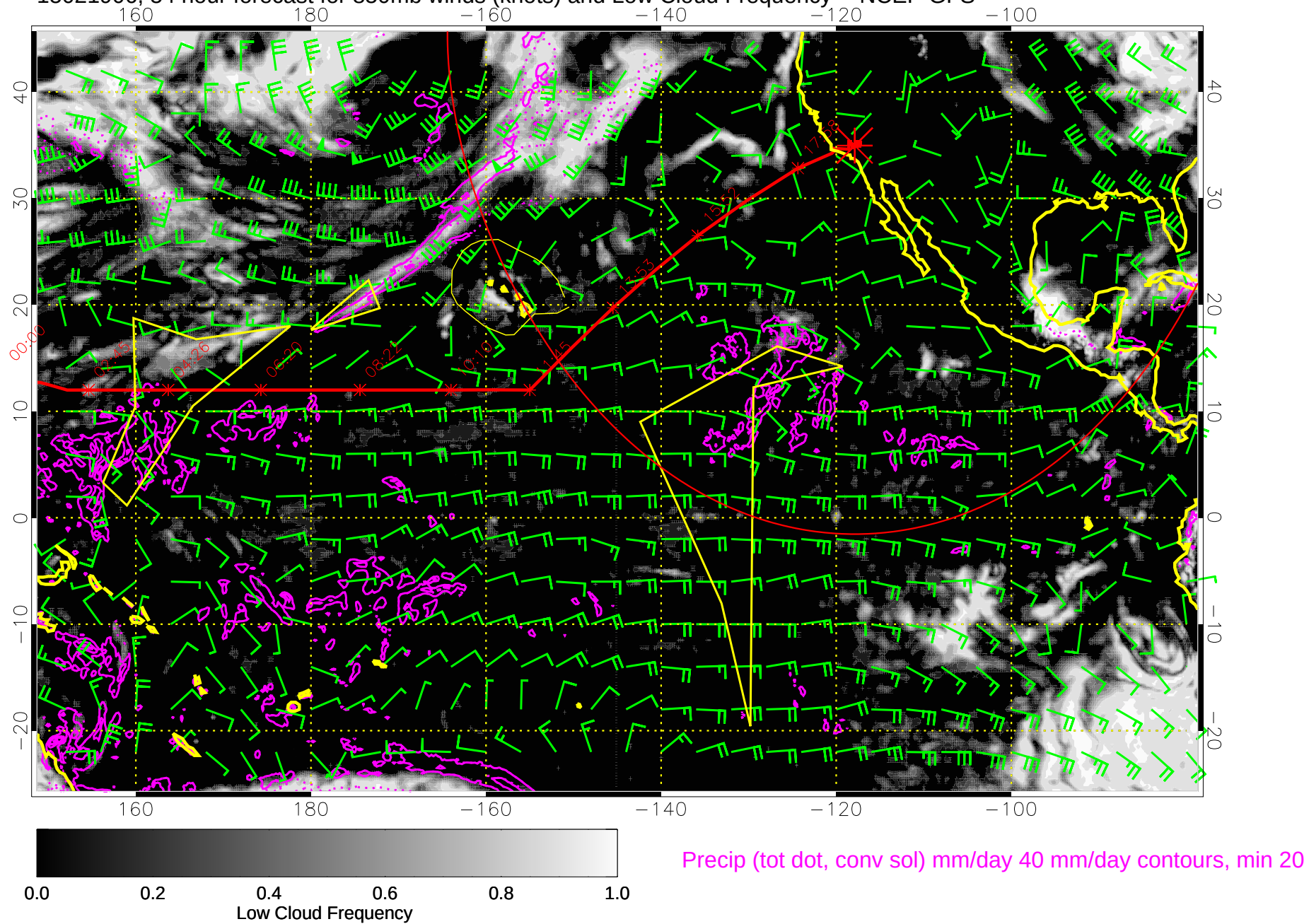
15021906, 54 hour forecast for 850mb winds (knots) and Low Cloud Frequency -- NCEP GFS
