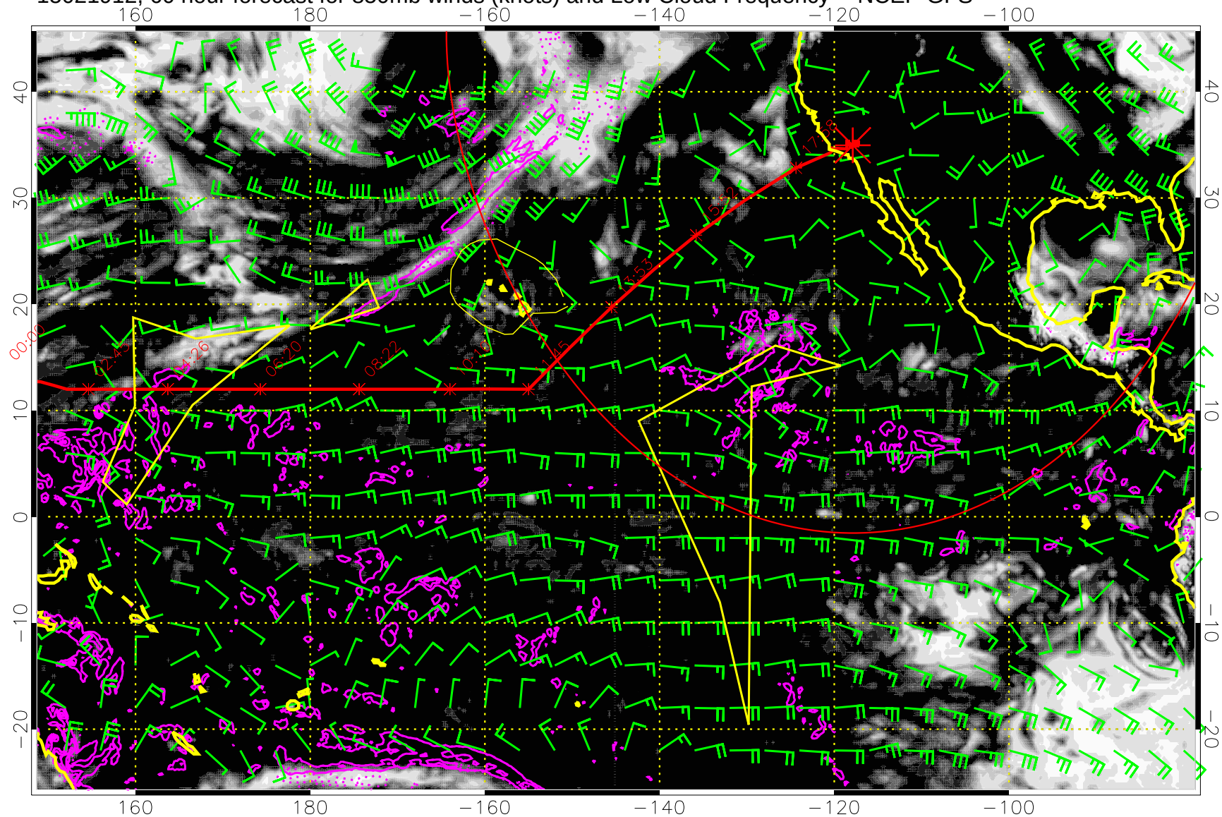
15021912, 60 hour forecast for 850mb winds (knots) and Low Cloud Frequency -- NCEP GFS
