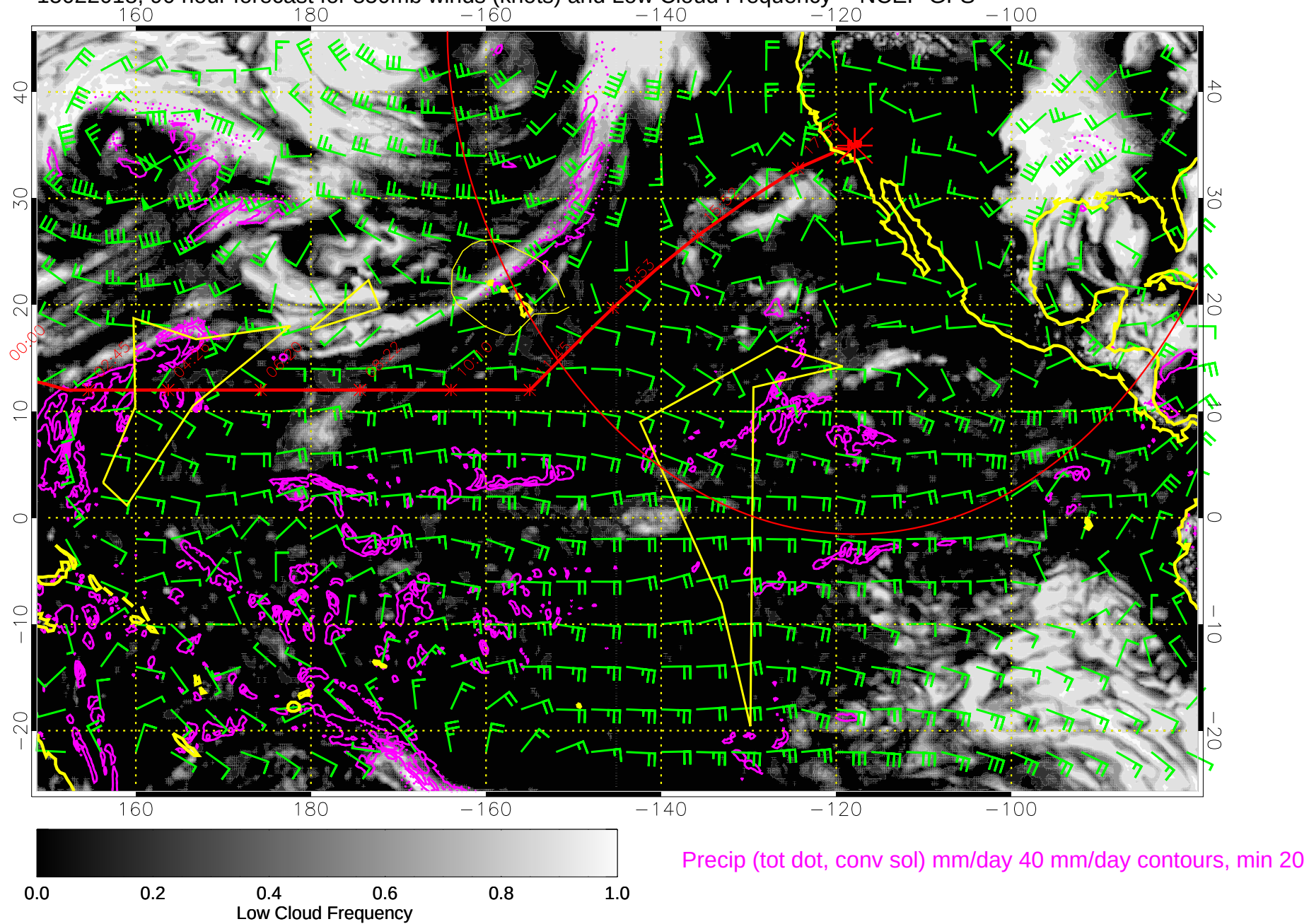
15022018, 90 hour forecast for 850mb winds (knots) and Low Cloud Frequency -- NCEP GFS
