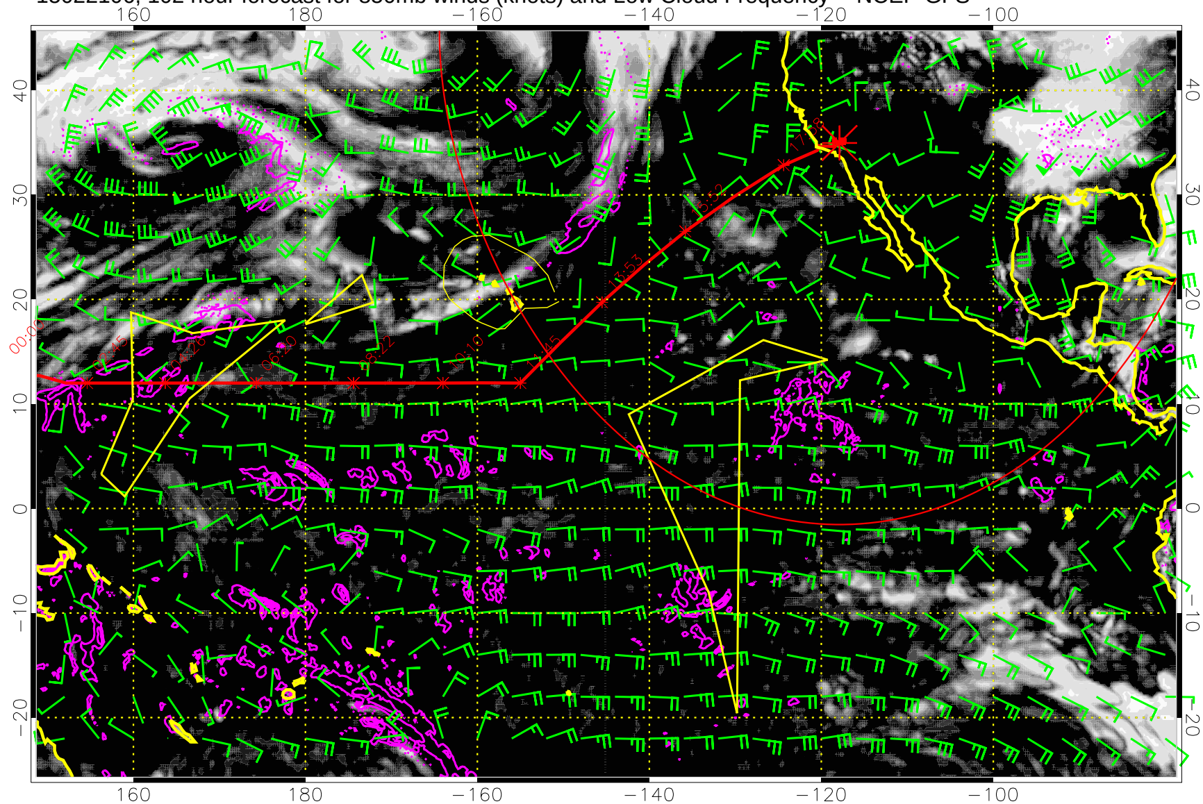
15022106, 102 hour forecast for 850mb winds (knots) and Low Cloud Frequency -- NCEP GFS
