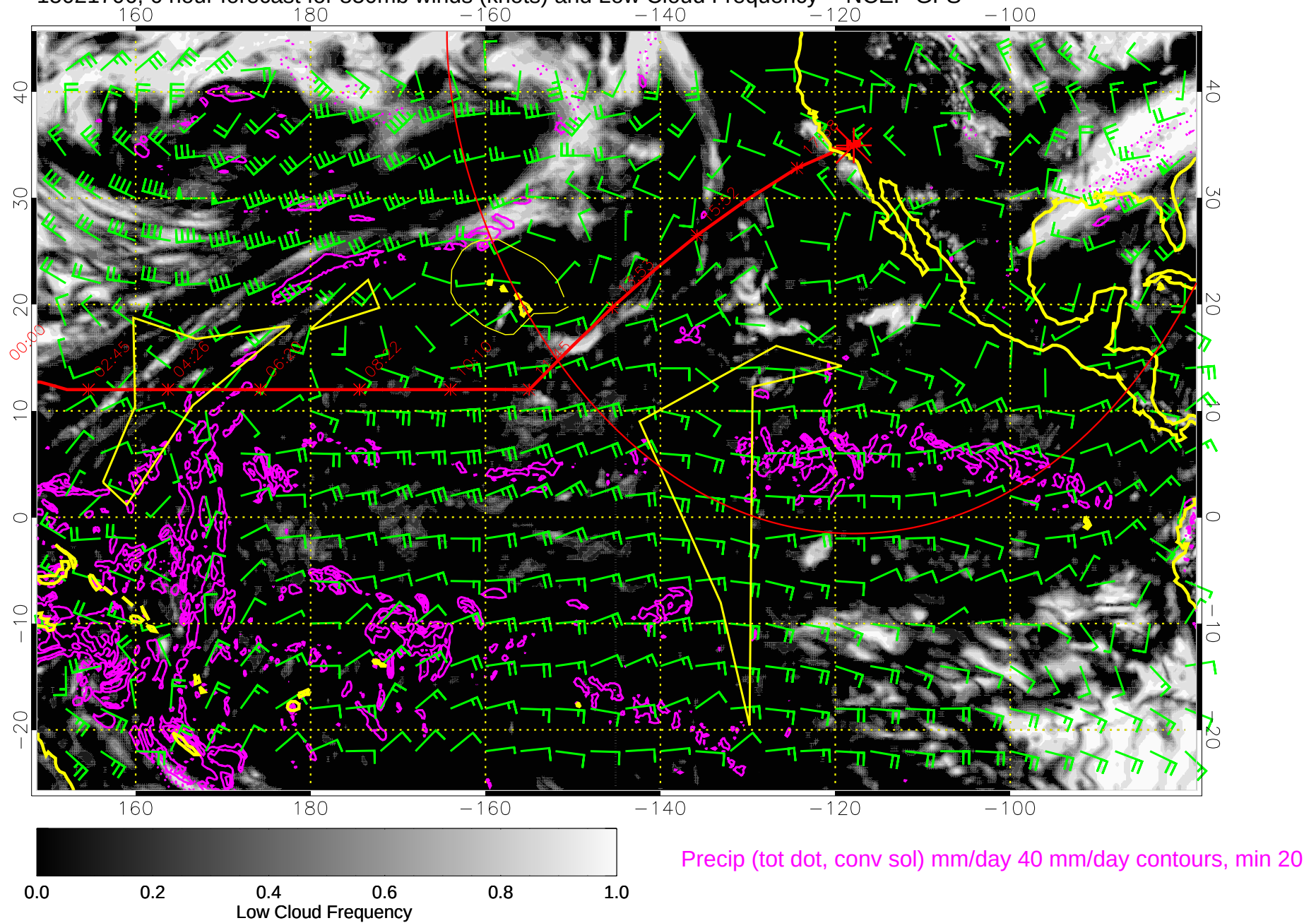
15021706, 6 hour forecast for 850mb winds (knots) and Low Cloud Frequency -- NCEP GFS
