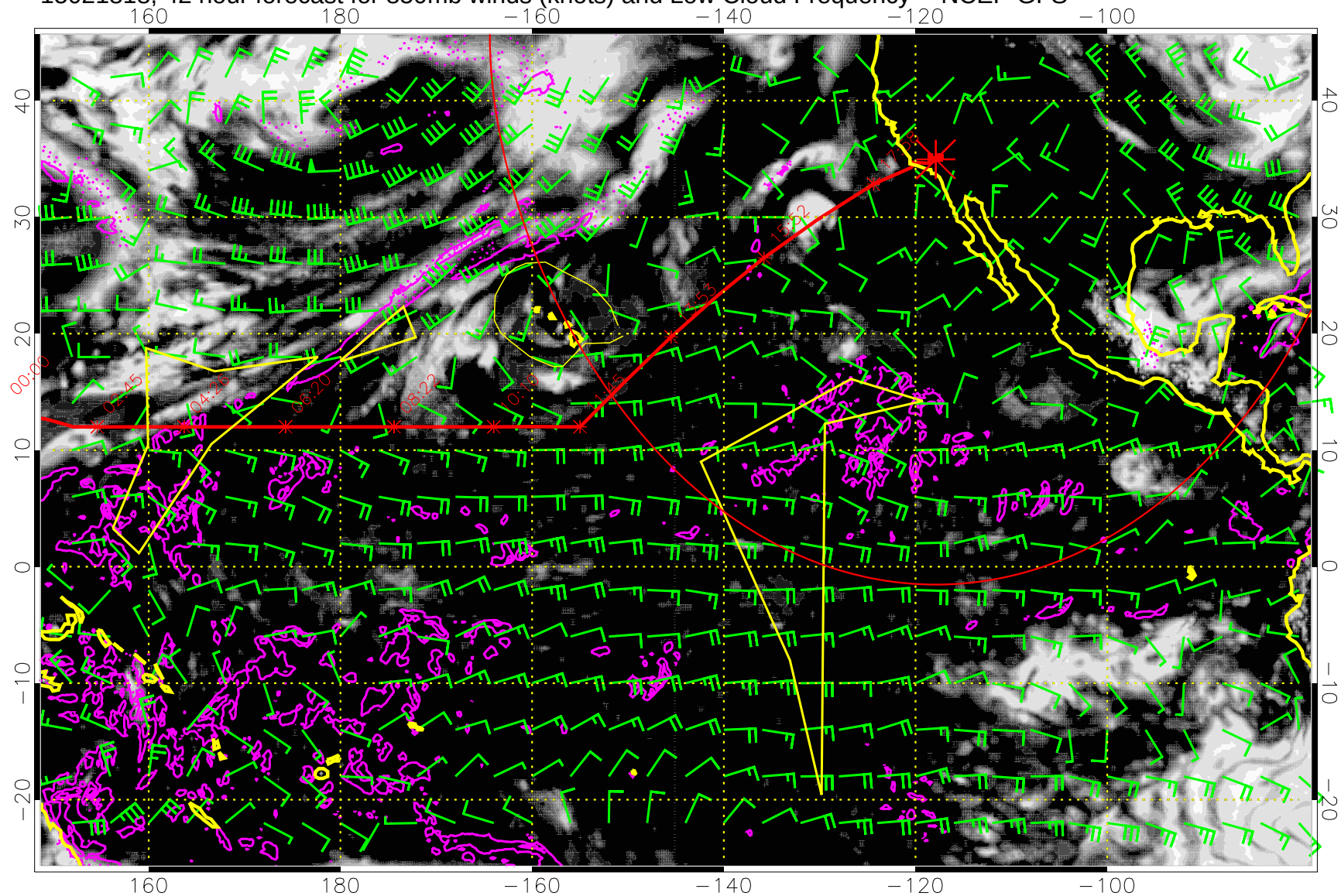
15021818, 42 hour forecast for 850mb winds (knots) and Low Cloud Frequency -- NCEP GFS
