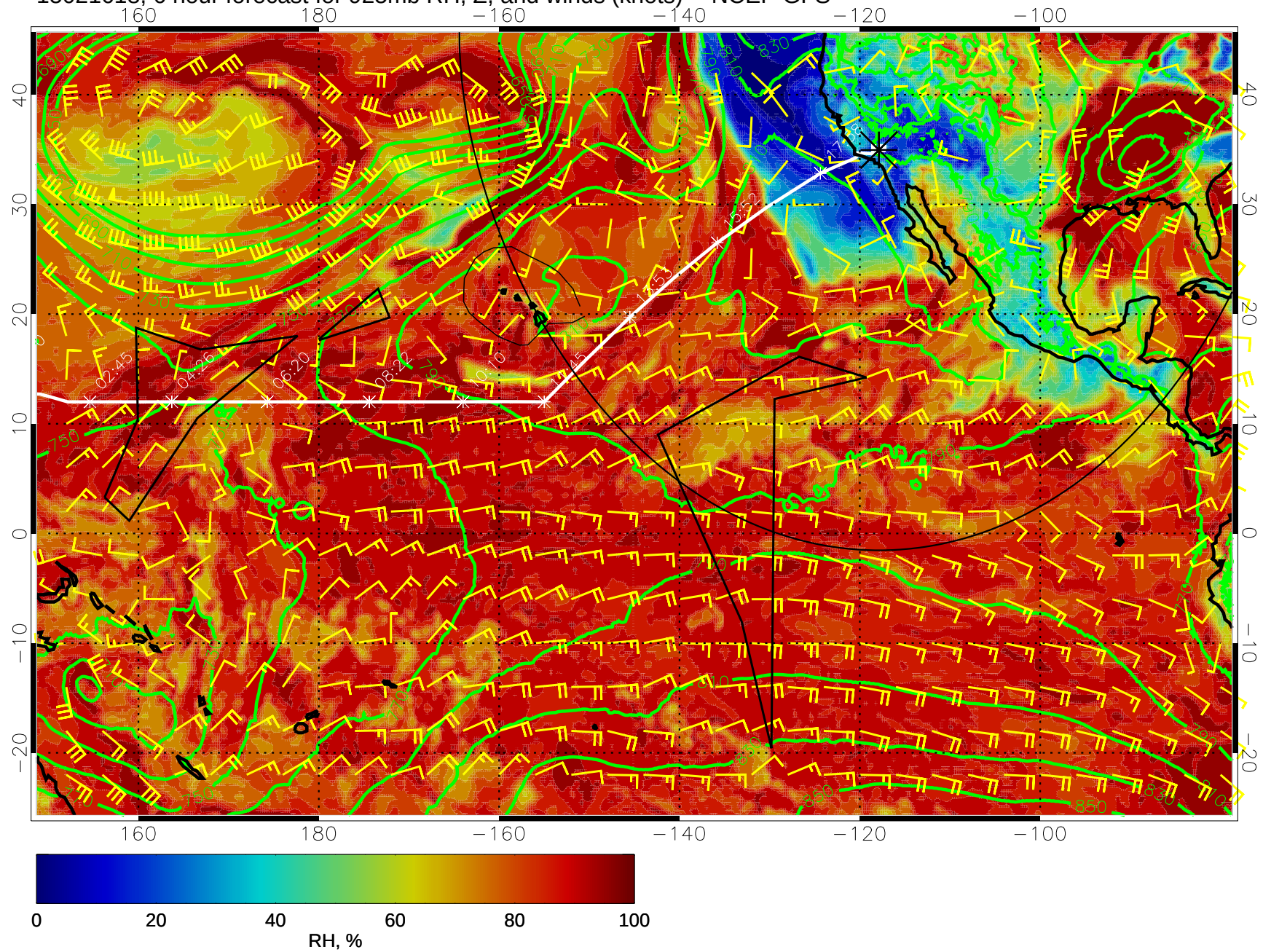
15021618, 6 hour forecast for 925mb RH, Z, and winds (knots) -- NCEP GFS
