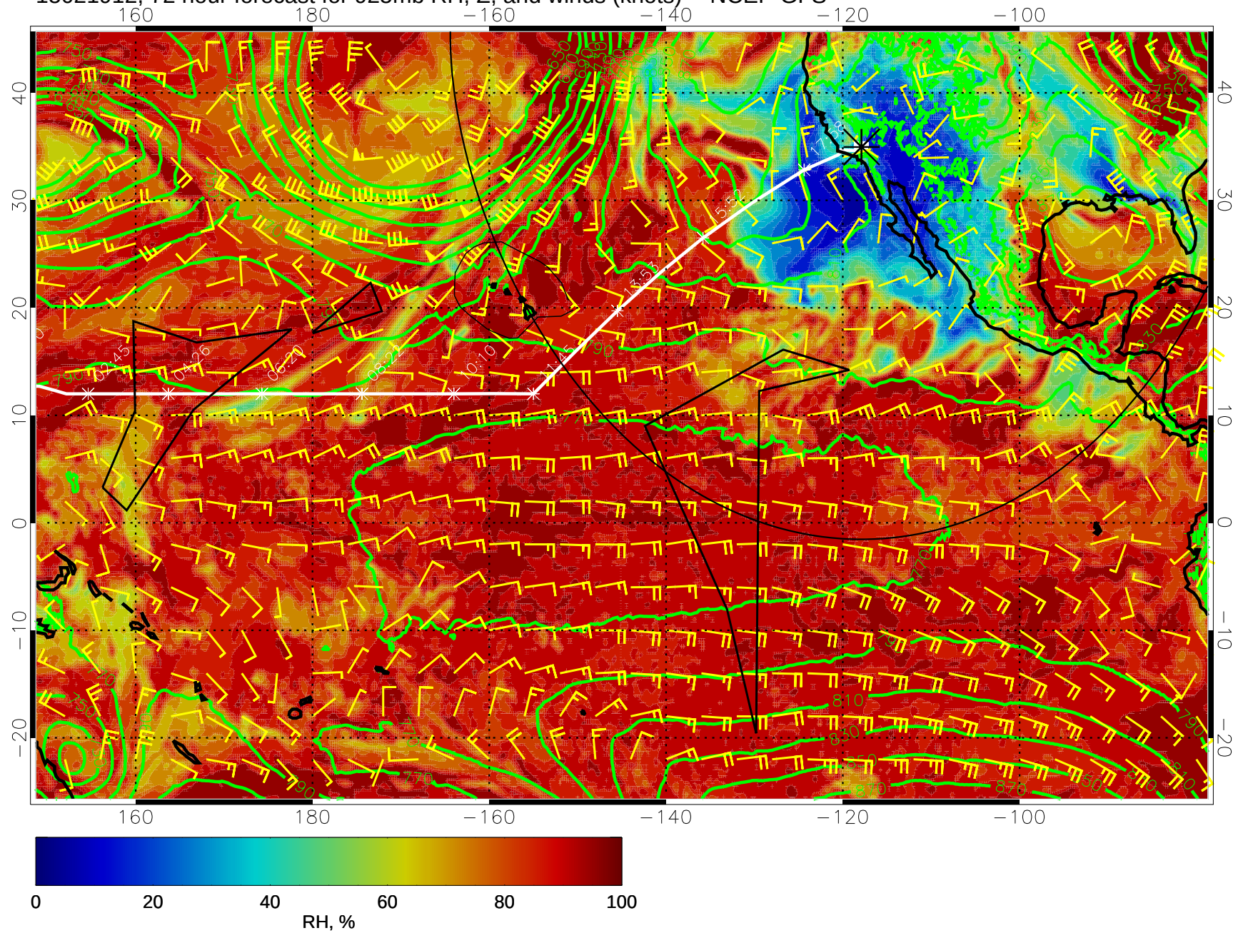
15021912, 72 hour forecast for 925mb RH, Z, and winds (knots) -- NCEP GFS
