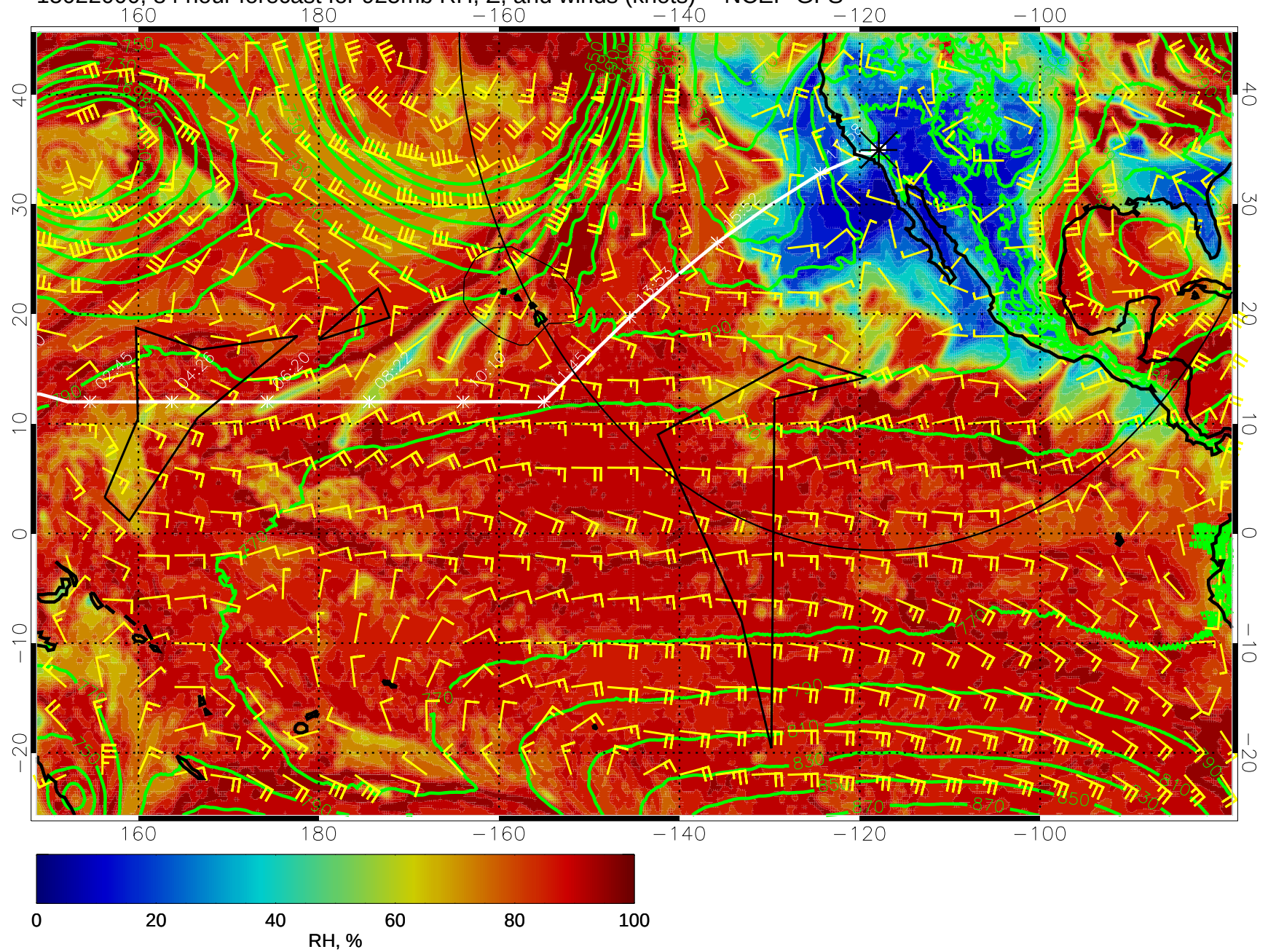
15022000, 84 hour forecast for 925mb RH, Z, and winds (knots) -- NCEP GFS
