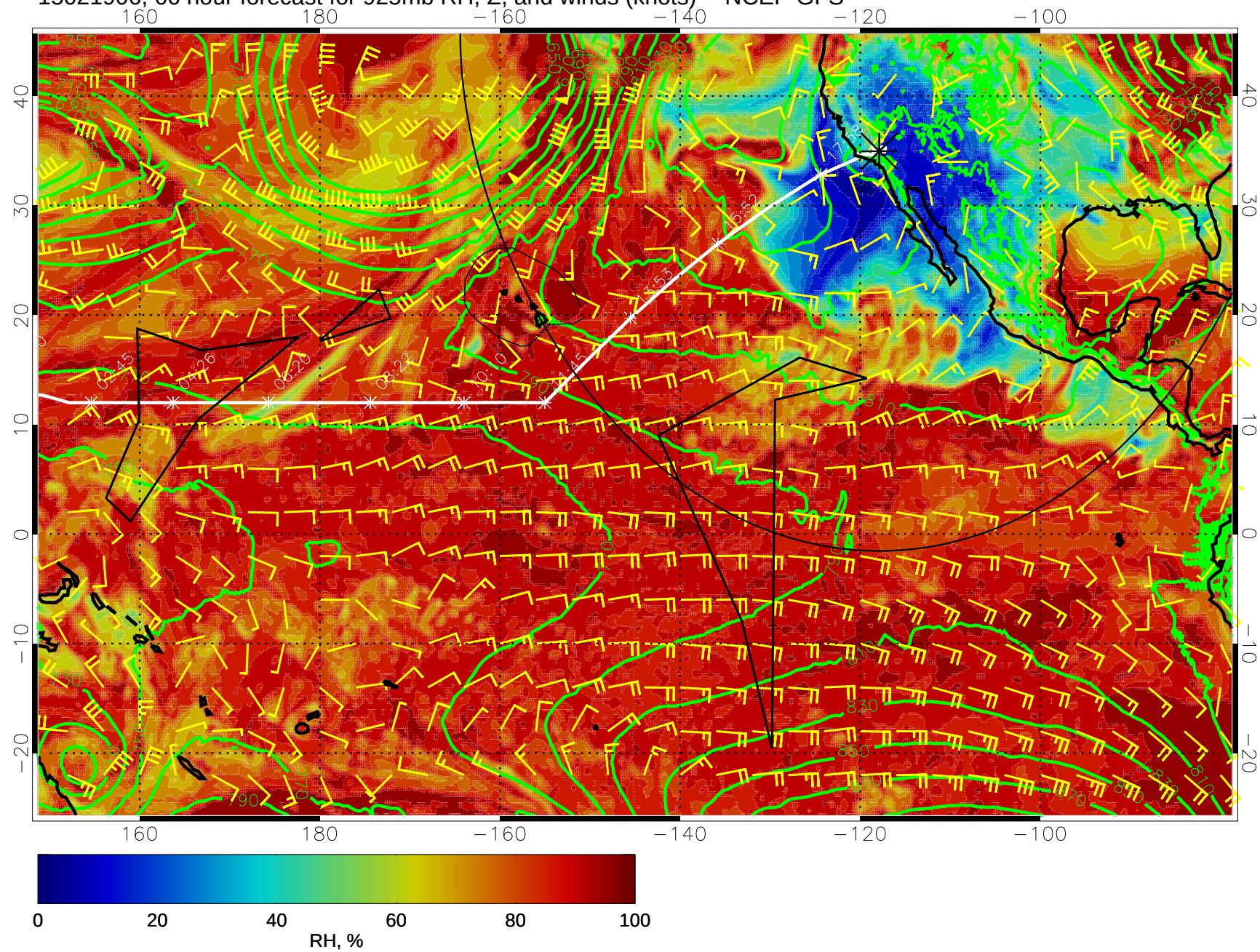
15021906, 66 hour forecast for 925mb RH, Z, and winds (knots) -- NCEP GFS
