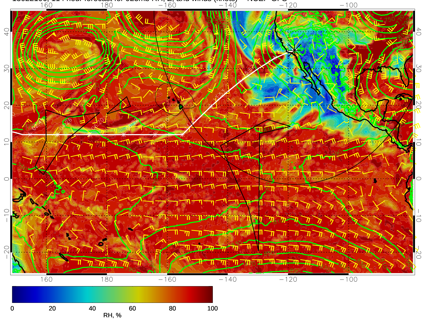
15022106, 114 hour forecast for 925mb RH, Z, and winds (knots) -- NCEP GFS
