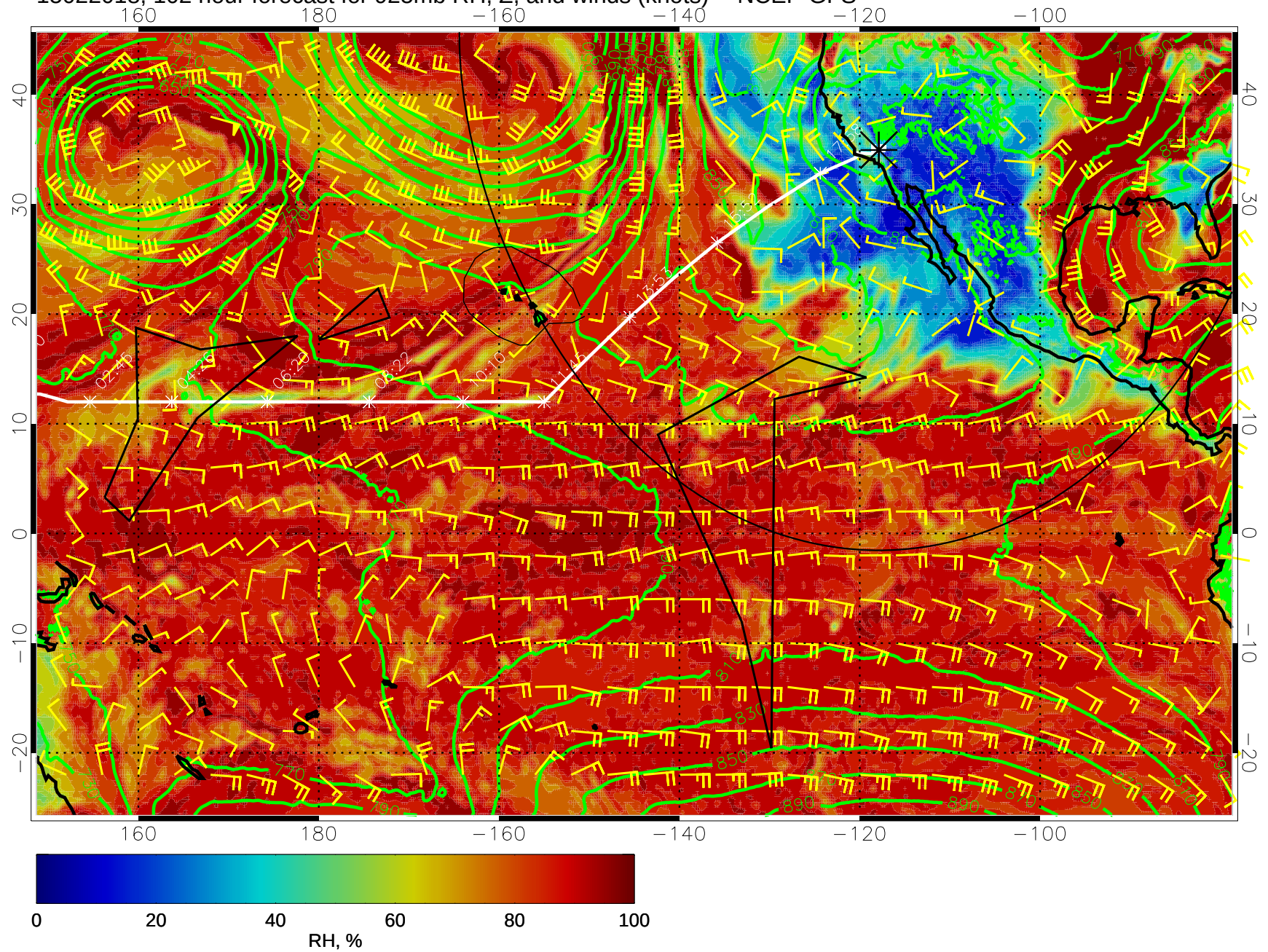
15022018, 102 hour forecast for 925mb RH, Z, and winds (knots) -- NCEP GFS
