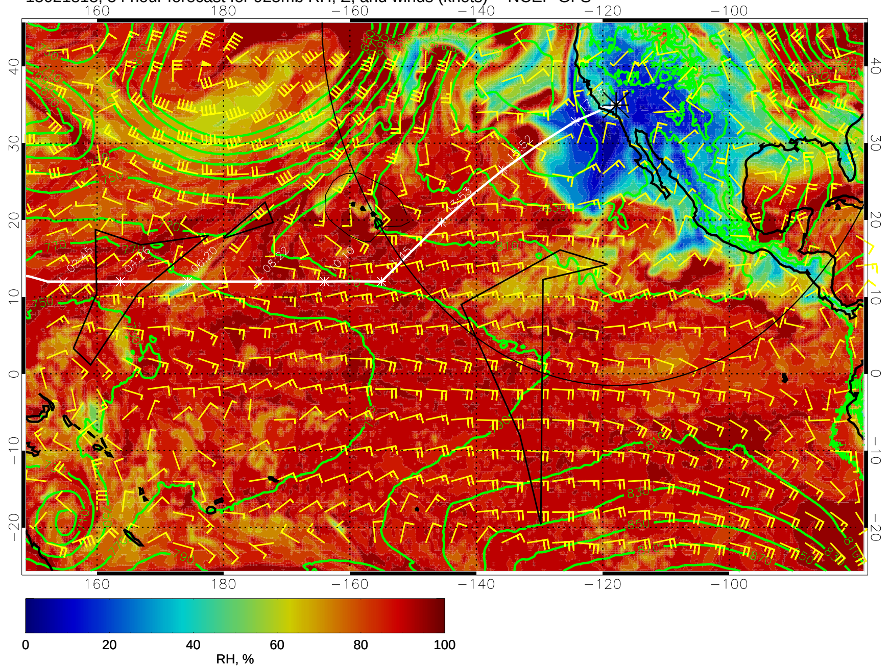
15021818, 54 hour forecast for 925mb RH, Z, and winds (knots) -- NCEP GFS
