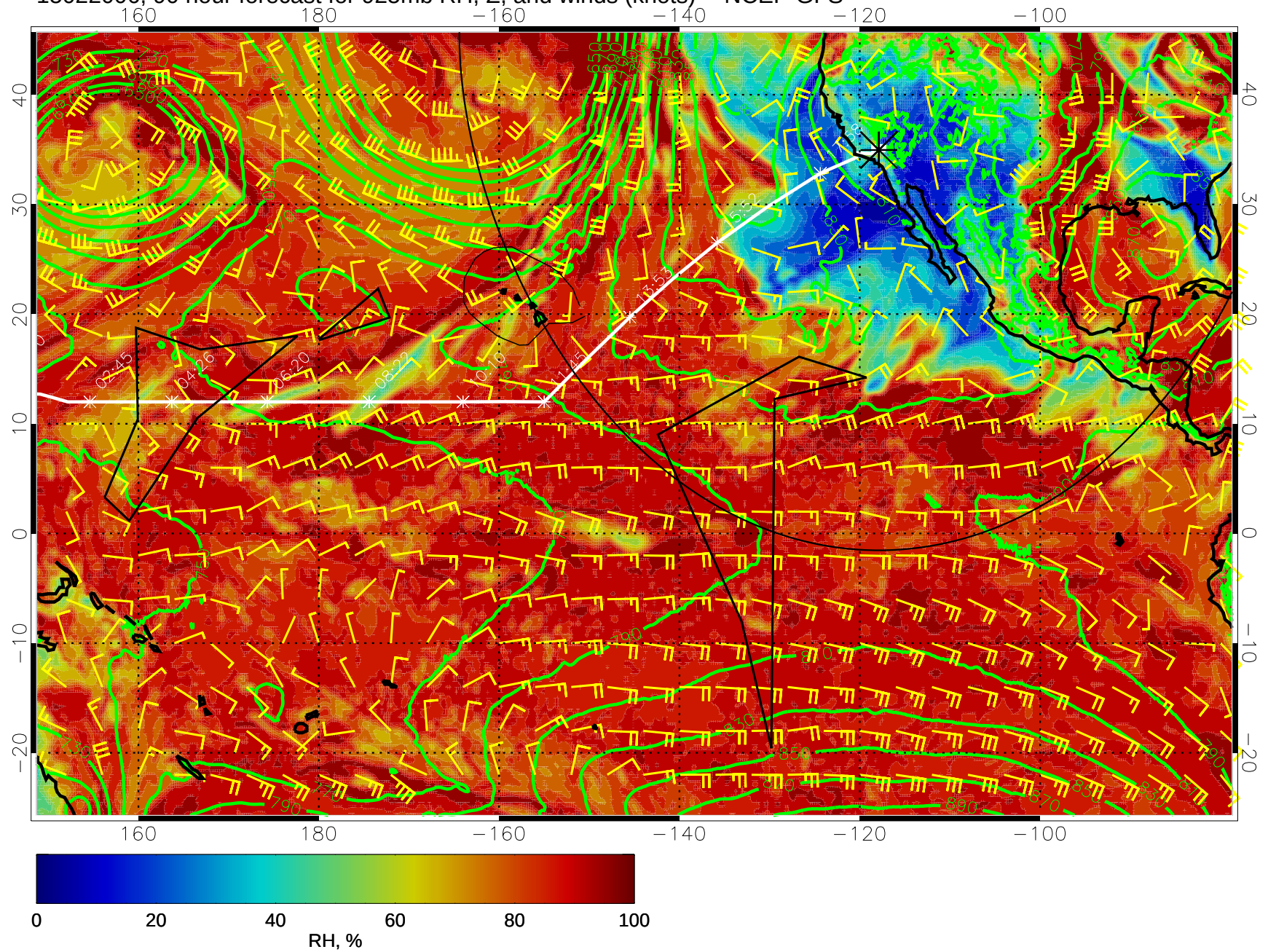
15022006, 90 hour forecast for 925mb RH, Z, and winds (knots) -- NCEP GFS
