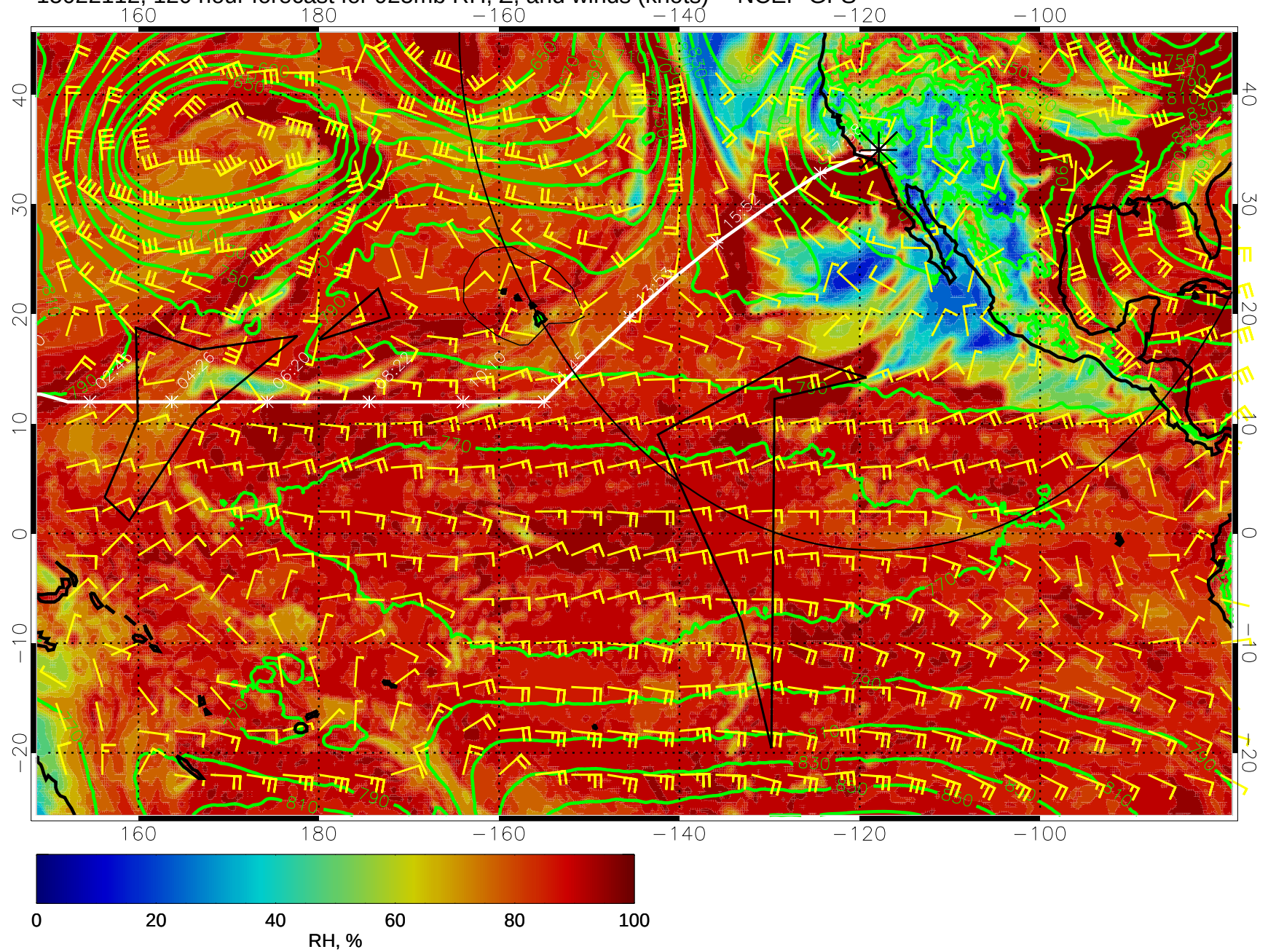
15022112, 120 hour forecast for 925mb RH, Z, and winds (knots) -- NCEP GFS
