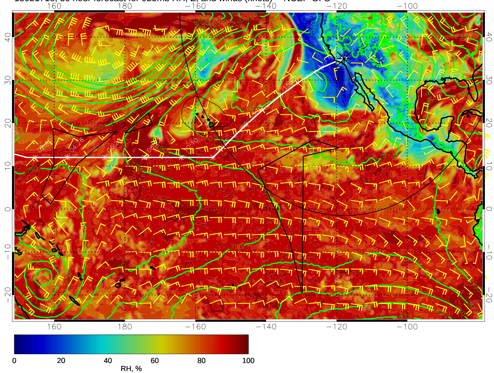
15021718, 30 hour forecast for 925mb RH, Z, and winds (knots) -- NCEP GFS
