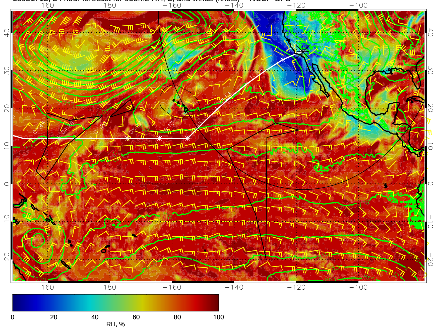
15021712, 24 hour forecast for 925mb RH, Z, and winds (knots) -- NCEP GFS
