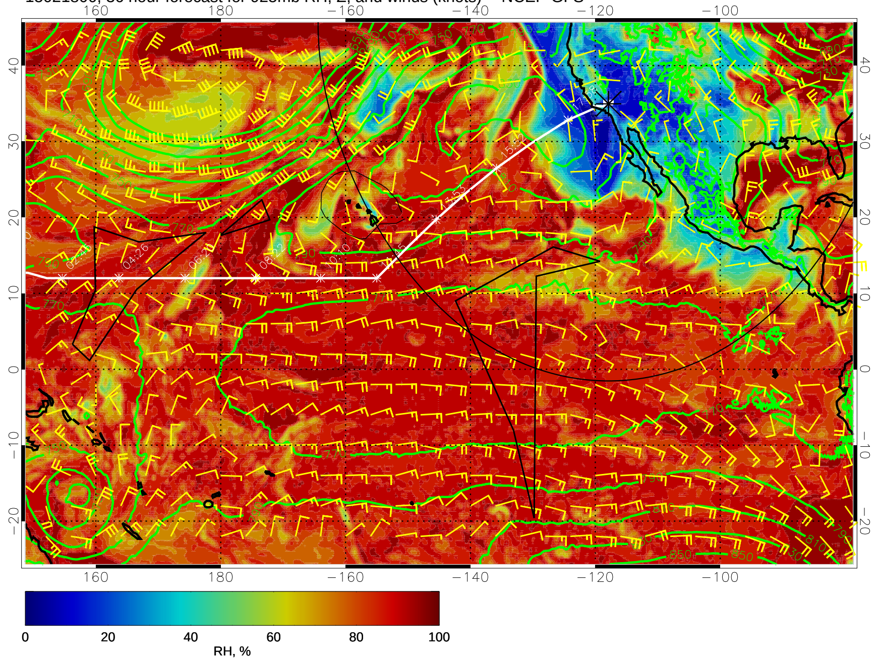
15021800, 36 hour forecast for 925mb RH, Z, and winds (knots) -- NCEP GFS
