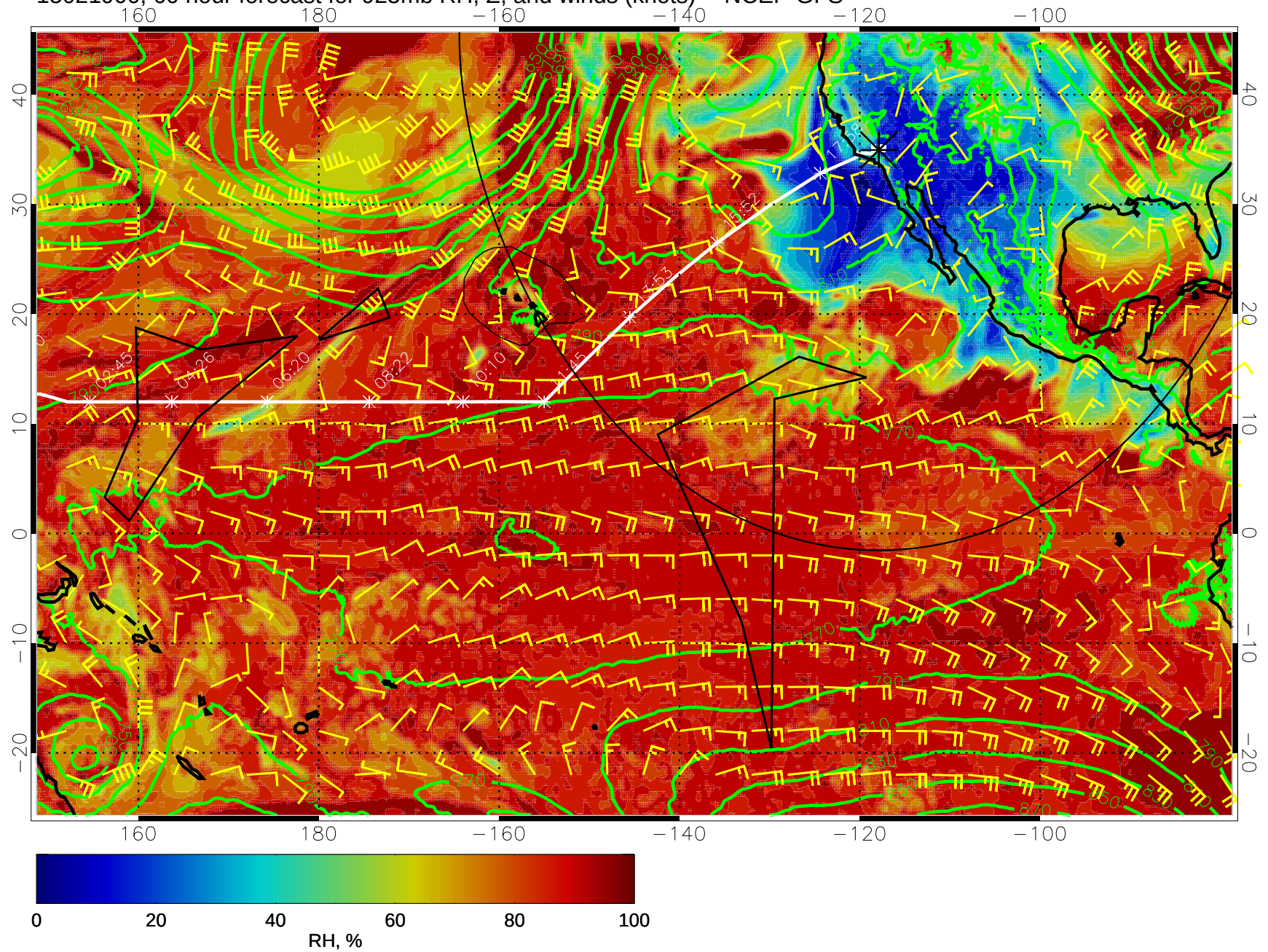
15021900, 60 hour forecast for 925mb RH, Z, and winds (knots) -- NCEP GFS
