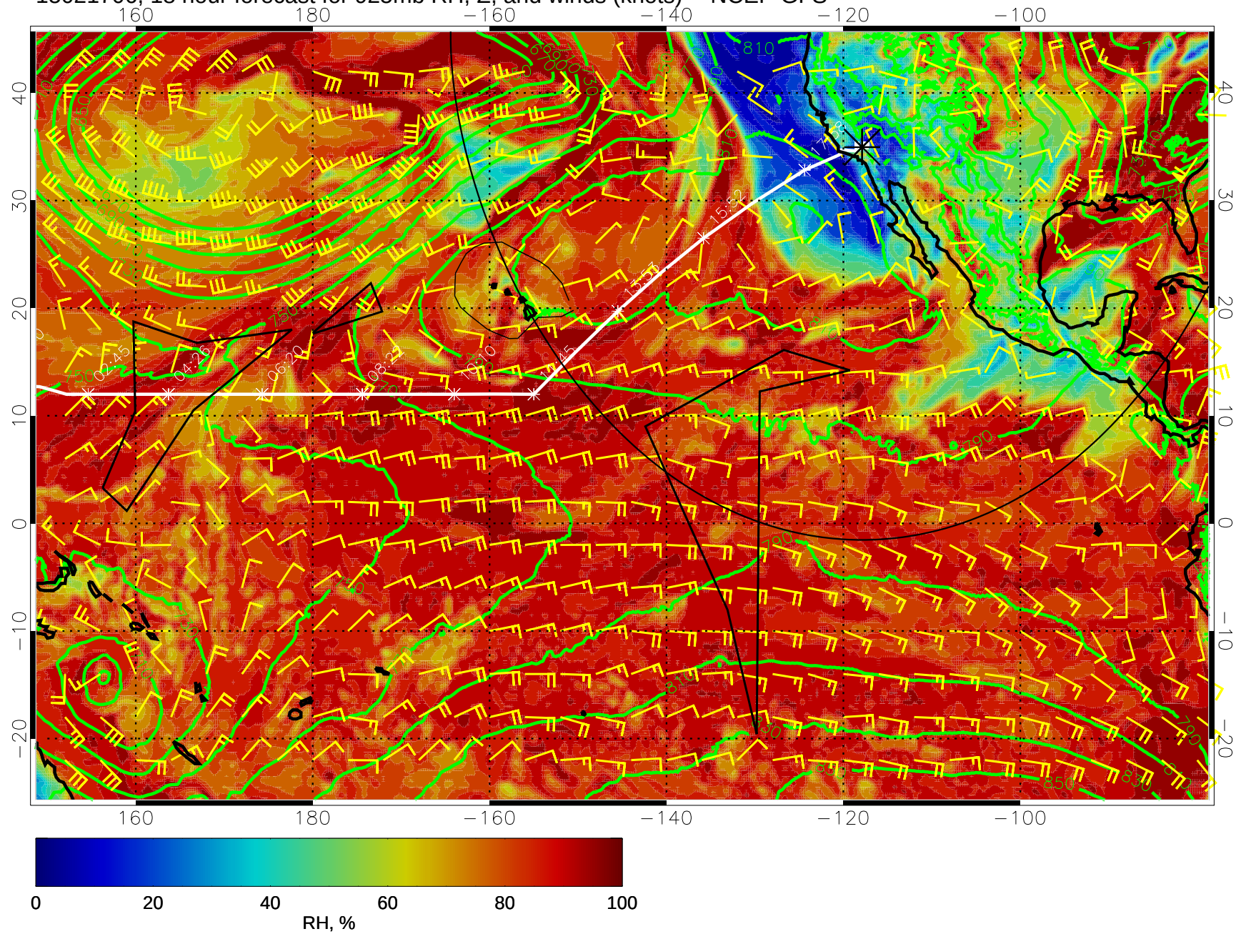
15021706, 18 hour forecast for 925mb RH, Z, and winds (knots) -- NCEP GFS
