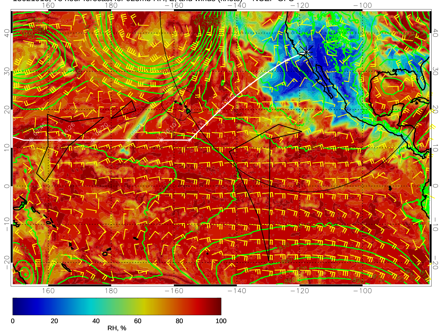
15021918, 78 hour forecast for 925mb RH, Z, and winds (knots) -- NCEP GFS
