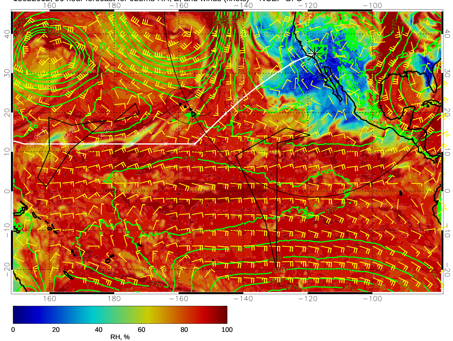
15022012, 96 hour forecast for 925mb RH, Z, and winds (knots) -- NCEP GFS
