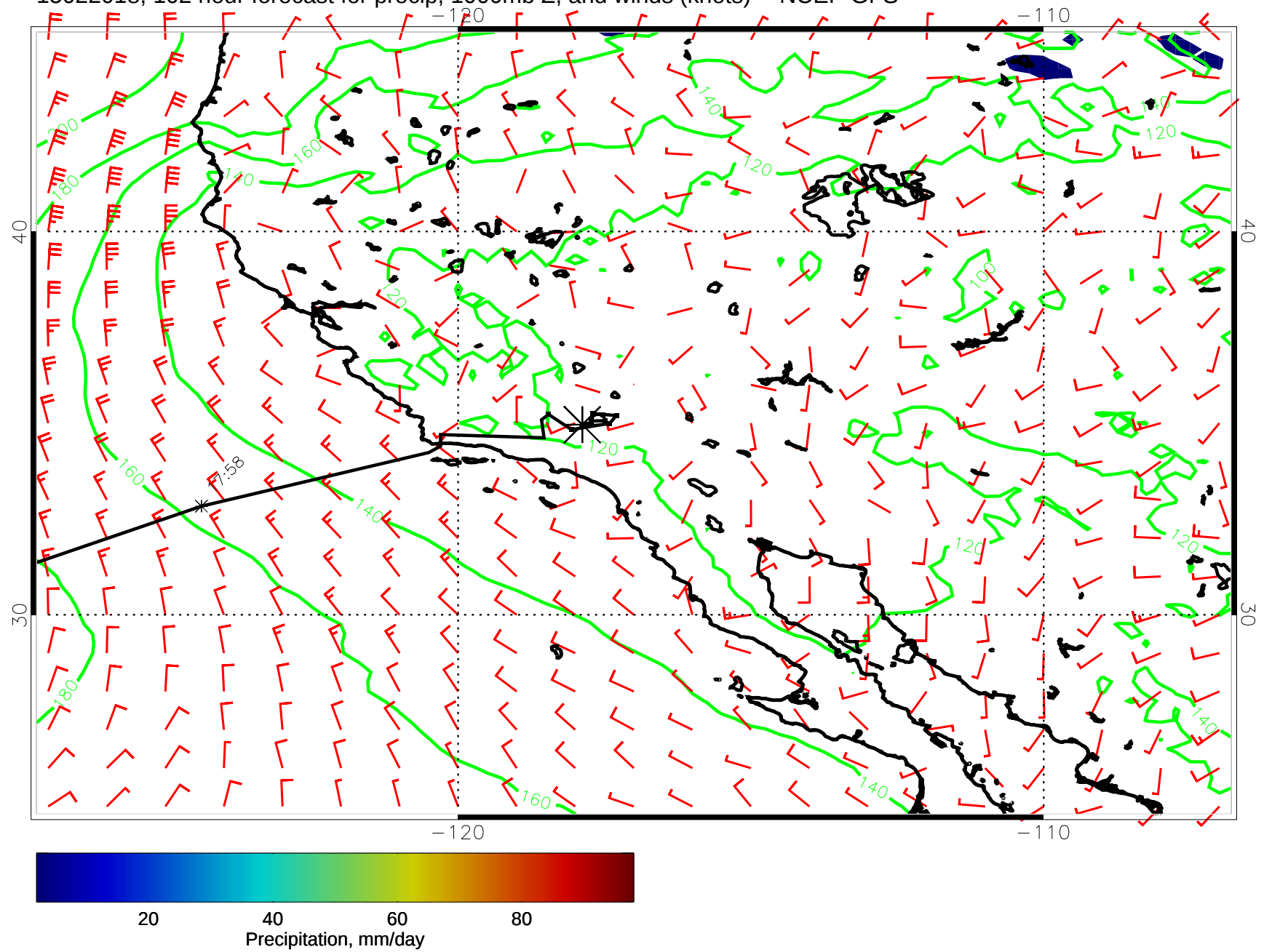
15022018, 102 hour forecast for precip, 1000mb Z, and winds (knots) -- NCEP GFS
