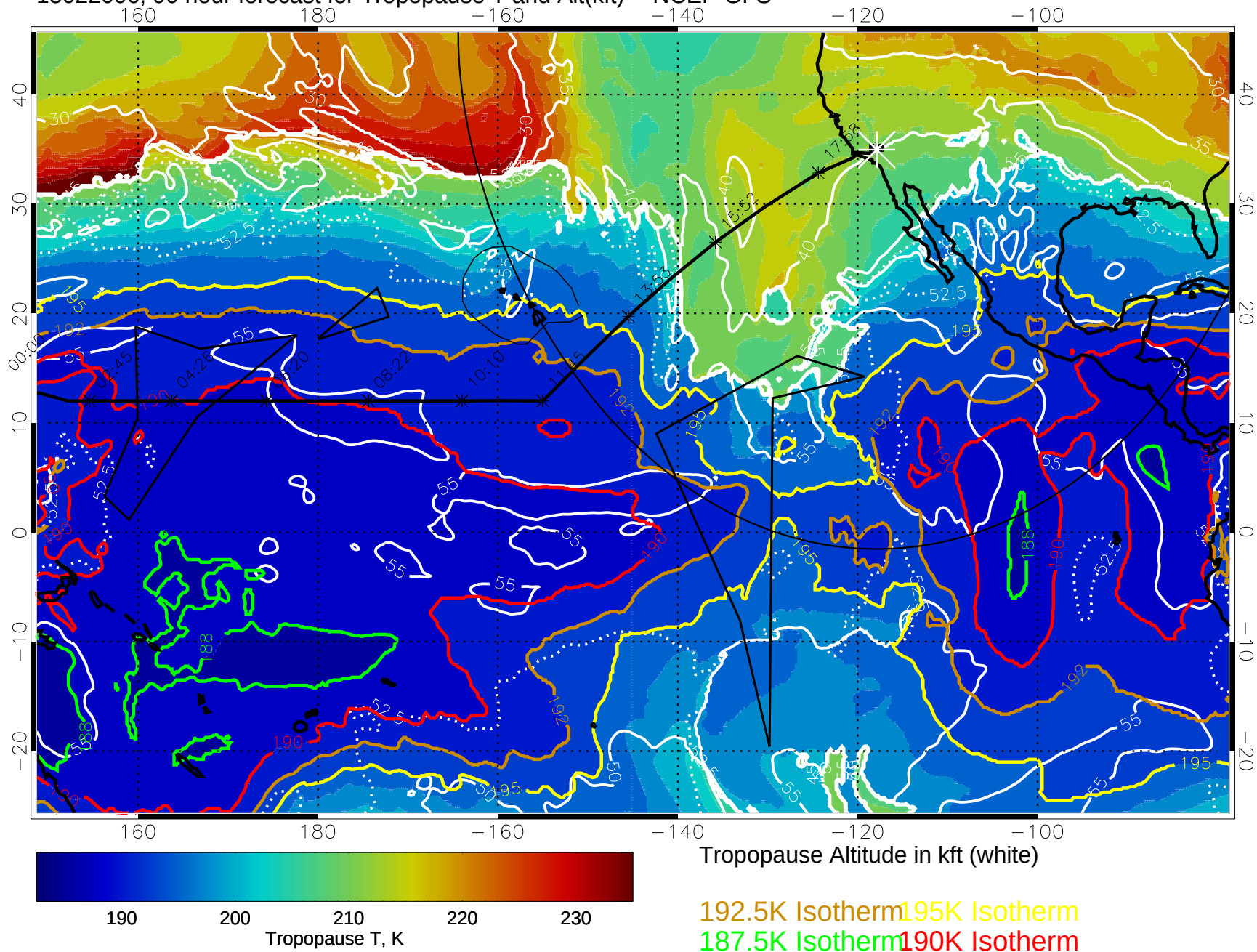
15022006, 90 hour forecast for Tropopause T and Alt(kft) -- NCEP GFS
