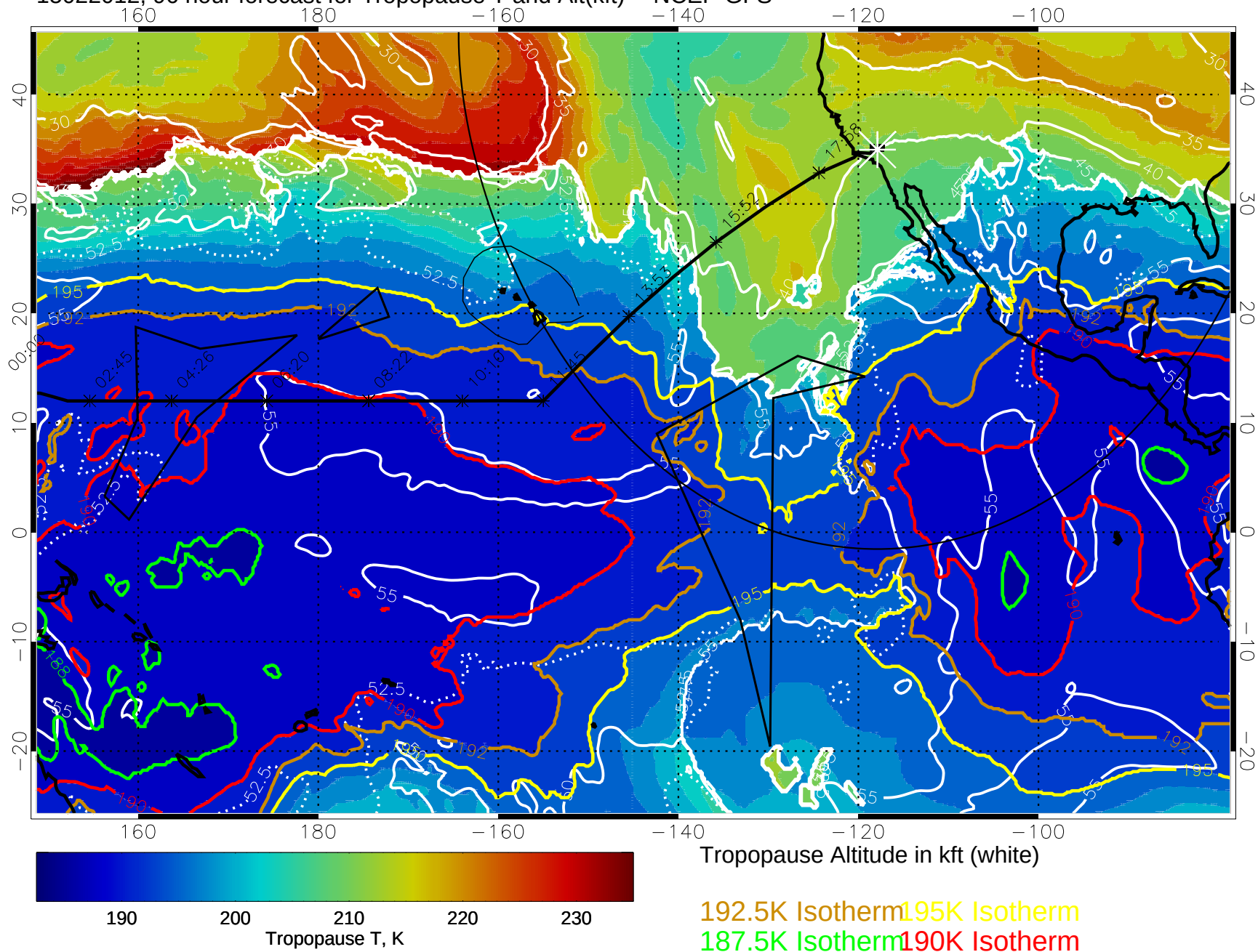
15022012, 96 hour forecast for Tropopause T and Alt(kft) -- NCEP GFS
