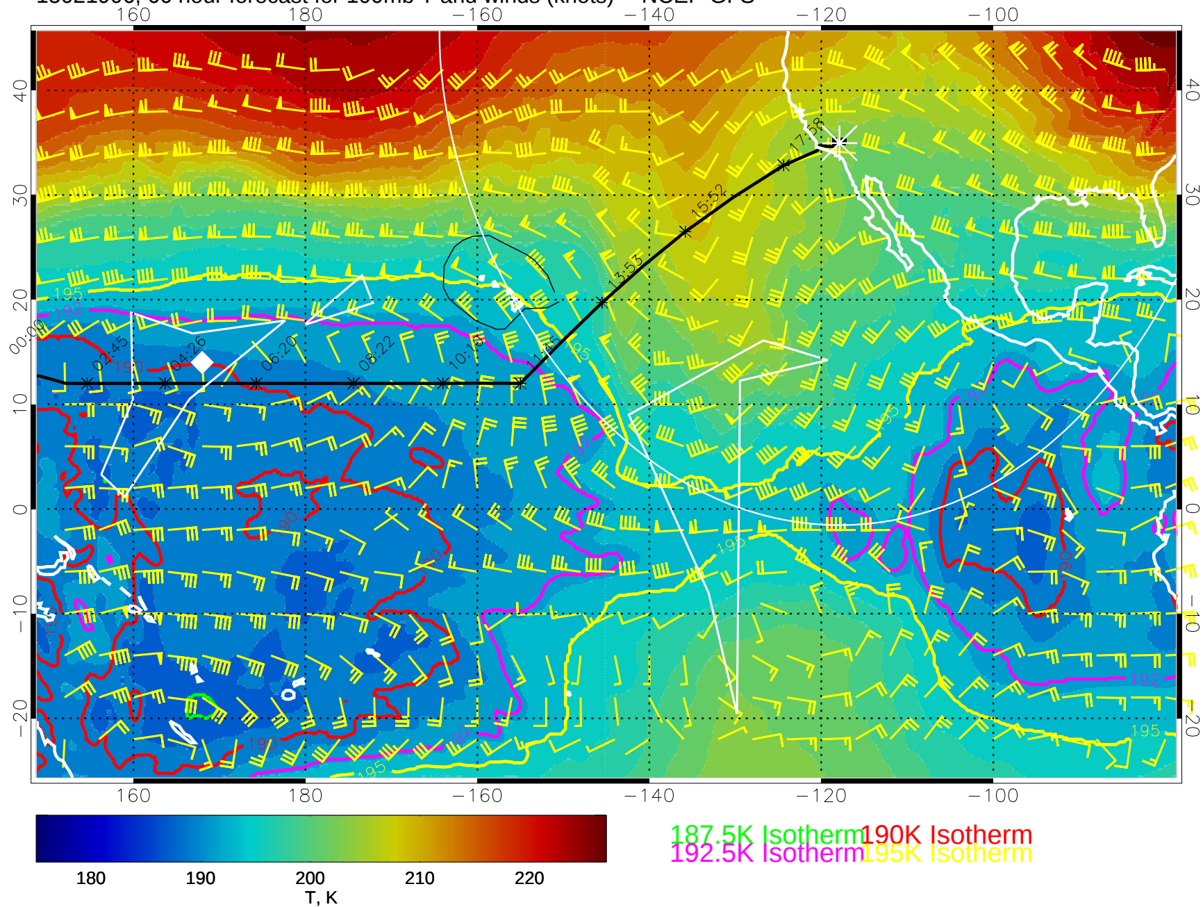
15021906, 66 hour forecast for 100mb T and winds (knots) -- NCEP GFS
