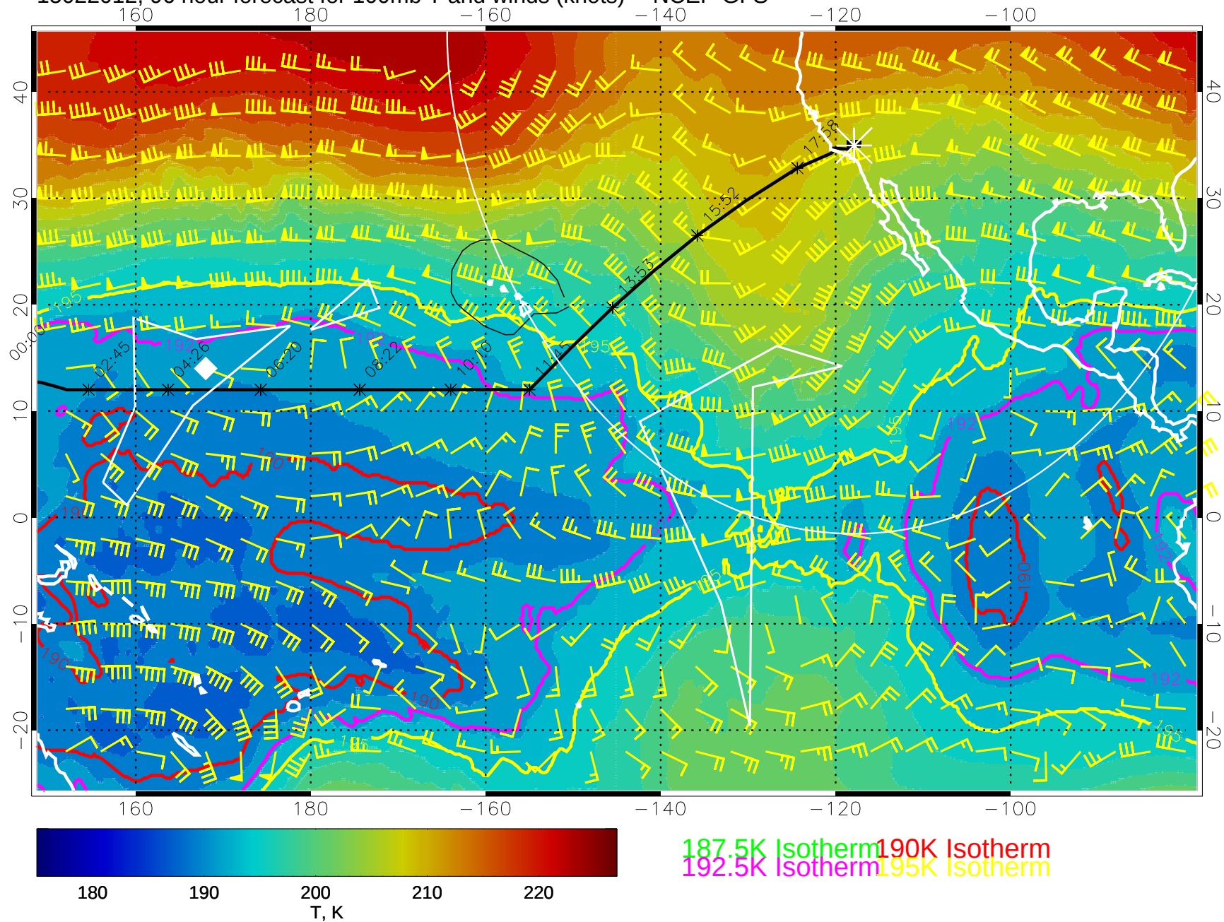
15022012, 96 hour forecast for 100mb T and winds (knots) -- NCEP GFS
