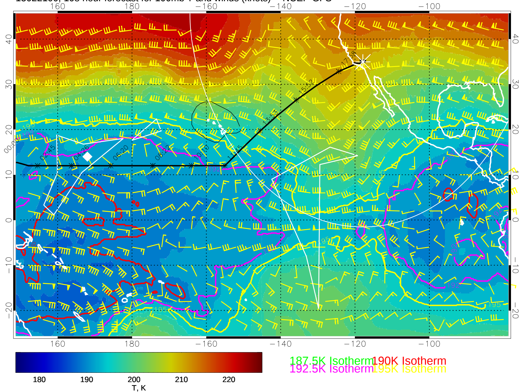
15022100, 108 hour forecast for 100mb T and winds (knots) -- NCEP GFS
