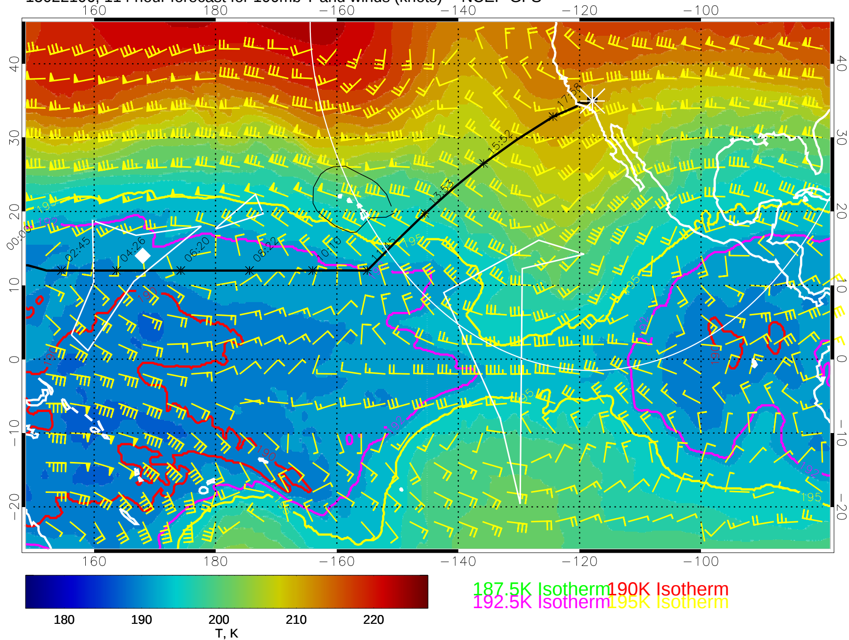
15022106, 114 hour forecast for 100mb T and winds (knots) -- NCEP GFS
