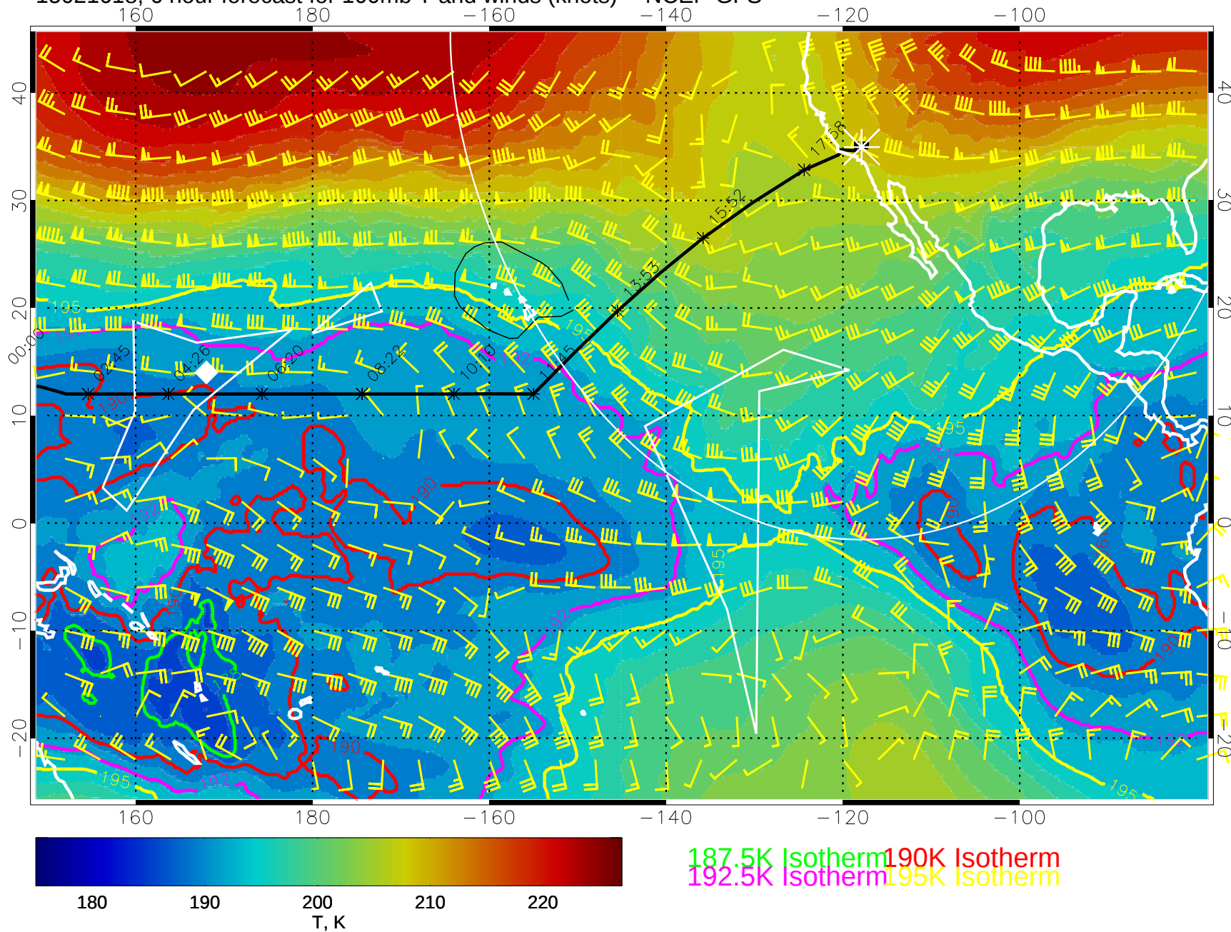
15021618, 6 hour forecast for 100mb T and winds (knots) -- NCEP GFS
