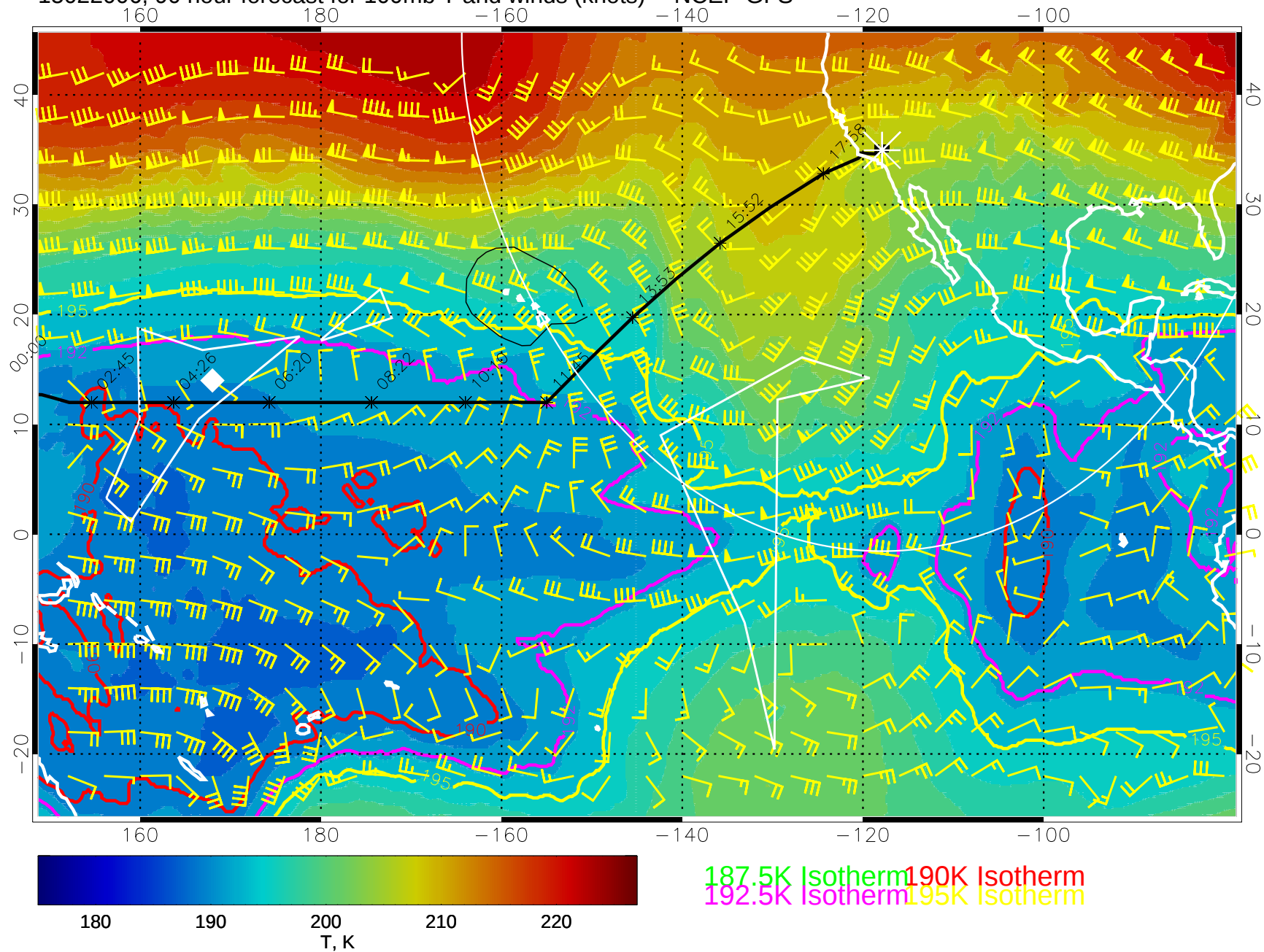
15022006, 90 hour forecast for 100mb T and winds (knots) -- NCEP GFS
