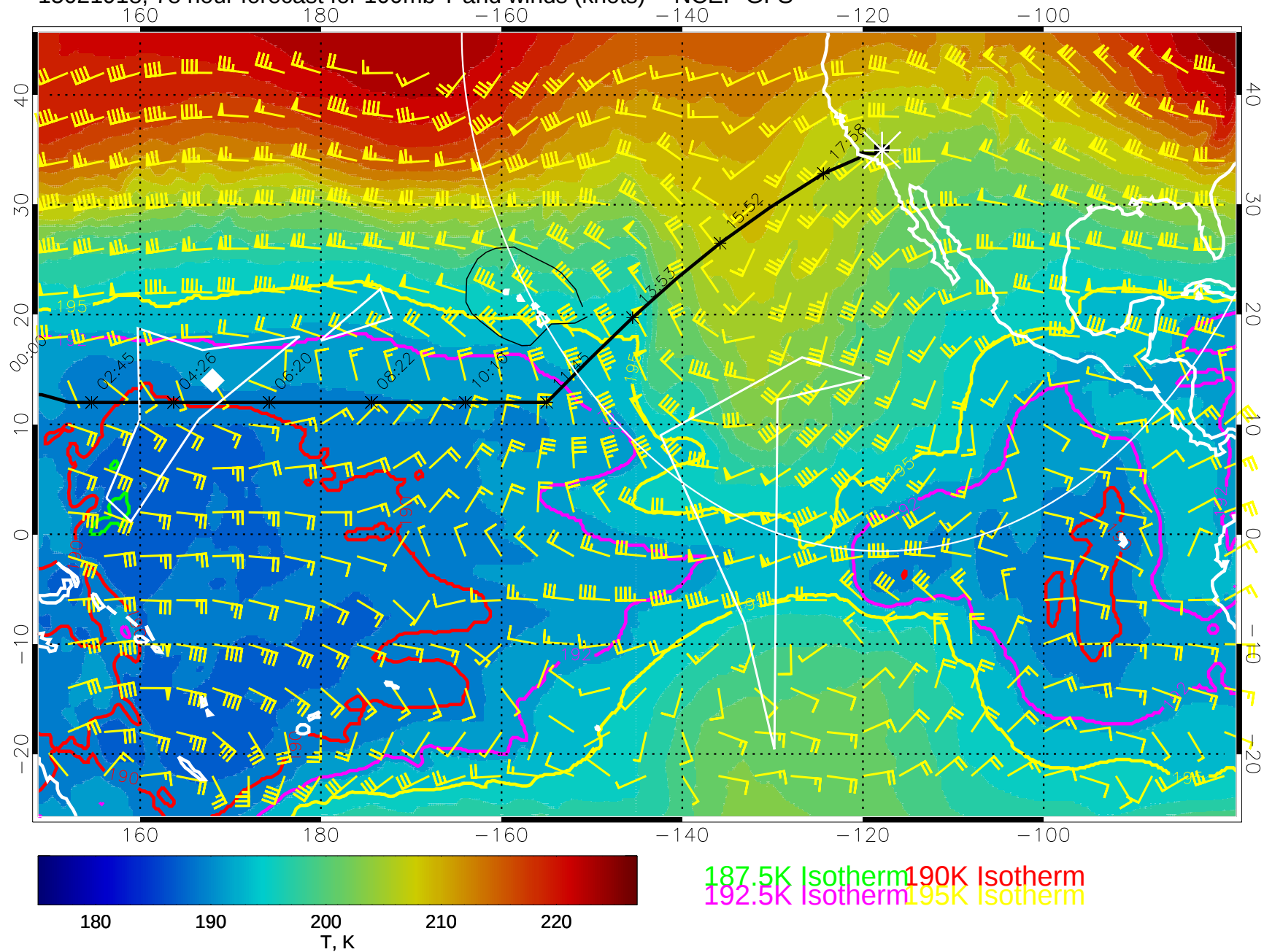
15021918, 78 hour forecast for 100mb T and winds (knots) -- NCEP GFS
