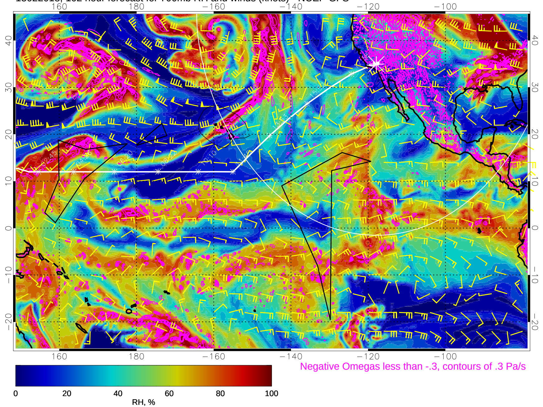
15022018, 102 hour forecast for 700mb RH and winds (knots) - NCEP GFS
