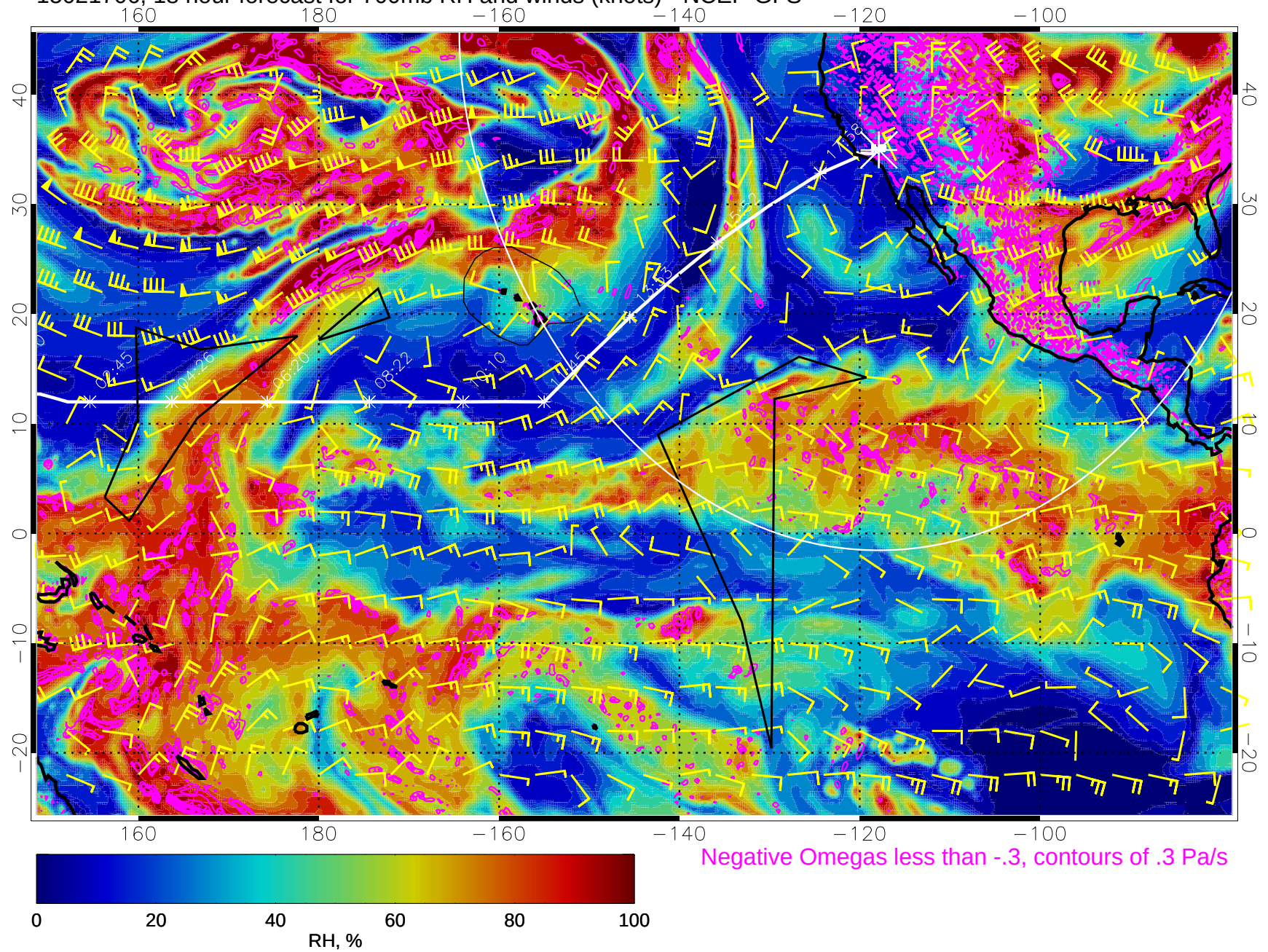
15021706, 18 hour forecast for 700mb RH and winds (knots) - NCEP GFS
