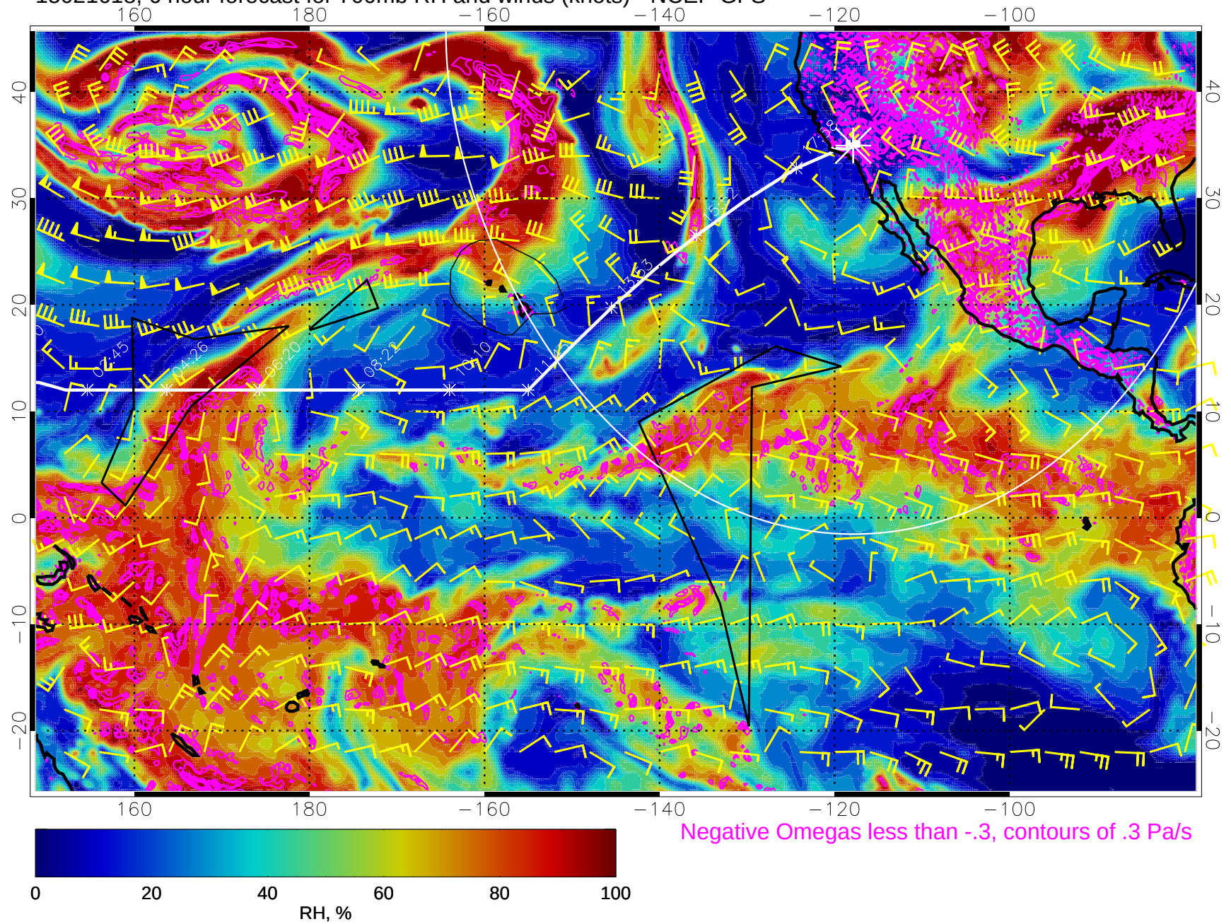
15021618, 6 hour forecast for 700mb RH and winds (knots) - NCEP GFS
