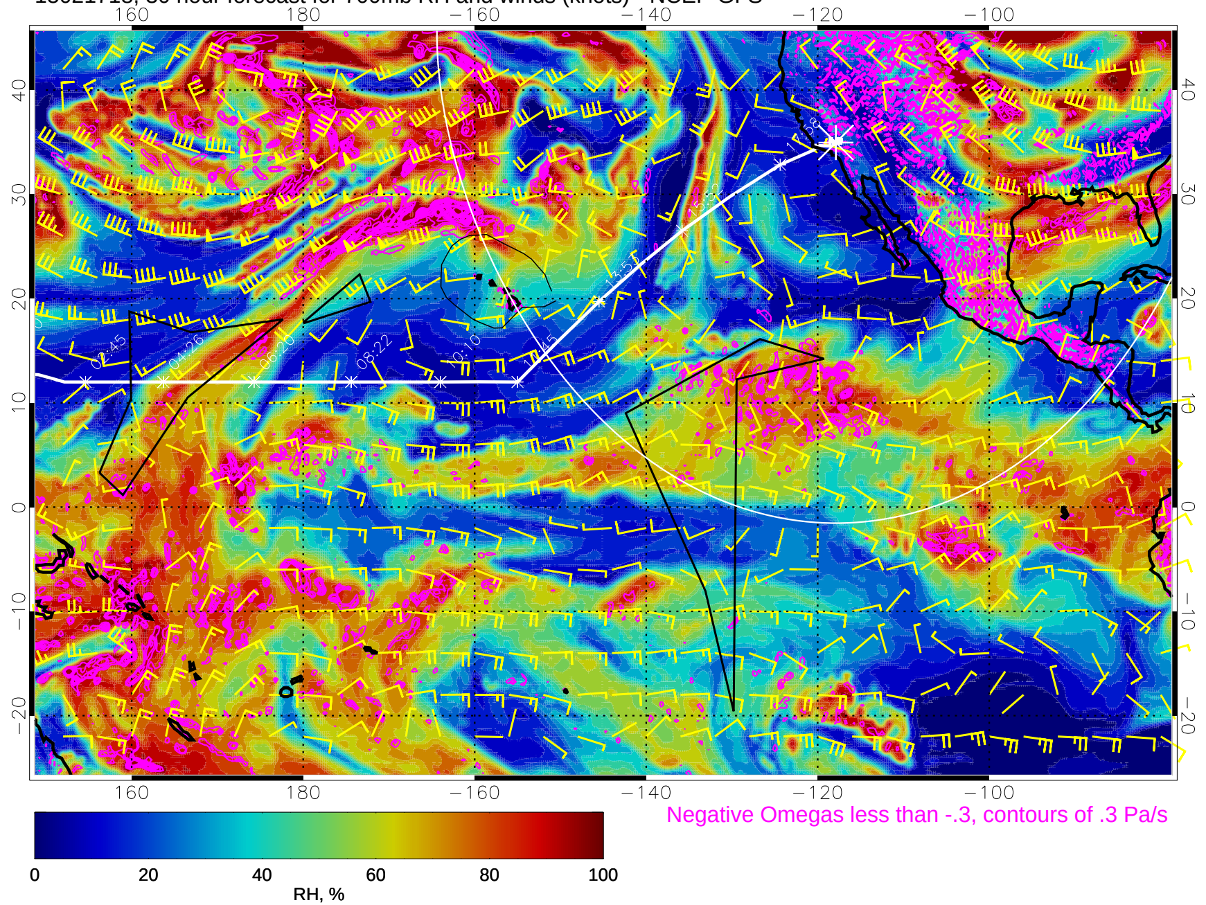
15021718, 30 hour forecast for 700mb RH and winds (knots) - NCEP GFS
