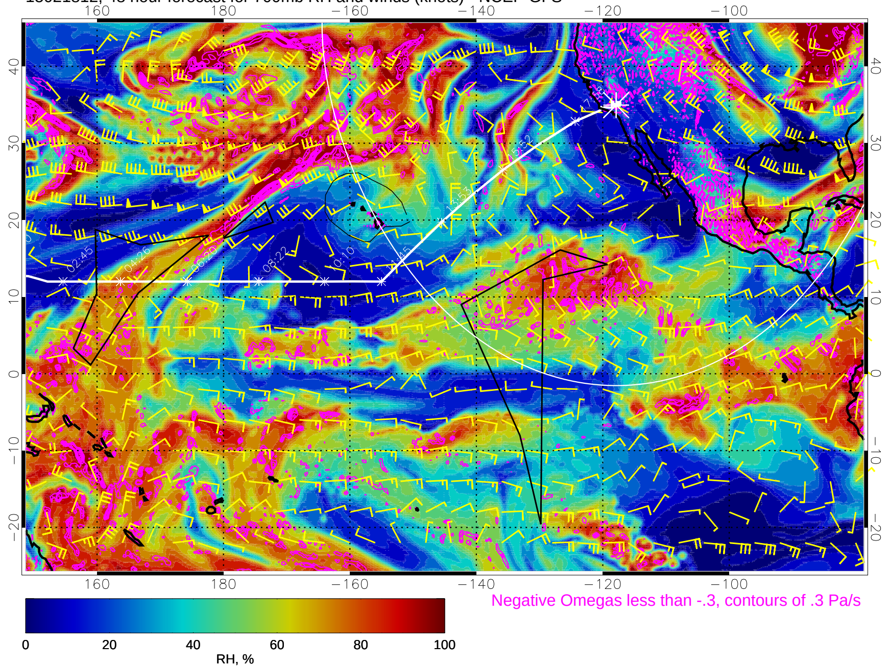
15021812, 48 hour forecast for 700mb RH and winds (knots) - NCEP GFS
