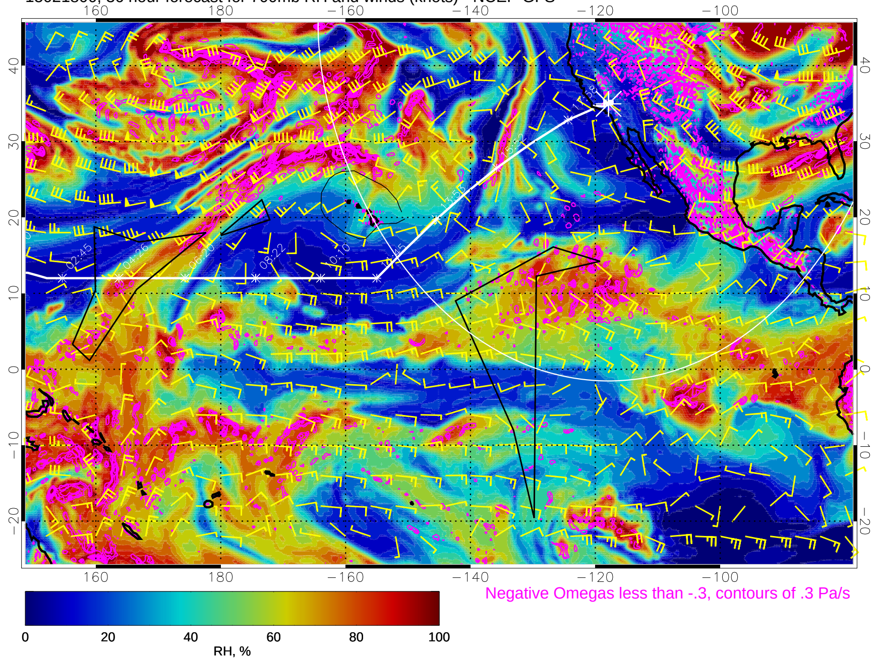
15021800, 36 hour forecast for 700mb RH and winds (knots) - NCEP GFS
