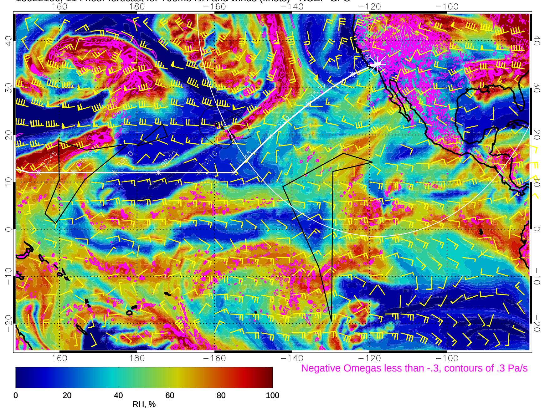
15022106, 114 hour forecast for 700mb RH and winds (knots) - NCEP GFS
