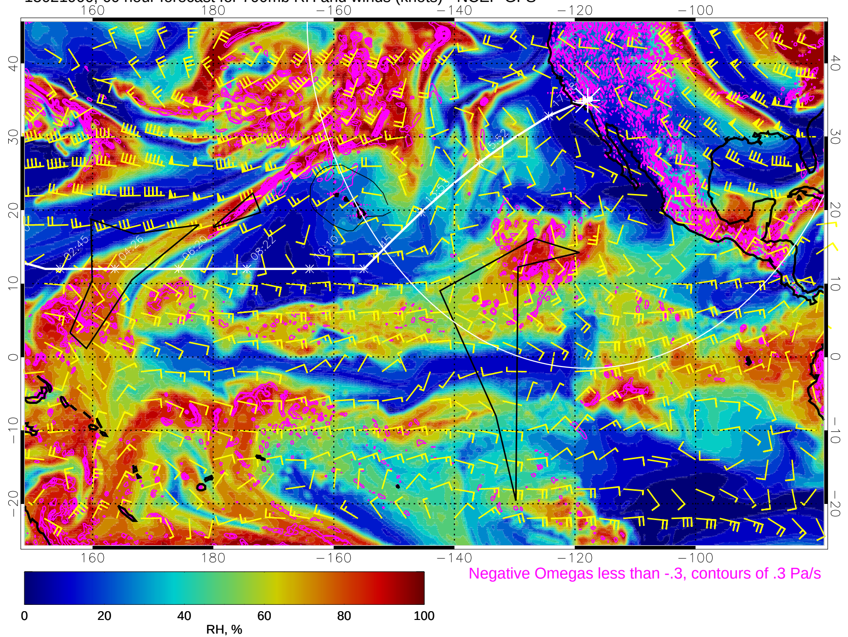
15021900, 60 hour forecast for 700mb RH and winds (knots) - NCEP GFS
