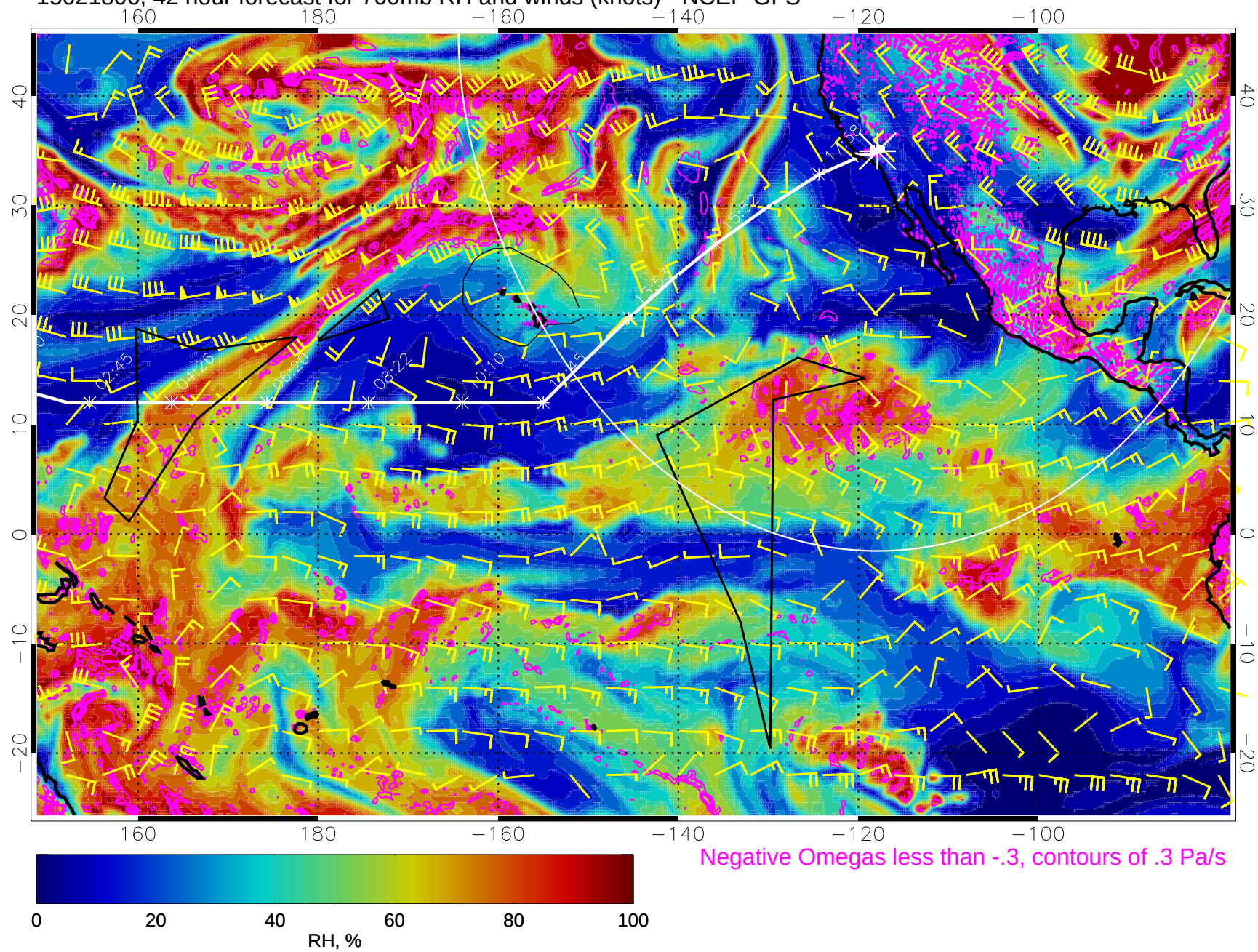
15021806, 42 hour forecast for 700mb RH and winds (knots) - NCEP GFS
