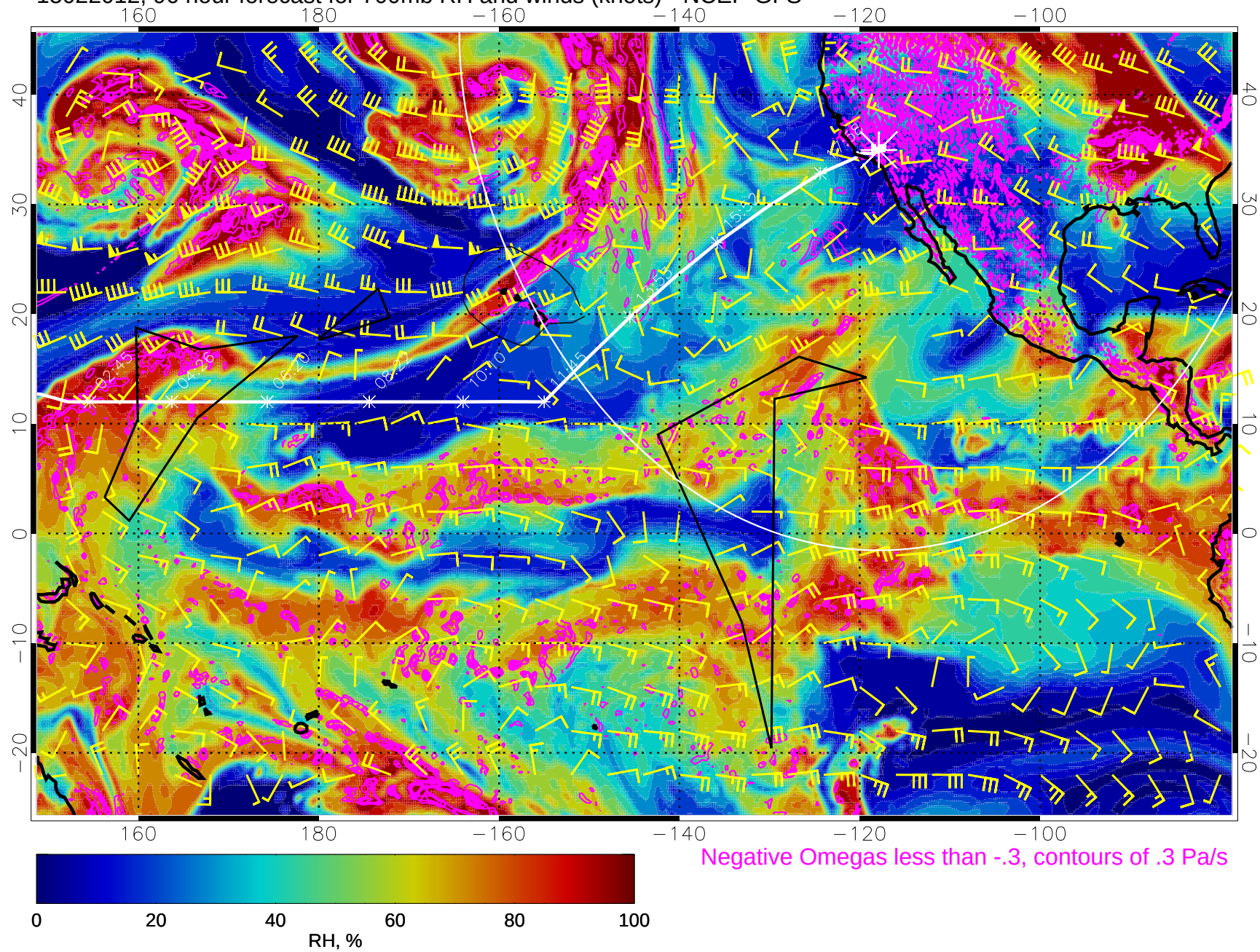
15022012, 96 hour forecast for 700mb RH and winds (knots) - NCEP GFS
