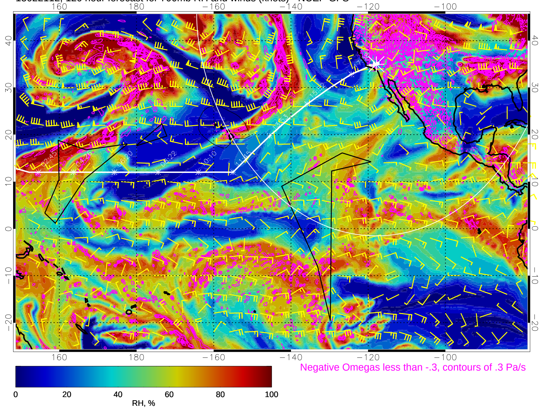
15022112, 120 hour forecast for 700mb RH and winds (knots) - NCEP GFS
