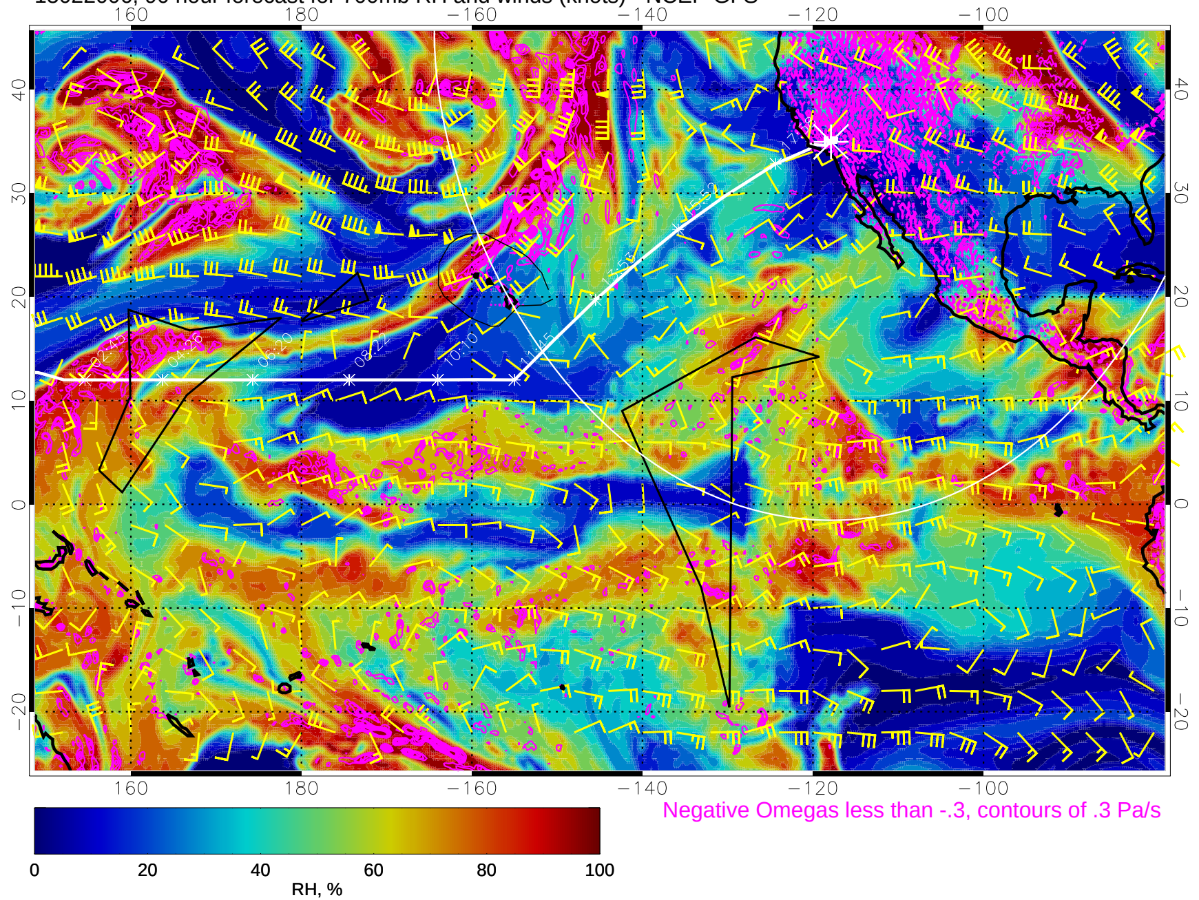
15022006, 90 hour forecast for 700mb RH and winds (knots) - NCEP GFS
