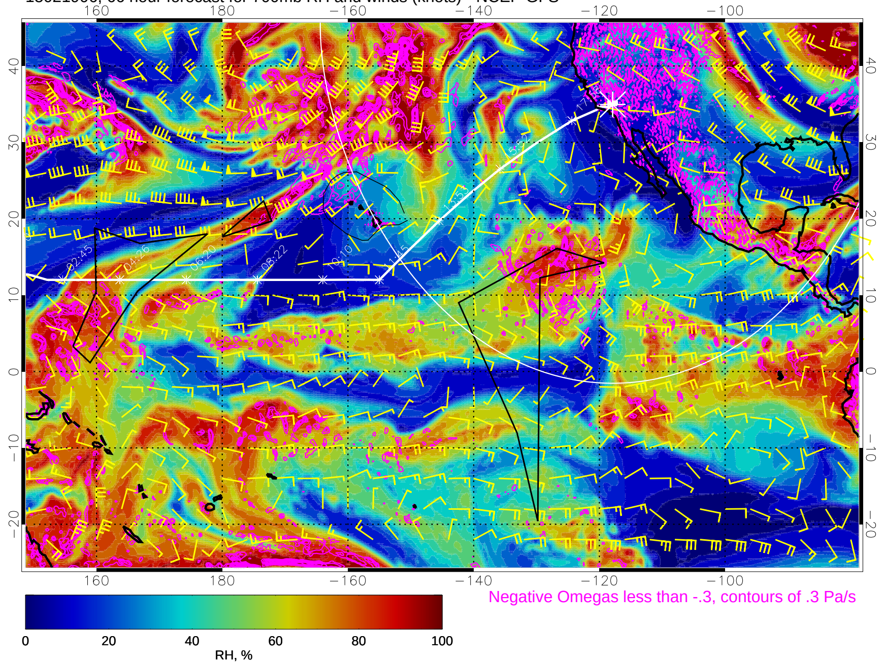
15021906, 66 hour forecast for 700mb RH and winds (knots) - NCEP GFS
