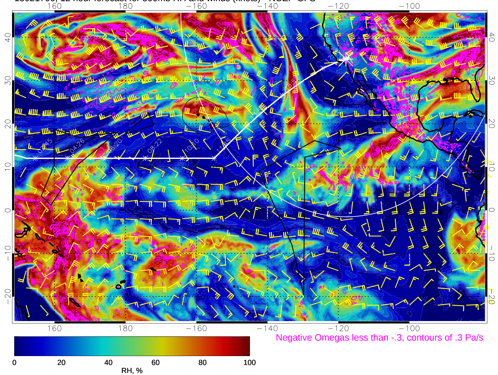
15021700, 12 hour forecast for 500mb RH and winds (knots) - NCEP GFS
