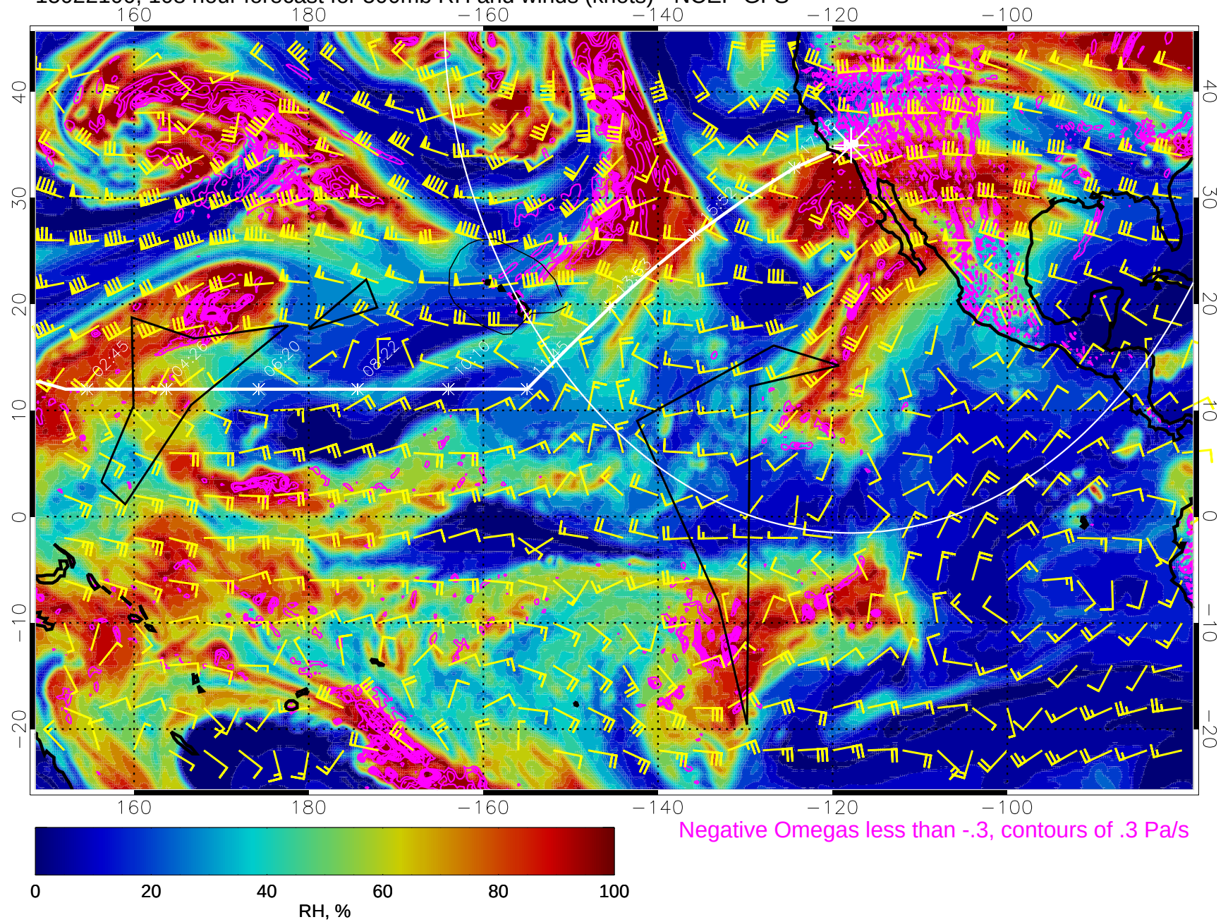
15022100, 108 hour forecast for 500mb RH and winds (knots) - NCEP GFS
