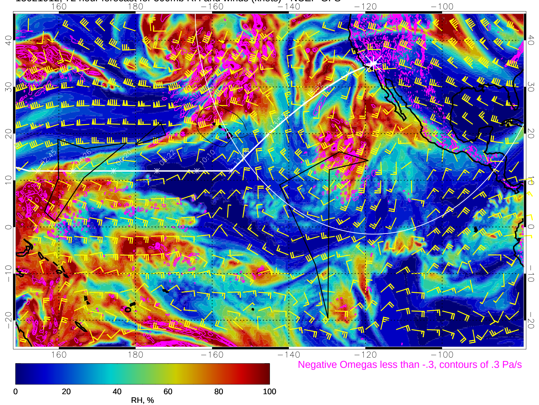
15021912, 72 hour forecast for 500mb RH and winds (knots) - NCEP GFS
