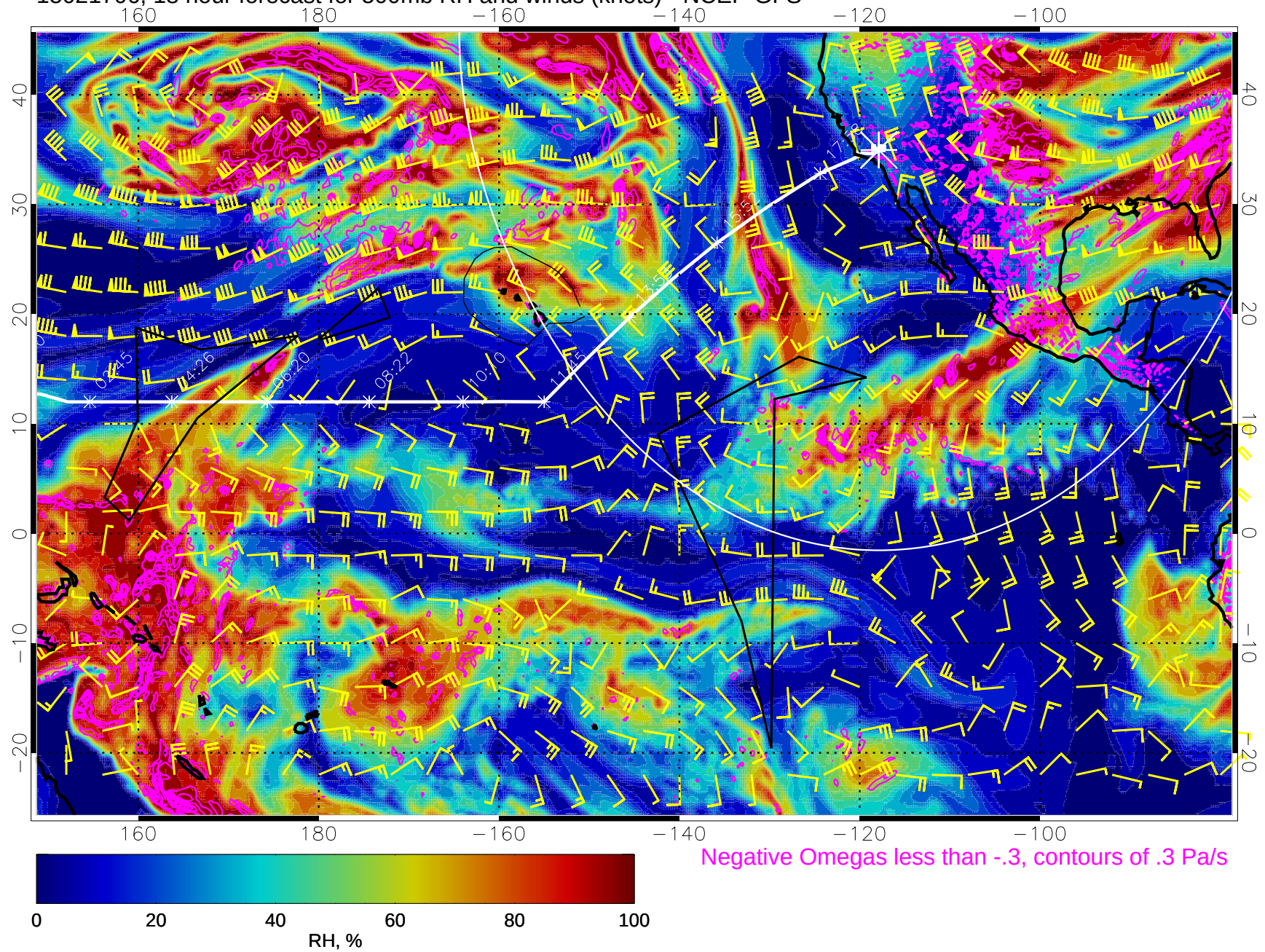
15021706, 18 hour forecast for 500mb RH and winds (knots) - NCEP GFS
