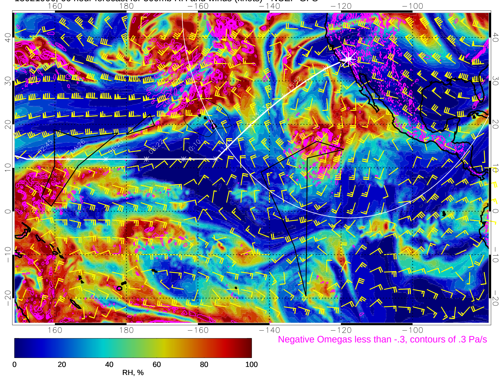
15021906, 66 hour forecast for 500mb RH and winds (knots) - NCEP GFS
