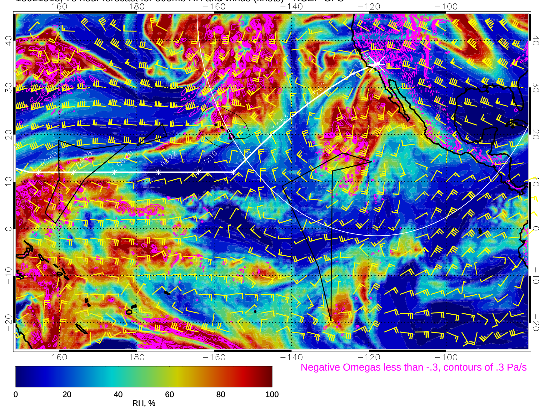
15021918, 78 hour forecast for 500mb RH and winds (knots) - NCEP GFS
