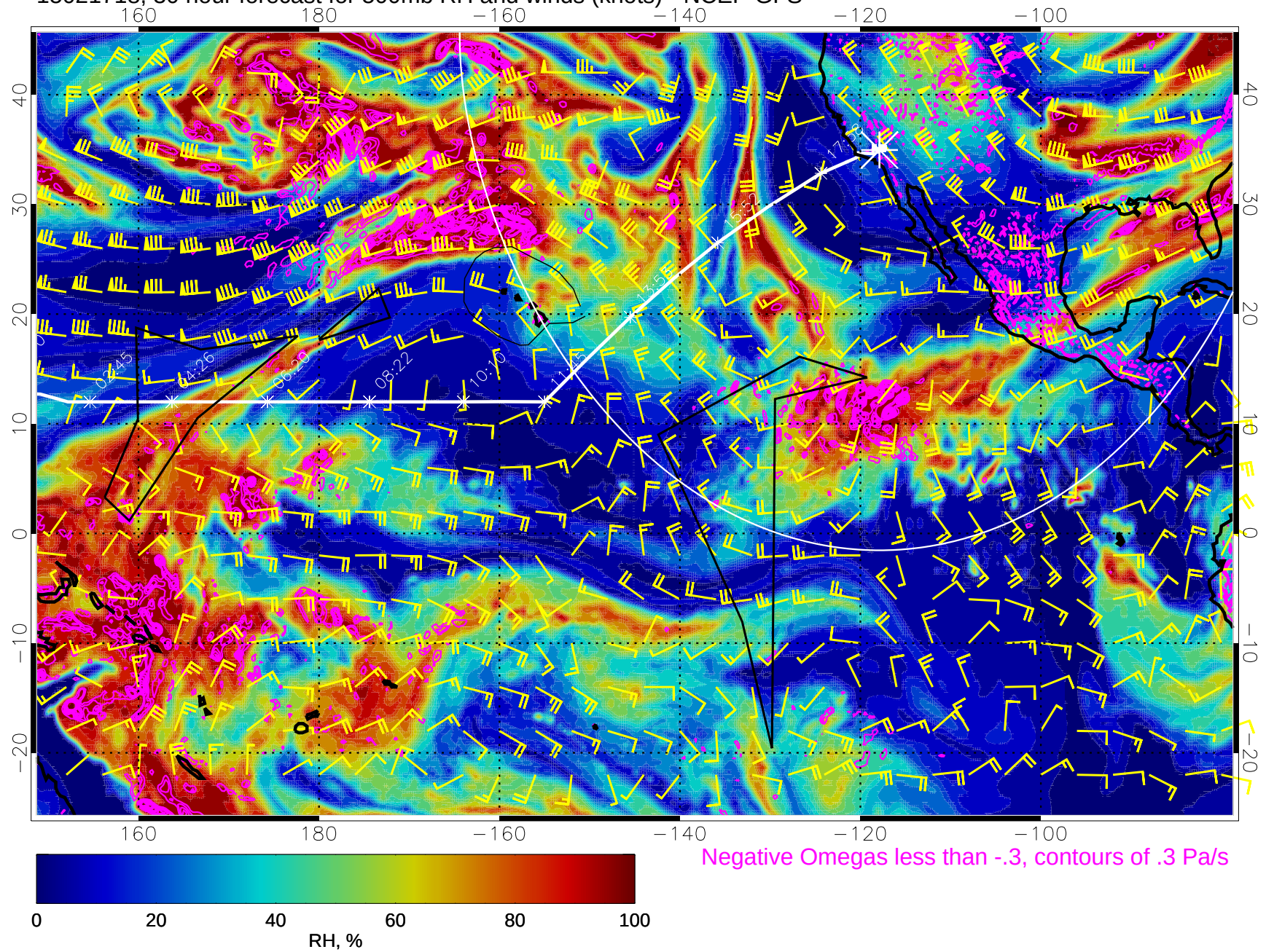
15021718, 30 hour forecast for 500mb RH and winds (knots) - NCEP GFS
