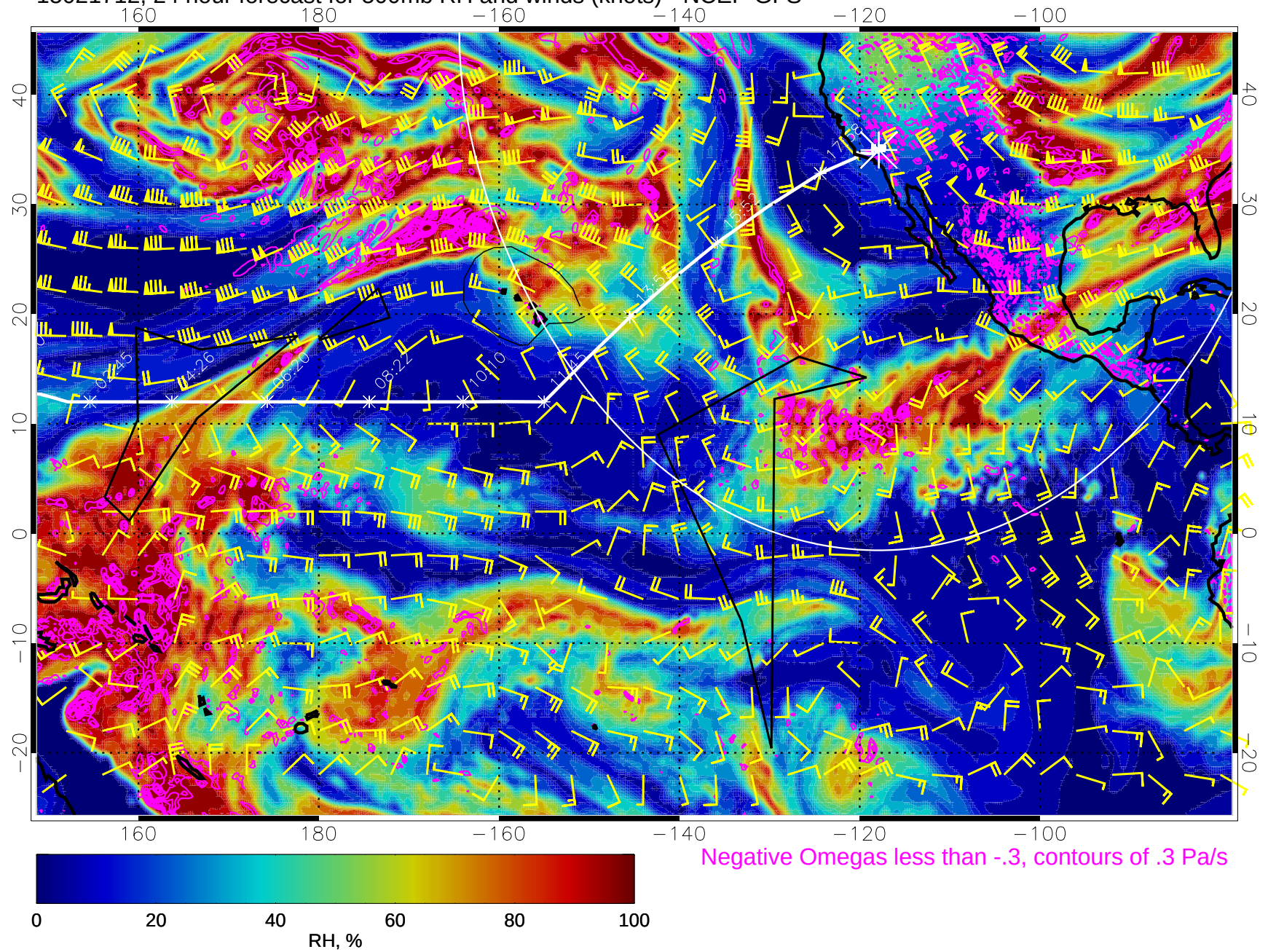
15021712, 24 hour forecast for 500mb RH and winds (knots) - NCEP GFS
