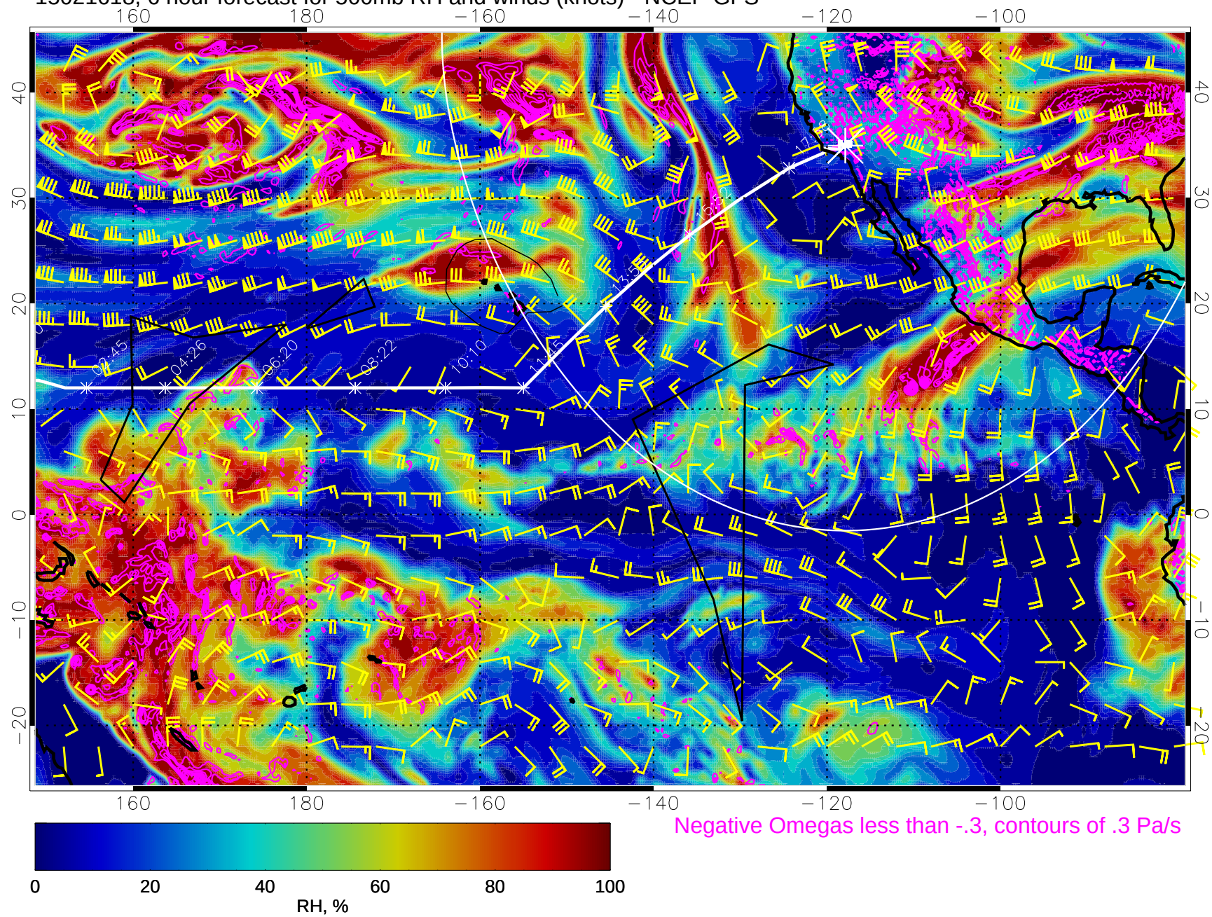
15021618, 6 hour forecast for 500mb RH and winds (knots) - NCEP GFS
