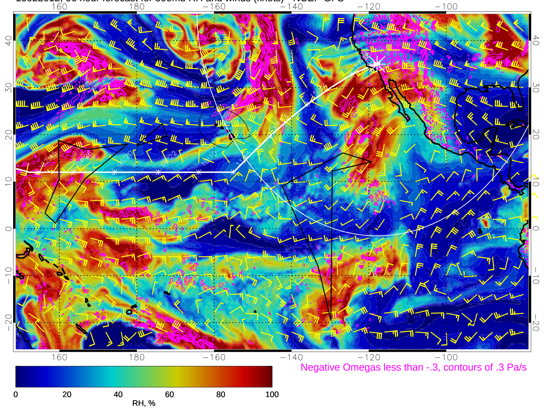
15022012, 96 hour forecast for 500mb RH and winds (knots) - NCEP GFS
