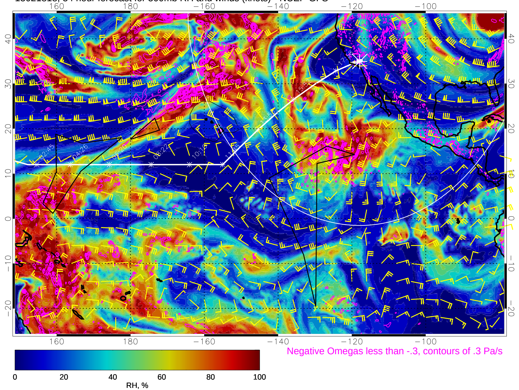
15021818, 54 hour forecast for 500mb RH and winds (knots) - NCEP GFS
