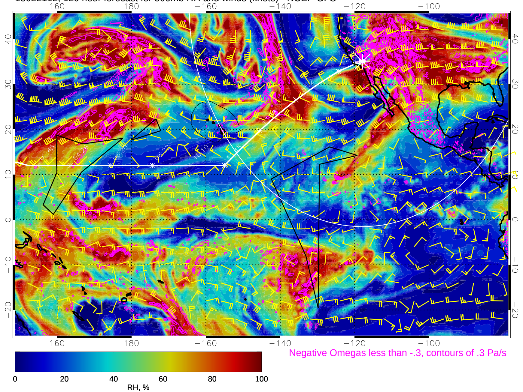
15022112, 120 hour forecast for 500mb RH and winds (knots) - NCEP GFS
