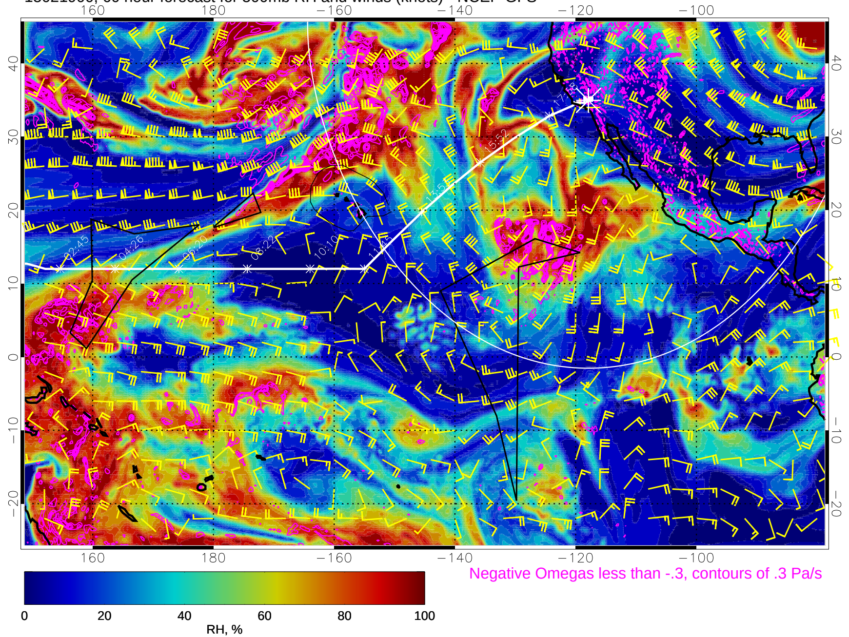
15021900, 60 hour forecast for 500mb RH and winds (knots) - NCEP GFS
