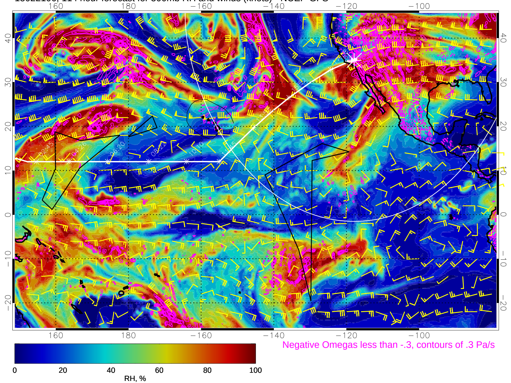
15022106, 114 hour forecast for 500mb RH and winds (knots) - NCEP GFS
