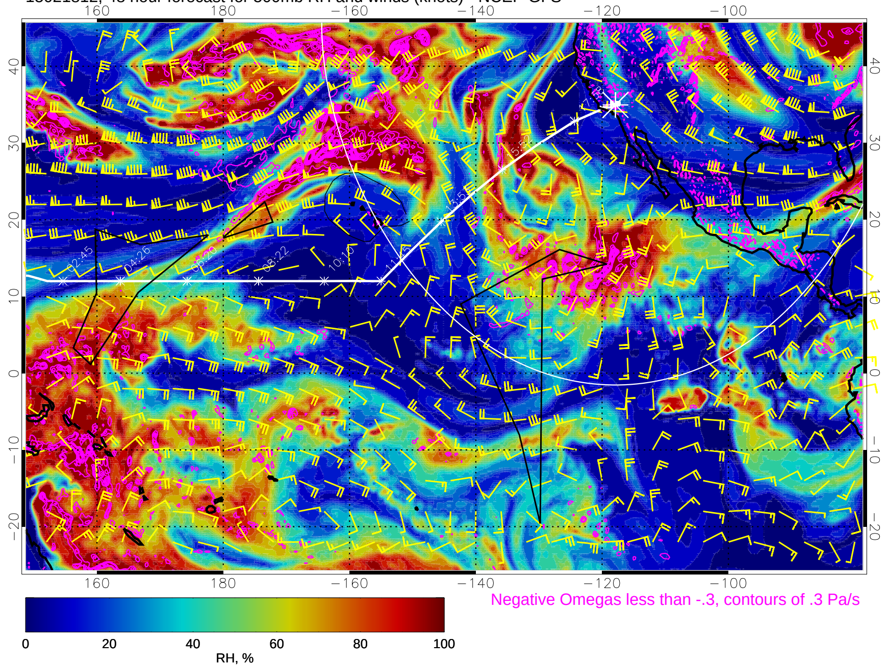
15021812, 48 hour forecast for 500mb RH and winds (knots) - NCEP GFS
