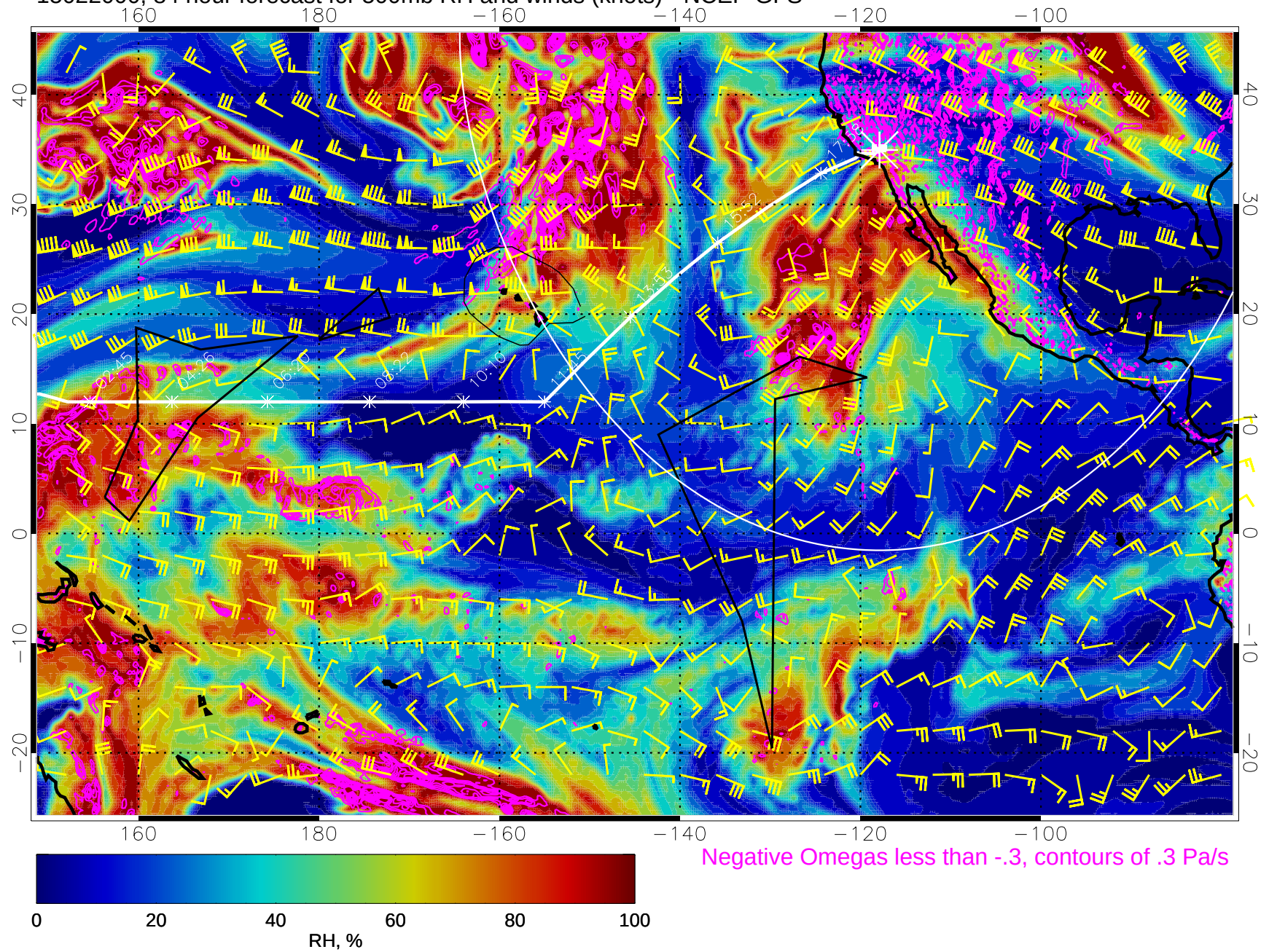
15022000, 84 hour forecast for 500mb RH and winds (knots) - NCEP GFS
