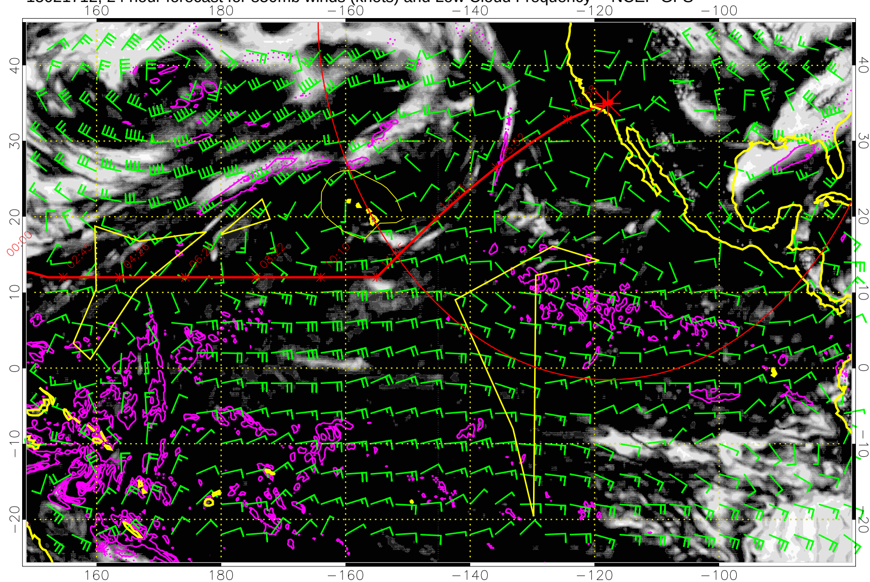
15021712, 24 hour forecast for 850mb winds (knots) and Low Cloud Frequency -- NCEP GFS
