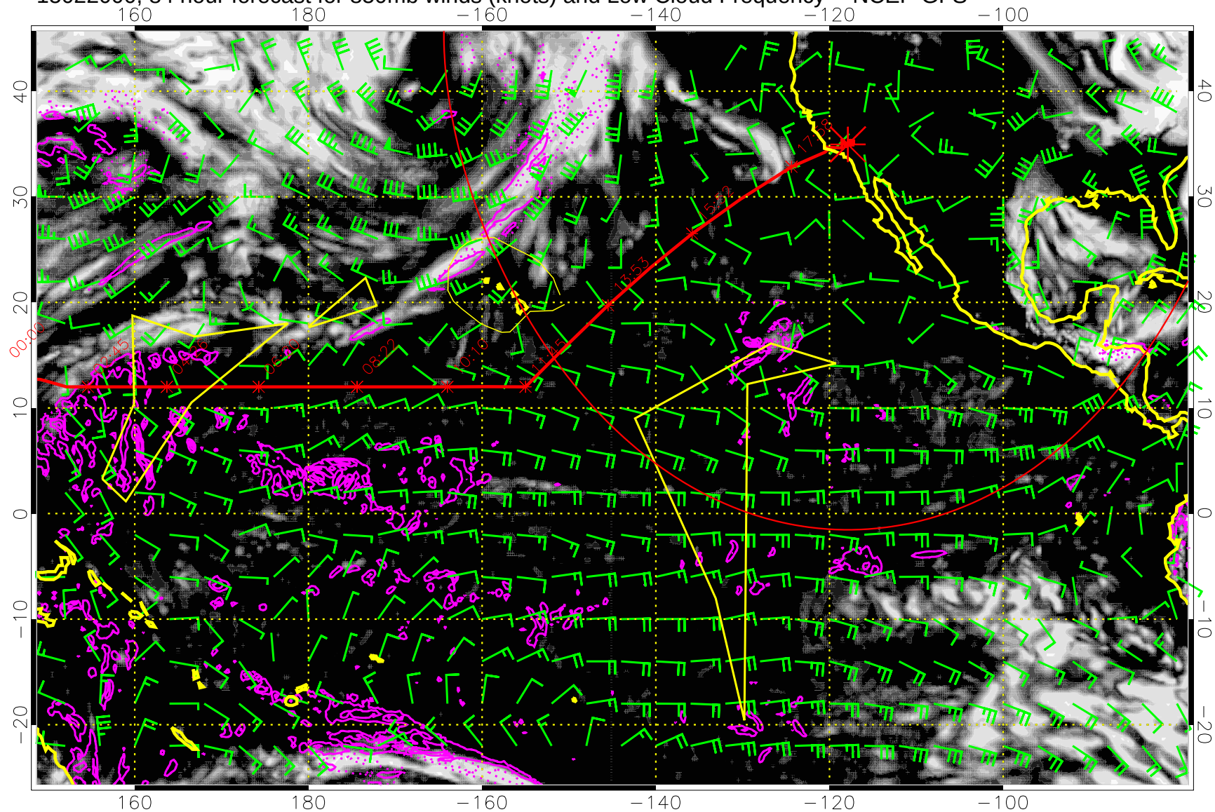
15022000, 84 hour forecast for 850mb winds (knots) and Low Cloud Frequency -- NCEP GFS
