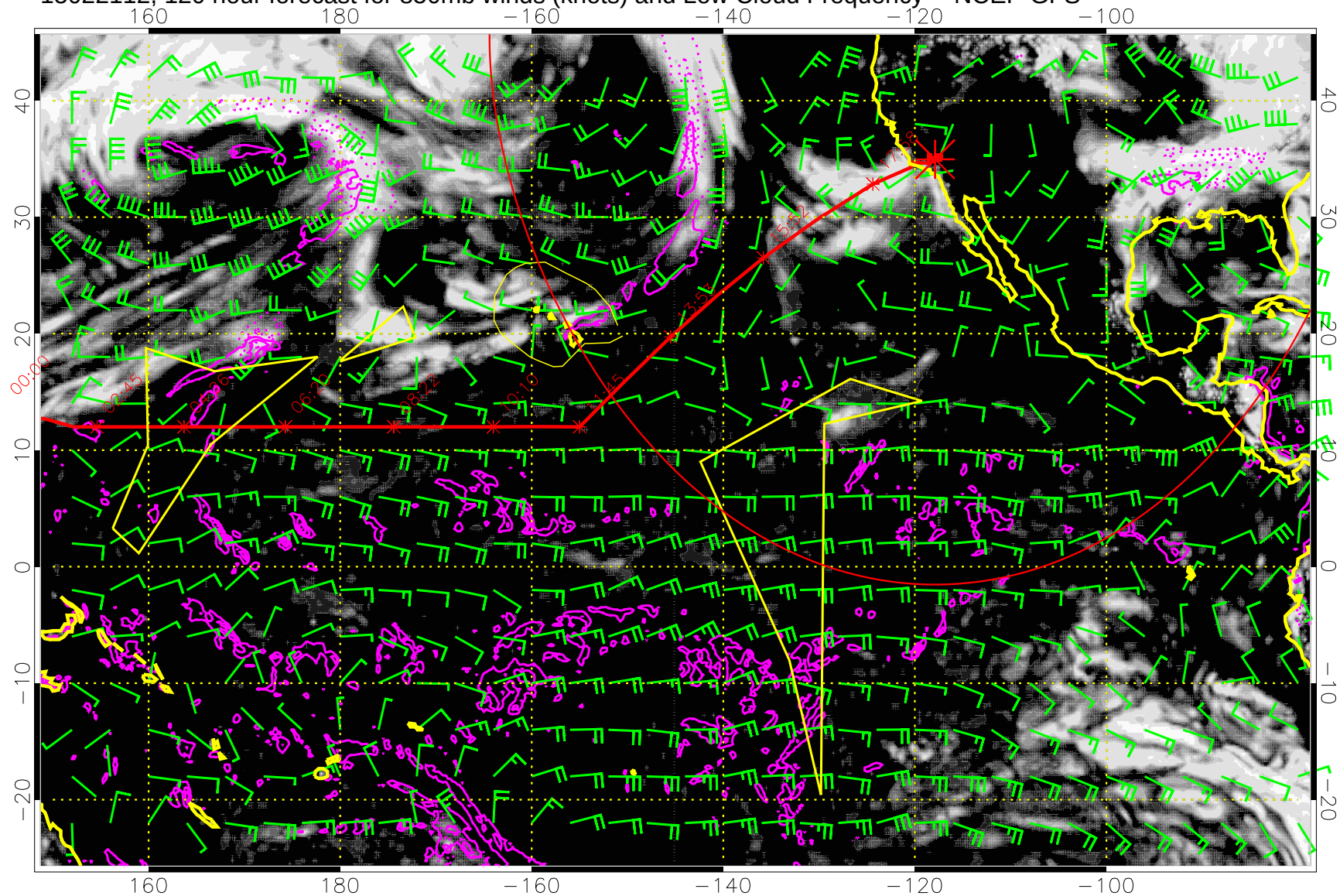
15022112, 120 hour forecast for 850mb winds (knots) and Low Cloud Frequency -- NCEP GFS
