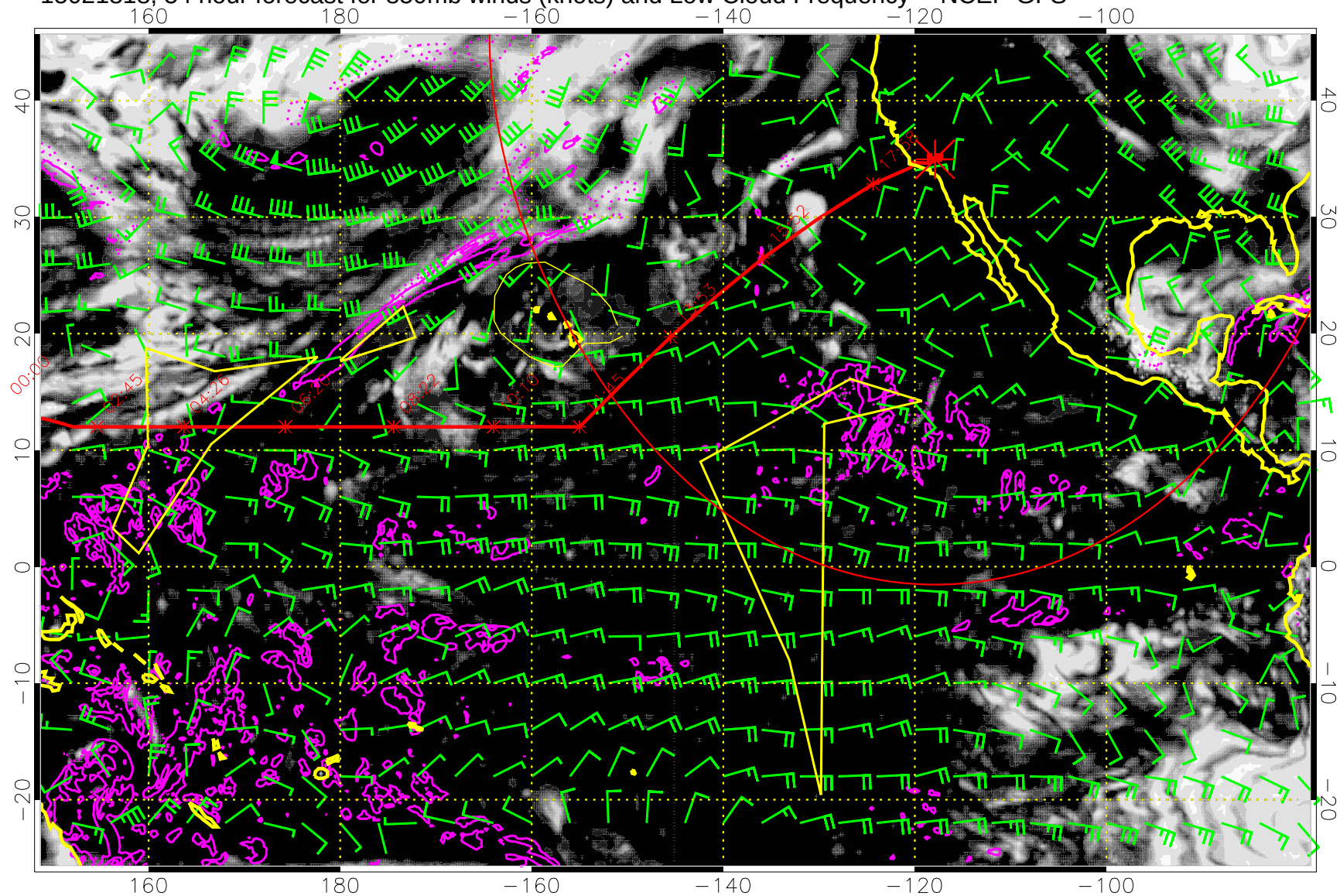
15021818, 54 hour forecast for 850mb winds (knots) and Low Cloud Frequency -- NCEP GFS
