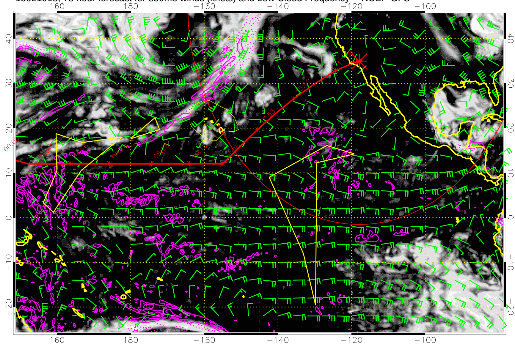
15021918, 78 hour forecast for 850mb winds (knots) and Low Cloud Frequency -- NCEP GFS
