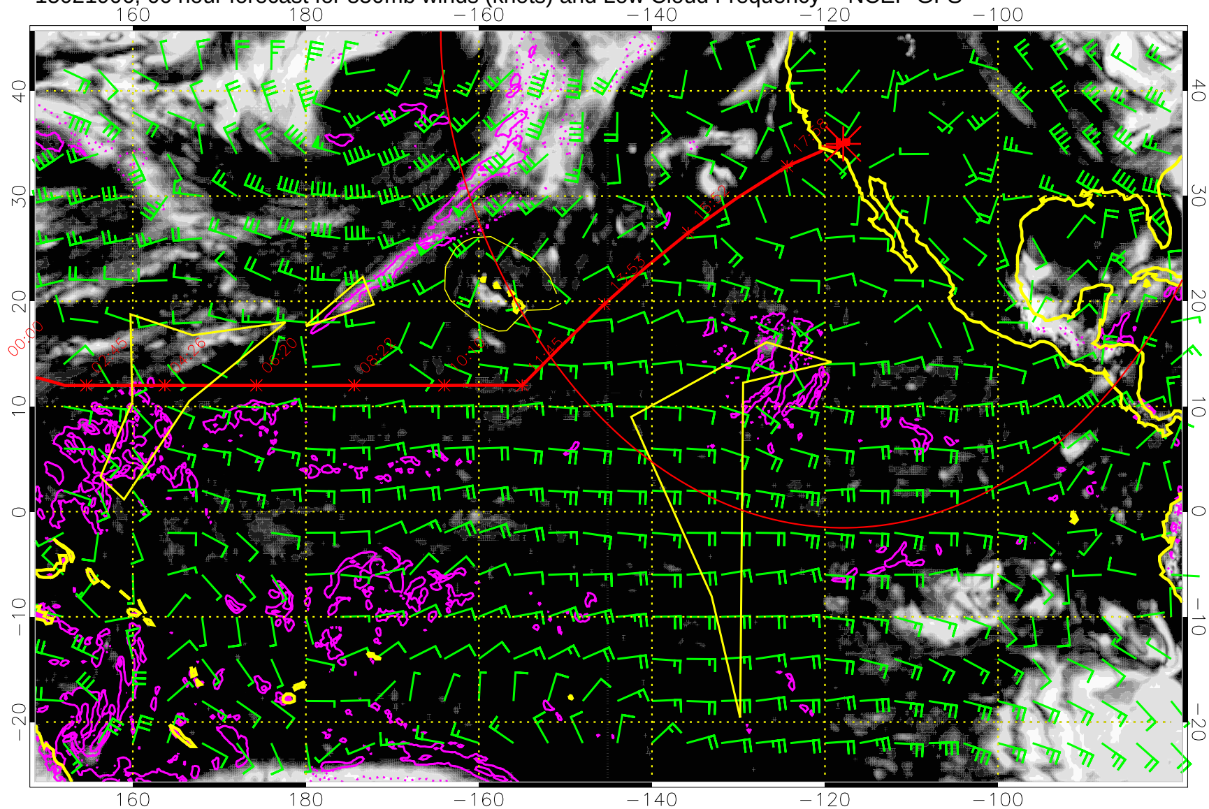
15021906, 66 hour forecast for 850mb winds (knots) and Low Cloud Frequency -- NCEP GFS
