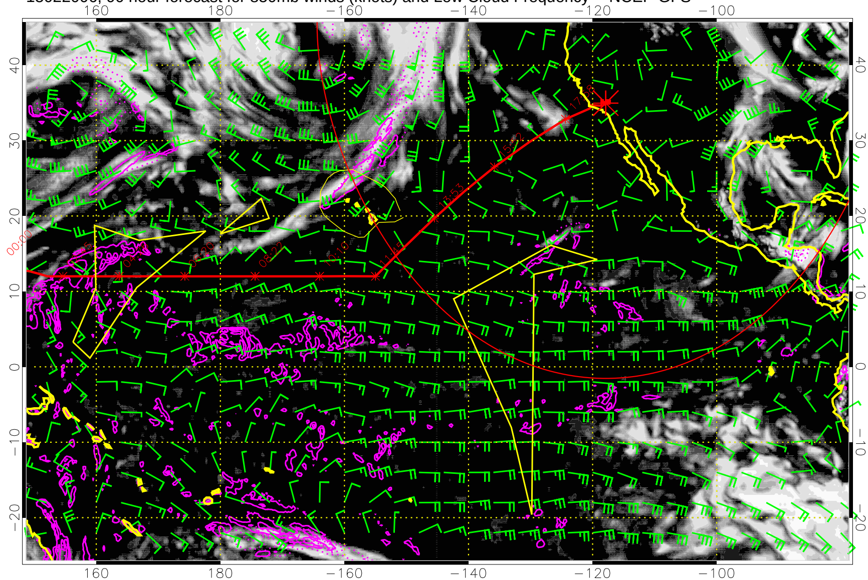
15022006, 90 hour forecast for 850mb winds (knots) and Low Cloud Frequency -- NCEP GFS
