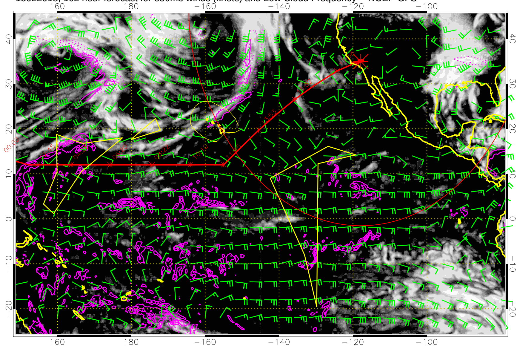
15022018, 102 hour forecast for 850mb winds (knots) and Low Cloud Frequency -- NCEP GFS
