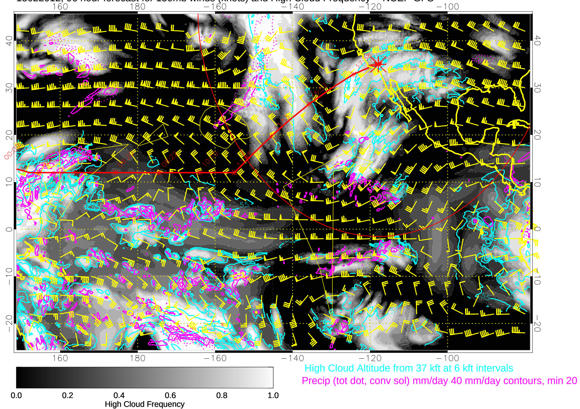
15022012, 96 hour forecast for 150mb winds (knots) and High Cloud Frequency -- NCEP GFS
