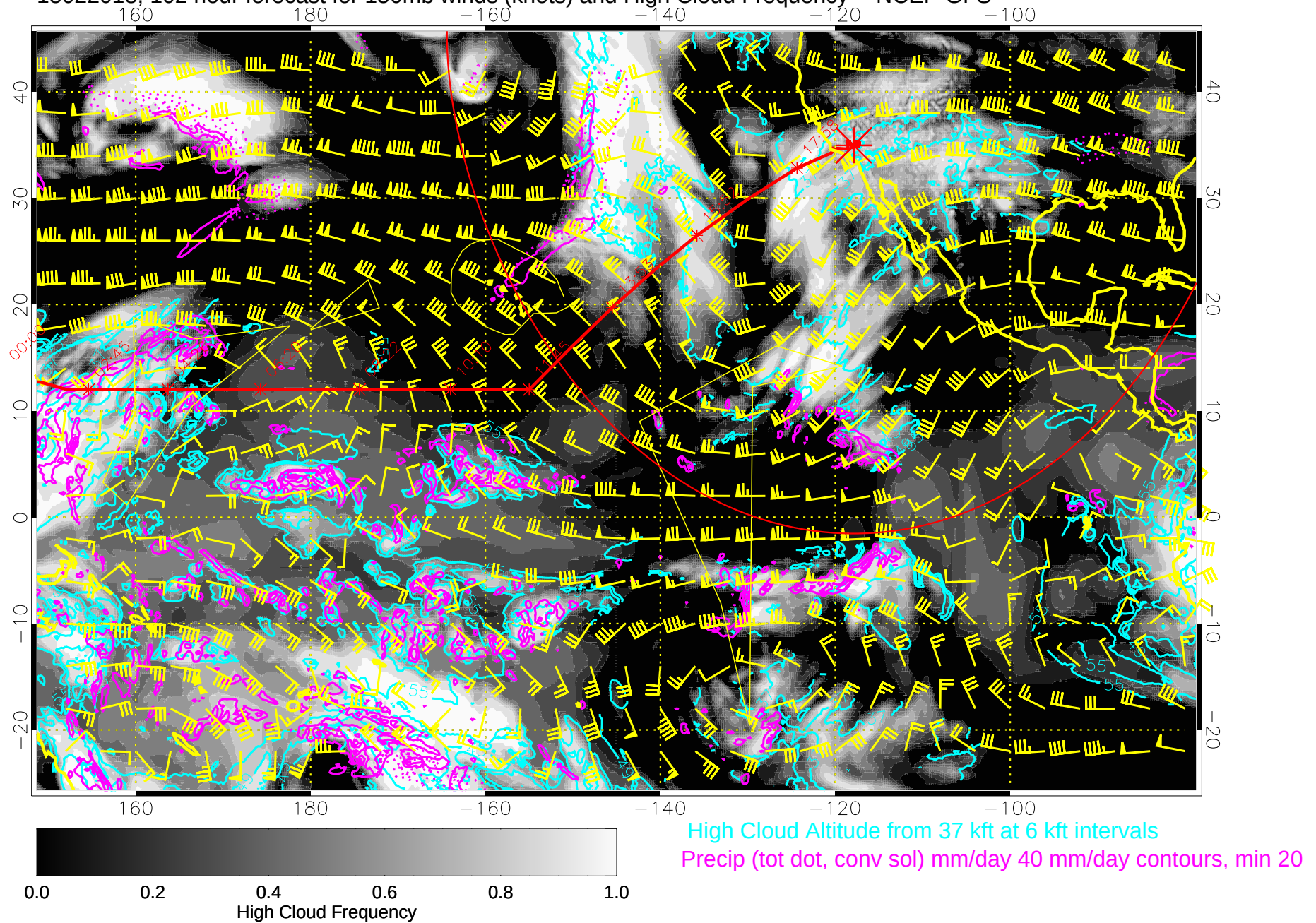
15022018, 102 hour forecast for 150mb winds (knots) and High Cloud Frequency -- NCEP GFS
