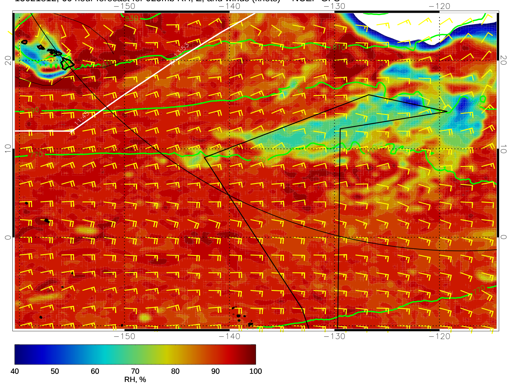
15021812, 60 hour forecast for 925mb RH, Z, and winds (knots) -- NCEP GFS
