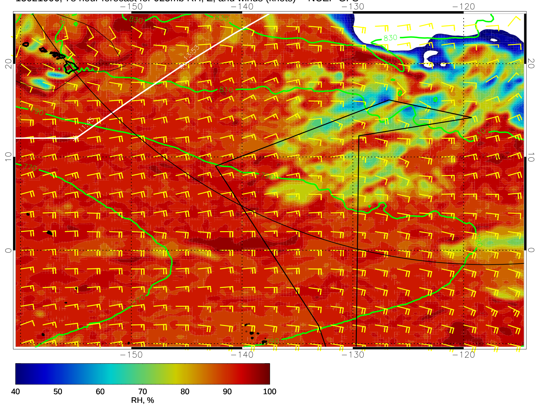
15021906, 78 hour forecast for 925mb RH, Z, and winds (knots) -- NCEP GFS
