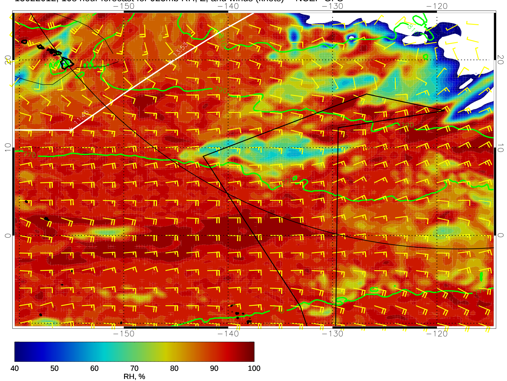
15022012, 108 hour forecast for 925mb RH, Z, and winds (knots) -- NCEP GFS
