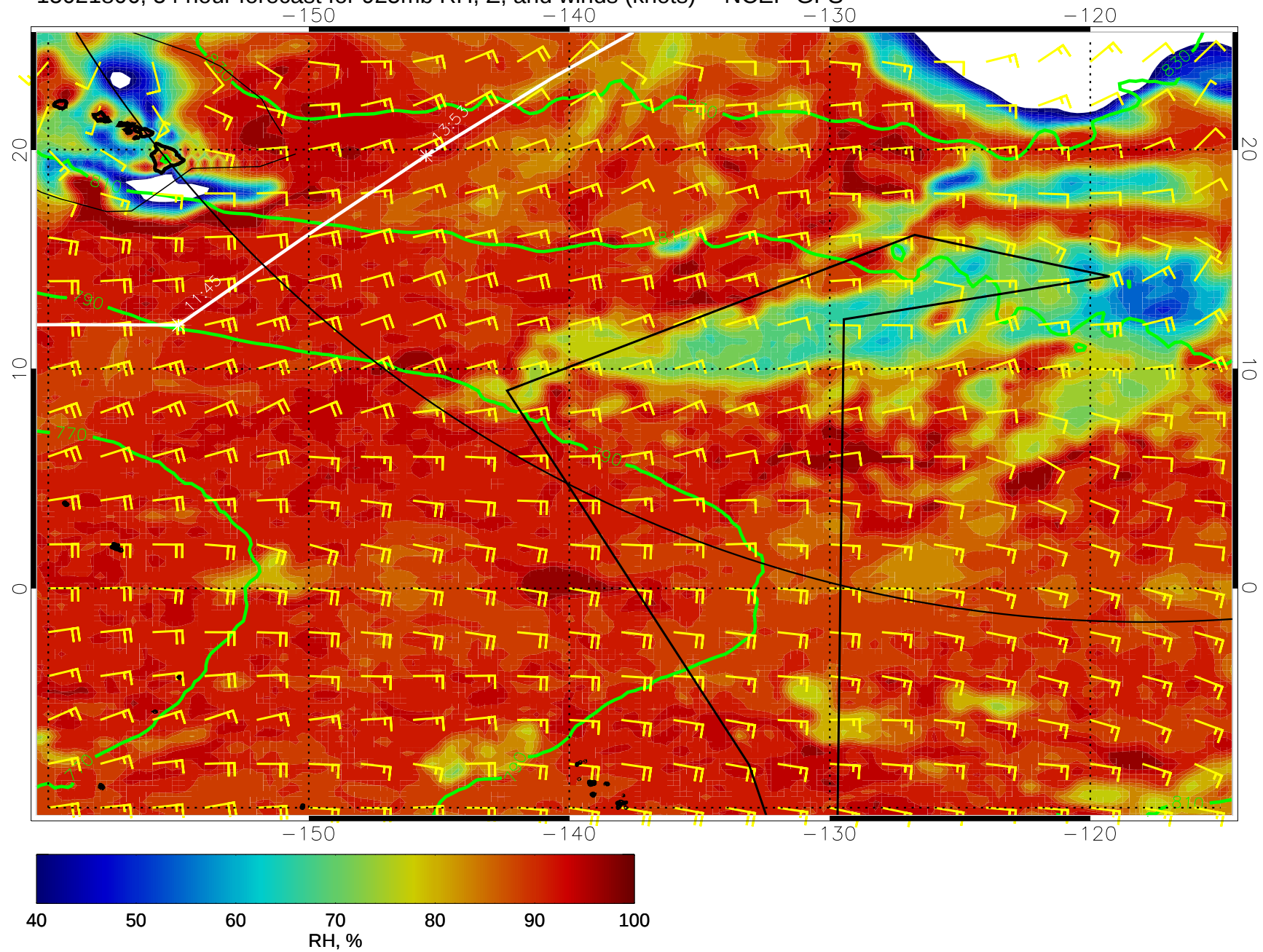
15021806, 54 hour forecast for 925mb RH, Z, and winds (knots) -- NCEP GFS
