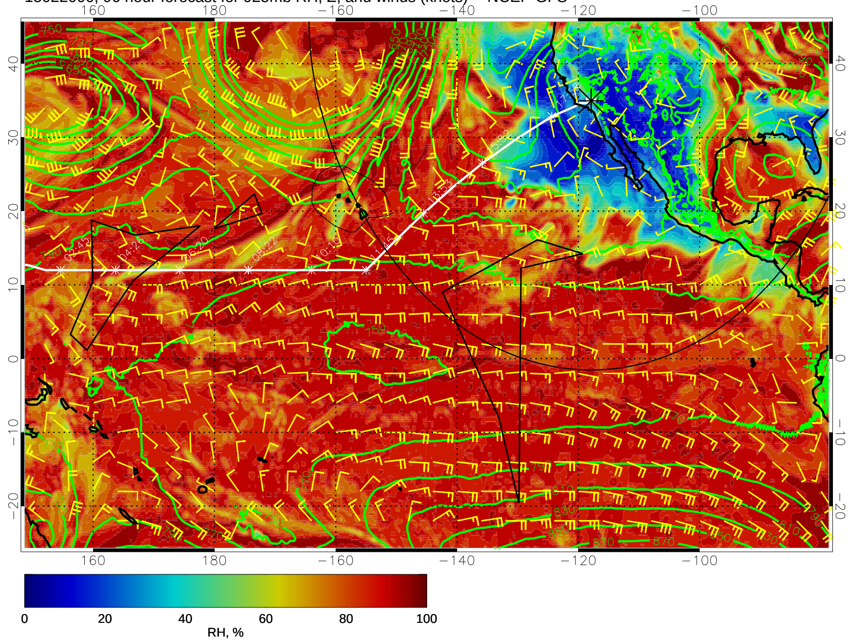
15022000, 96 hour forecast for 925mb RH, Z, and winds (knots) -- NCEP GFS
