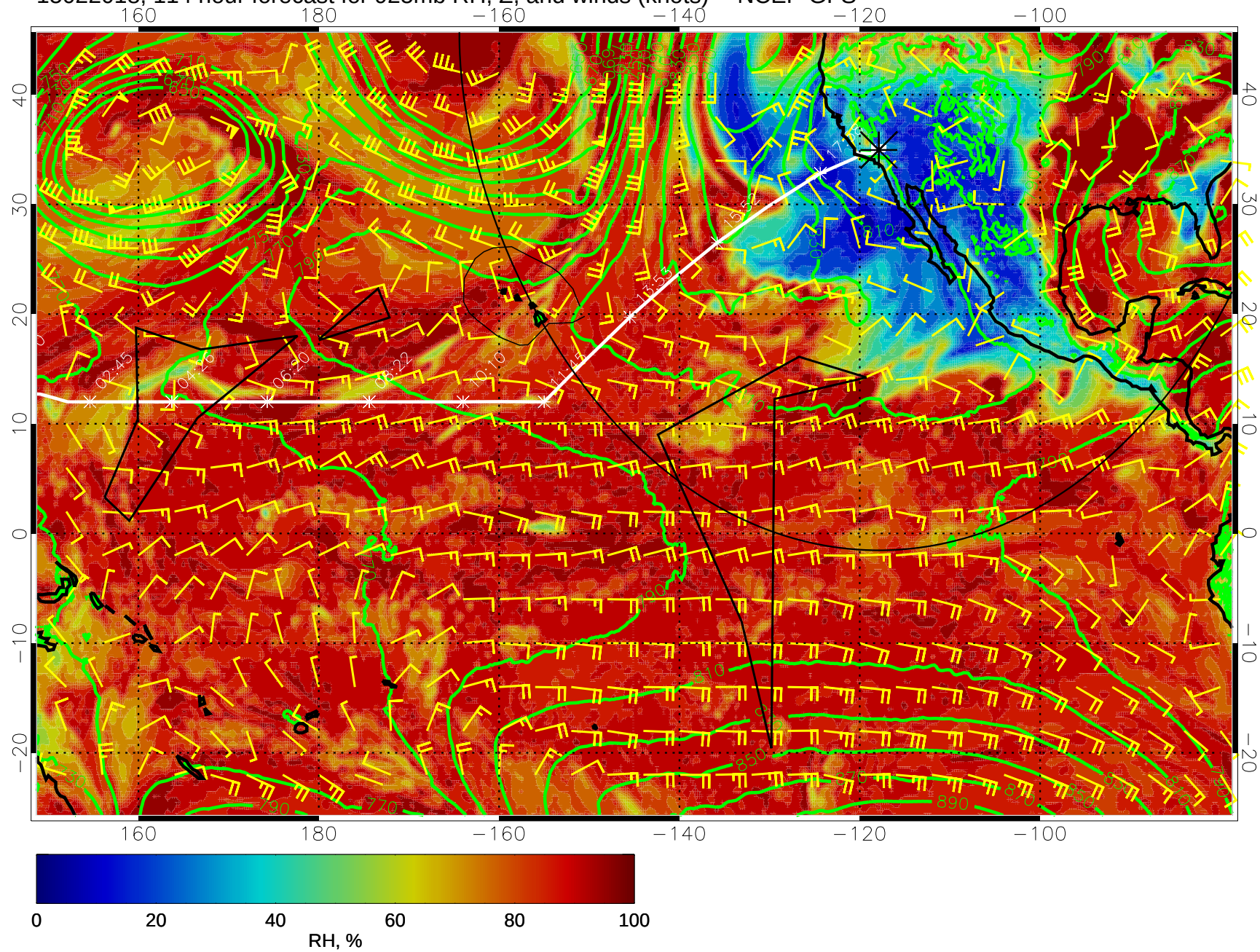
15022018, 114 hour forecast for 925mb RH, Z, and winds (knots) -- NCEP GFS
