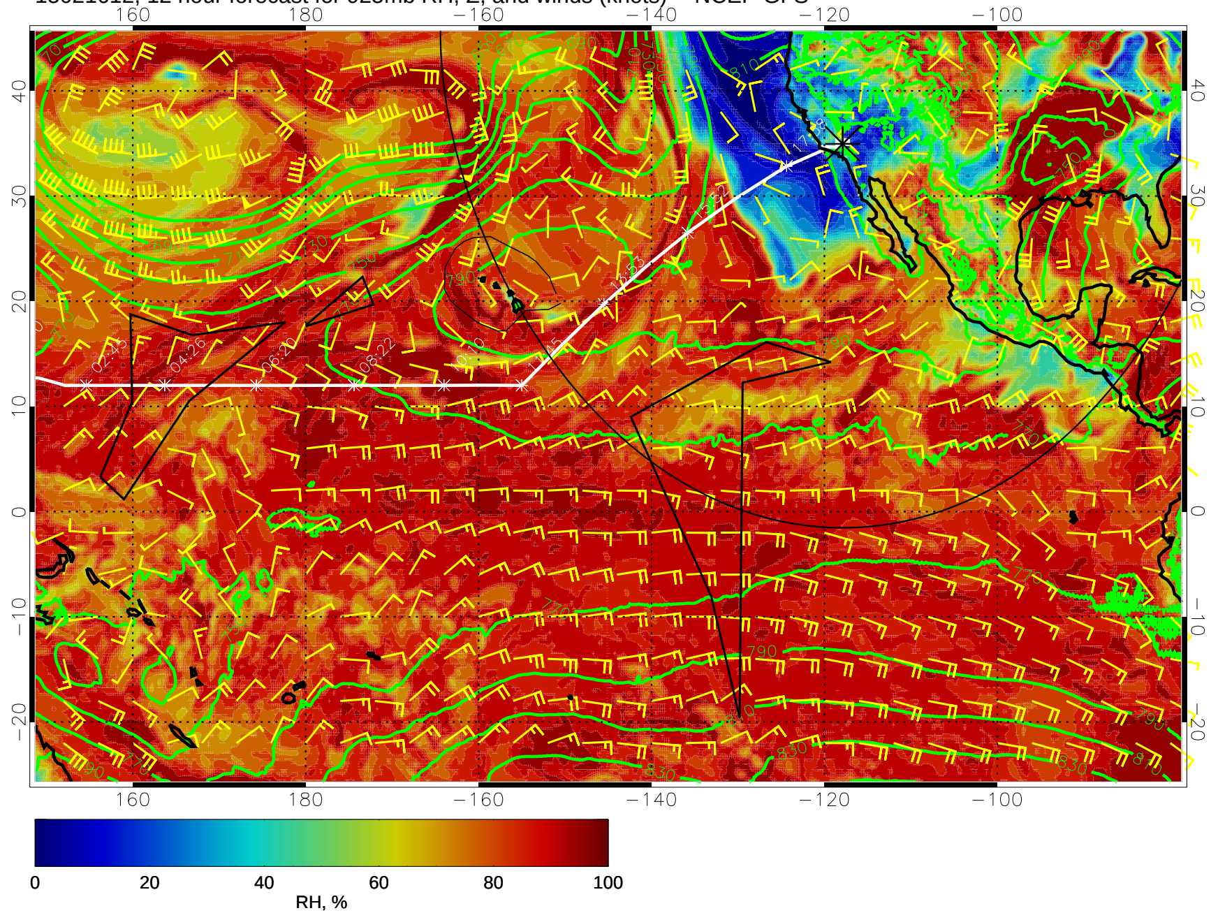
15021612, 12 hour forecast for 925mb RH, Z, and winds (knots) -- NCEP GFS
