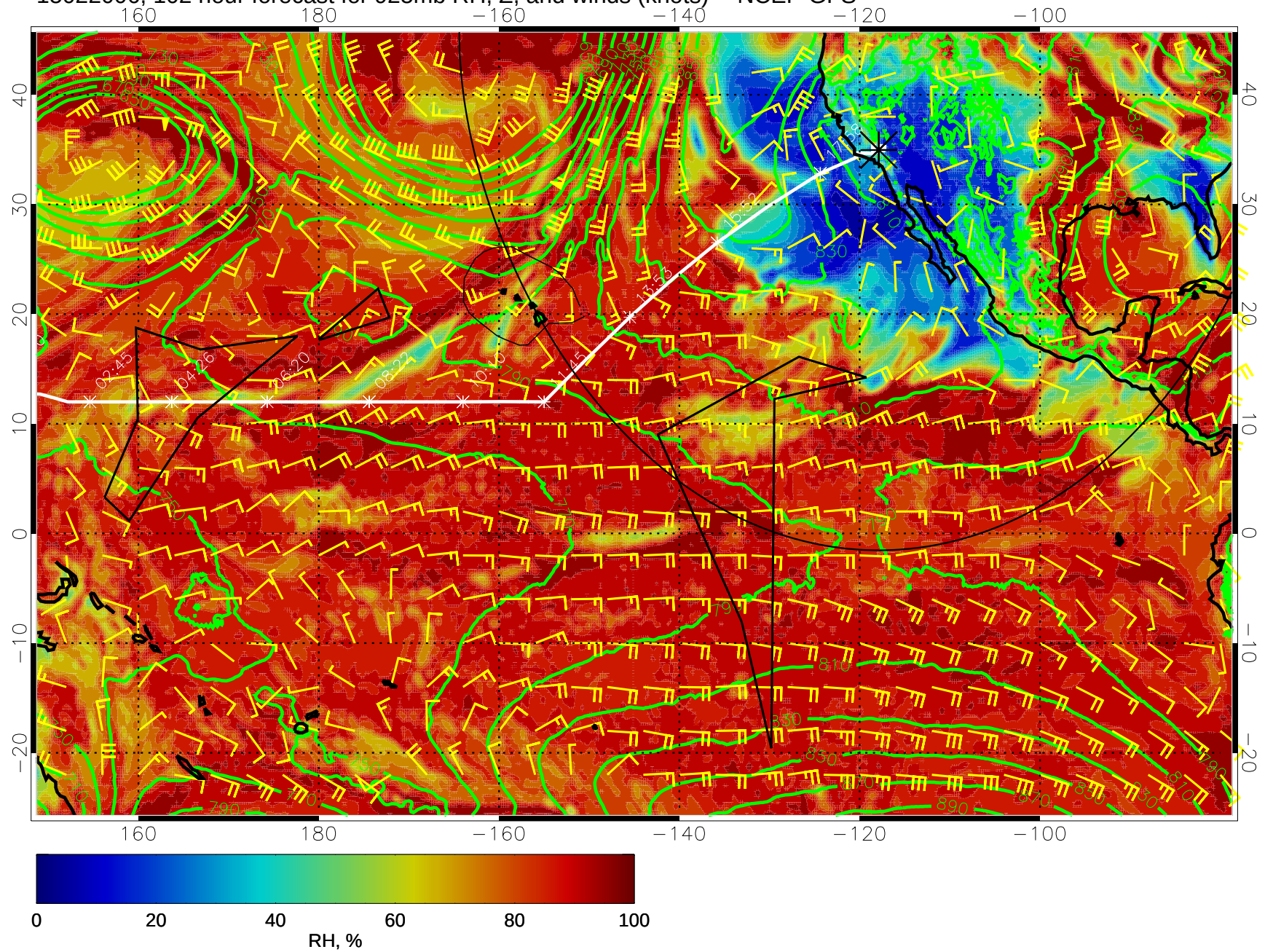
15022006, 102 hour forecast for 925mb RH, Z, and winds (knots) -- NCEP GFS
