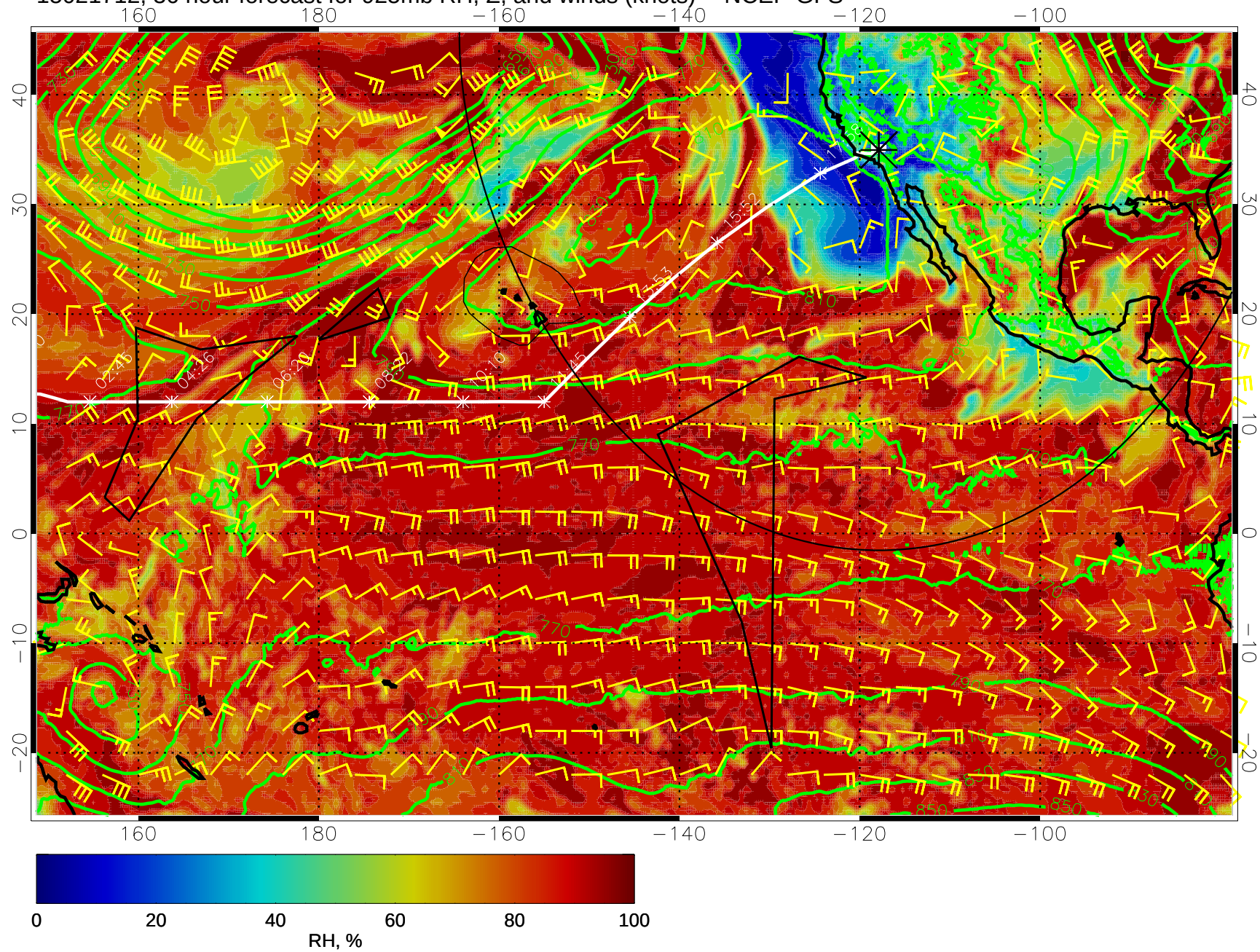
15021712, 36 hour forecast for 925mb RH, Z, and winds (knots) -- NCEP GFS
