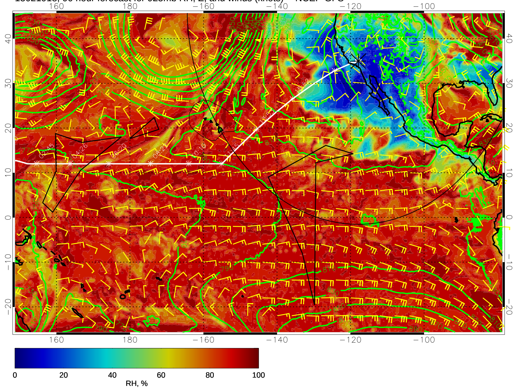
15021918, 90 hour forecast for 925mb RH, Z, and winds (knots) -- NCEP GFS
