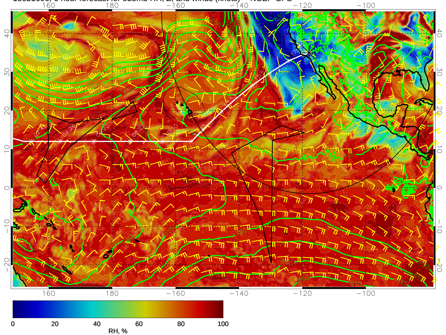
15021606, 6 hour forecast for 925mb RH, Z, and winds (knots) -- NCEP GFS
