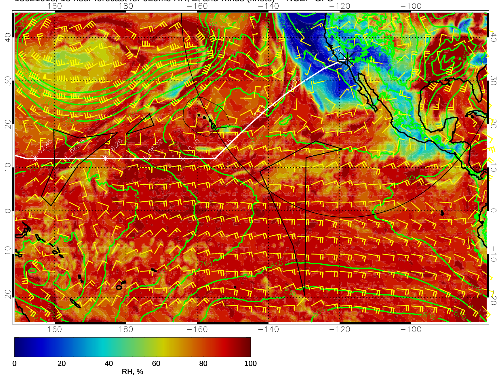
15021618, 18 hour forecast for 925mb RH, Z, and winds (knots) -- NCEP GFS
