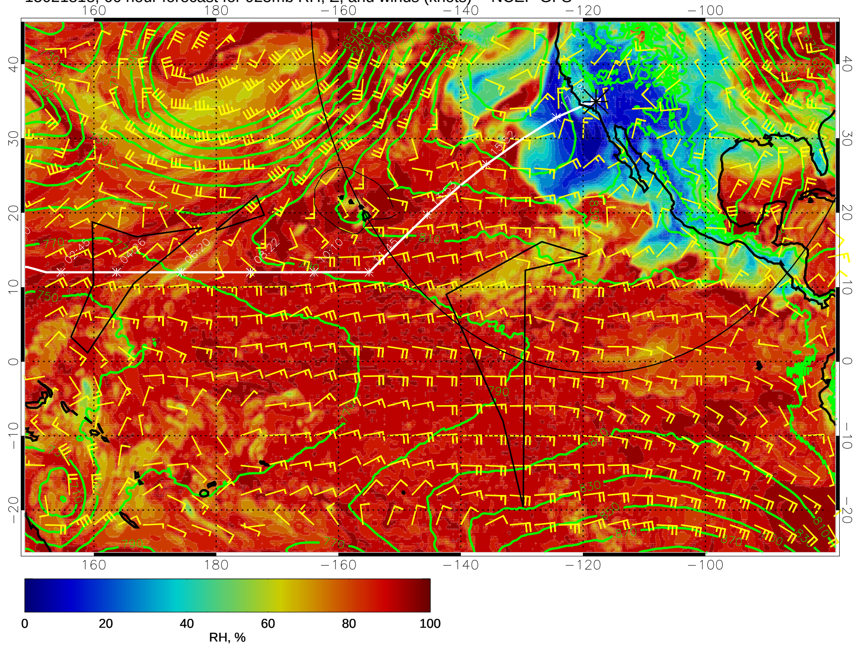
15021818, 66 hour forecast for 925mb RH, Z, and winds (knots) -- NCEP GFS
