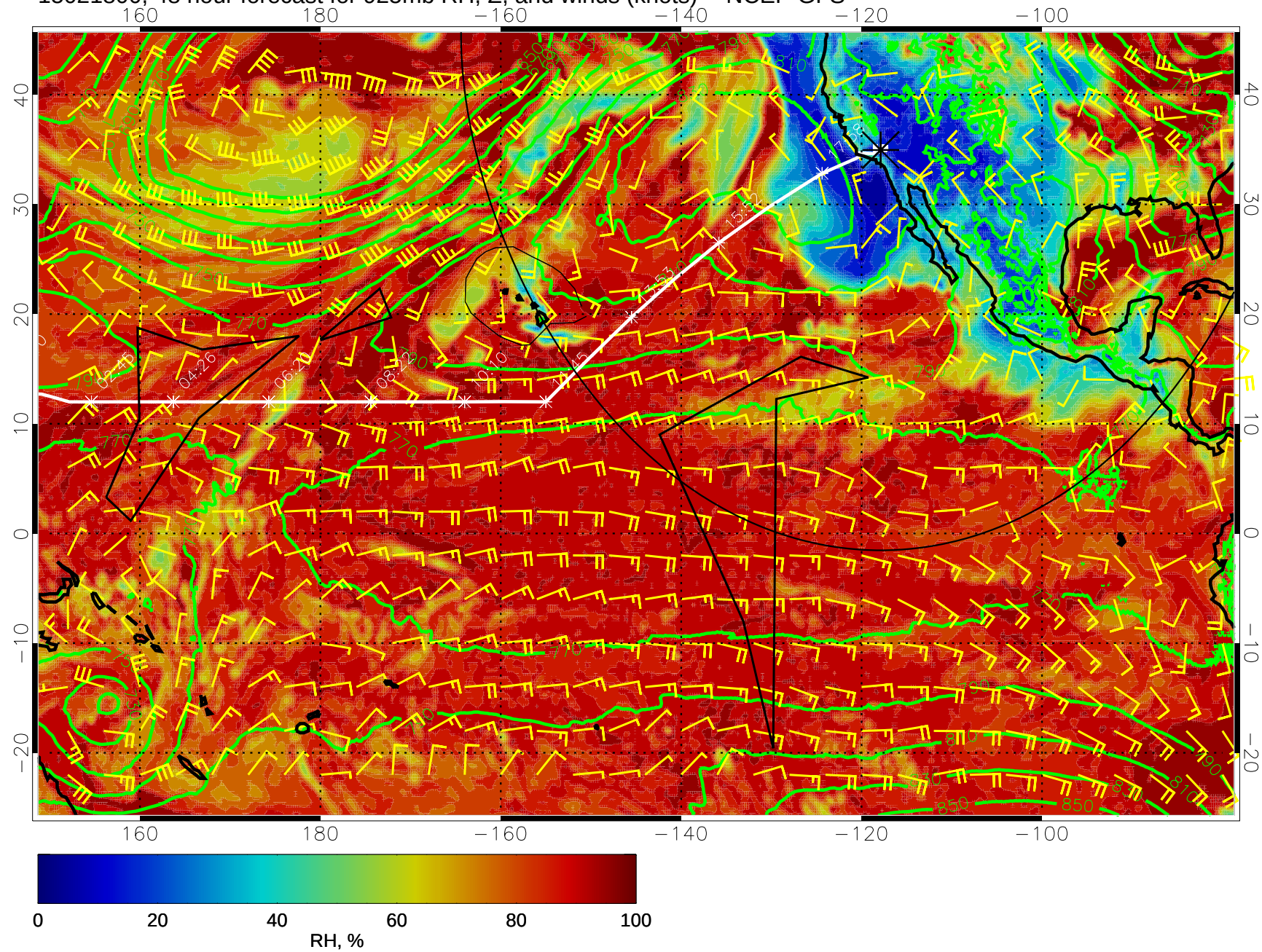
15021800, 48 hour forecast for 925mb RH, Z, and winds (knots) -- NCEP GFS
