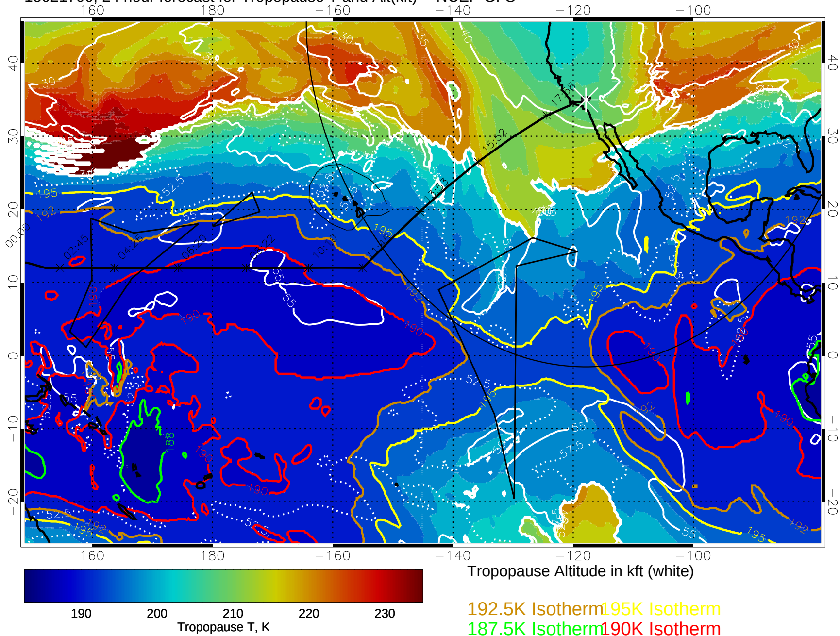
15021700, 24 hour forecast for Tropopause T and Alt(kft) -- NCEP GFS
