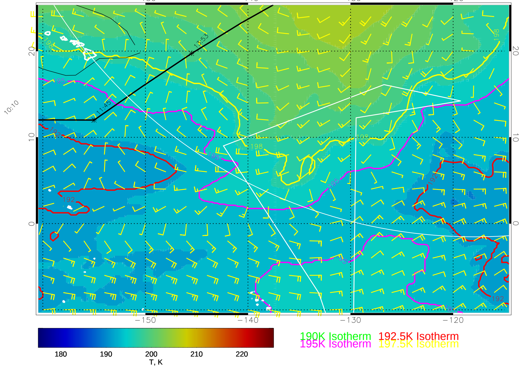
15022012, 108 hour forecast for 70mb T and winds (knots) -- NCEP GFS
