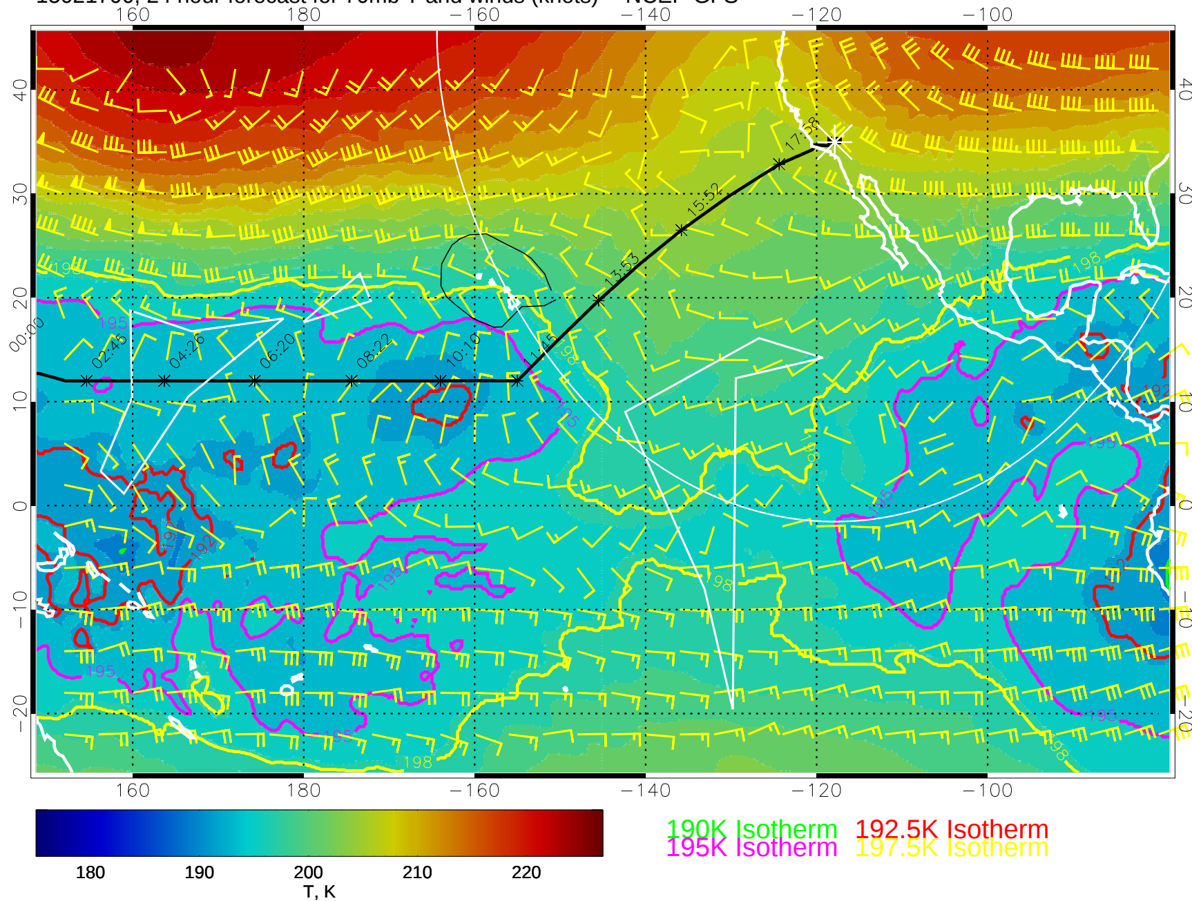
15021700, 24 hour forecast for 70mb T and winds (knots) -- NCEP GFS
