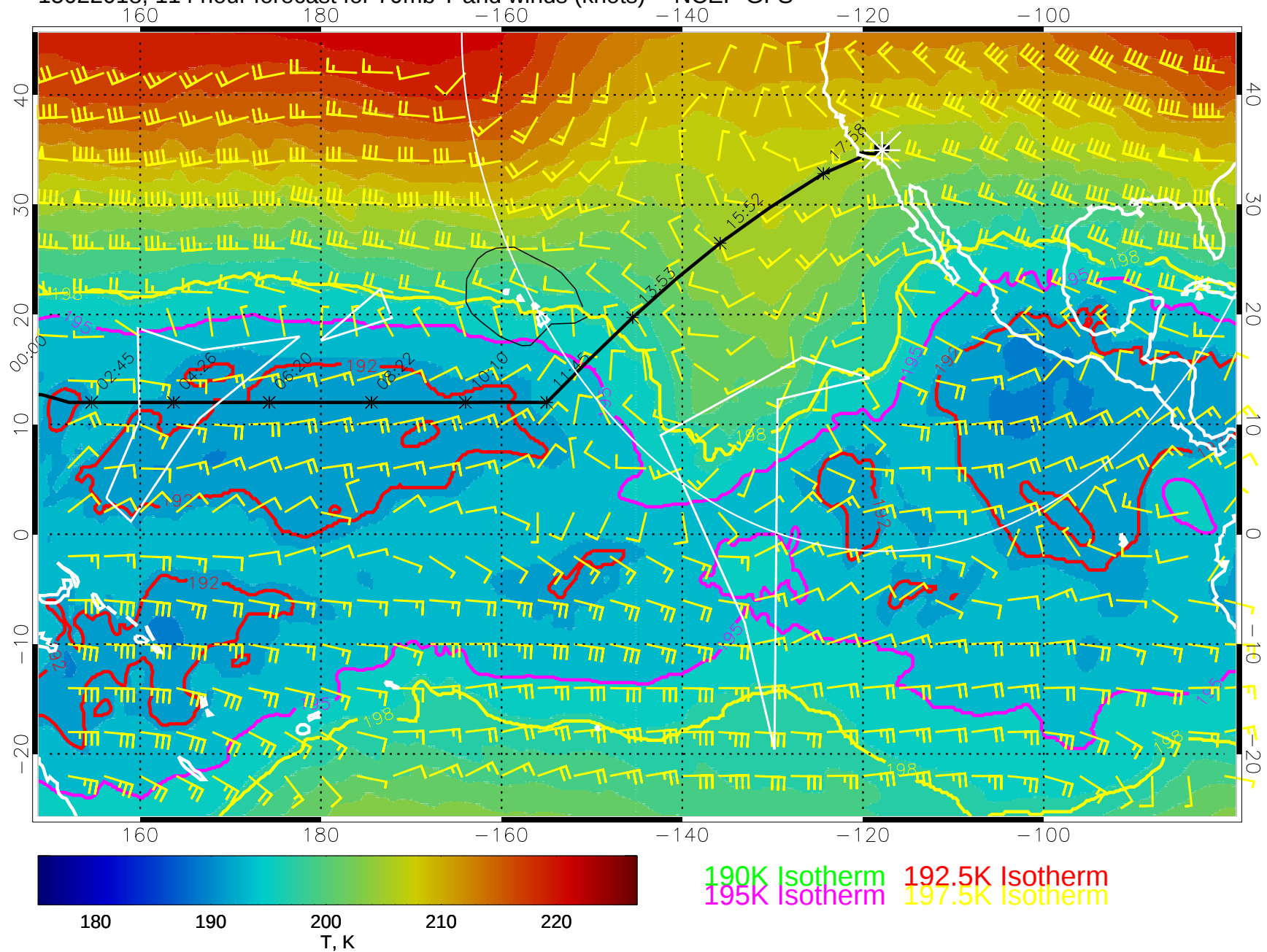
15022018, 114 hour forecast for 70mb T and winds (knots) -- NCEP GFS
