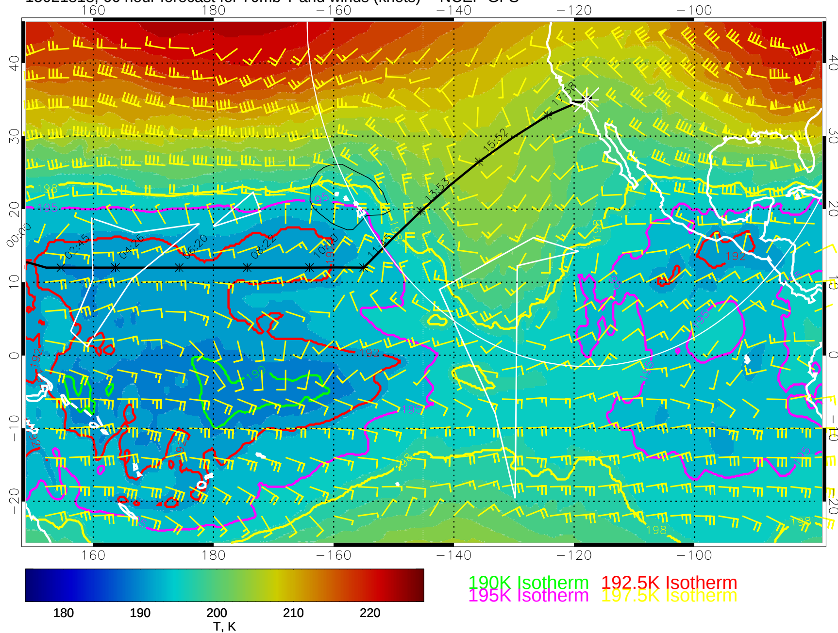
15021818, 66 hour forecast for 70mb T and winds (knots) -- NCEP GFS
