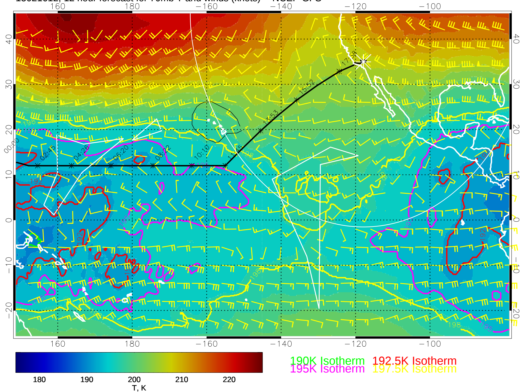
15021612, 12 hour forecast for 70mb T and winds (knots) -- NCEP GFS
