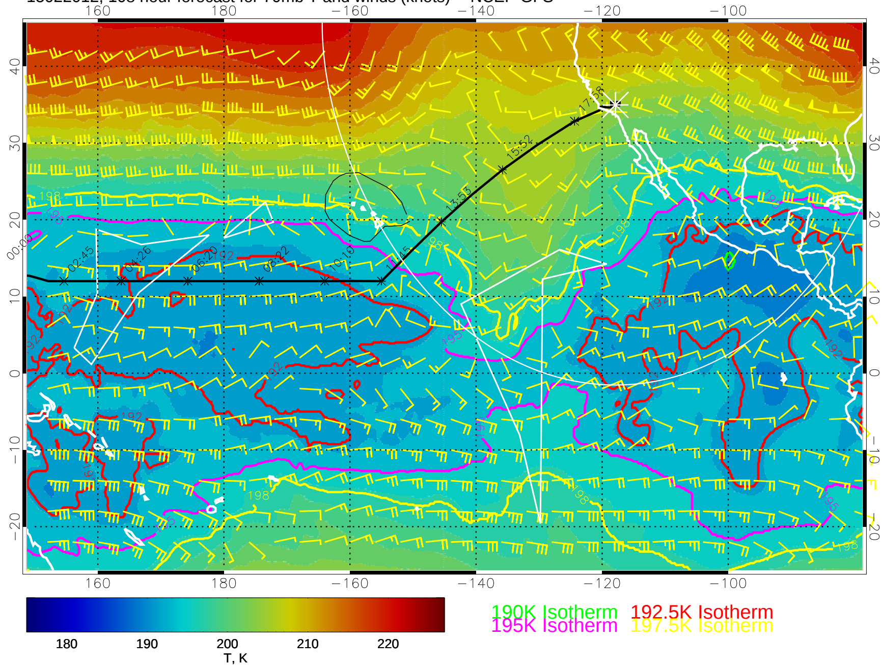
15022012, 108 hour forecast for 70mb T and winds (knots) -- NCEP GFS
