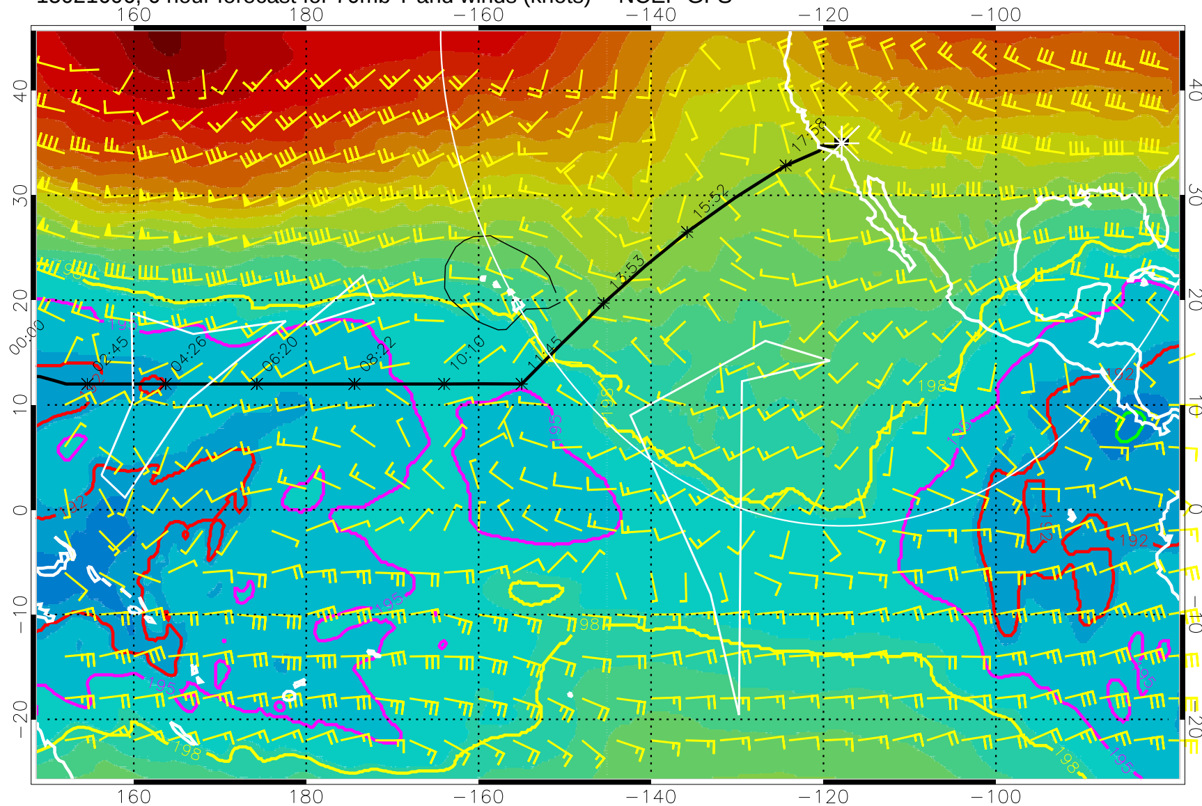
15021606, 6 hour forecast for 70mb T and winds (knots) -- NCEP GFS
