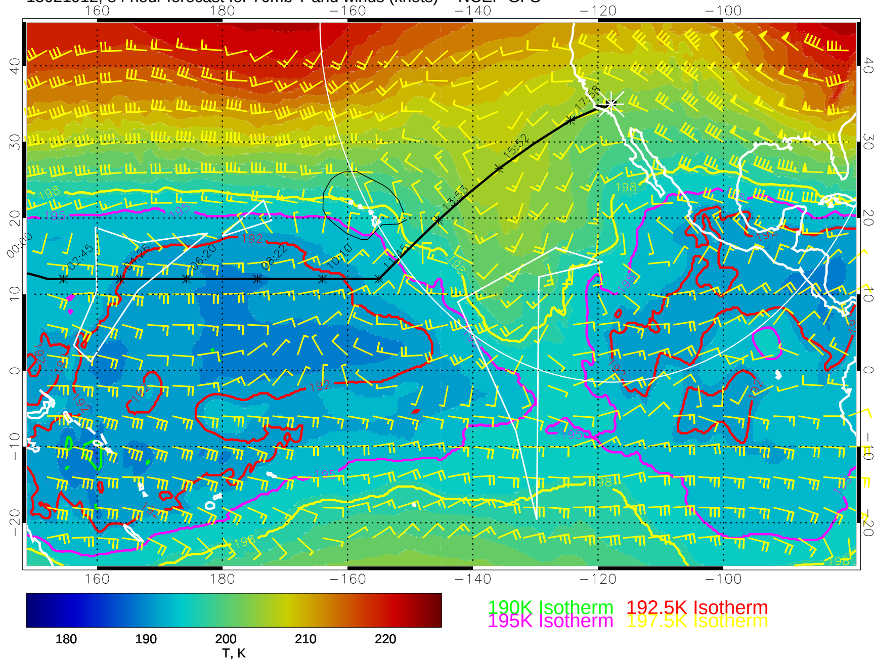
15021912, 84 hour forecast for 70mb T and winds (knots) -- NCEP GFS
