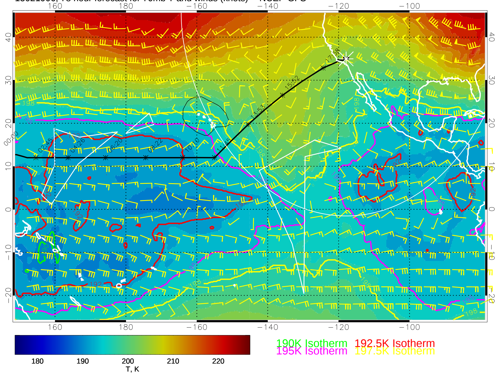
15021906, 78 hour forecast for 70mb T and winds (knots) -- NCEP GFS
