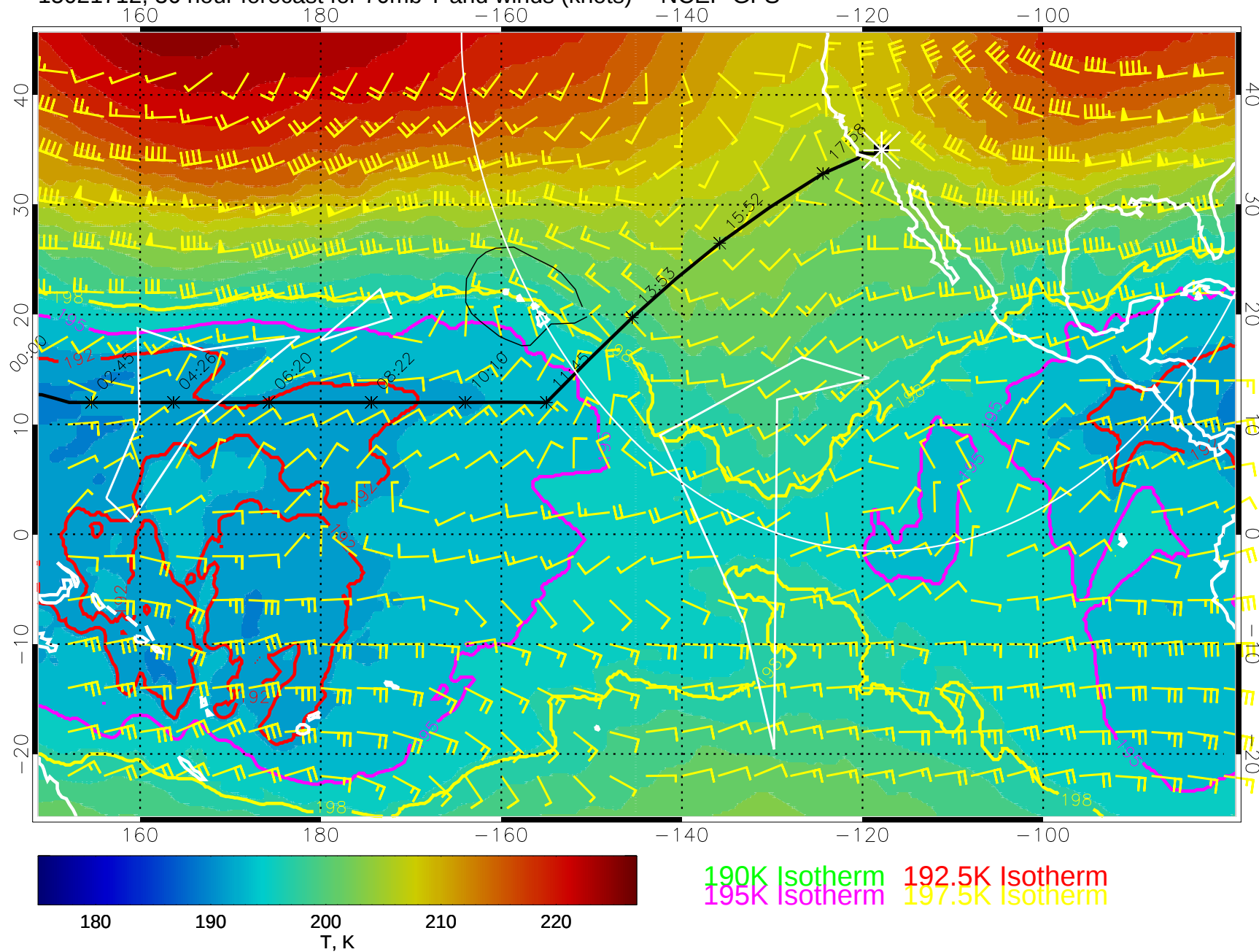
15021712, 36 hour forecast for 70mb T and winds (knots) -- NCEP GFS
