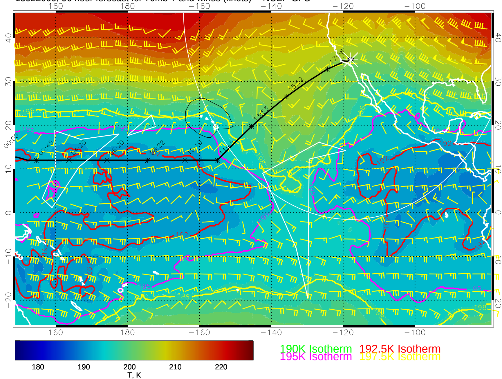
15022000, 96 hour forecast for 70mb T and winds (knots) -- NCEP GFS
