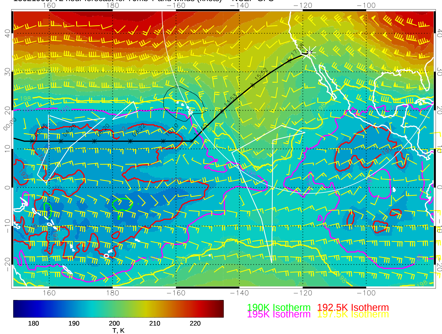
15021900, 72 hour forecast for 70mb T and winds (knots) -- NCEP GFS
