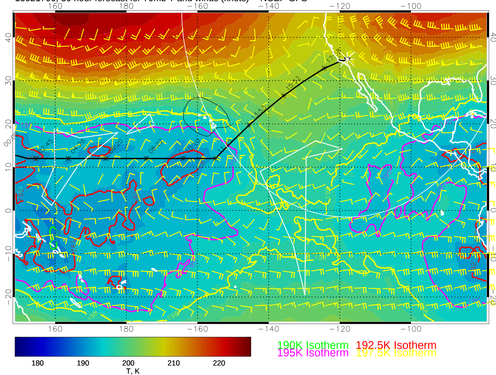
15021706, 30 hour forecast for 70mb T and winds (knots) -- NCEP GFS
