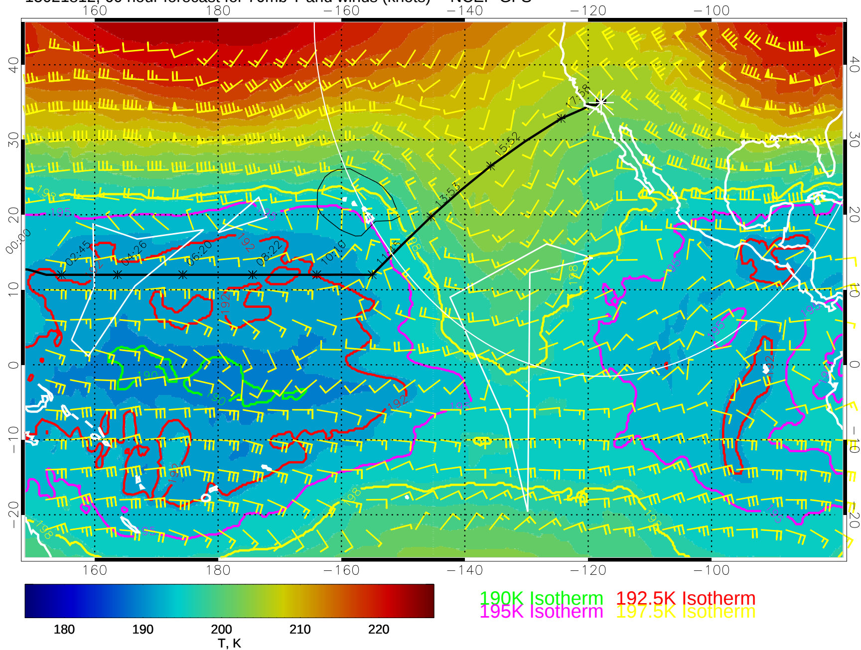
15021812, 60 hour forecast for 70mb T and winds (knots) -- NCEP GFS
