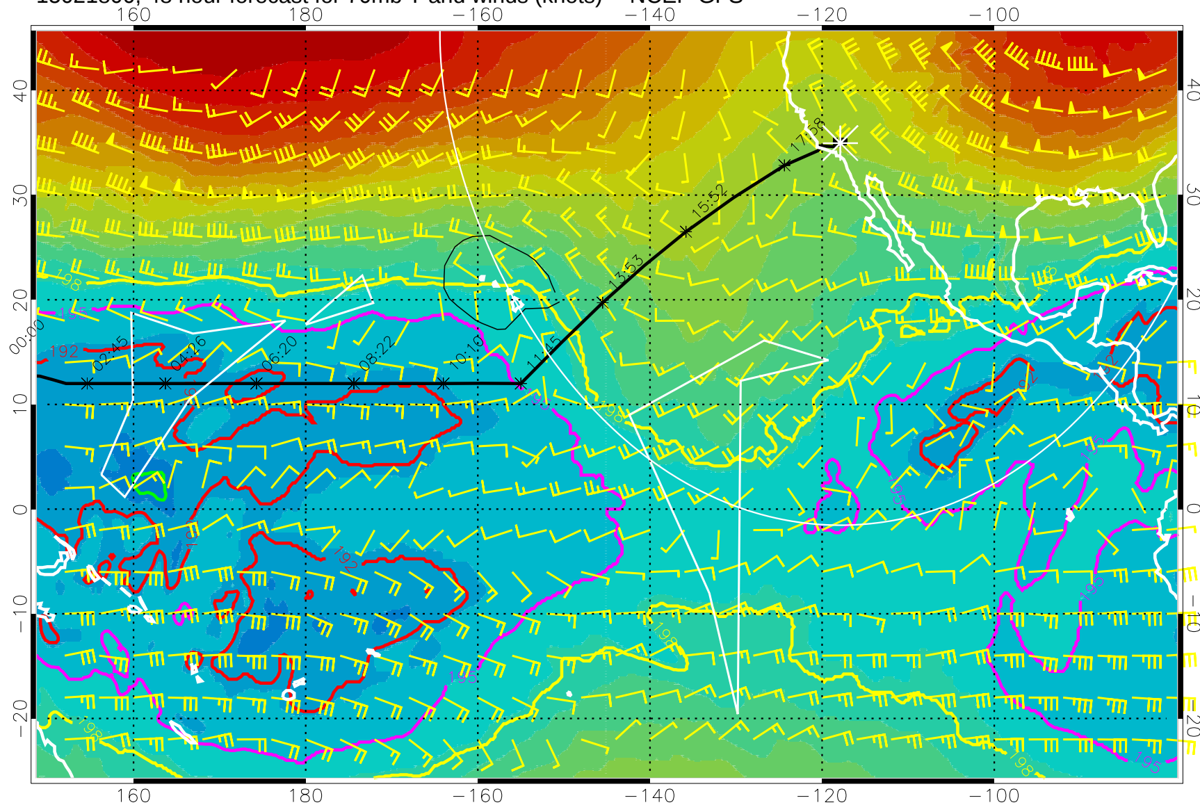
15021800, 48 hour forecast for 70mb T and winds (knots) -- NCEP GFS
