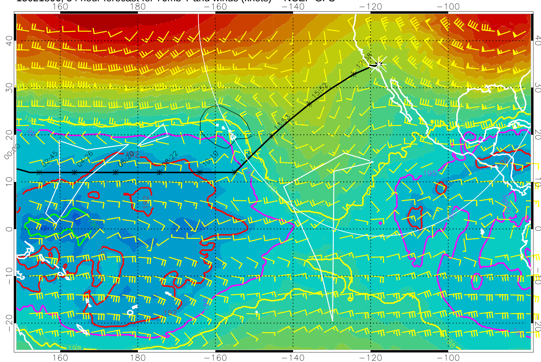
15021806, 54 hour forecast for 70mb T and winds (knots) -- NCEP GFS
