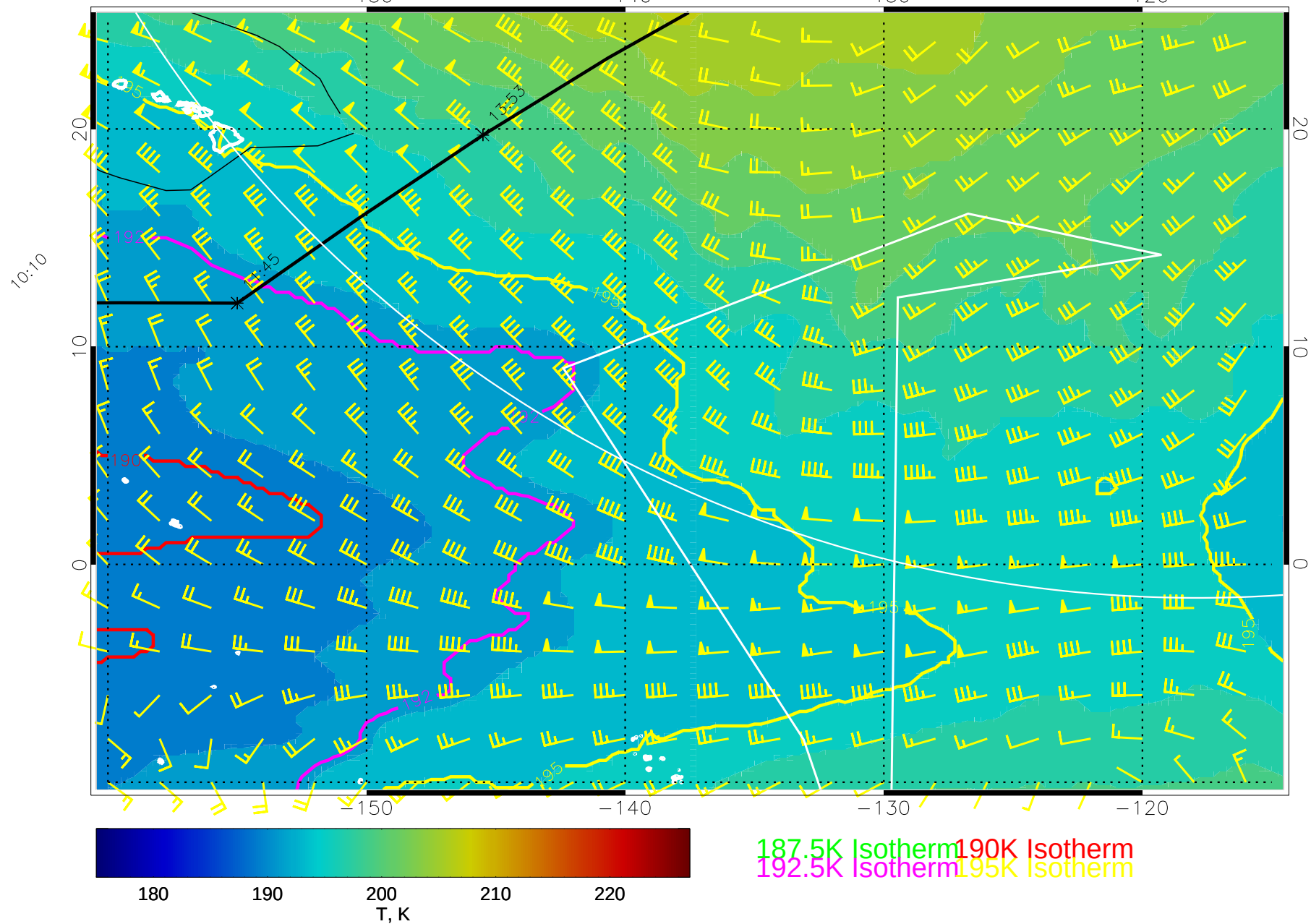
15021712, 36 hour forecast for 100mb T and winds (knots) -- NCEP GFS
