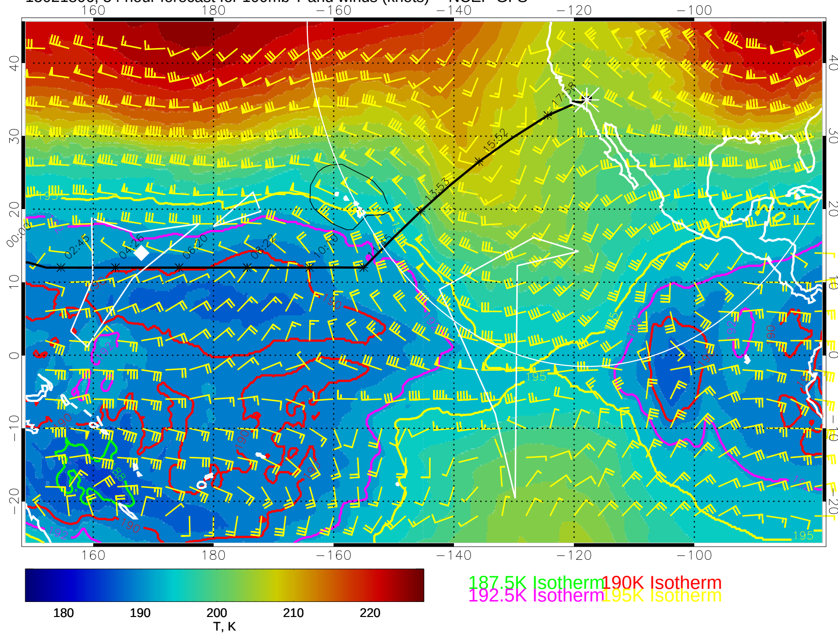
15021806, 54 hour forecast for 100mb T and winds (knots) -- NCEP GFS
