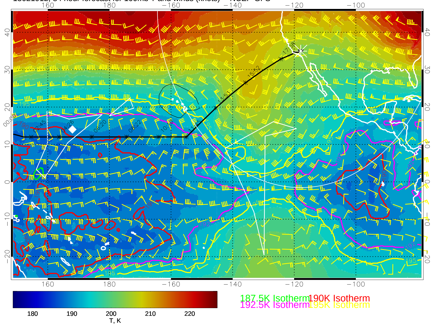
15021912, 84 hour forecast for 100mb T and winds (knots) -- NCEP GFS
