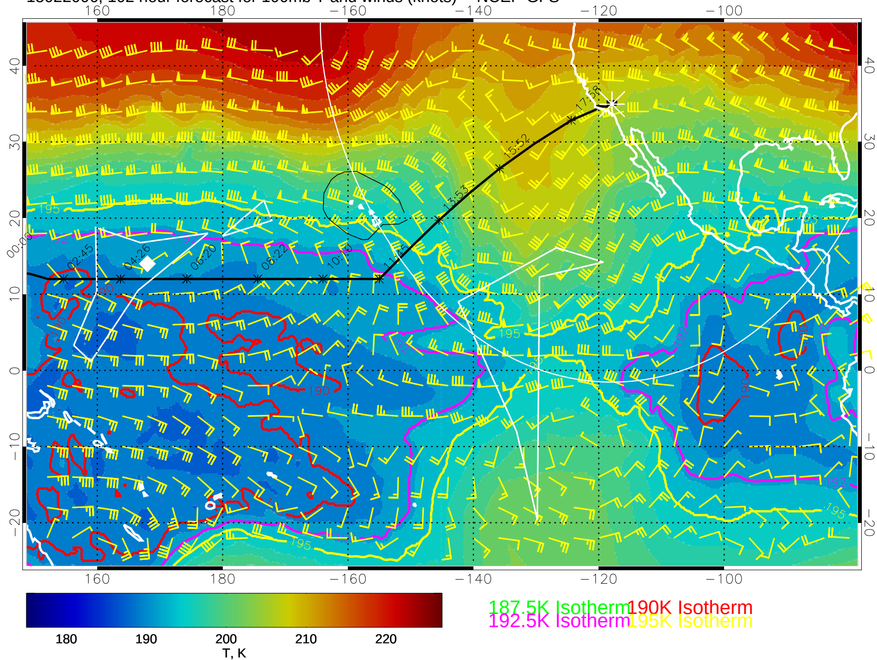
15022006, 102 hour forecast for 100mb T and winds (knots) -- NCEP GFS
