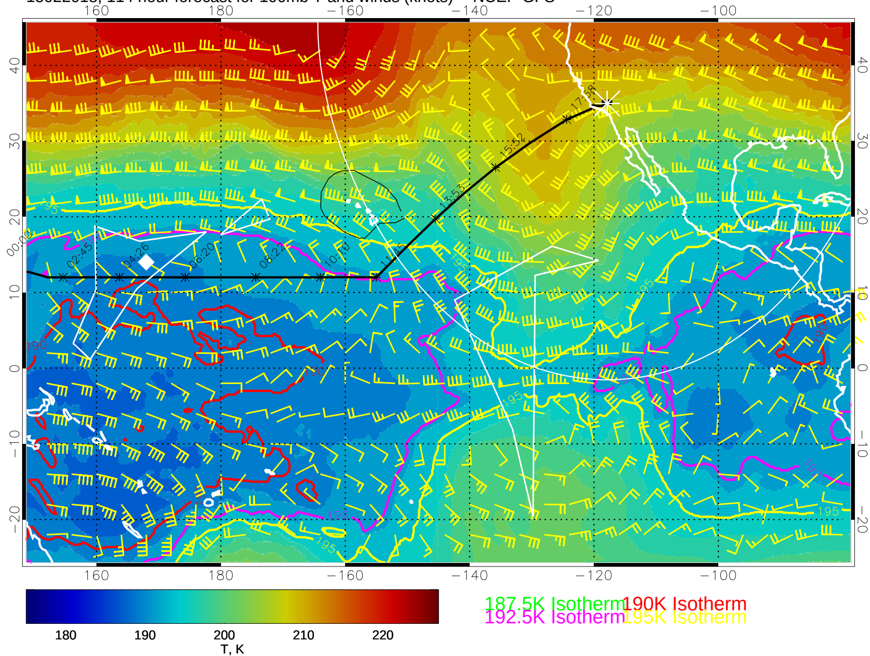
15022018, 114 hour forecast for 100mb T and winds (knots) -- NCEP GFS
