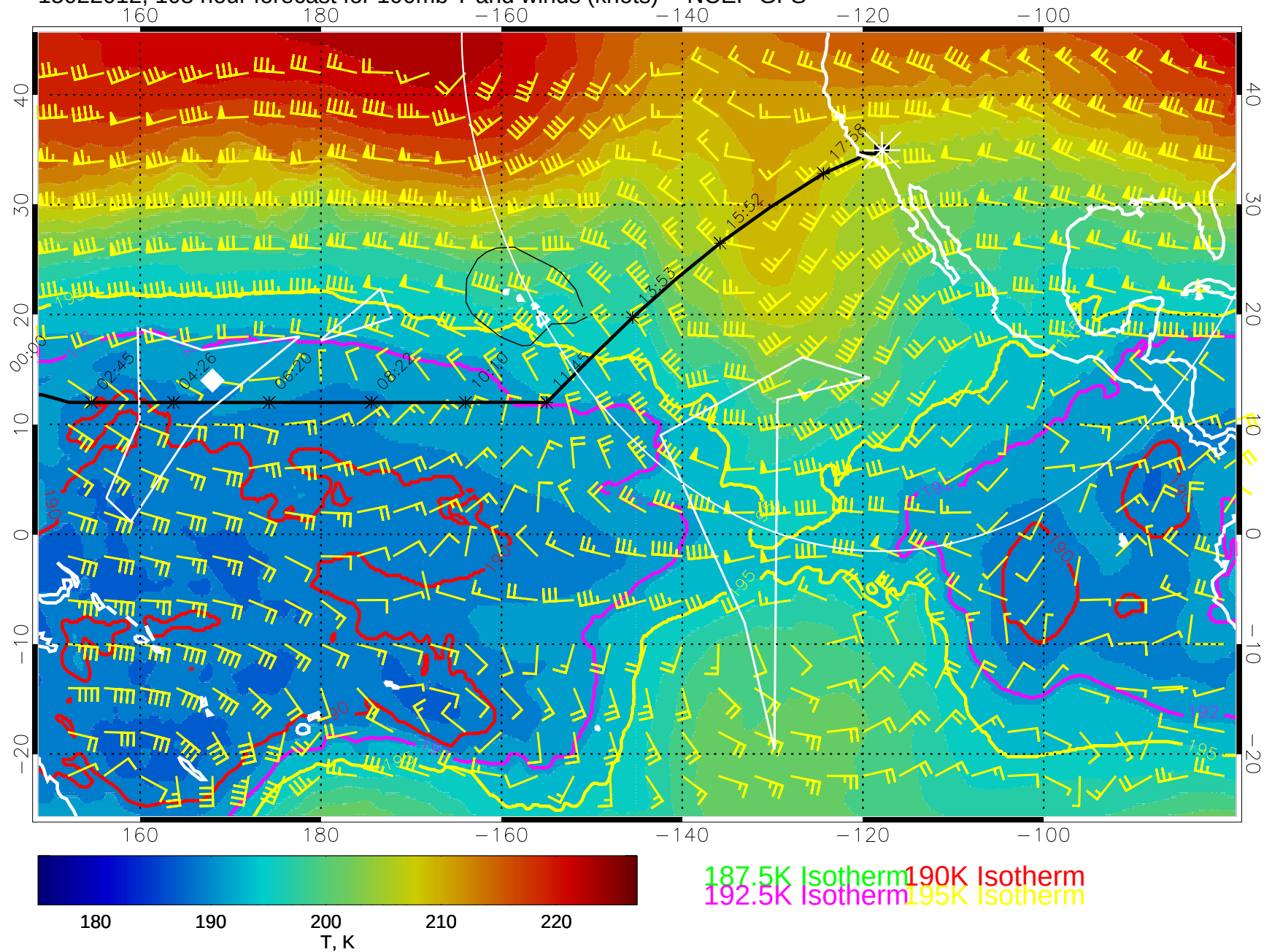
15022012, 108 hour forecast for 100mb T and winds (knots) -- NCEP GFS
