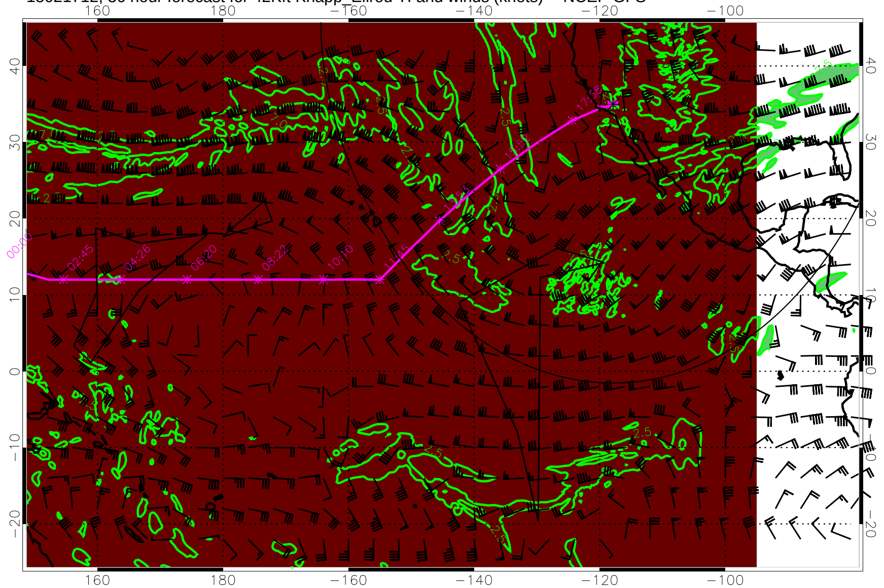
15021712, 36 hour forecast for 42Kft Knapp_Ellrod TI and winds (knots) -- NCEP GFS
