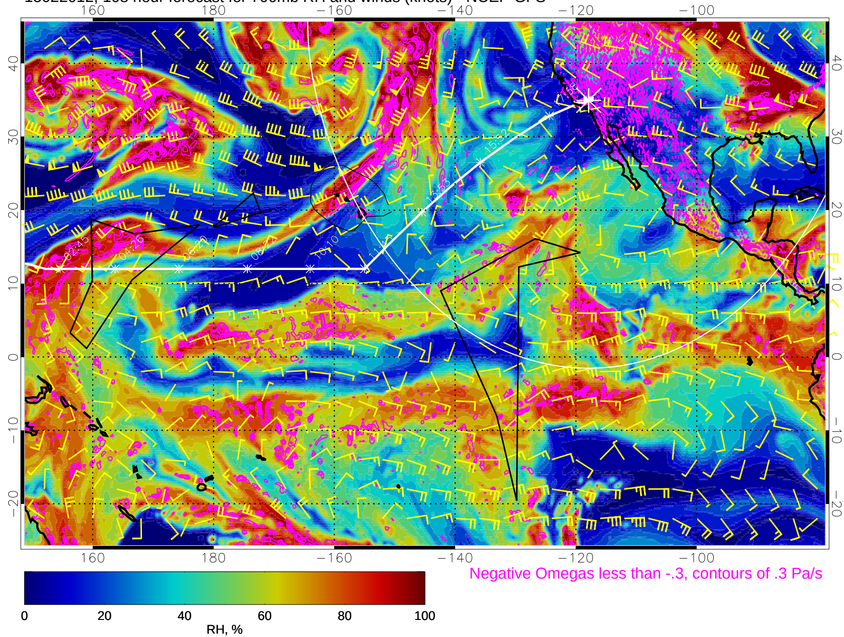
15022012, 108 hour forecast for 700mb RH and winds (knots) - NCEP GFS
