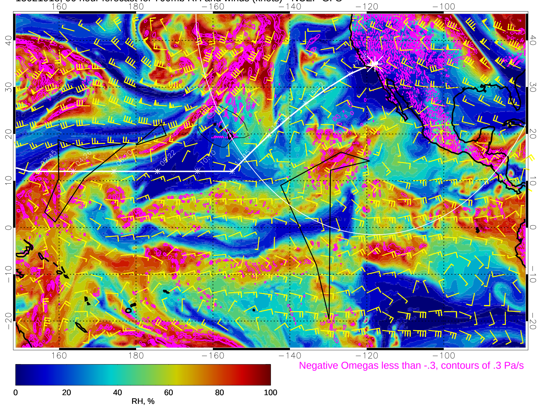
15021918, 90 hour forecast for 700mb RH and winds (knots) - NCEP GFS
