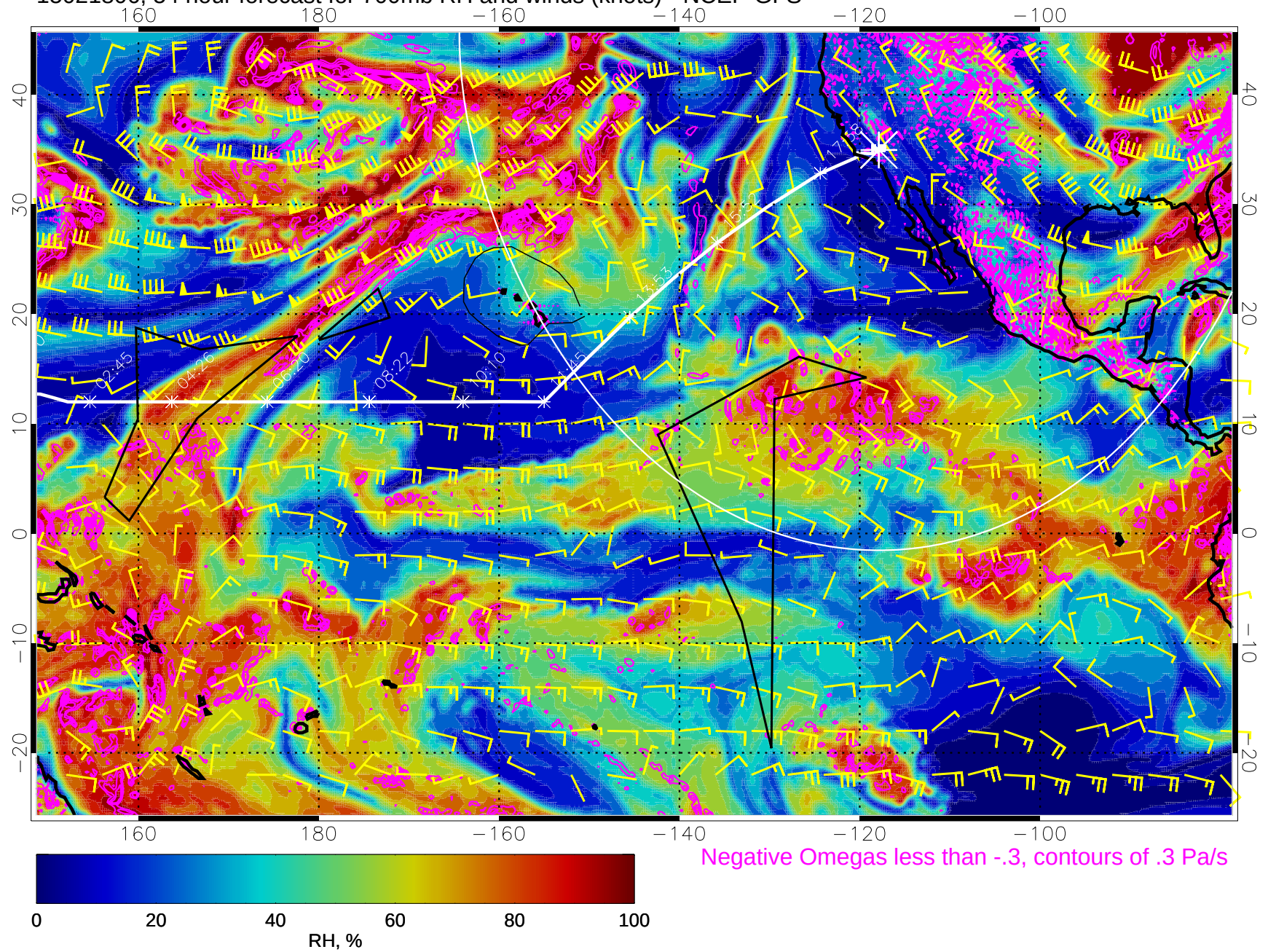
15021806, 54 hour forecast for 700mb RH and winds (knots) - NCEP GFS
