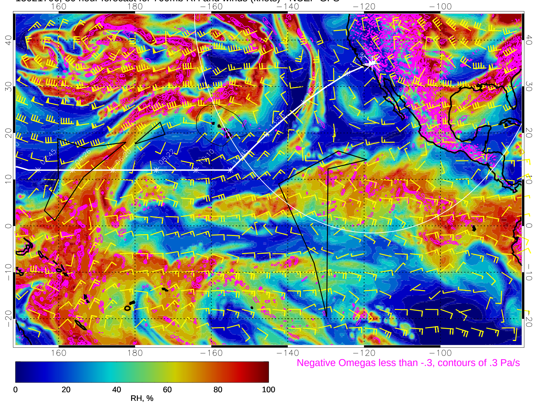
15021706, 30 hour forecast for 700mb RH and winds (knots) - NCEP GFS
