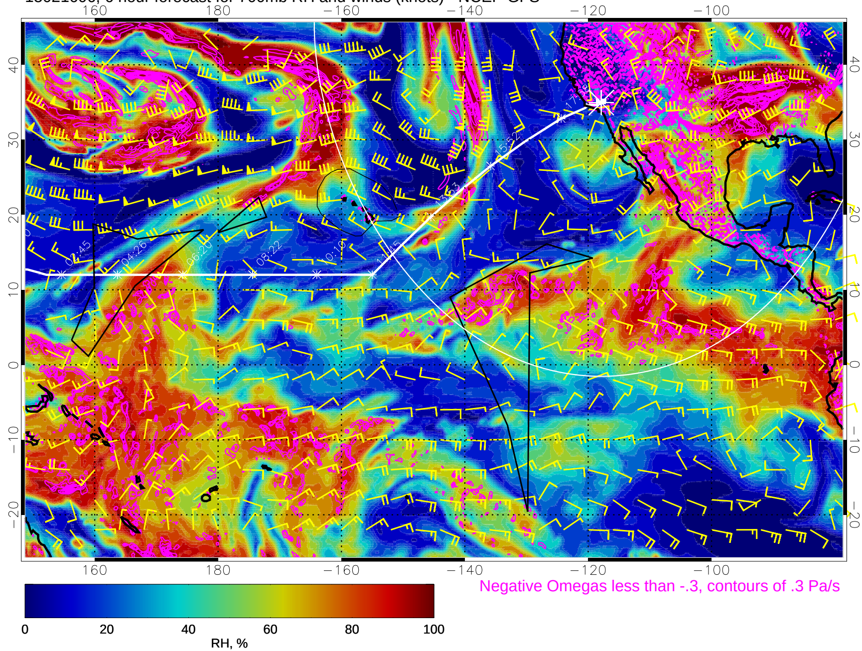
15021606, 6 hour forecast for 700mb RH and winds (knots) - NCEP GFS
