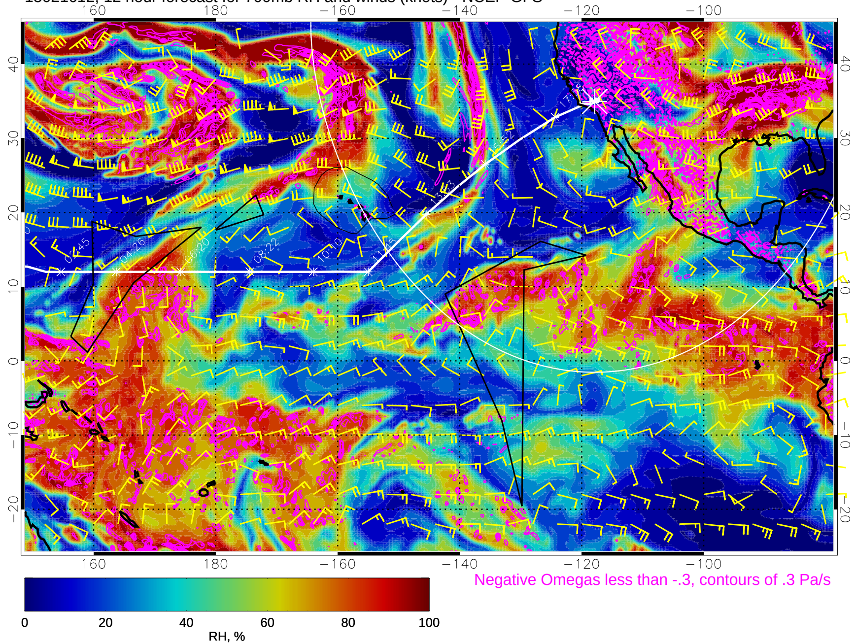
15021612, 12 hour forecast for 700mb RH and winds (knots) - NCEP GFS
