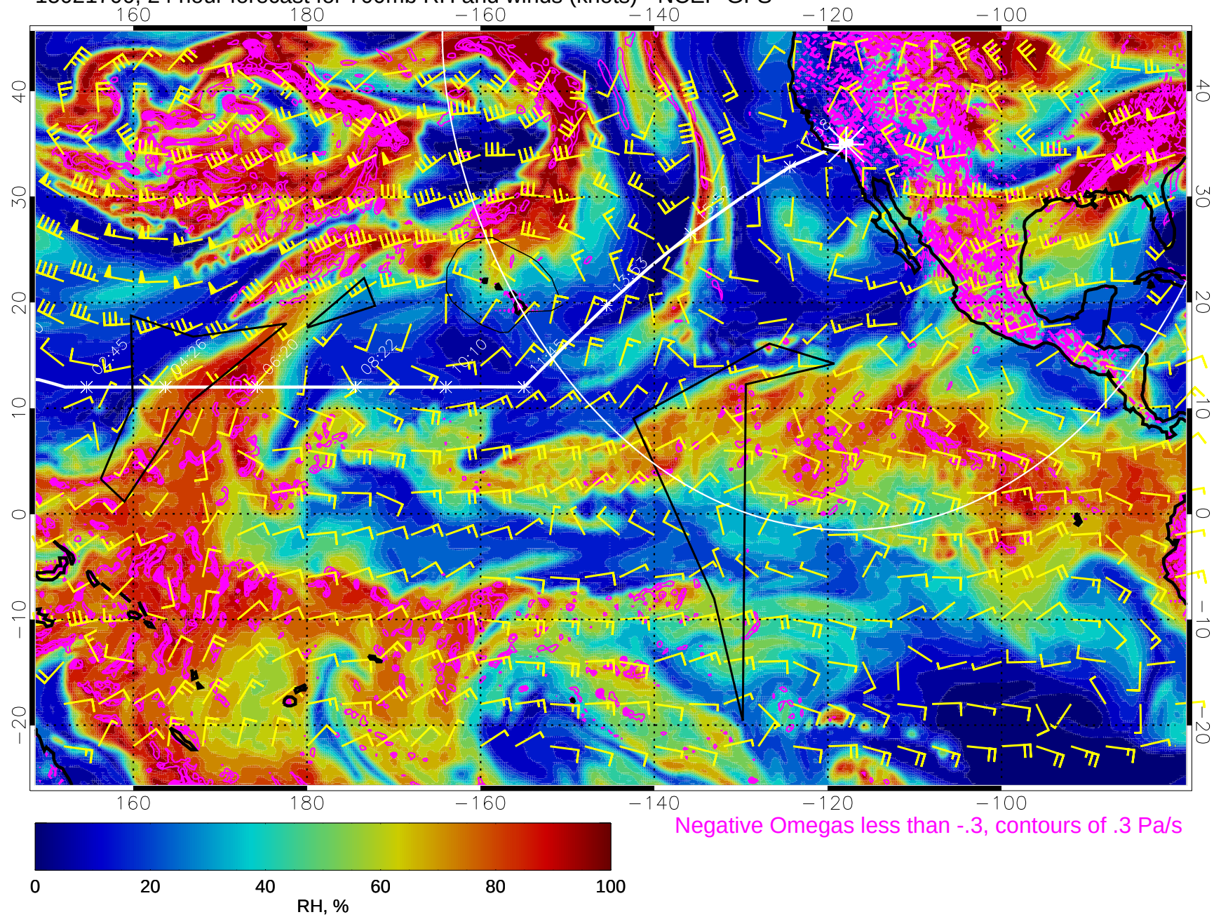
15021700, 24 hour forecast for 700mb RH and winds (knots) - NCEP GFS
