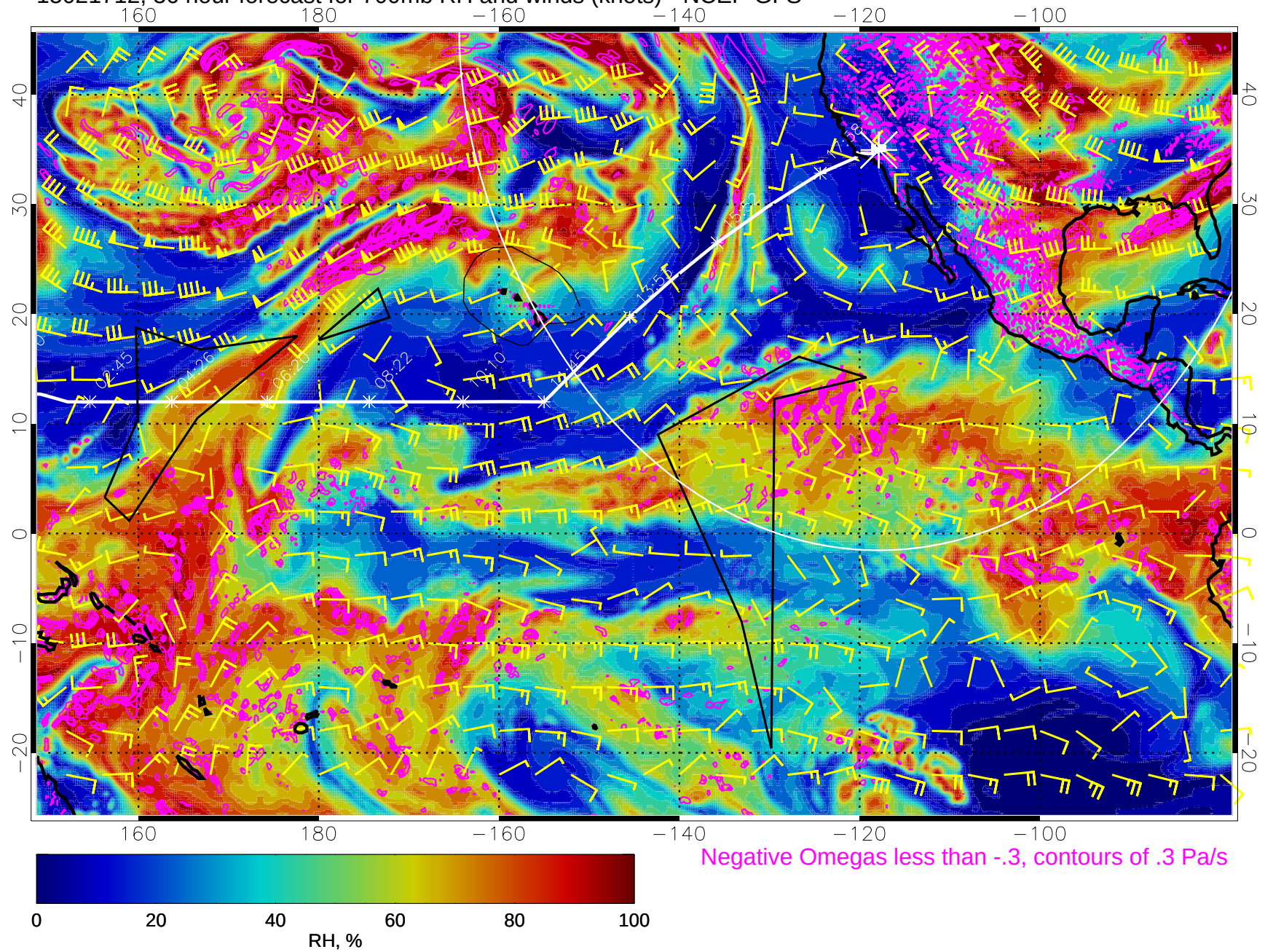
15021712, 36 hour forecast for 700mb RH and winds (knots) - NCEP GFS
