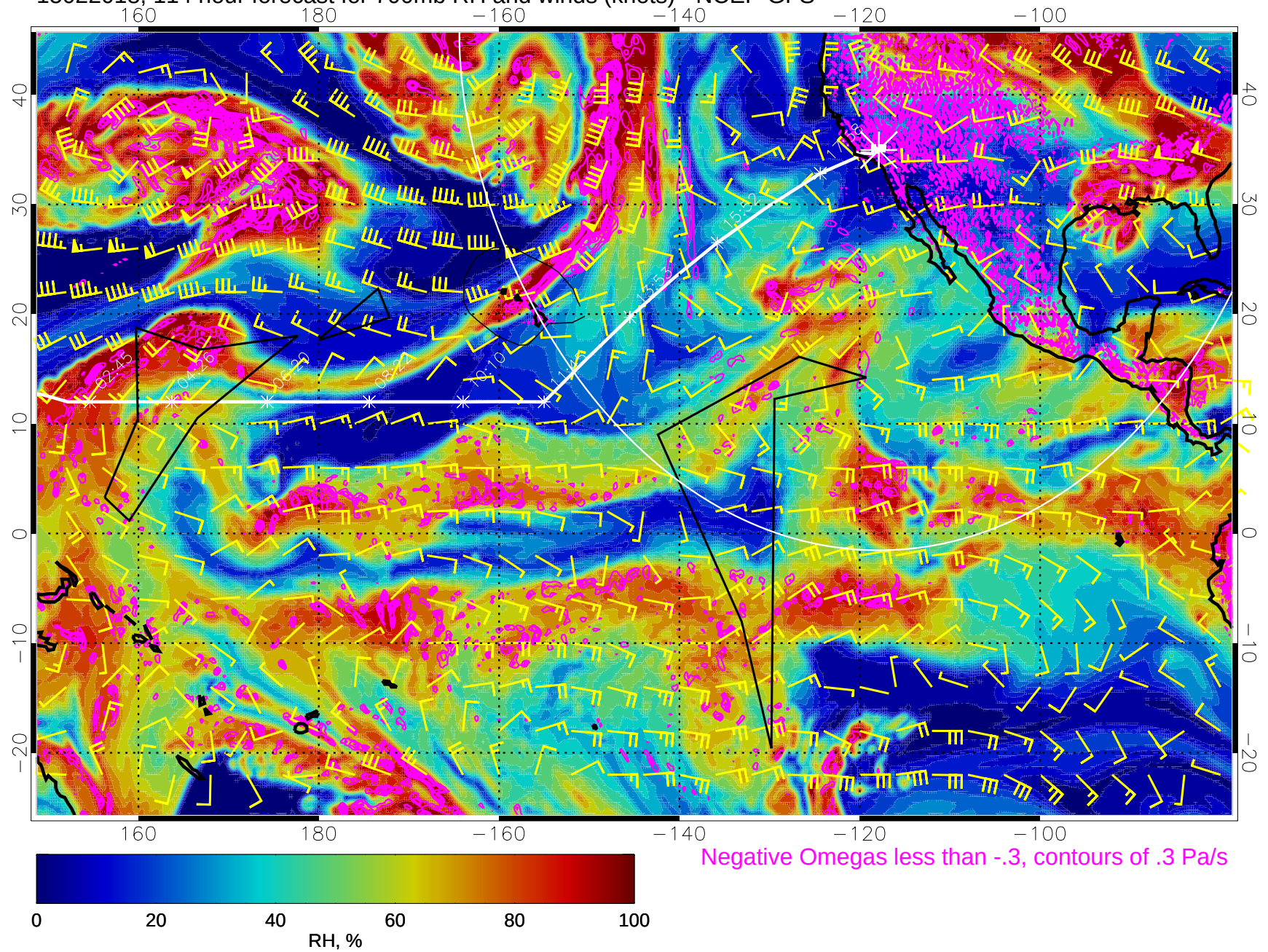
15022018, 114 hour forecast for 700mb RH and winds (knots) - NCEP GFS
