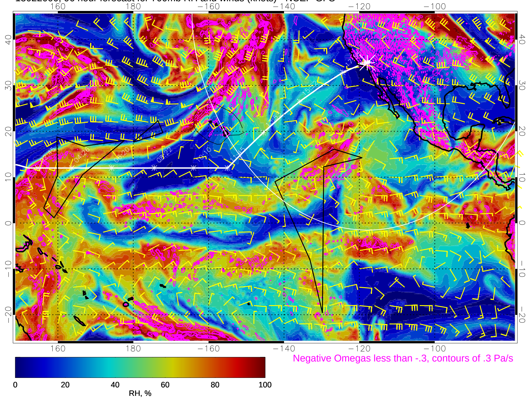
15022000, 96 hour forecast for 700mb RH and winds (knots) - NCEP GFS
