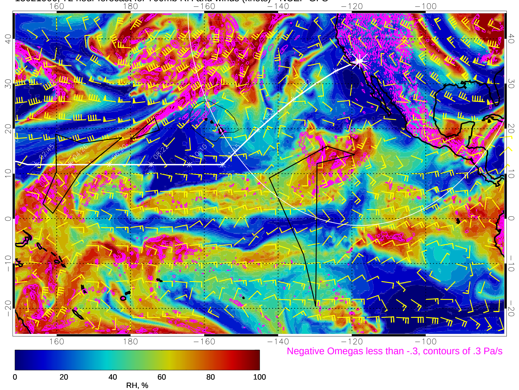
15021900, 72 hour forecast for 700mb RH and winds (knots) - NCEP GFS
