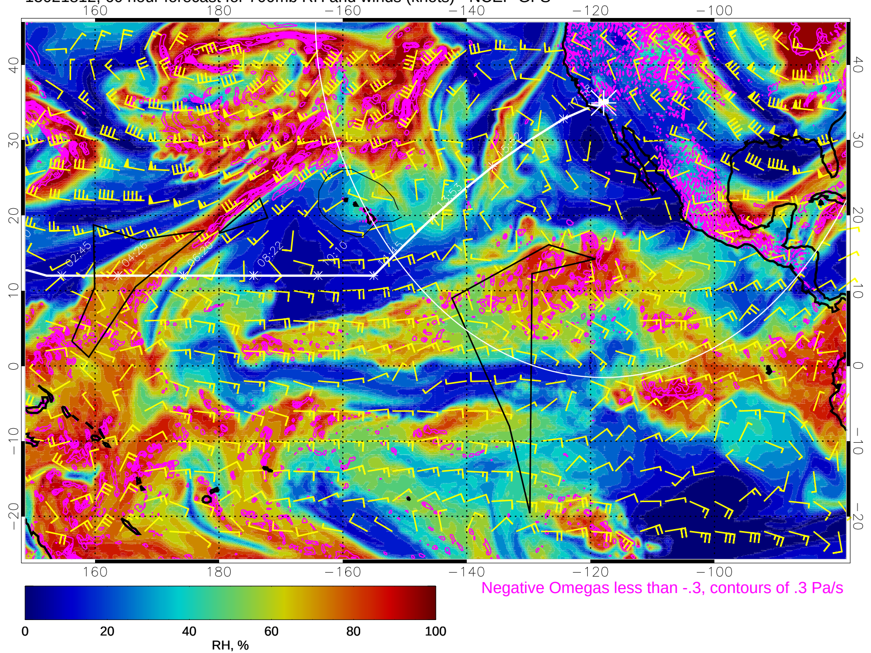
15021812, 60 hour forecast for 700mb RH and winds (knots) - NCEP GFS
