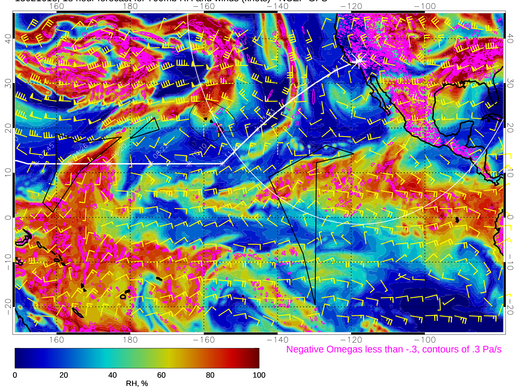
15021618, 18 hour forecast for 700mb RH and winds (knots) - NCEP GFS
