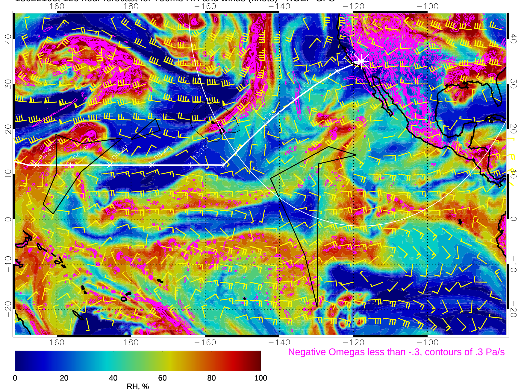
15022100, 120 hour forecast for 700mb RH and winds (knots) - NCEP GFS
