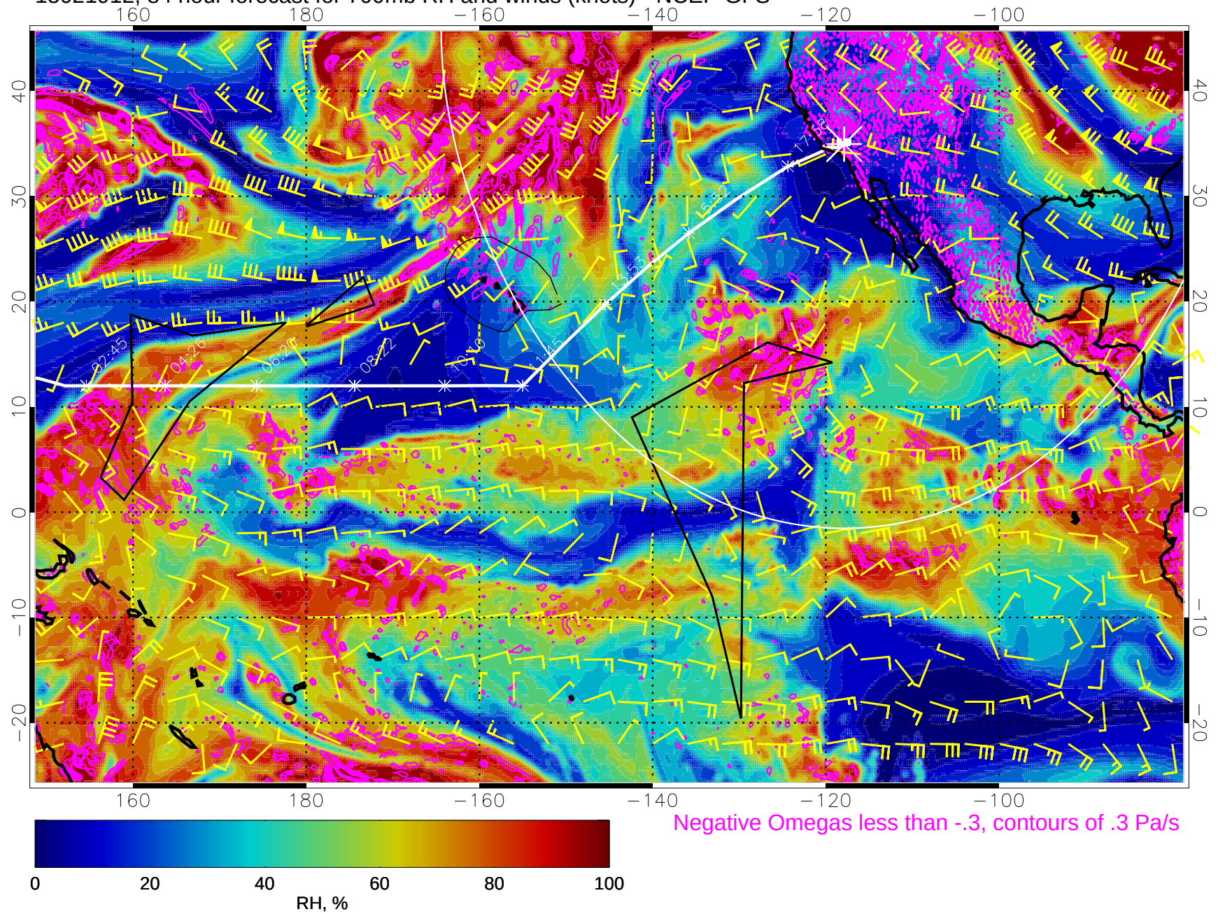
15021912, 84 hour forecast for 700mb RH and winds (knots) - NCEP GFS
