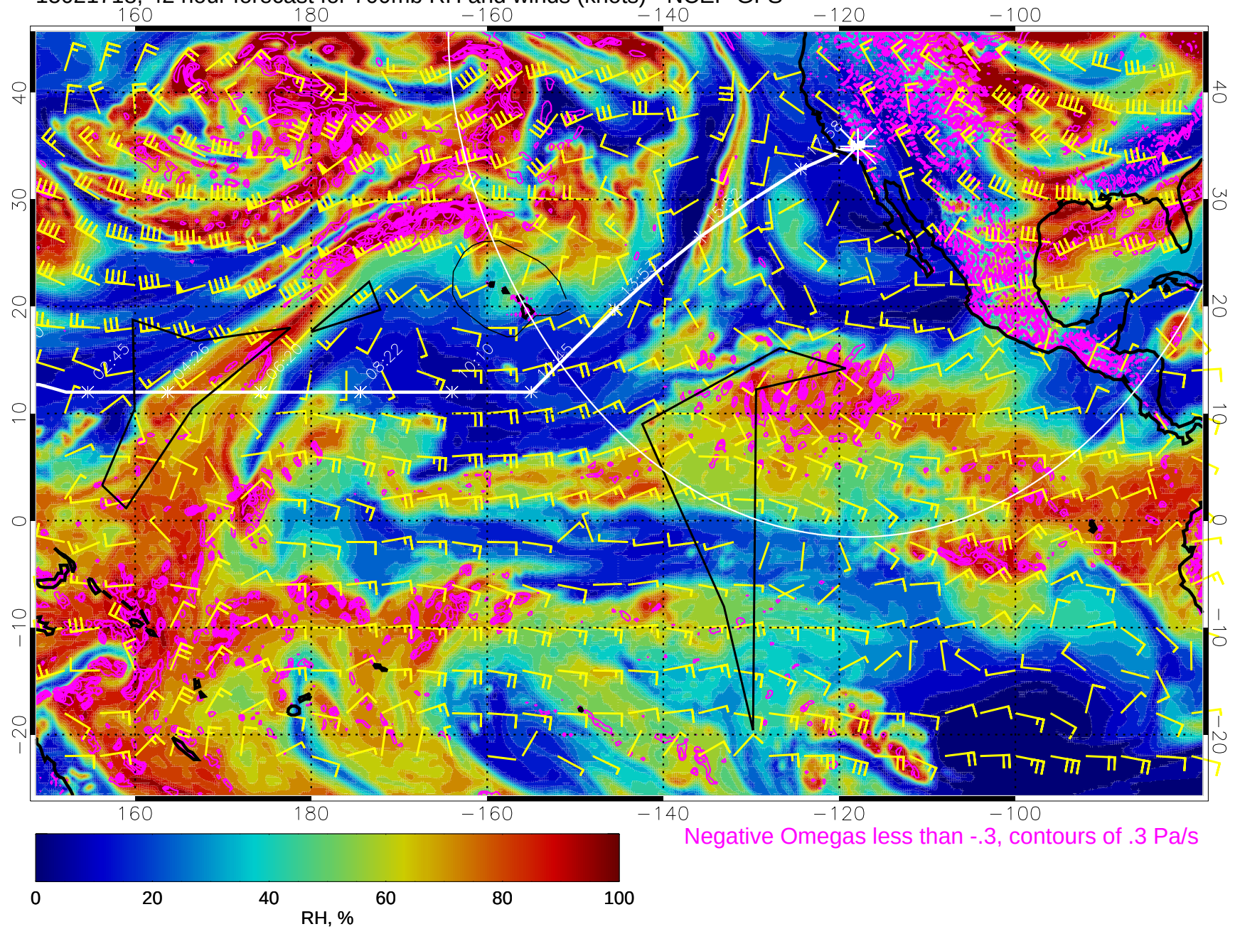
15021718, 42 hour forecast for 700mb RH and winds (knots) - NCEP GFS
