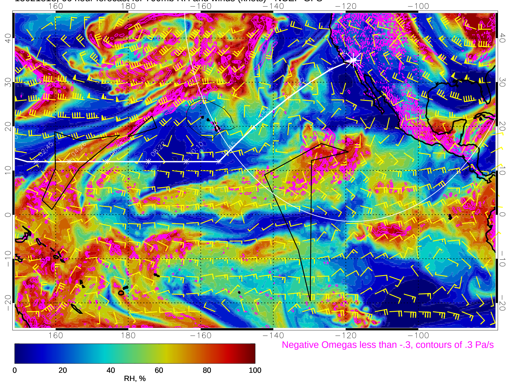
15021818, 66 hour forecast for 700mb RH and winds (knots) - NCEP GFS
