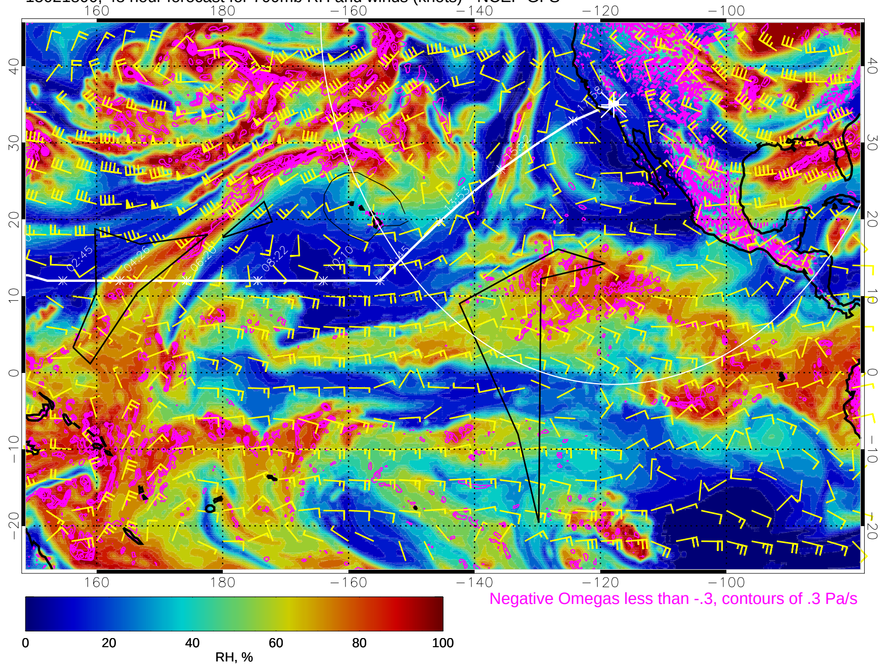
15021800, 48 hour forecast for 700mb RH and winds (knots) - NCEP GFS
