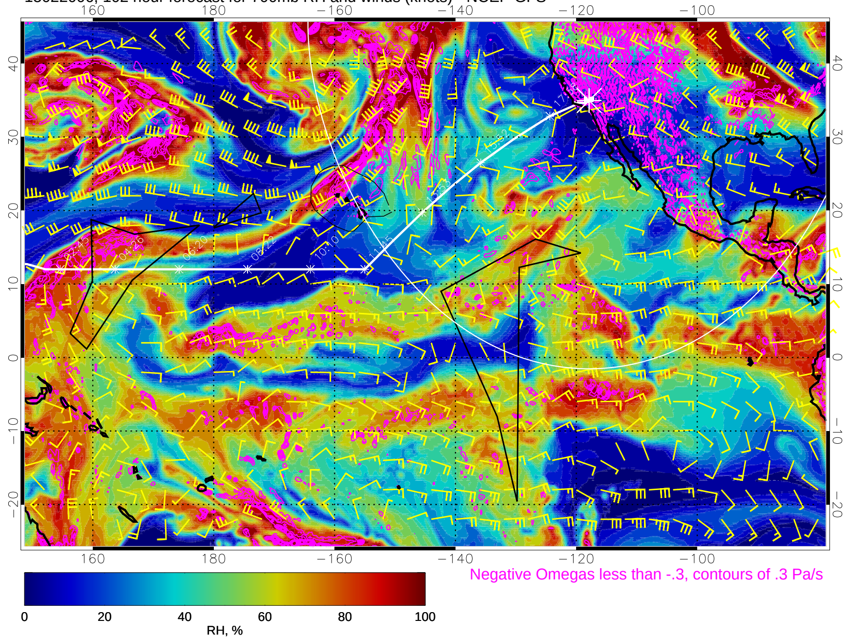
15022006, 102 hour forecast for 700mb RH and winds (knots) - NCEP GFS
