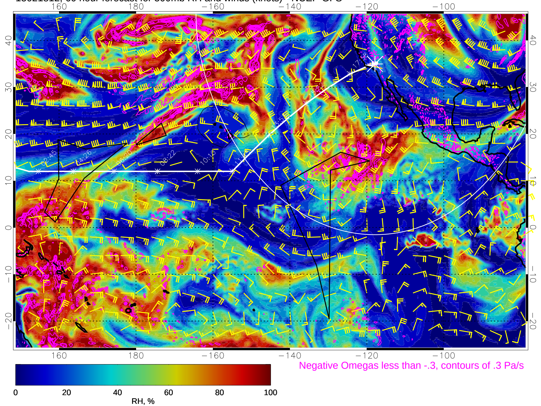
15021812, 60 hour forecast for 500mb RH and winds (knots) - NCEP GFS
