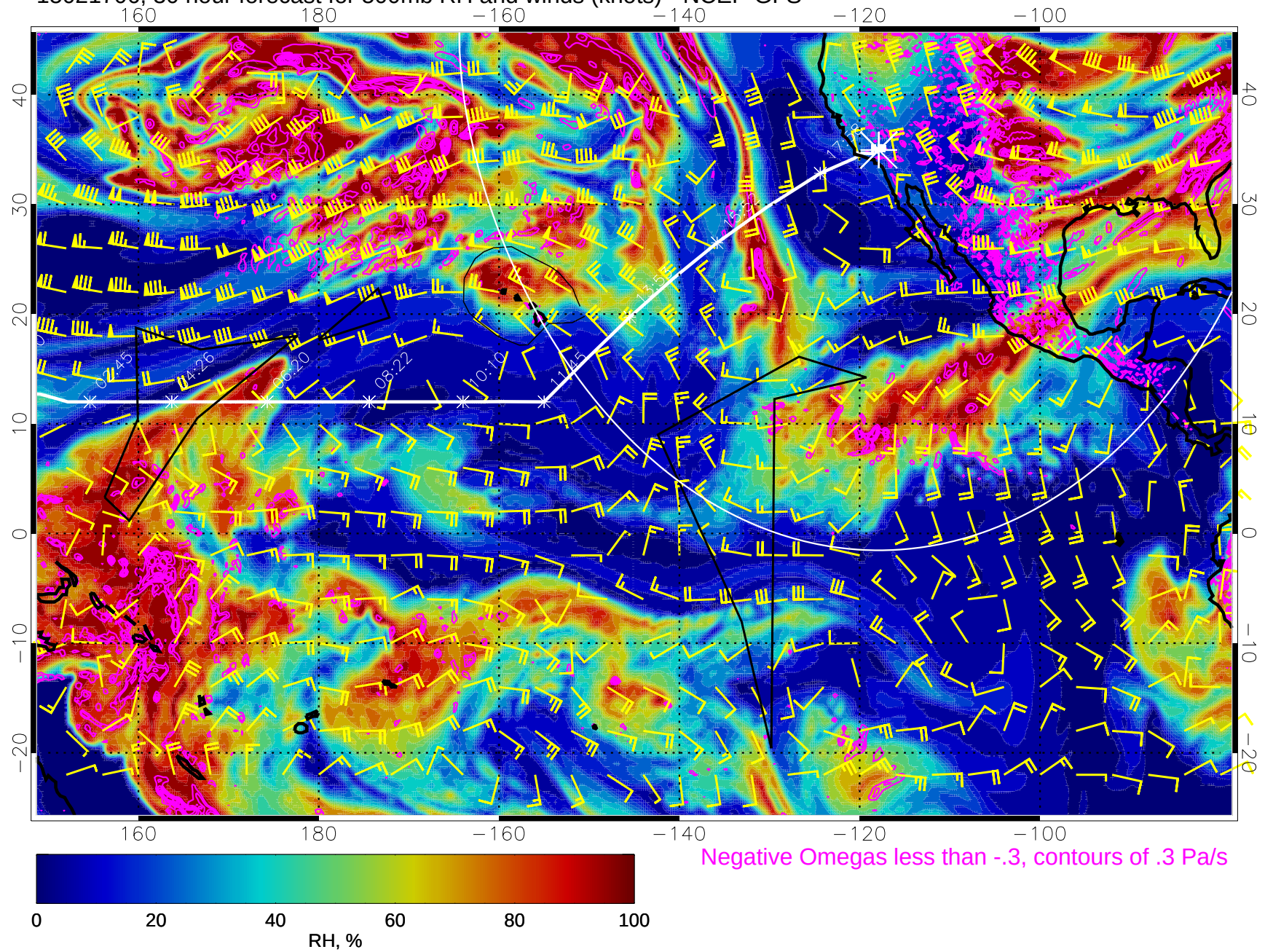
15021706, 30 hour forecast for 500mb RH and winds (knots) - NCEP GFS
