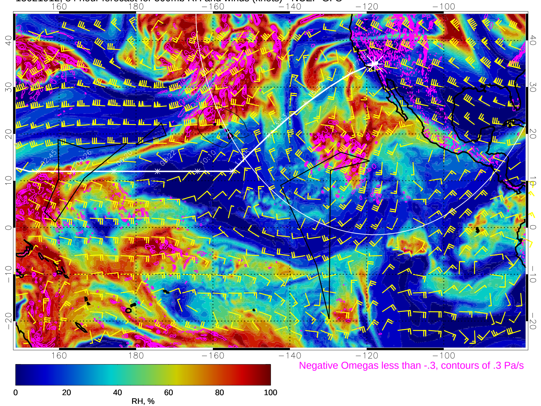
15021912, 84 hour forecast for 500mb RH and winds (knots) - NCEP GFS
