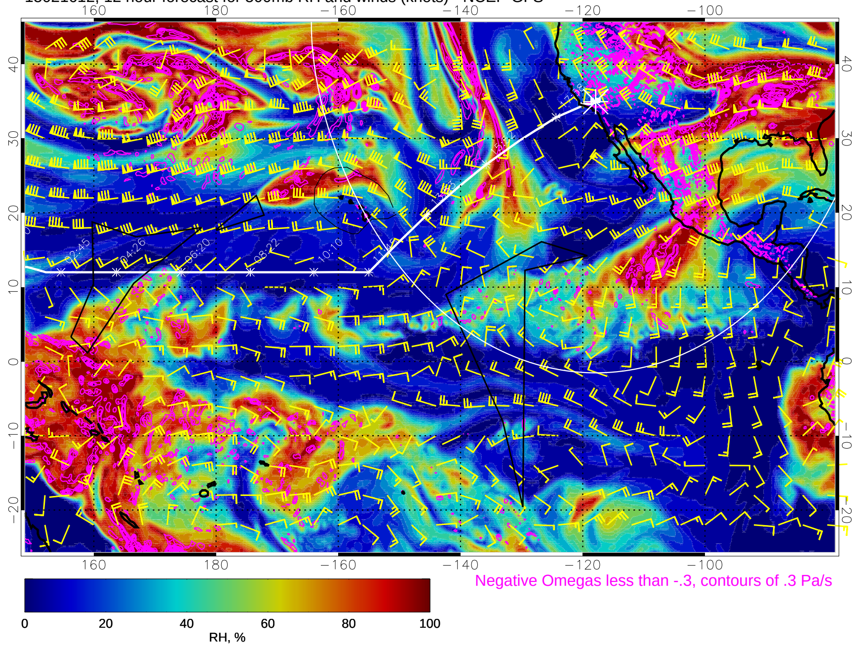
15021612, 12 hour forecast for 500mb RH and winds (knots) - NCEP GFS
