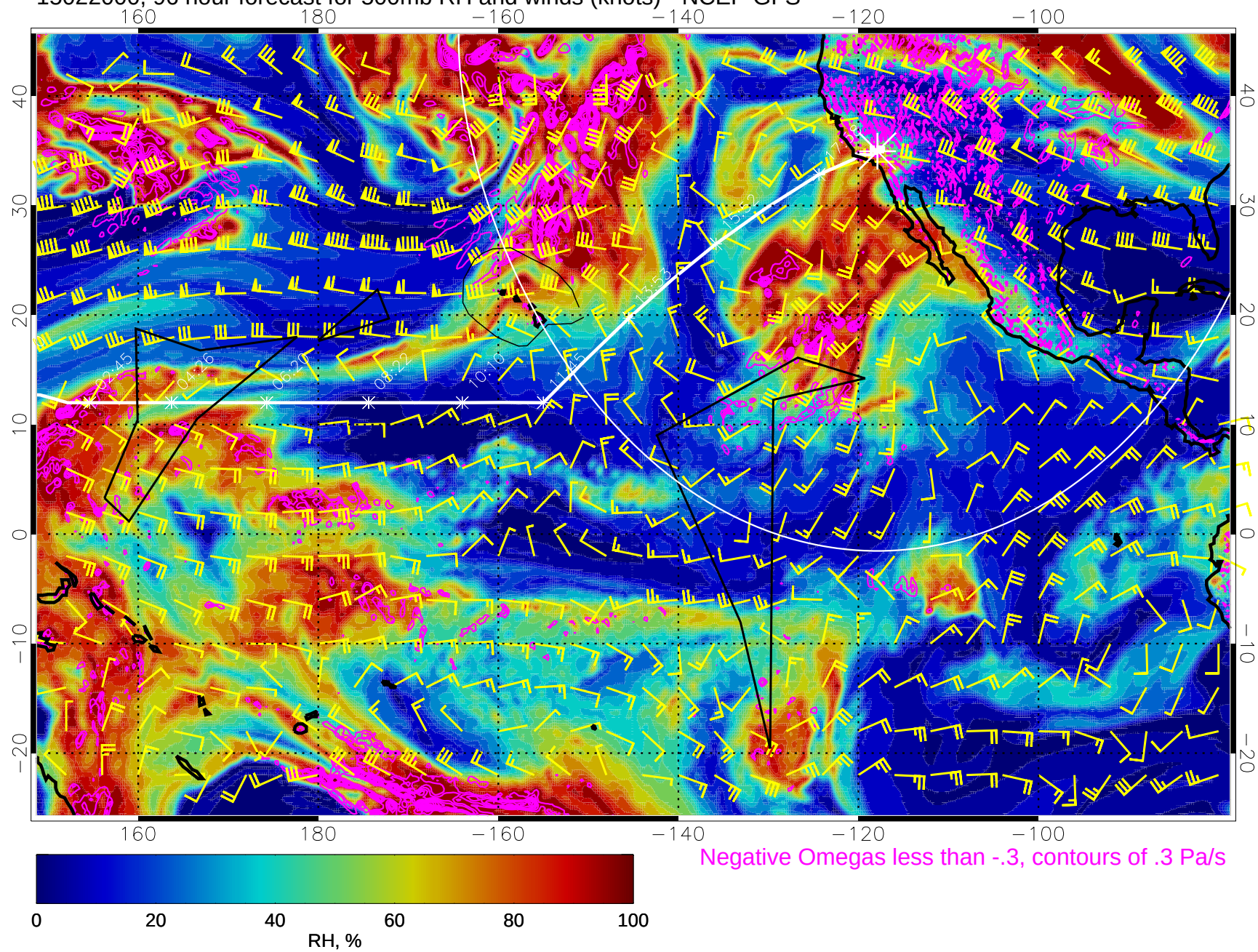
15022000, 96 hour forecast for 500mb RH and winds (knots) - NCEP GFS
