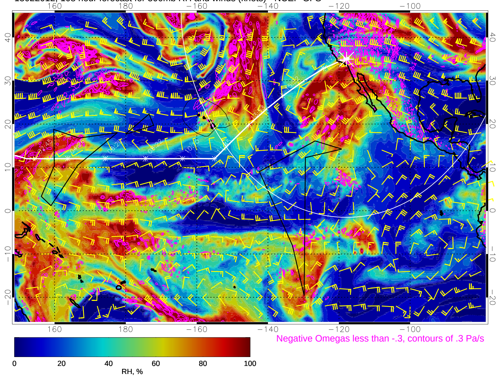
15022012, 108 hour forecast for 500mb RH and winds (knots) - NCEP GFS
