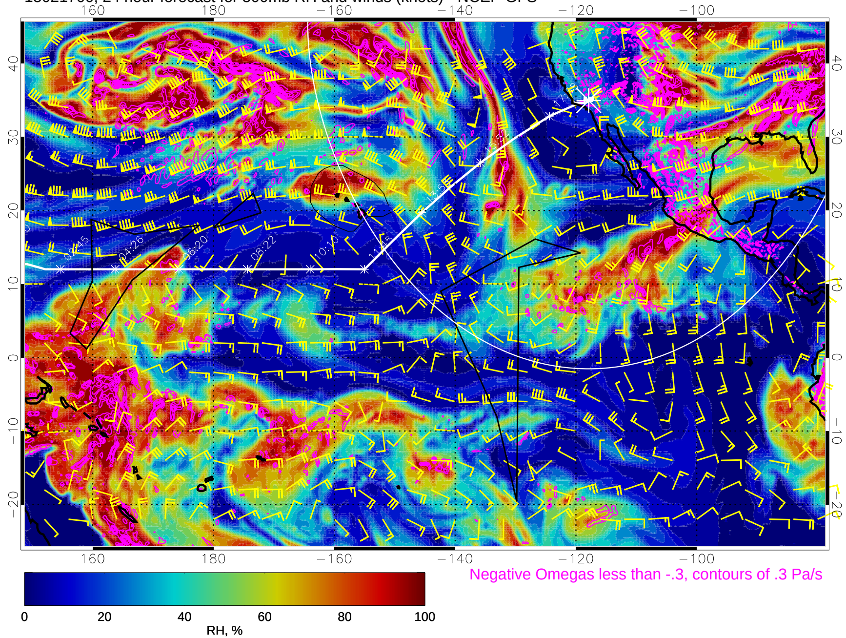
15021700, 24 hour forecast for 500mb RH and winds (knots) - NCEP GFS
