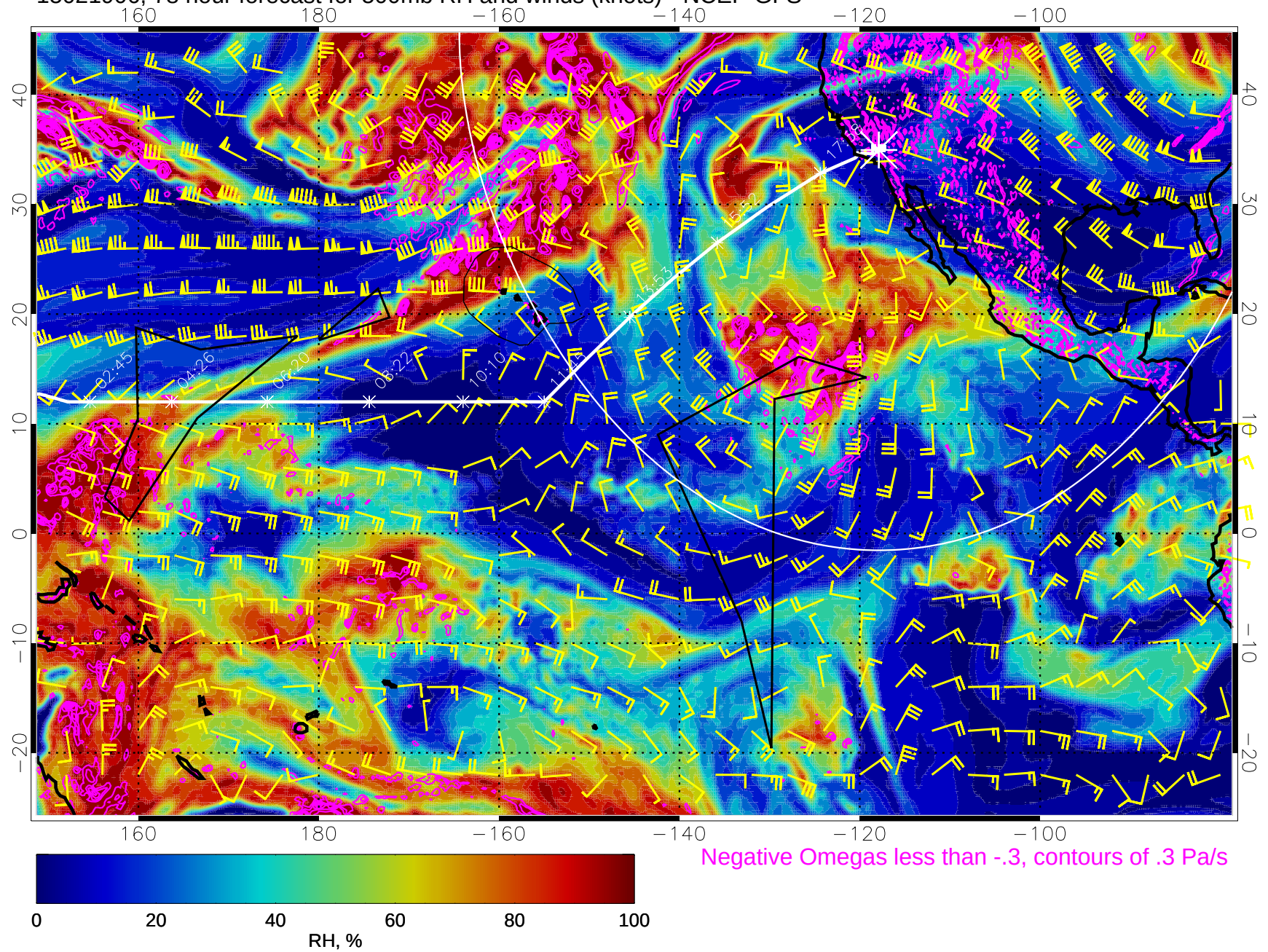
15021906, 78 hour forecast for 500mb RH and winds (knots) - NCEP GFS
