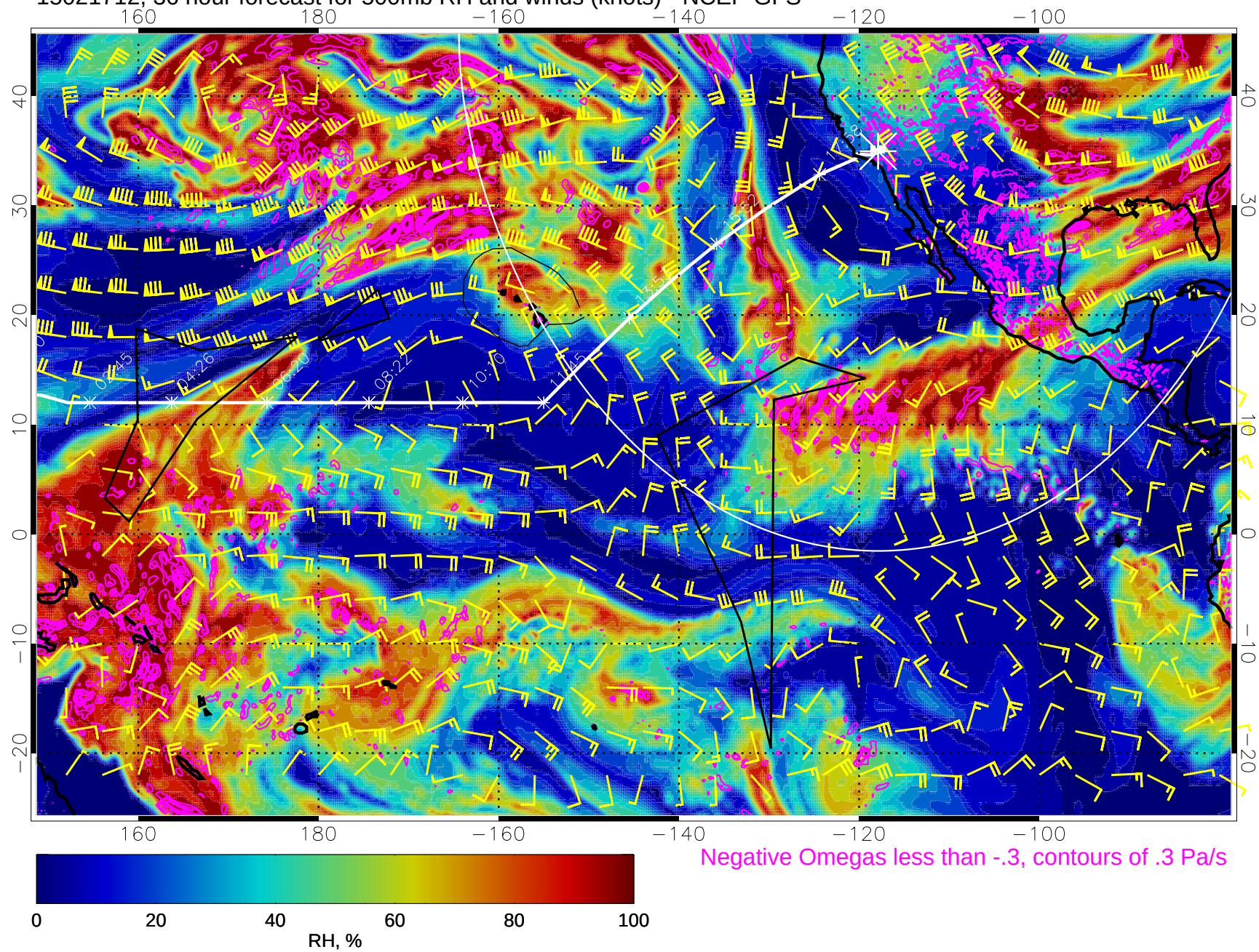
15021712, 36 hour forecast for 500mb RH and winds (knots) - NCEP GFS
