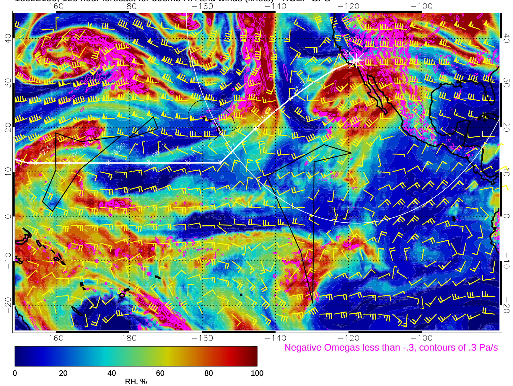
15022100, 120 hour forecast for 500mb RH and winds (knots) - NCEP GFS
