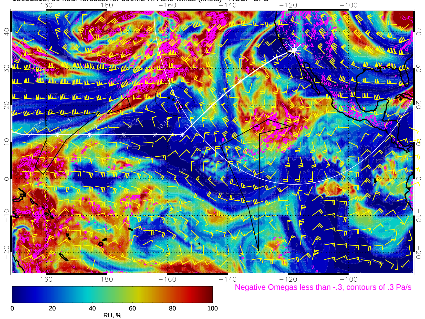
15021818, 66 hour forecast for 500mb RH and winds (knots) - NCEP GFS
