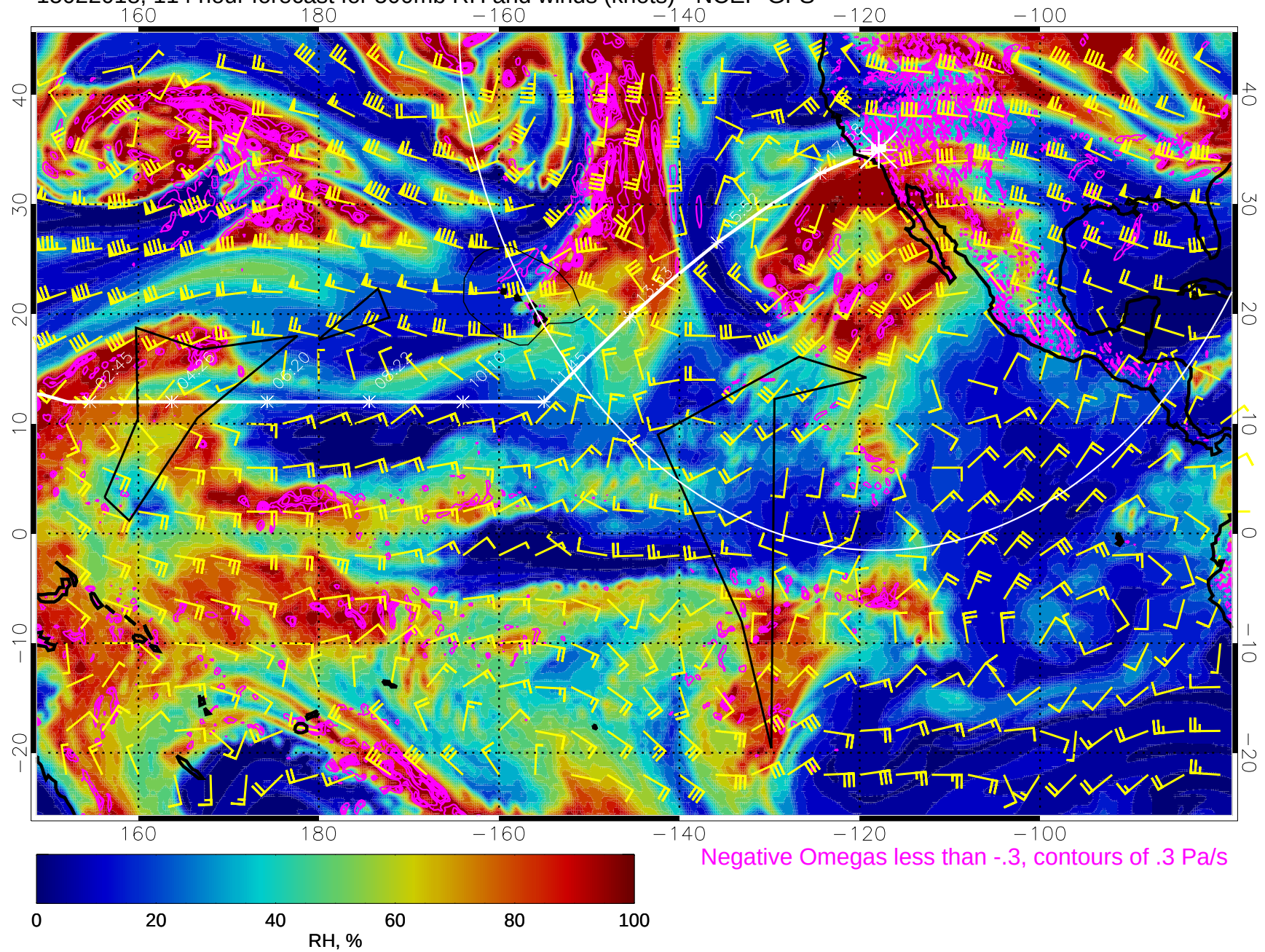
15022018, 114 hour forecast for 500mb RH and winds (knots) - NCEP GFS
