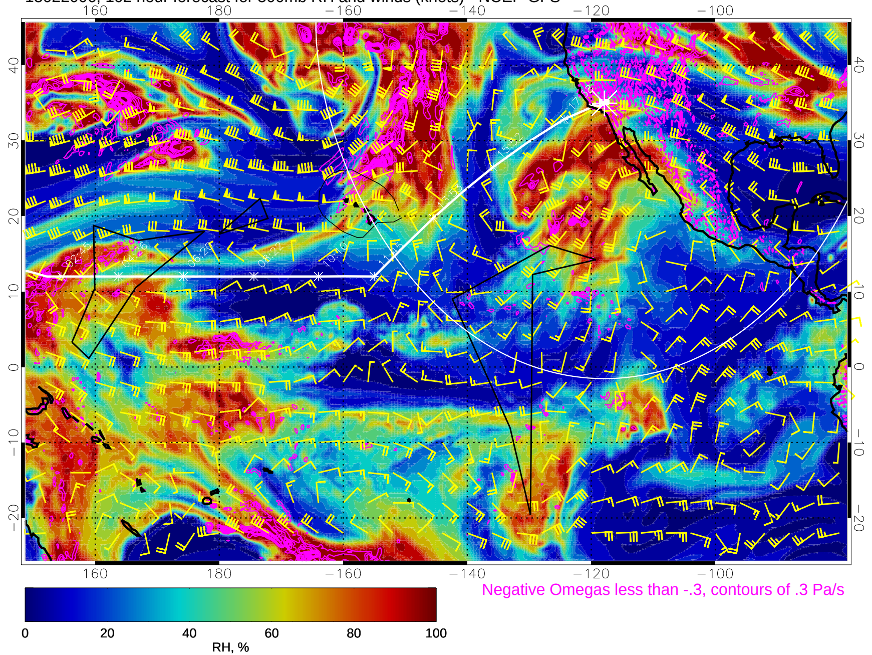
15022006, 102 hour forecast for 500mb RH and winds (knots) - NCEP GFS
