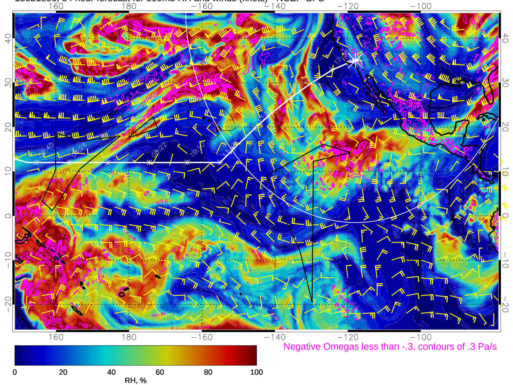
15021806, 54 hour forecast for 500mb RH and winds (knots) - NCEP GFS
