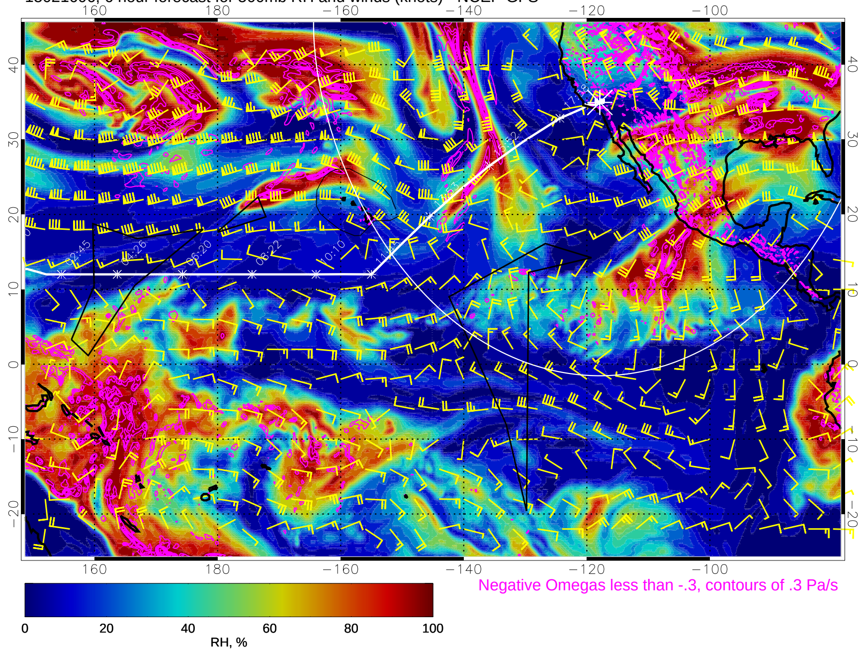
15021606, 6 hour forecast for 500mb RH and winds (knots) - NCEP GFS
