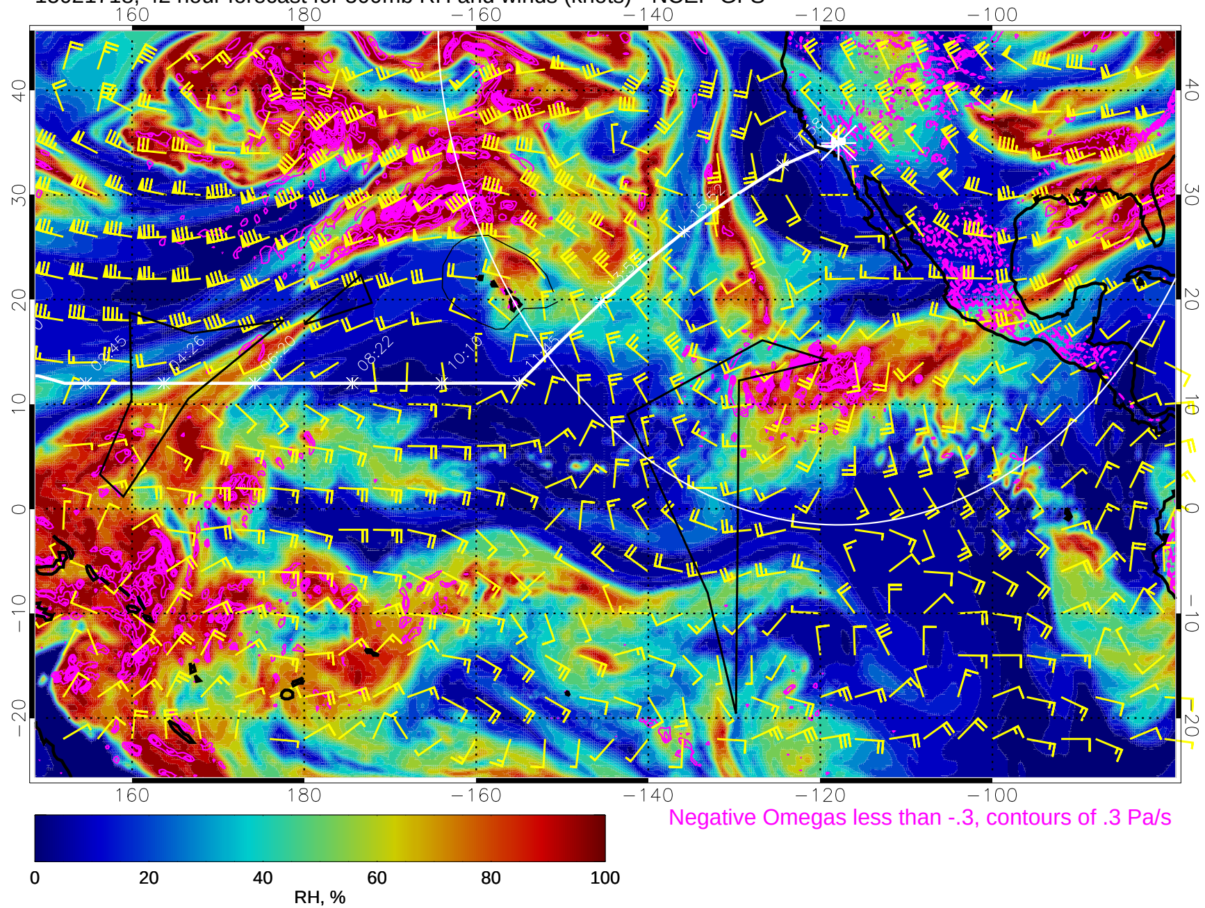
15021718, 42 hour forecast for 500mb RH and winds (knots) - NCEP GFS
