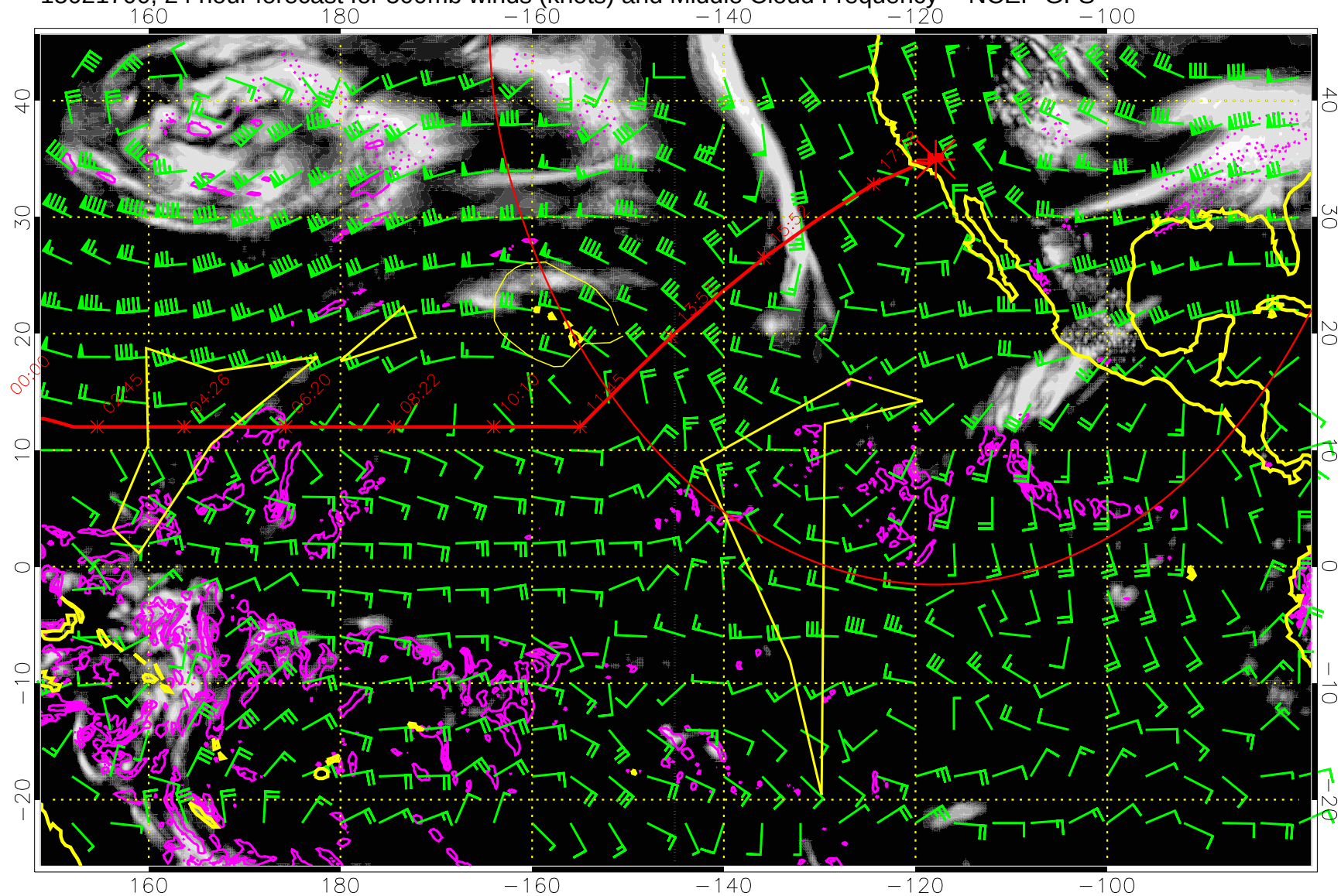
15021700, 24 hour forecast for 500mb winds (knots) and Middle Cloud Frequency -- NCEP GFS
