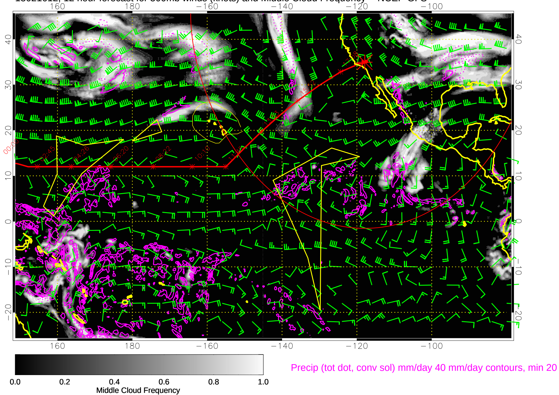
15021612, 12 hour forecast for 500mb winds (knots) and Middle Cloud Frequency -- NCEP GFS
