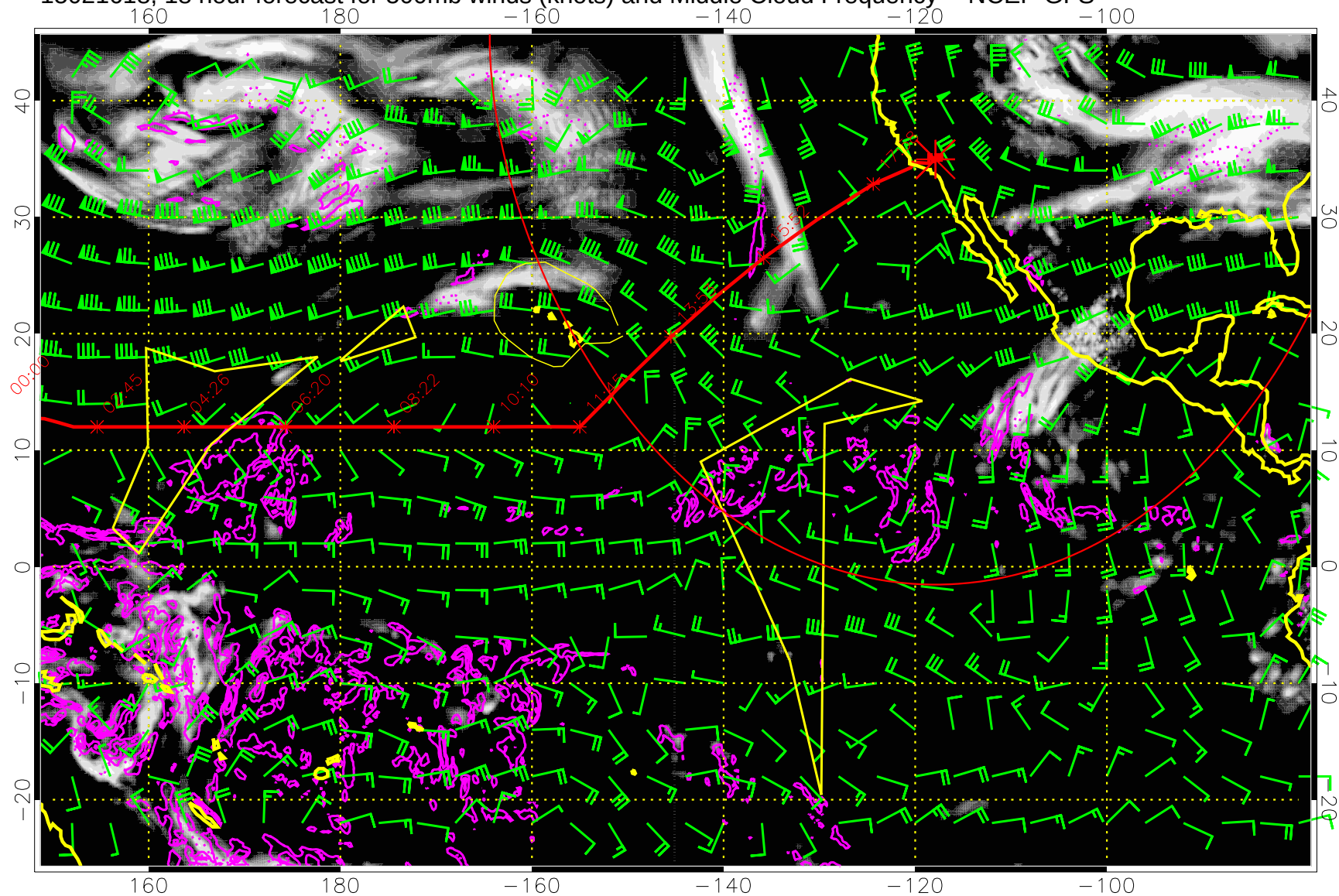
15021618, 18 hour forecast for 500mb winds (knots) and Middle Cloud Frequency -- NCEP GFS
