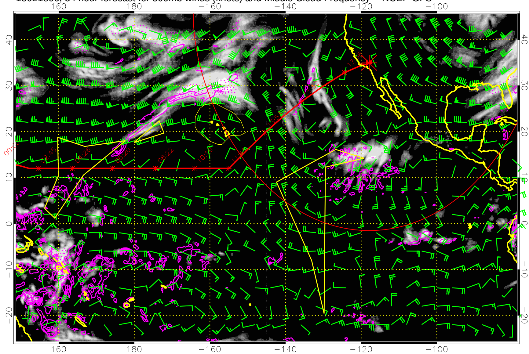
15021806, 54 hour forecast for 500mb winds (knots) and Middle Cloud Frequency -- NCEP GFS
