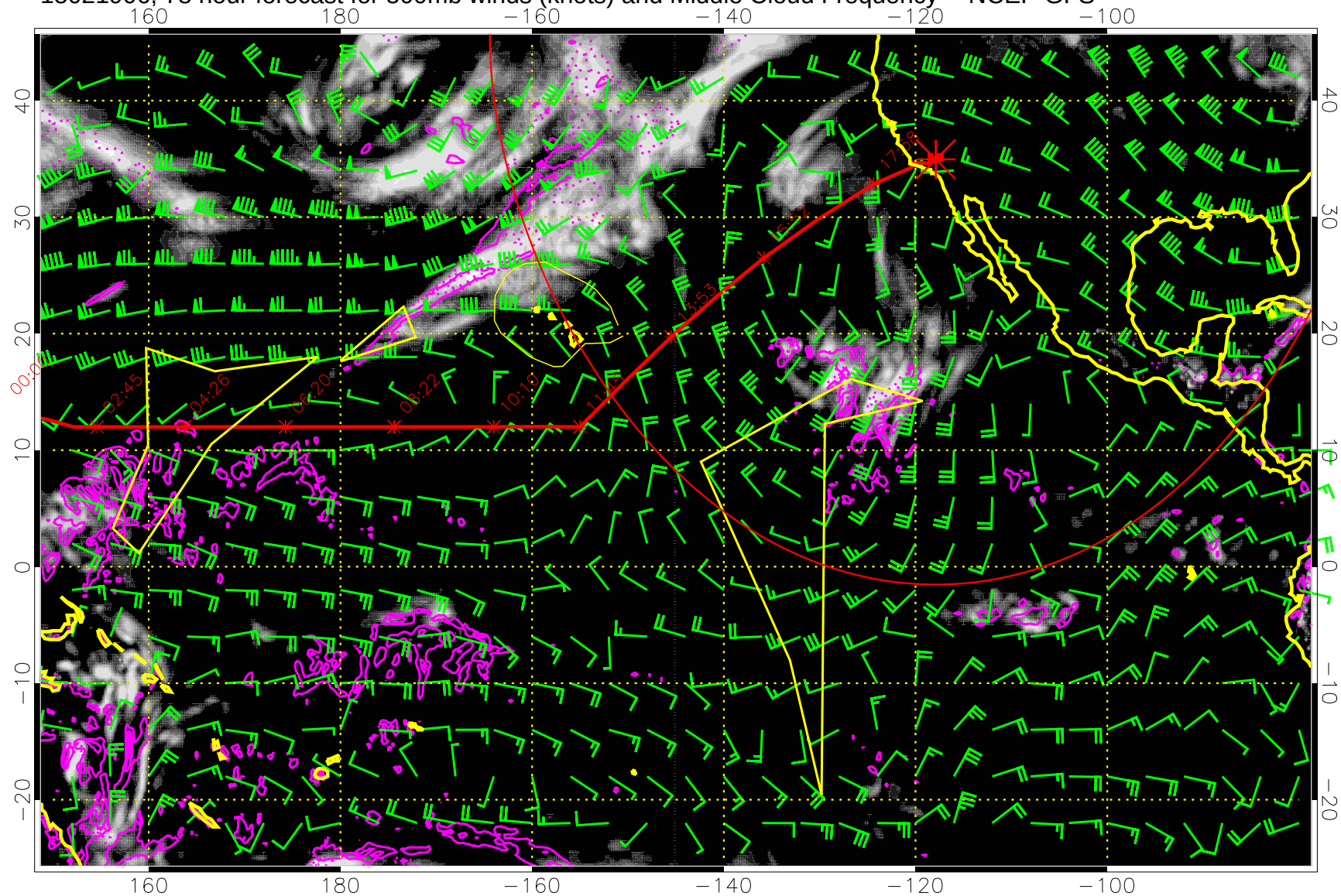
15021906, 78 hour forecast for 500mb winds (knots) and Middle Cloud Frequency -- NCEP GFS
