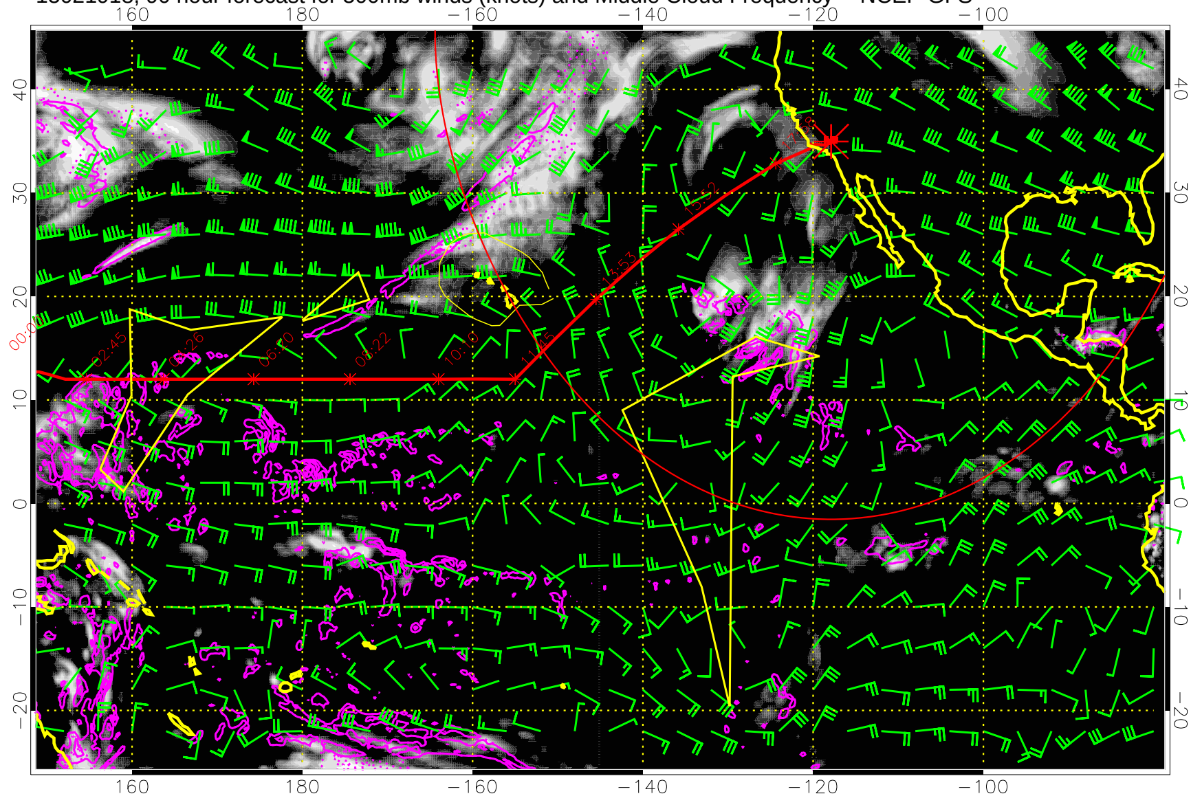
15021918, 90 hour forecast for 500mb winds (knots) and Middle Cloud Frequency -- NCEP GFS
