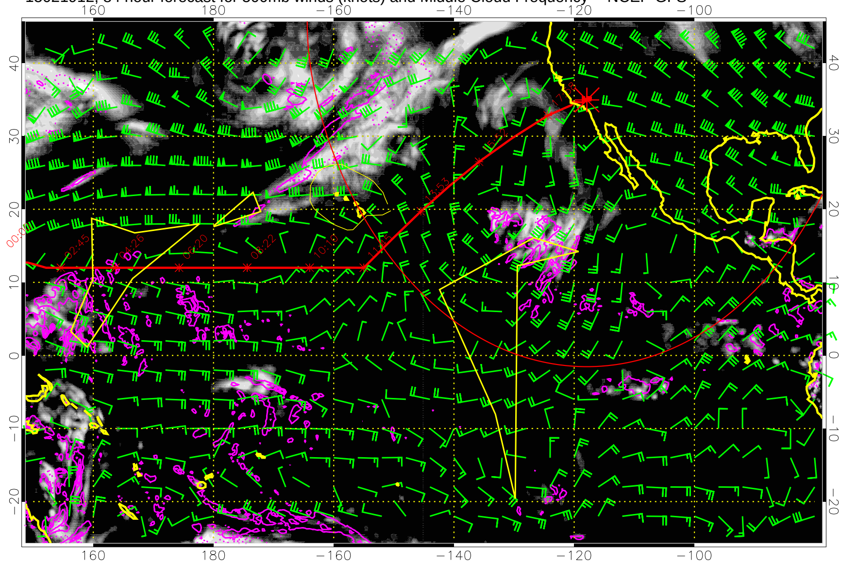
15021912, 84 hour forecast for 500mb winds (knots) and Middle Cloud Frequency -- NCEP GFS
