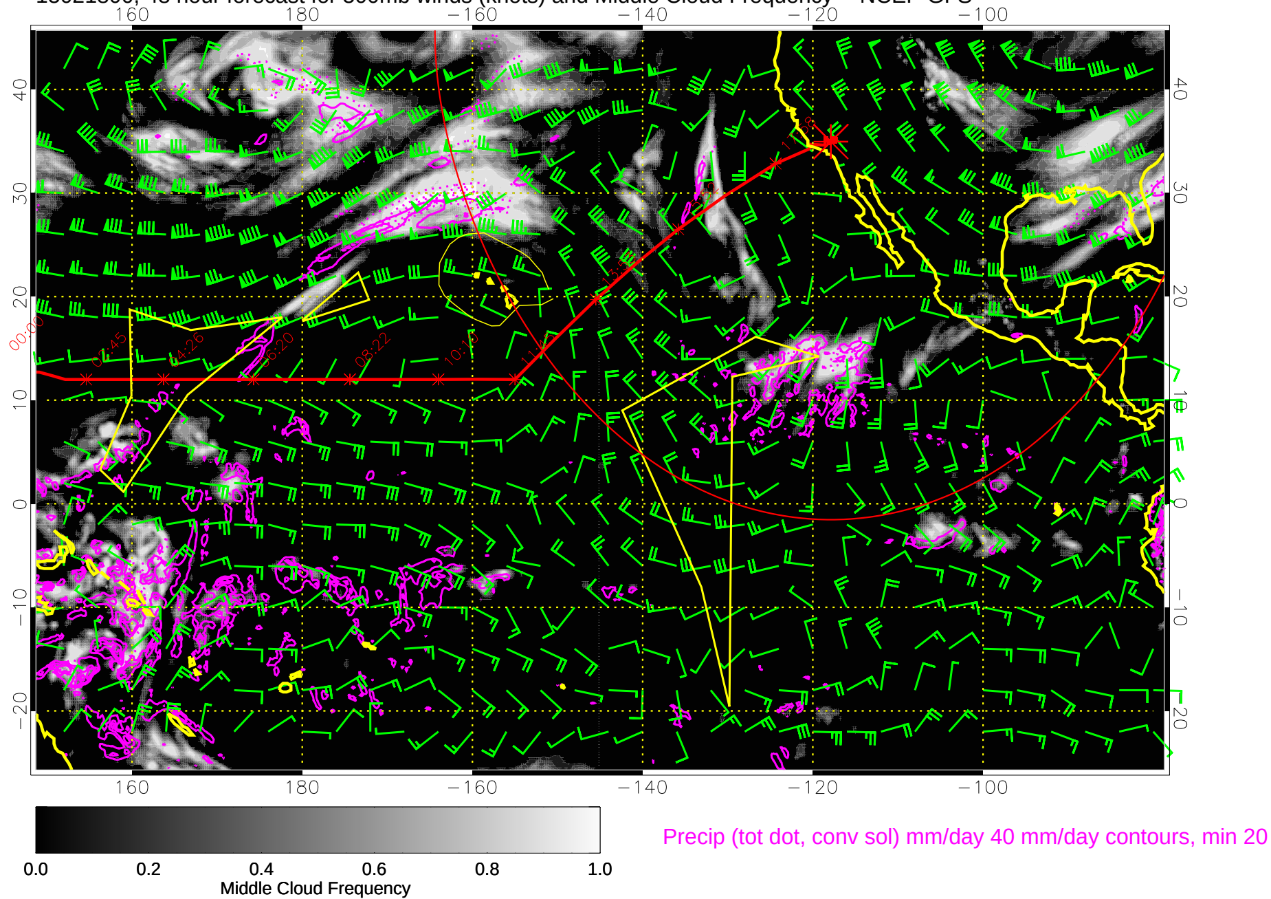
15021800, 48 hour forecast for 500mb winds (knots) and Middle Cloud Frequency -- NCEP GFS
