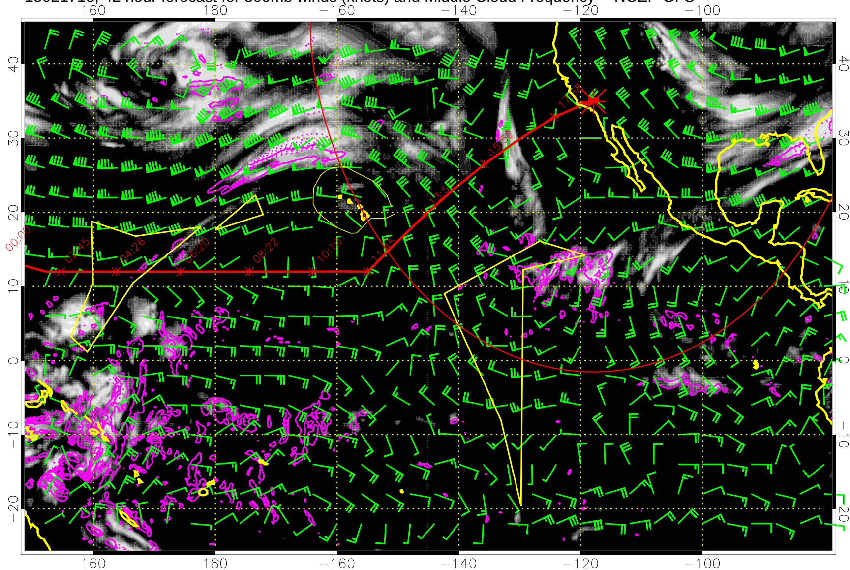
15021718, 42 hour forecast for 500mb winds (knots) and Middle Cloud Frequency -- NCEP GFS
