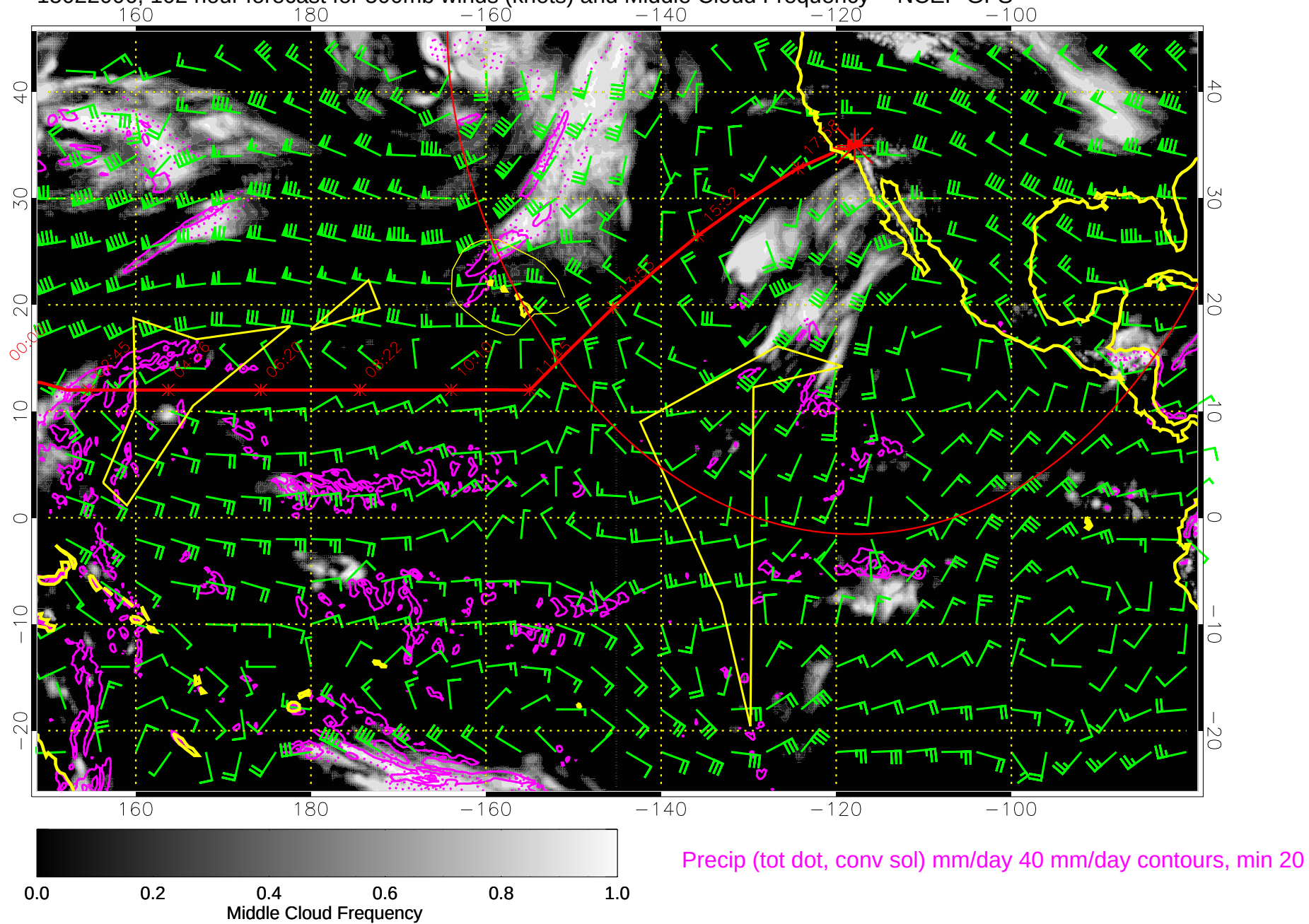
15022006, 102 hour forecast for 500mb winds (knots) and Middle Cloud Frequency -- NCEP GFS
