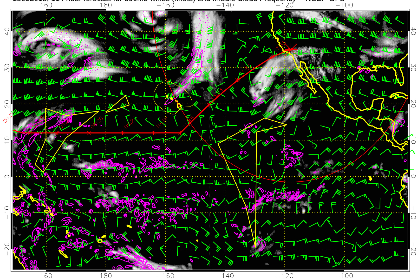
15022018, 114 hour forecast for 500mb winds (knots) and Middle Cloud Frequency -- NCEP GFS
