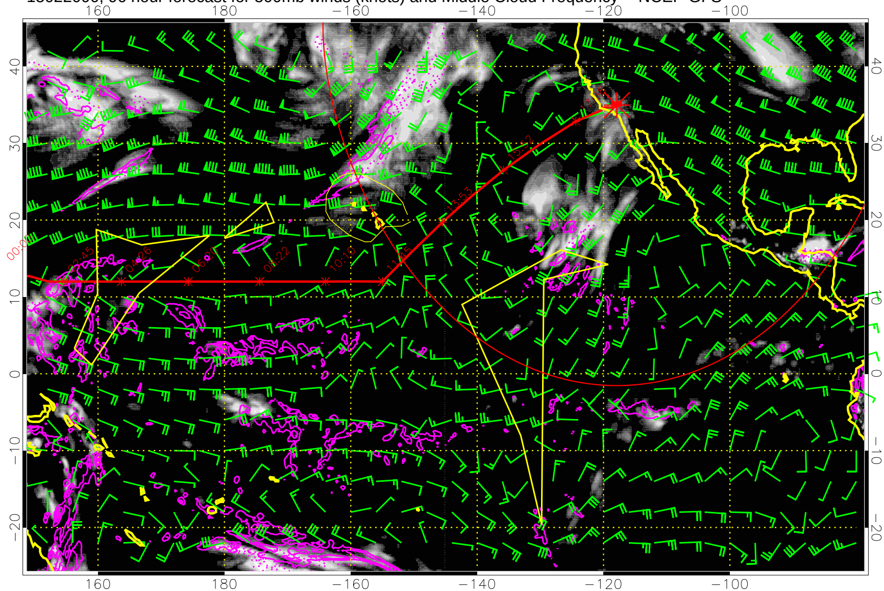
15022000, 96 hour forecast for 500mb winds (knots) and Middle Cloud Frequency -- NCEP GFS
