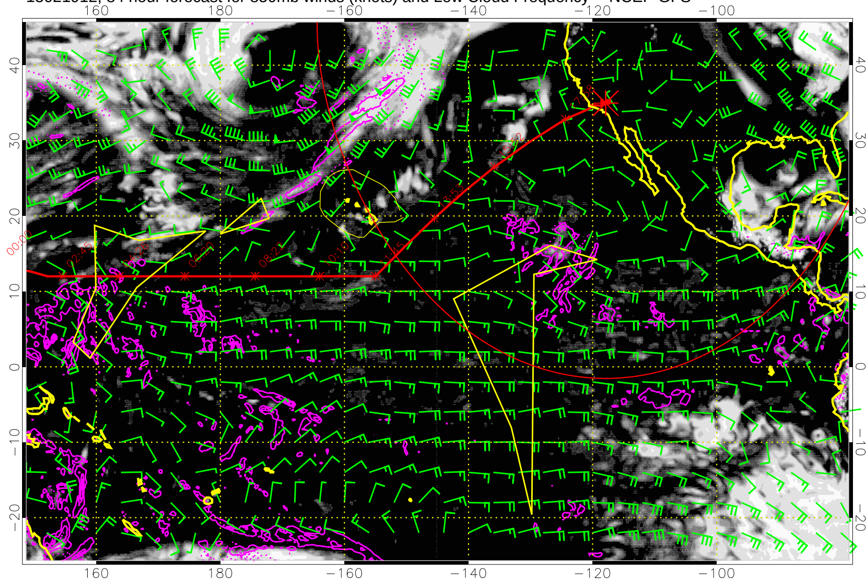
15021912, 84 hour forecast for 850mb winds (knots) and Low Cloud Frequency -- NCEP GFS
