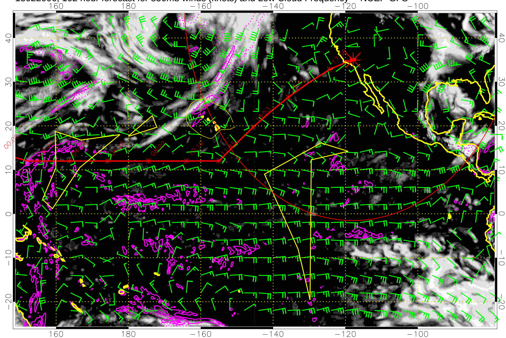
15022006, 102 hour forecast for 850mb winds (knots) and Low Cloud Frequency -- NCEP GFS
