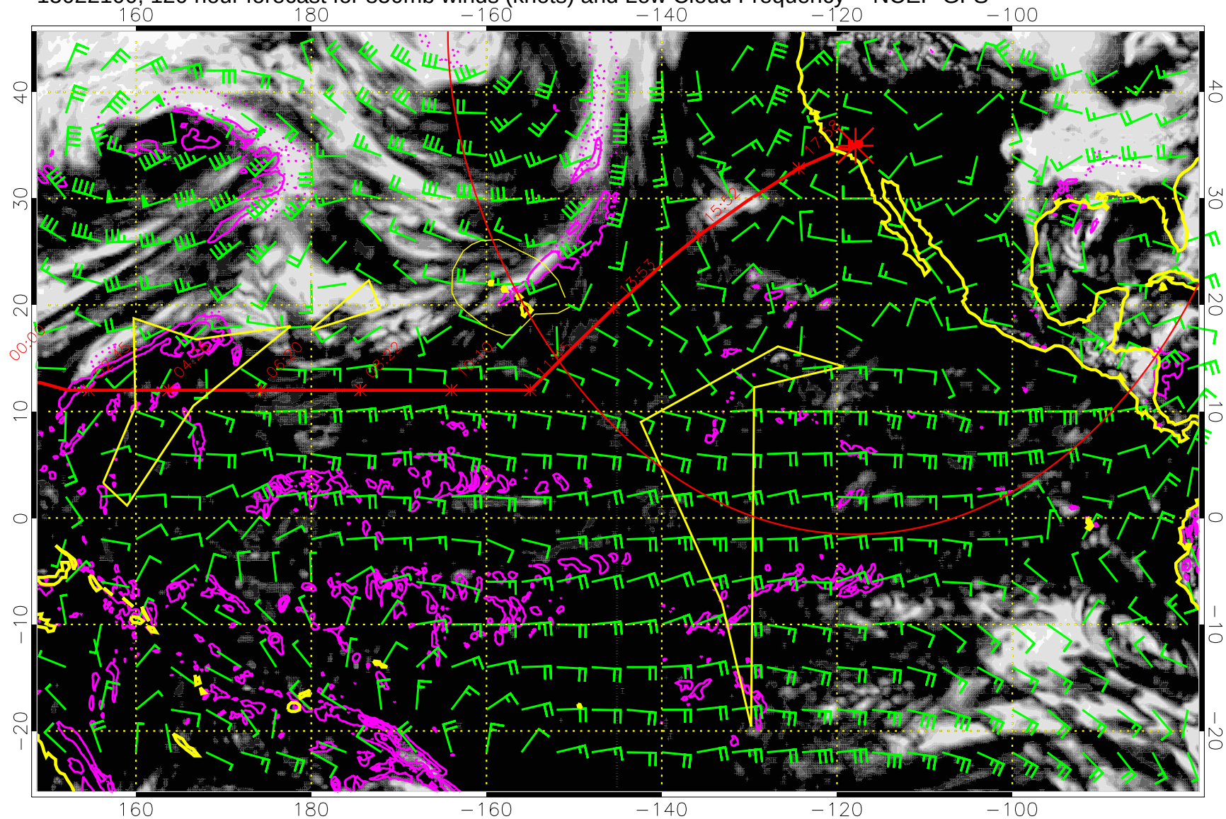
15022100, 120 hour forecast for 850mb winds (knots) and Low Cloud Frequency -- NCEP GFS
