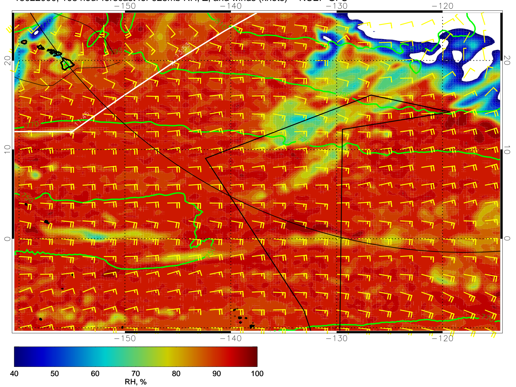
15022000, 108 hour forecast for 925mb RH, Z, and winds (knots) -- NCEP GFS
