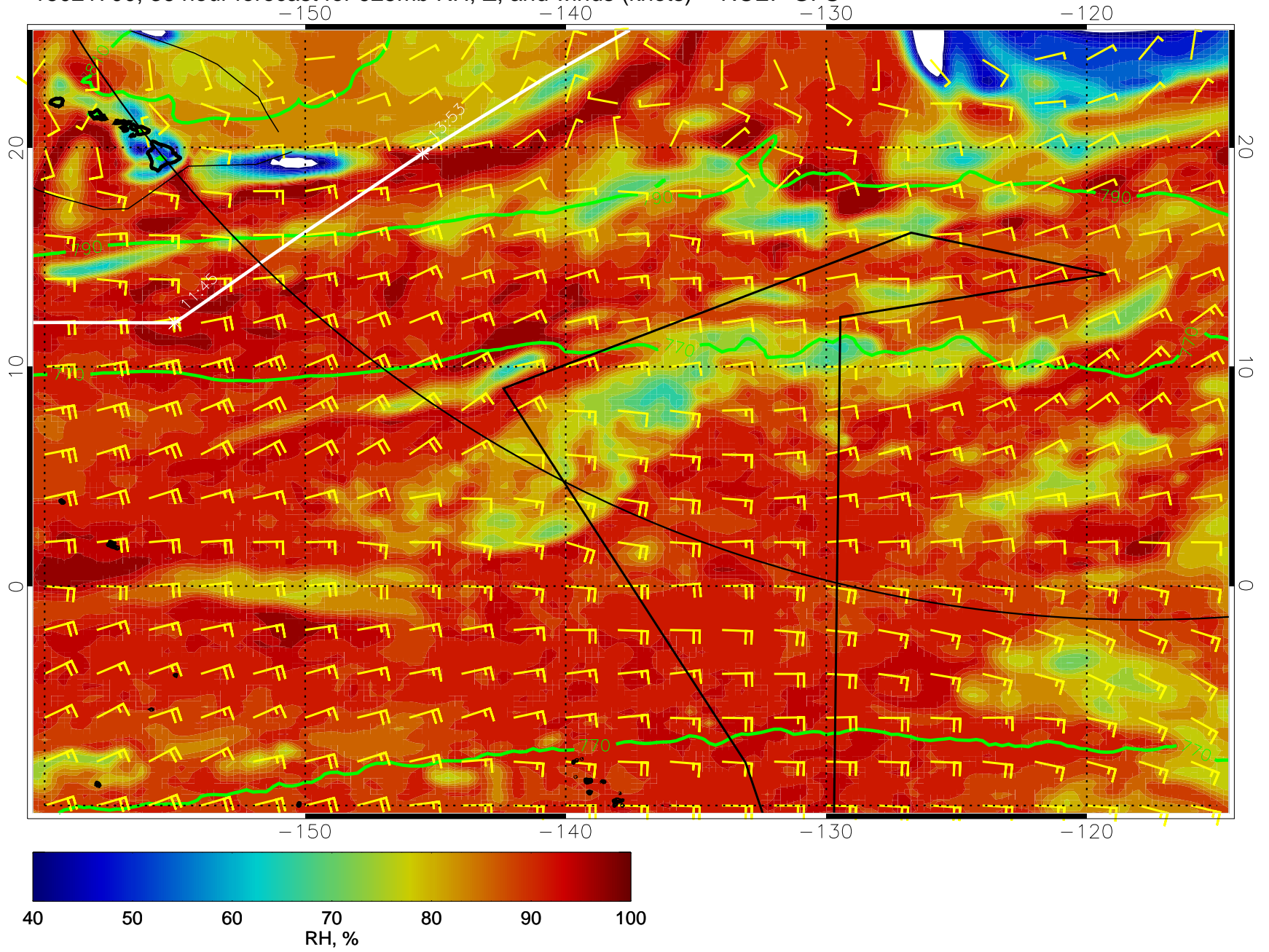
15021700, 36 hour forecast for 925mb RH, Z, and winds (knots) -- NCEP GFS
