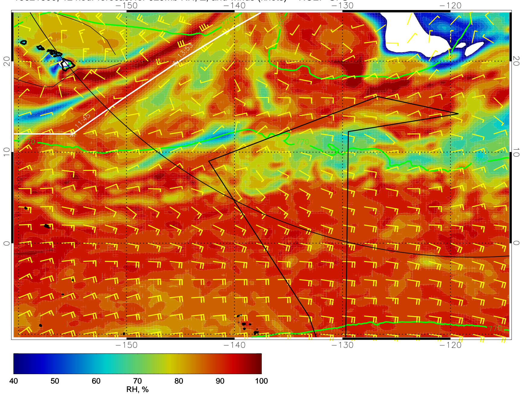
15021600, 12 hour forecast for 925mb RH, Z, and winds (knots) -- NCEP GFS
