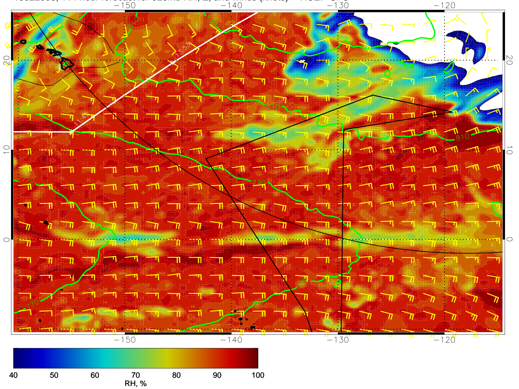
15022006, 114 hour forecast for 925mb RH, Z, and winds (knots) -- NCEP GFS
