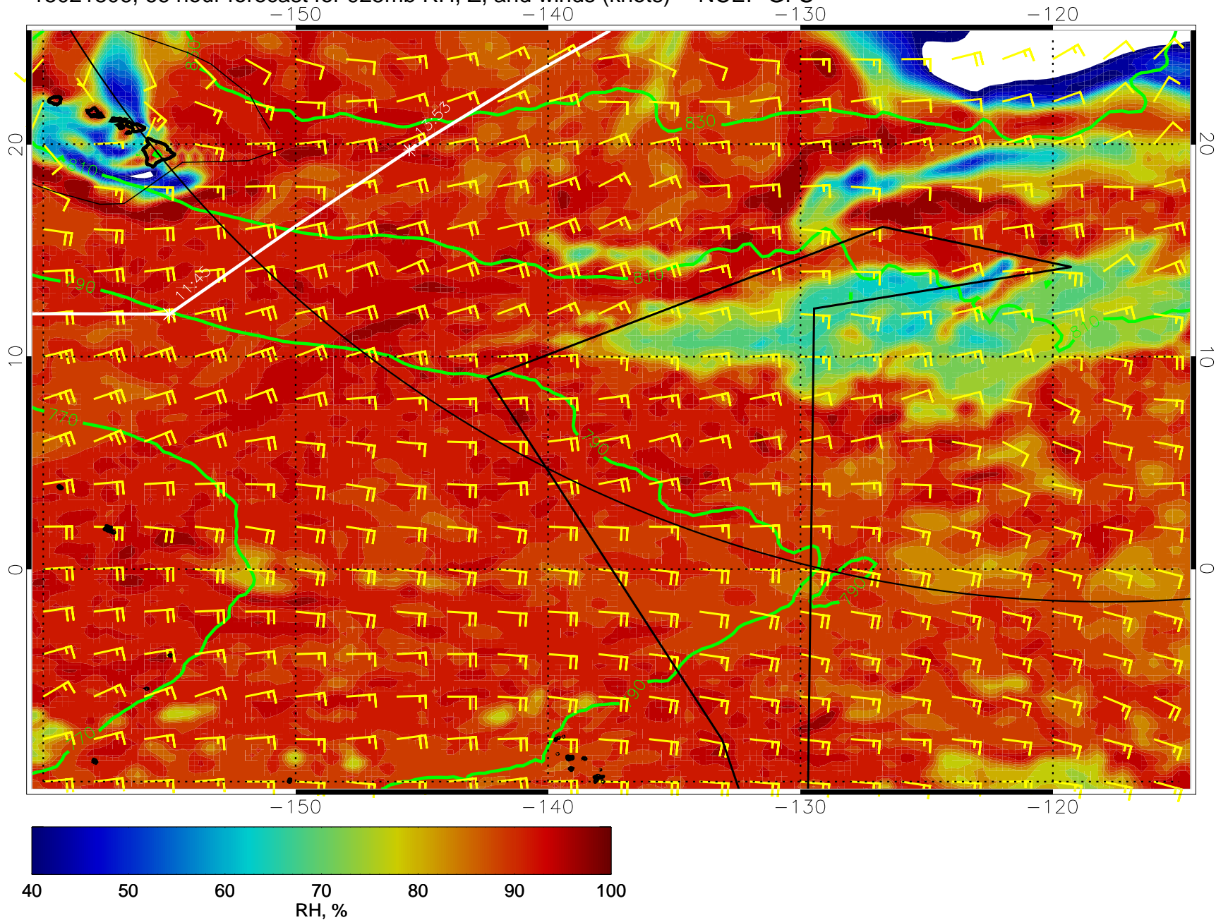
15021806, 66 hour forecast for 925mb RH, Z, and winds (knots) -- NCEP GFS
