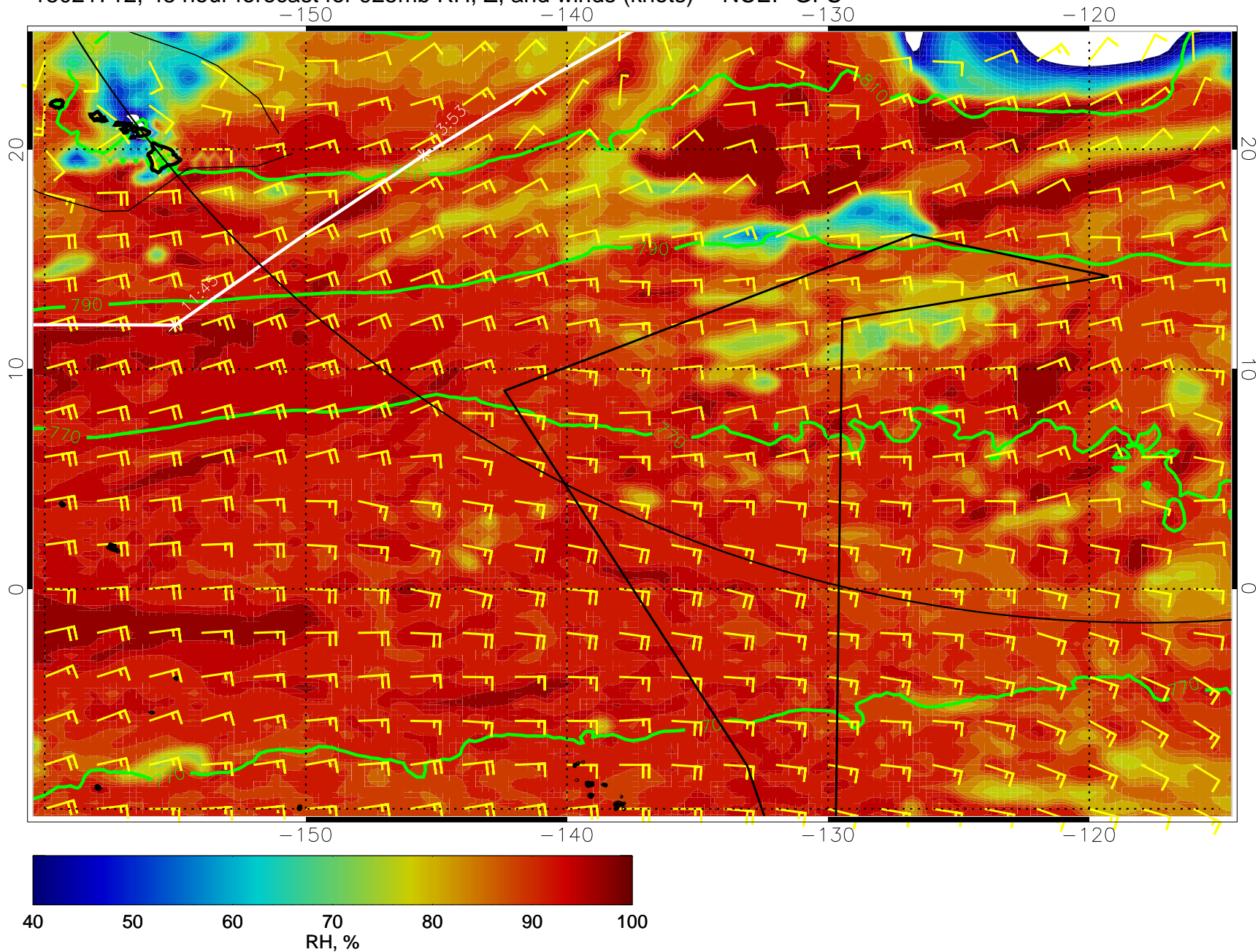
15021712, 48 hour forecast for 925mb RH, Z, and winds (knots) -- NCEP GFS
