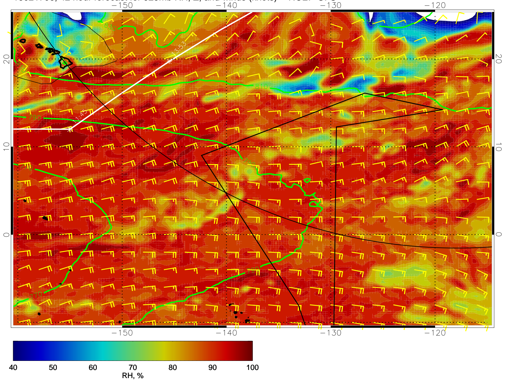
15021706, 42 hour forecast for 925mb RH, Z, and winds (knots) -- NCEP GFS
