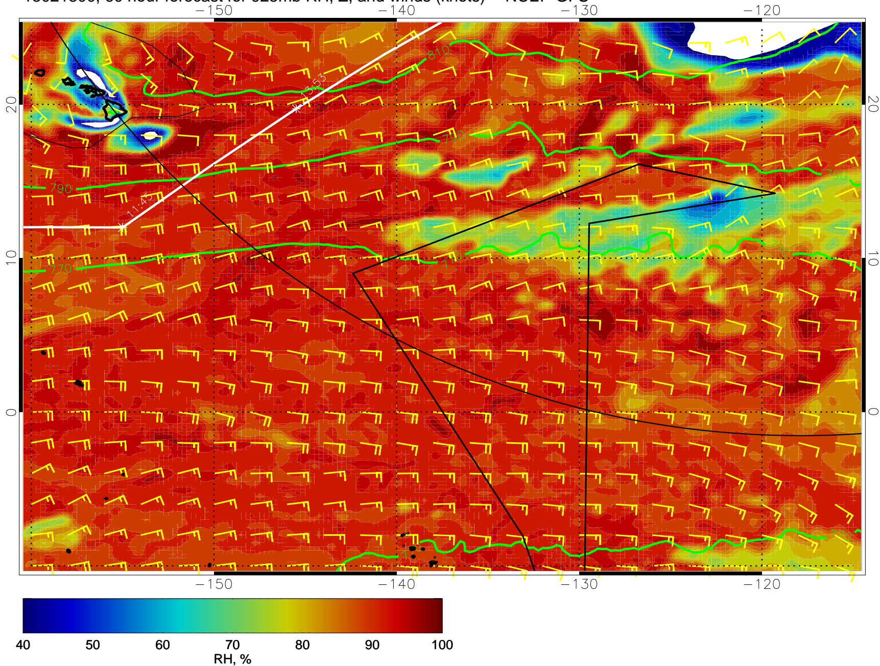
15021800, 60 hour forecast for 925mb RH, Z, and winds (knots) -- NCEP GFS
